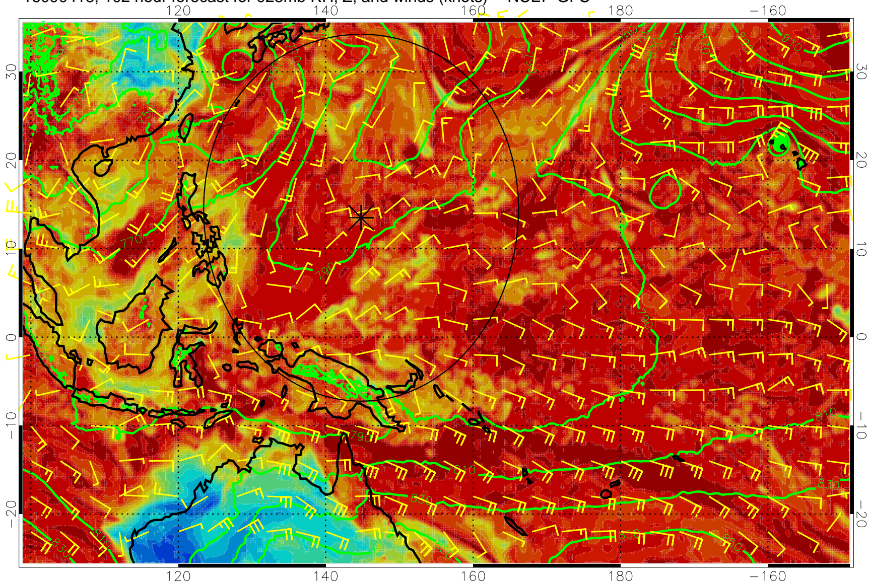
16090418, 102 hour forecast for 925mb RH, Z, and winds (knots) -- NCEP GFS
