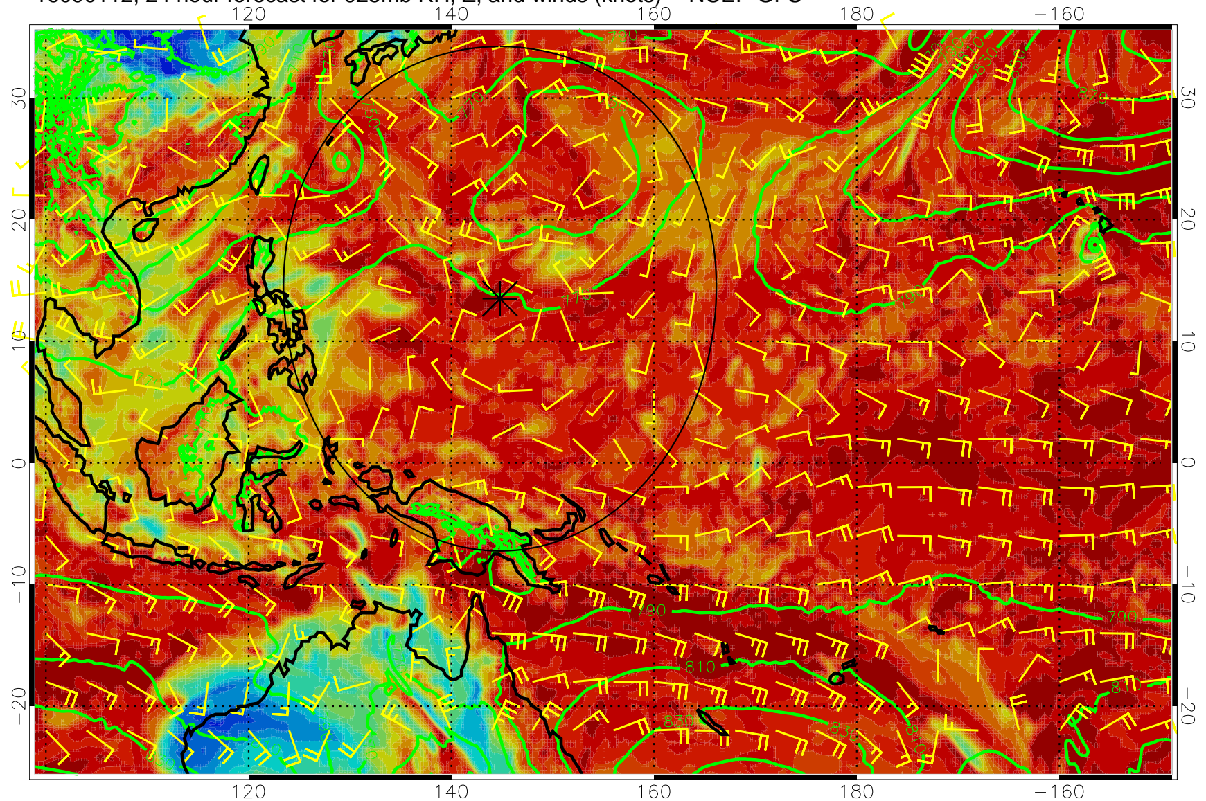
16090112, 24 hour forecast for 925mb RH, Z, and winds (knots) -- NCEP GFS
