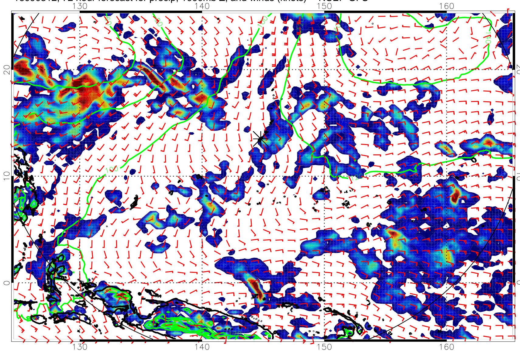
16090312, 72 hour forecast for precip, 1000mb Z, and winds (knots) -- NCEP GFS
