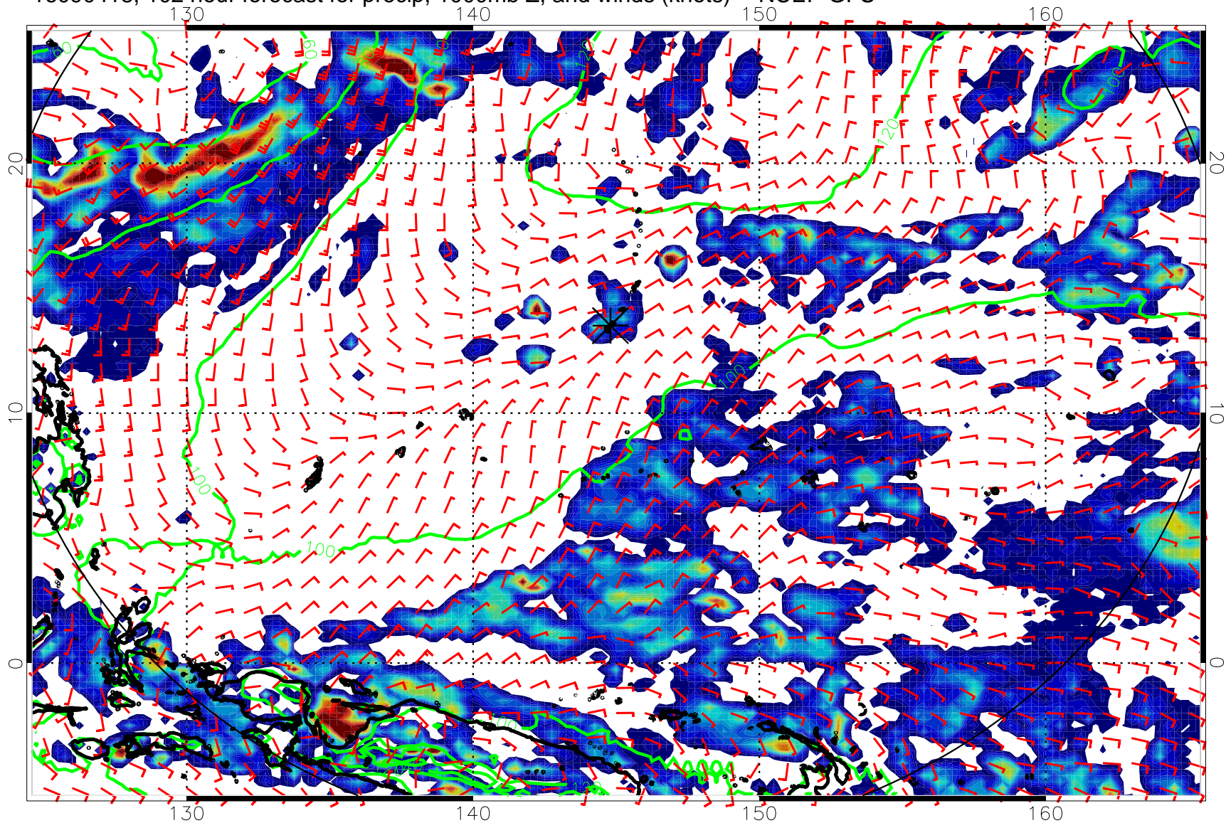
16090418, 102 hour forecast for precip, 1000mb Z, and winds (knots) -- NCEP GFS
