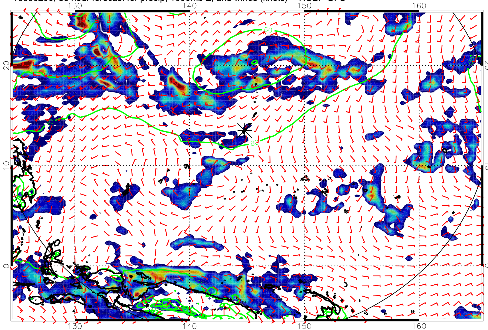
16090200, 36 hour forecast for precip, 1000mb Z, and winds (knots) -- NCEP GFS
