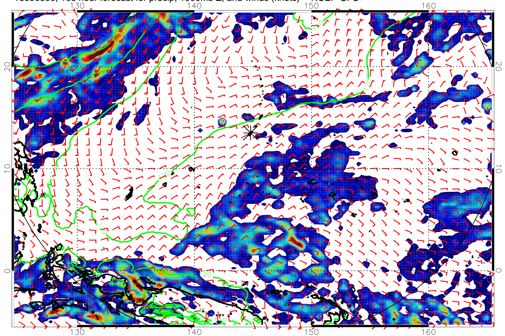
16090500, 108 hour forecast for precip, 1000mb Z, and winds (knots) -- NCEP GFS
