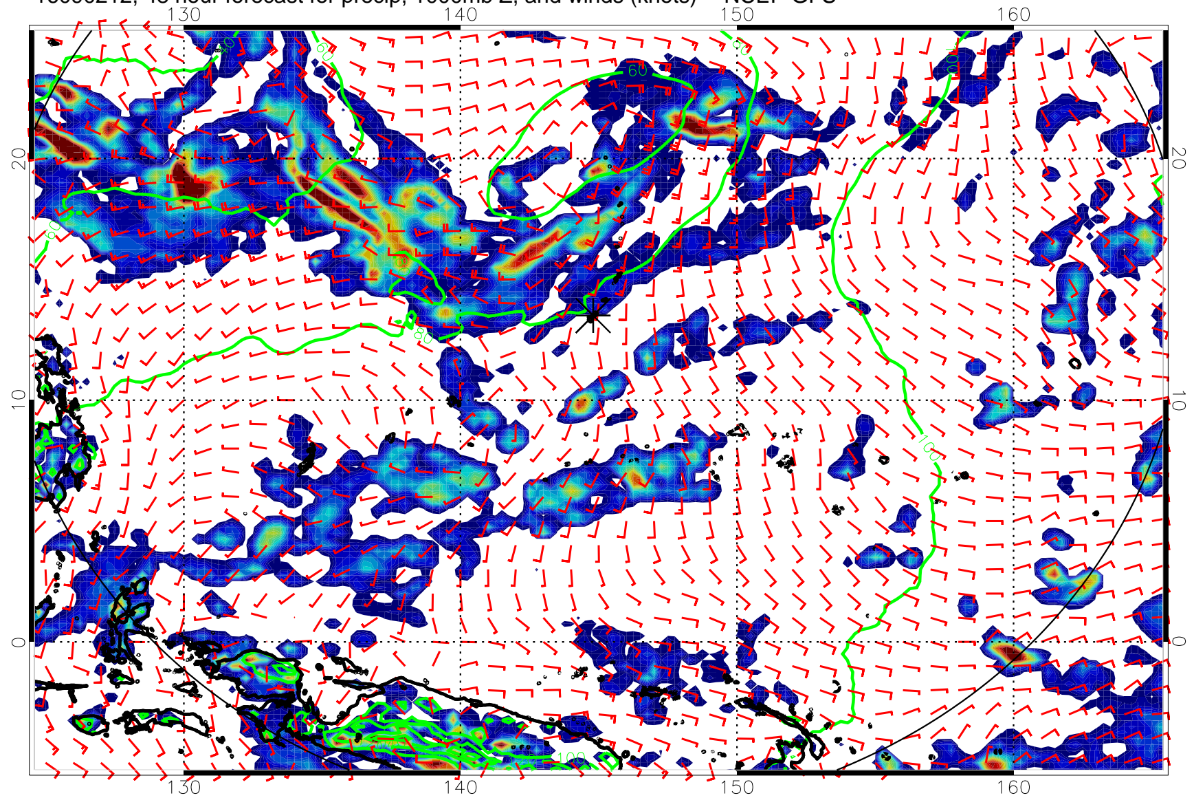
16090212, 48 hour forecast for precip, 1000mb Z, and winds (knots) -- NCEP GFS
