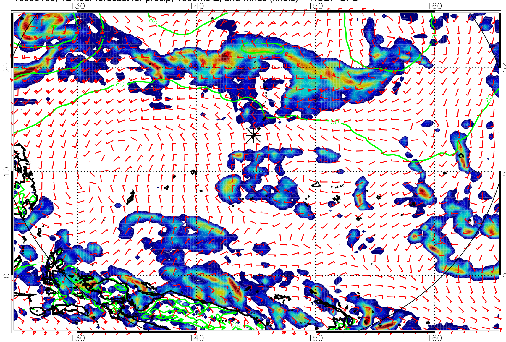
16090100, 12 hour forecast for precip, 1000mb Z, and winds (knots) -- NCEP GFS
