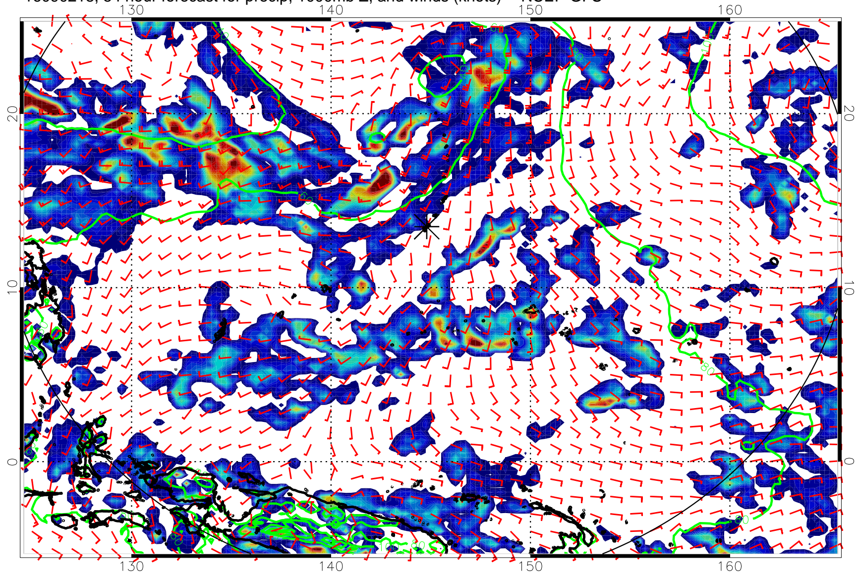
16090218, 54 hour forecast for precip, 1000mb Z, and winds (knots) -- NCEP GFS
