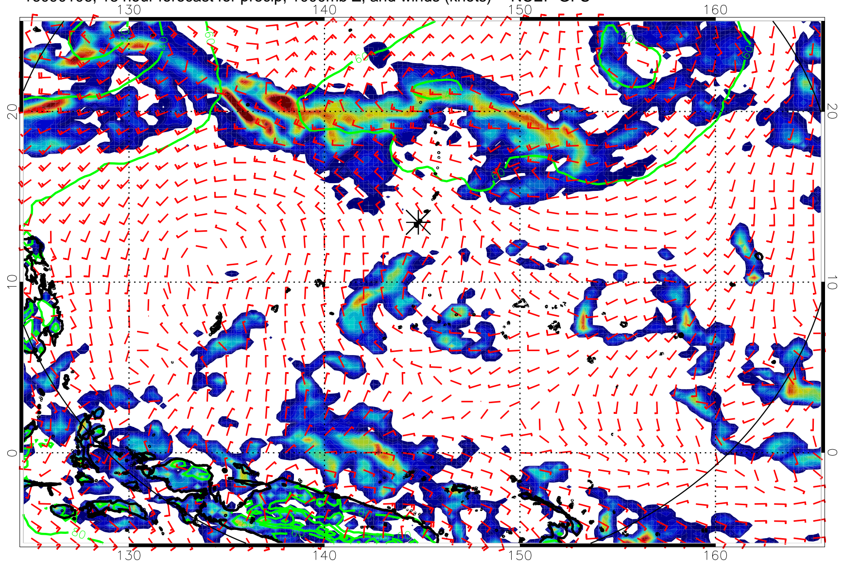
16090106, 18 hour forecast for precip, 1000mb Z, and winds (knots) -- NCEP GFS
