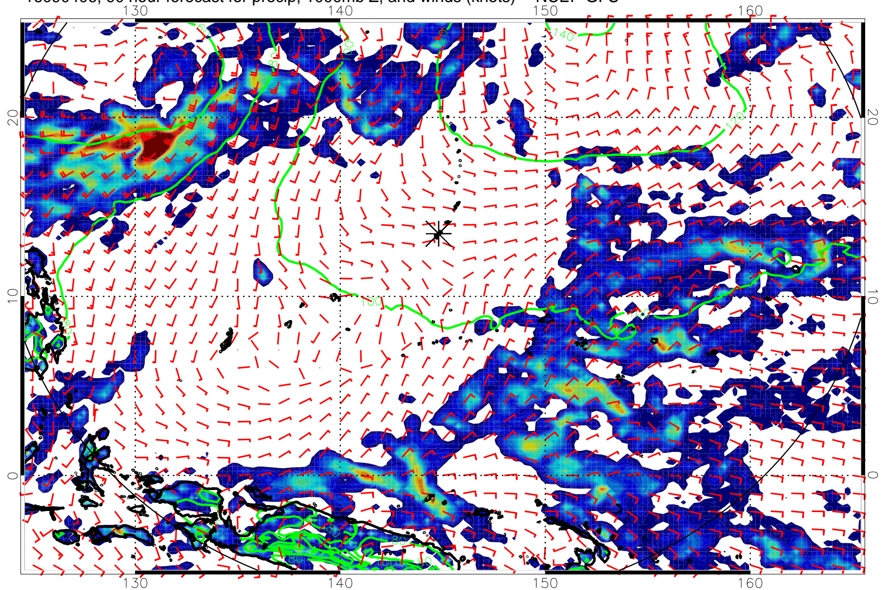
16090406, 90 hour forecast for precip, 1000mb Z, and winds (knots) -- NCEP GFS
