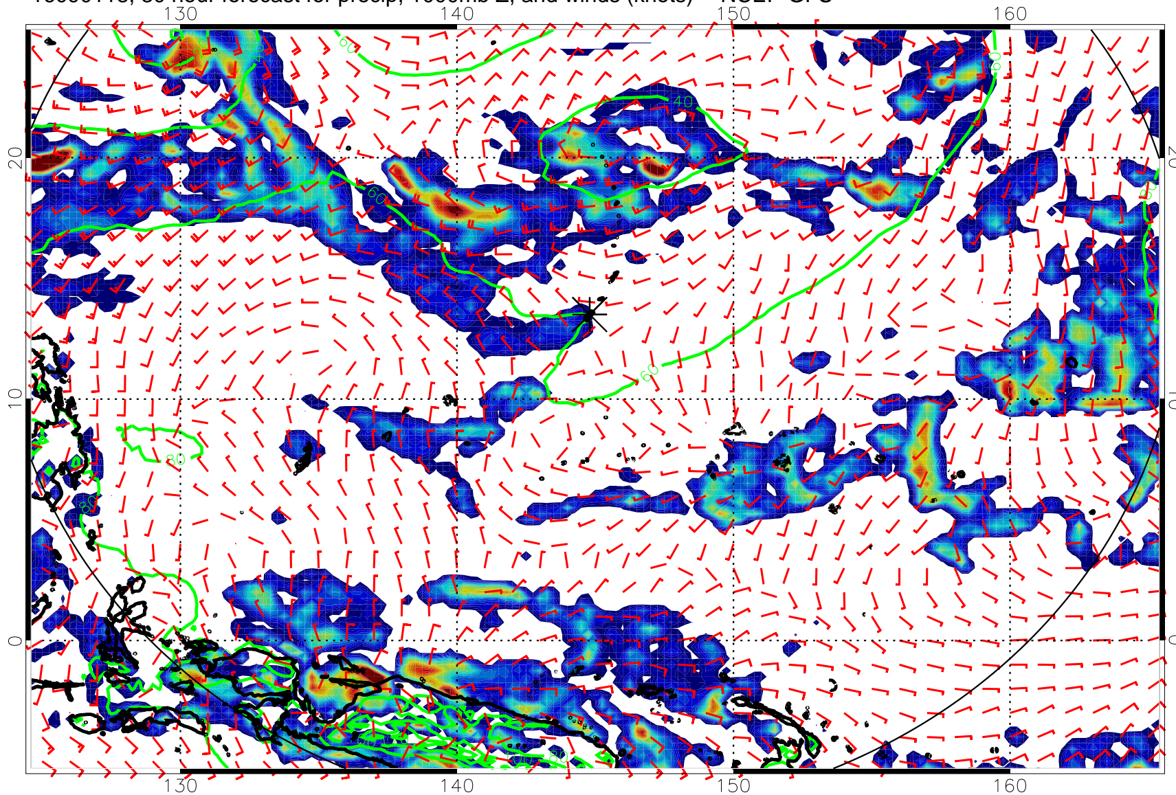
16090118, 30 hour forecast for precip, 1000mb Z, and winds (knots) -- NCEP GFS
