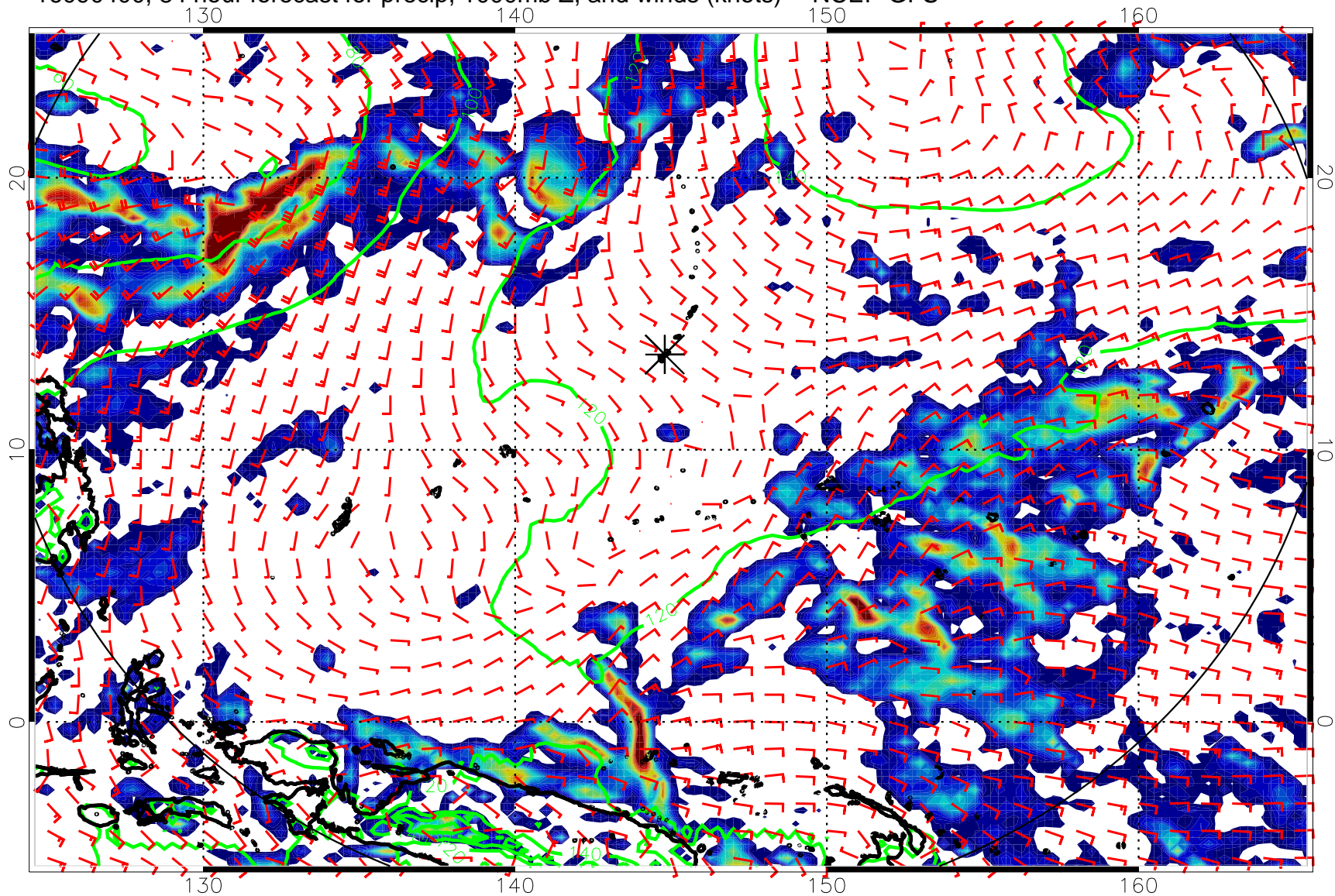
16090400, 84 hour forecast for precip, 1000mb Z, and winds (knots) -- NCEP GFS
