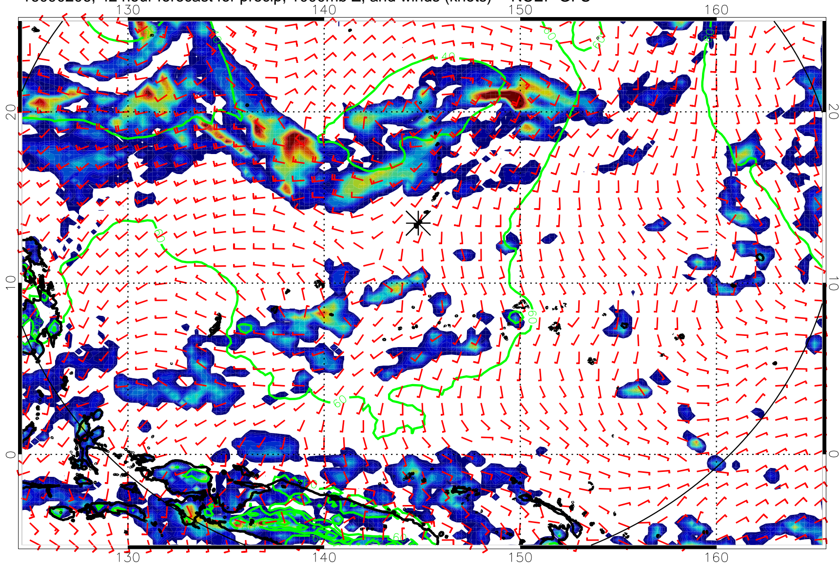
16090206, 42 hour forecast for precip, 1000mb Z, and winds (knots) -- NCEP GFS
