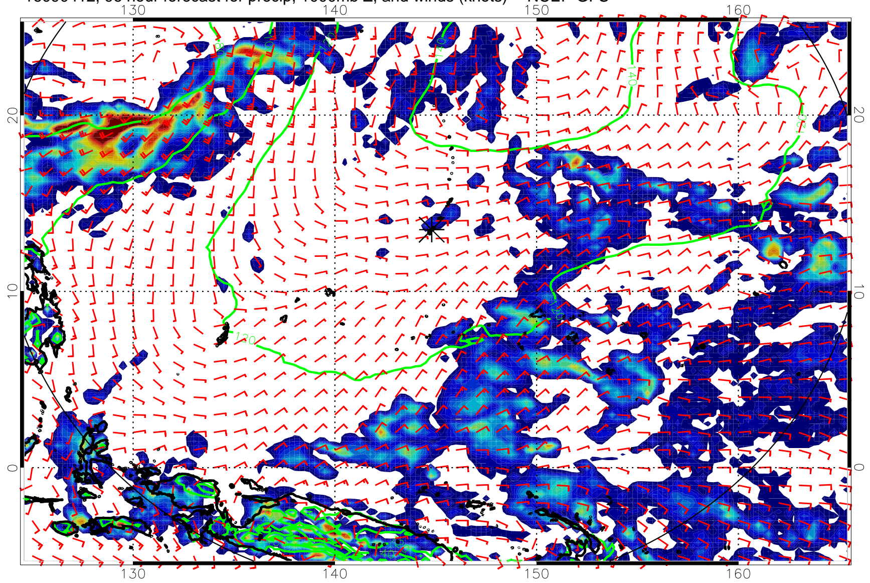
16090412, 96 hour forecast for precip, 1000mb Z, and winds (knots) -- NCEP GFS
