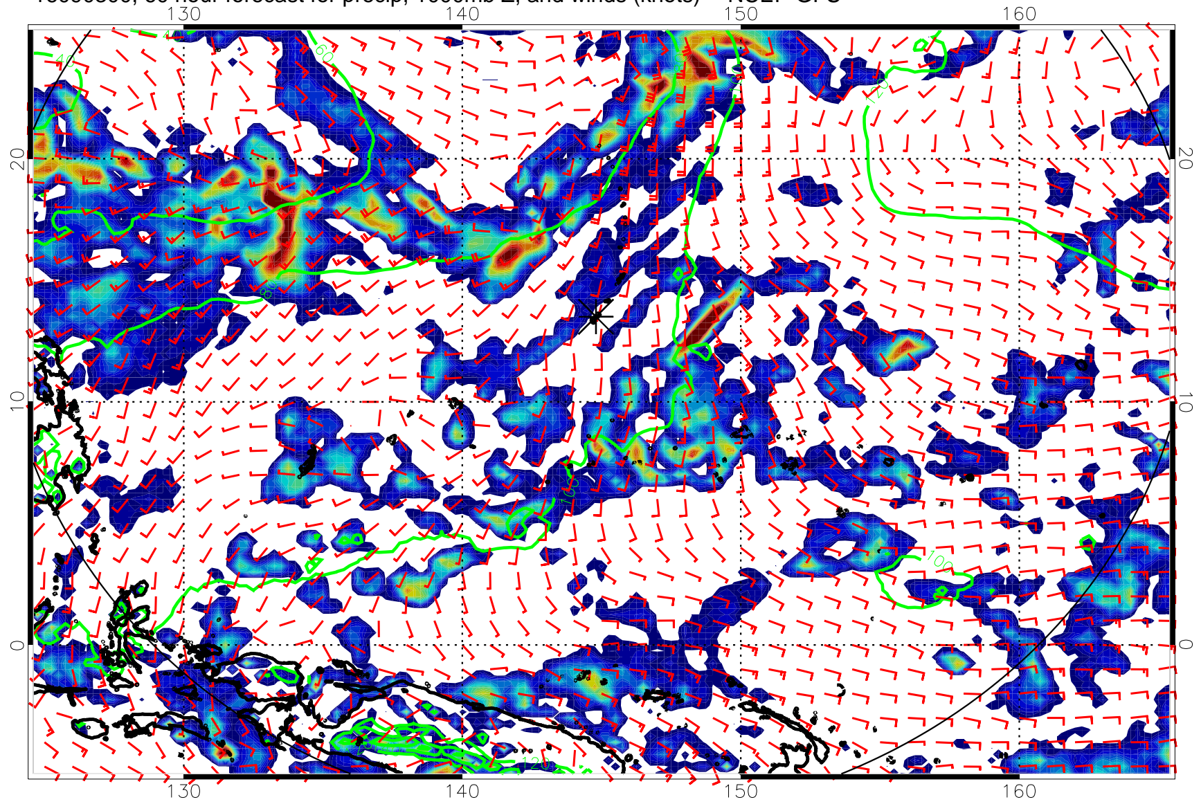
16090300, 60 hour forecast for precip, 1000mb Z, and winds (knots) -- NCEP GFS
