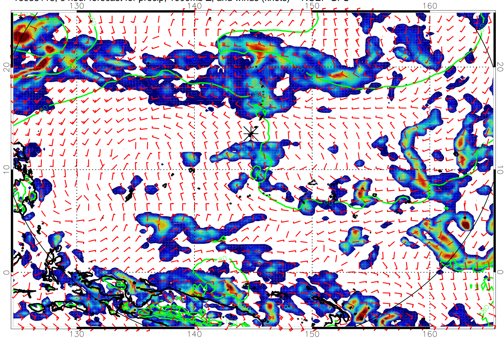
16083118, 6 hour forecast for precip, 1000mb Z, and winds (knots) -- NCEP GFS
