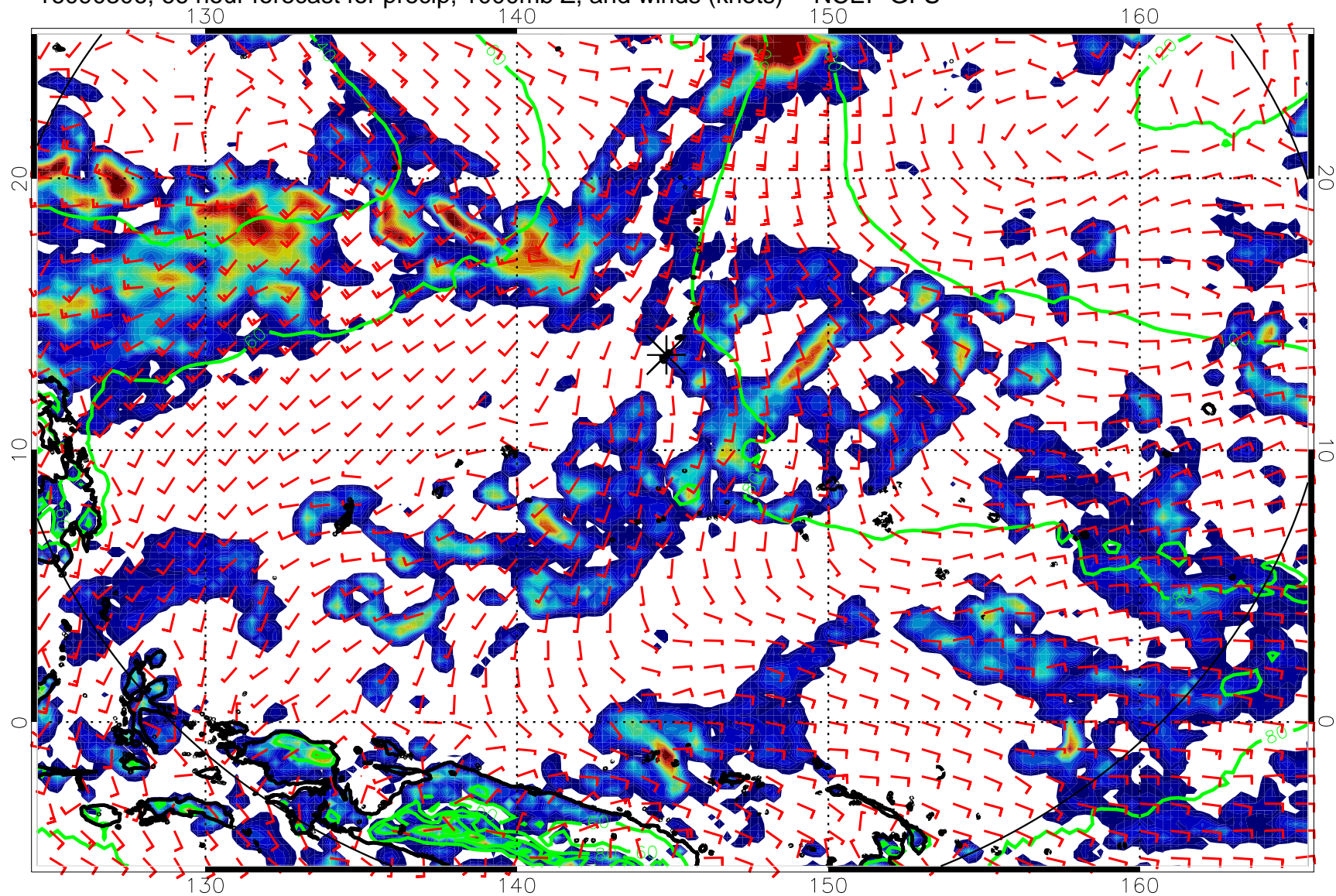
16090306, 66 hour forecast for precip, 1000mb Z, and winds (knots) -- NCEP GFS
