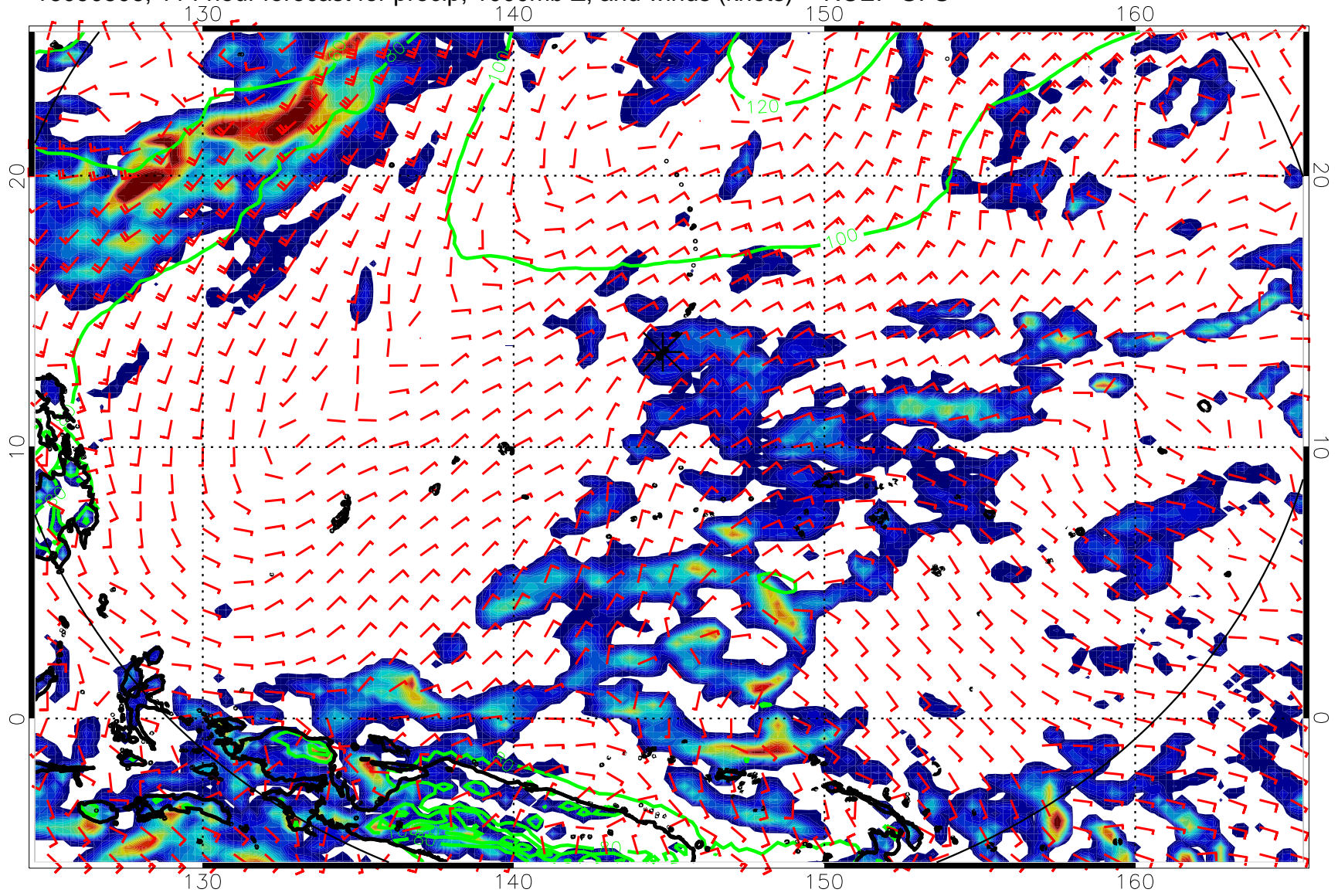
16090506, 114 hour forecast for precip, 1000mb Z, and winds (knots) -- NCEP GFS
