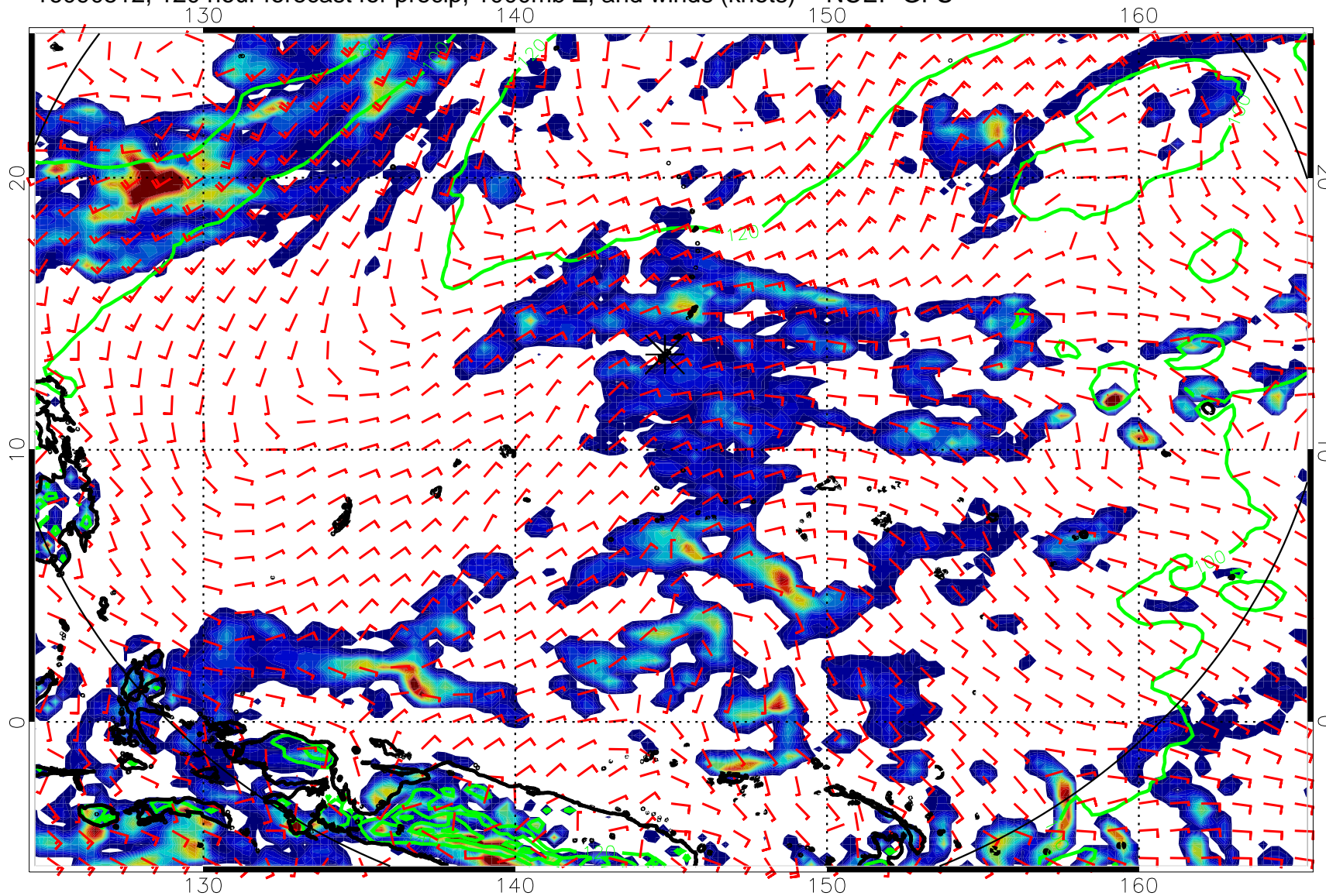
16090512, 120 hour forecast for precip, 1000mb Z, and winds (knots) -- NCEP GFS
