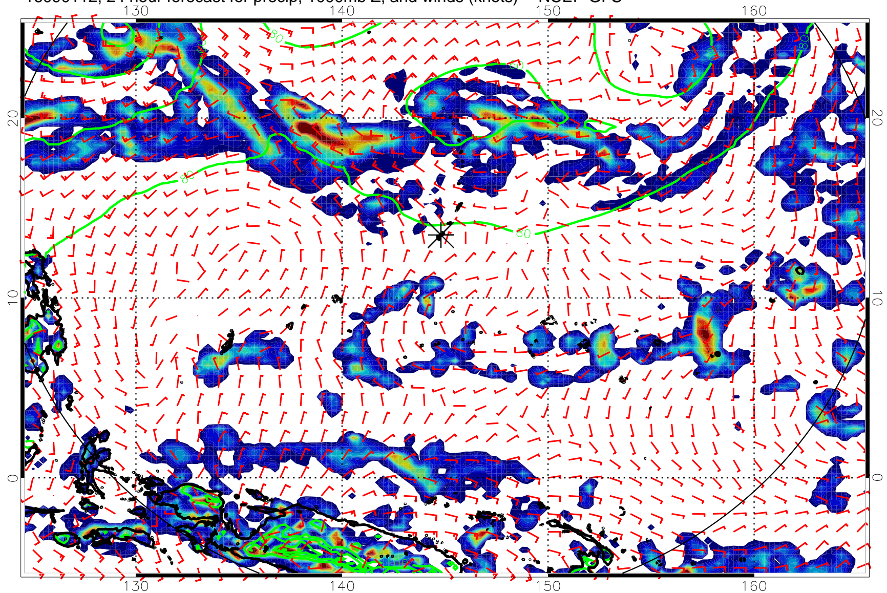
16090112, 24 hour forecast for precip, 1000mb Z, and winds (knots) -- NCEP GFS
