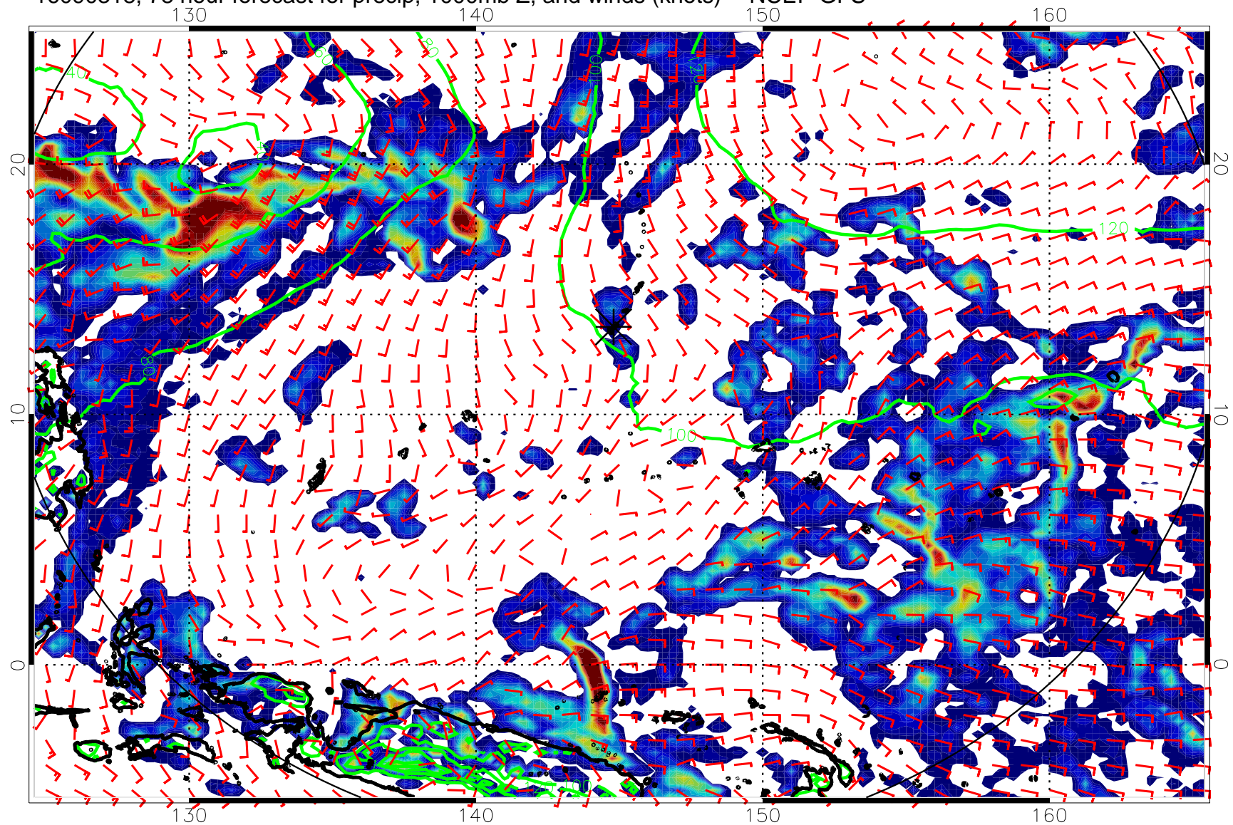
16090318, 78 hour forecast for precip, 1000mb Z, and winds (knots) -- NCEP GFS
