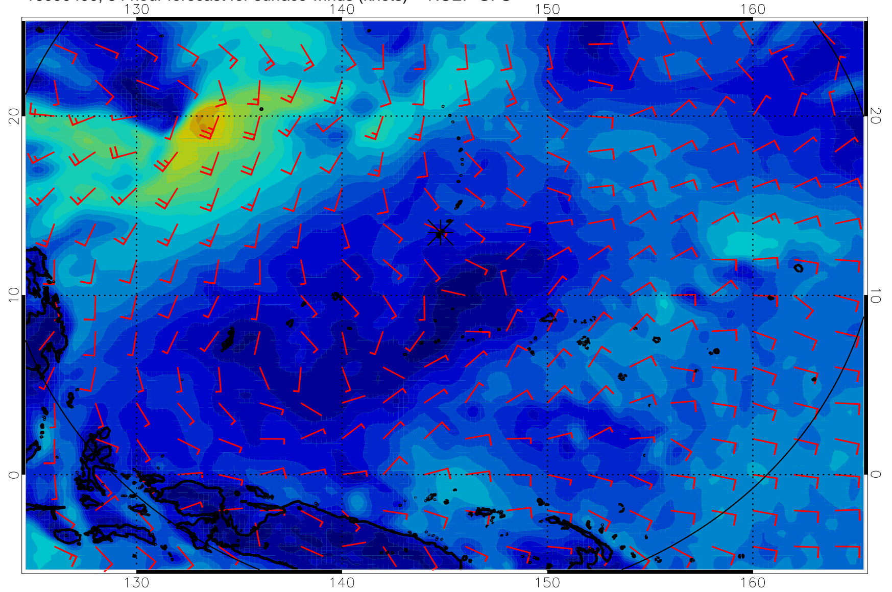
16090400, 84 hour forecast for surface winds (knots) -- NCEP GFS
