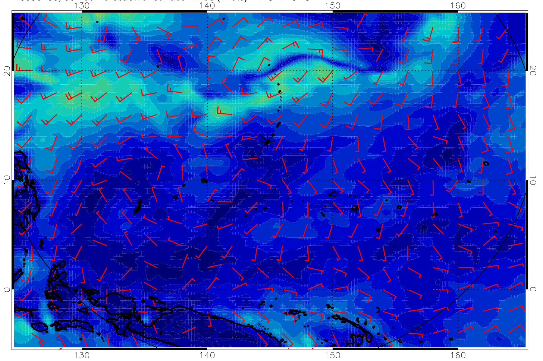
16090200, 36 hour forecast for surface winds (knots) -- NCEP GFS
