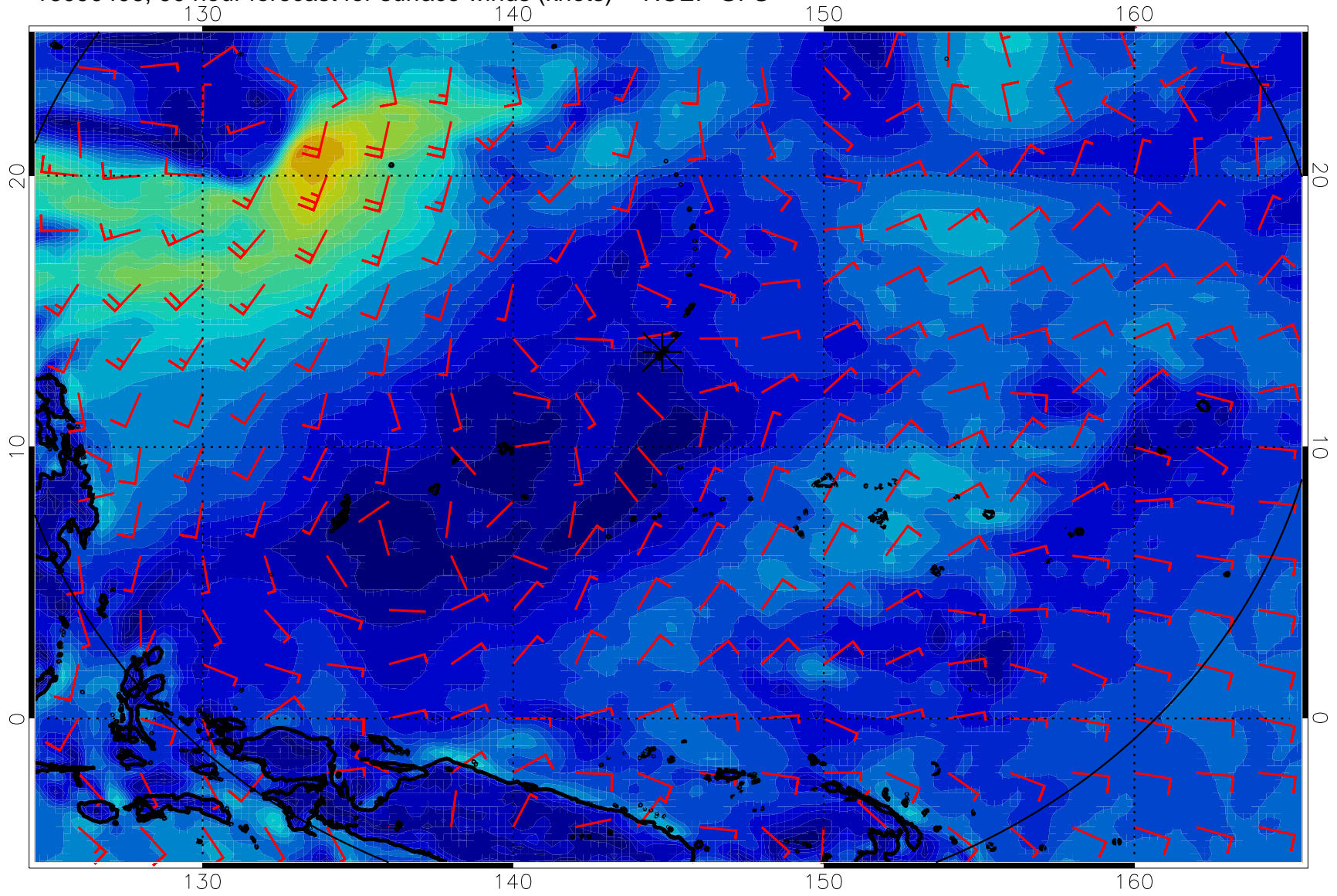
16090406, 90 hour forecast for surface winds (knots) -- NCEP GFS
