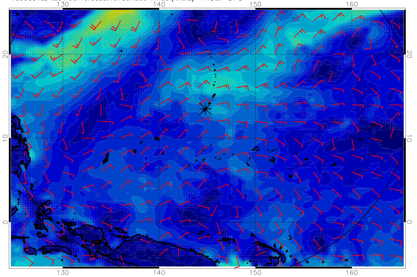
16090512, 120 hour forecast for surface winds (knots) -- NCEP GFS
