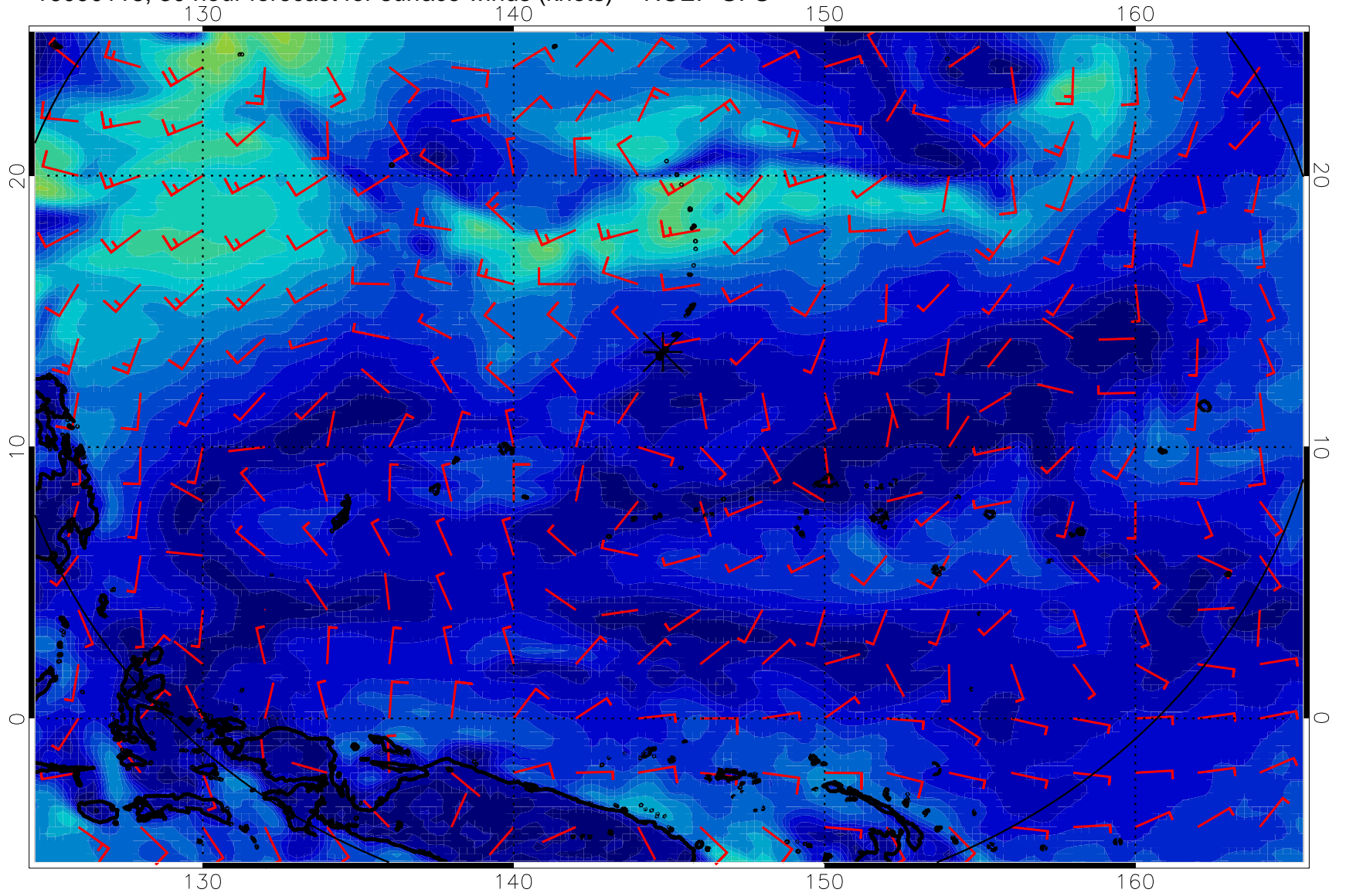
16090118, 30 hour forecast for surface winds (knots) -- NCEP GFS
