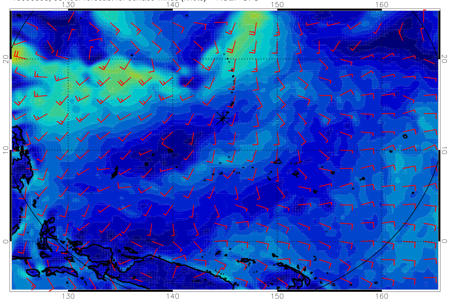
16090306, 66 hour forecast for surface winds (knots) -- NCEP GFS
