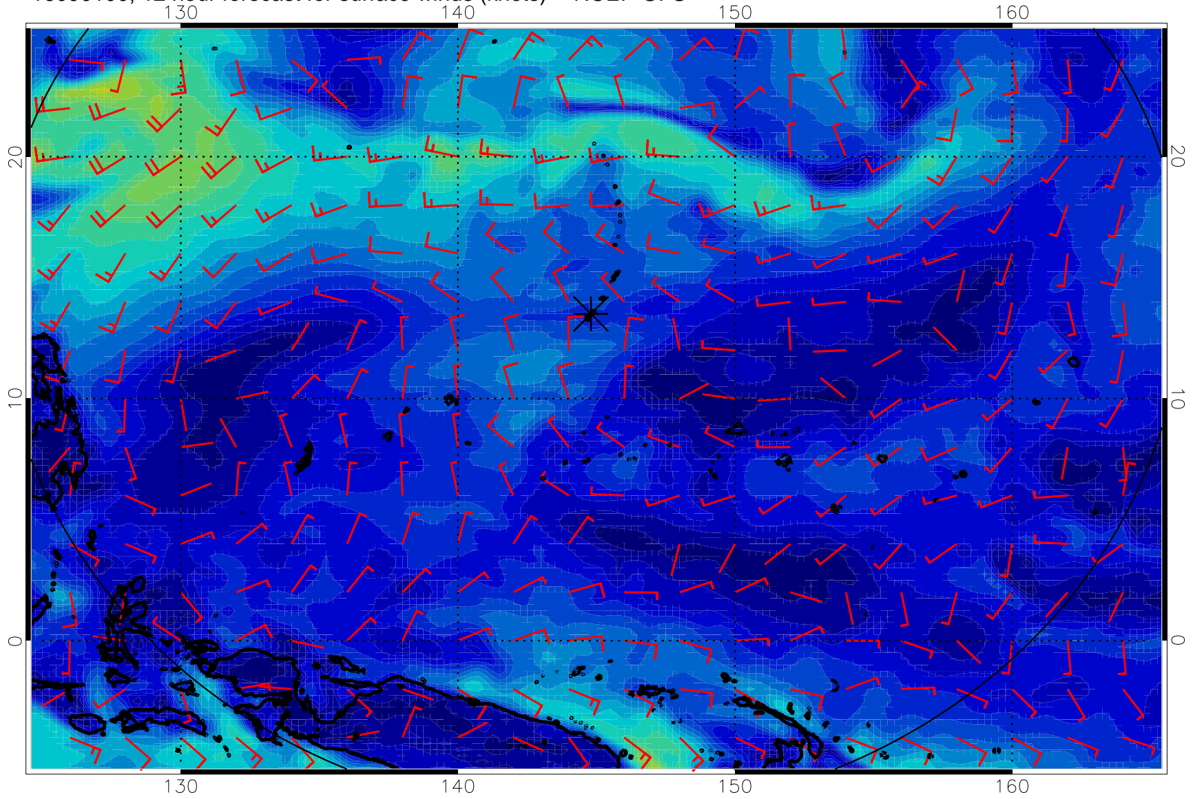
16090100, 12 hour forecast for surface winds (knots) -- NCEP GFS
