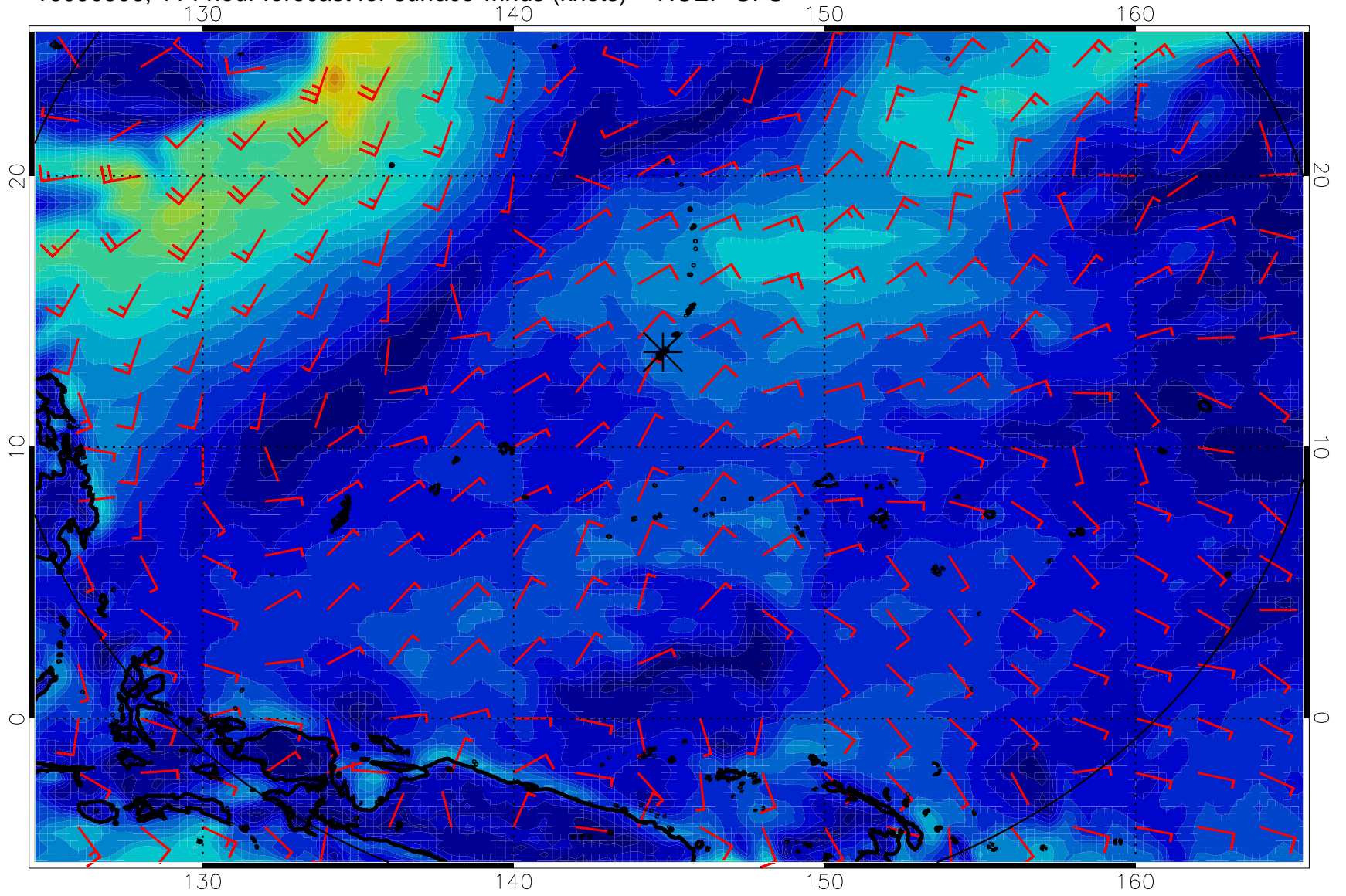
16090506, 114 hour forecast for surface winds (knots) -- NCEP GFS
