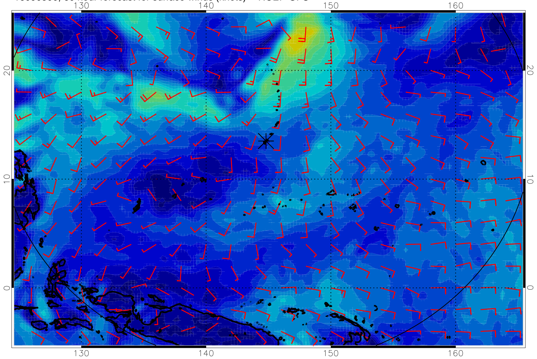
16090300, 60 hour forecast for surface winds (knots) -- NCEP GFS
