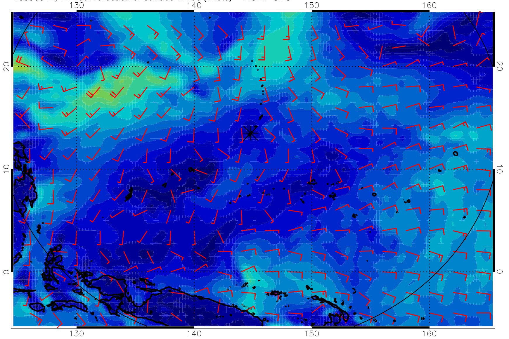
16090312, 72 hour forecast for surface winds (knots) -- NCEP GFS
