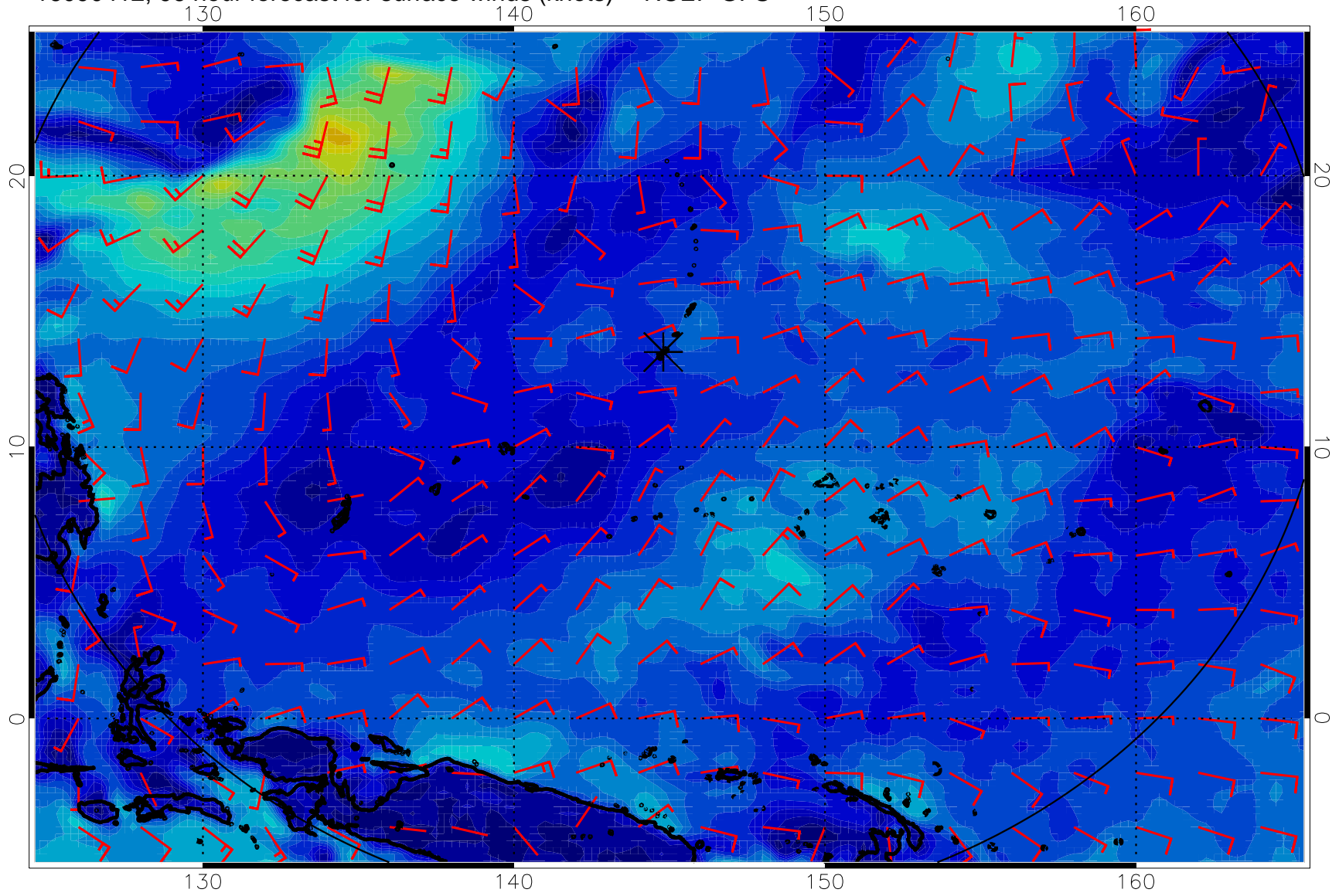
16090412, 96 hour forecast for surface winds (knots) -- NCEP GFS
