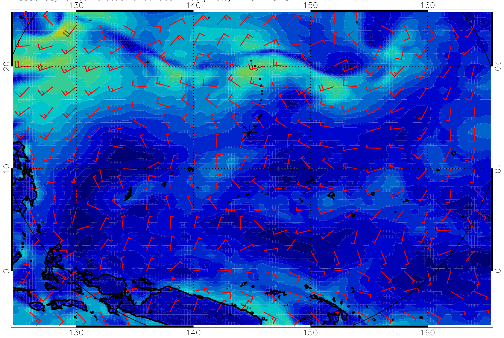
16090106, 18 hour forecast for surface winds (knots) -- NCEP GFS
