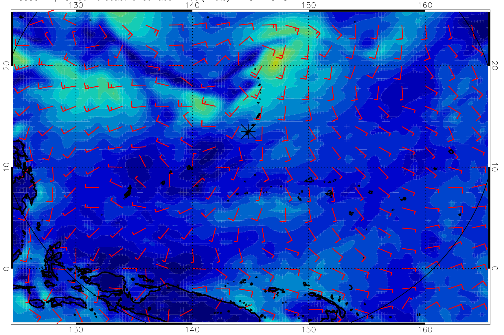
16090212, 48 hour forecast for surface winds (knots) -- NCEP GFS
