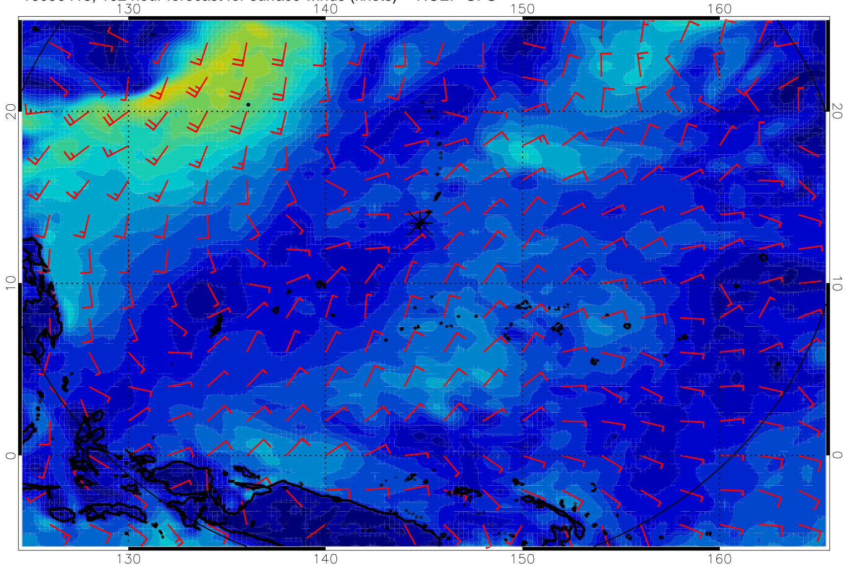
16090418, 102 hour forecast for surface winds (knots) -- NCEP GFS
