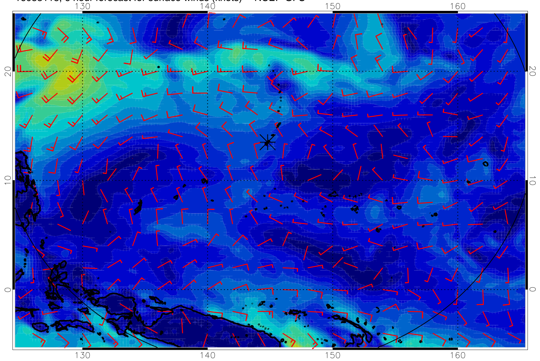
16083118, 6 hour forecast for surface winds (knots) -- NCEP GFS
