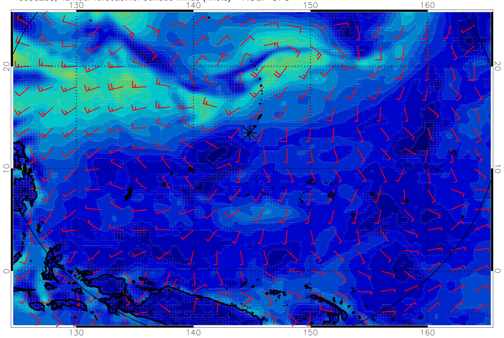
16090206, 42 hour forecast for surface winds (knots) -- NCEP GFS
