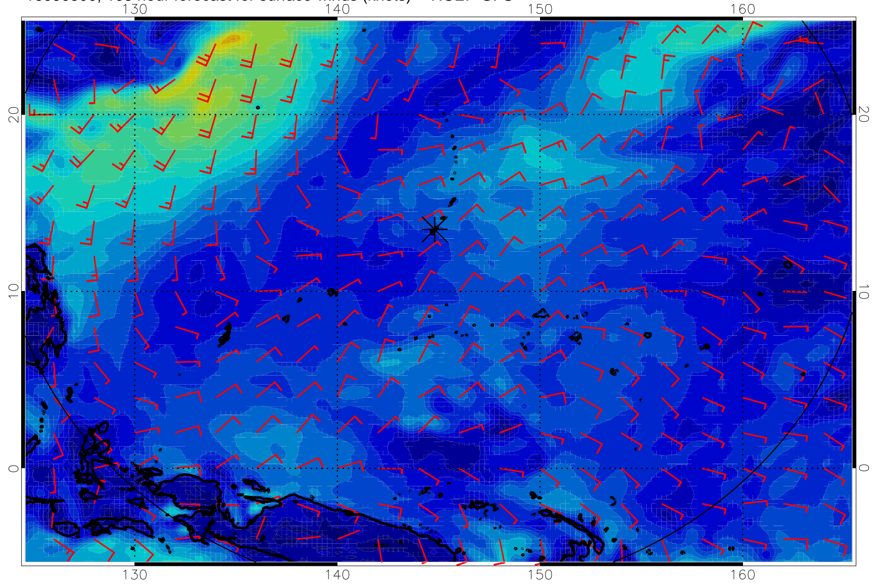
16090500, 108 hour forecast for surface winds (knots) -- NCEP GFS
