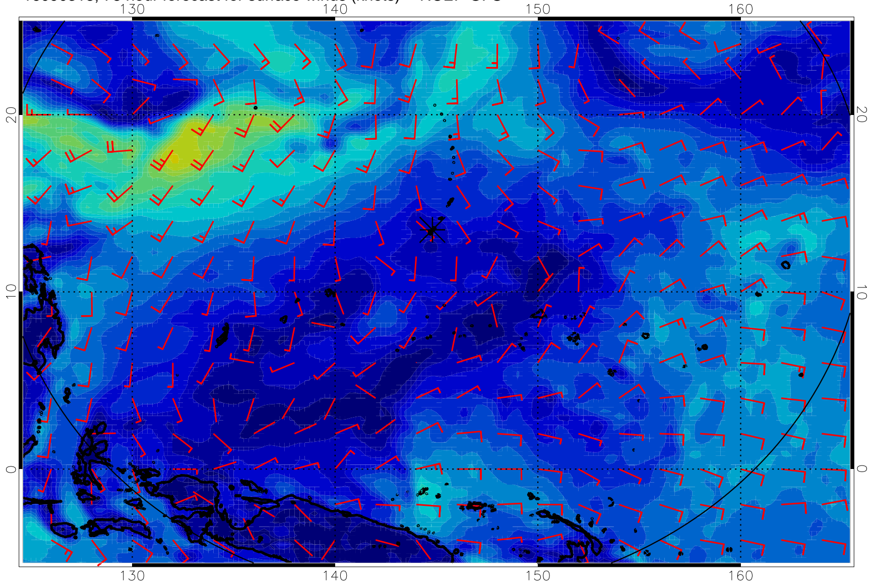
16090318, 78 hour forecast for surface winds (knots) -- NCEP GFS
