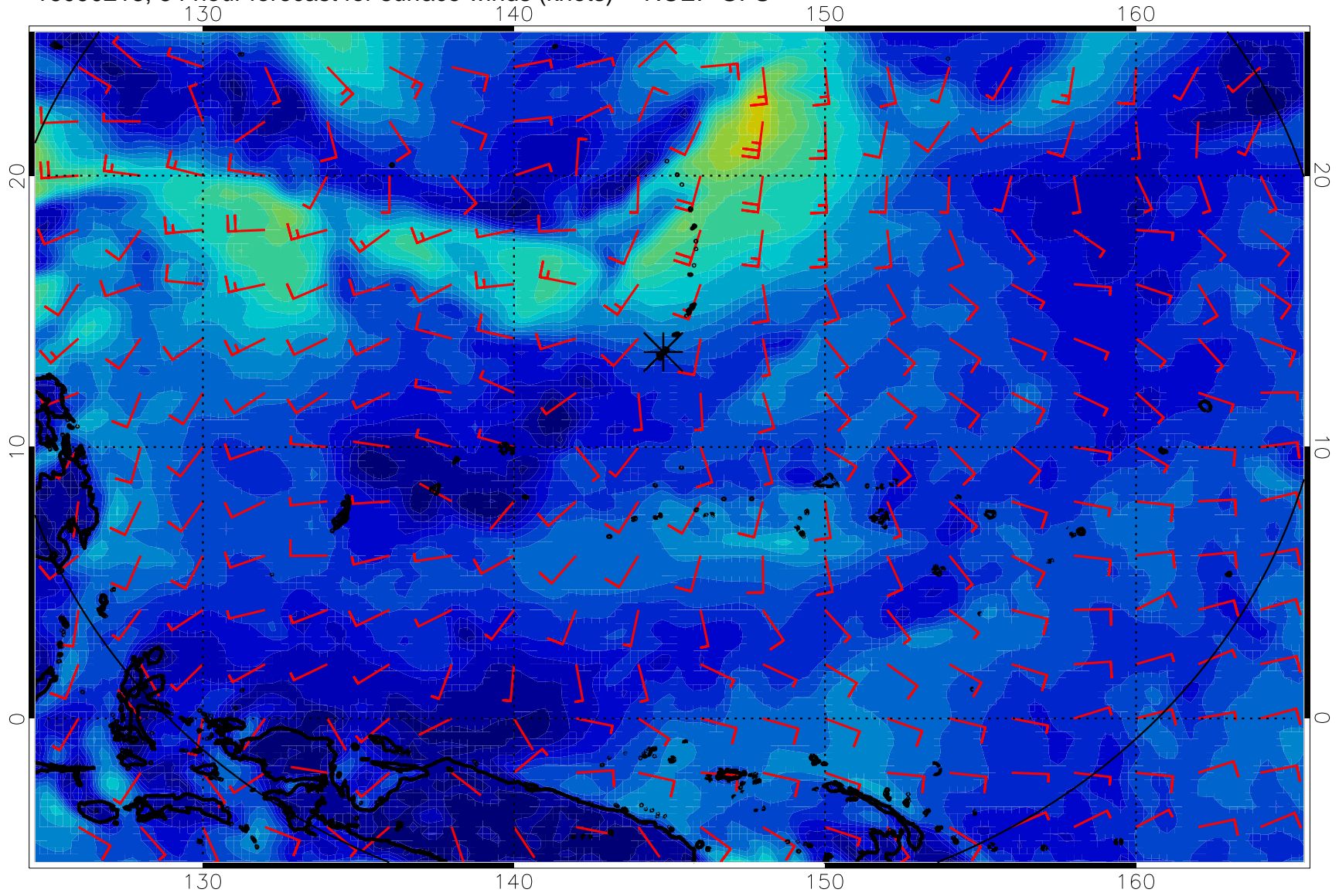
16090218, 54 hour forecast for surface winds (knots) -- NCEP GFS
