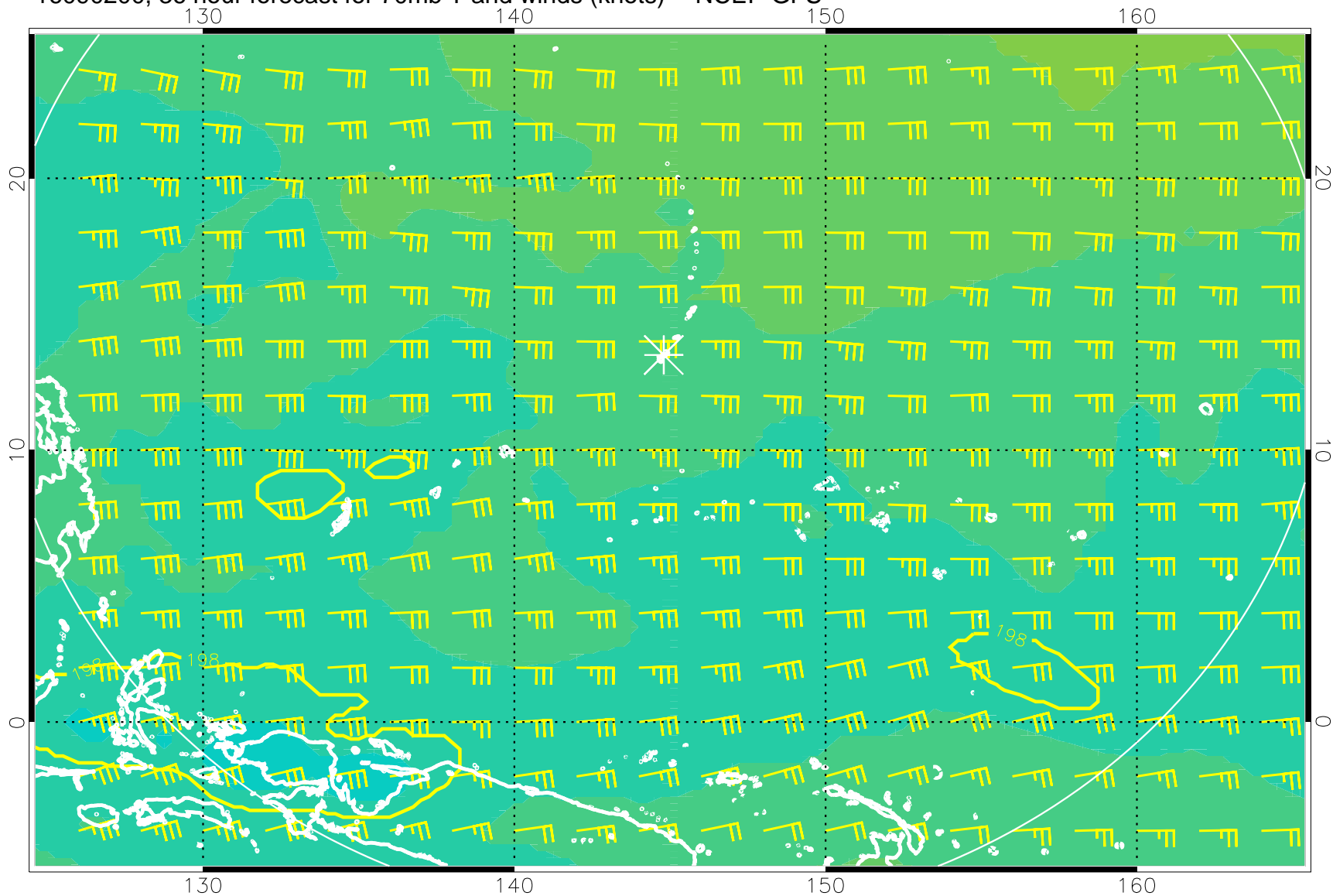
16090200, 36 hour forecast for 70mb T and winds (knots) -- NCEP GFS
