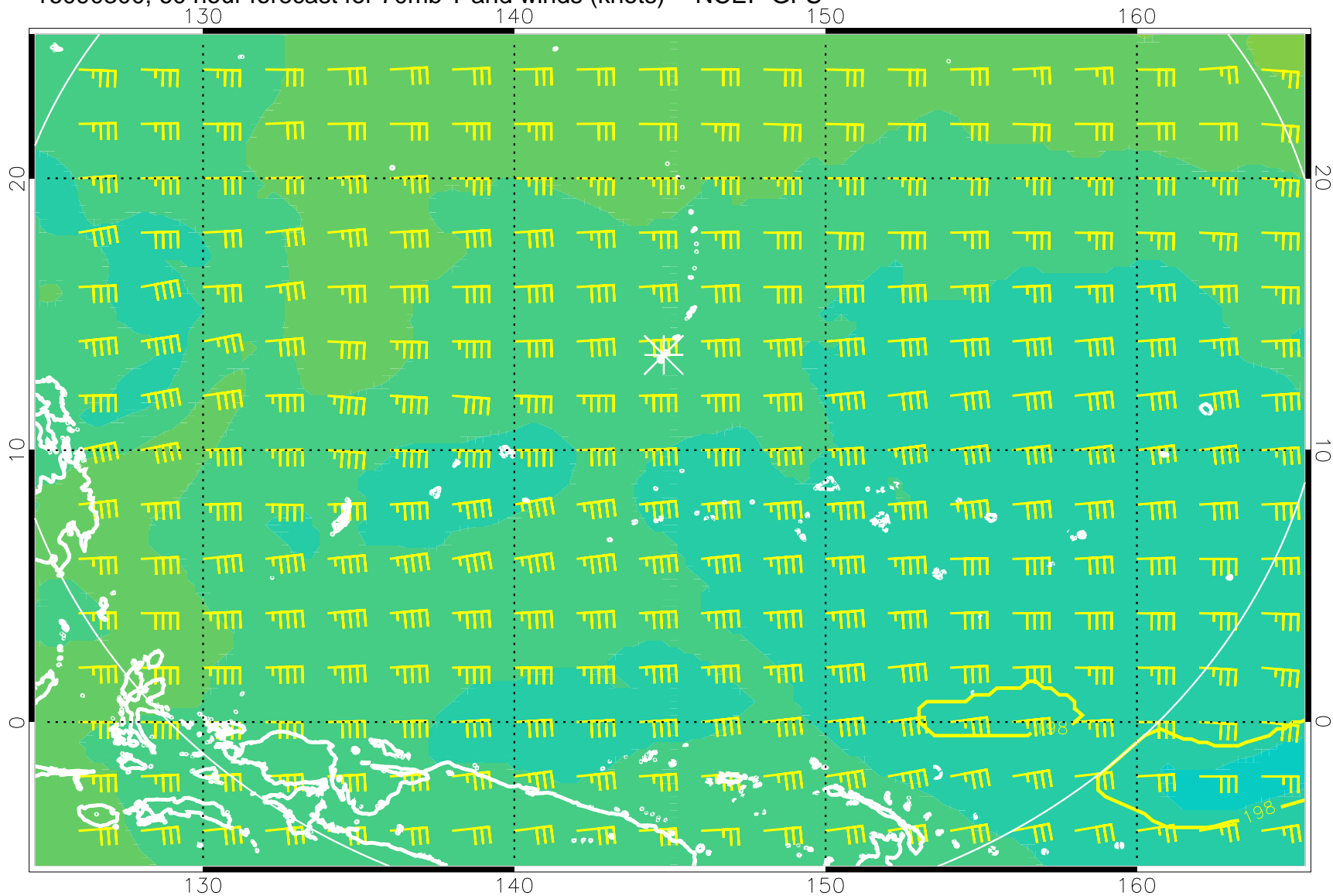
16090300, 60 hour forecast for 70mb T and winds (knots) -- NCEP GFS
