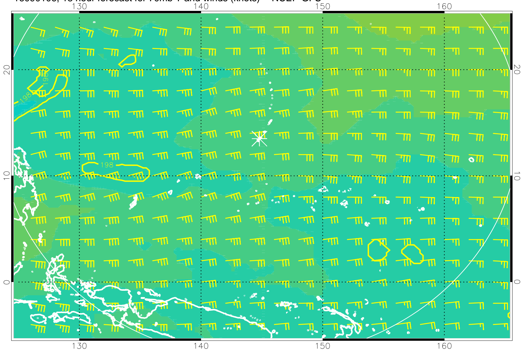
16090106, 18 hour forecast for 70mb T and winds (knots) -- NCEP GFS
