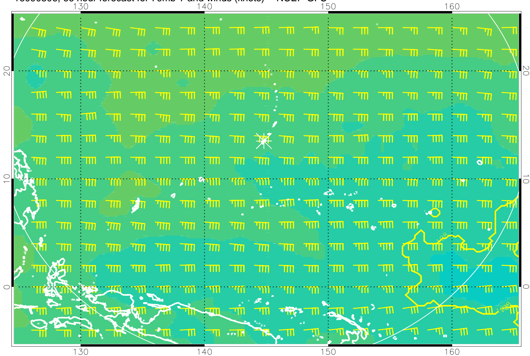
16090306, 66 hour forecast for 70mb T and winds (knots) -- NCEP GFS
