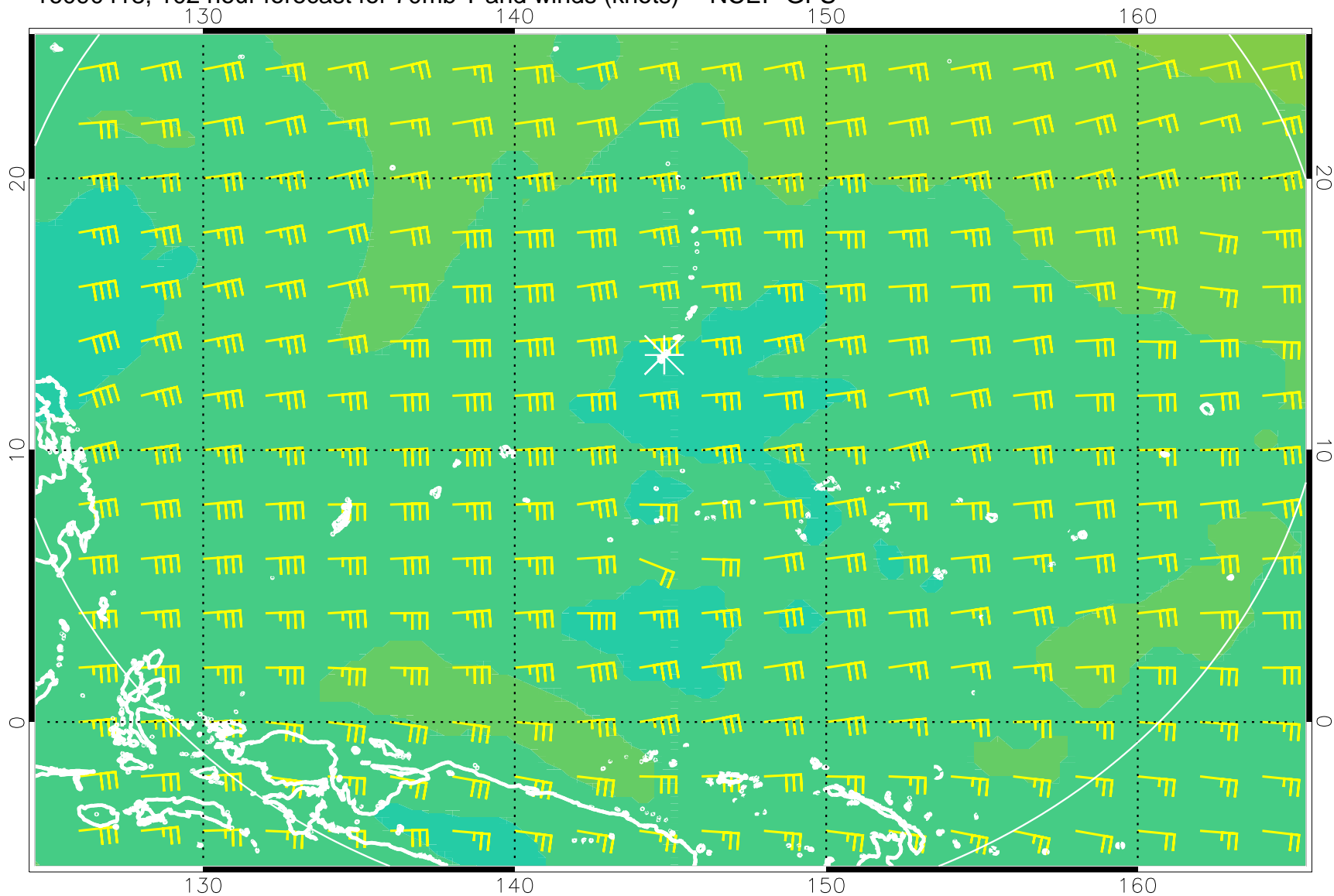
16090418, 102 hour forecast for 70mb T and winds (knots) -- NCEP GFS
