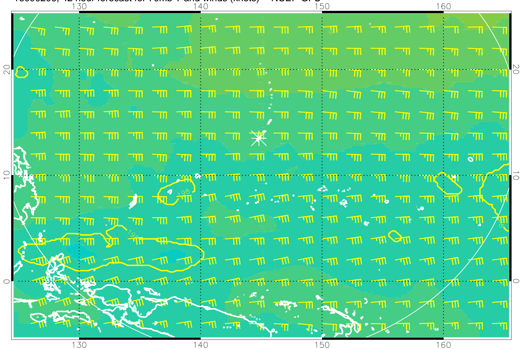
16090206, 42 hour forecast for 70mb T and winds (knots) -- NCEP GFS
