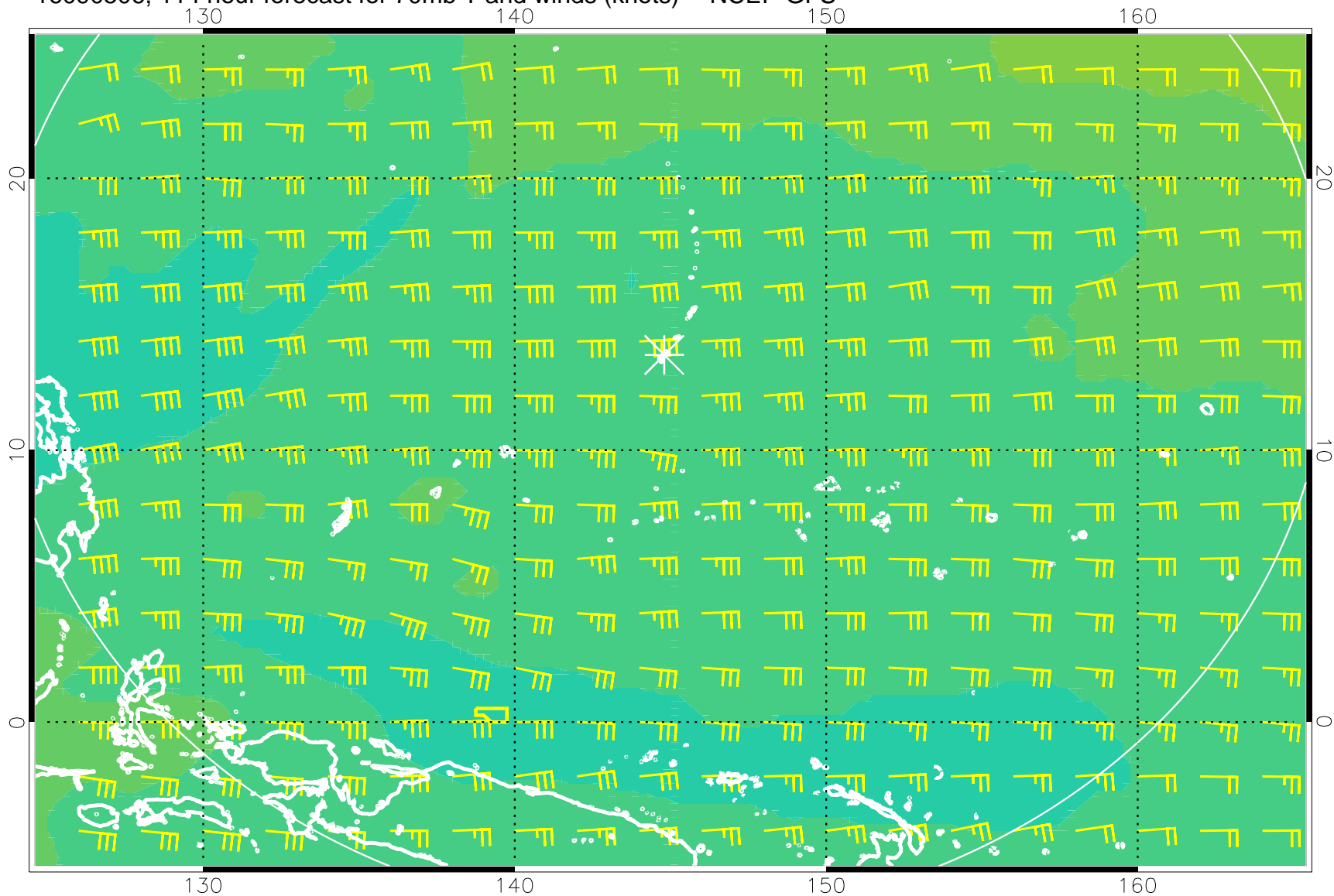
16090506, 114 hour forecast for 70mb T and winds (knots) -- NCEP GFS
