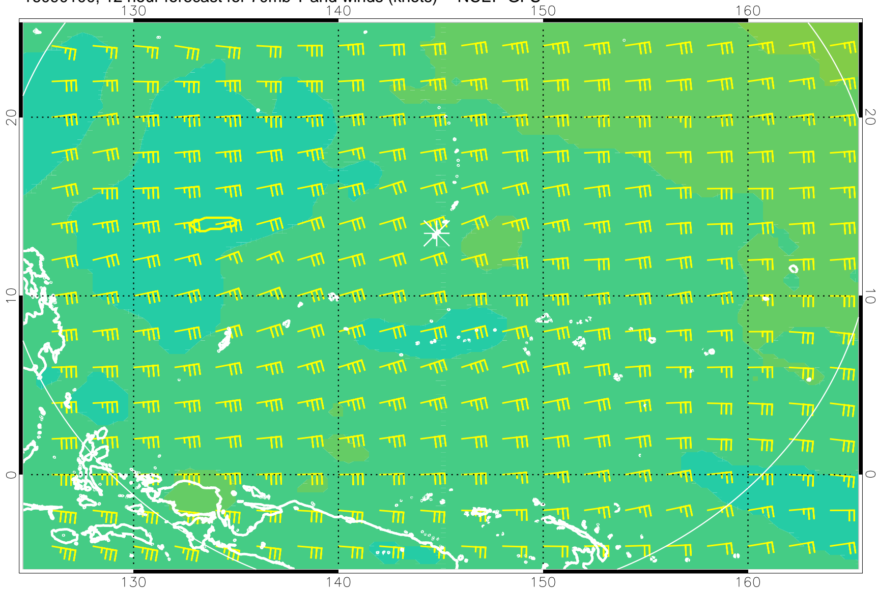
16090100, 12 hour forecast for 70mb T and winds (knots) -- NCEP GFS
