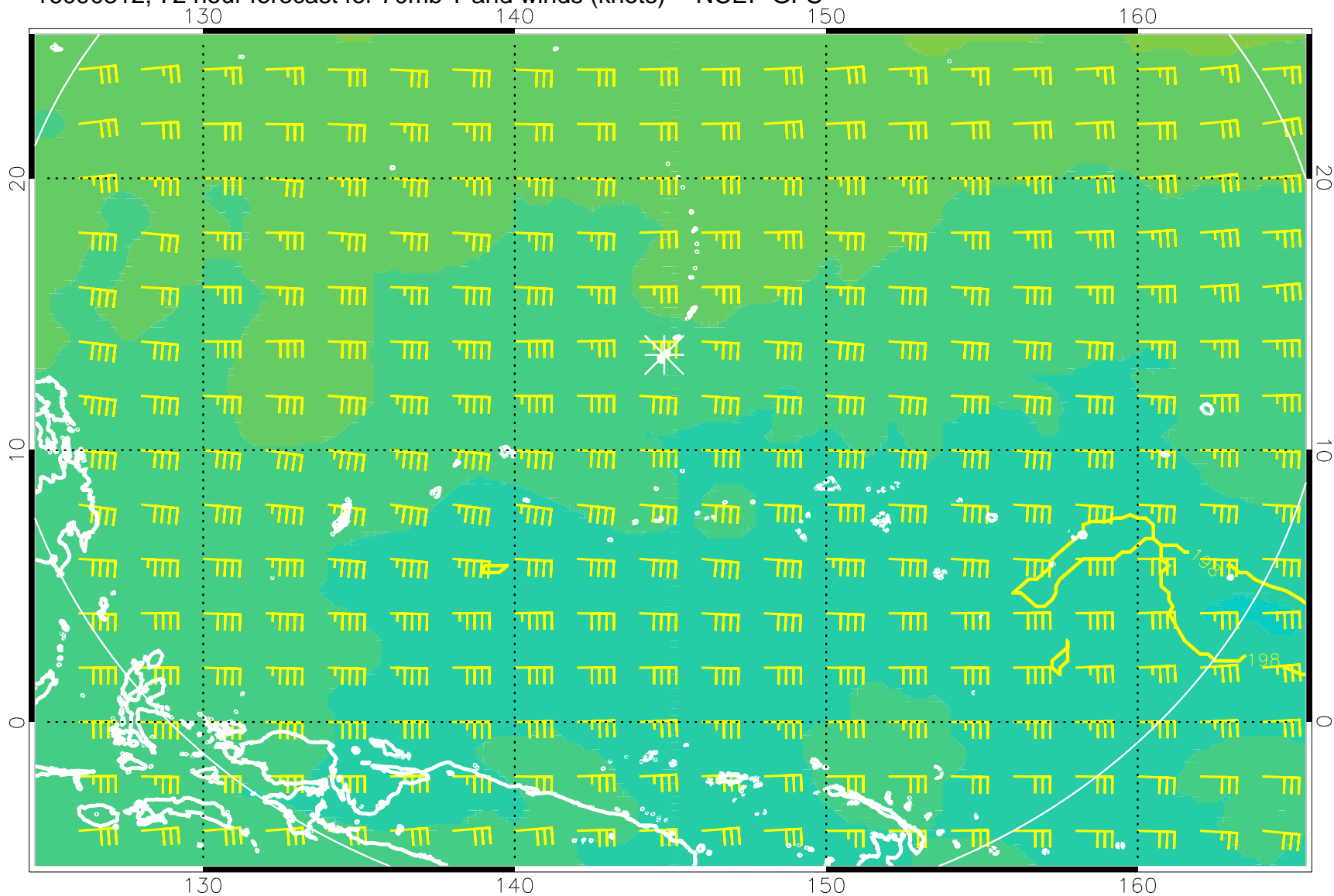
16090312, 72 hour forecast for 70mb T and winds (knots) -- NCEP GFS
