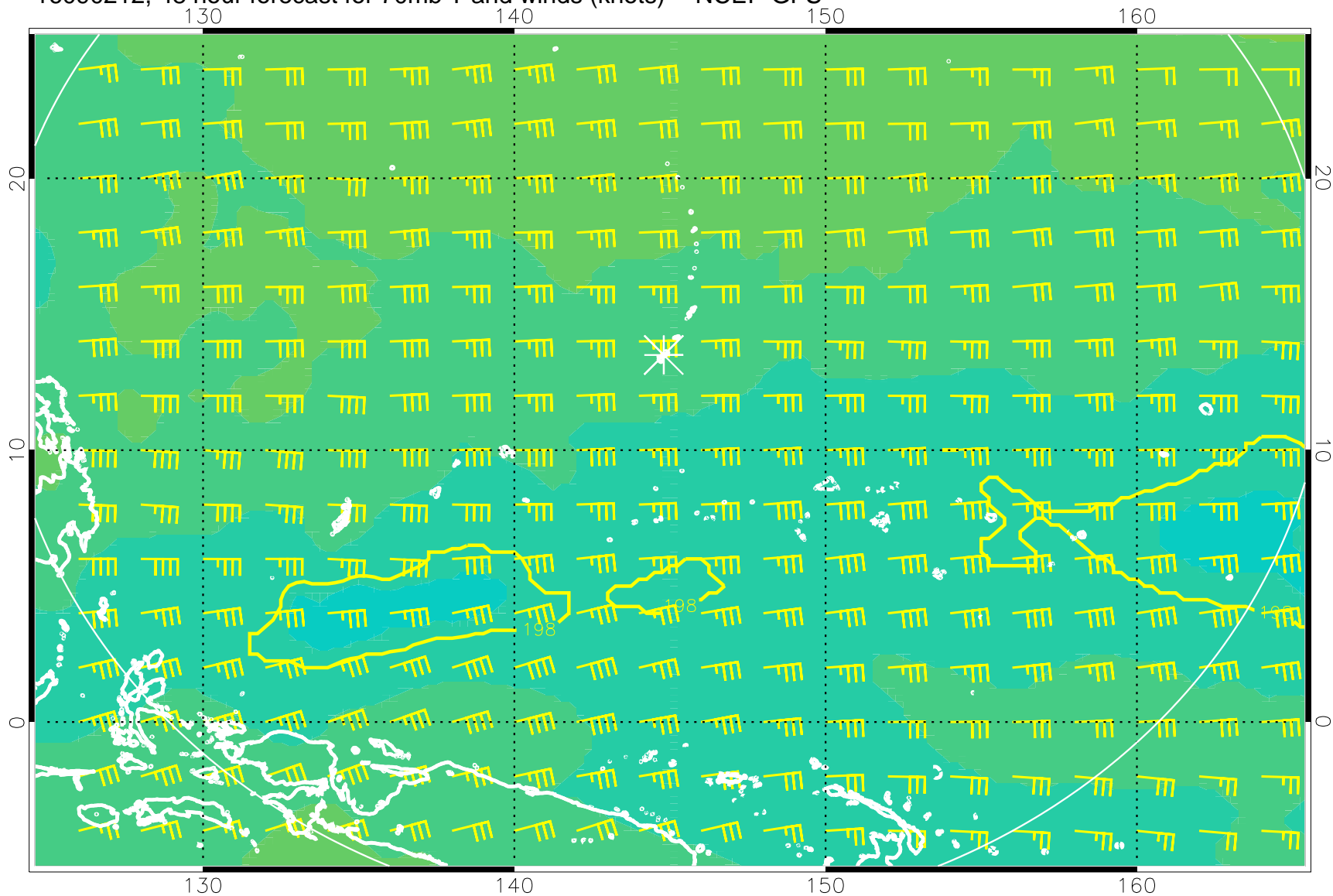
16090212, 48 hour forecast for 70mb T and winds (knots) -- NCEP GFS
