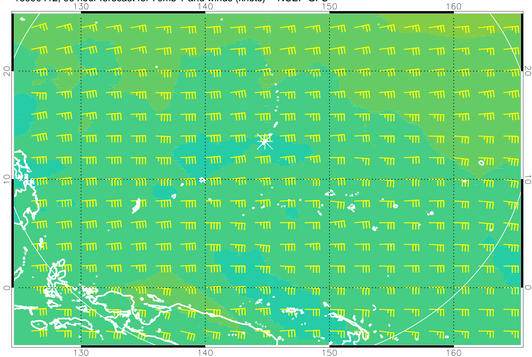
16090412, 96 hour forecast for 70mb T and winds (knots) -- NCEP GFS
