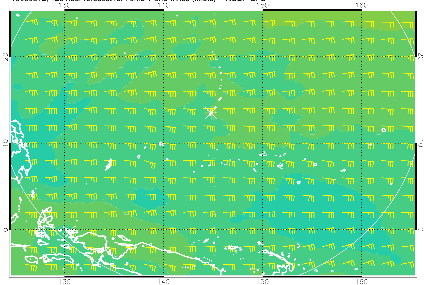
16090512, 120 hour forecast for 70mb T and winds (knots) -- NCEP GFS
