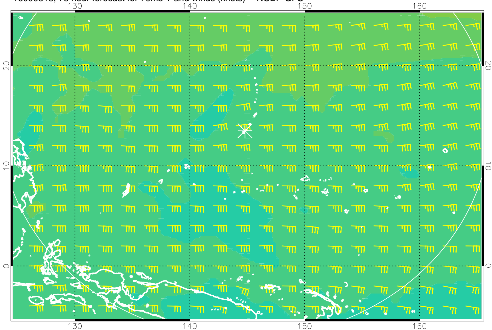
16090318, 78 hour forecast for 70mb T and winds (knots) -- NCEP GFS
