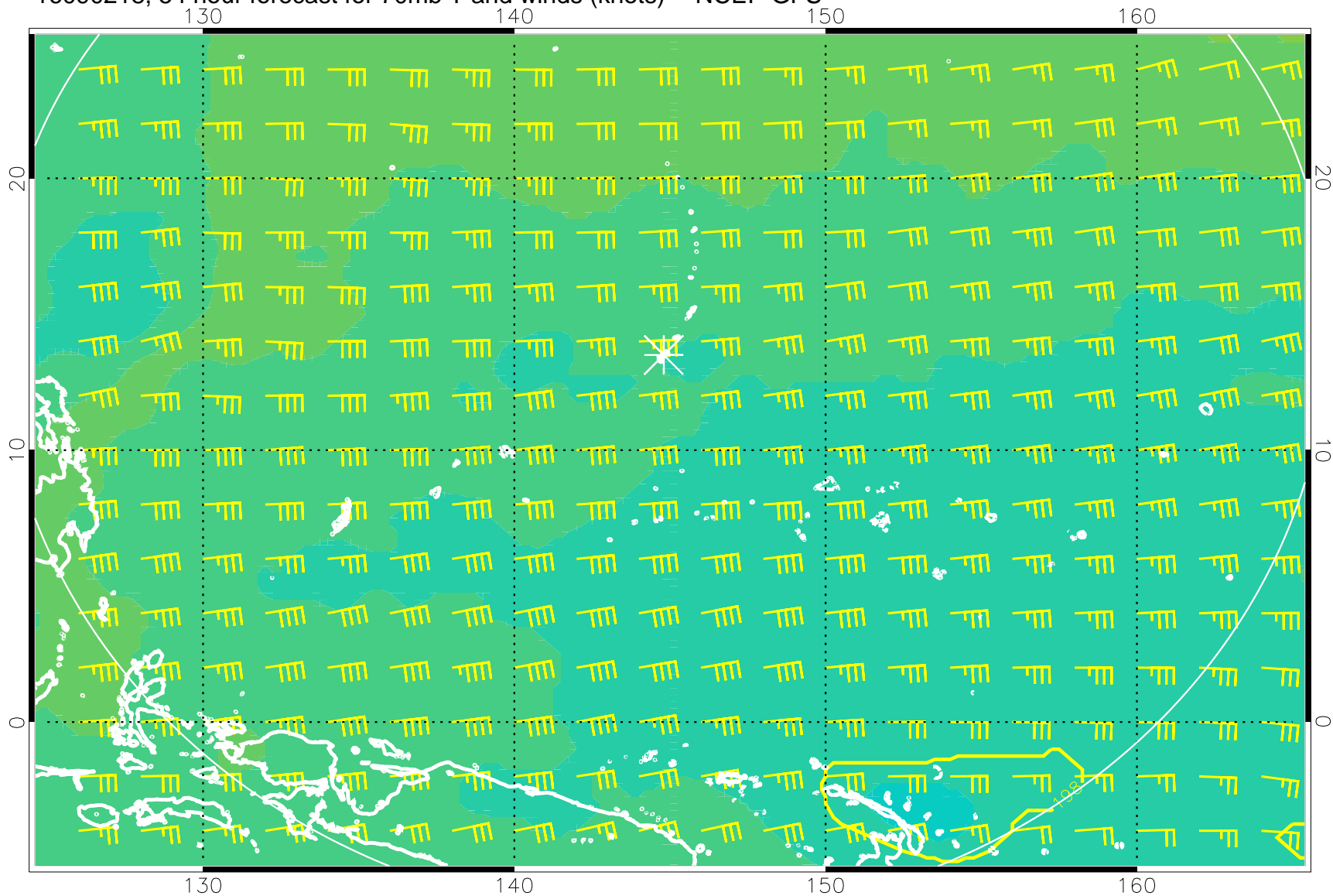
16090218, 54 hour forecast for 70mb T and winds (knots) -- NCEP GFS
