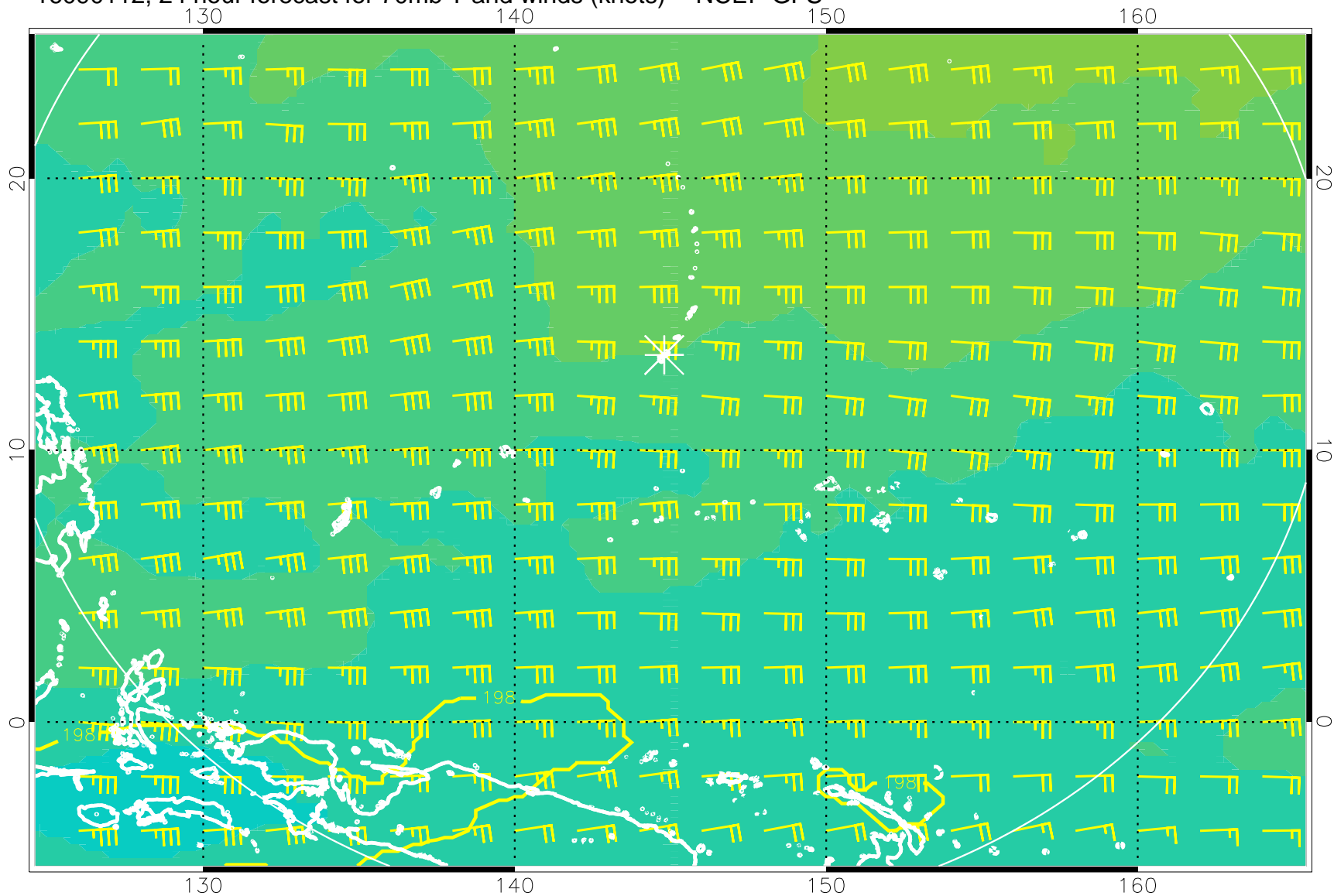
16090112, 24 hour forecast for 70mb T and winds (knots) -- NCEP GFS
