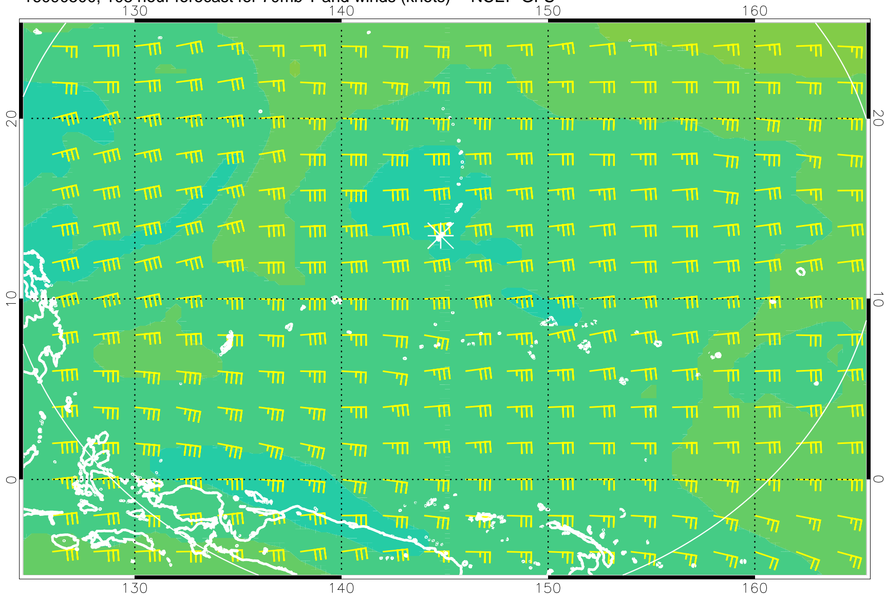
16090500, 108 hour forecast for 70mb T and winds (knots) -- NCEP GFS
