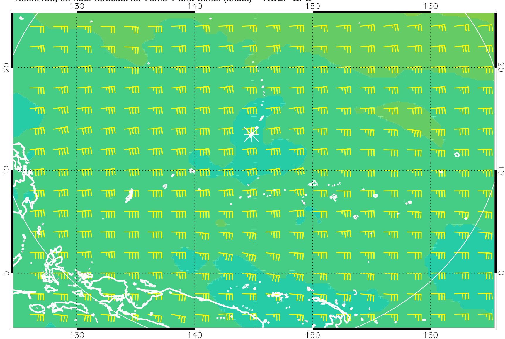
16090406, 90 hour forecast for 70mb T and winds (knots) -- NCEP GFS
