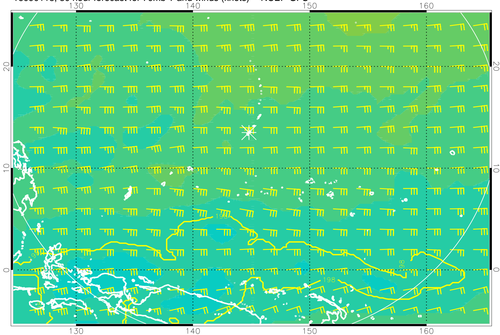
16090118, 30 hour forecast for 70mb T and winds (knots) -- NCEP GFS
