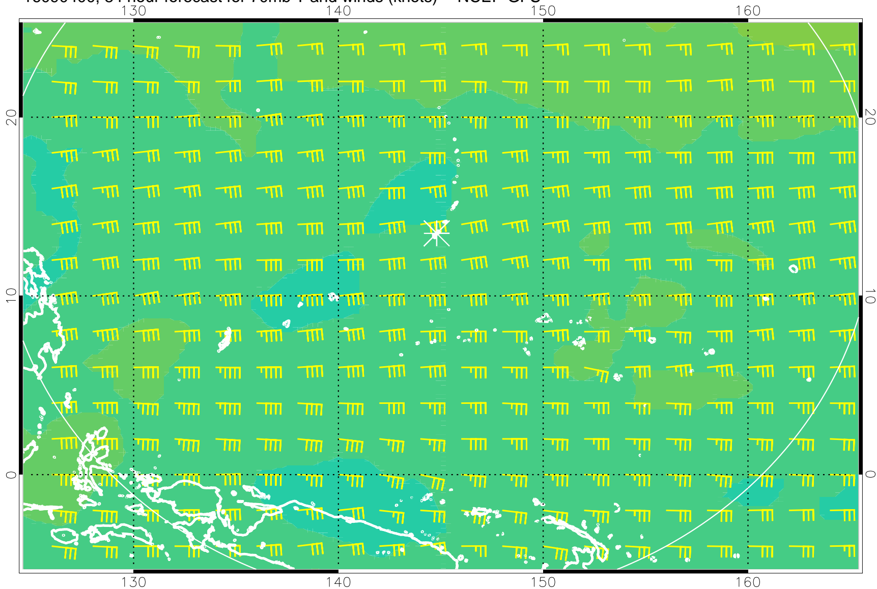
16090400, 84 hour forecast for 70mb T and winds (knots) -- NCEP GFS
