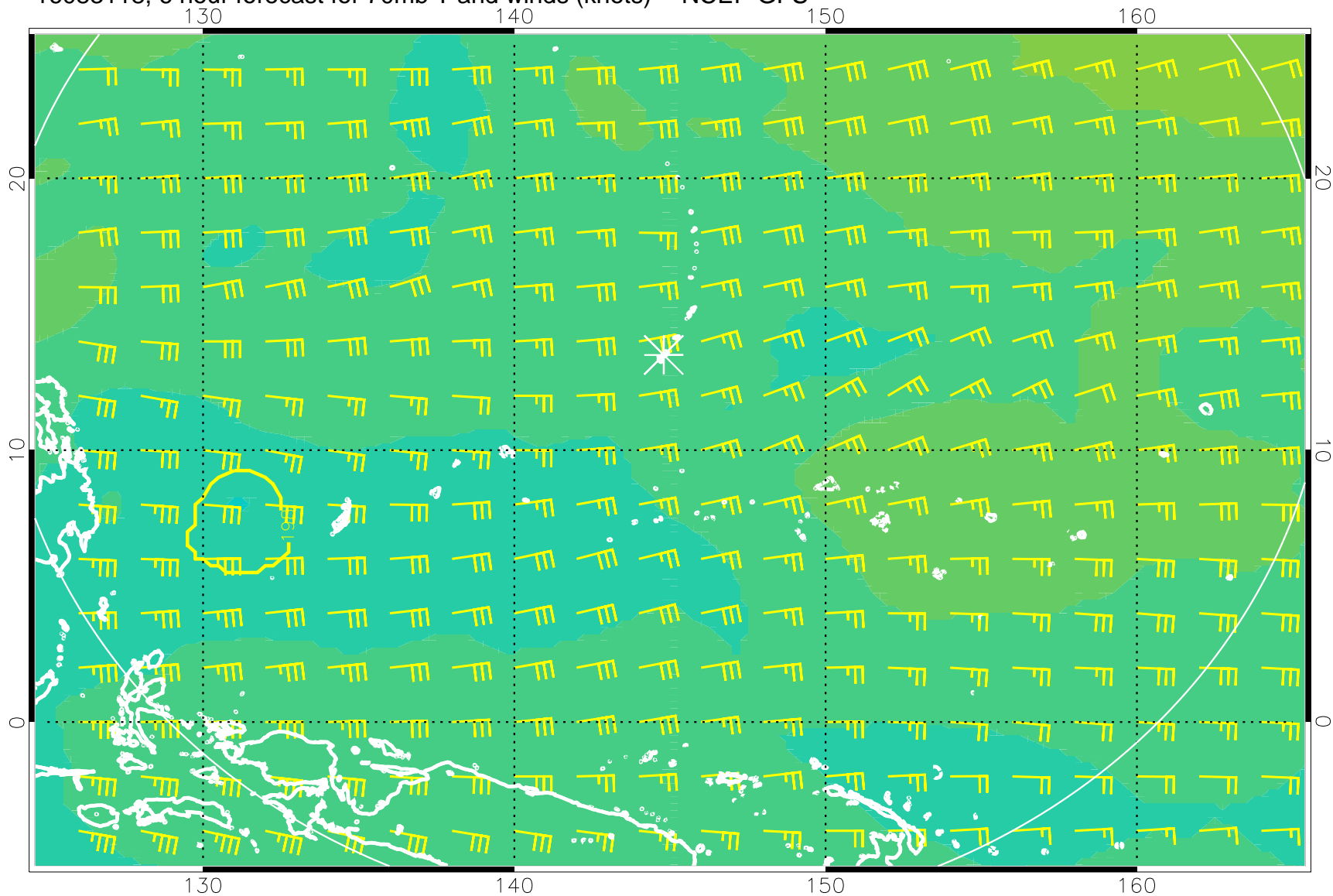
16083118, 6 hour forecast for 70mb T and winds (knots) -- NCEP GFS
