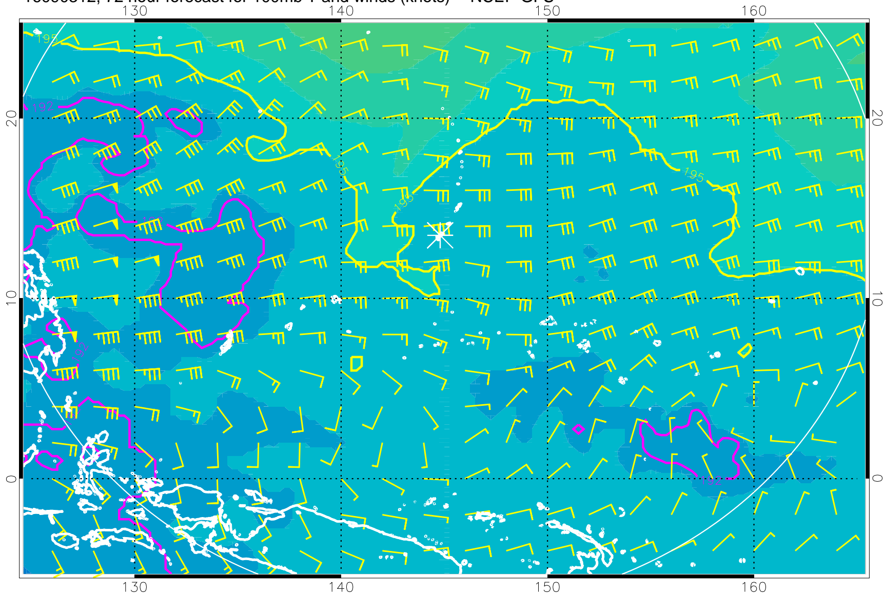
16090312, 72 hour forecast for 100mb T and winds (knots) -- NCEP GFS
