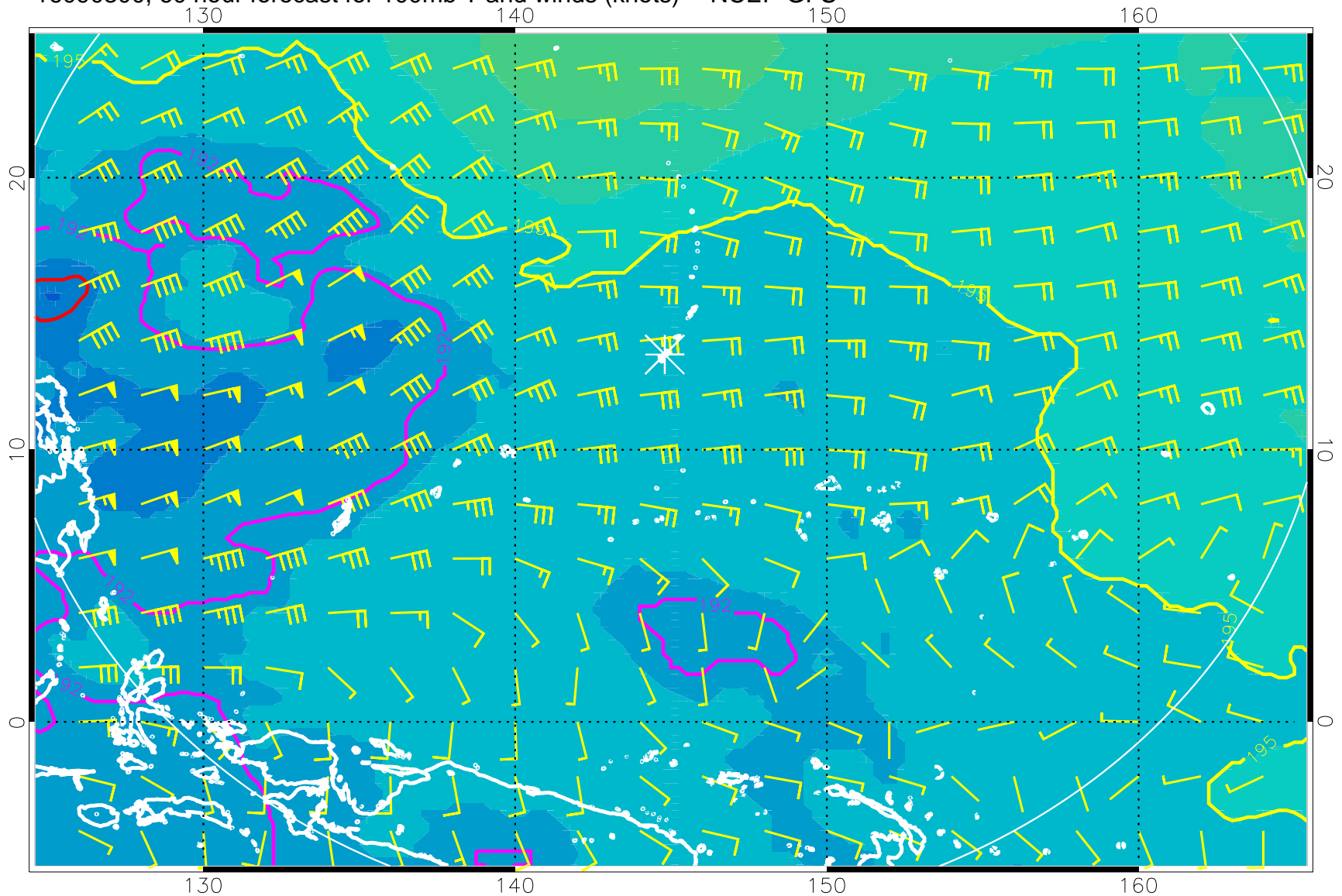
16090300, 60 hour forecast for 100mb T and winds (knots) -- NCEP GFS
