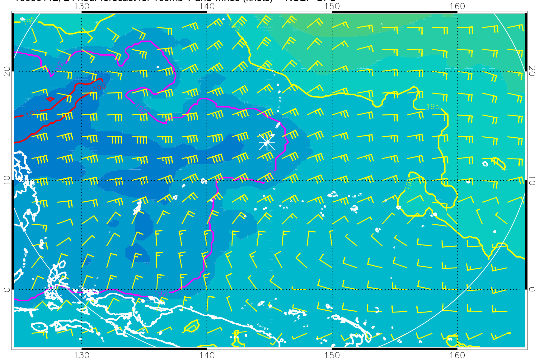
16090112, 24 hour forecast for 100mb T and winds (knots) -- NCEP GFS
