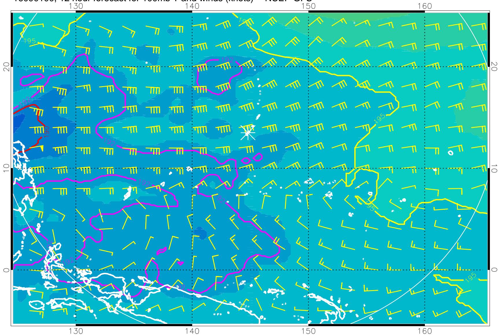
16090100, 12 hour forecast for 100mb T and winds (knots) -- NCEP GFS
