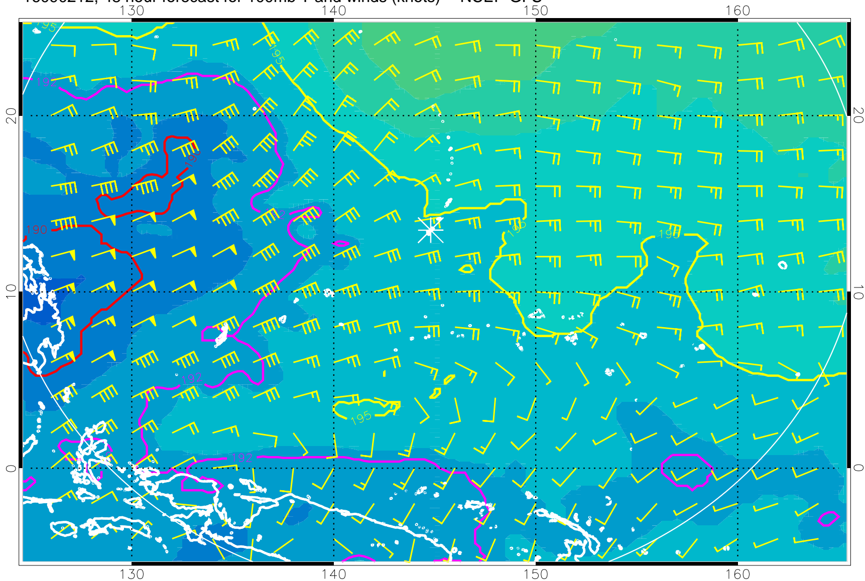
16090212, 48 hour forecast for 100mb T and winds (knots) -- NCEP GFS
