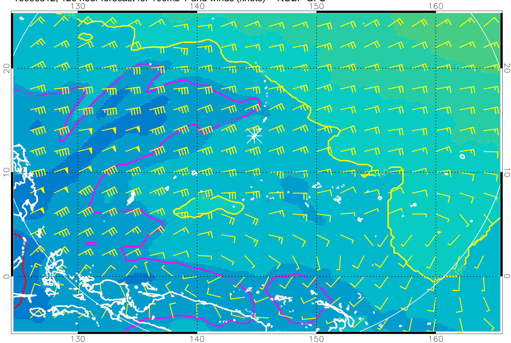
16090512, 120 hour forecast for 100mb T and winds (knots) -- NCEP GFS
