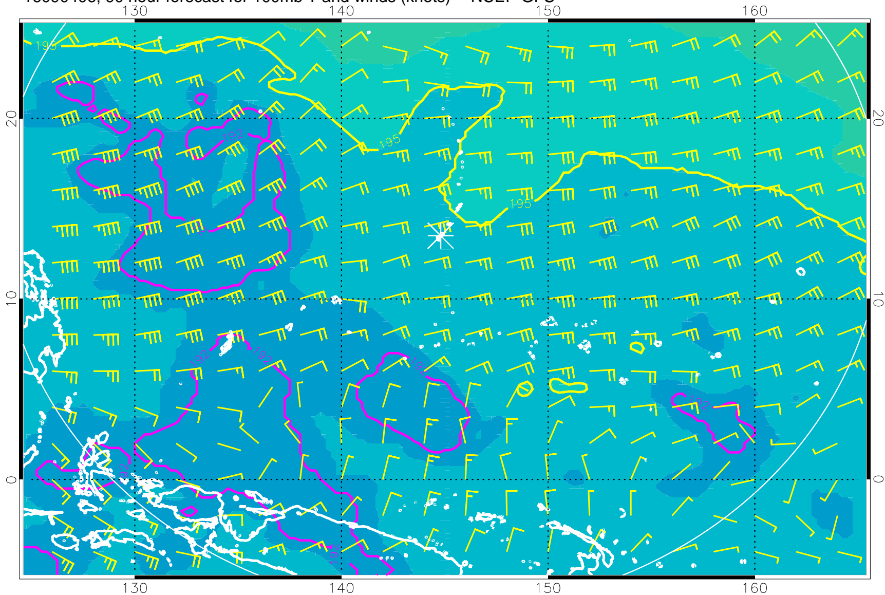
16090406, 90 hour forecast for 100mb T and winds (knots) -- NCEP GFS
