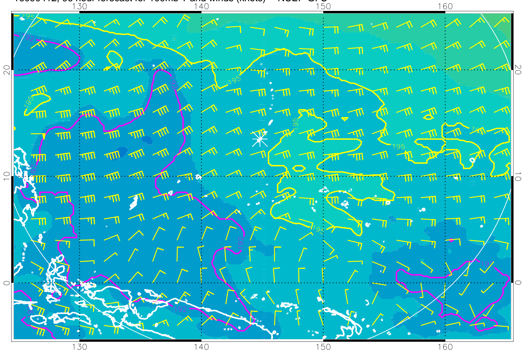
16090412, 96 hour forecast for 100mb T and winds (knots) -- NCEP GFS
