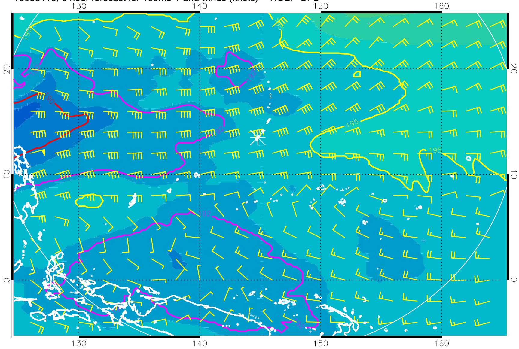
16083118, 6 hour forecast for 100mb T and winds (knots) -- NCEP GFS
