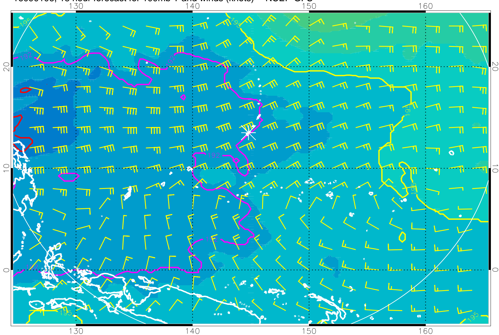
16090106, 18 hour forecast for 100mb T and winds (knots) -- NCEP GFS
