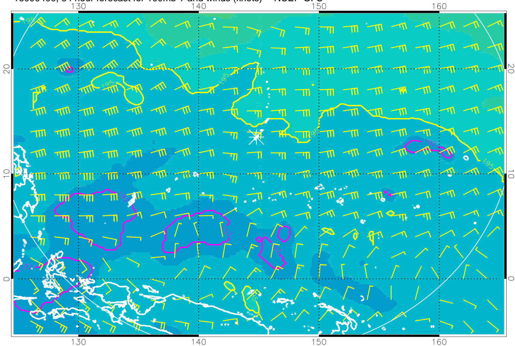
16090400, 84 hour forecast for 100mb T and winds (knots) -- NCEP GFS
