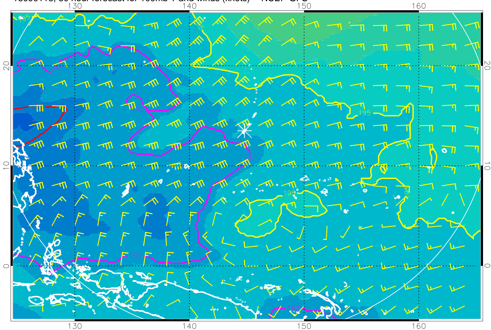
16090118, 30 hour forecast for 100mb T and winds (knots) -- NCEP GFS
