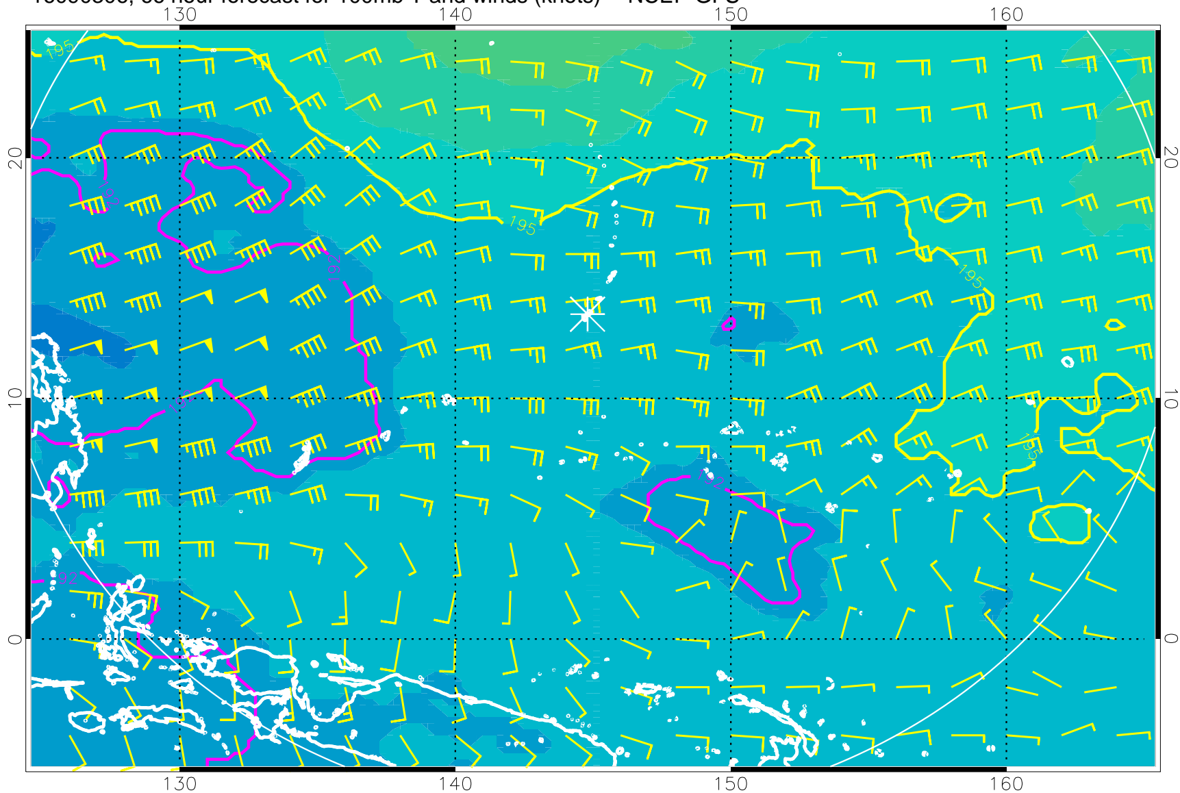
16090306, 66 hour forecast for 100mb T and winds (knots) -- NCEP GFS
