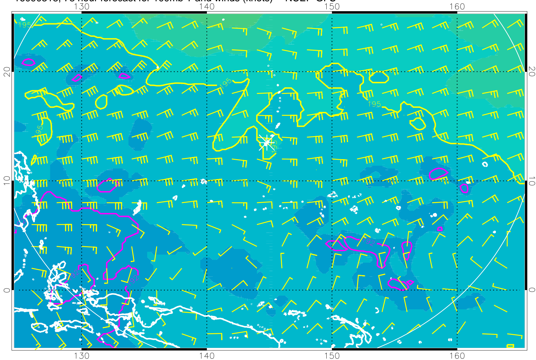
16090318, 78 hour forecast for 100mb T and winds (knots) -- NCEP GFS
