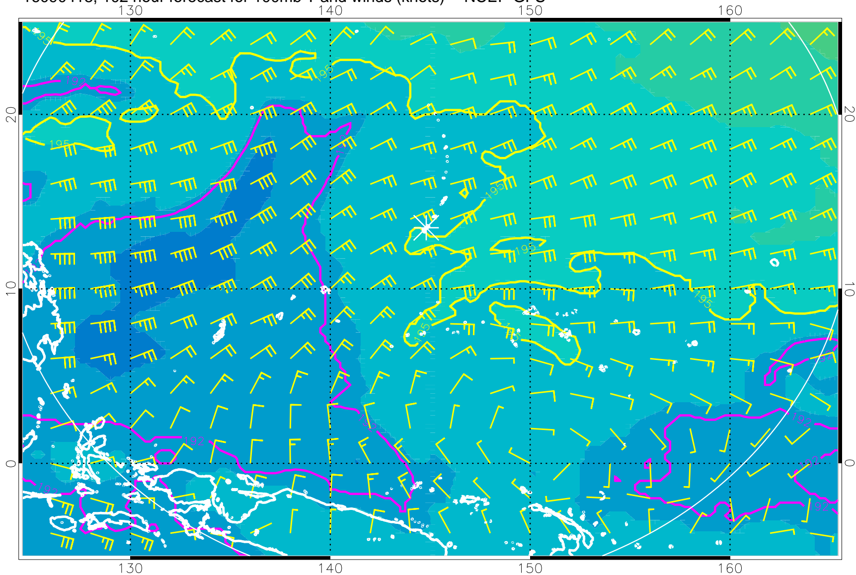
16090418, 102 hour forecast for 100mb T and winds (knots) -- NCEP GFS
