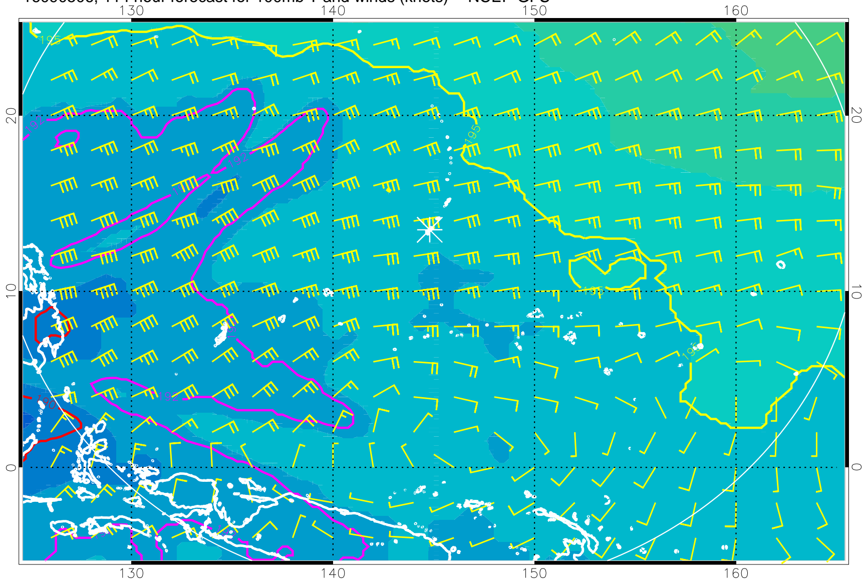
16090506, 114 hour forecast for 100mb T and winds (knots) -- NCEP GFS
