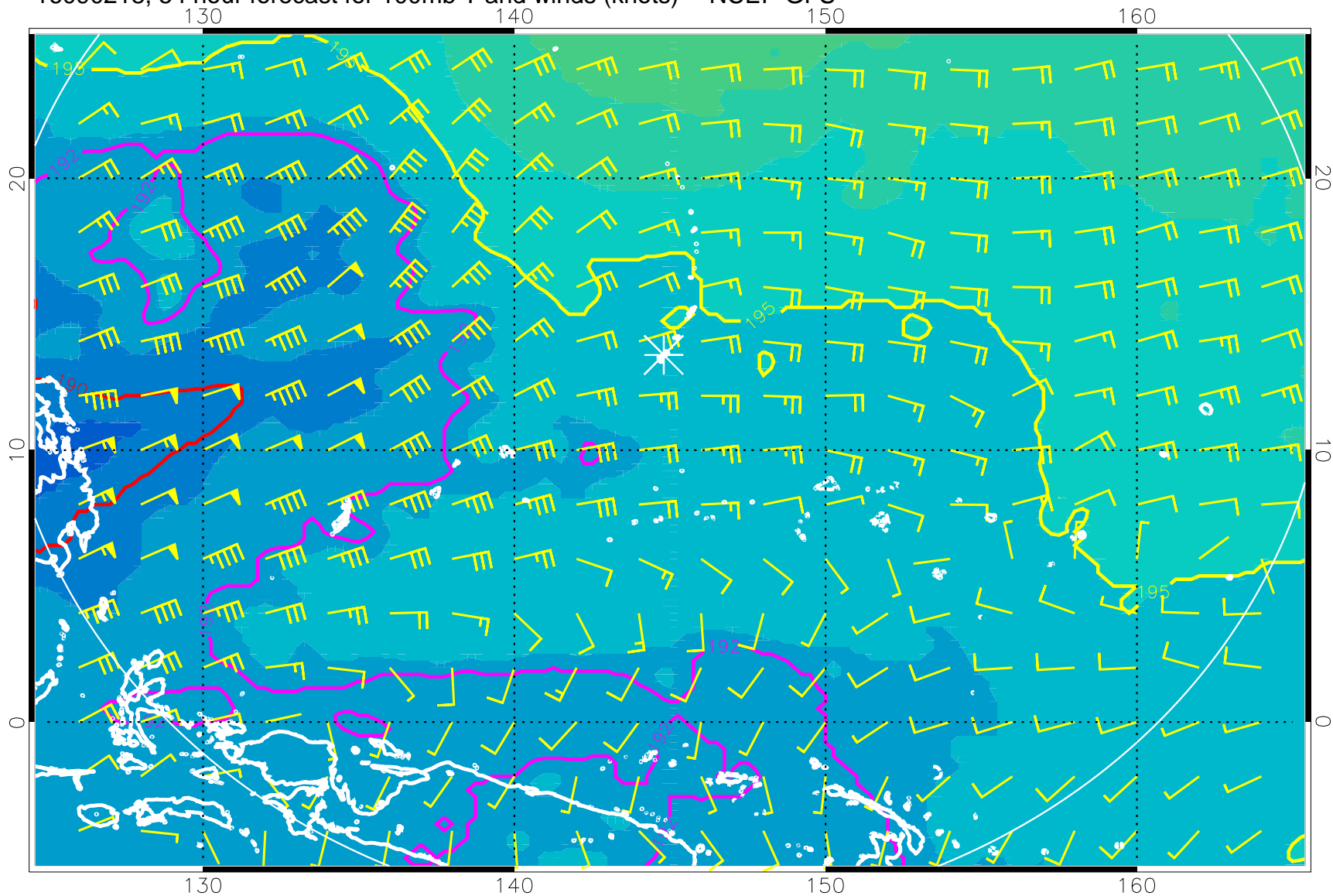
16090218, 54 hour forecast for 100mb T and winds (knots) -- NCEP GFS
