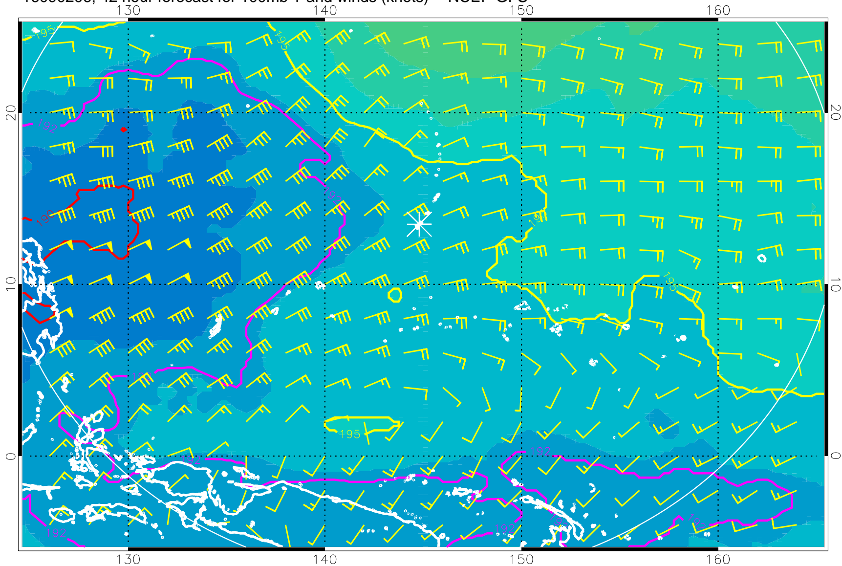
16090206, 42 hour forecast for 100mb T and winds (knots) -- NCEP GFS
