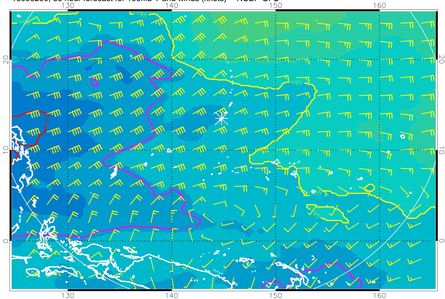
16090200, 36 hour forecast for 100mb T and winds (knots) -- NCEP GFS
