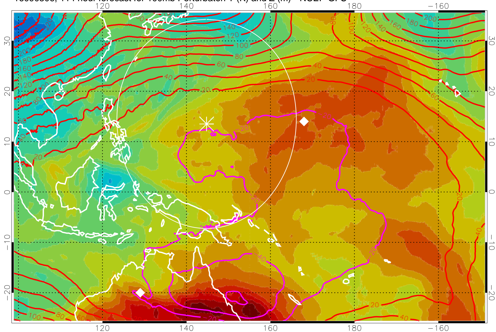
16090506, 114 hour forecast for 100mb Perturbaton T (K) and Z (m)-- NCEP GFS
