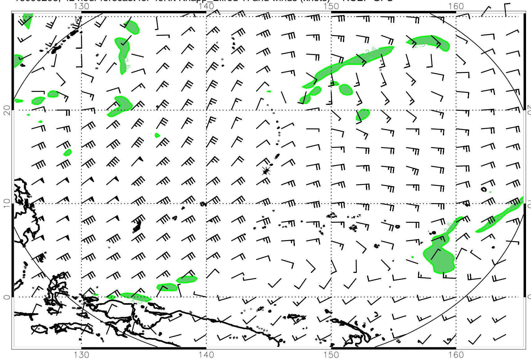
16090206, 42 hour forecast for 49Kft Knapp_Ellrod TI and winds (knots) -- NCEP GFS
