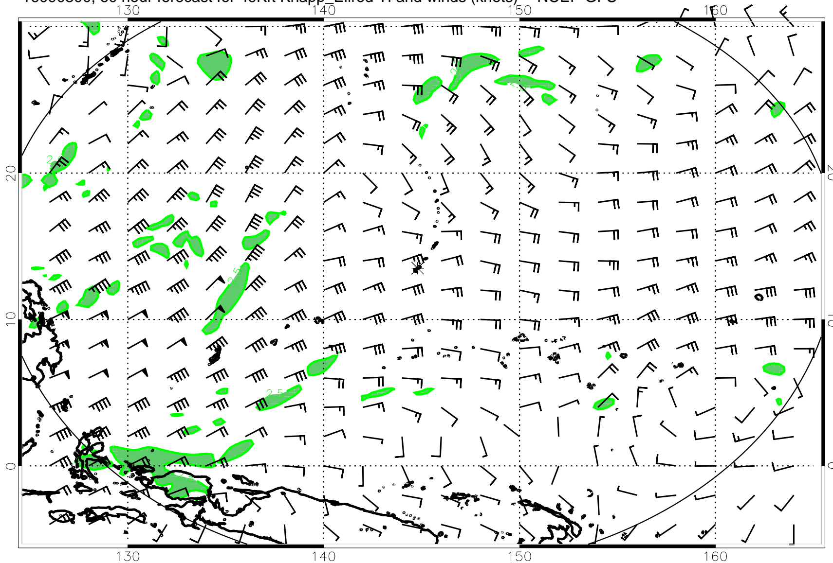
16090300, 60 hour forecast for 49Kft Knapp_Ellrod TI and winds (knots) -- NCEP GFS
