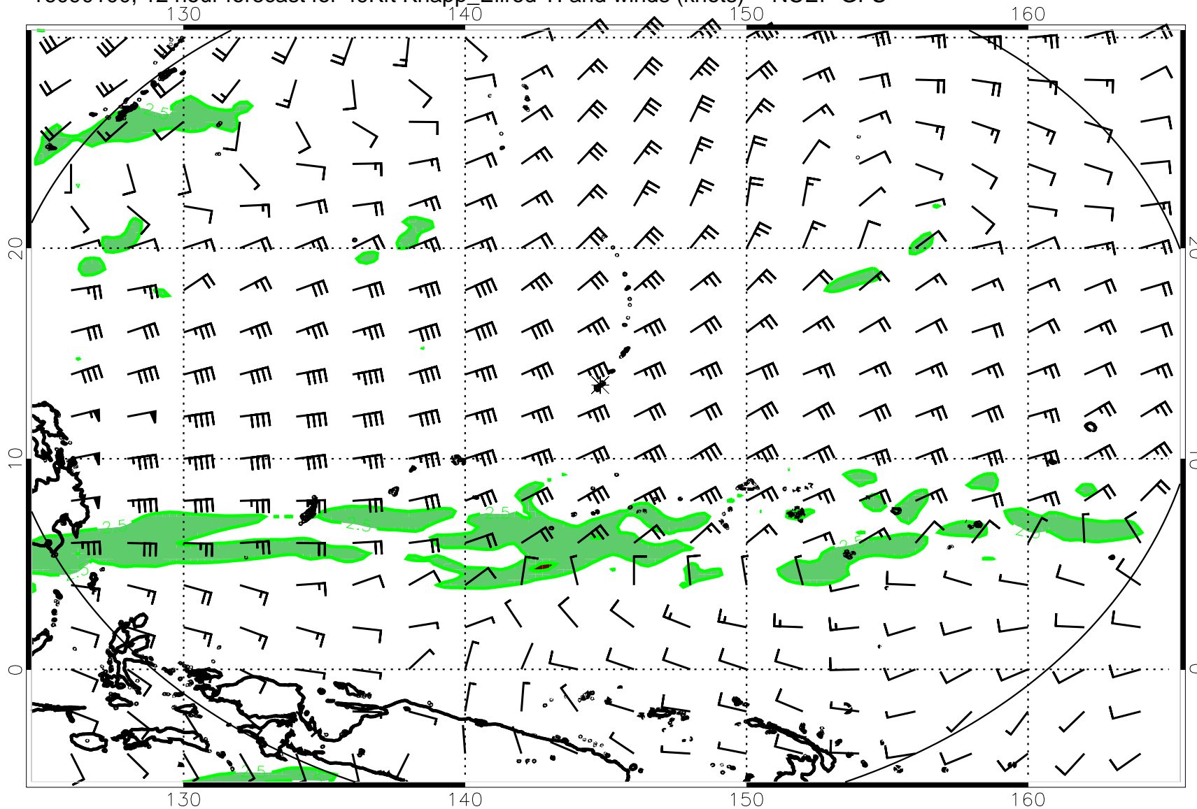
16090100, 12 hour forecast for 49Kft Knapp_Ellrod TI and winds (knots) -- NCEP GFS
