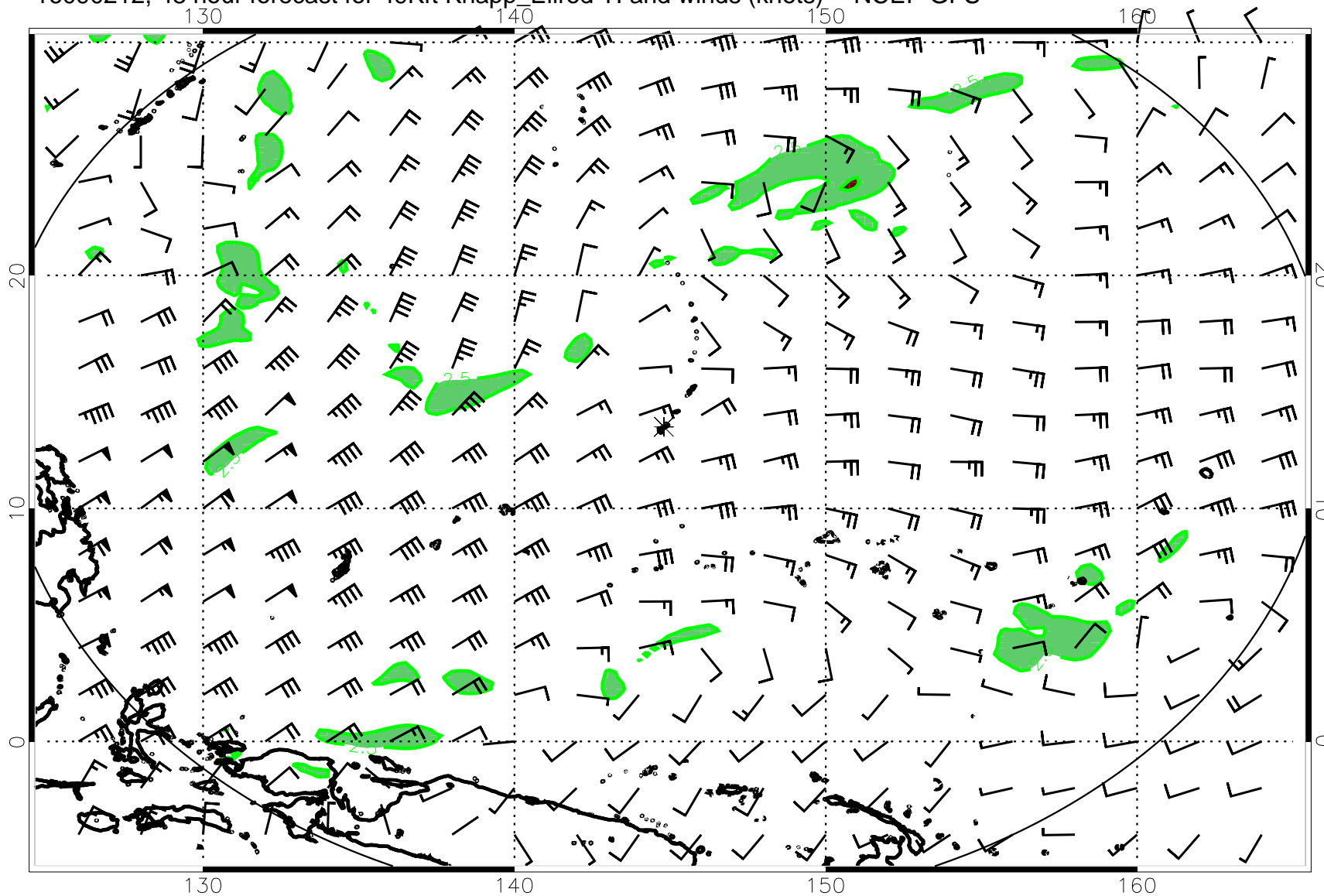
16090212, 48 hour forecast for 49Kft Knapp_Ellrod TI and winds (knots) -- NCEP GFS
