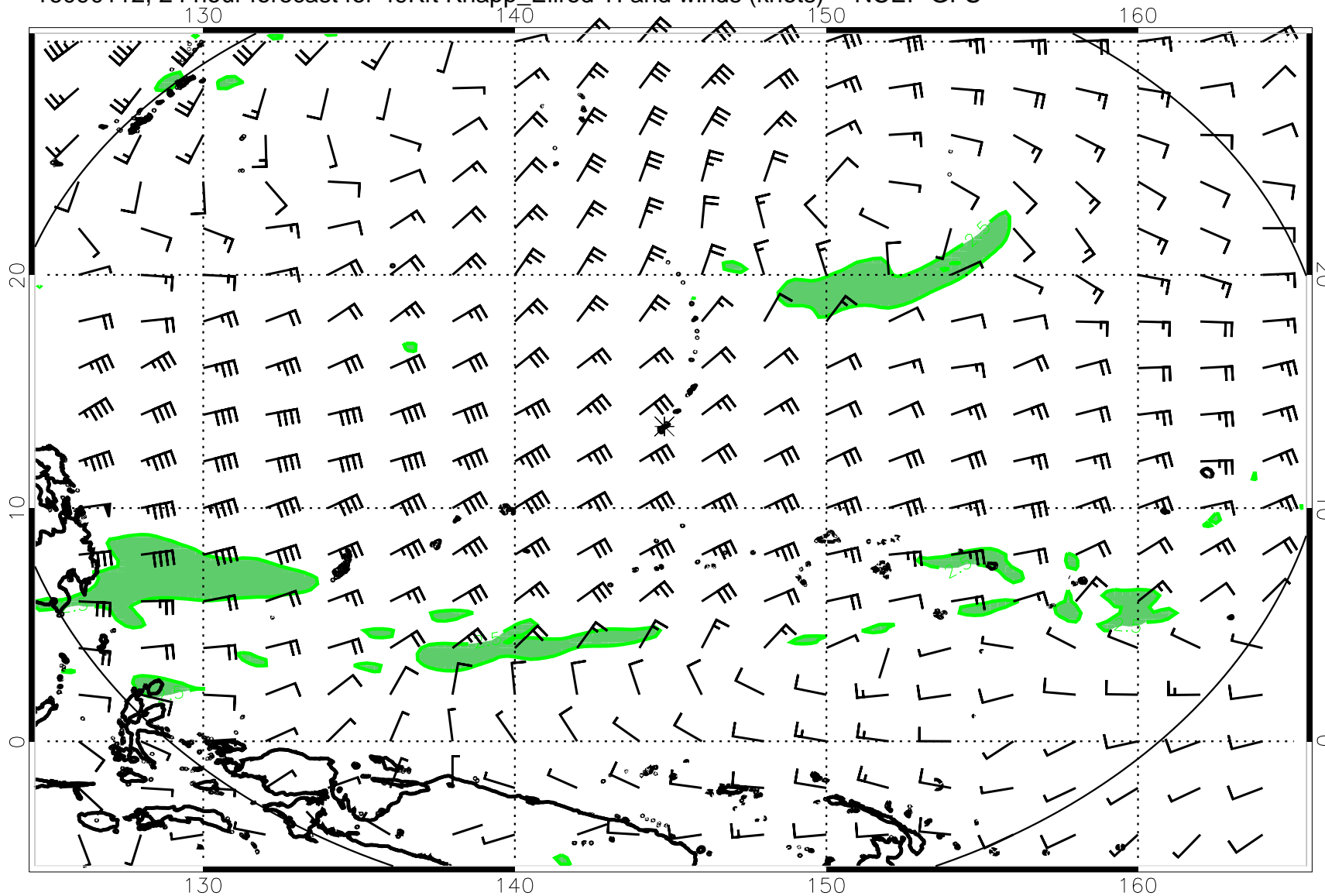
16090112, 24 hour forecast for 49Kft Knapp_Ellrod TI and winds (knots) -- NCEP GFS
