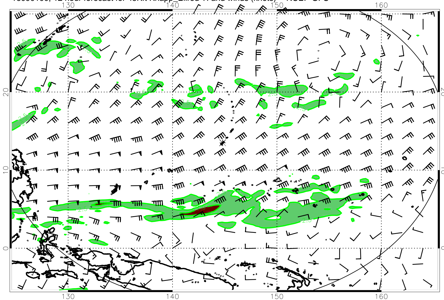
16090100, 12 hour forecast for 45Kft Knapp_Ellrod TI and winds (knots) -- NCEP GFS
