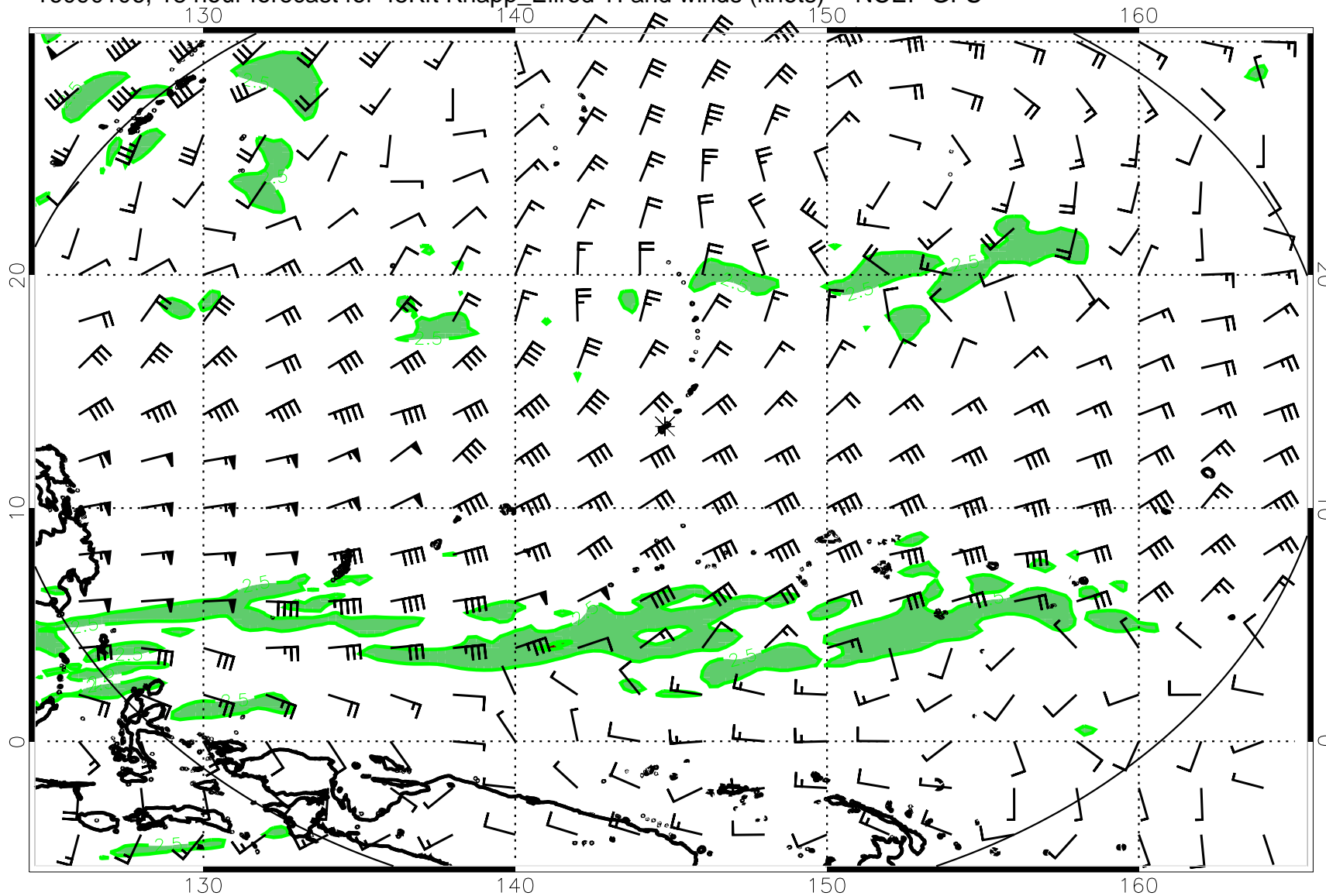
16090106, 18 hour forecast for 45Kft Knapp_Ellrod TI and winds (knots) -- NCEP GFS
