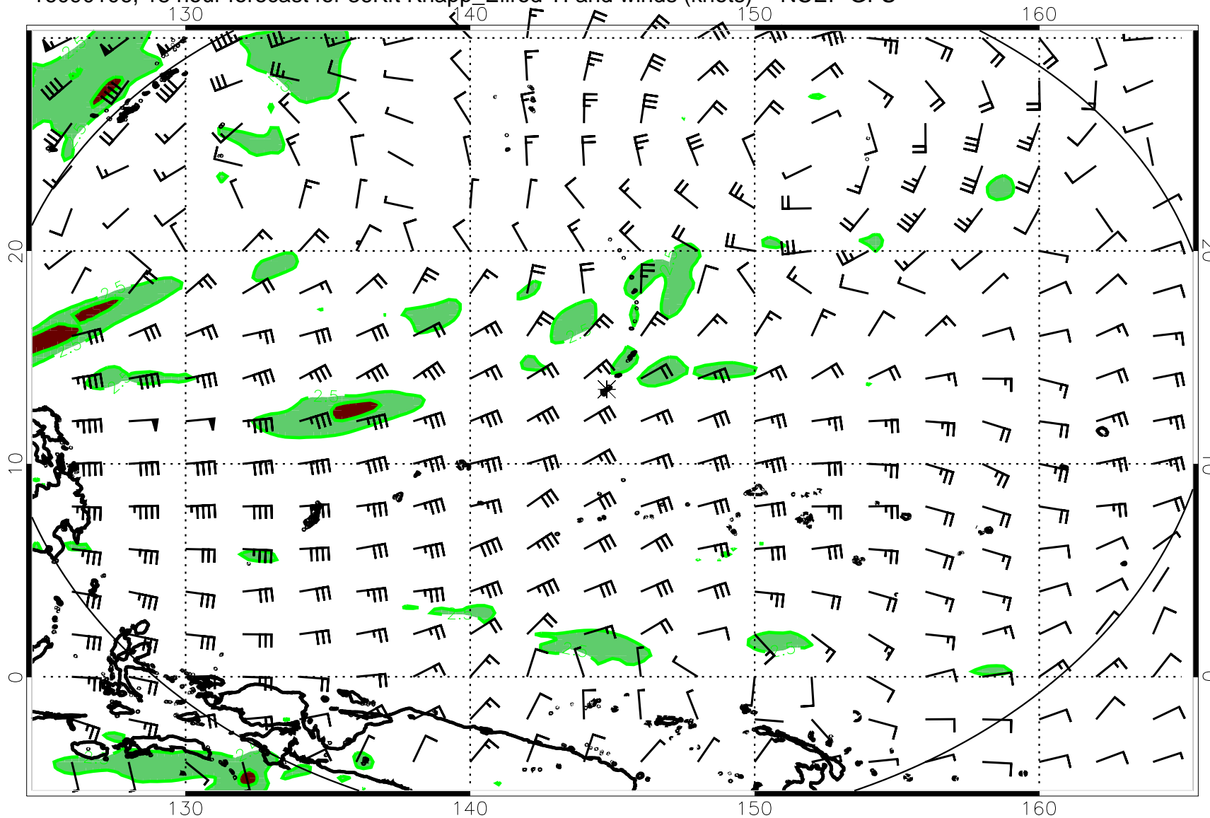
16090106, 18 hour forecast for 36Kft Knapp_Ellrod TI and winds (knots) -- NCEP GFS
