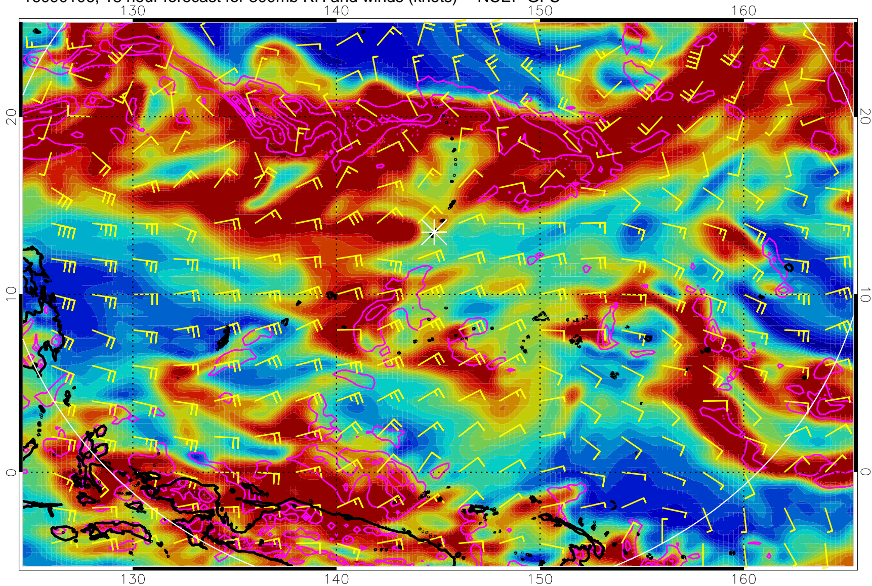
16090106, 18 hour forecast for 300mb RH and winds (knots) -- NCEP GFS
