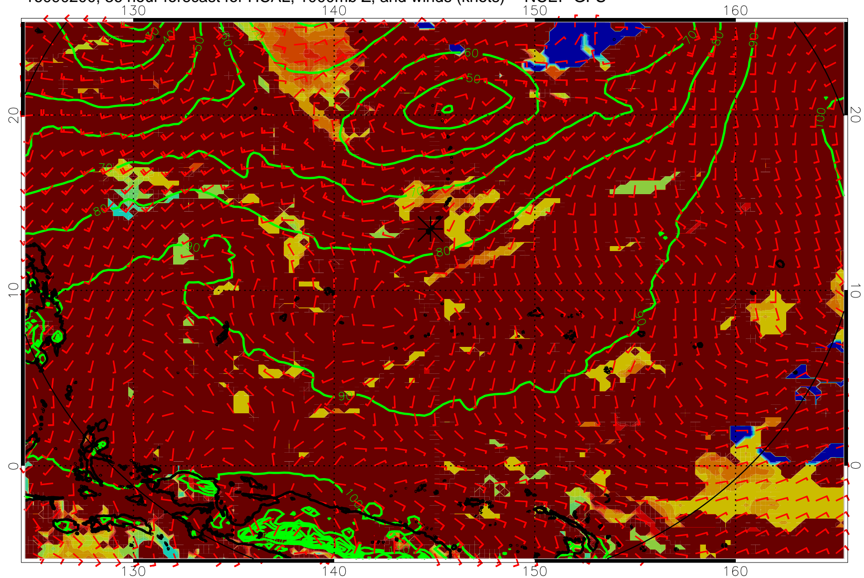
16090200, 36 hour forecast for HCAL, 1000mb Z, and winds (knots) -- NCEP GFS
