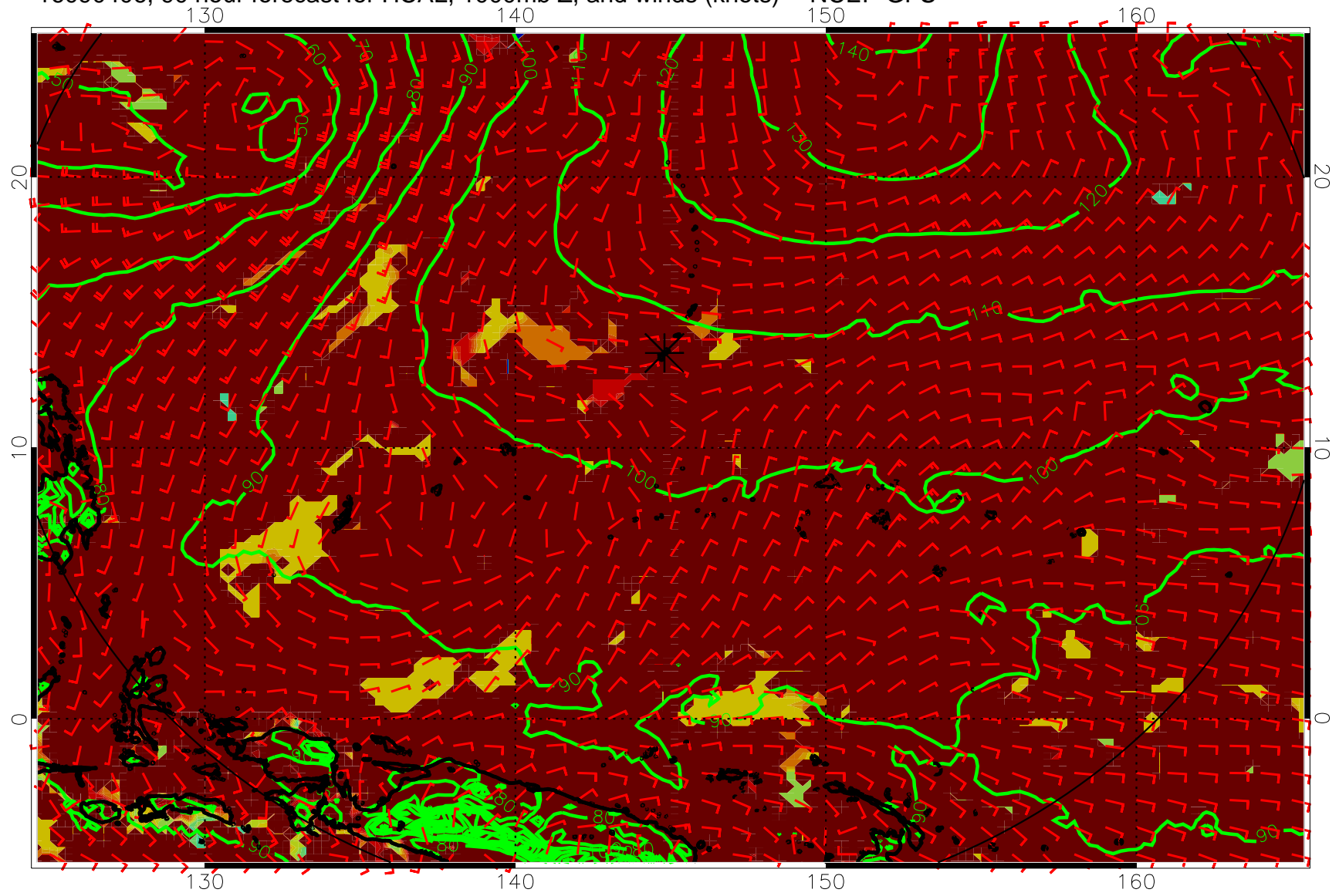
16090406, 90 hour forecast for HCAL, 1000mb Z, and winds (knots) -- NCEP GFS
