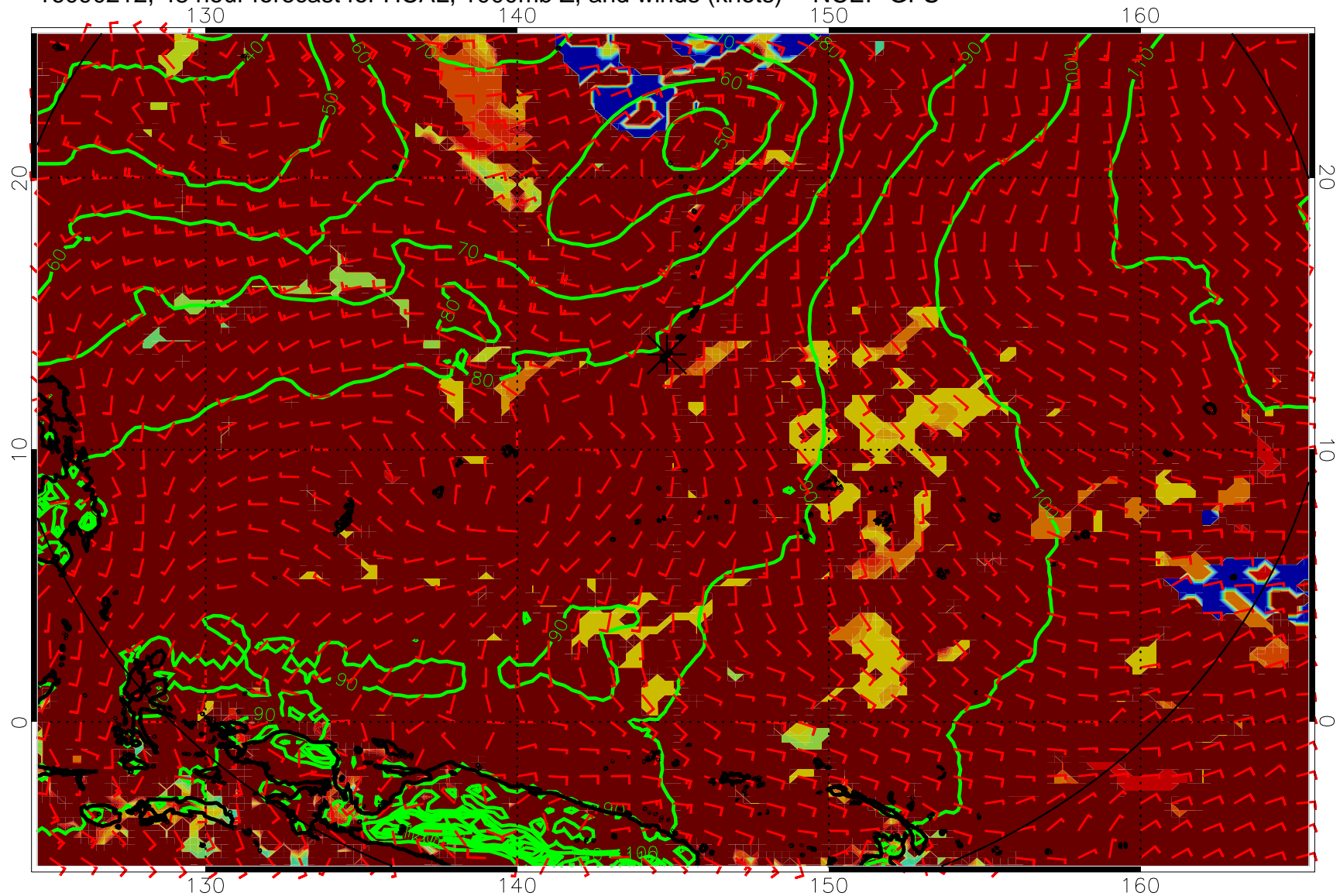
16090212, 48 hour forecast for HCAL, 1000mb Z, and winds (knots) -- NCEP GFS
