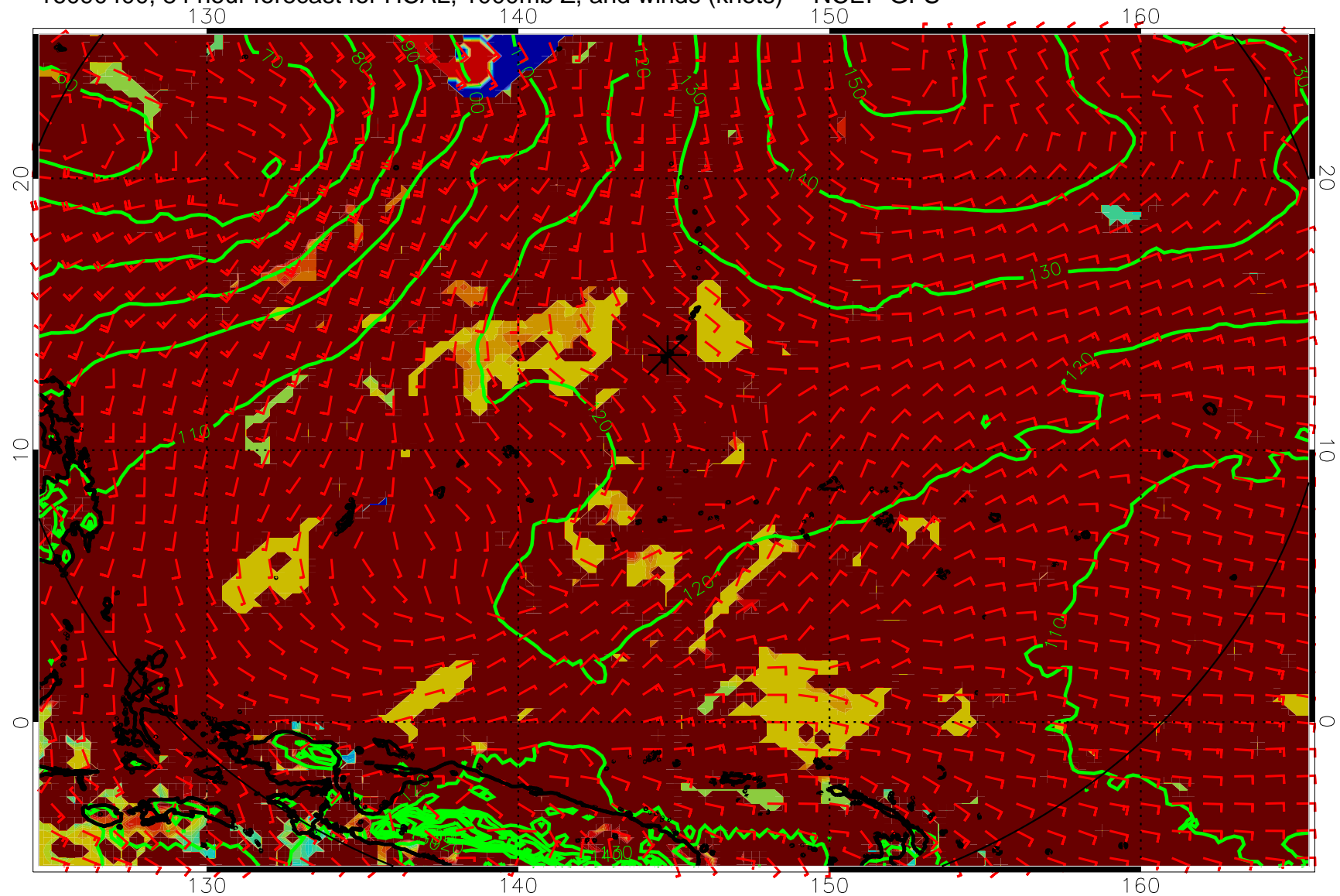
16090400, 84 hour forecast for HCAL, 1000mb Z, and winds (knots) -- NCEP GFS
