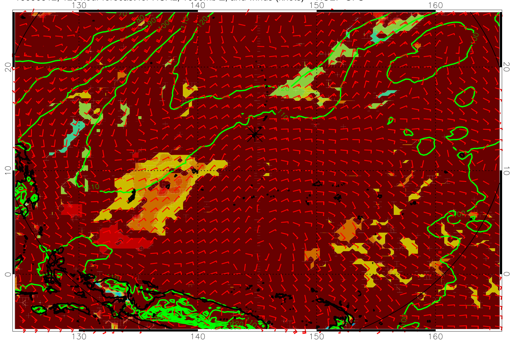
16090512, 120 hour forecast for HCAL, 1000mb Z, and winds (knots) -- NCEP GFS
