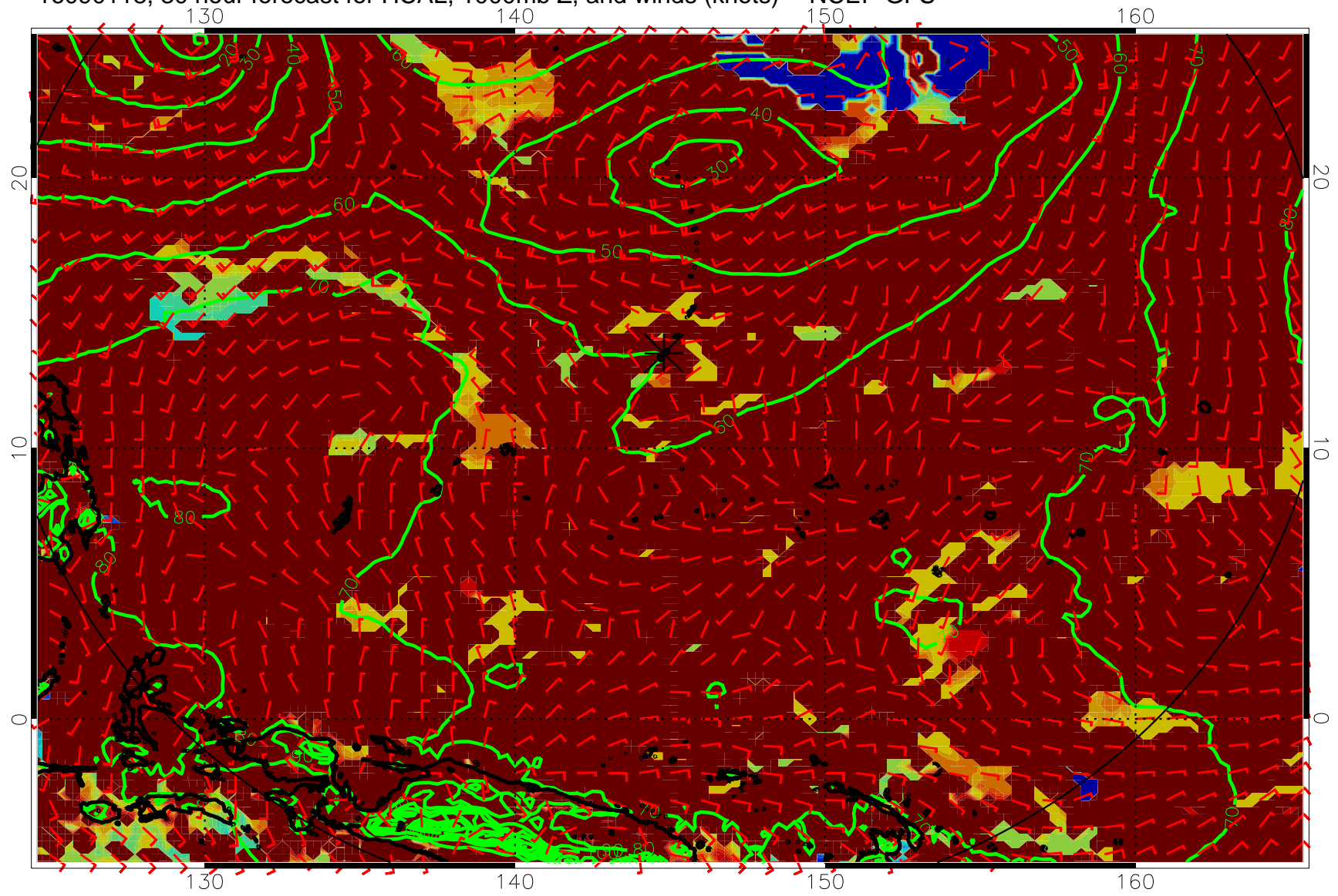
16090118, 30 hour forecast for HCAL, 1000mb Z, and winds (knots) -- NCEP GFS
