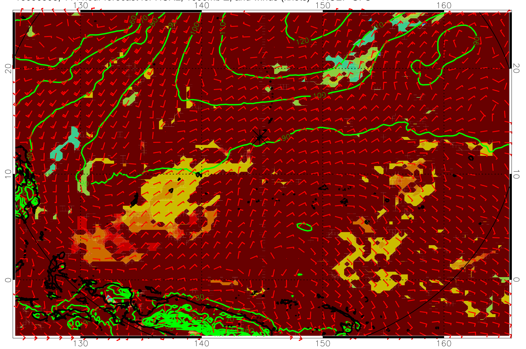
16090506, 114 hour forecast for HCAL, 1000mb Z, and winds (knots) -- NCEP GFS
