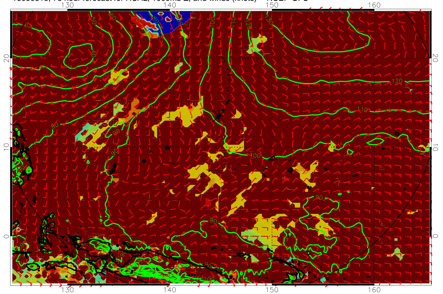
16090318, 78 hour forecast for HCAL, 1000mb Z, and winds (knots) -- NCEP GFS
