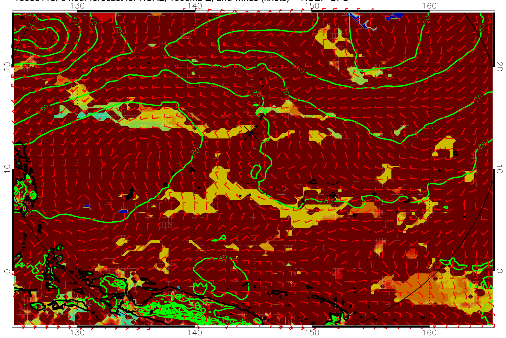
16083118, 6 hour forecast for HCAL, 1000mb Z, and winds (knots) -- NCEP GFS
