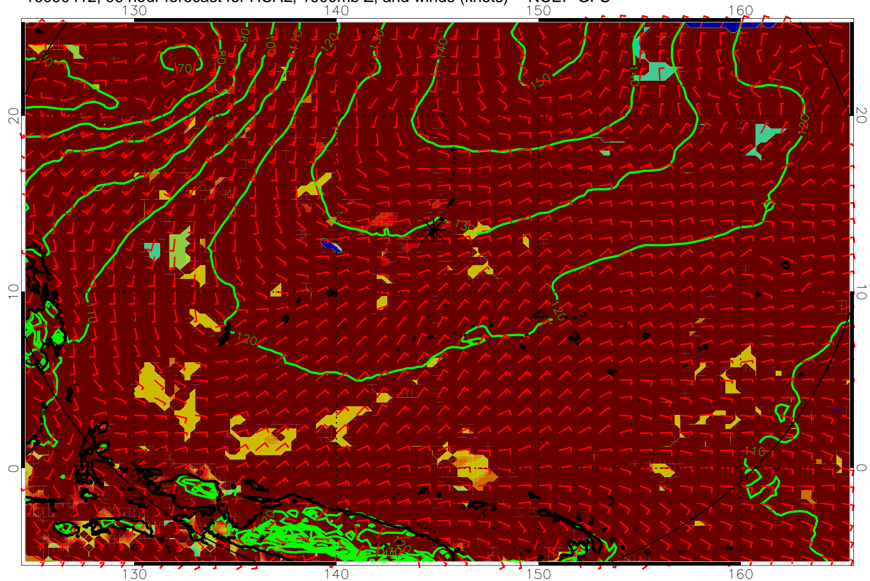
16090412, 96 hour forecast for HCAL, 1000mb Z, and winds (knots) -- NCEP GFS
