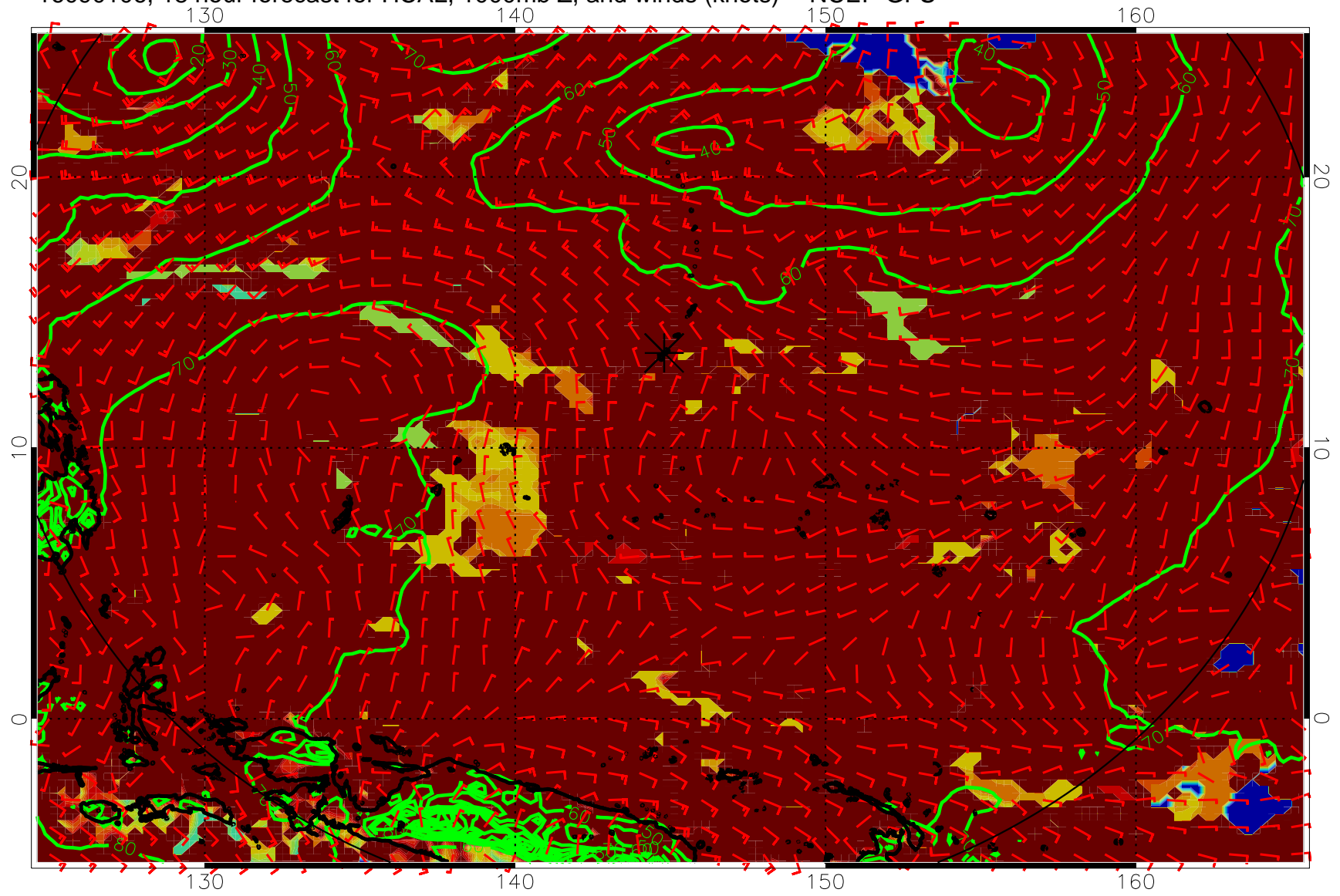
16090106, 18 hour forecast for HCAL, 1000mb Z, and winds (knots) -- NCEP GFS
