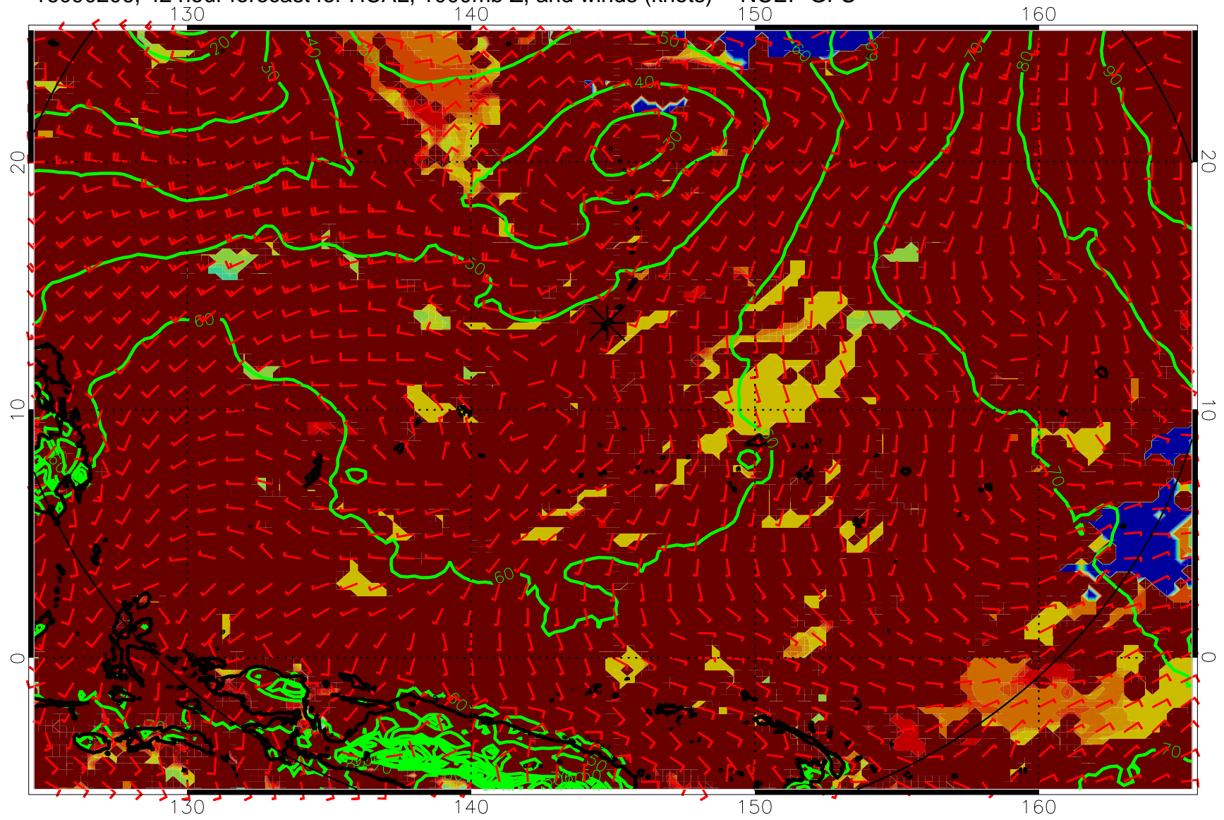
16090206, 42 hour forecast for HCAL, 1000mb Z, and winds (knots) -- NCEP GFS
