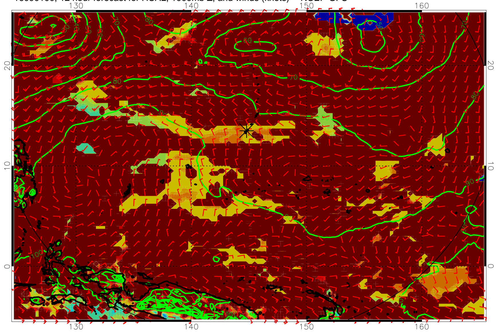
16090100, 12 hour forecast for HCAL, 1000mb Z, and winds (knots) -- NCEP GFS
