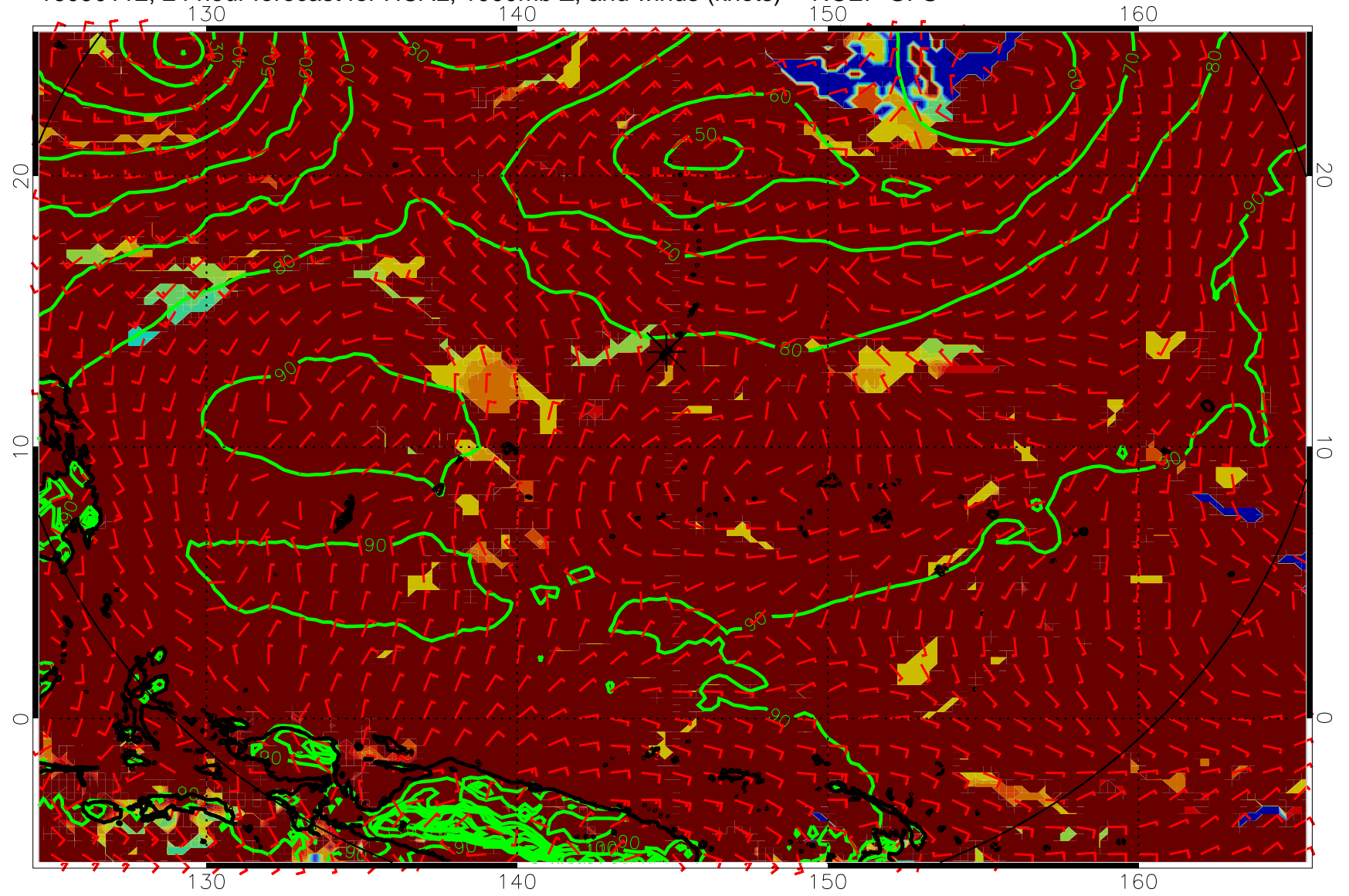
16090112, 24 hour forecast for HCAL, 1000mb Z, and winds (knots) -- NCEP GFS
