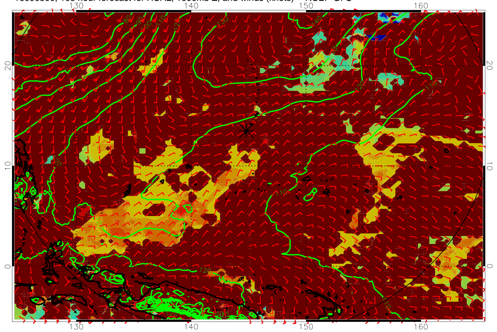
16090500, 108 hour forecast for HCAL, 1000mb Z, and winds (knots) -- NCEP GFS
