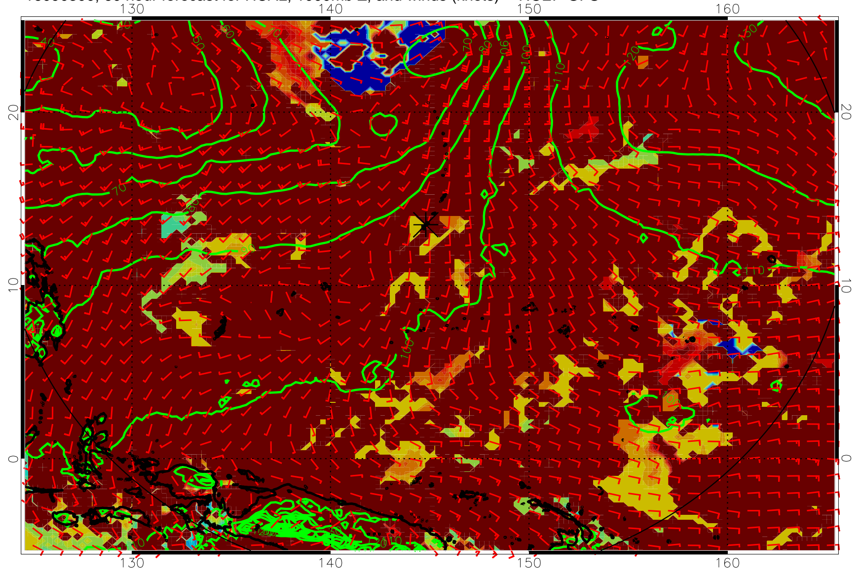
16090300, 60 hour forecast for HCAL, 1000mb Z, and winds (knots) -- NCEP GFS
