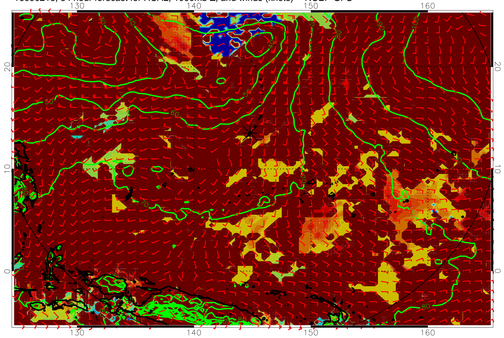
16090218, 54 hour forecast for HCAL, 1000mb Z, and winds (knots) -- NCEP GFS
