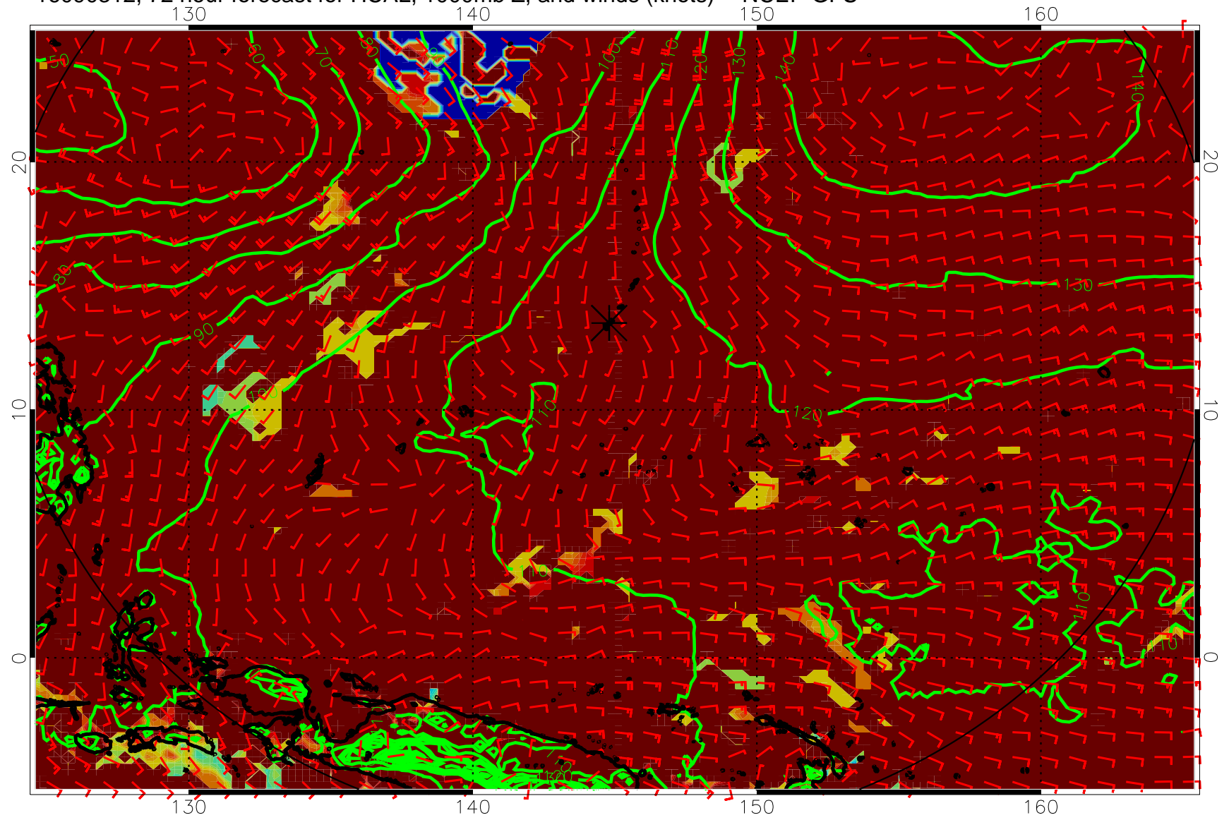
16090312, 72 hour forecast for HCAL, 1000mb Z, and winds (knots) -- NCEP GFS
