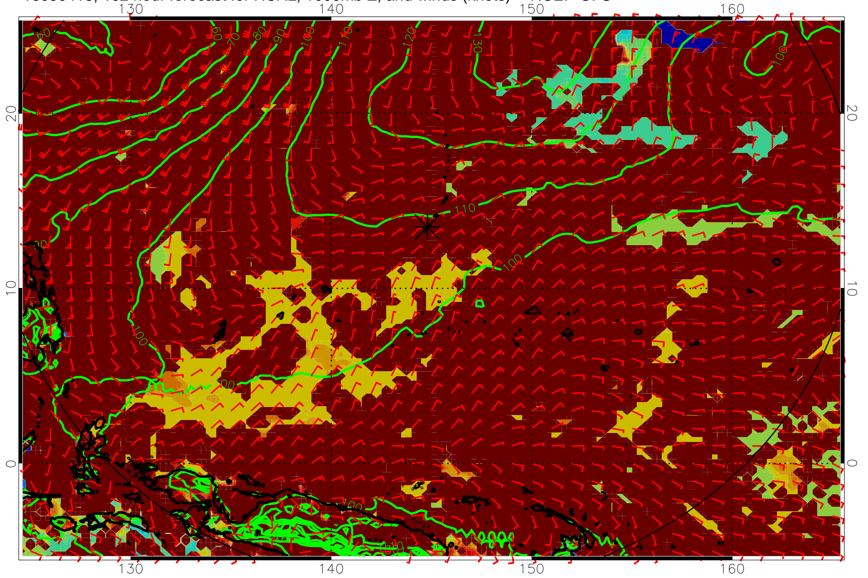
16090418, 102 hour forecast for HCAL, 1000mb Z, and winds (knots) -- NCEP GFS
