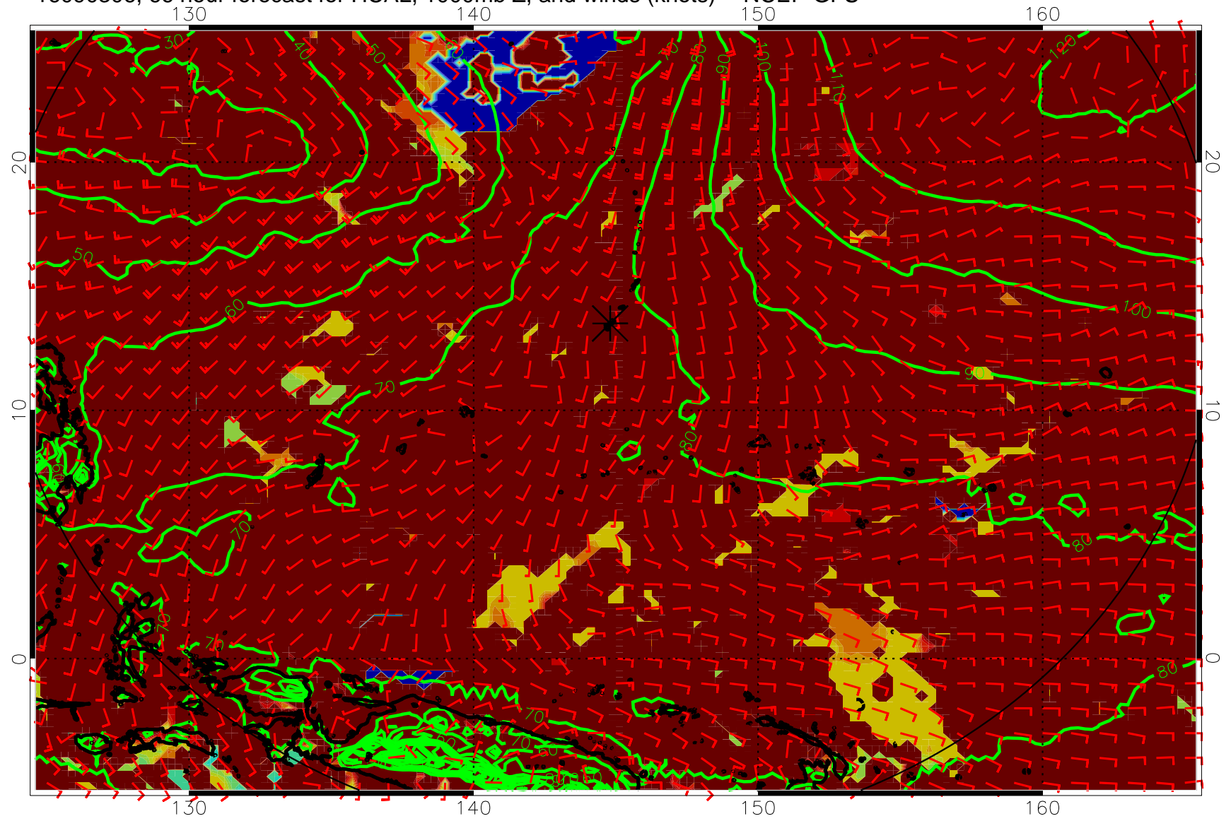
16090306, 66 hour forecast for HCAL, 1000mb Z, and winds (knots) -- NCEP GFS
