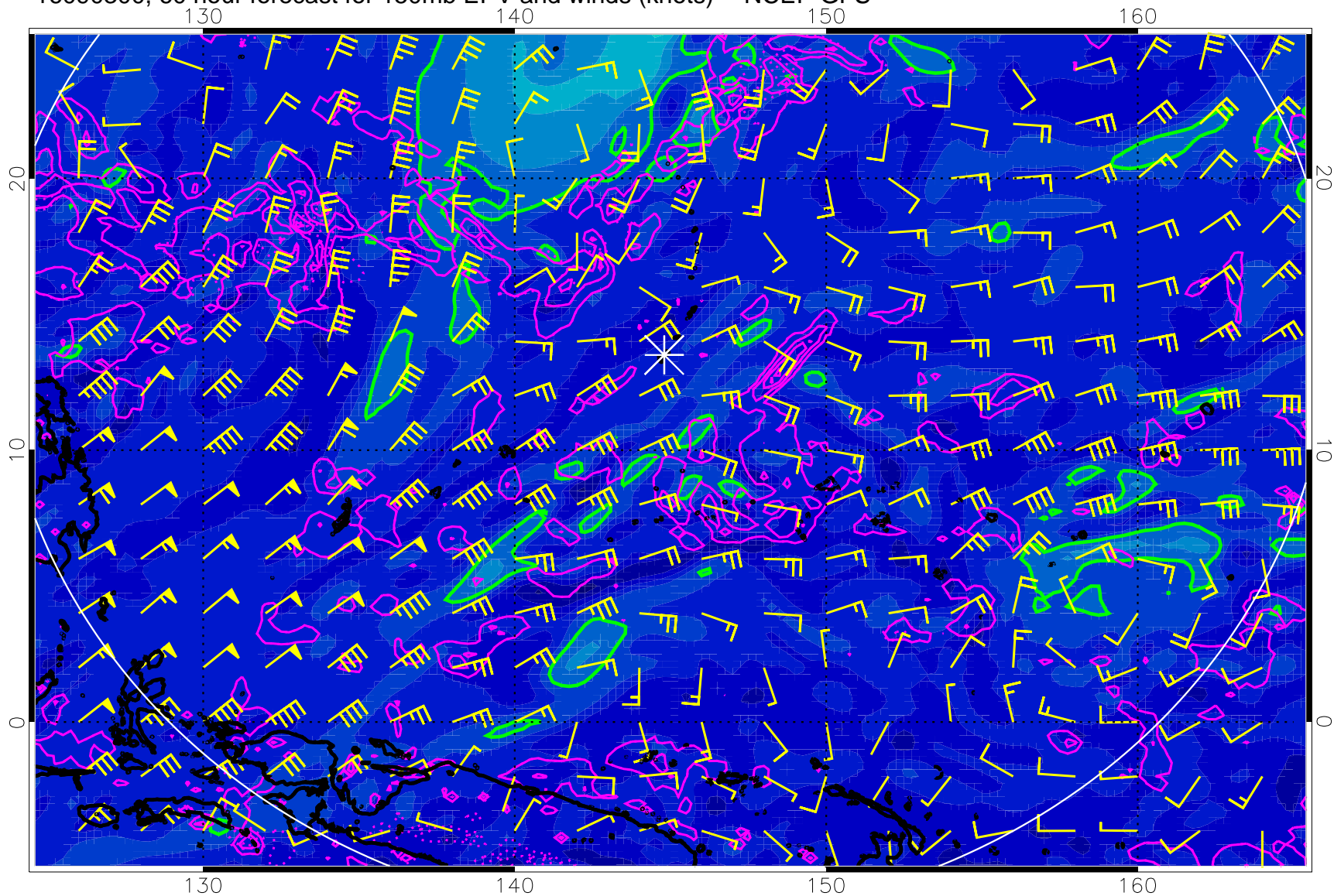
16090300, 60 hour forecast for 150mb EPV and winds (knots) -- NCEP GFS
