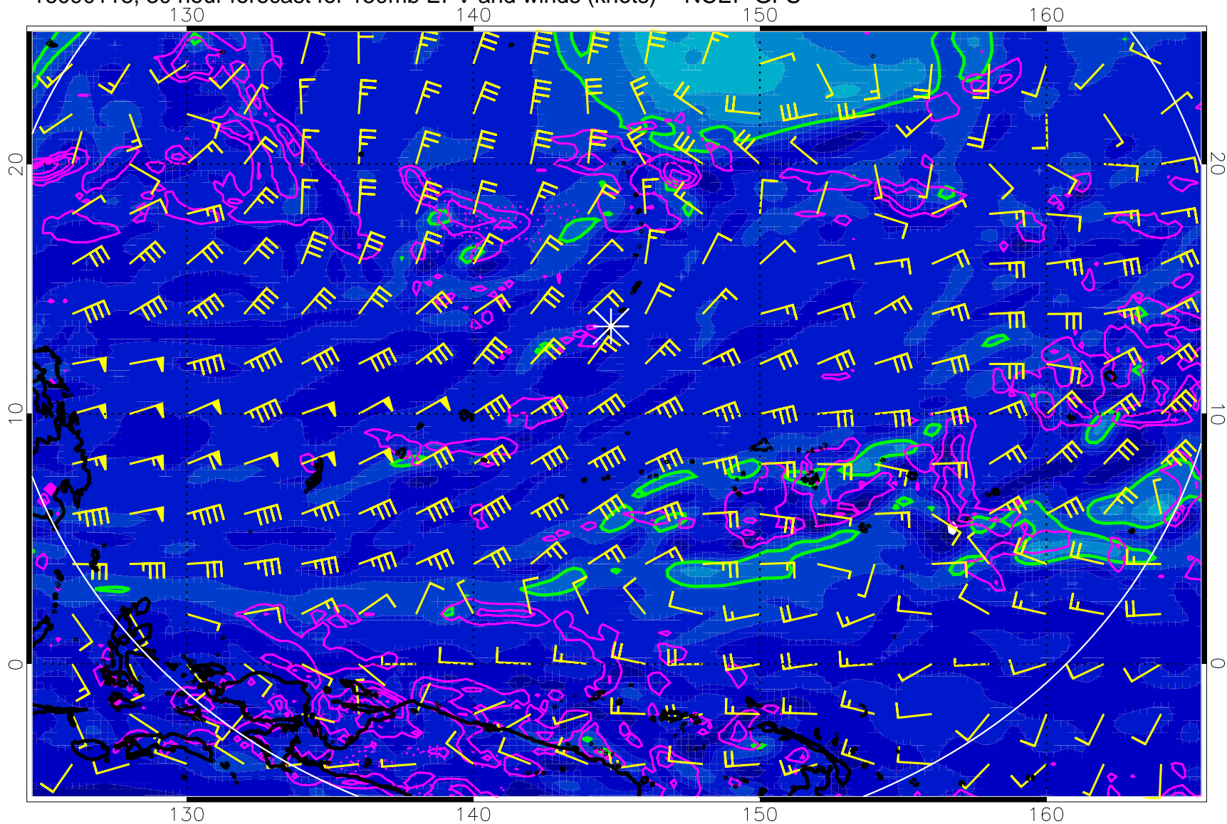
16090118, 30 hour forecast for 150mb EPV and winds (knots) -- NCEP GFS
