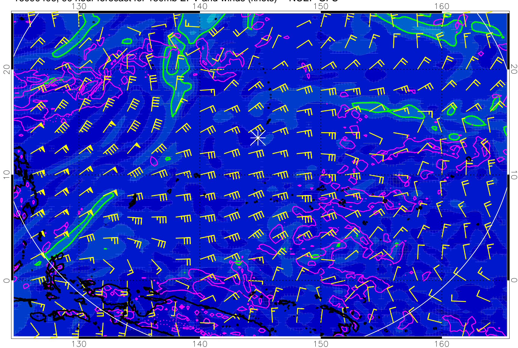
16090406, 90 hour forecast for 150mb EPV and winds (knots) -- NCEP GFS
