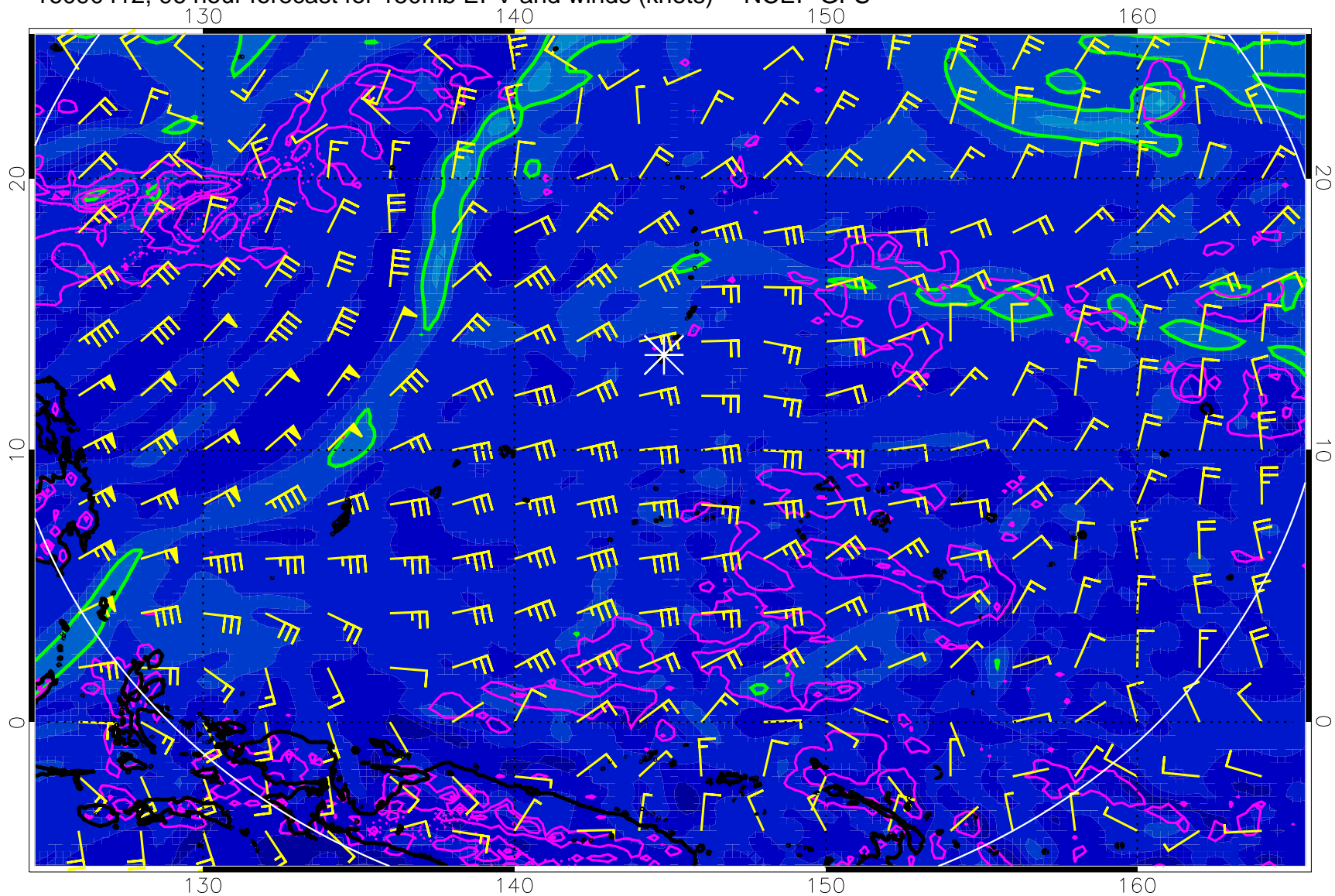
16090412, 96 hour forecast for 150mb EPV and winds (knots) -- NCEP GFS
