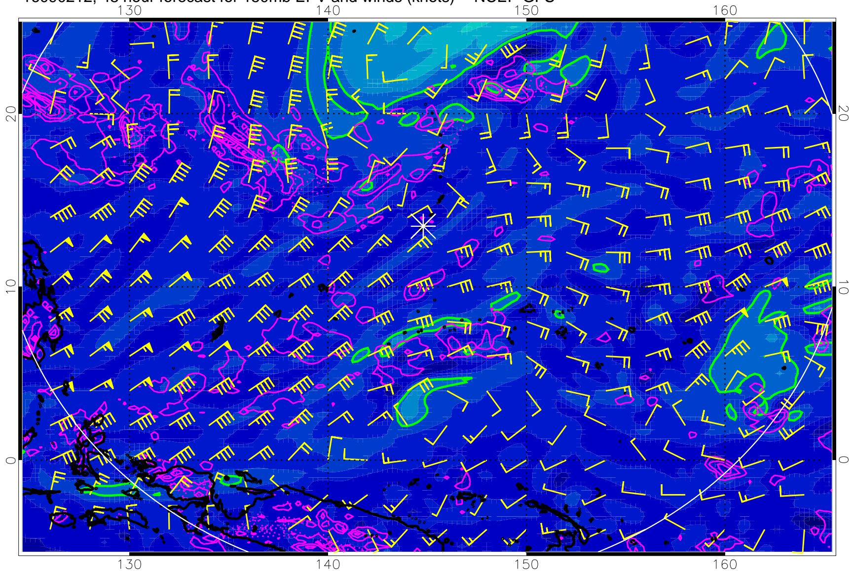
16090212, 48 hour forecast for 150mb EPV and winds (knots) -- NCEP GFS
