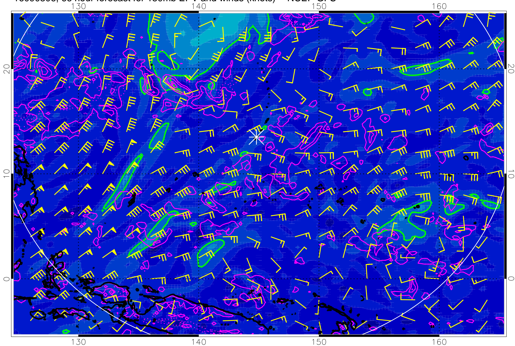
16090306, 66 hour forecast for 150mb EPV and winds (knots) -- NCEP GFS
