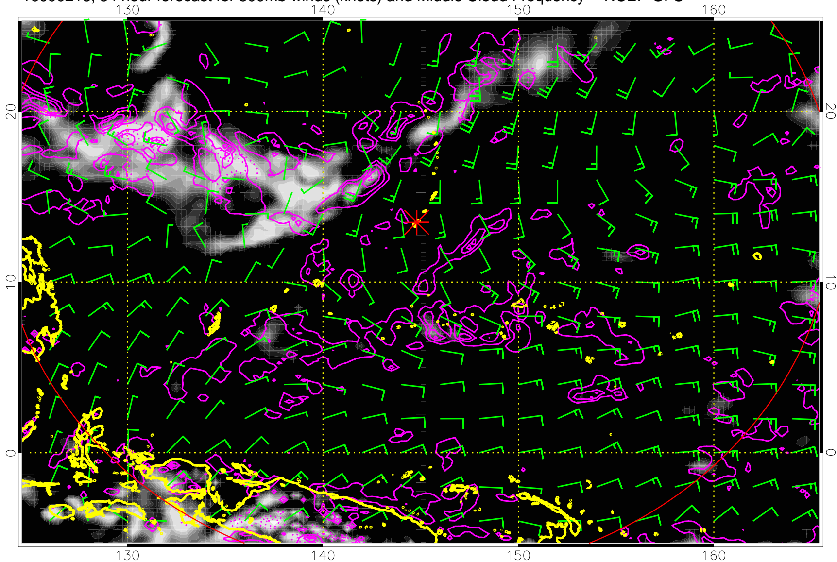
16090218, 54 hour forecast for 500mb winds (knots) and Middle Cloud Frequency -- NCEP GFS
