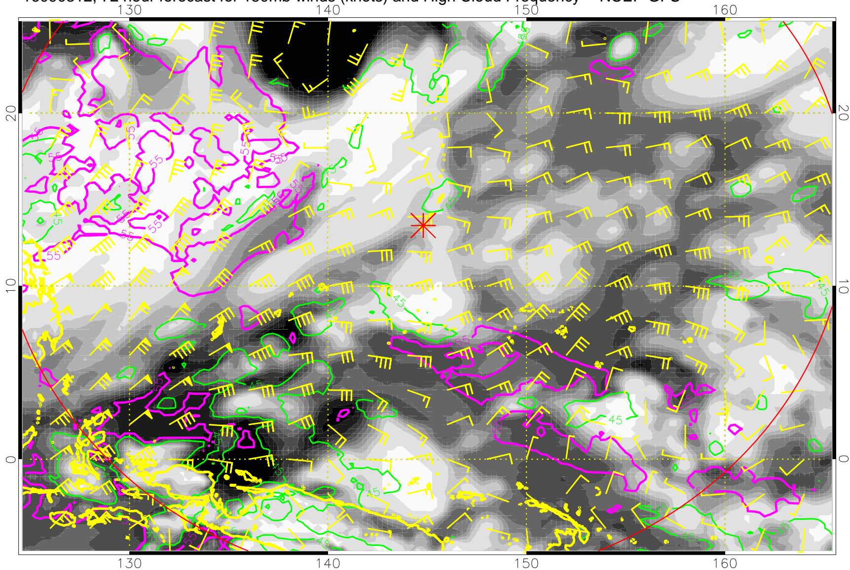
16090312, 72 hour forecast for 150mb winds (knots) and High Cloud Frequency -- NCEP GFS
