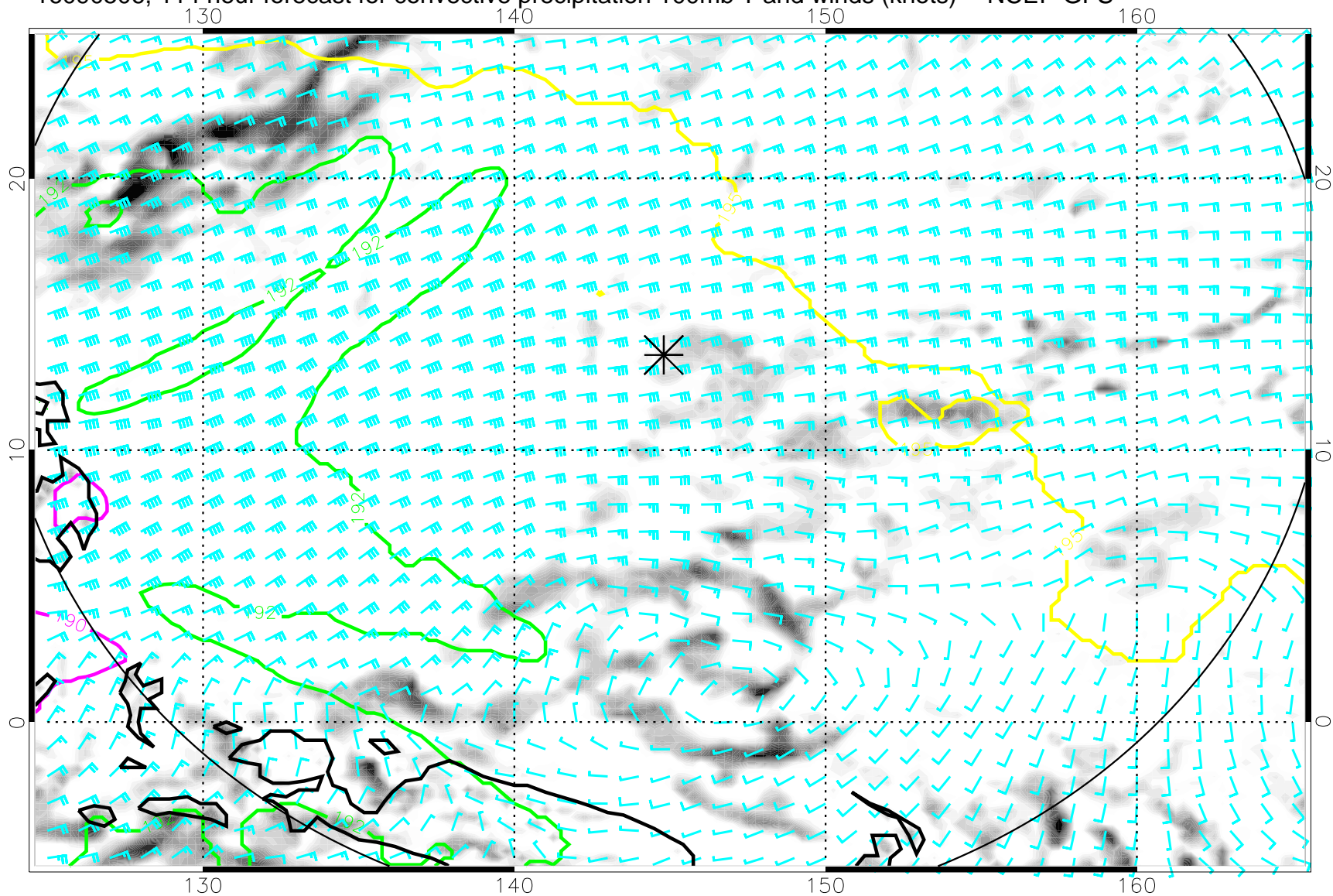
16090506, 114 hour forecast for convective precipitation 100mb T and winds (knots) -- NCEP GFS
