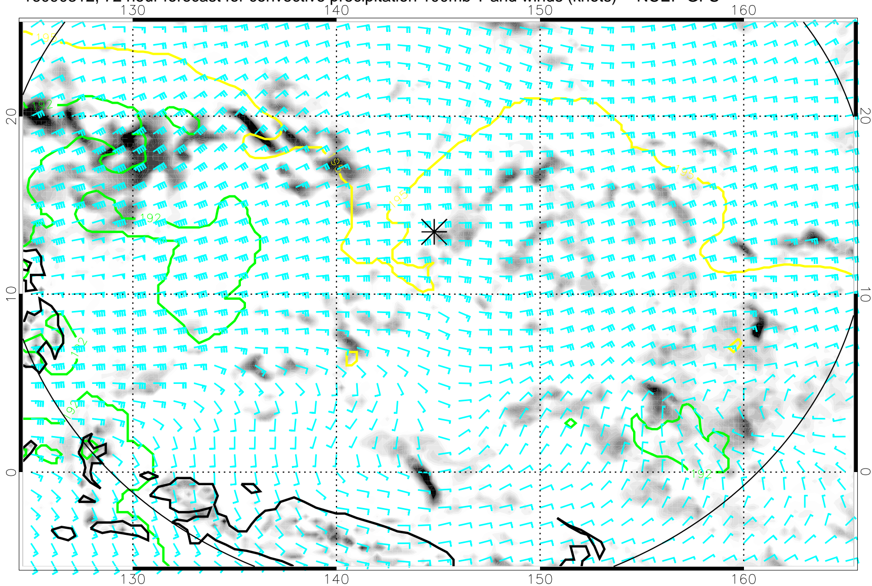
16090312, 72 hour forecast for convective precipitation 100mb T and winds (knots) -- NCEP GFS
