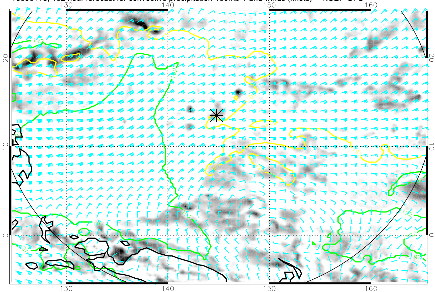
16090418, 102 hour forecast for convective precipitation 100mb T and winds (knots) -- NCEP GFS
