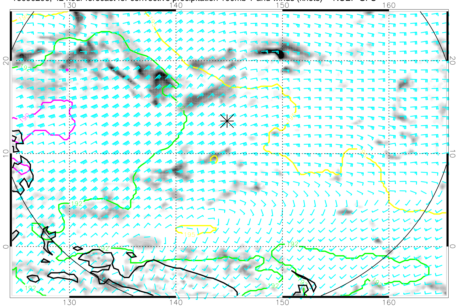
16090206, 42 hour forecast for convective precipitation 100mb T and winds (knots) -- NCEP GFS
