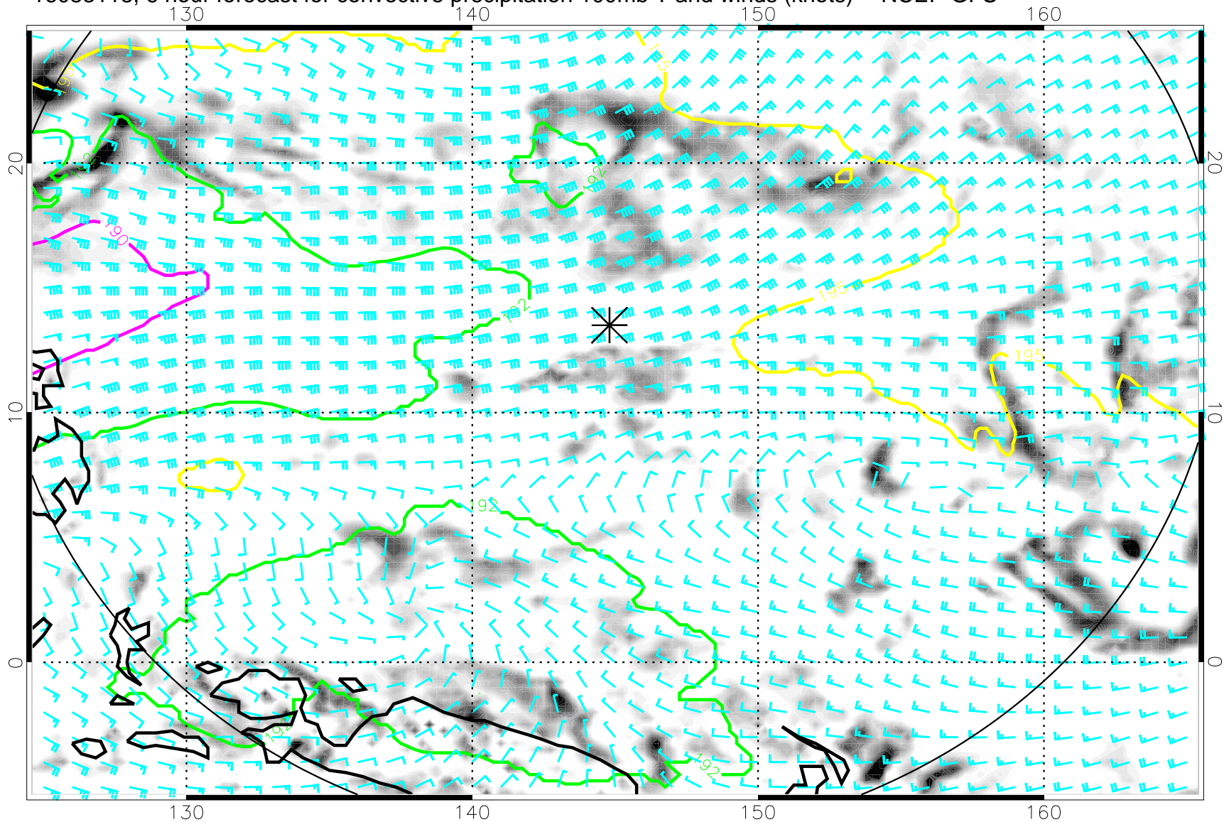
16083118, 6 hour forecast for convective precipitation 100mb T and winds (knots) -- NCEP GFS
