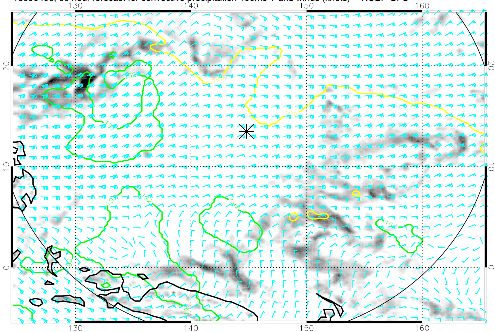
16090406, 90 hour forecast for convective precipitation 100mb T and winds (knots) -- NCEP GFS
