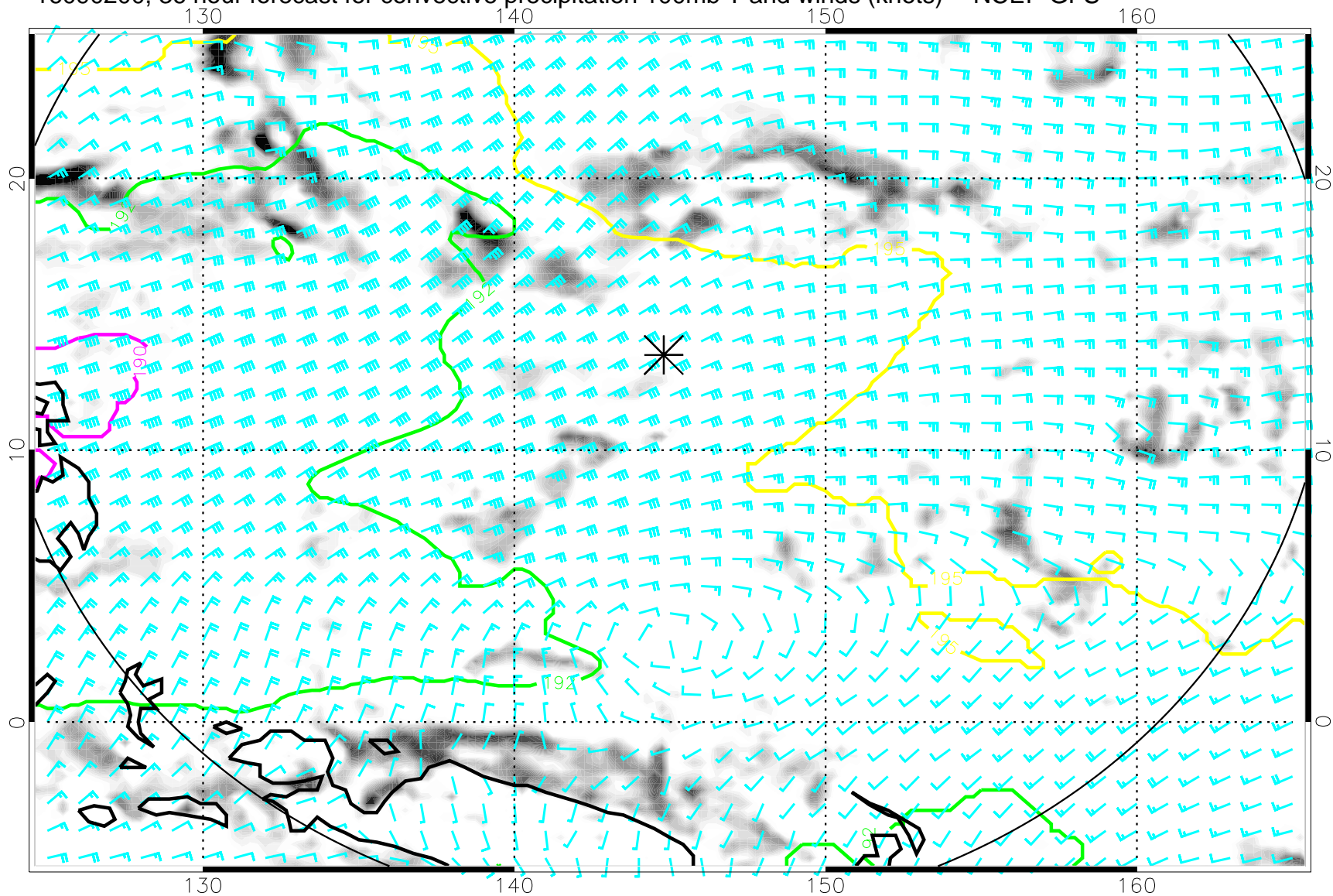
16090200, 36 hour forecast for convective precipitation 100mb T and winds (knots) -- NCEP GFS
