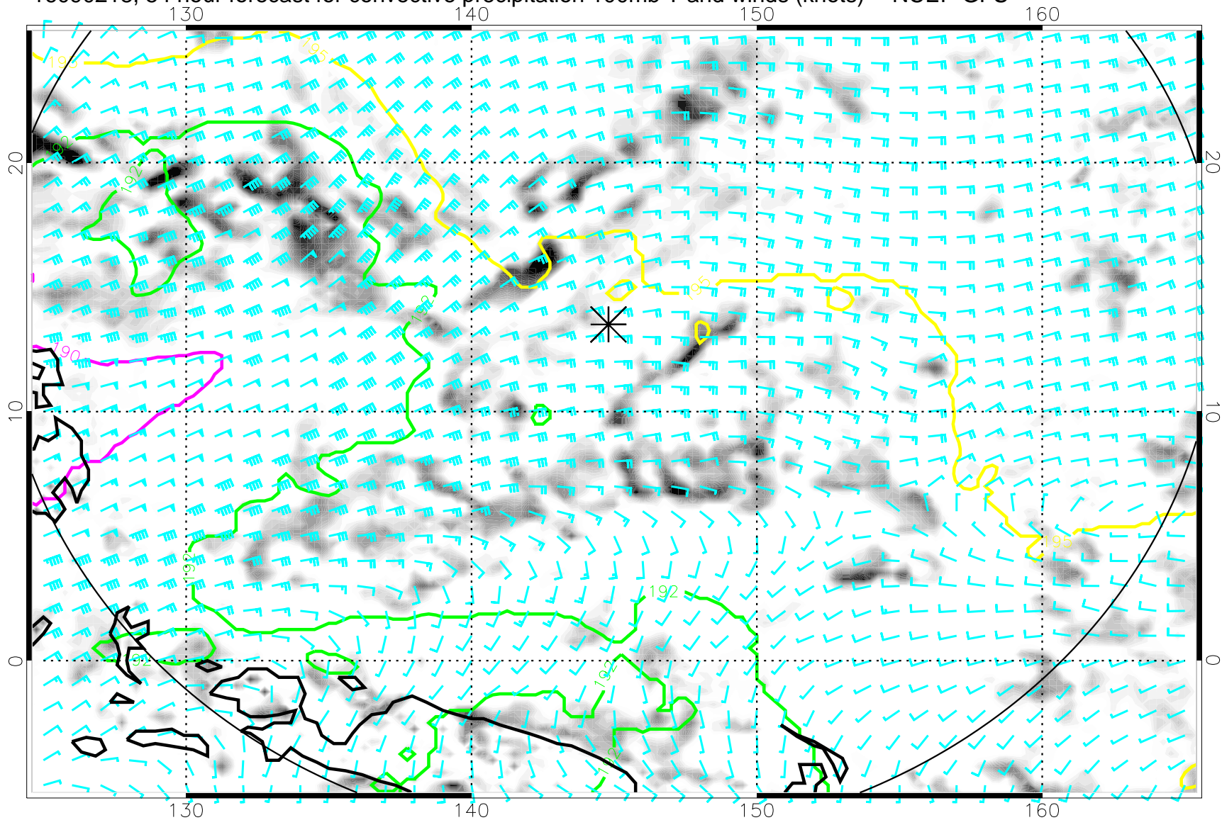
16090218, 54 hour forecast for convective precipitation 100mb T and winds (knots) -- NCEP GFS
