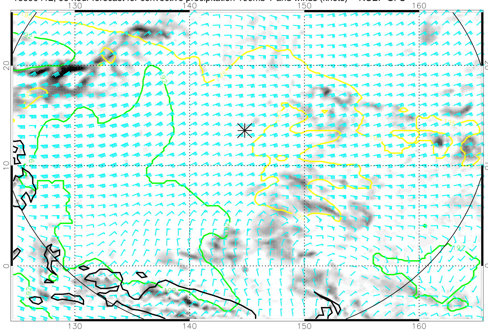
16090412, 96 hour forecast for convective precipitation 100mb T and winds (knots) -- NCEP GFS
