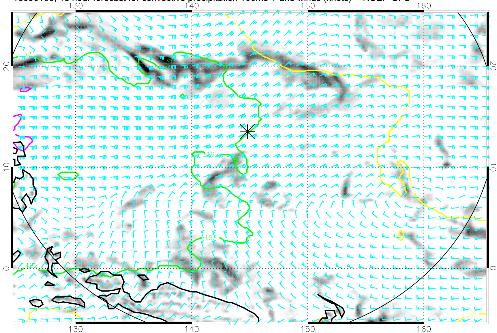
16090106, 18 hour forecast for convective precipitation 100mb T and winds (knots) -- NCEP GFS
