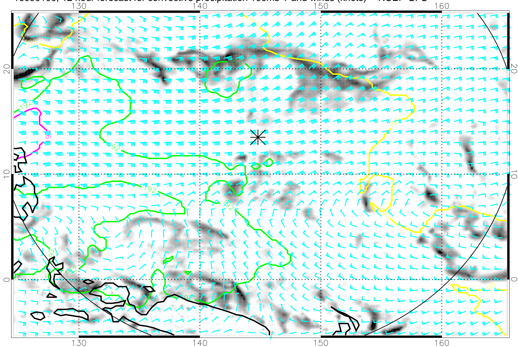
16090100, 12 hour forecast for convective precipitation 100mb T and winds (knots) -- NCEP GFS
