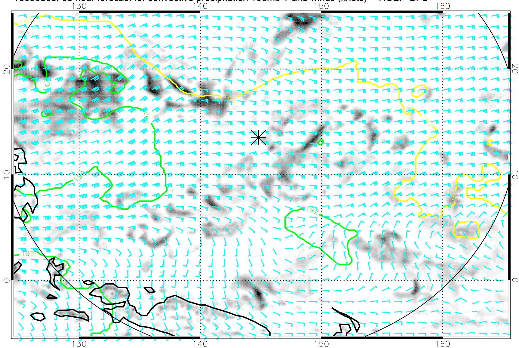
16090306, 66 hour forecast for convective precipitation 100mb T and winds (knots) -- NCEP GFS
