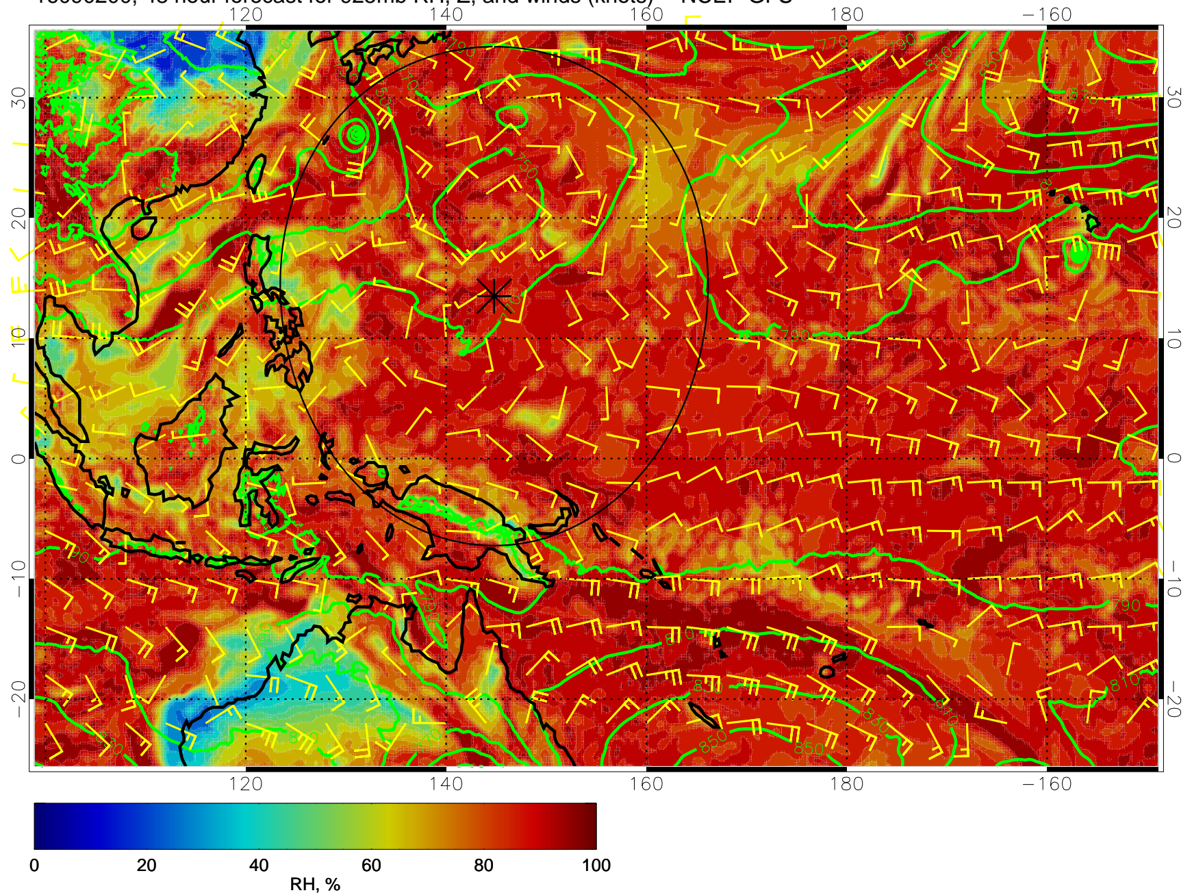
16090200, 48 hour forecast for 925mb RH, Z, and winds (knots) -- NCEP GFS
