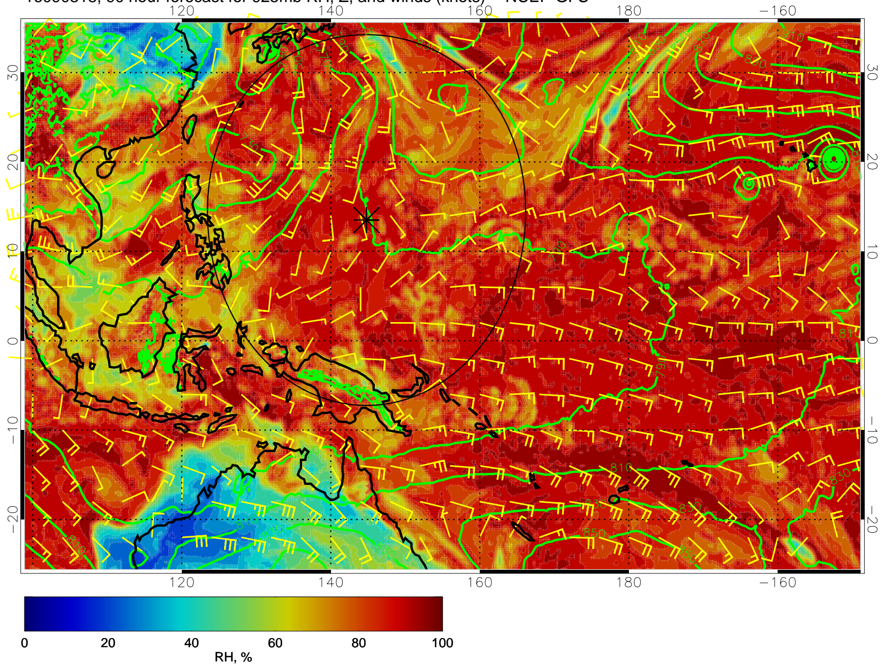
16090318, 90 hour forecast for 925mb RH, Z, and winds (knots) -- NCEP GFS
