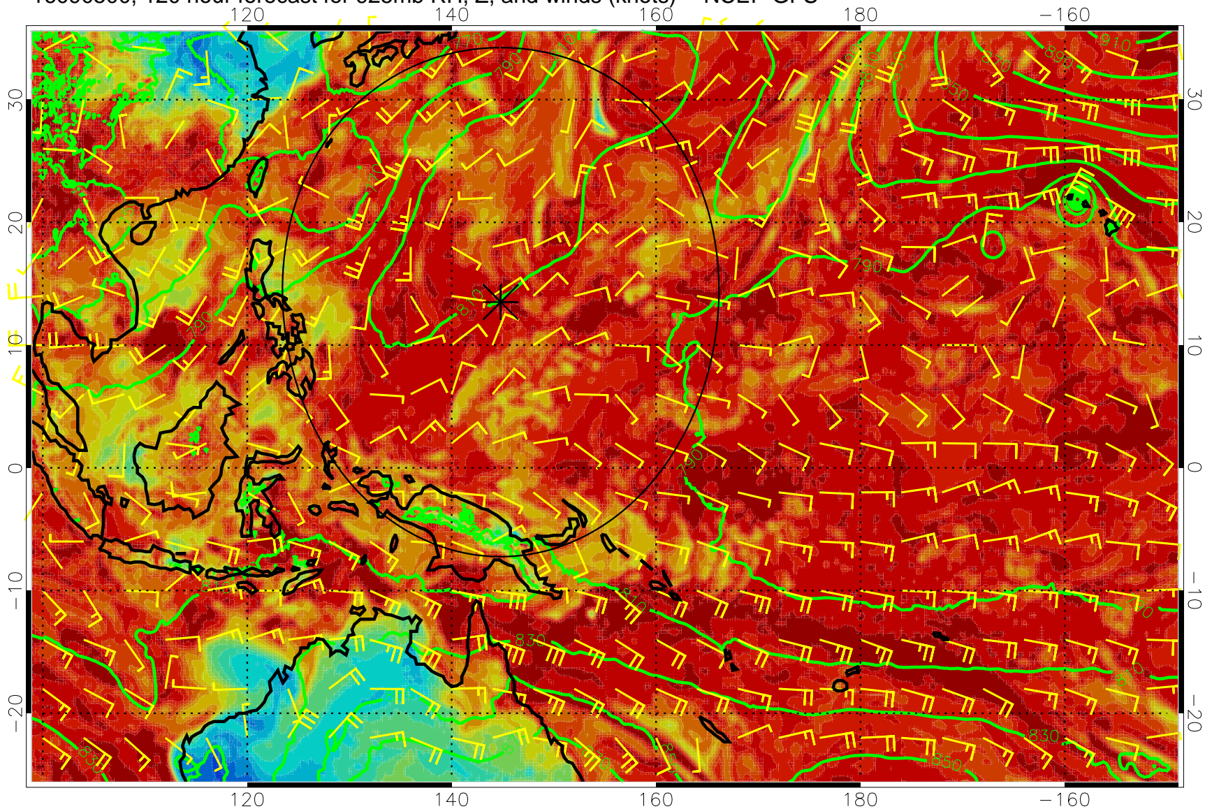
16090500, 120 hour forecast for 925mb RH, Z, and winds (knots) -- NCEP GFS
