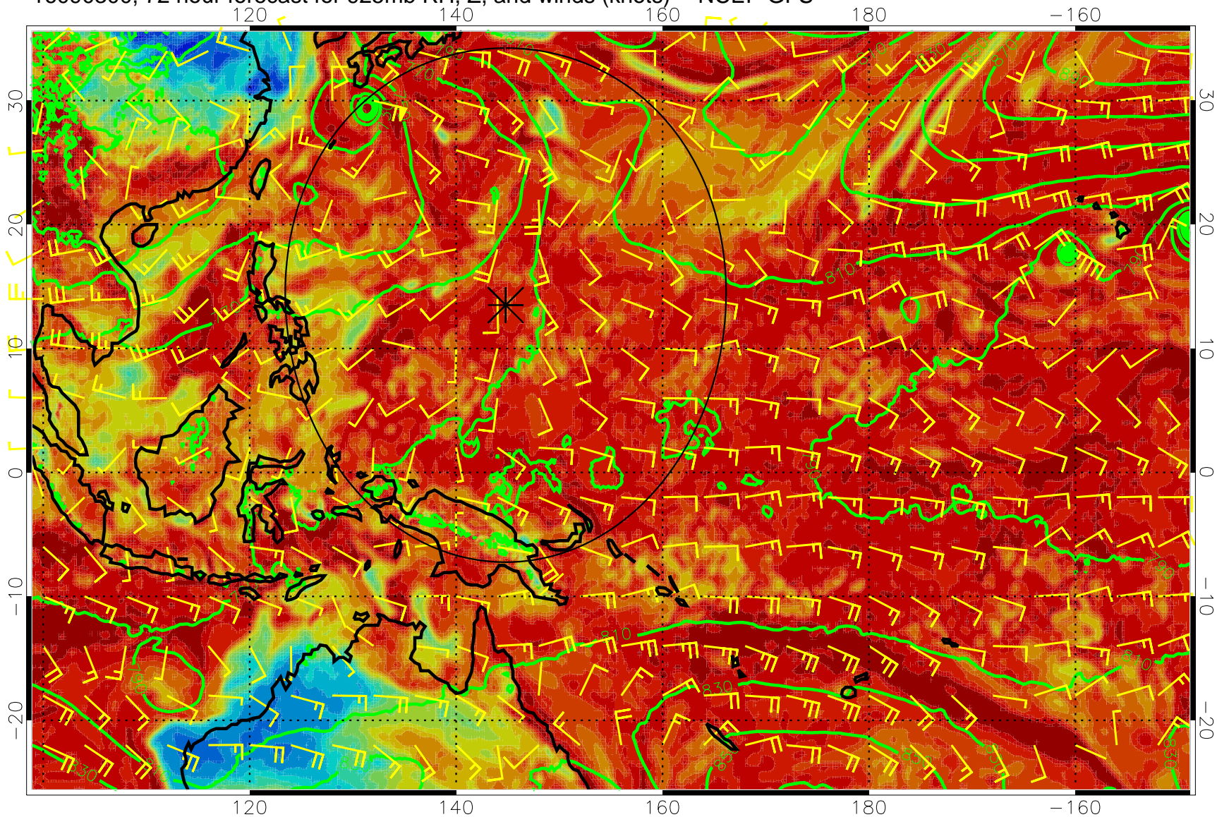
16090300, 72 hour forecast for 925mb RH, Z, and winds (knots) -- NCEP GFS
