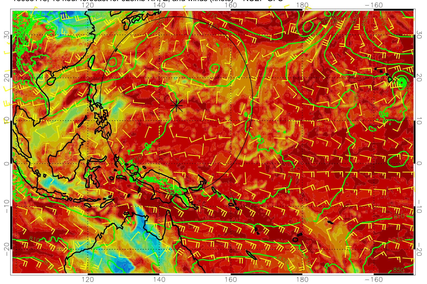
16083118, 18 hour forecast for 925mb RH, Z, and winds (knots) -- NCEP GFS
