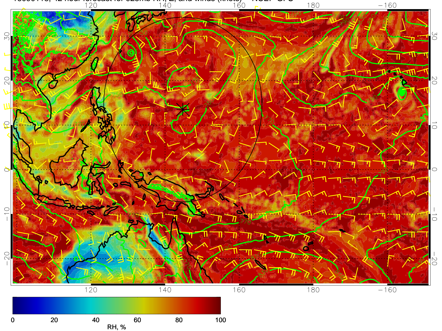
16090118, 42 hour forecast for 925mb RH, Z, and winds (knots) -- NCEP GFS
