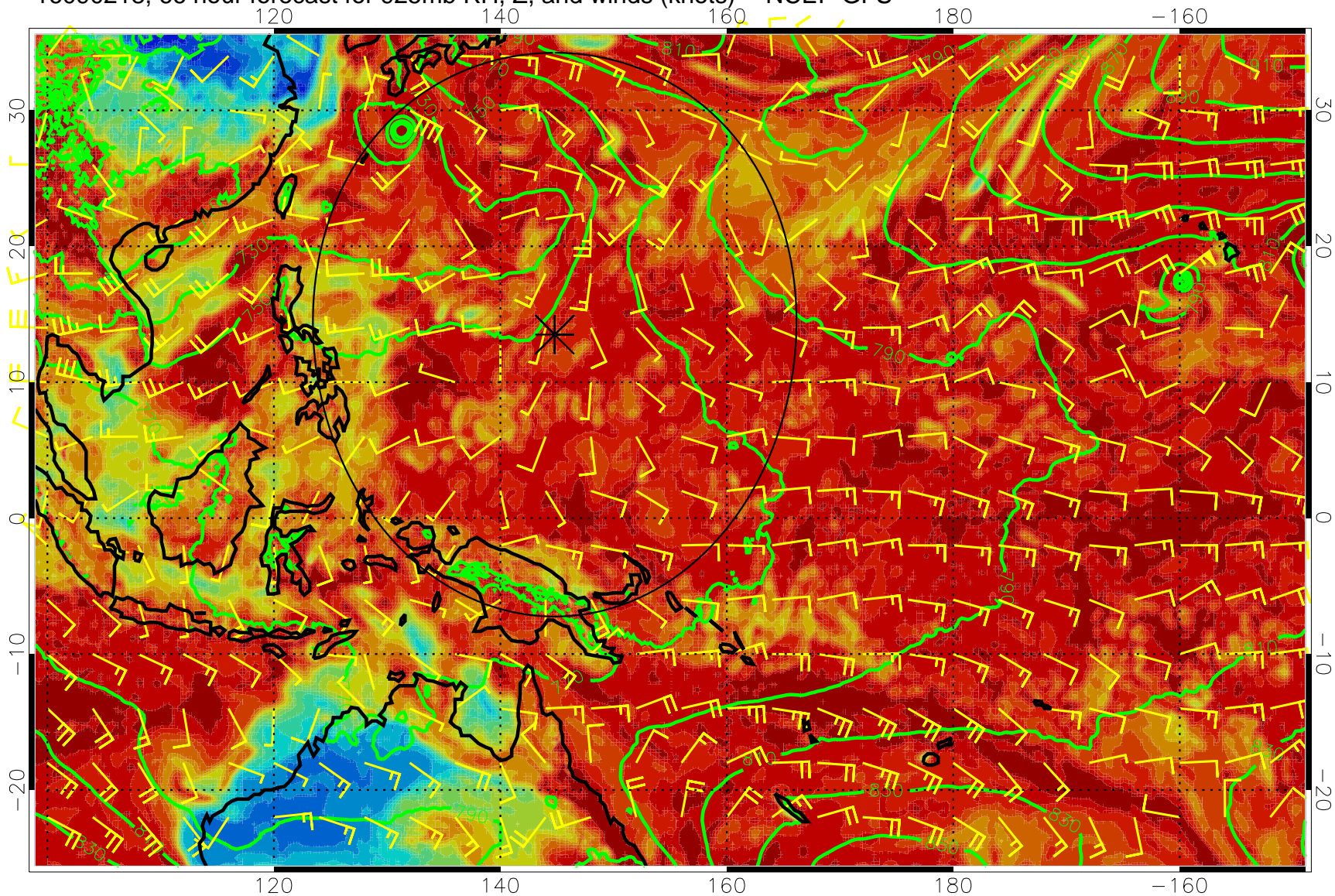
16090218, 66 hour forecast for 925mb RH, Z, and winds (knots) -- NCEP GFS
