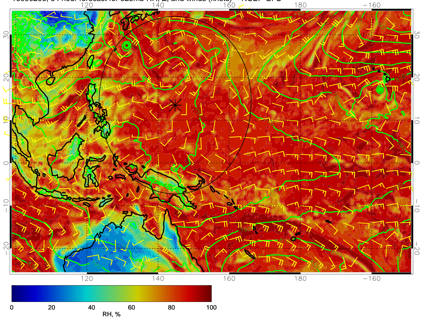
16090206, 54 hour forecast for 925mb RH, Z, and winds (knots) -- NCEP GFS
