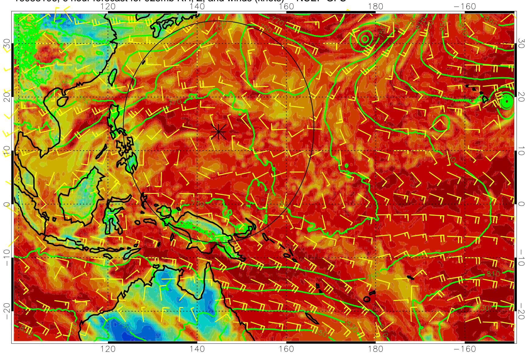
16083106, 6 hour forecast for 925mb RH, Z, and winds (knots) -- NCEP GFS
