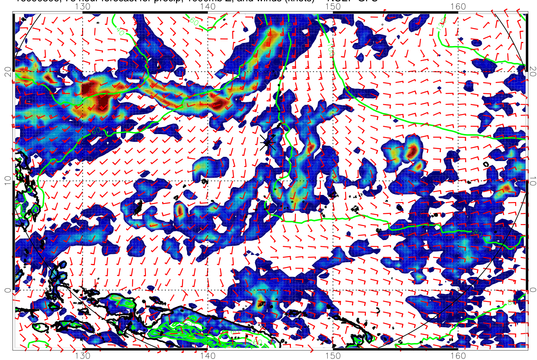
16090306, 78 hour forecast for precip, 1000mb Z, and winds (knots) -- NCEP GFS
