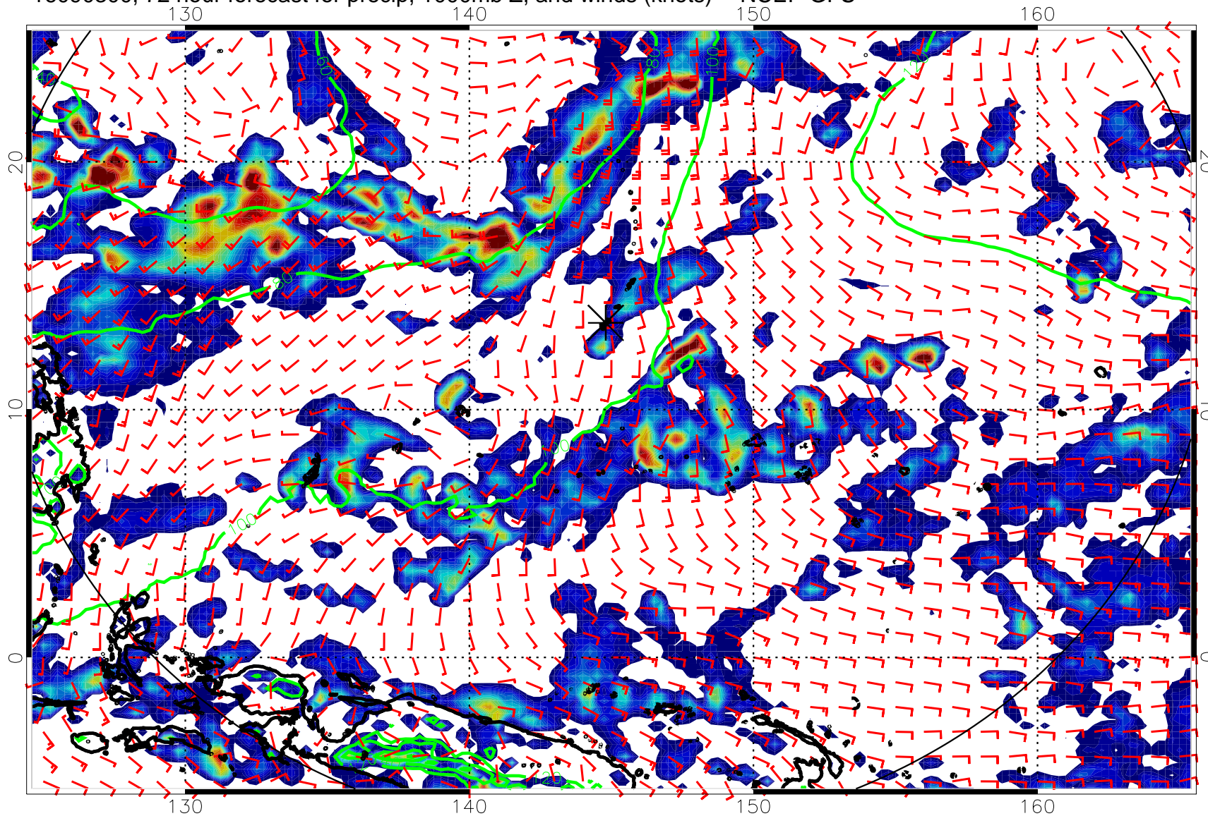
16090300, 72 hour forecast for precip, 1000mb Z, and winds (knots) -- NCEP GFS
