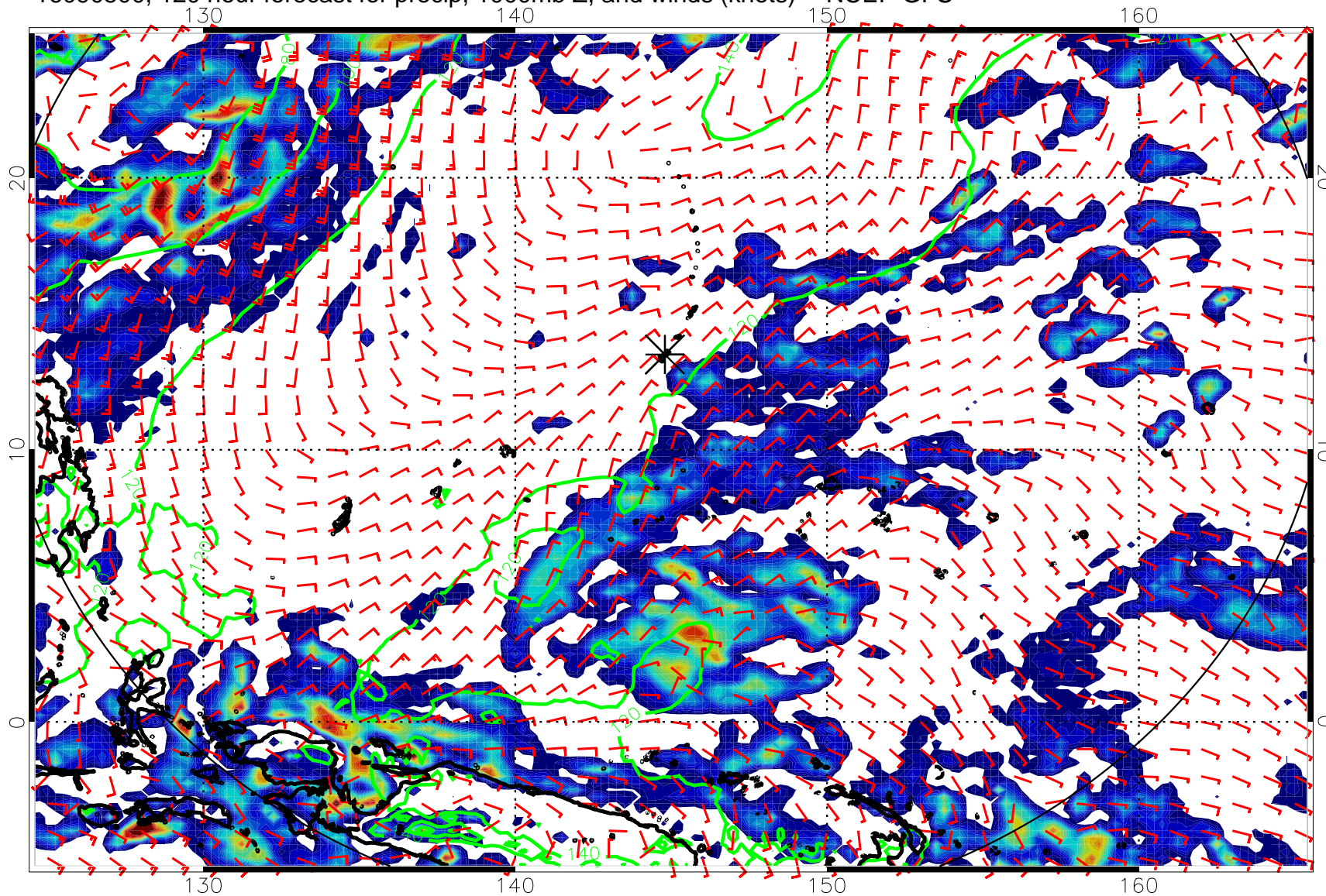
16090500, 120 hour forecast for precip, 1000mb Z, and winds (knots) -- NCEP GFS
