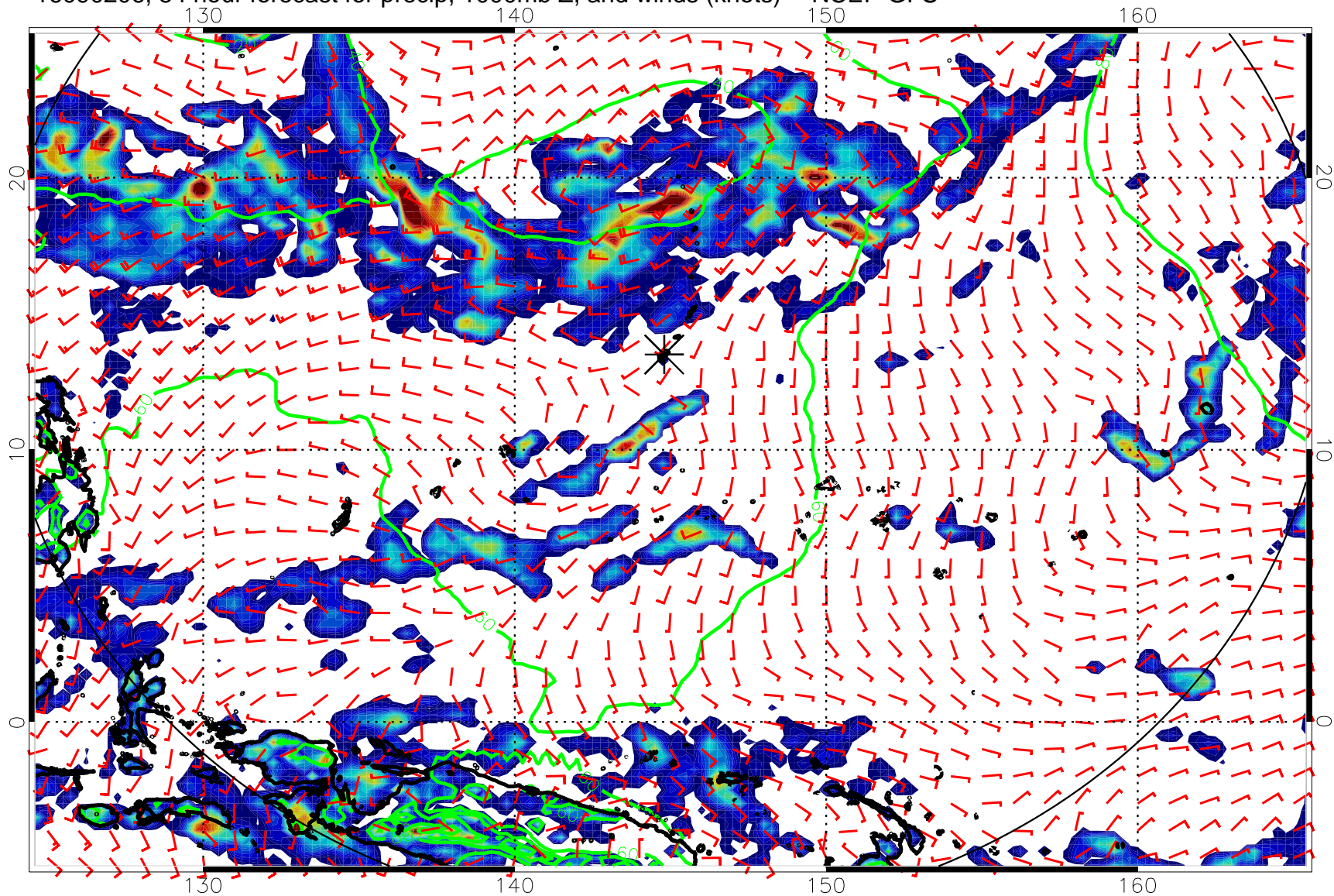
16090206, 54 hour forecast for precip, 1000mb Z, and winds (knots) -- NCEP GFS
