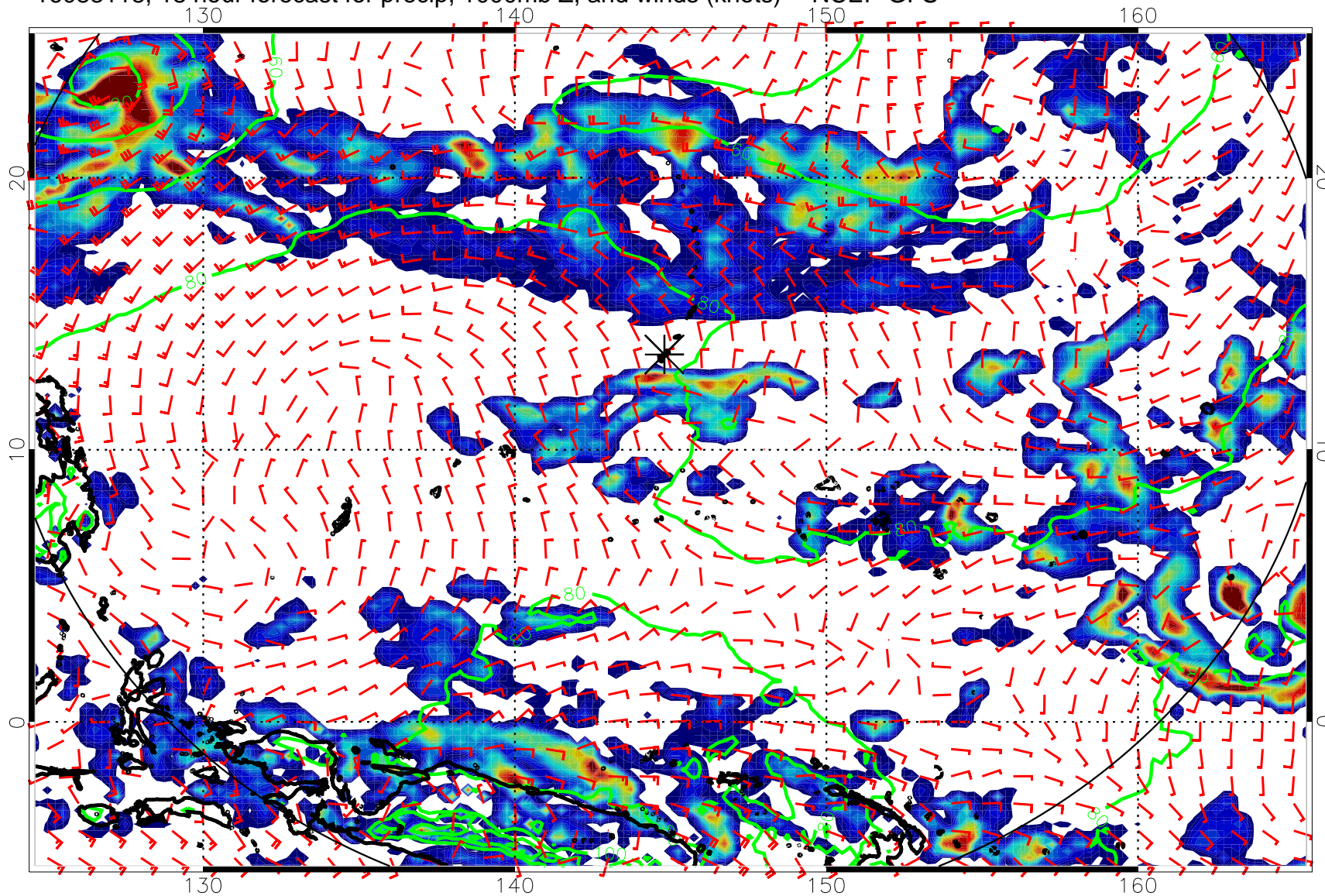
16083118, 18 hour forecast for precip, 1000mb Z, and winds (knots) -- NCEP GFS
