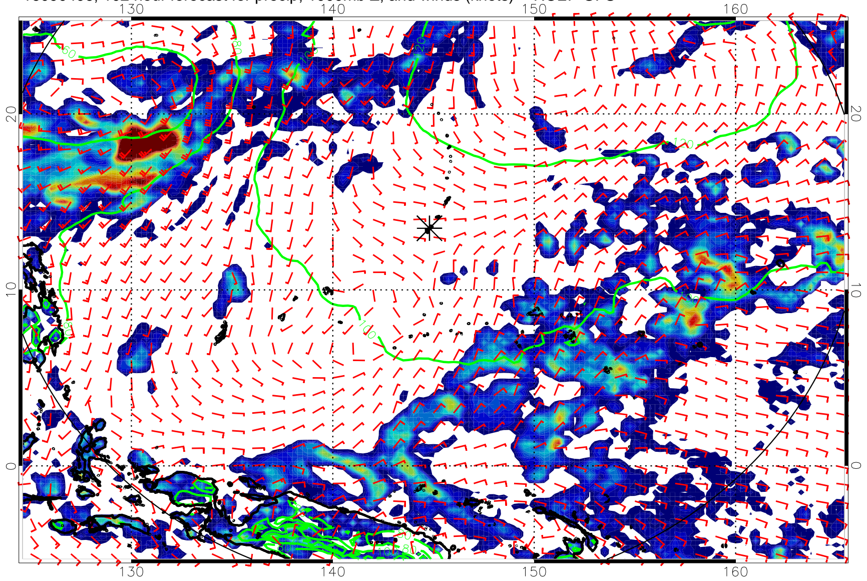
16090406, 102 hour forecast for precip, 1000mb Z, and winds (knots) -- NCEP GFS
