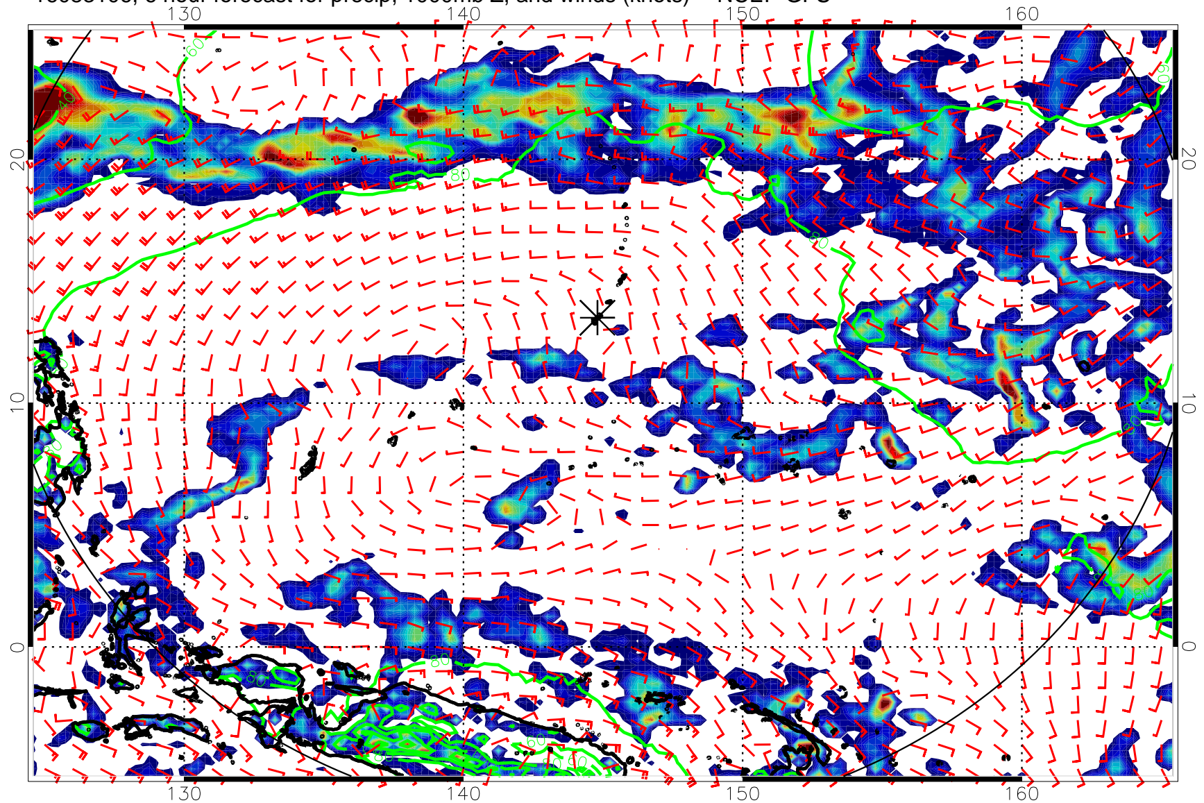
16083106, 6 hour forecast for precip, 1000mb Z, and winds (knots) -- NCEP GFS
