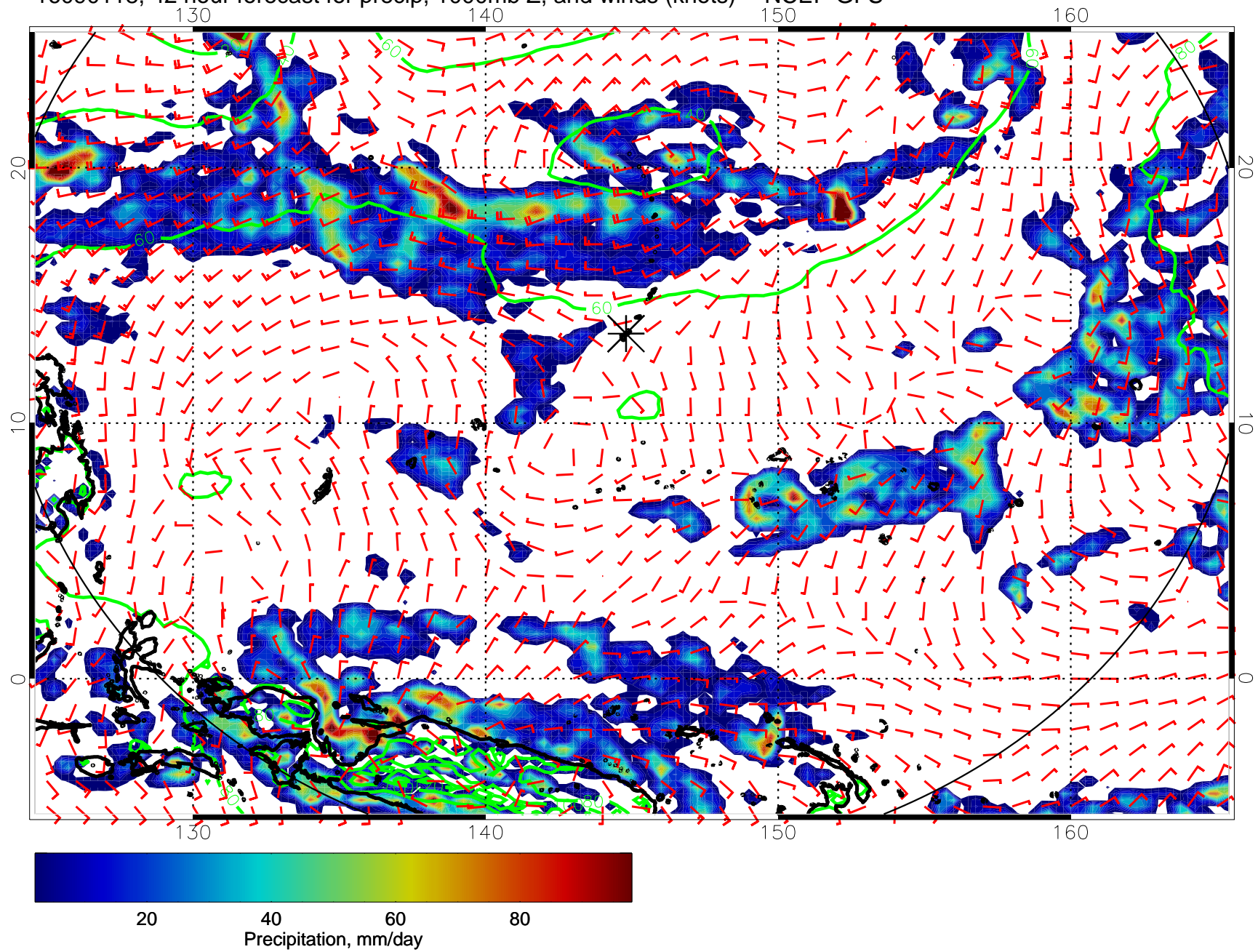
16090118, 42 hour forecast for precip, 1000mb Z, and winds (knots) -- NCEP GFS
