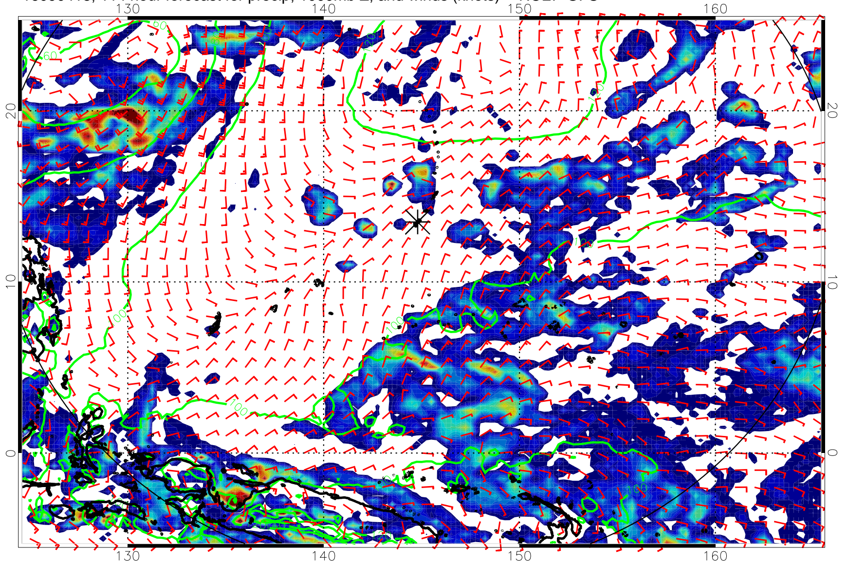
16090418, 114 hour forecast for precip, 1000mb Z, and winds (knots) -- NCEP GFS
