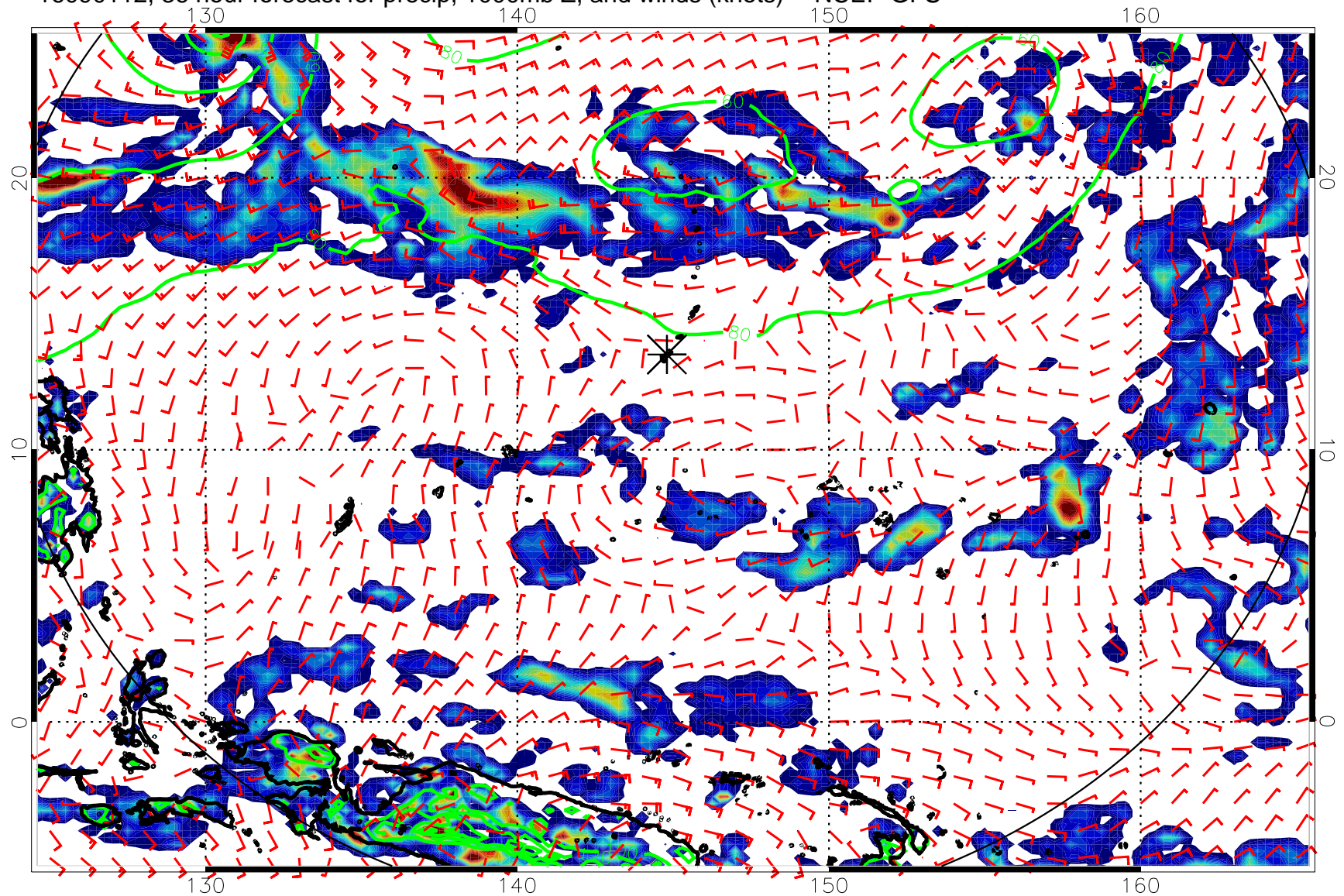
16090112, 36 hour forecast for precip, 1000mb Z, and winds (knots) -- NCEP GFS
