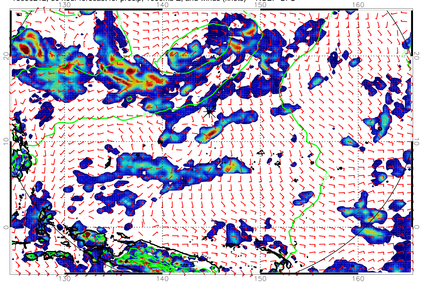
16090212, 60 hour forecast for precip, 1000mb Z, and winds (knots) -- NCEP GFS
