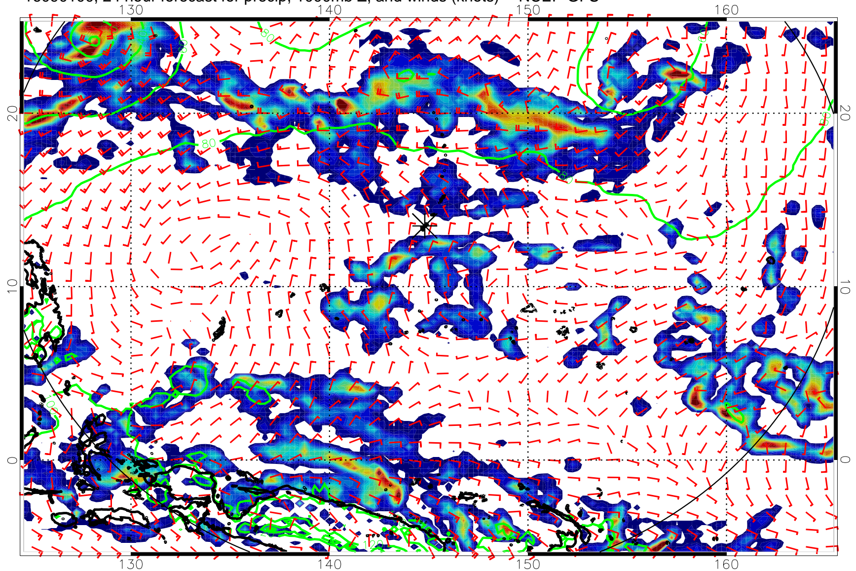
16090100, 24 hour forecast for precip, 1000mb Z, and winds (knots) -- NCEP GFS
