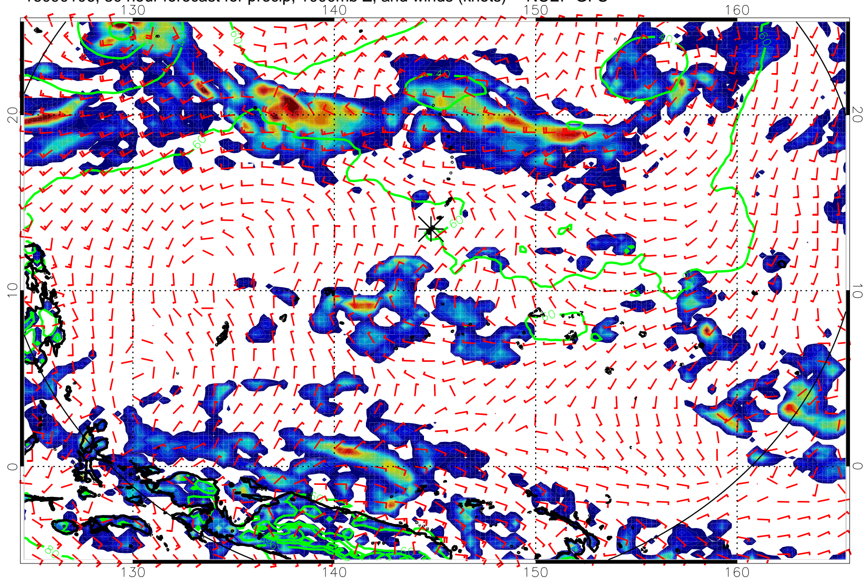
16090106, 30 hour forecast for precip, 1000mb Z, and winds (knots) -- NCEP GFS
