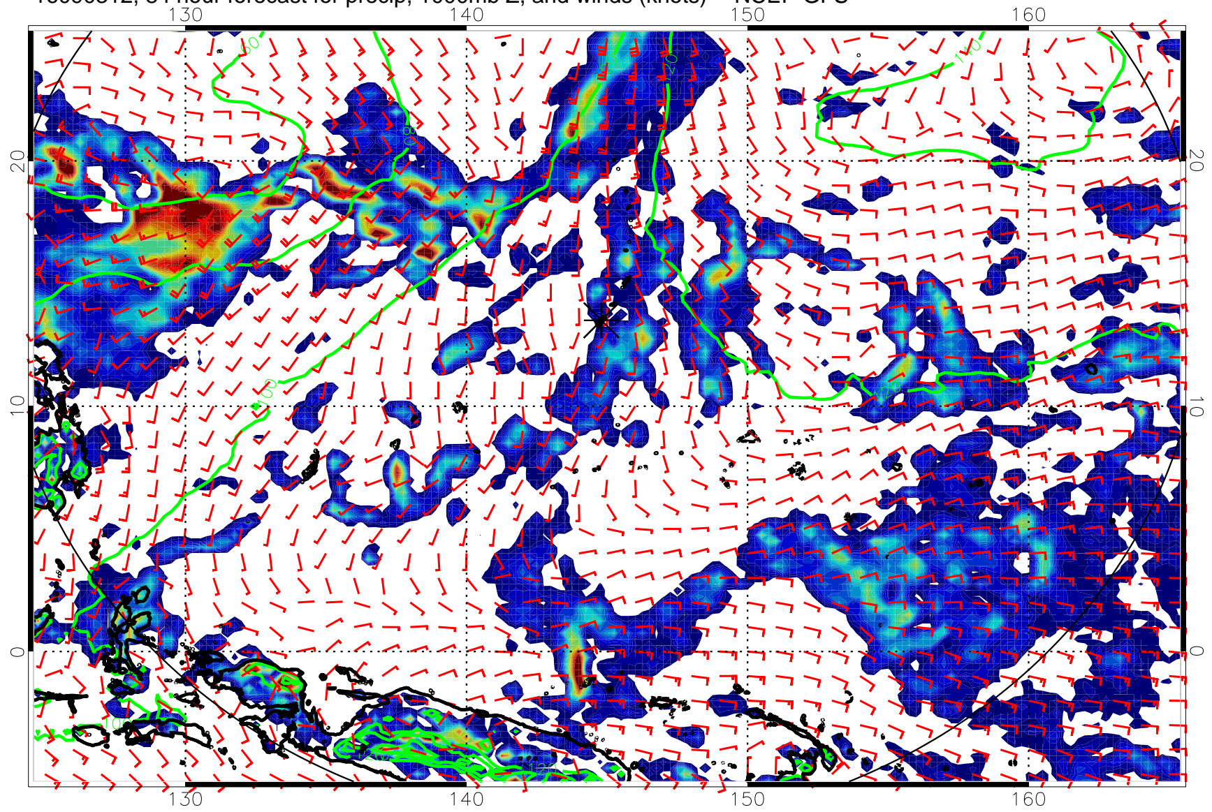
16090312, 84 hour forecast for precip, 1000mb Z, and winds (knots) -- NCEP GFS
