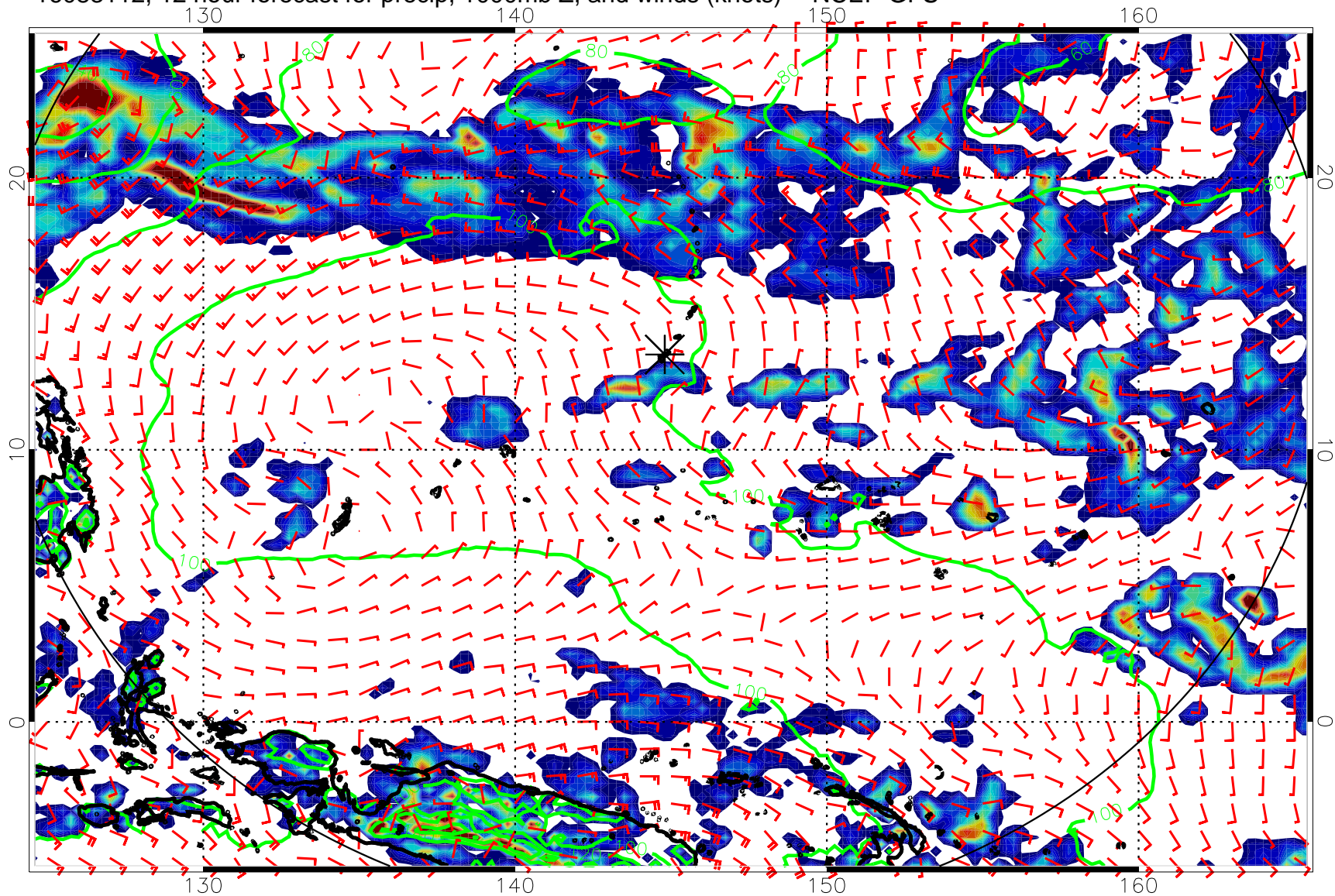
16083112, 12 hour forecast for precip, 1000mb Z, and winds (knots) -- NCEP GFS
