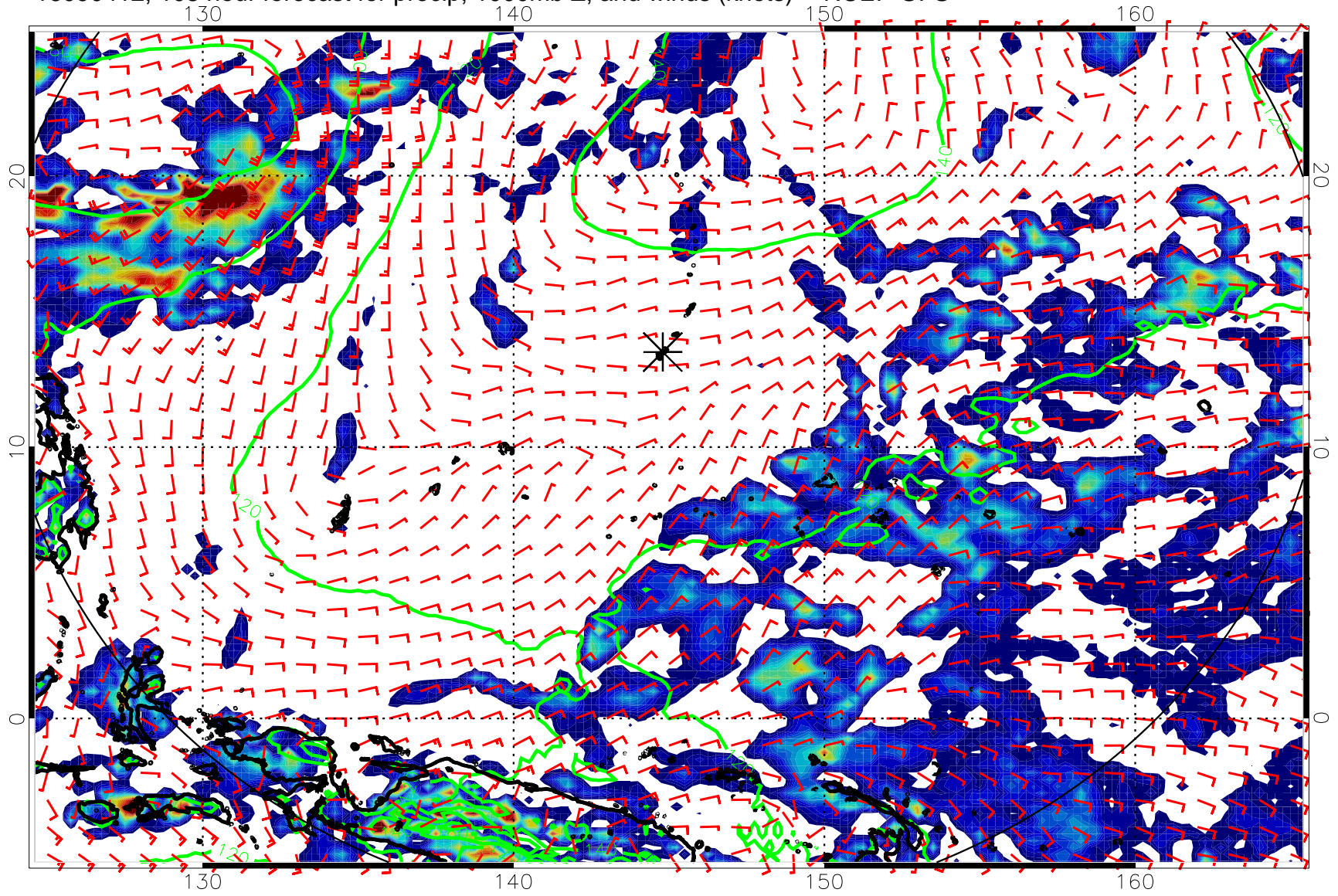
16090412, 108 hour forecast for precip, 1000mb Z, and winds (knots) -- NCEP GFS
