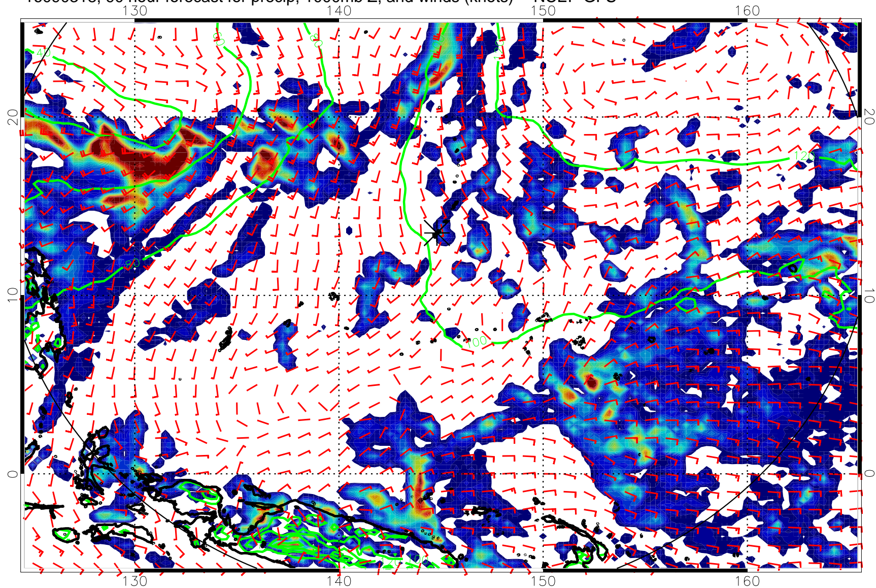
16090318, 90 hour forecast for precip, 1000mb Z, and winds (knots) -- NCEP GFS
