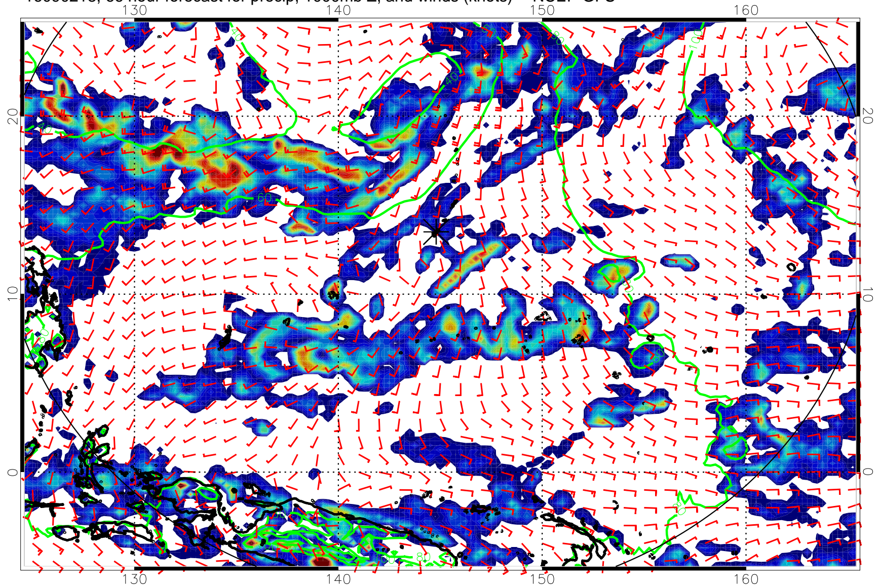
16090218, 66 hour forecast for precip, 1000mb Z, and winds (knots) -- NCEP GFS
