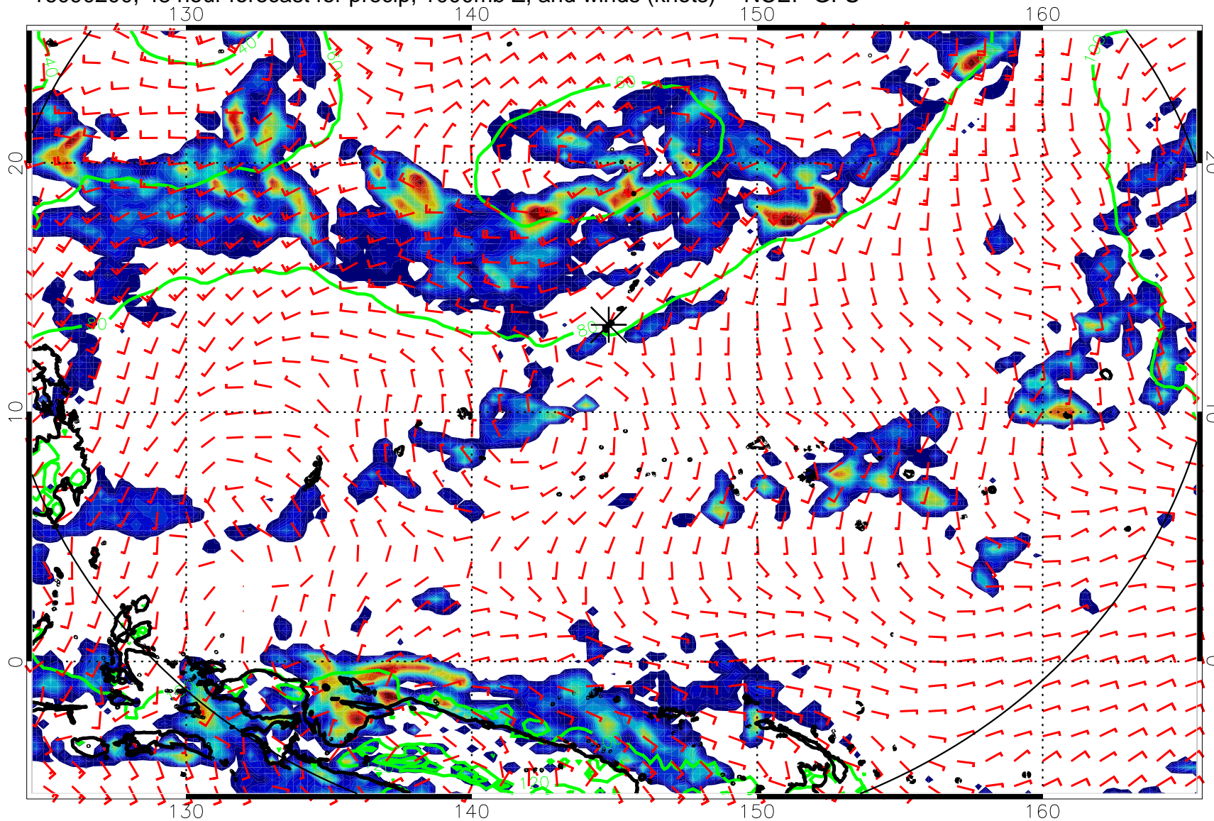
16090200, 48 hour forecast for precip, 1000mb Z, and winds (knots) -- NCEP GFS
