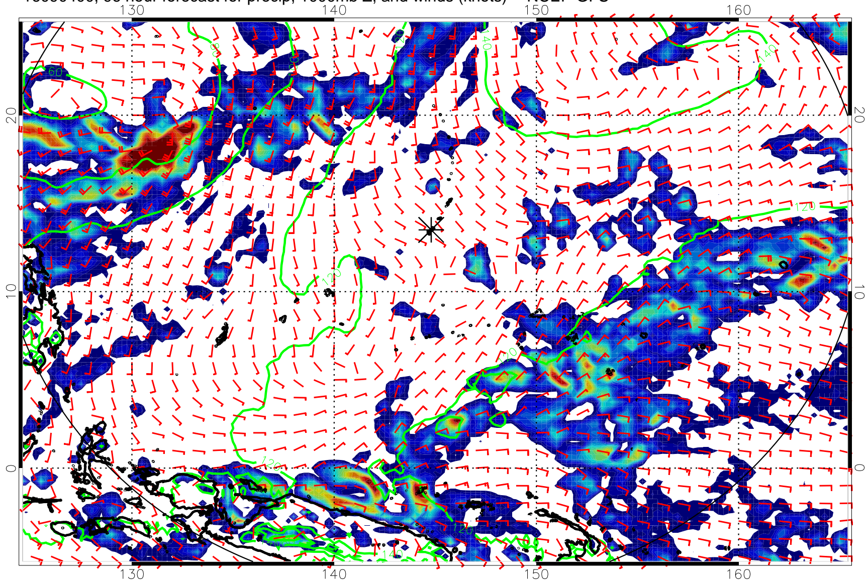
16090400, 96 hour forecast for precip, 1000mb Z, and winds (knots) -- NCEP GFS
