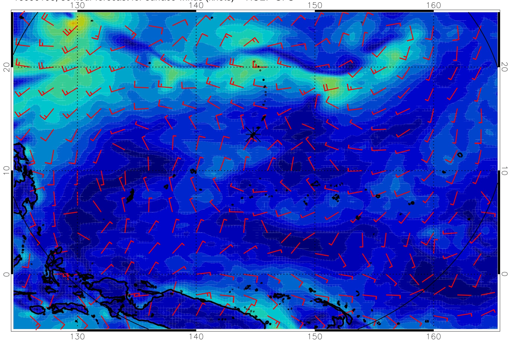
16090106, 30 hour forecast for surface winds (knots) -- NCEP GFS
