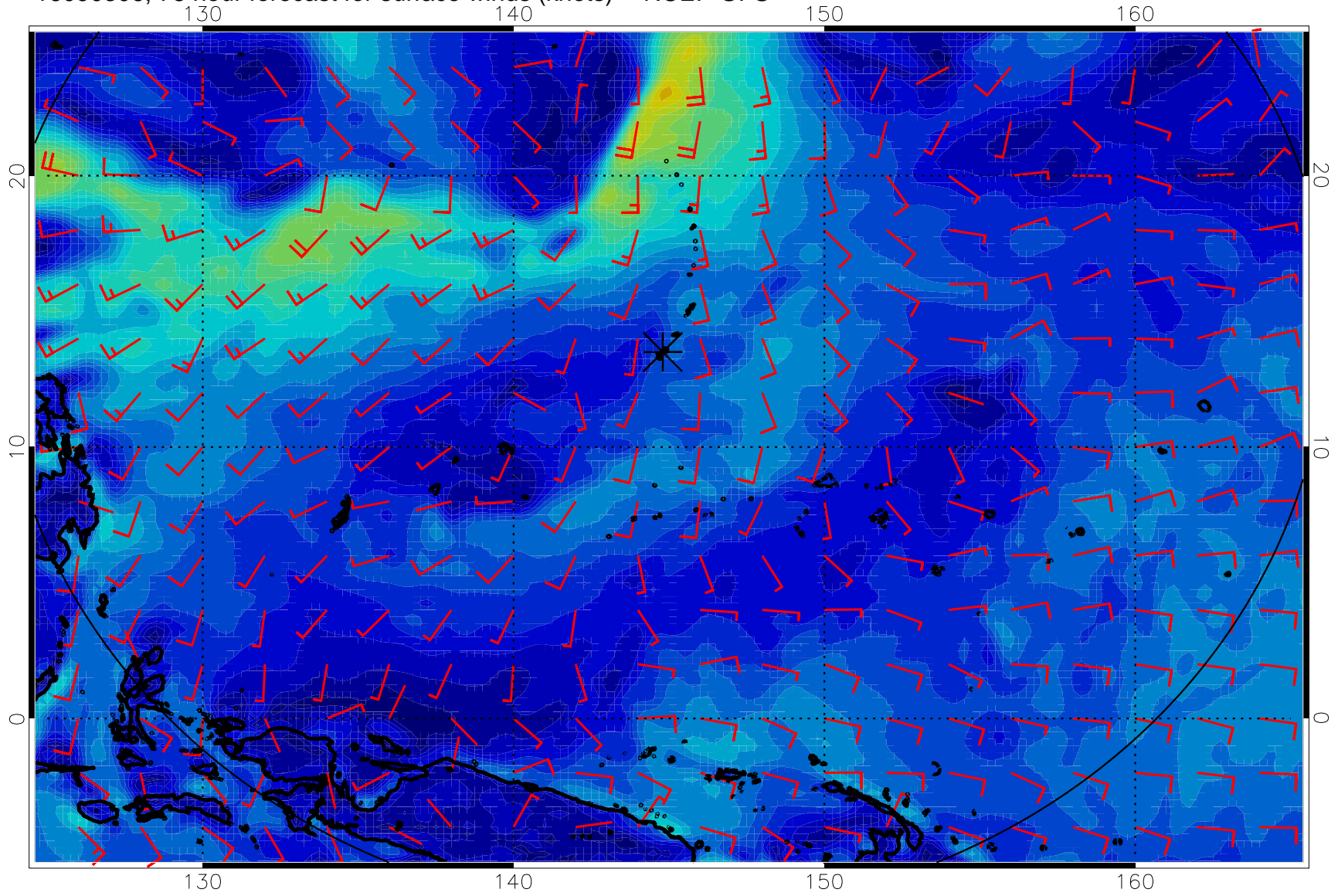
16090306, 78 hour forecast for surface winds (knots) -- NCEP GFS
