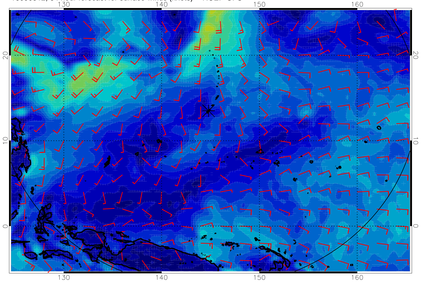
16090312, 84 hour forecast for surface winds (knots) -- NCEP GFS
