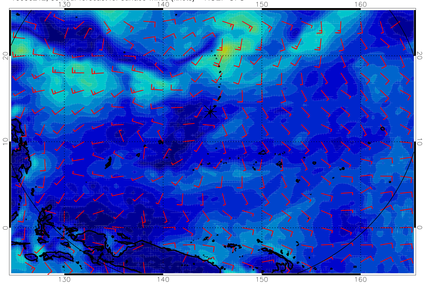
16090212, 60 hour forecast for surface winds (knots) -- NCEP GFS
