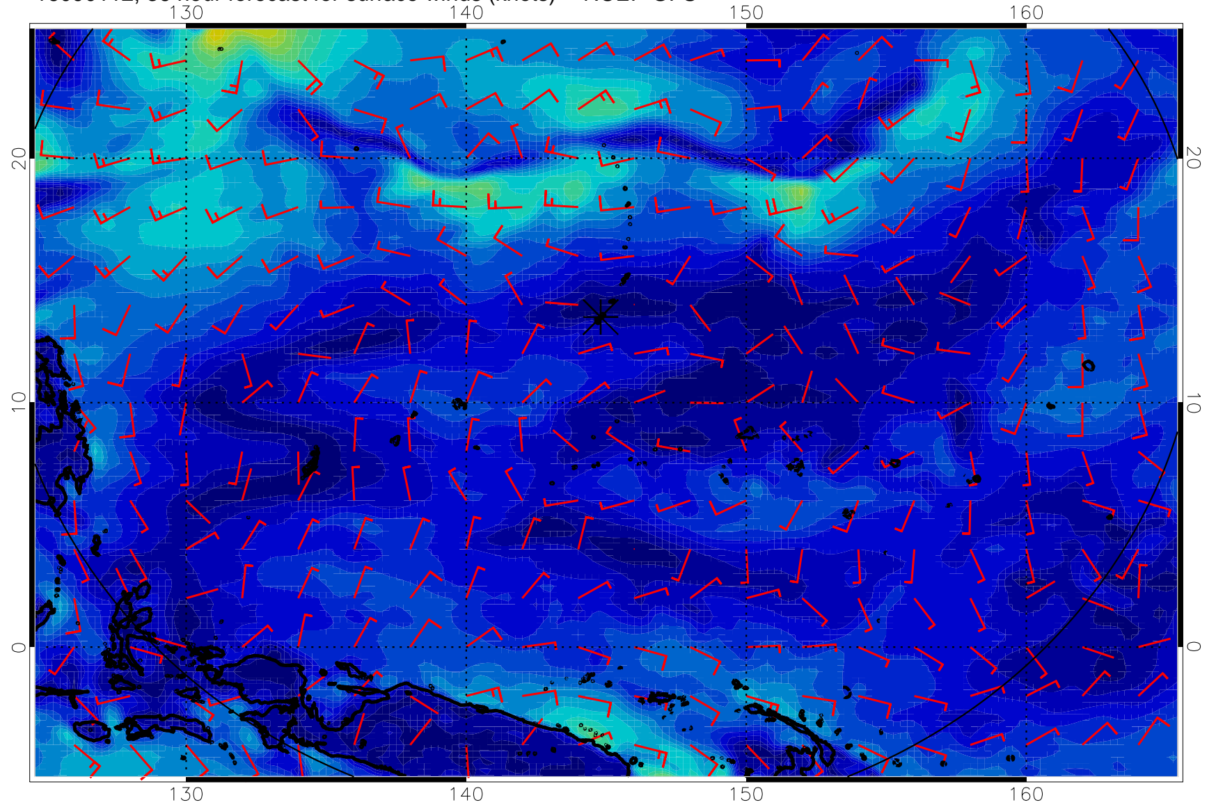
16090112, 36 hour forecast for surface winds (knots) -- NCEP GFS
