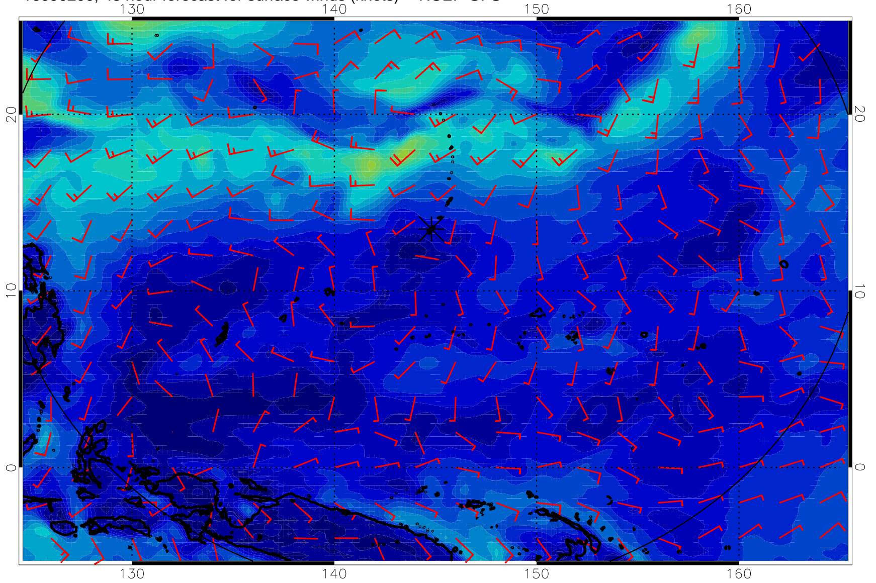
16090200, 48 hour forecast for surface winds (knots) -- NCEP GFS
