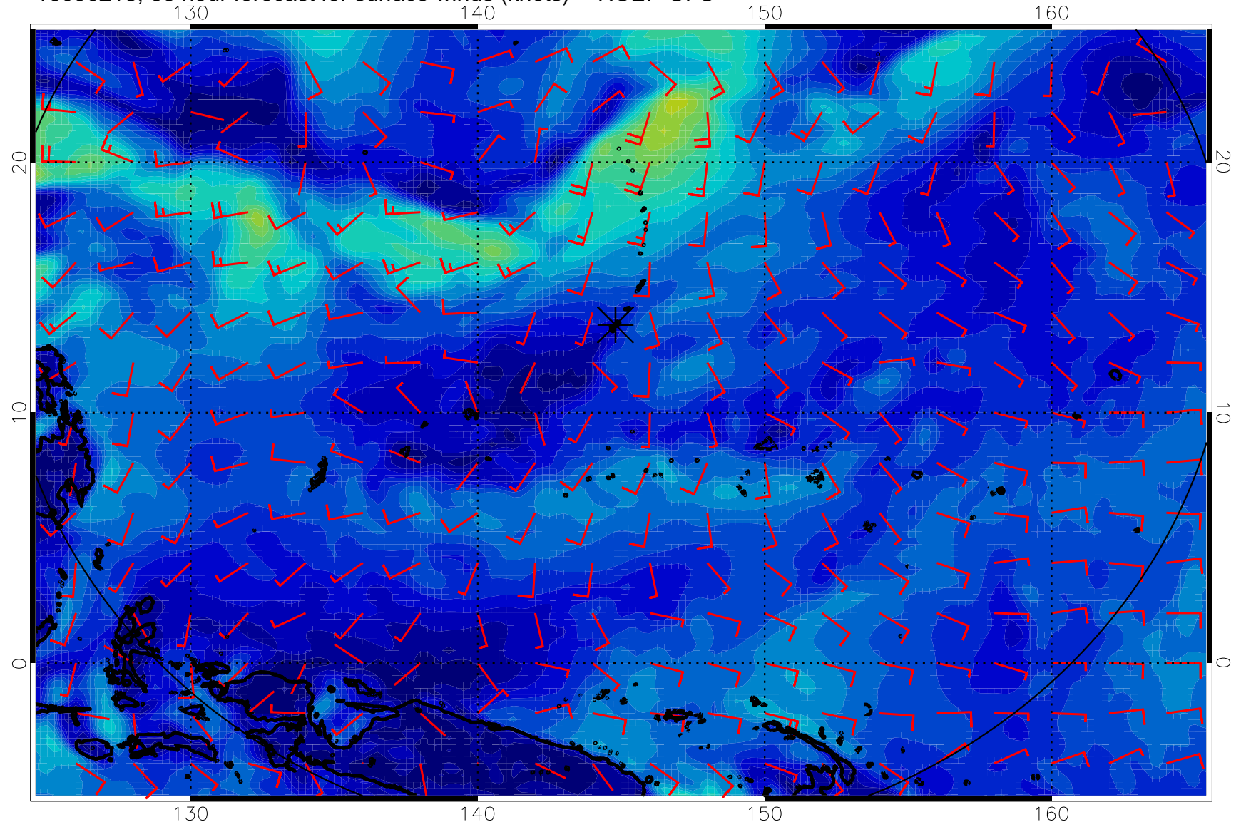
16090218, 66 hour forecast for surface winds (knots) -- NCEP GFS
