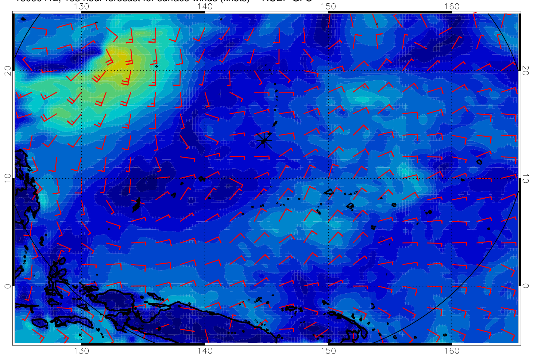
16090412, 108 hour forecast for surface winds (knots) -- NCEP GFS
