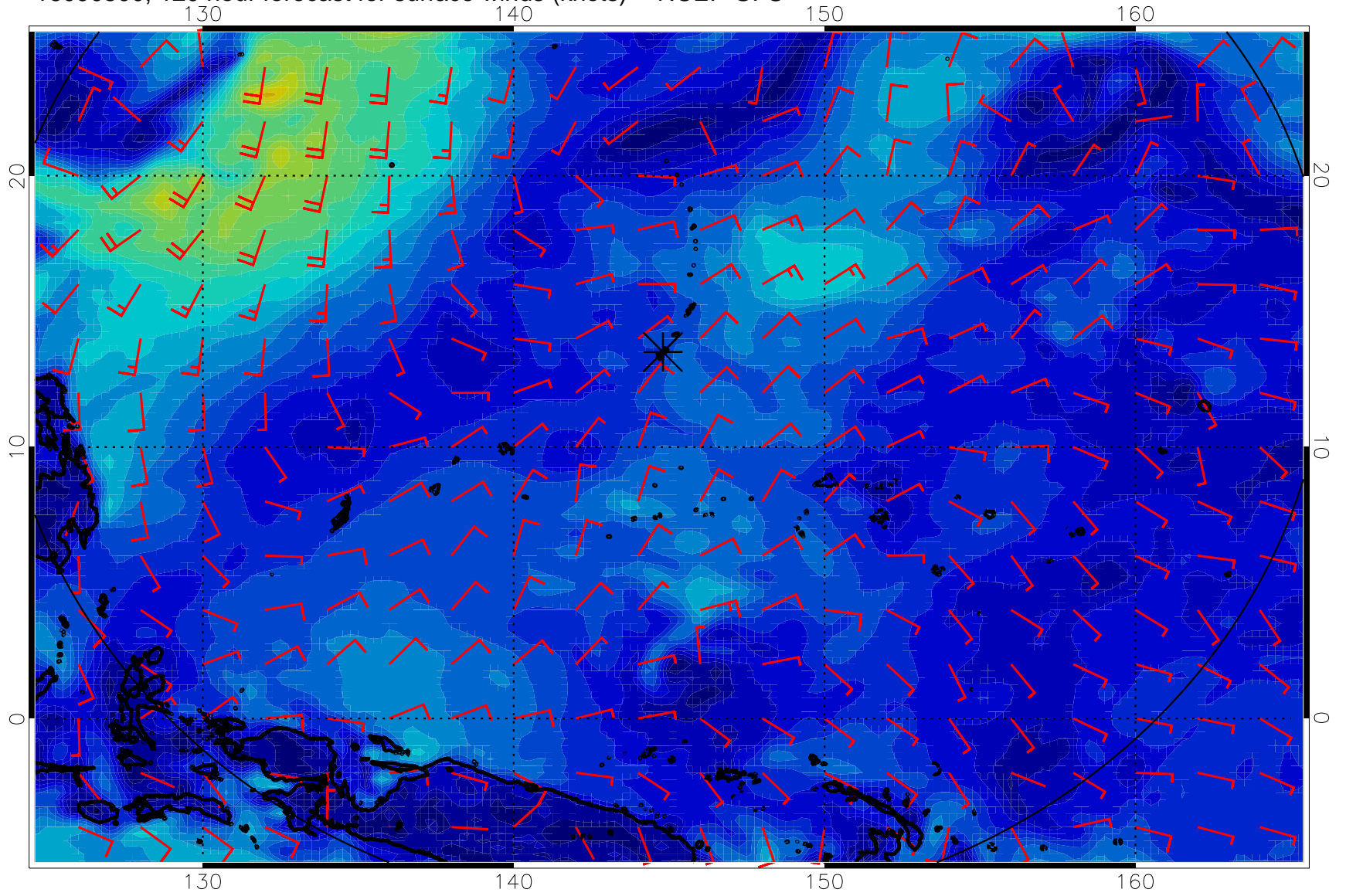
16090500, 120 hour forecast for surface winds (knots) -- NCEP GFS
