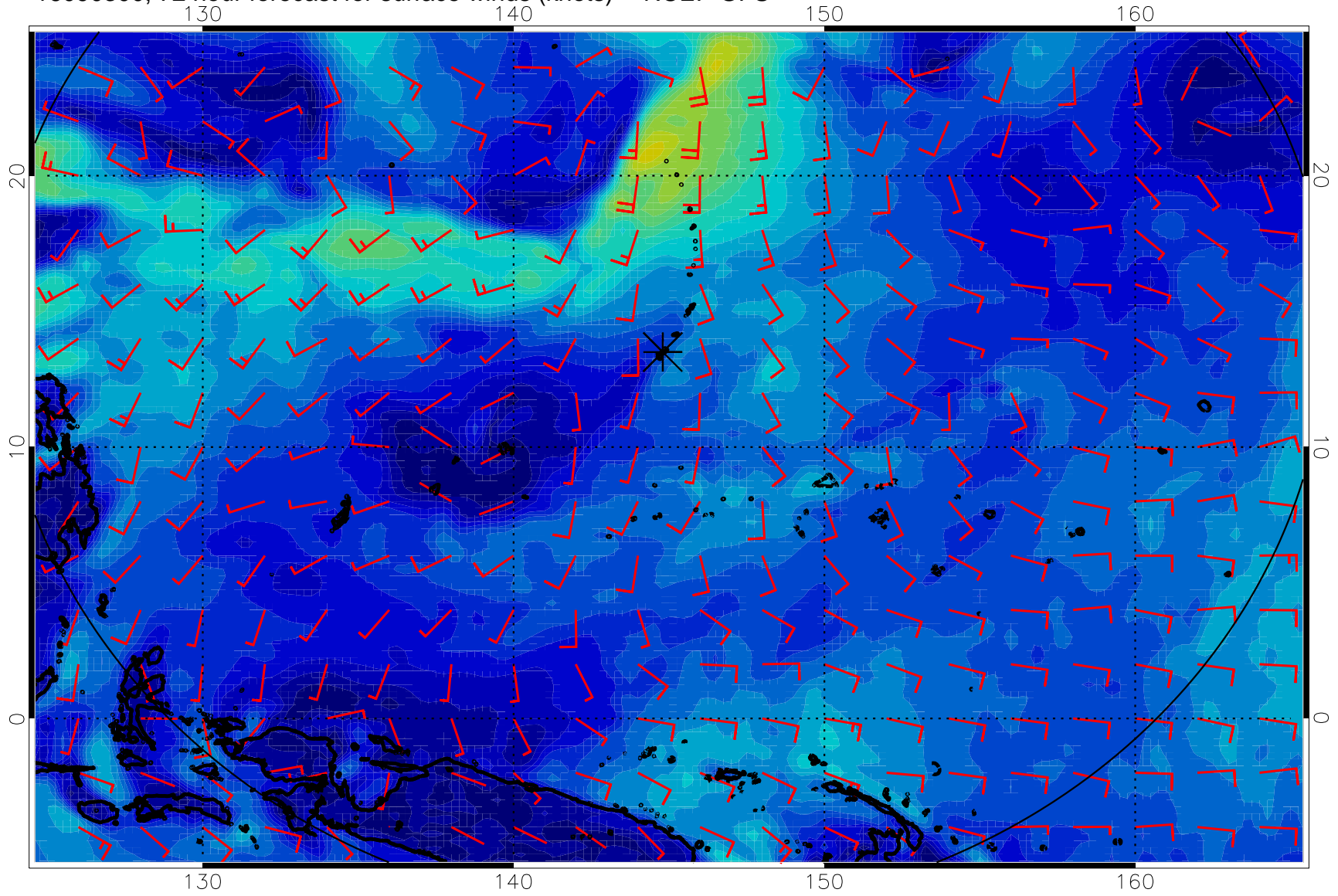
16090300, 72 hour forecast for surface winds (knots) -- NCEP GFS
