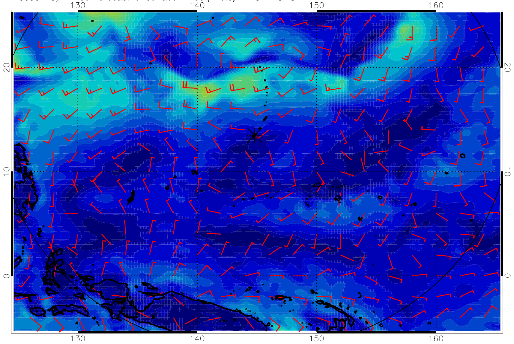
16090118, 42 hour forecast for surface winds (knots) -- NCEP GFS
