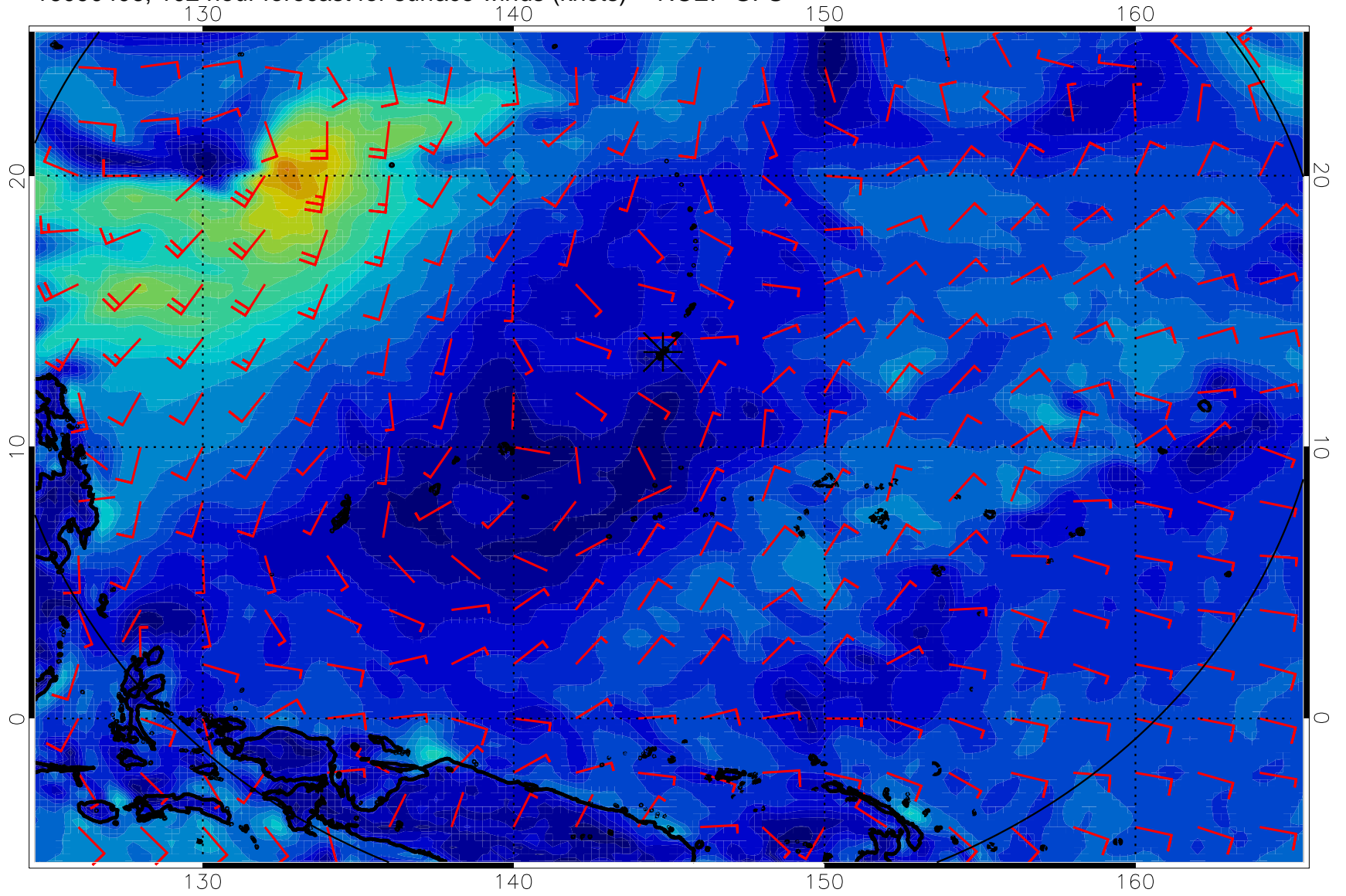
16090406, 102 hour forecast for surface winds (knots) -- NCEP GFS
