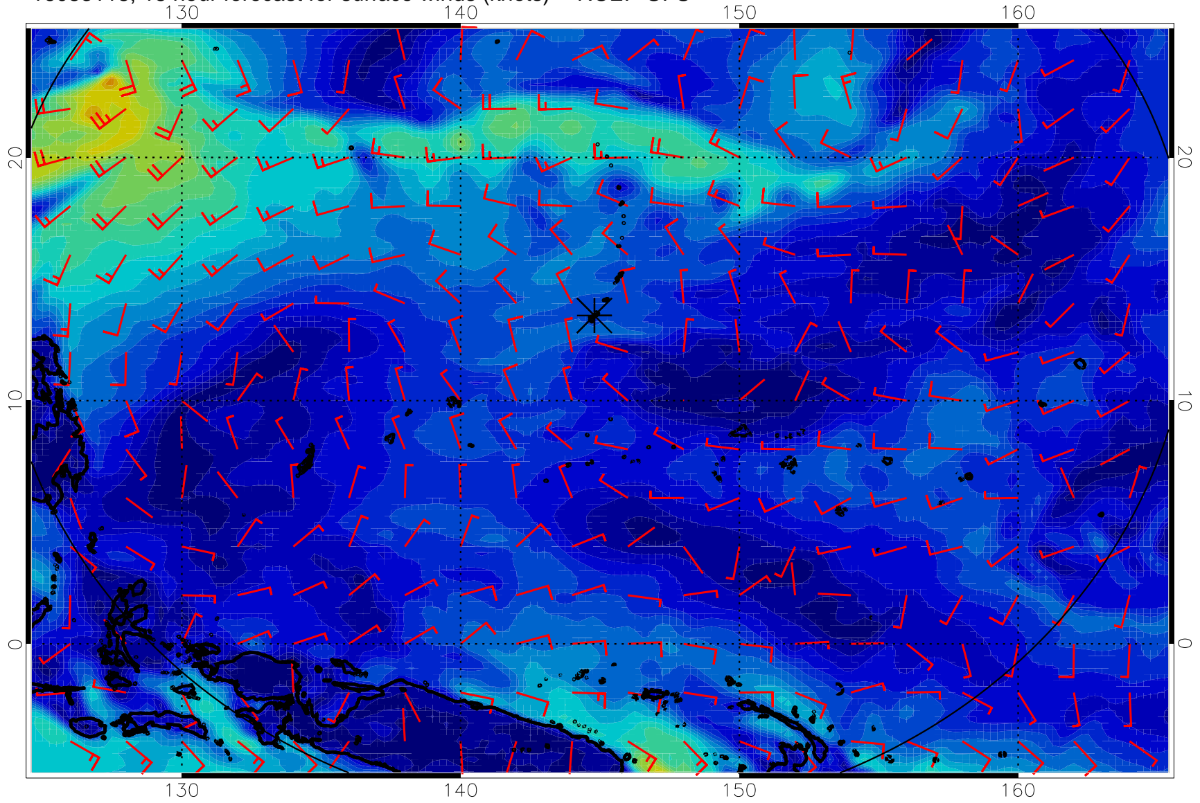
16083118, 18 hour forecast for surface winds (knots) -- NCEP GFS
