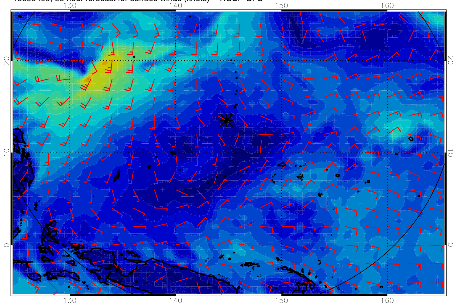
16090400, 96 hour forecast for surface winds (knots) -- NCEP GFS
