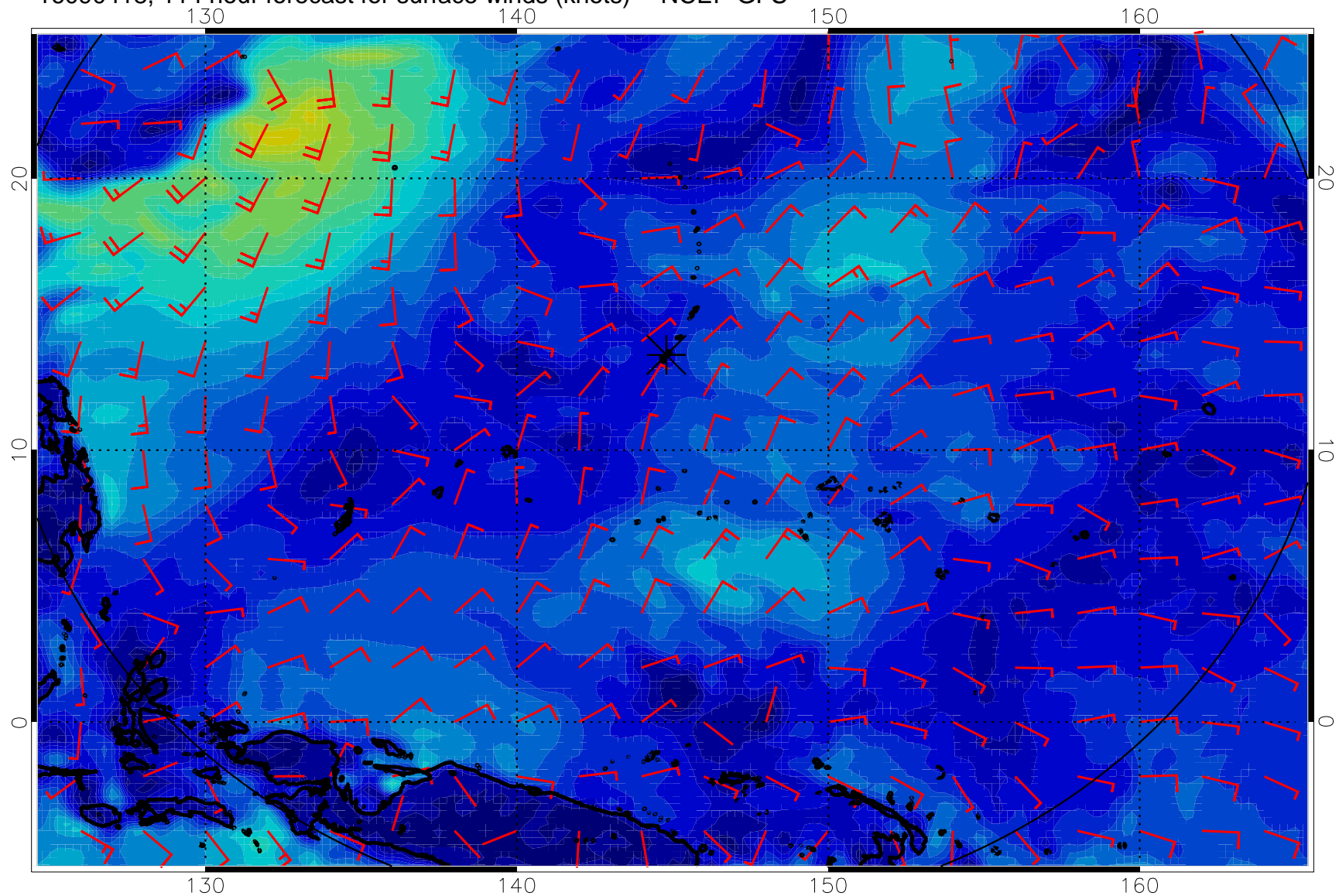
16090418, 114 hour forecast for surface winds (knots) -- NCEP GFS
