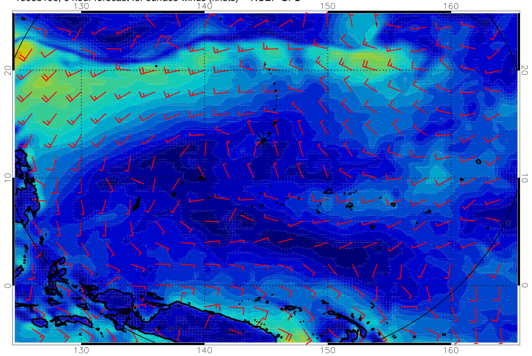
16083106, 6 hour forecast for surface winds (knots) -- NCEP GFS
