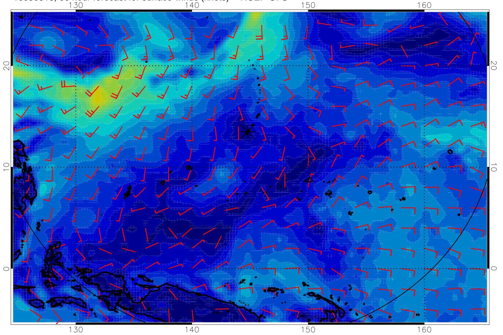
16090318, 90 hour forecast for surface winds (knots) -- NCEP GFS
