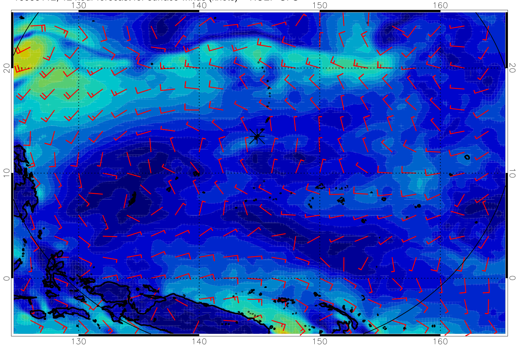
16083112, 12 hour forecast for surface winds (knots) -- NCEP GFS
