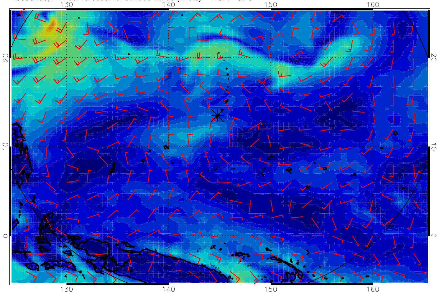
16090100, 24 hour forecast for surface winds (knots) -- NCEP GFS
