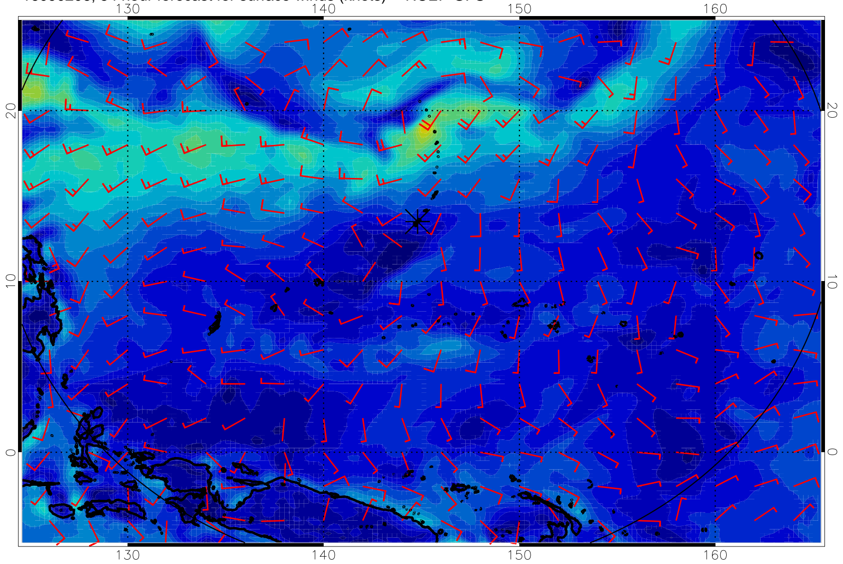
16090206, 54 hour forecast for surface winds (knots) -- NCEP GFS
