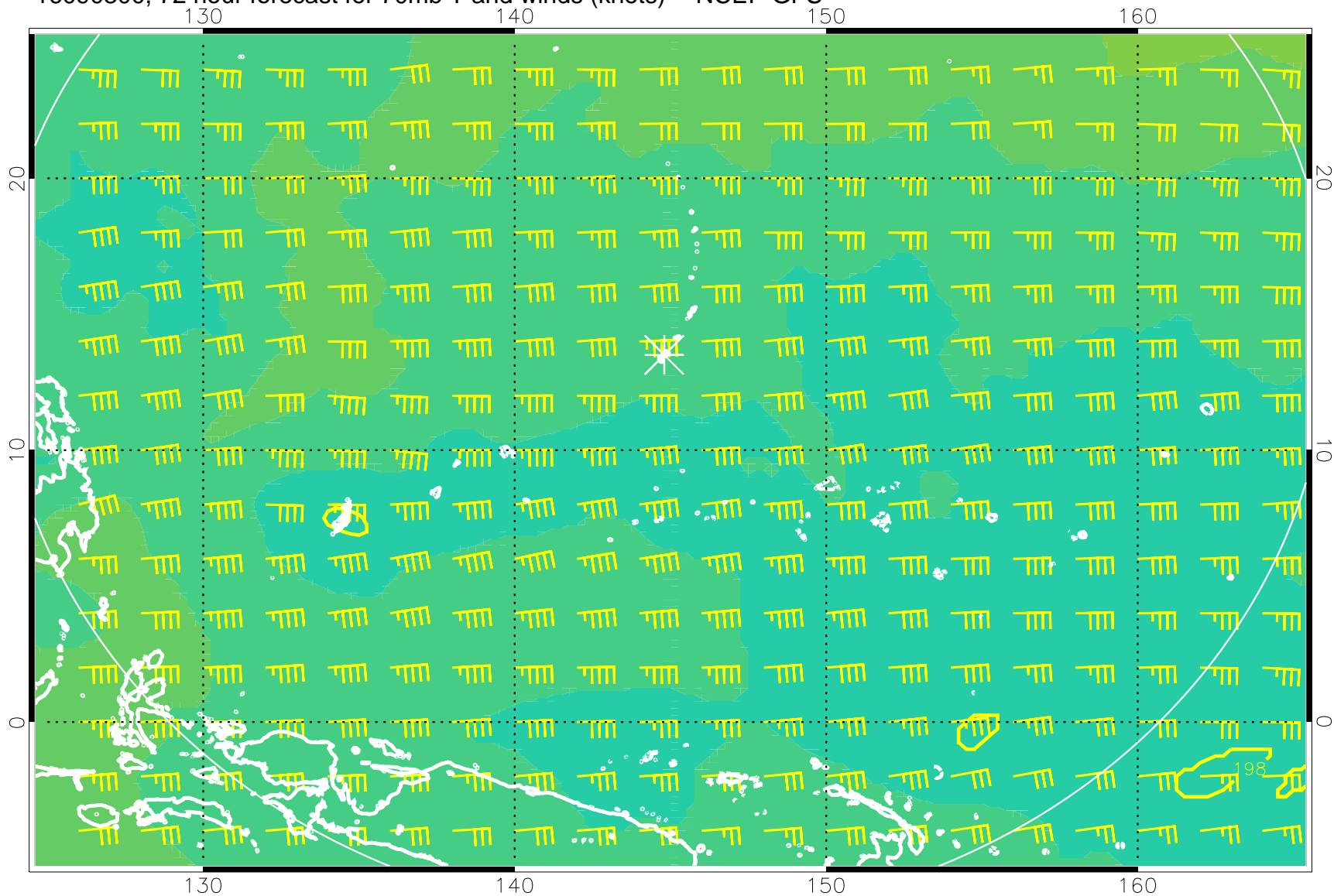
16090300, 72 hour forecast for 70mb T and winds (knots) -- NCEP GFS
