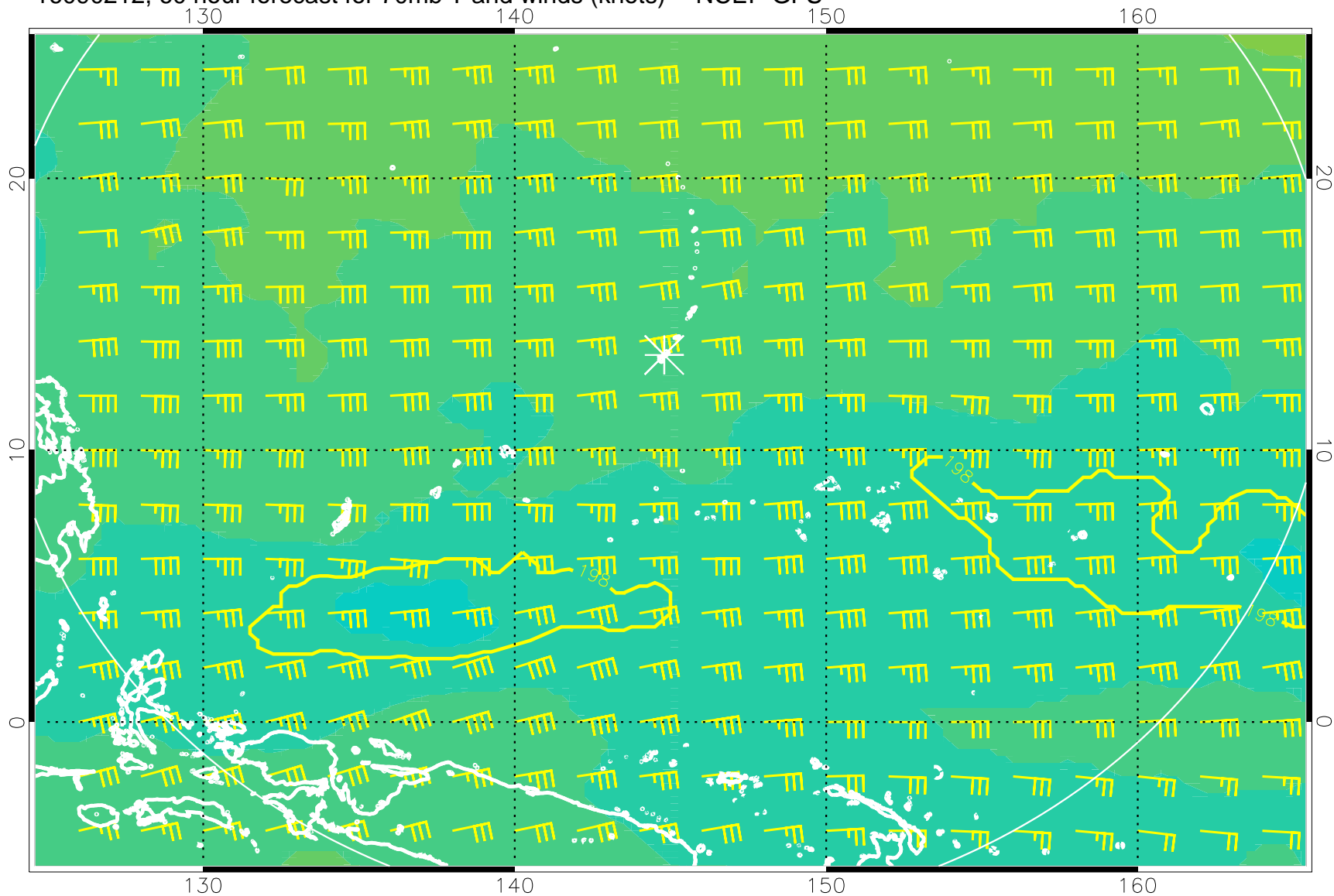
16090212, 60 hour forecast for 70mb T and winds (knots) -- NCEP GFS
