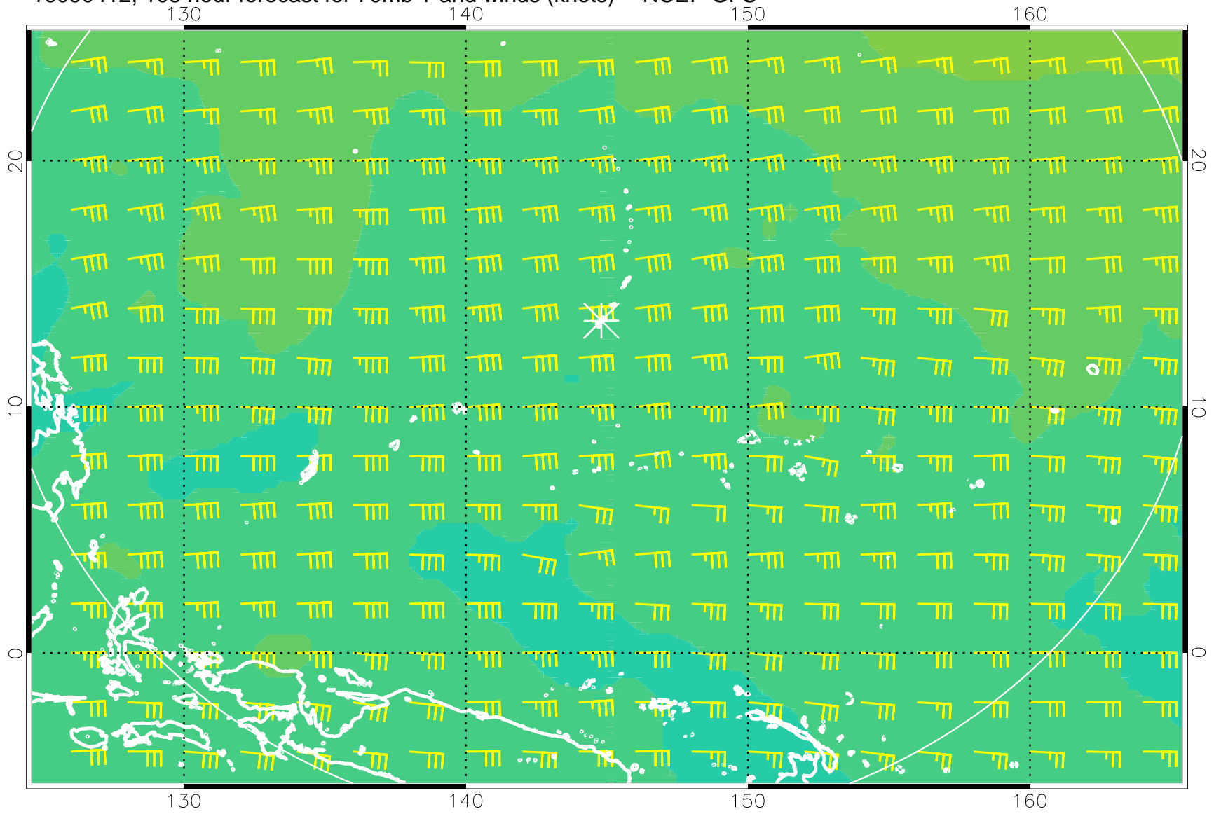
16090412, 108 hour forecast for 70mb T and winds (knots) -- NCEP GFS
