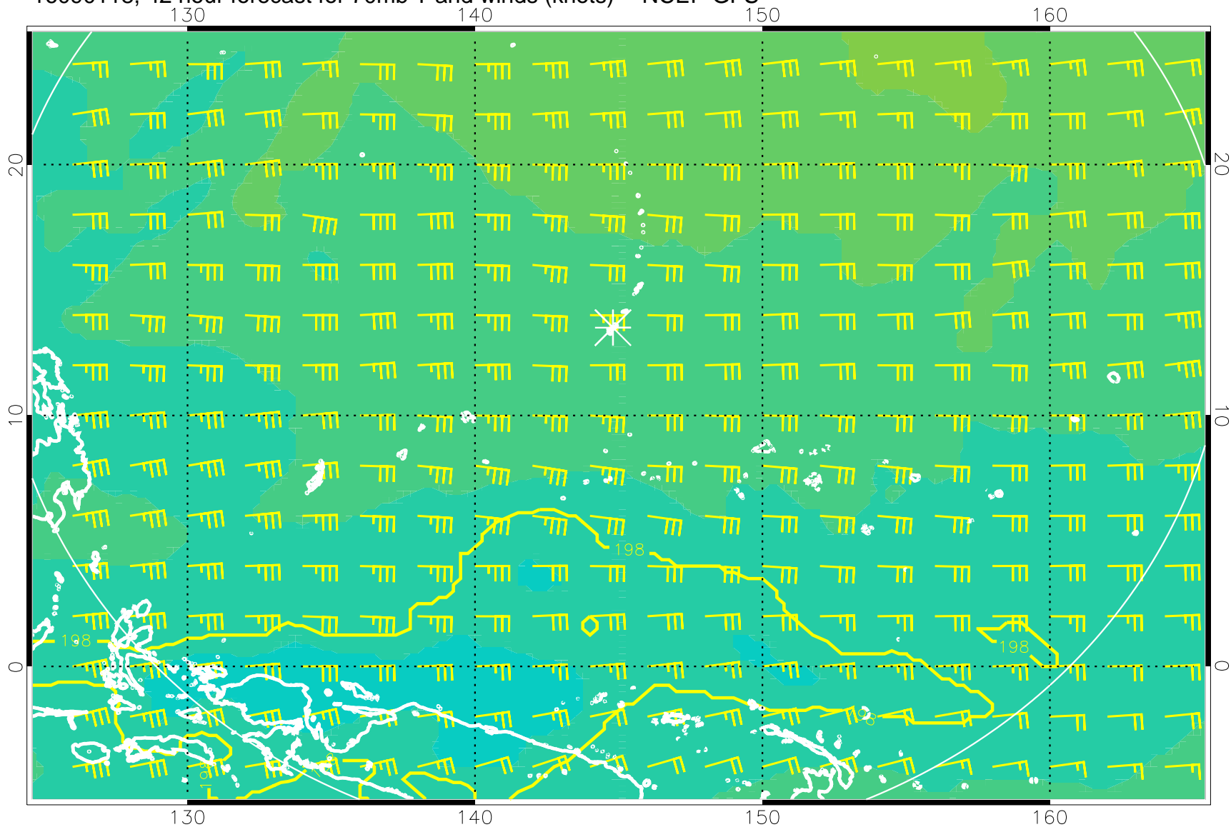
16090118, 42 hour forecast for 70mb T and winds (knots) -- NCEP GFS
