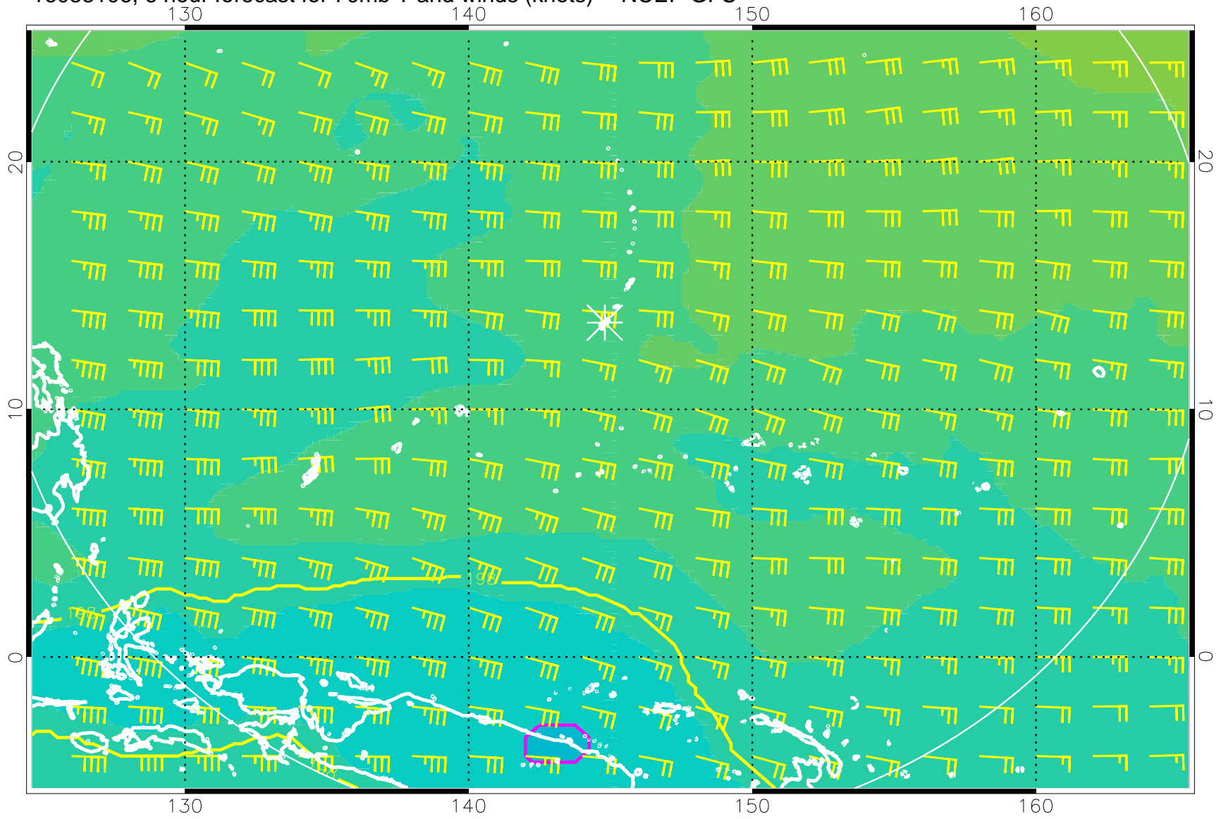
16083106, 6 hour forecast for 70mb T and winds (knots) -- NCEP GFS
