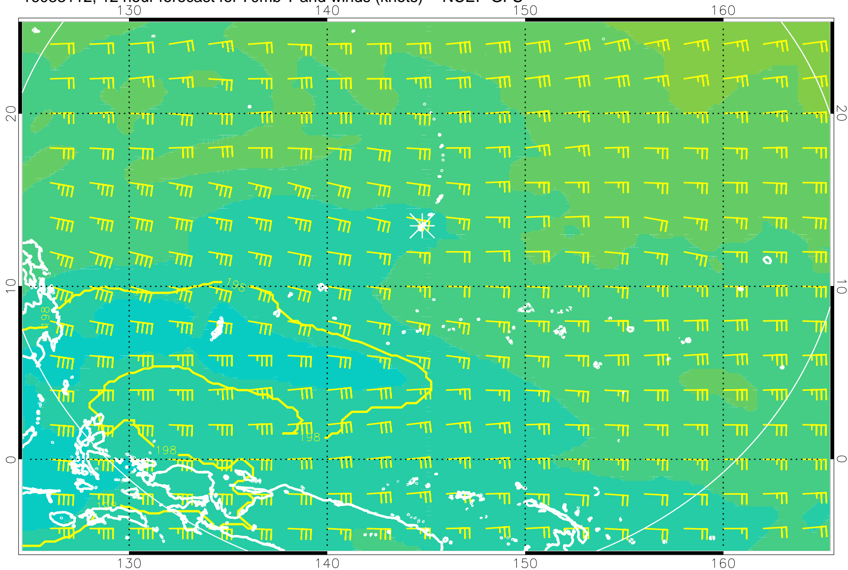
16083112, 12 hour forecast for 70mb T and winds (knots) -- NCEP GFS
