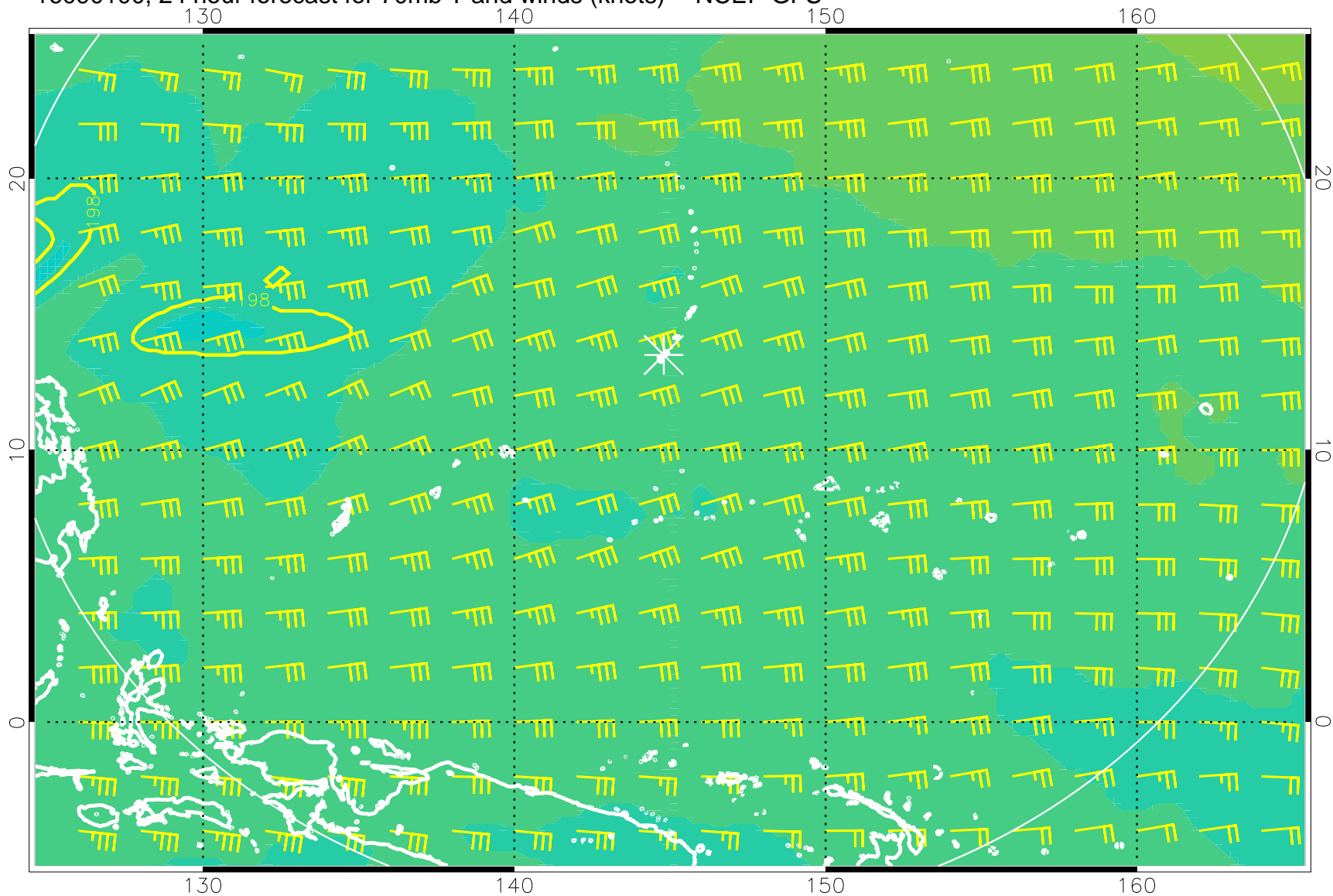
16090100, 24 hour forecast for 70mb T and winds (knots) -- NCEP GFS
