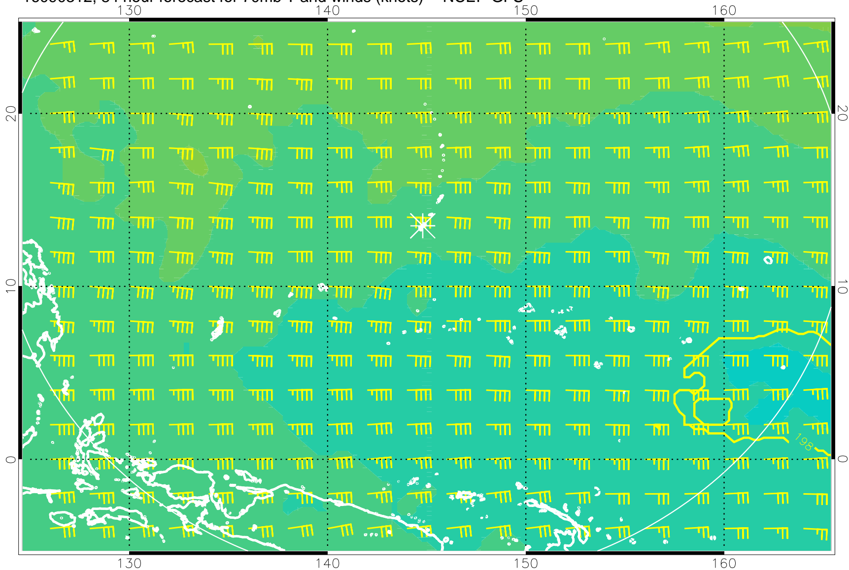
16090312, 84 hour forecast for 70mb T and winds (knots) -- NCEP GFS
