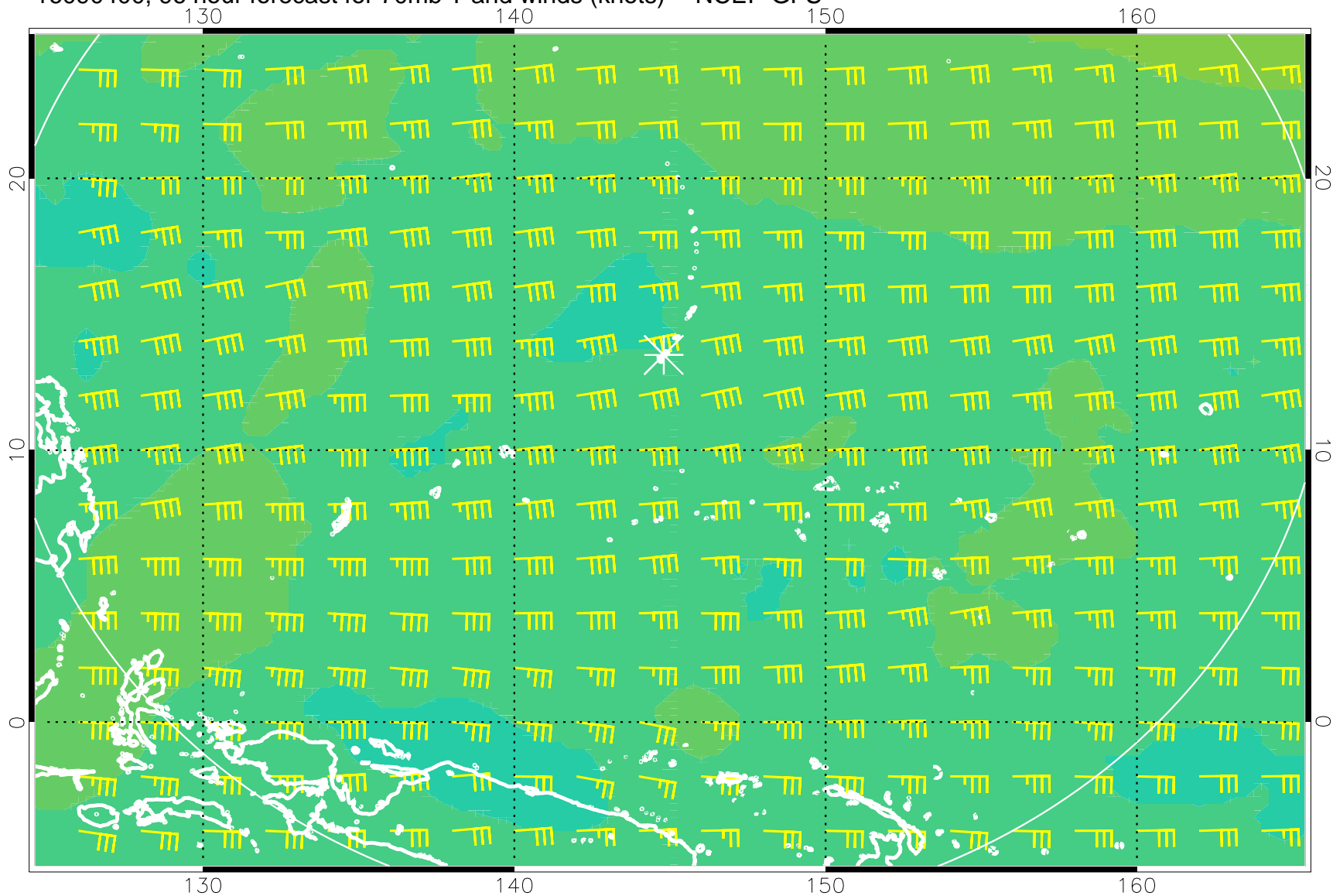
16090400, 96 hour forecast for 70mb T and winds (knots) -- NCEP GFS
