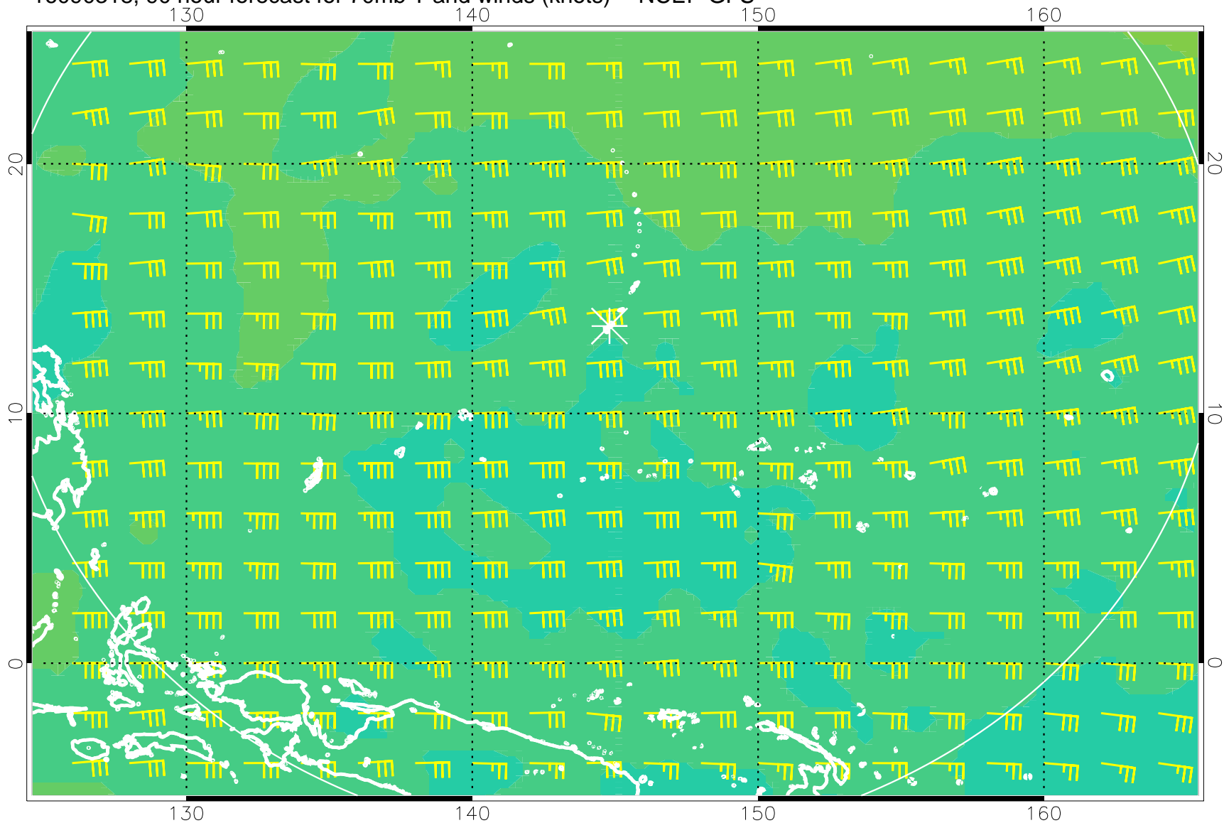
16090318, 90 hour forecast for 70mb T and winds (knots) -- NCEP GFS
