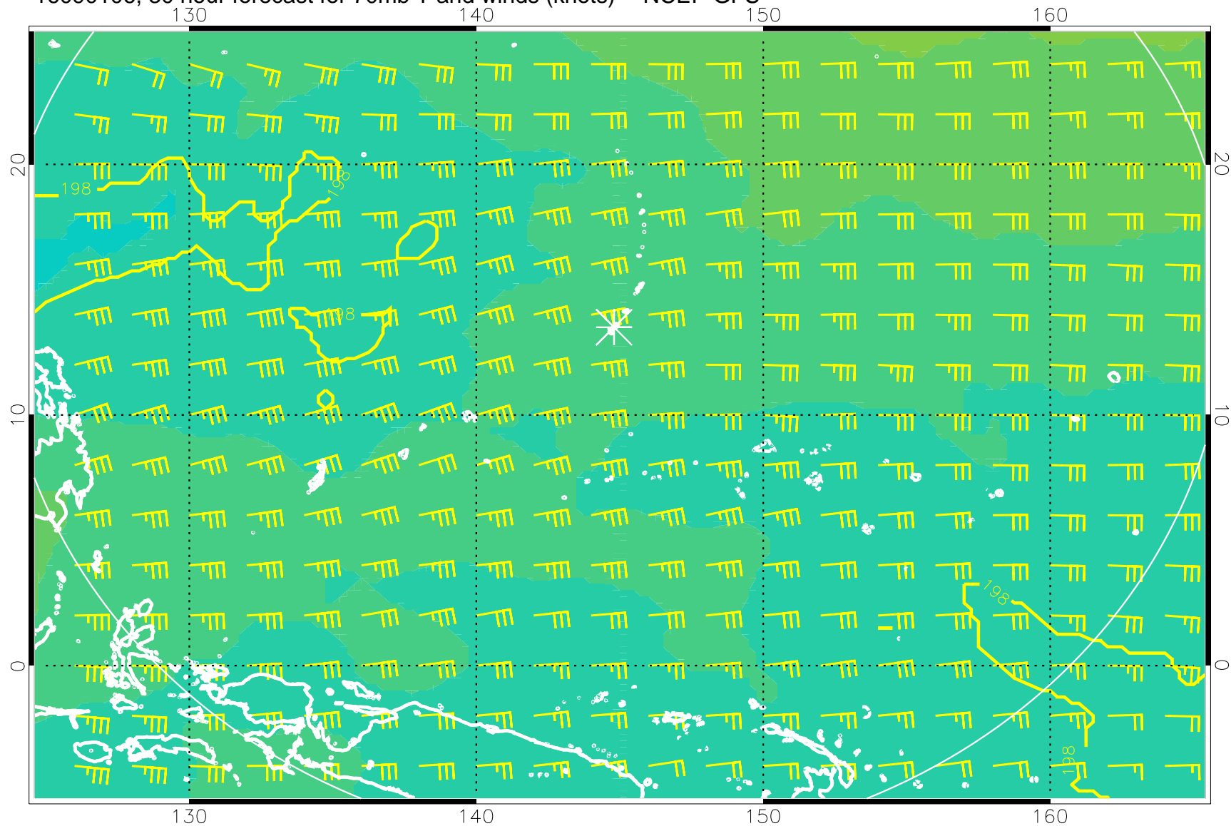
16090106, 30 hour forecast for 70mb T and winds (knots) -- NCEP GFS
