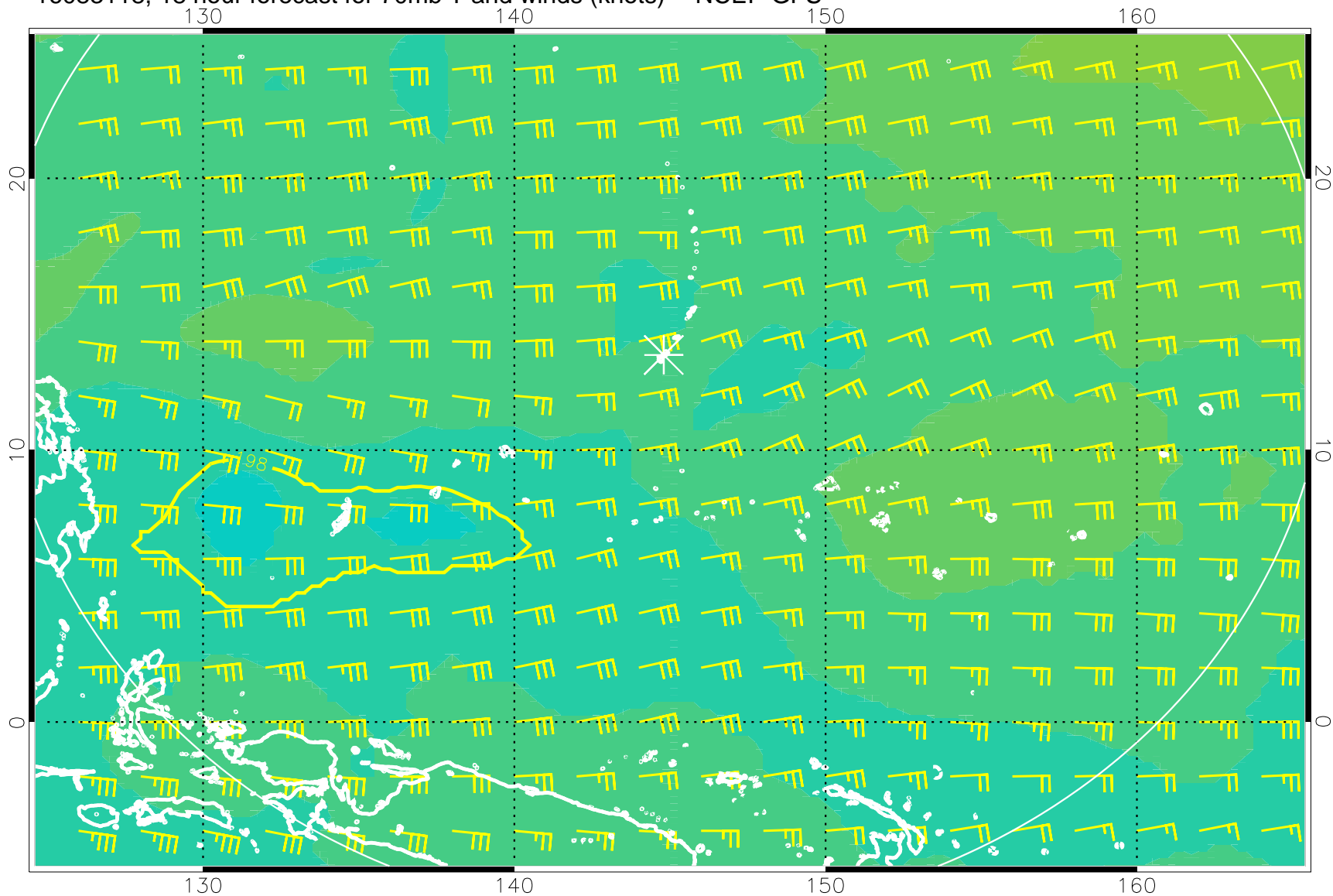
16083118, 18 hour forecast for 70mb T and winds (knots) -- NCEP GFS
