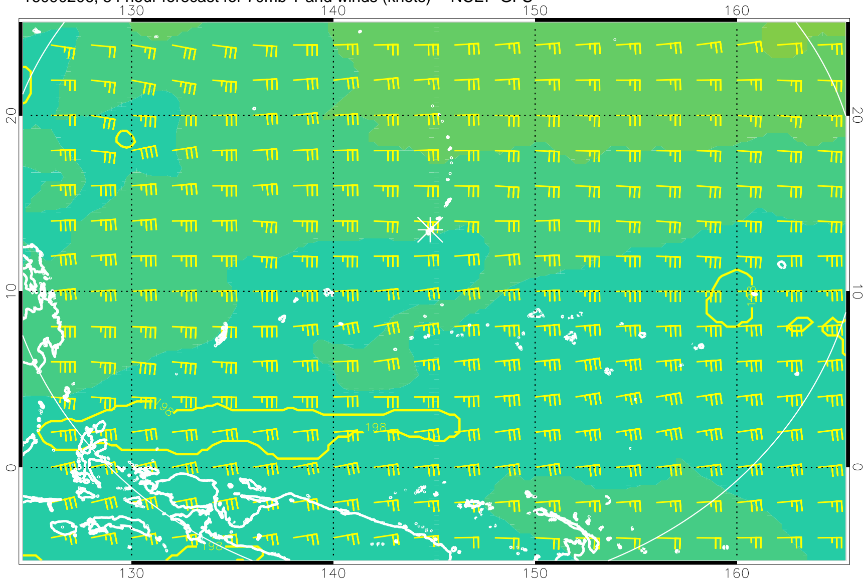
16090206, 54 hour forecast for 70mb T and winds (knots) -- NCEP GFS
