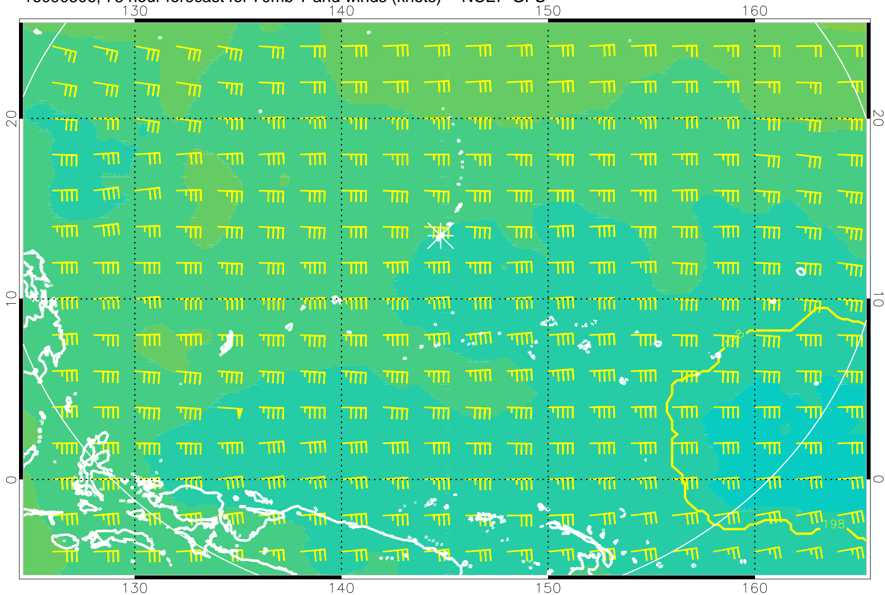
16090306, 78 hour forecast for 70mb T and winds (knots) -- NCEP GFS
