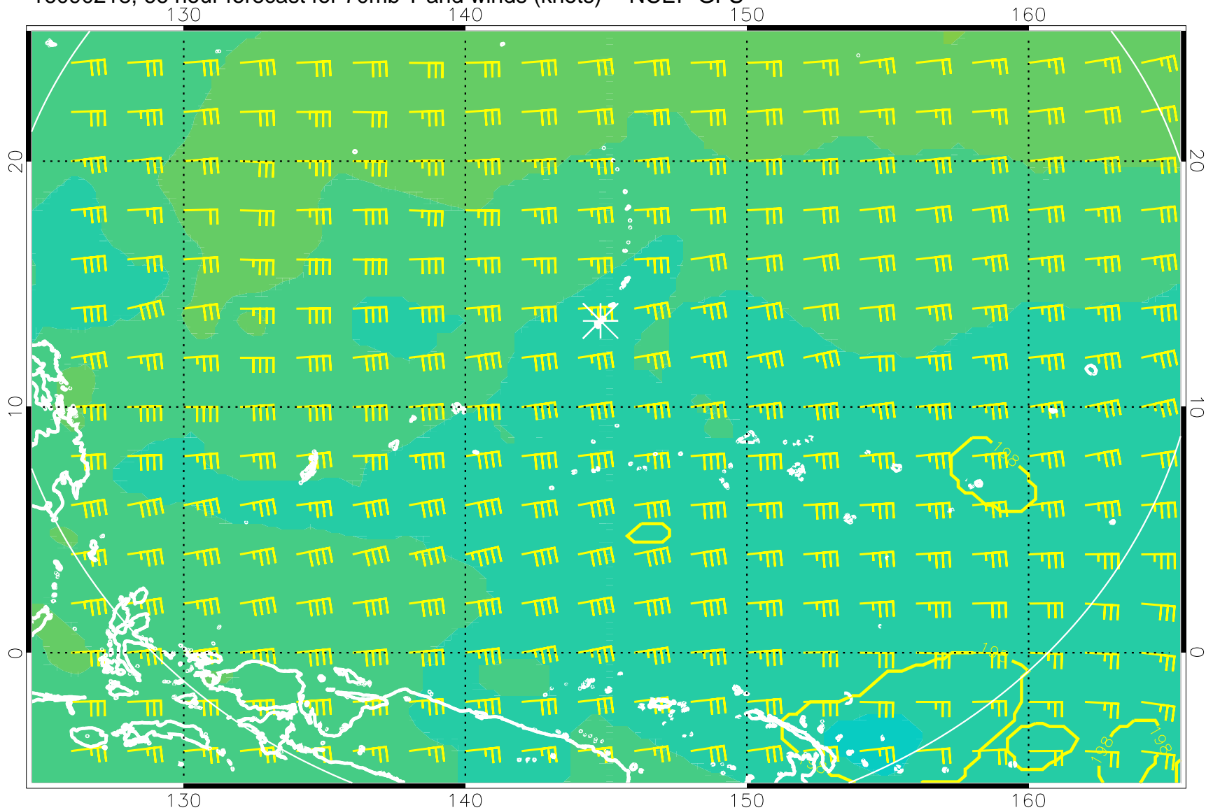
16090218, 66 hour forecast for 70mb T and winds (knots) -- NCEP GFS
