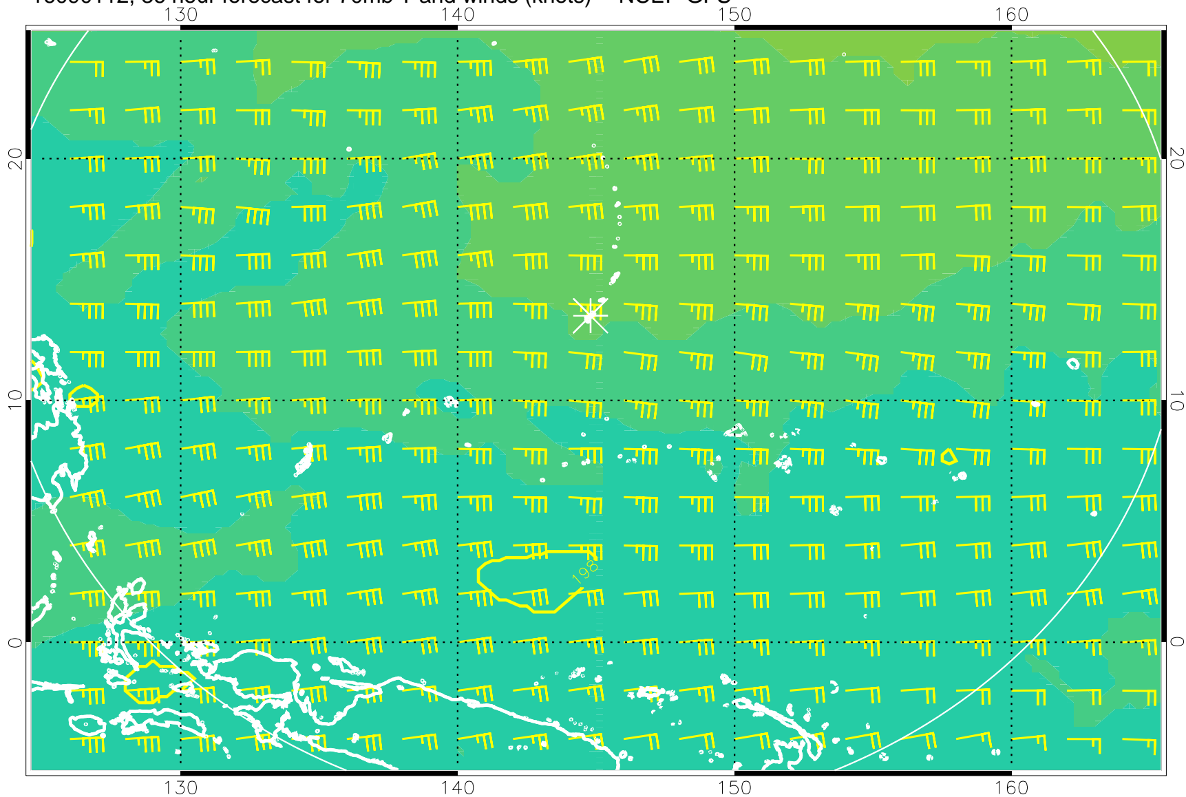
16090112, 36 hour forecast for 70mb T and winds (knots) -- NCEP GFS
