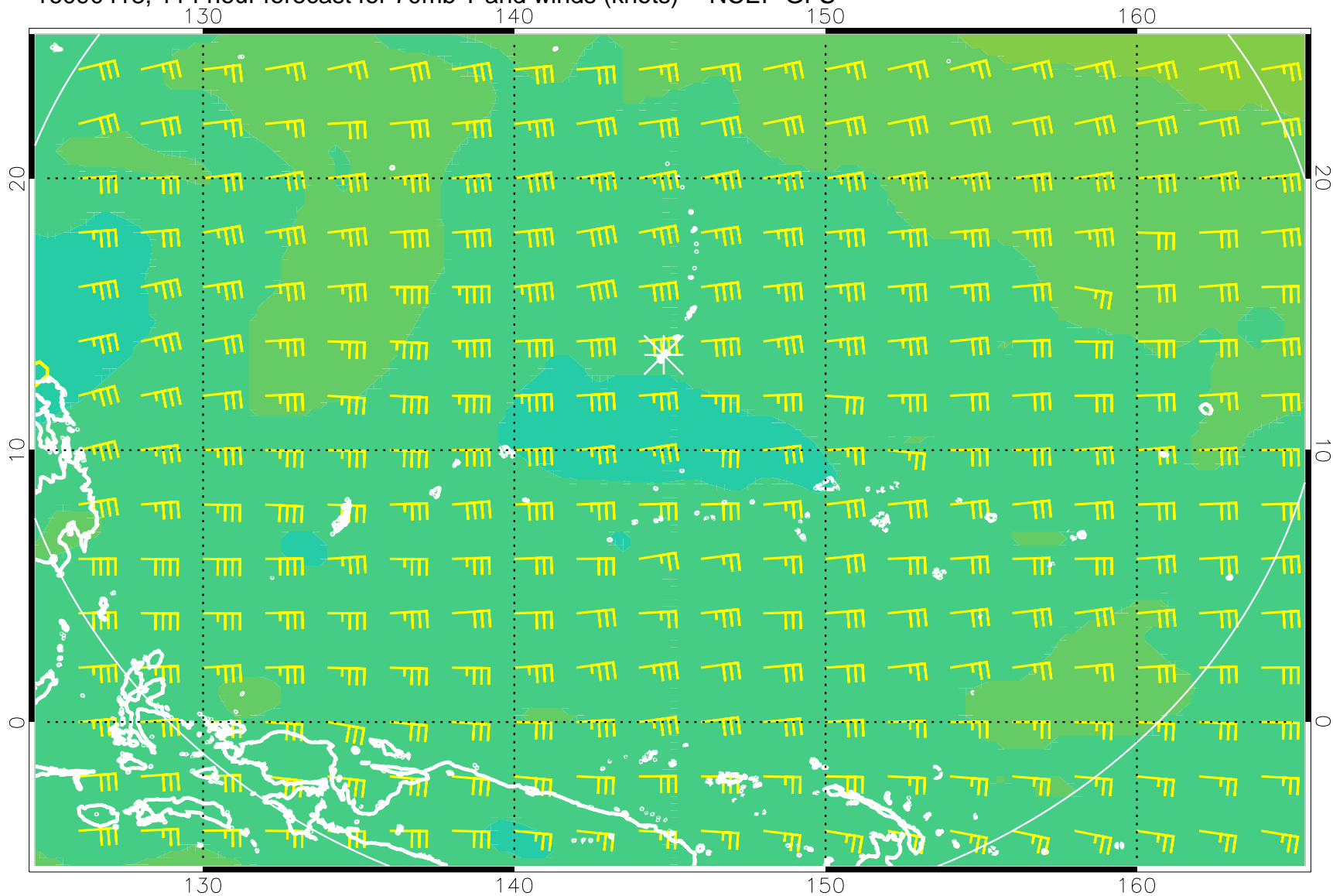
16090418, 114 hour forecast for 70mb T and winds (knots) -- NCEP GFS
