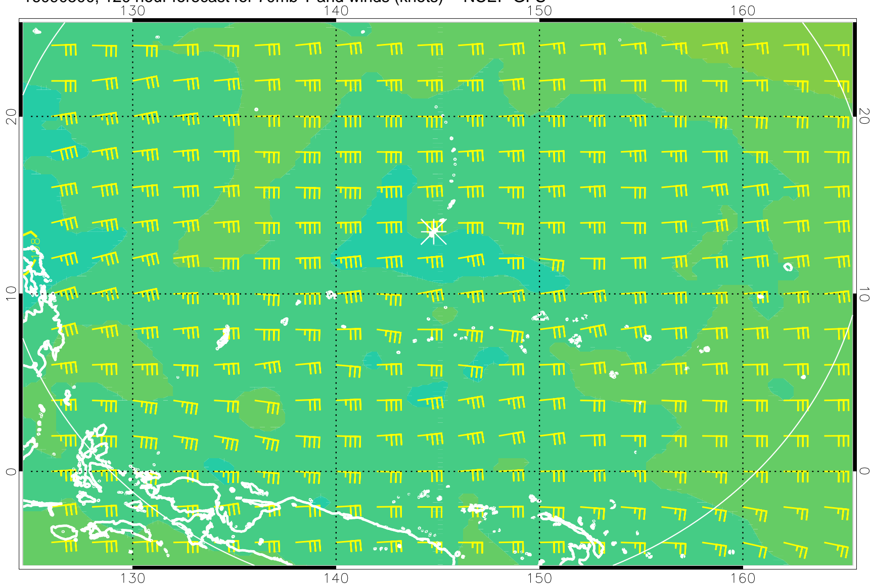
16090500, 120 hour forecast for 70mb T and winds (knots) -- NCEP GFS
