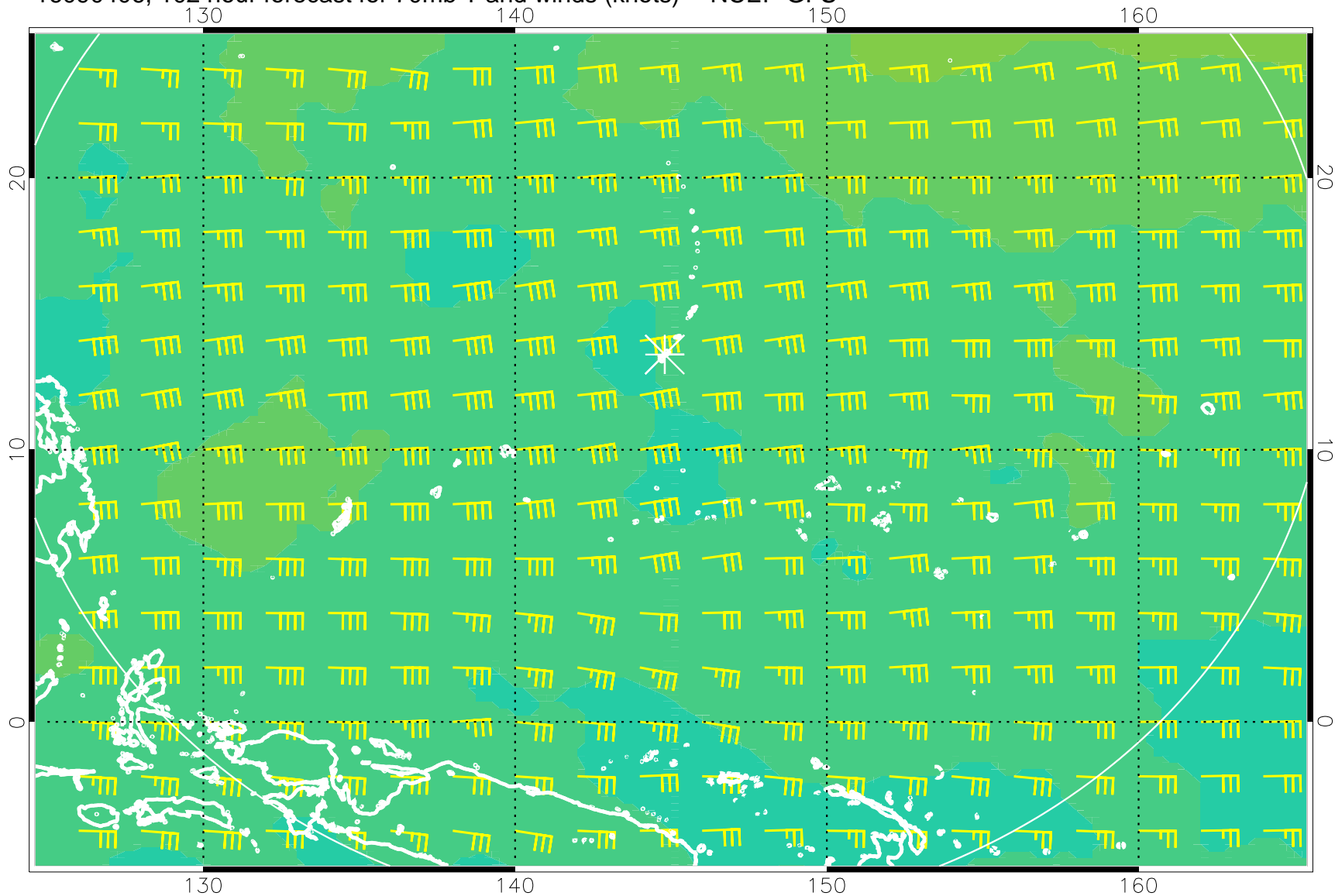
16090406, 102 hour forecast for 70mb T and winds (knots) -- NCEP GFS
