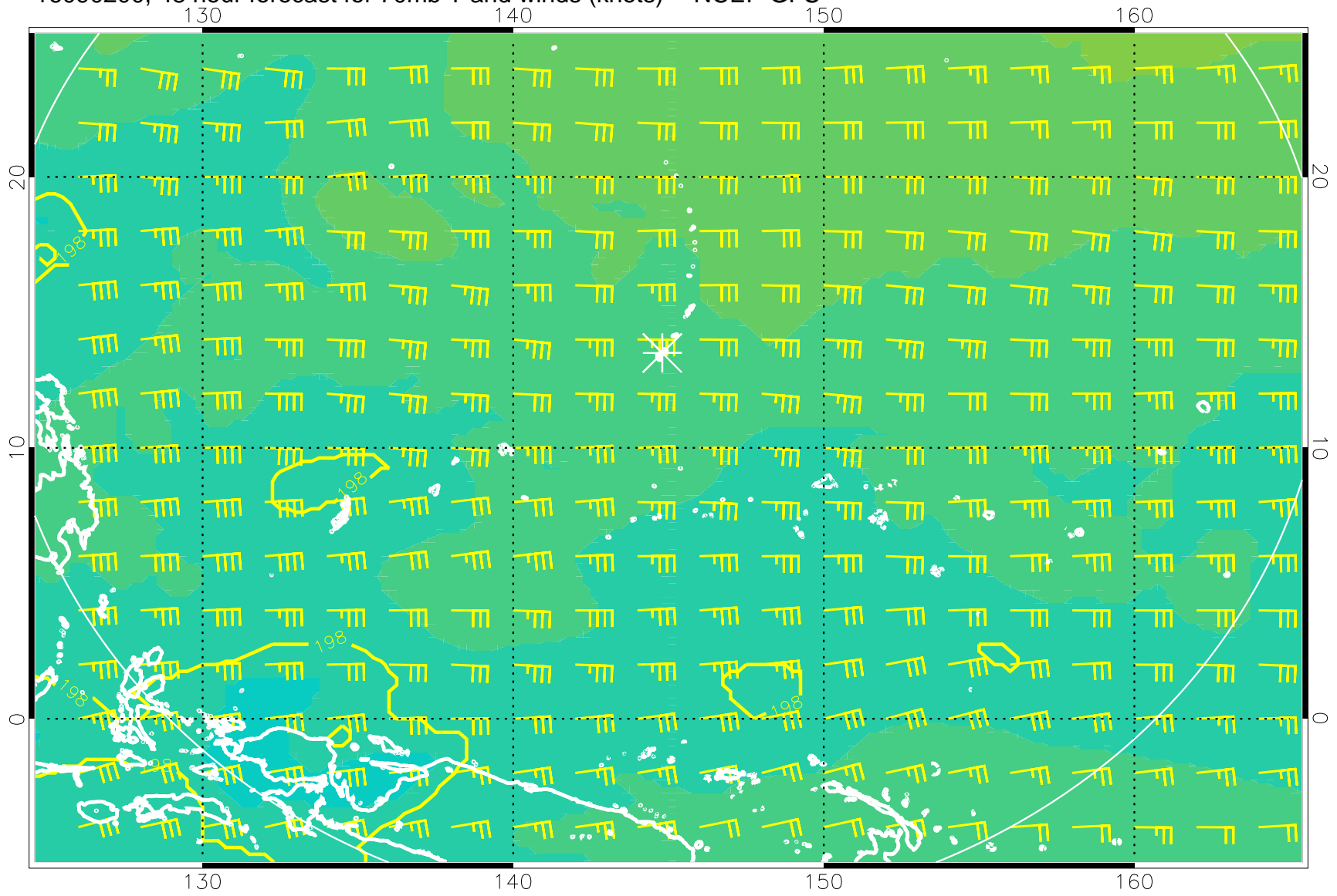
16090200, 48 hour forecast for 70mb T and winds (knots) -- NCEP GFS
