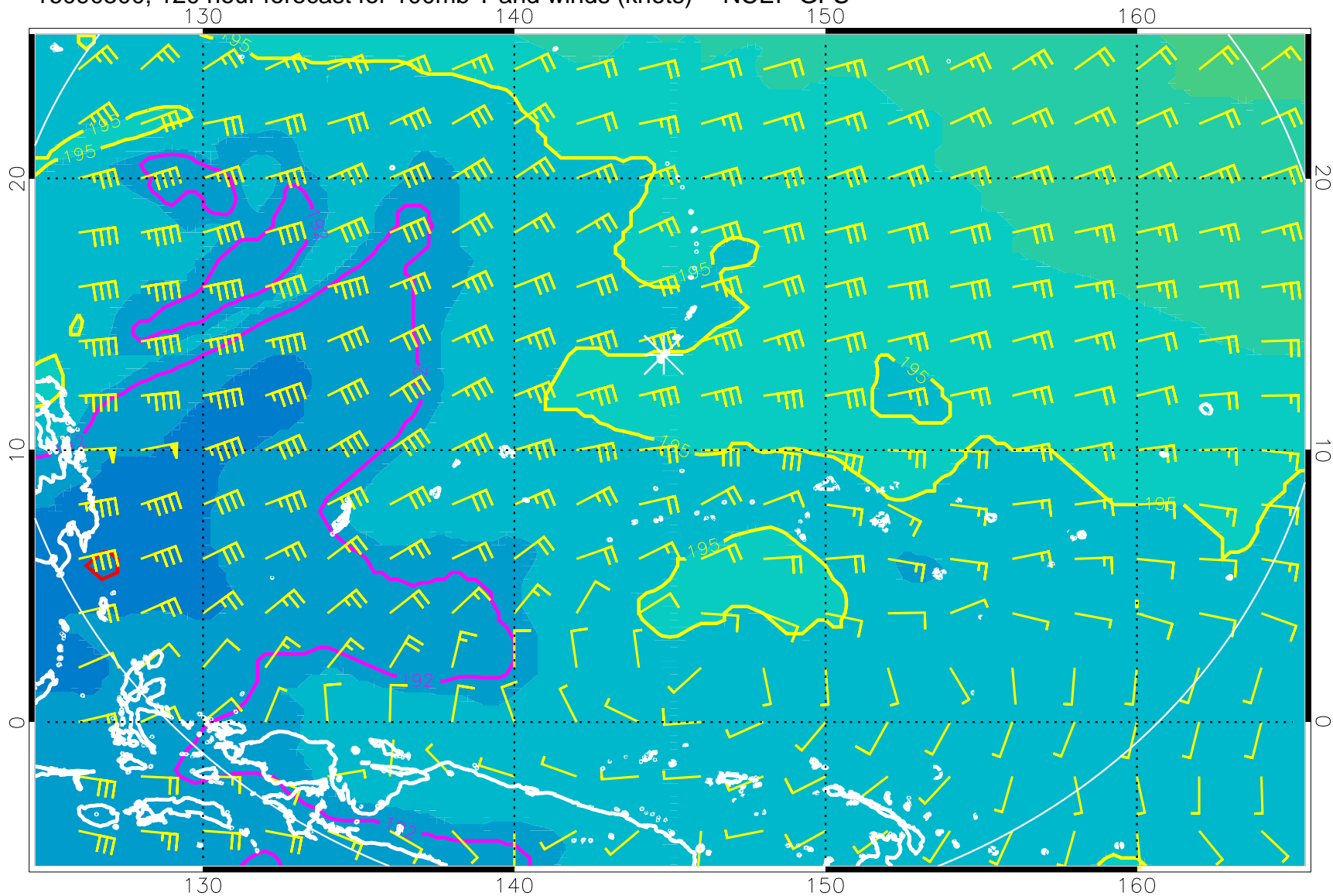
16090500, 120 hour forecast for 100mb T and winds (knots) -- NCEP GFS
