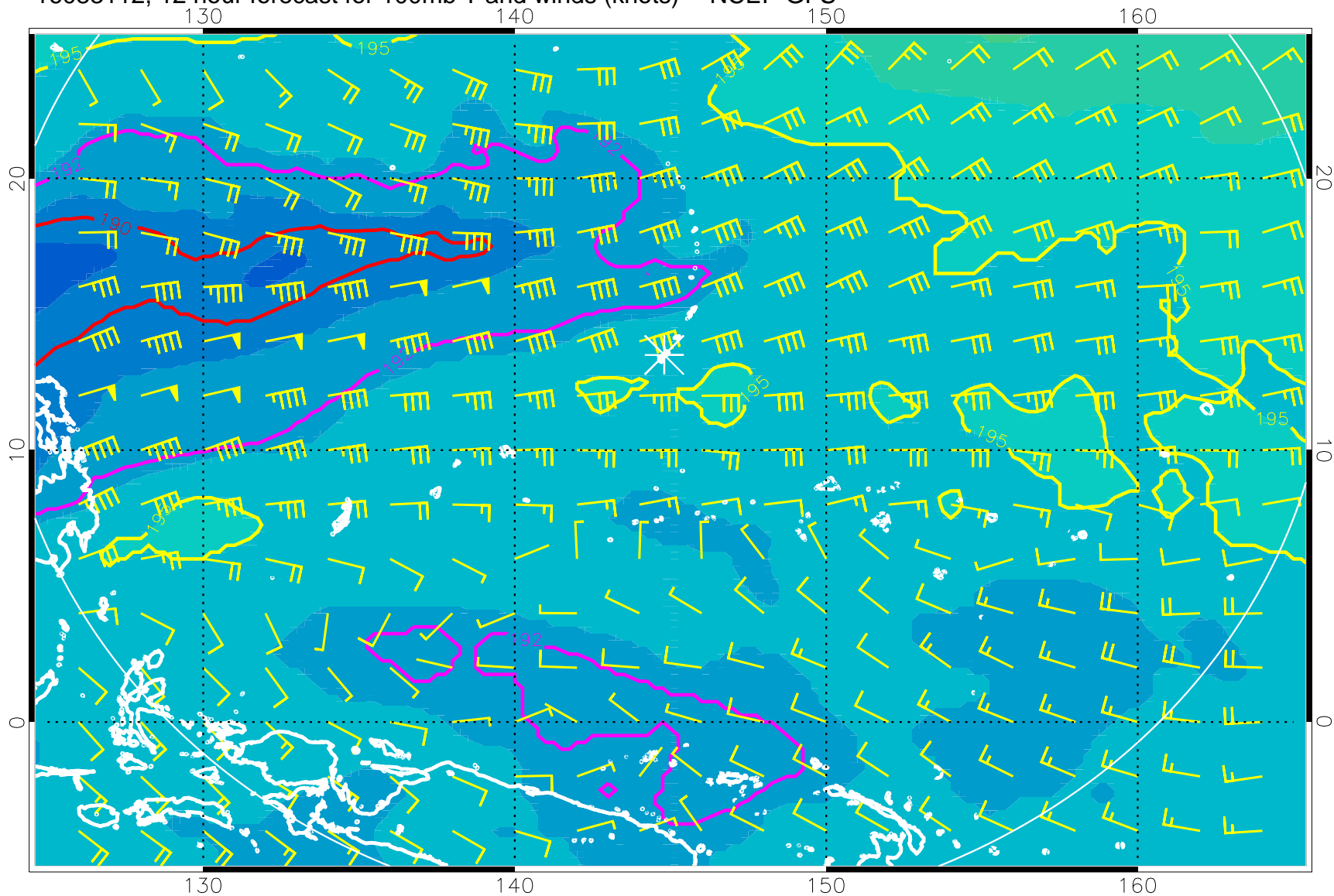
16083112, 12 hour forecast for 100mb T and winds (knots) -- NCEP GFS
