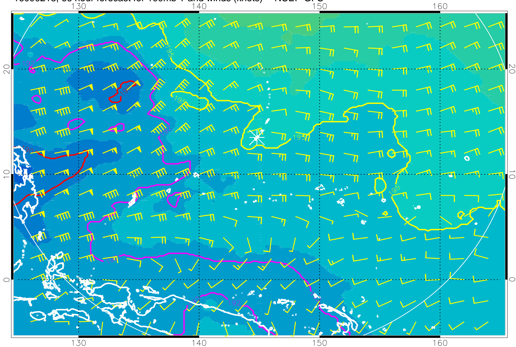
16090218, 66 hour forecast for 100mb T and winds (knots) -- NCEP GFS
