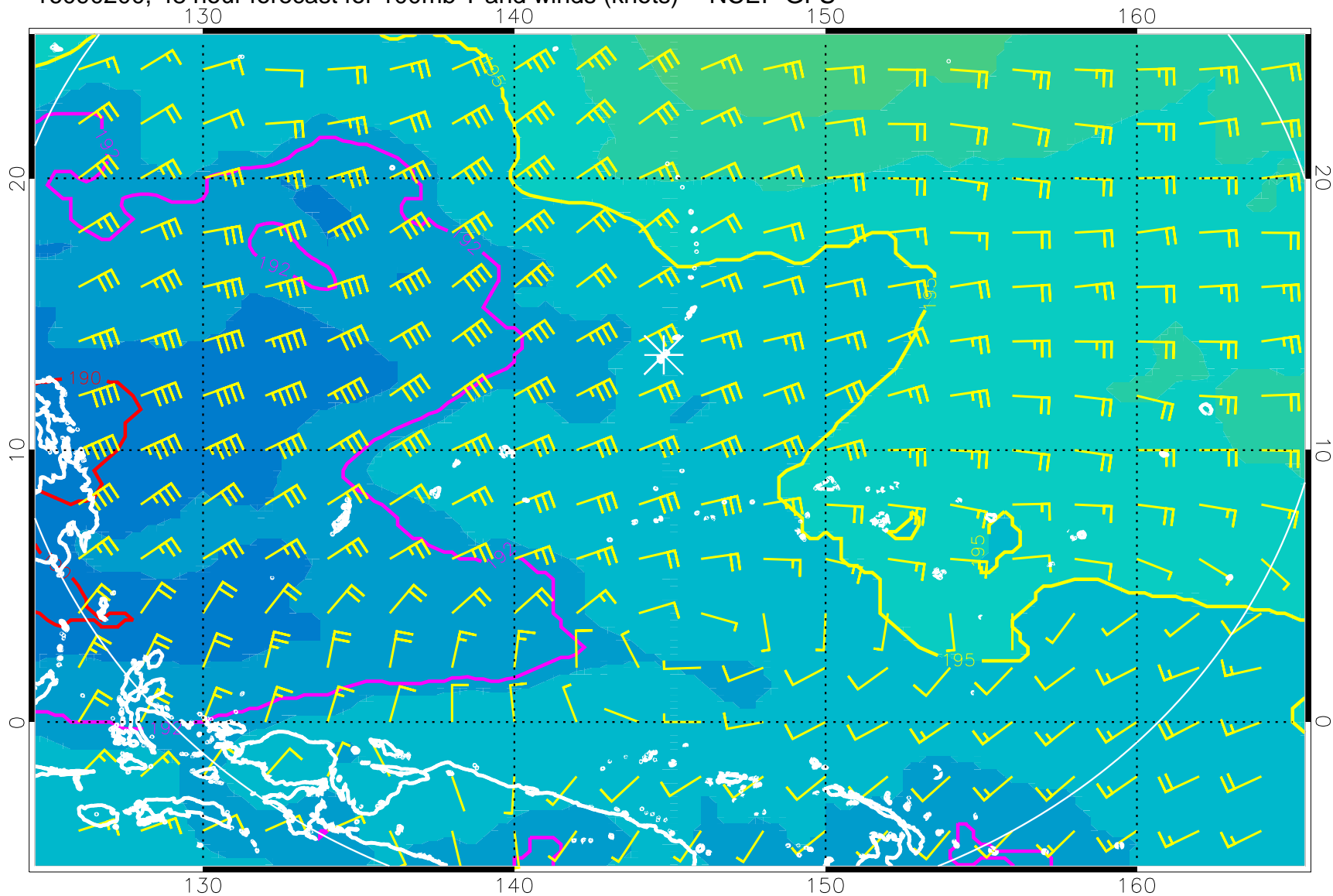
16090200, 48 hour forecast for 100mb T and winds (knots) -- NCEP GFS
