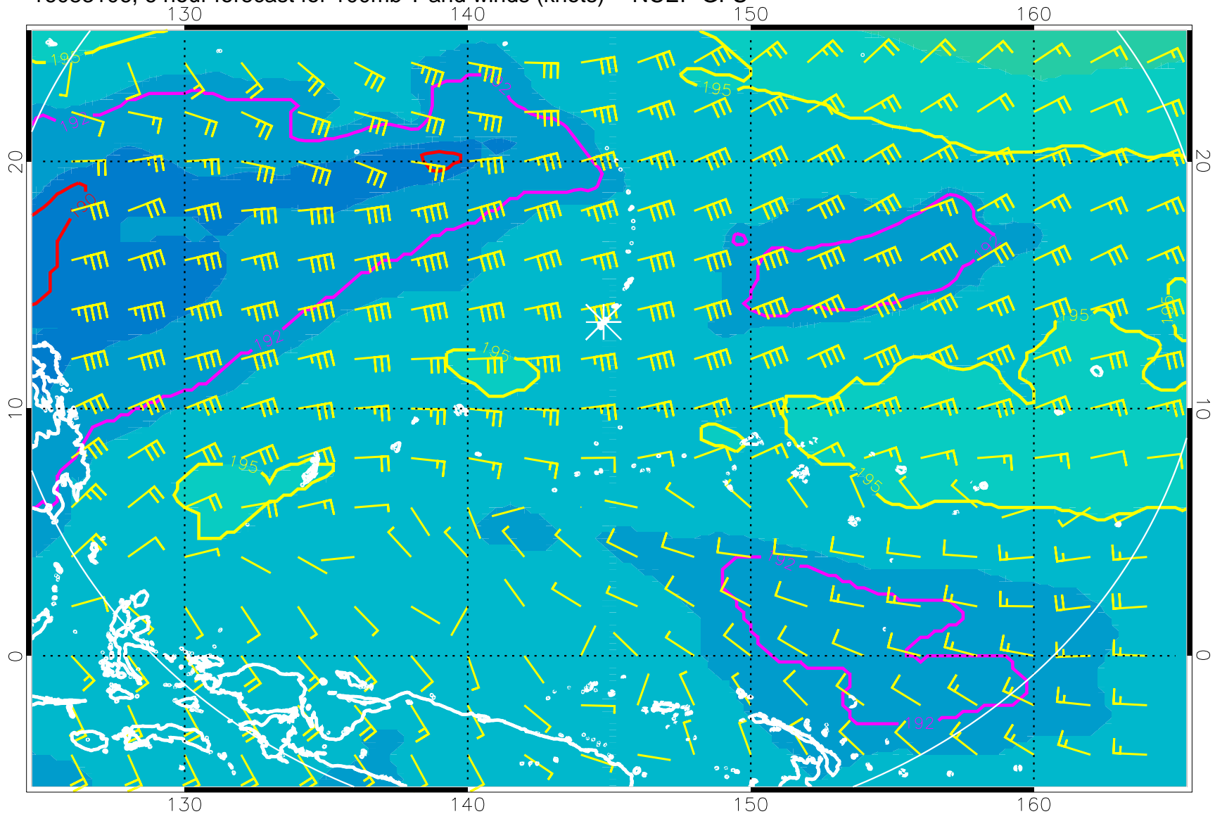
16083106, 6 hour forecast for 100mb T and winds (knots) -- NCEP GFS
