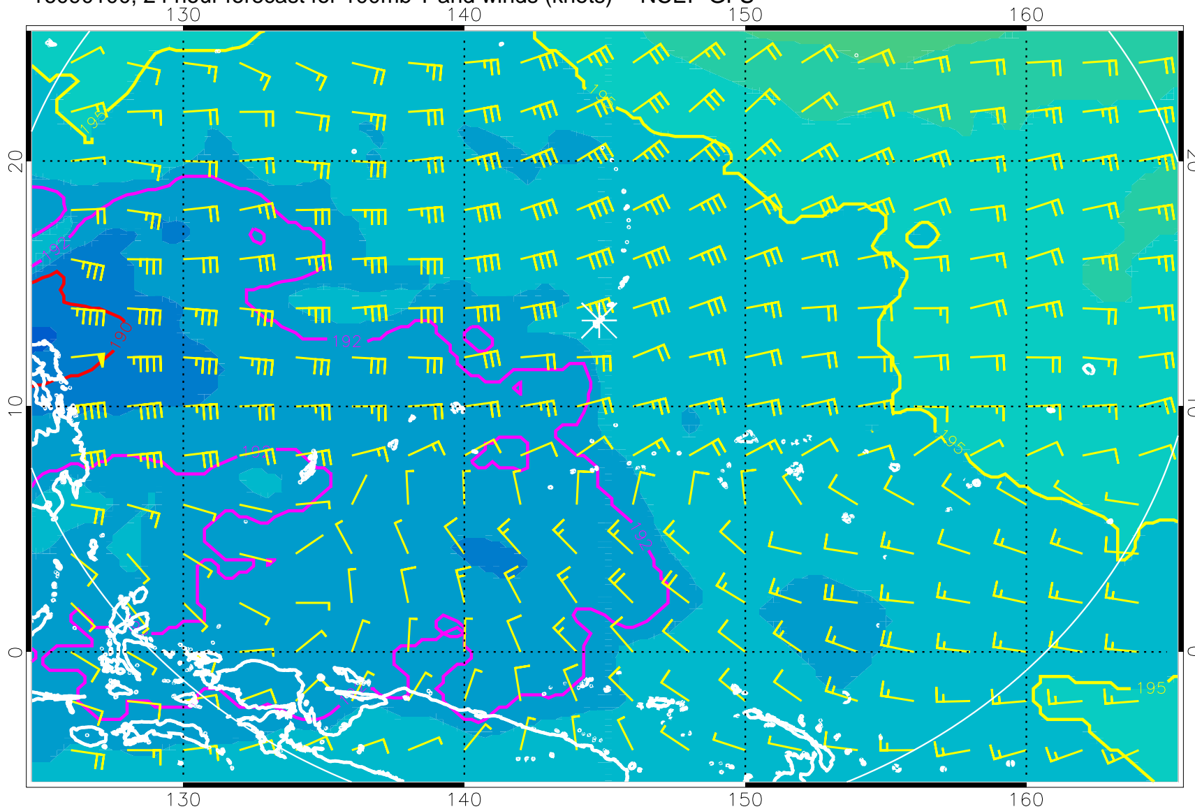
16090100, 24 hour forecast for 100mb T and winds (knots) -- NCEP GFS
