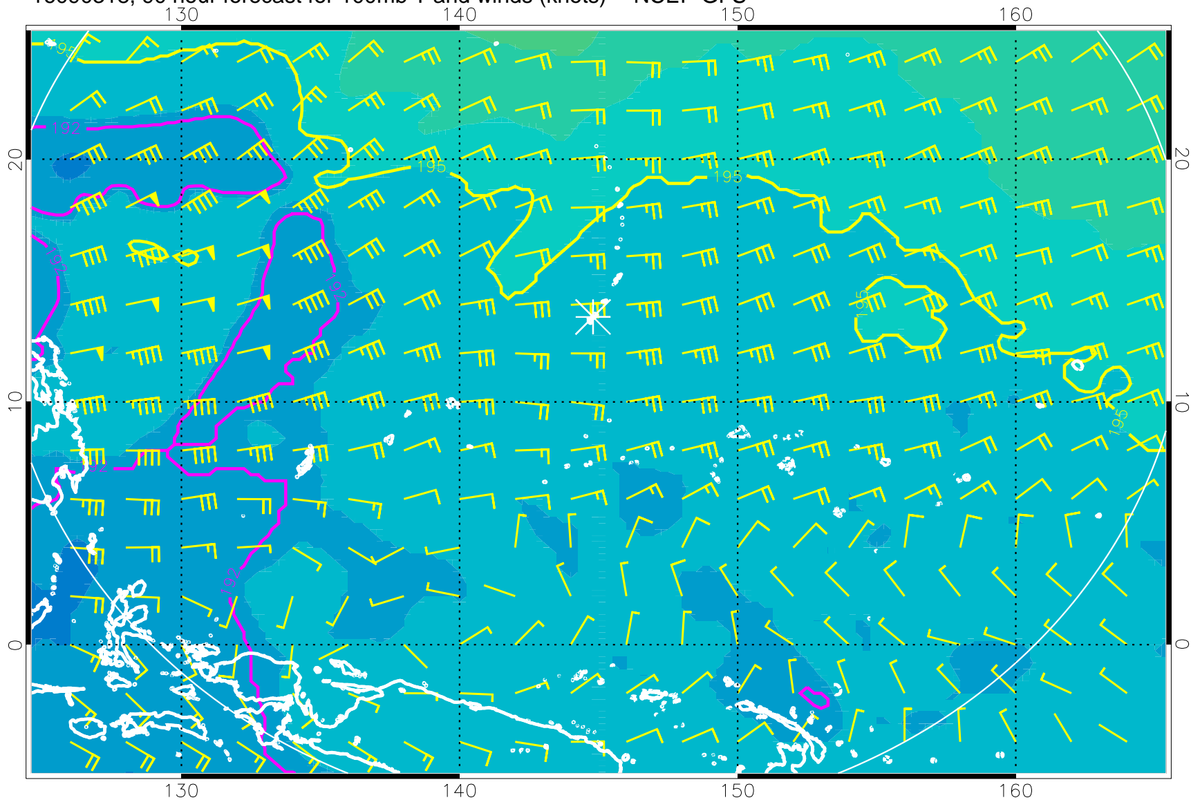
16090318, 90 hour forecast for 100mb T and winds (knots) -- NCEP GFS
