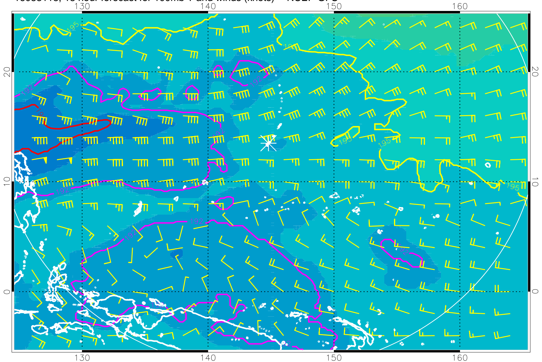
16083118, 18 hour forecast for 100mb T and winds (knots) -- NCEP GFS
