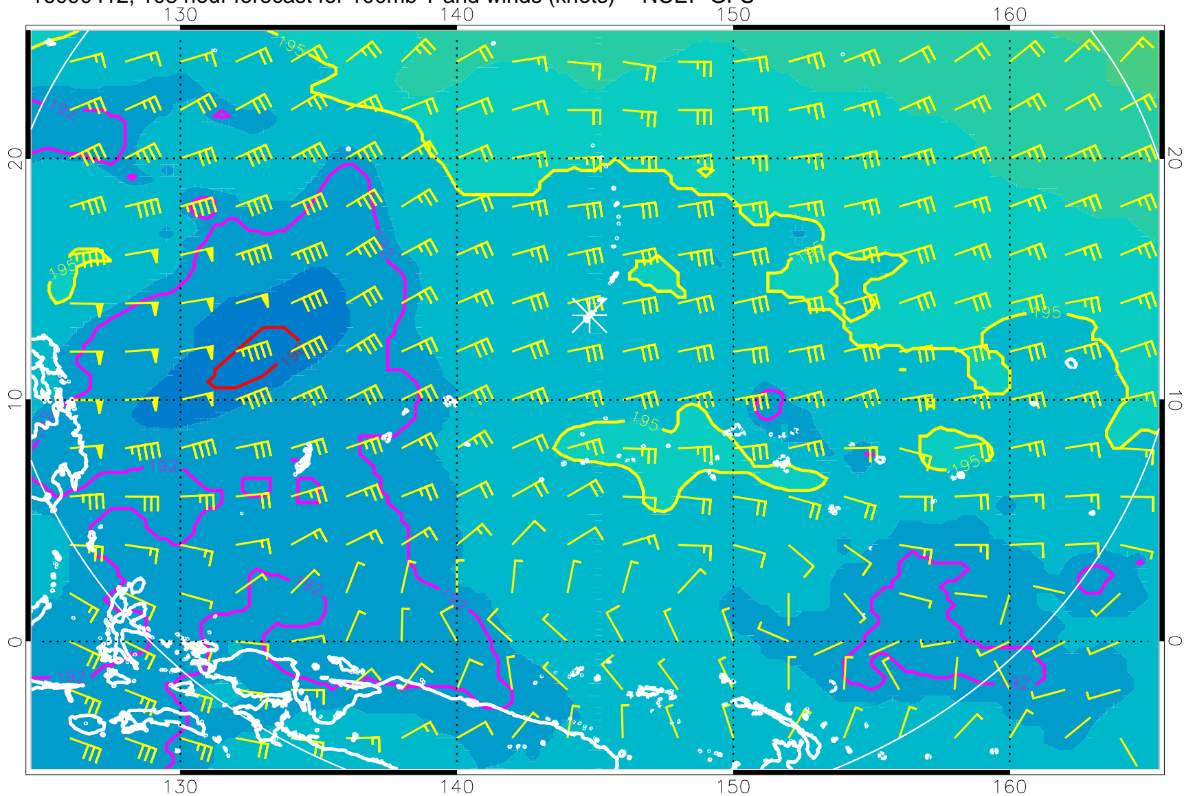
16090412, 108 hour forecast for 100mb T and winds (knots) -- NCEP GFS
