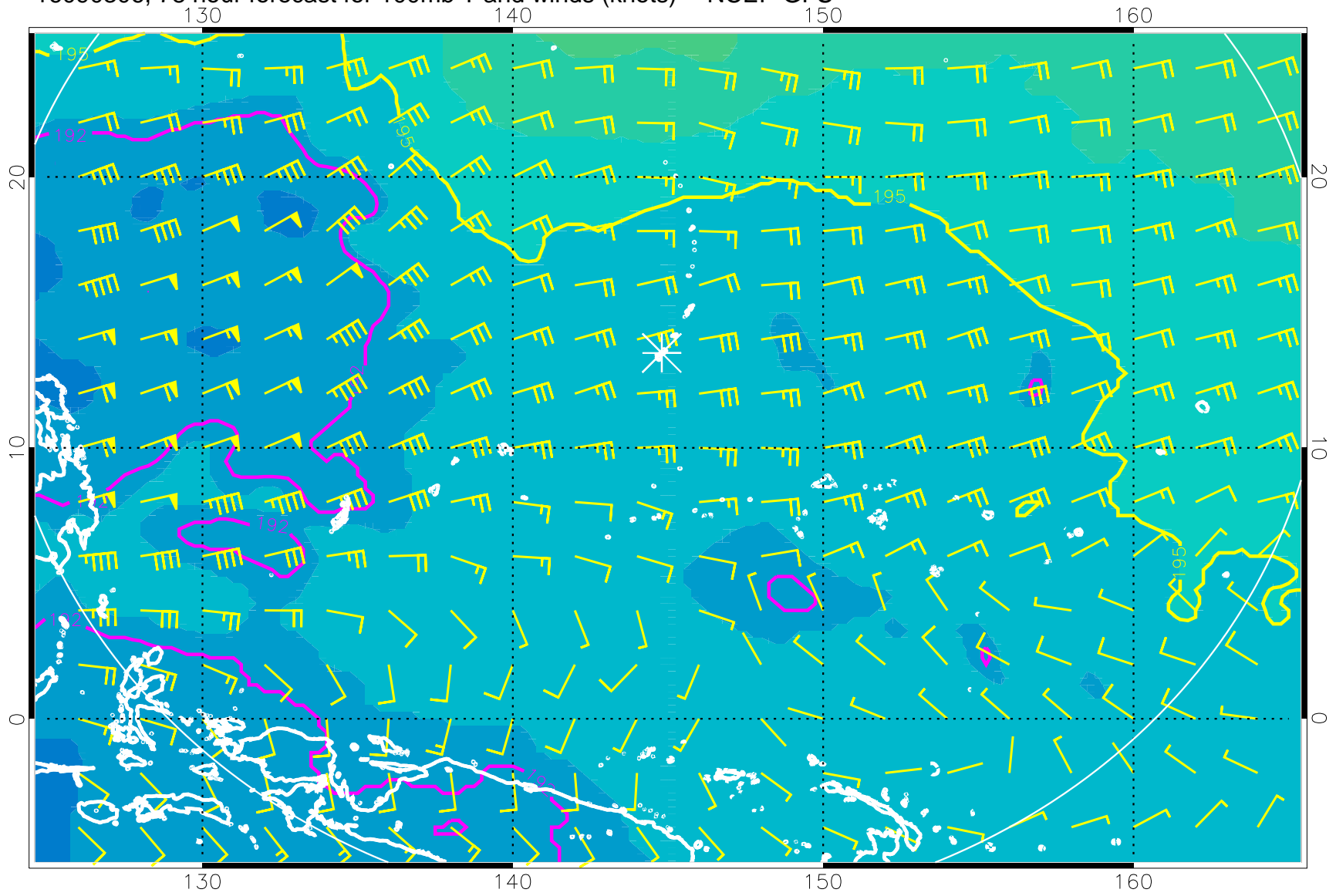
16090306, 78 hour forecast for 100mb T and winds (knots) -- NCEP GFS
