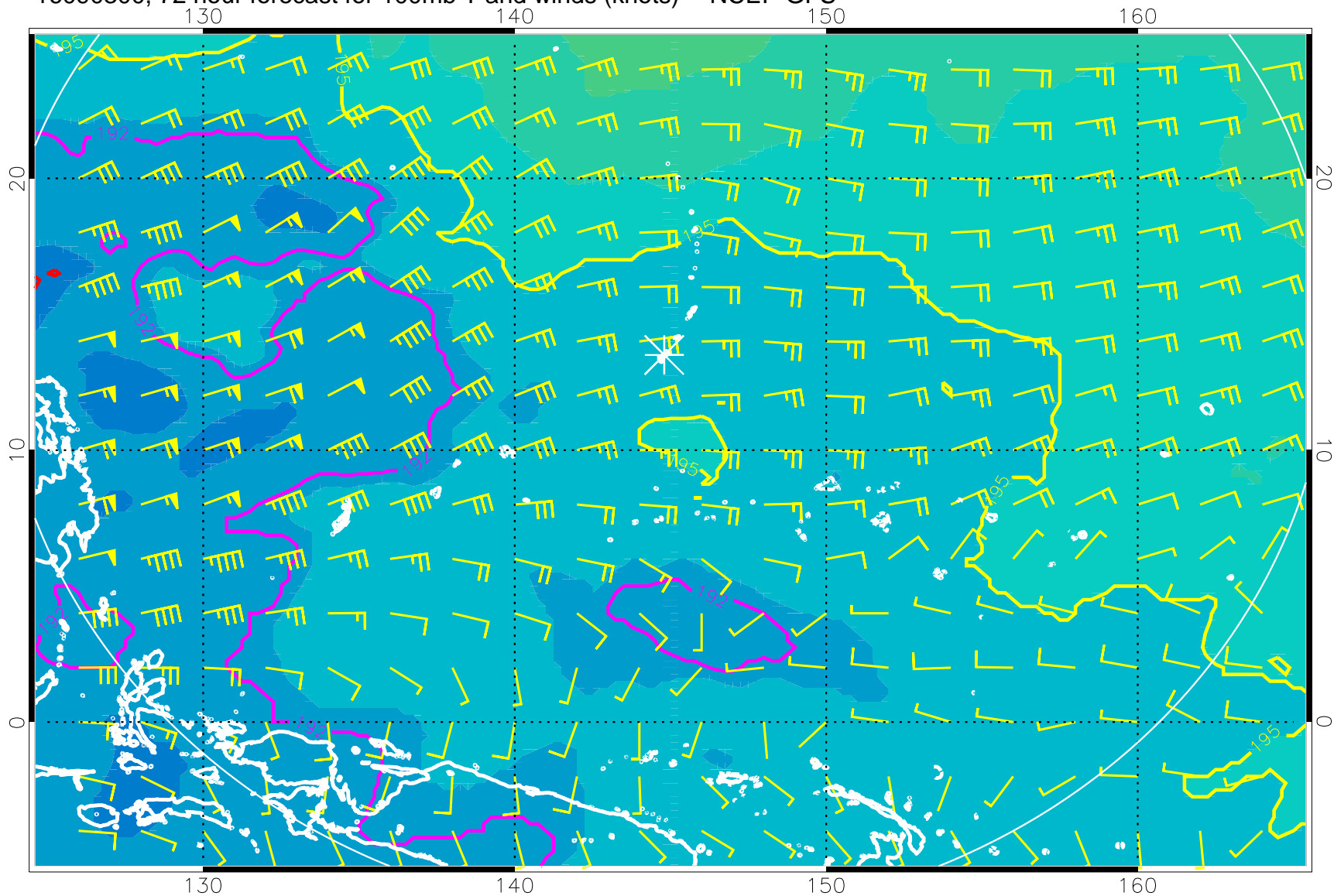
16090300, 72 hour forecast for 100mb T and winds (knots) -- NCEP GFS
