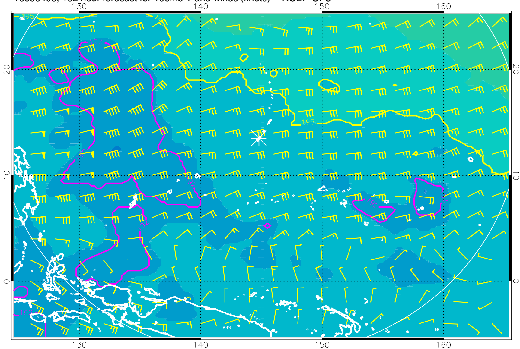
16090406, 102 hour forecast for 100mb T and winds (knots) -- NCEP GFS
