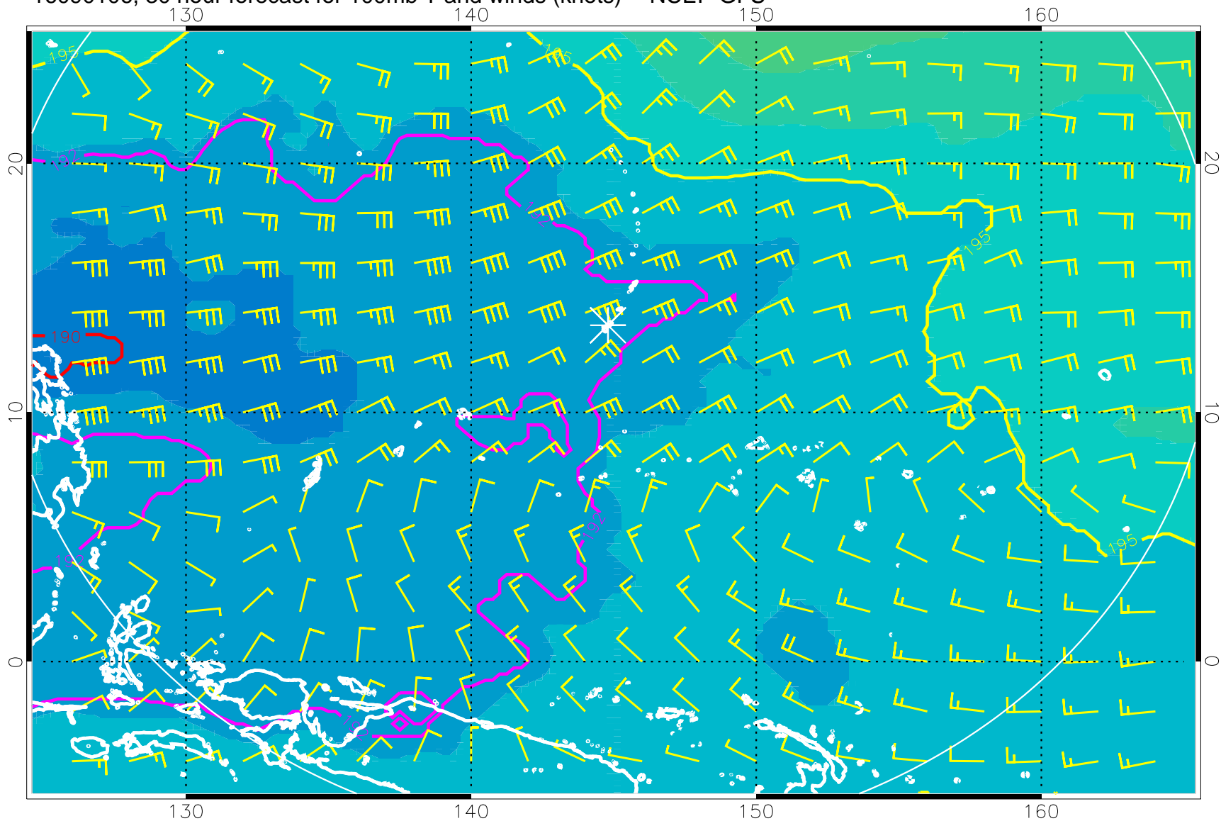
16090106, 30 hour forecast for 100mb T and winds (knots) -- NCEP GFS
