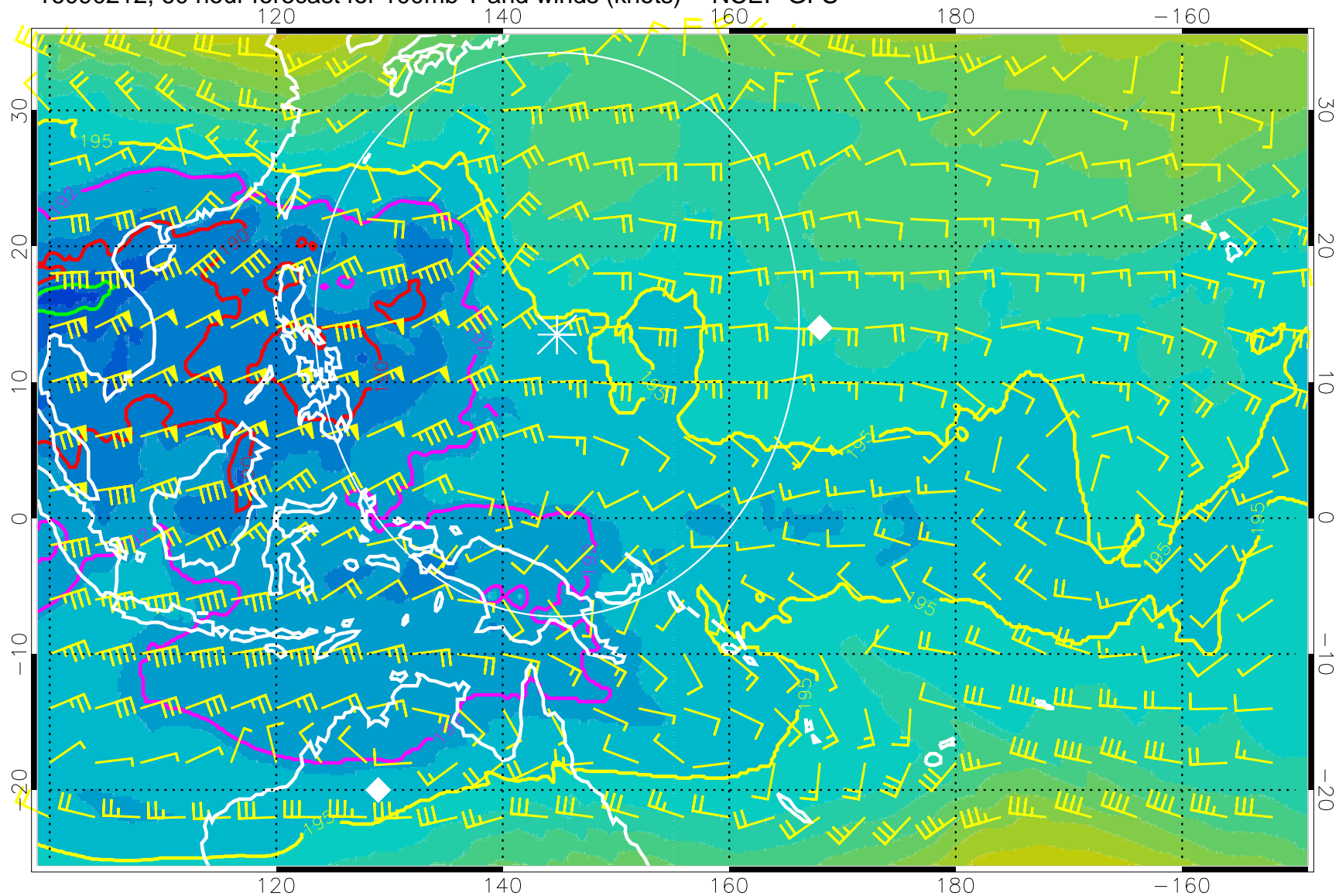
16090212, 60 hour forecast for 100mb T and winds (knots) -- NCEP GFS
