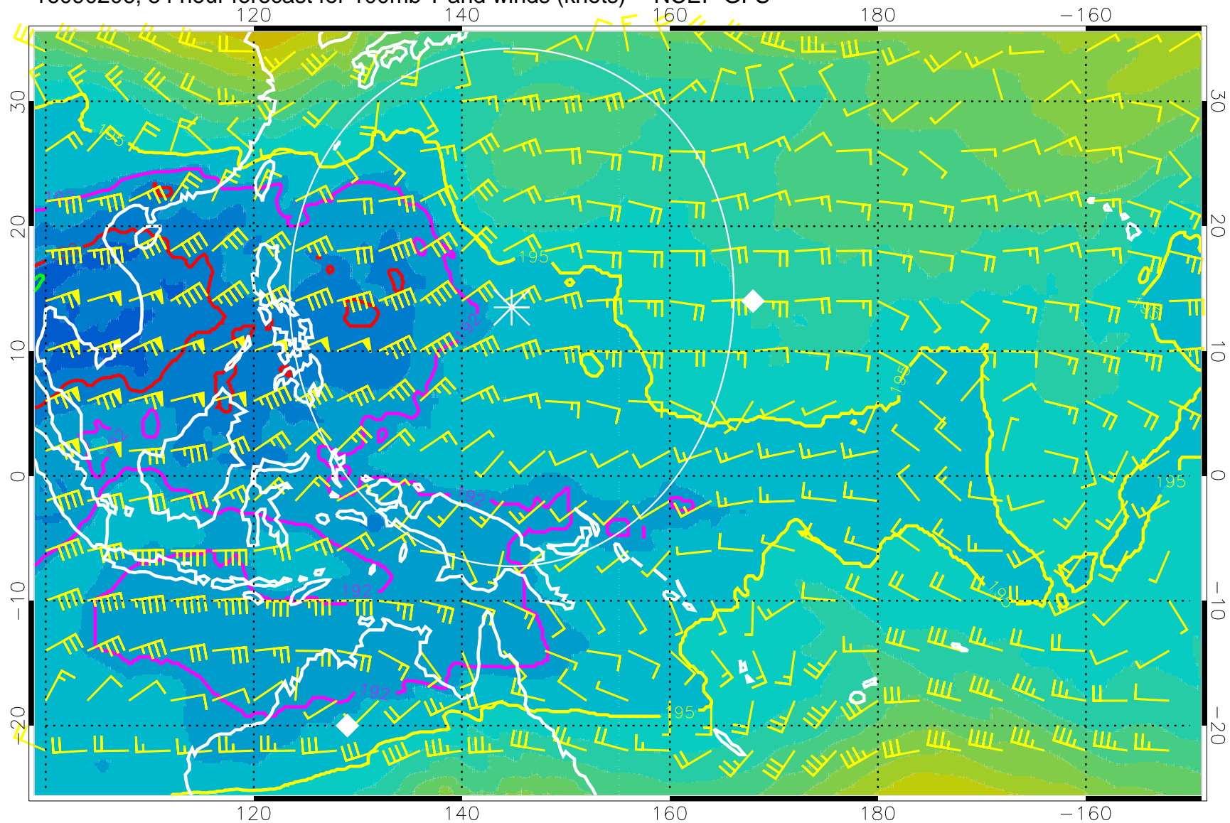
16090206, 54 hour forecast for 100mb T and winds (knots) -- NCEP GFS
