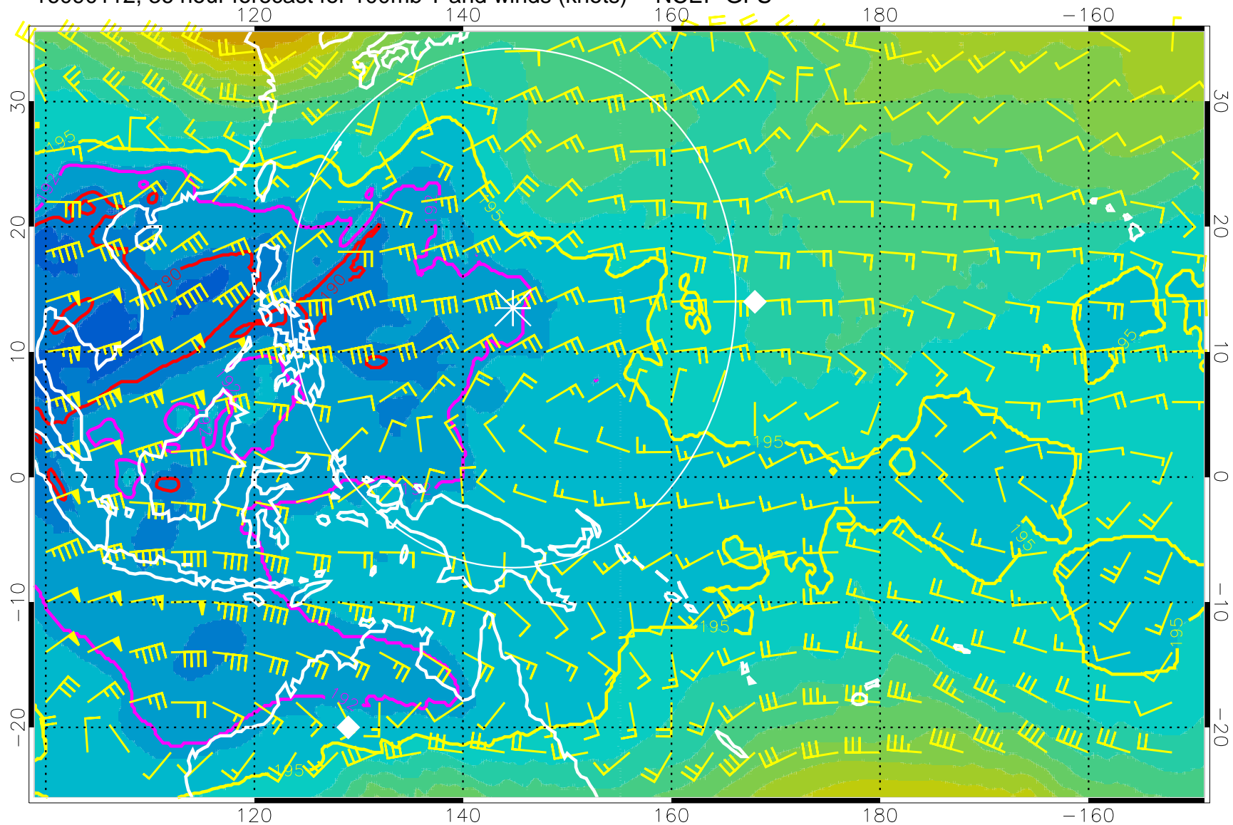
16090112, 36 hour forecast for 100mb T and winds (knots) -- NCEP GFS
