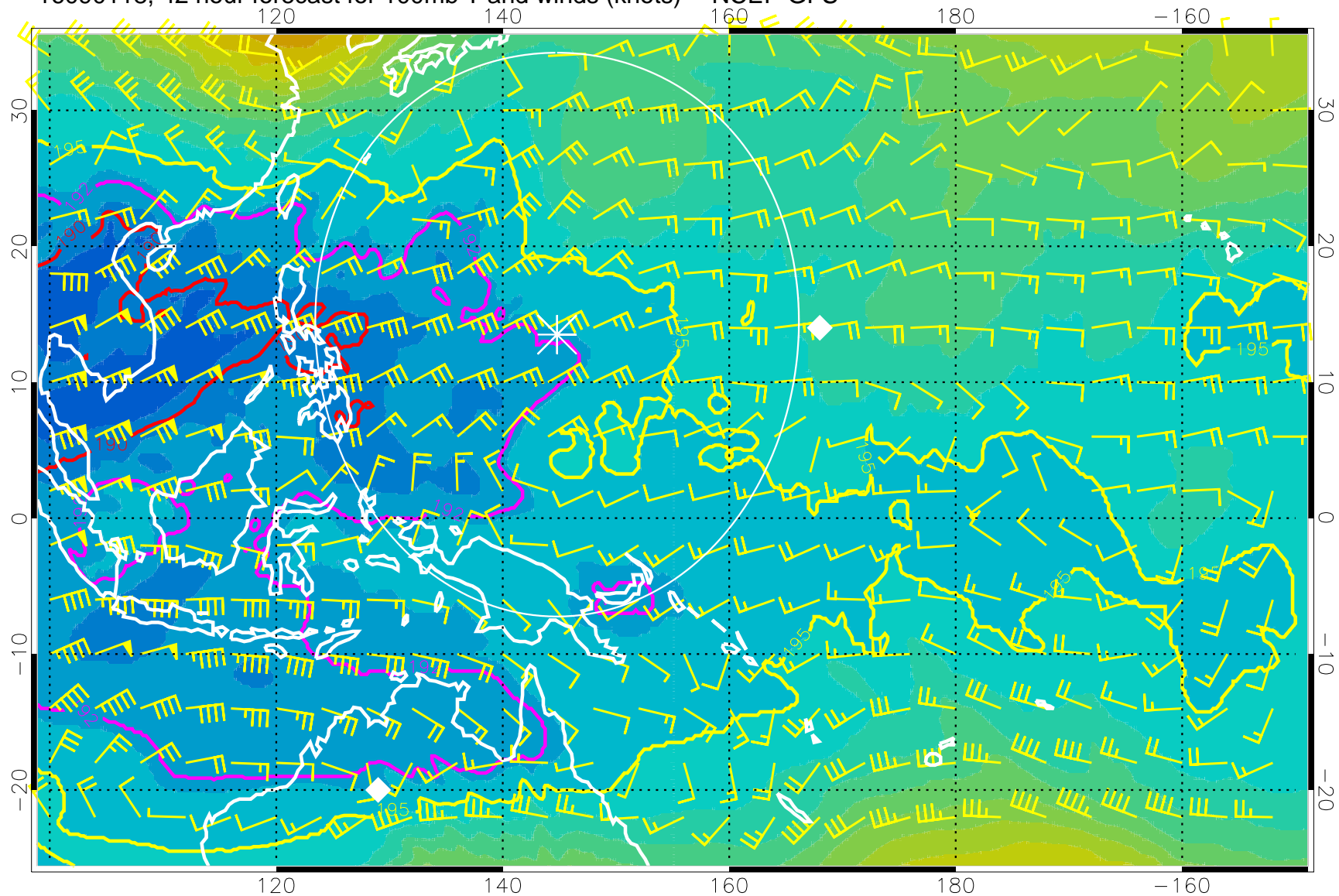
16090118, 42 hour forecast for 100mb T and winds (knots) -- NCEP GFS
