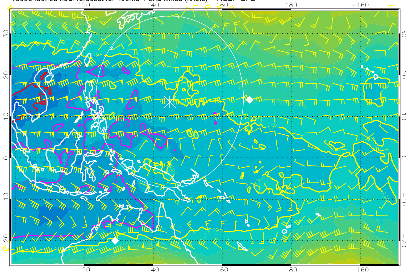
16090400, 96 hour forecast for 100mb T and winds (knots) -- NCEP GFS
