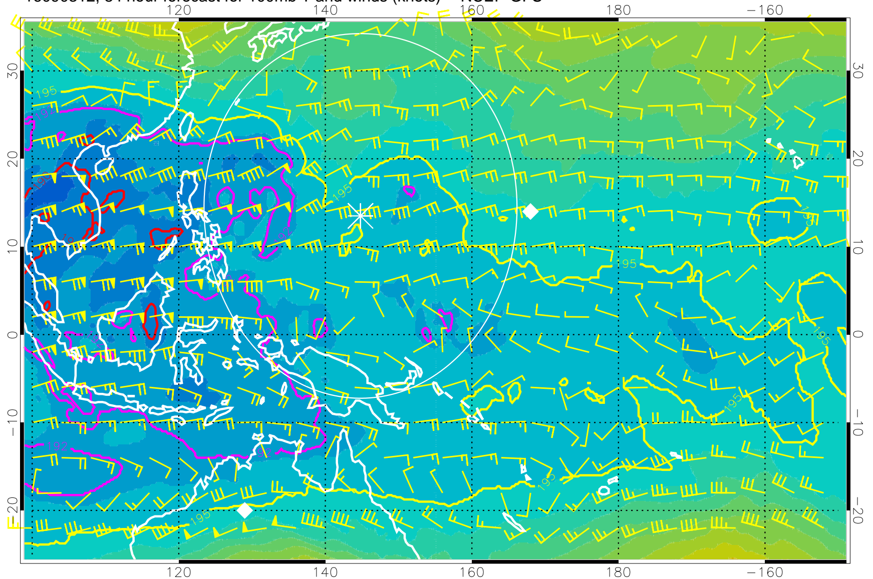
16090312, 84 hour forecast for 100mb T and winds (knots) -- NCEP GFS
