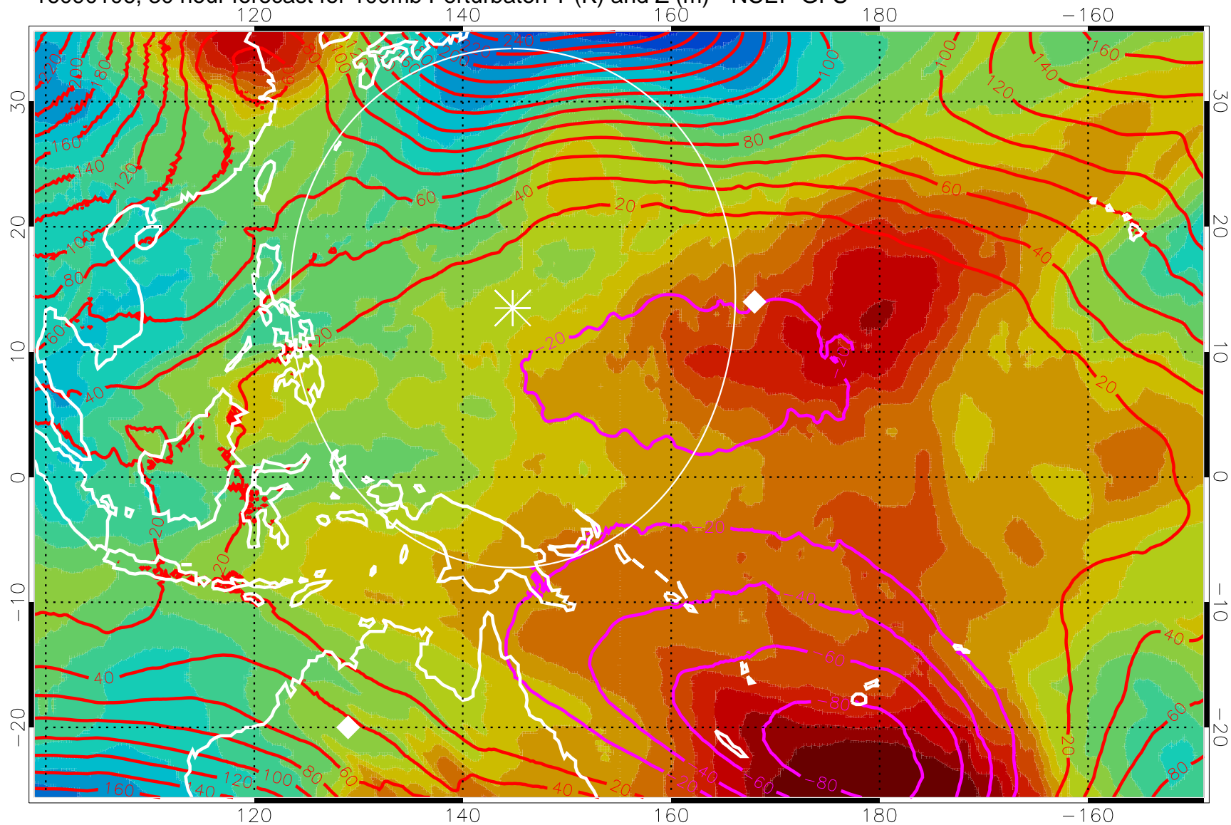
16090106, 30 hour forecast for 100mb Perturbaton T (K) and Z (m)-- NCEP GFS
