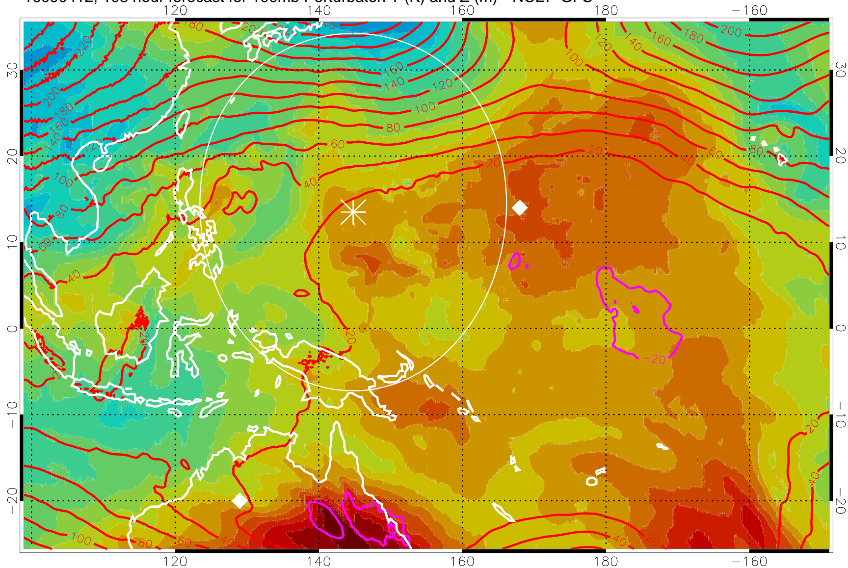
16090412, 108 hour forecast for 100mb Perturbaton T (K) and Z (m)-- NCEP GFS
