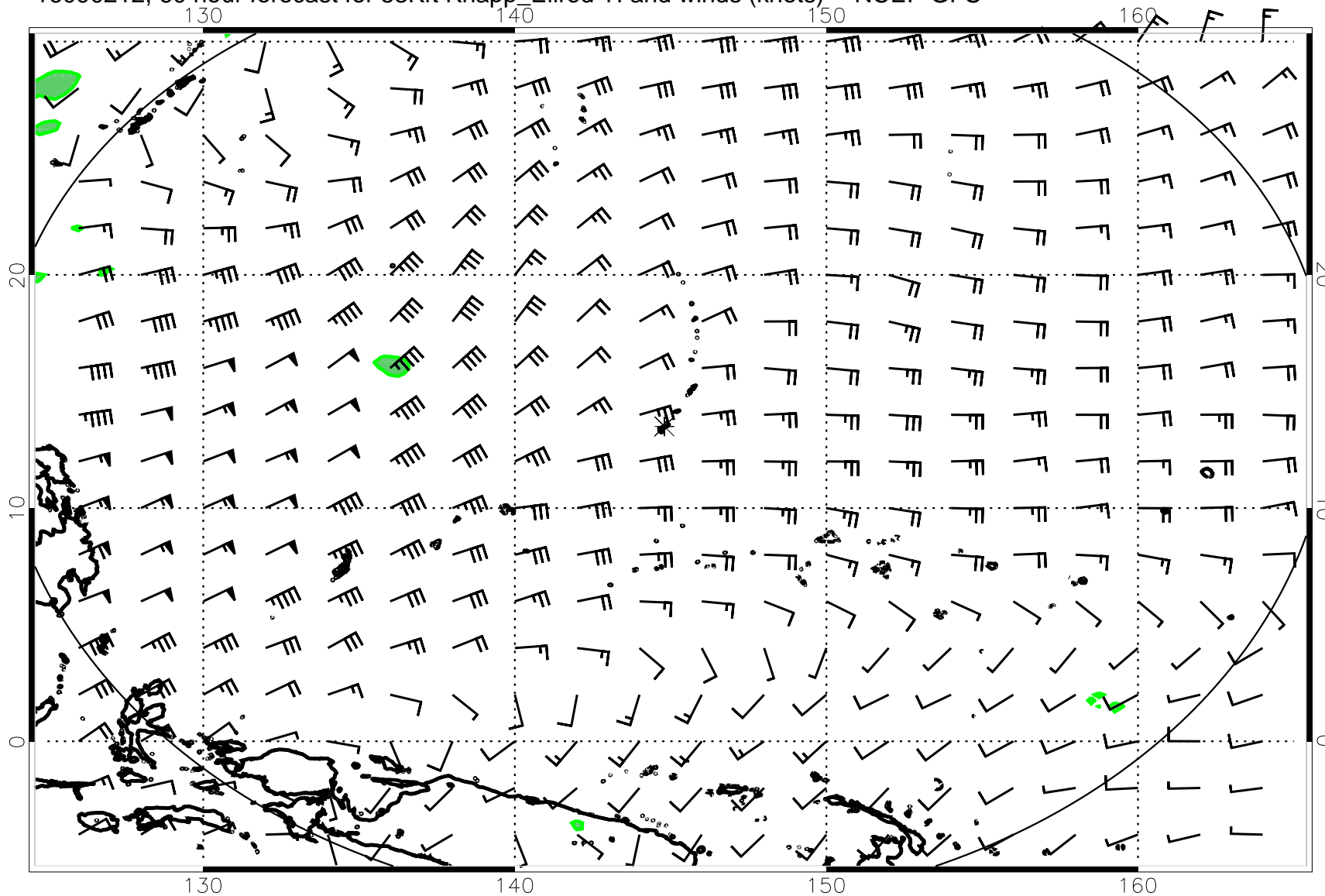
16090212, 60 hour forecast for 53Kft Knapp_Ellrod TI and winds (knots) -- NCEP GFS
