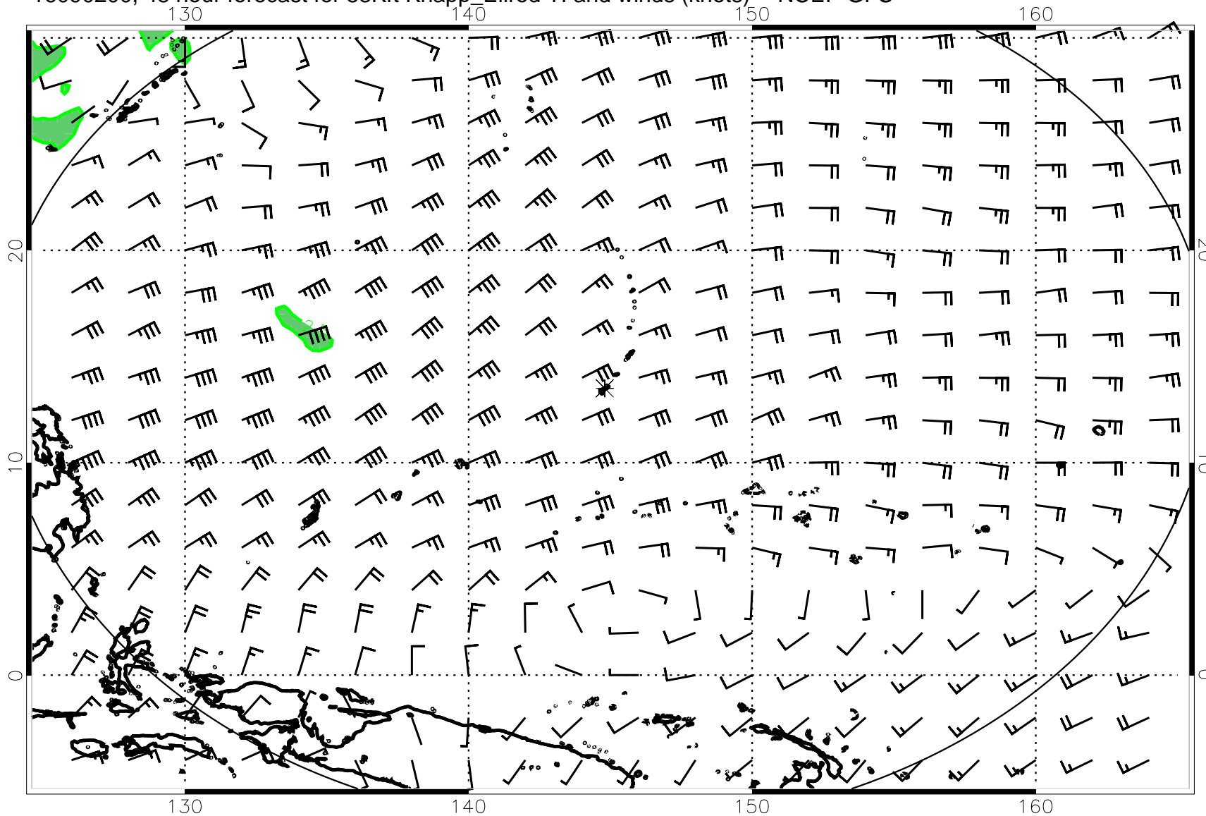
16090200, 48 hour forecast for 53Kft Knapp_Ellrod TI and winds (knots) -- NCEP GFS
