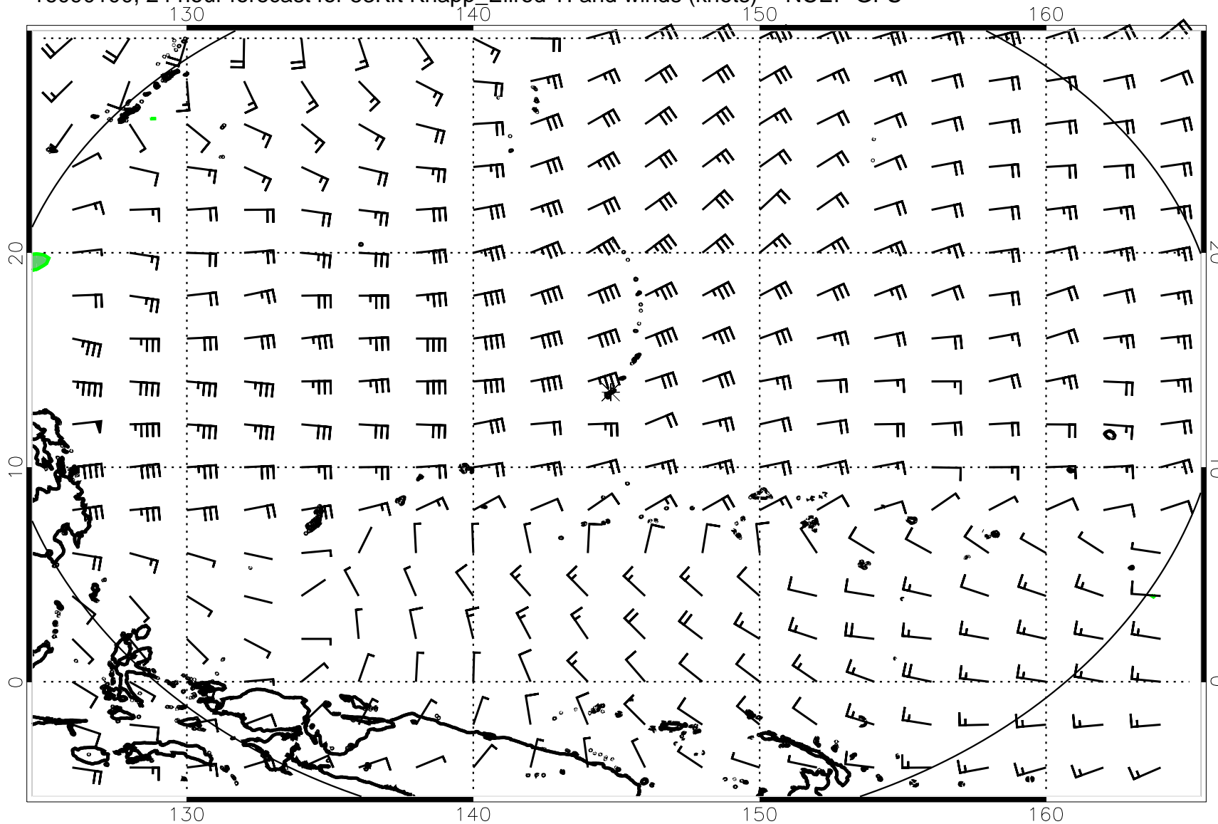
16090100, 24 hour forecast for 53Kft Knapp_Ellrod TI and winds (knots) -- NCEP GFS
