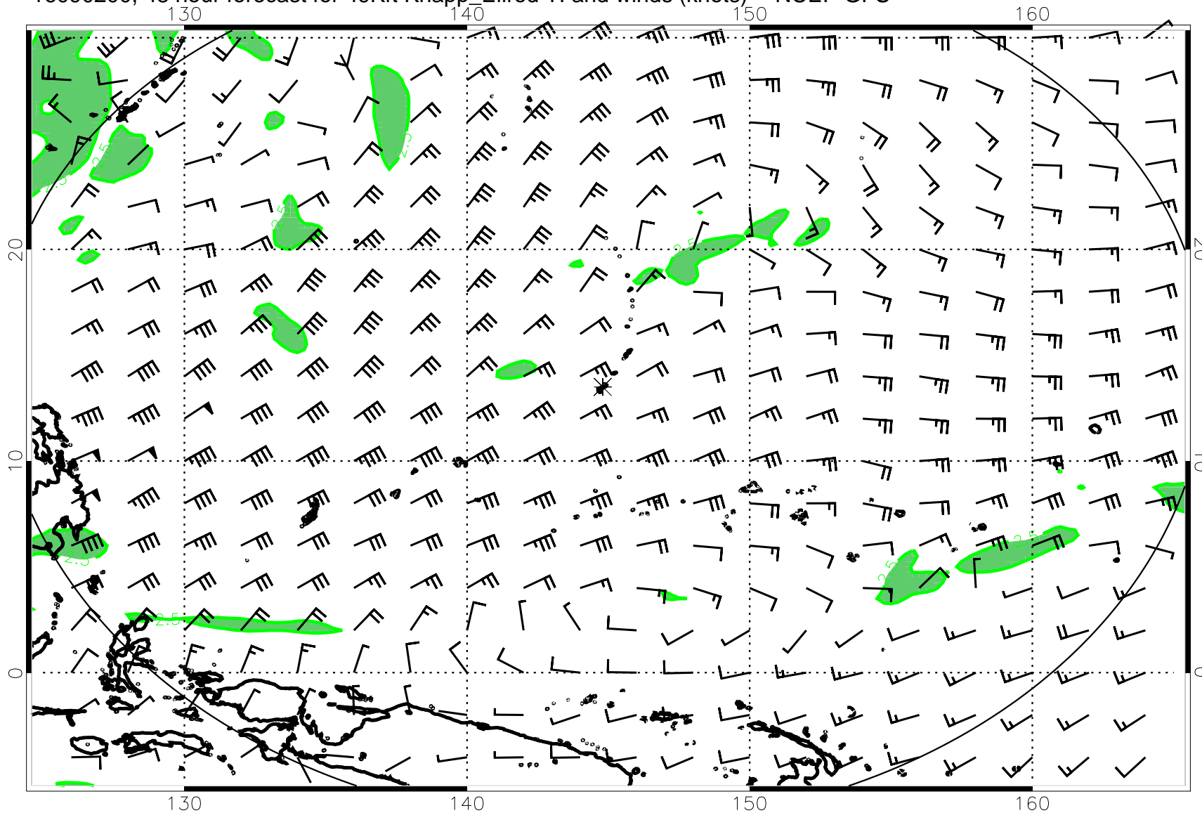
16090200, 48 hour forecast for 49Kft Knapp_Ellrod TI and winds (knots) -- NCEP GFS
