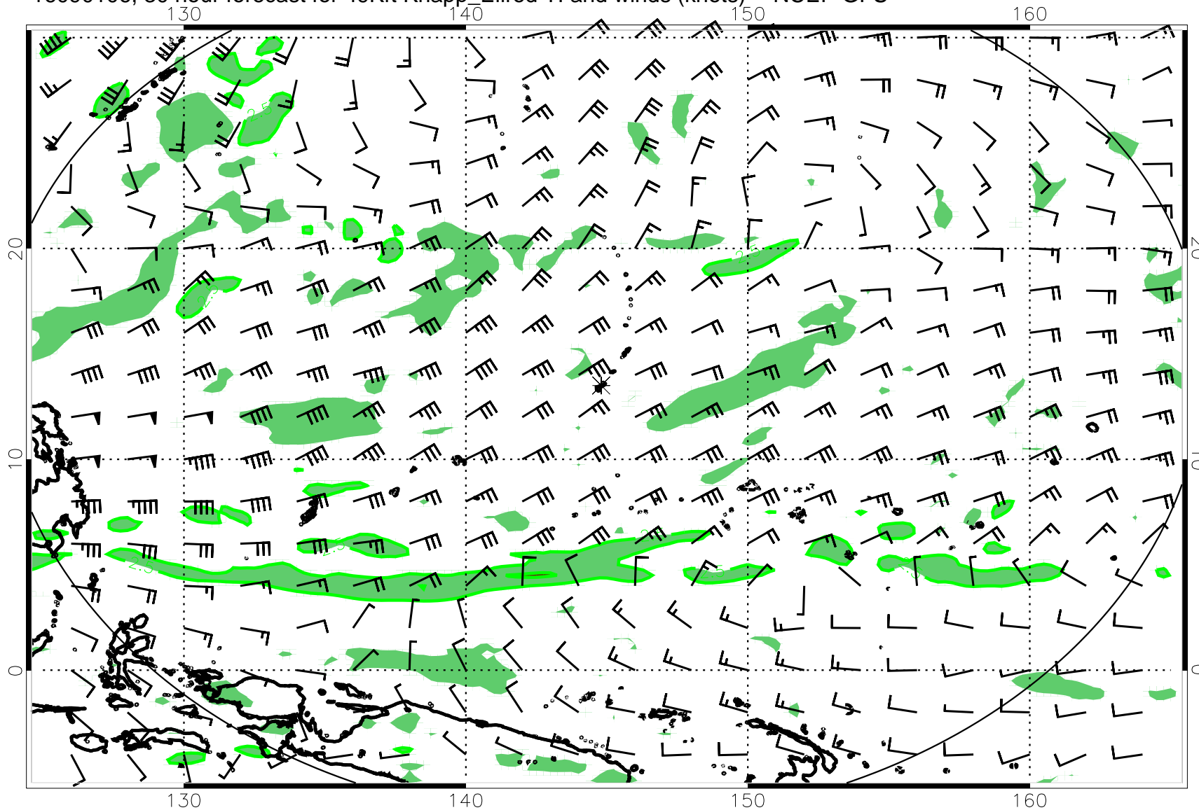
16090106, 30 hour forecast for 49Kft Knapp_Ellrod TI and winds (knots) -- NCEP GFS
