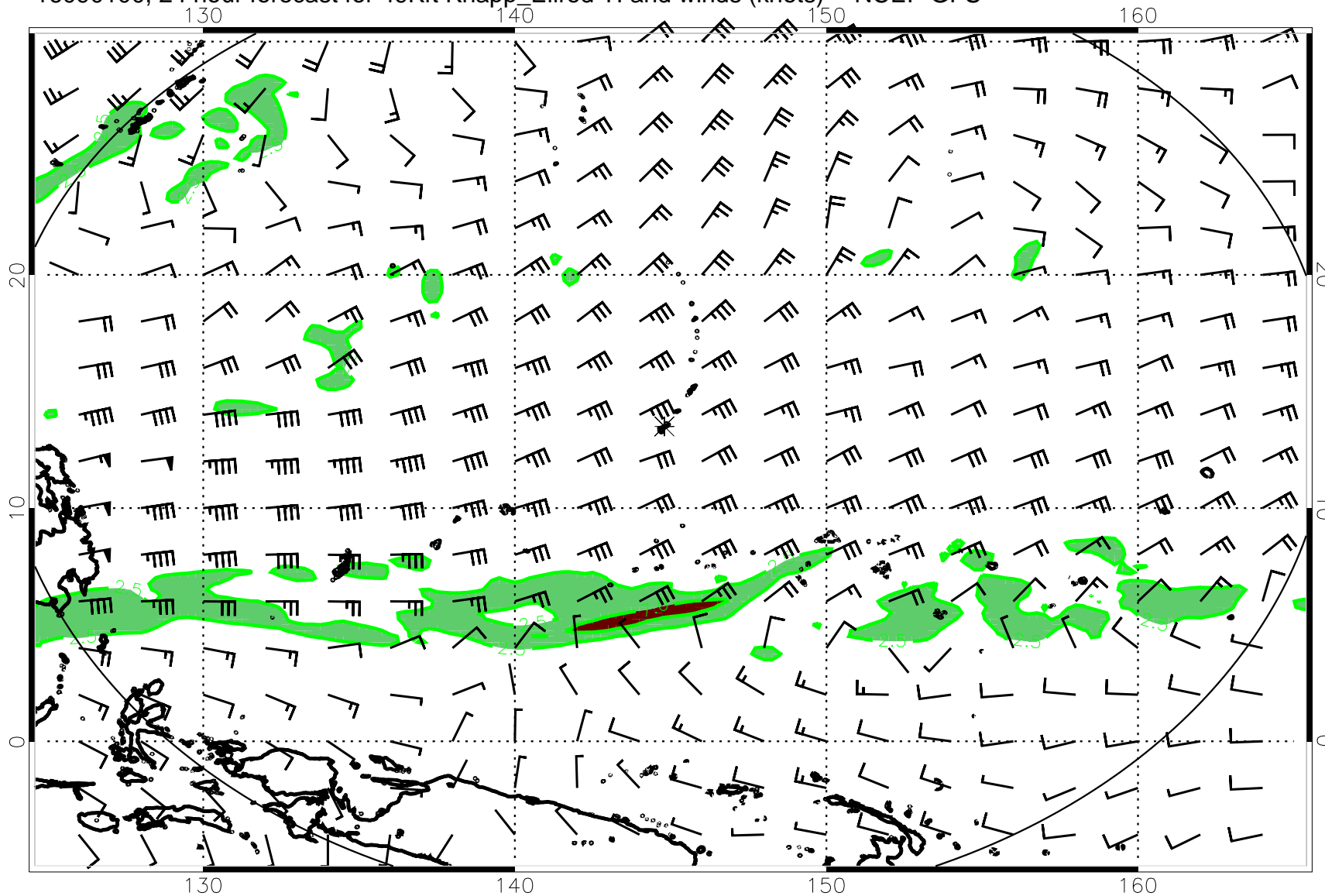
16090100, 24 hour forecast for 49Kft Knapp_Ellrod TI and winds (knots) -- NCEP GFS
