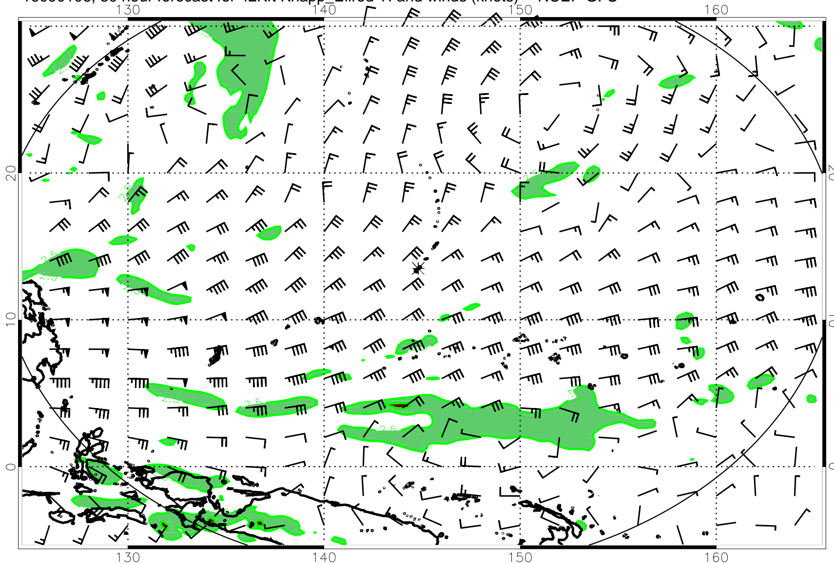
16090106, 30 hour forecast for 42Kft Knapp_Ellrod TI and winds (knots) -- NCEP GFS
