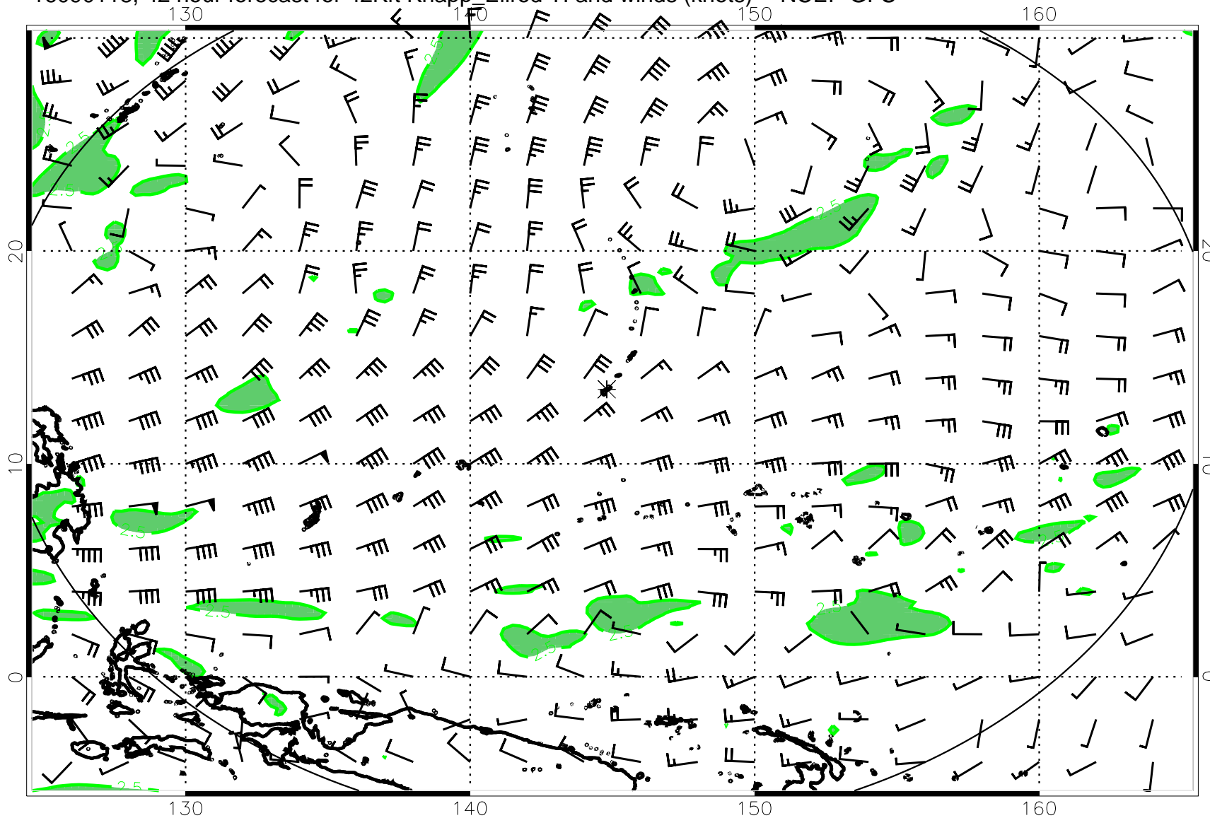
16090118, 42 hour forecast for 42Kft Knapp_Ellrod TI and winds (knots) -- NCEP GFS
