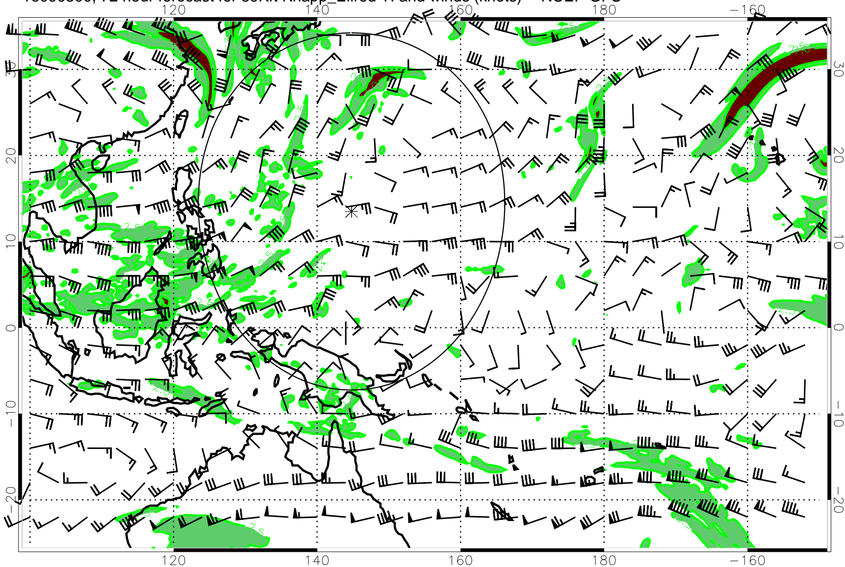
16090300, 72 hour forecast for 39Kft Knapp_Ellrod TI and winds (knots) -- NCEP GFS
