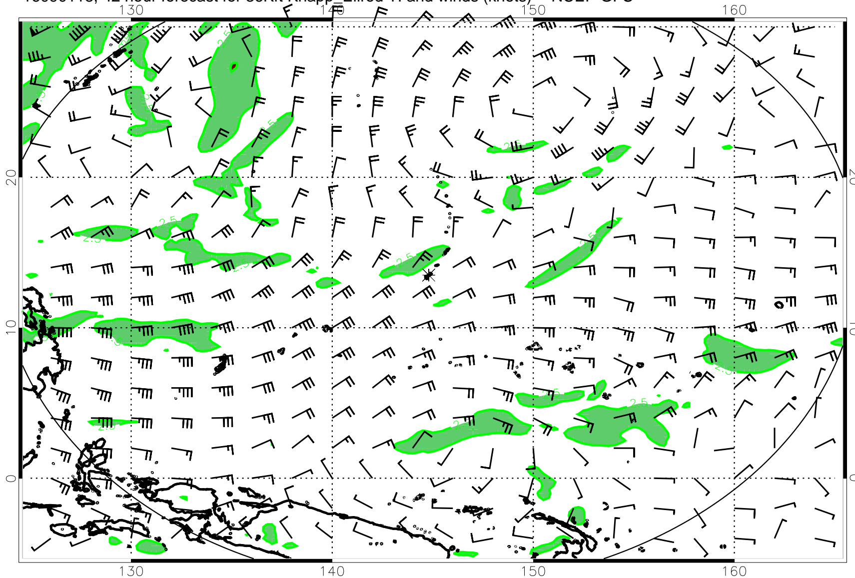
16090118, 42 hour forecast for 36Kft Knapp_Ellrod TI and winds (knots) -- NCEP GFS
