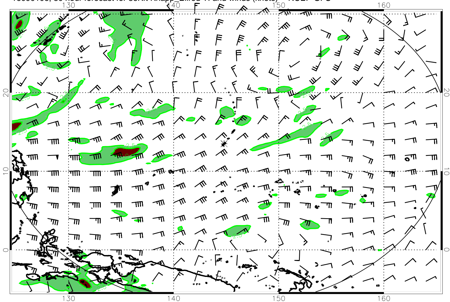
16090106, 30 hour forecast for 36Kft Knapp_Ellrod TI and winds (knots) -- NCEP GFS
