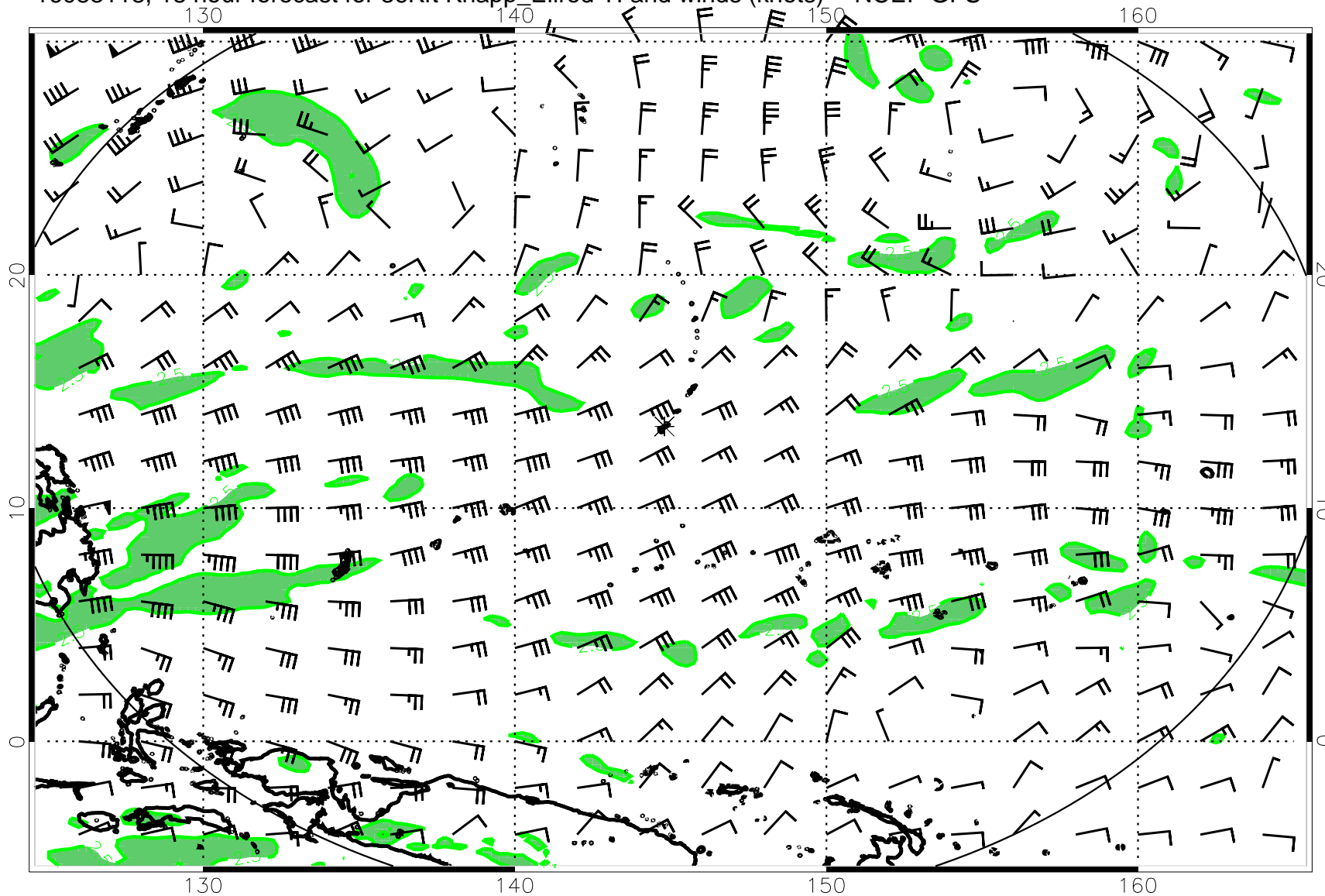
16083118, 18 hour forecast for 36Kft Knapp_Ellrod TI and winds (knots) -- NCEP GFS
