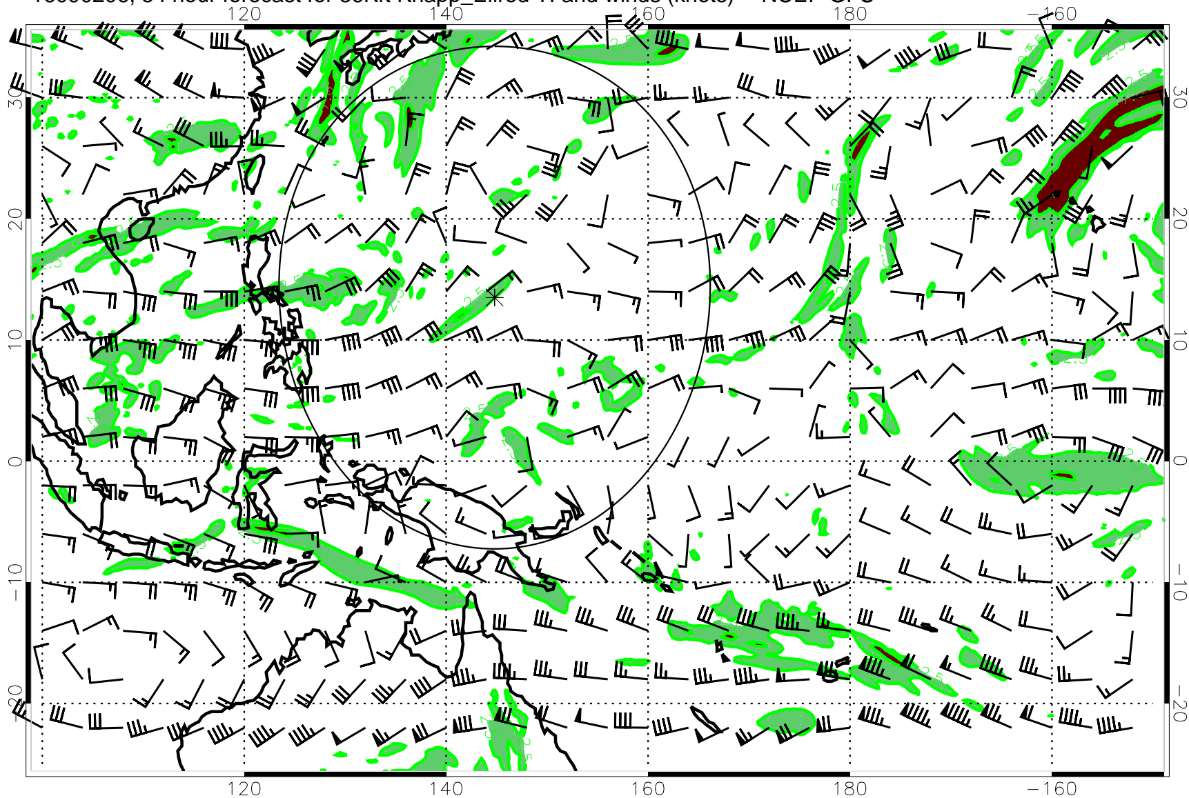
16090206, 54 hour forecast for 36Kft Knapp_Ellrod TI and winds (knots) -- NCEP GFS
