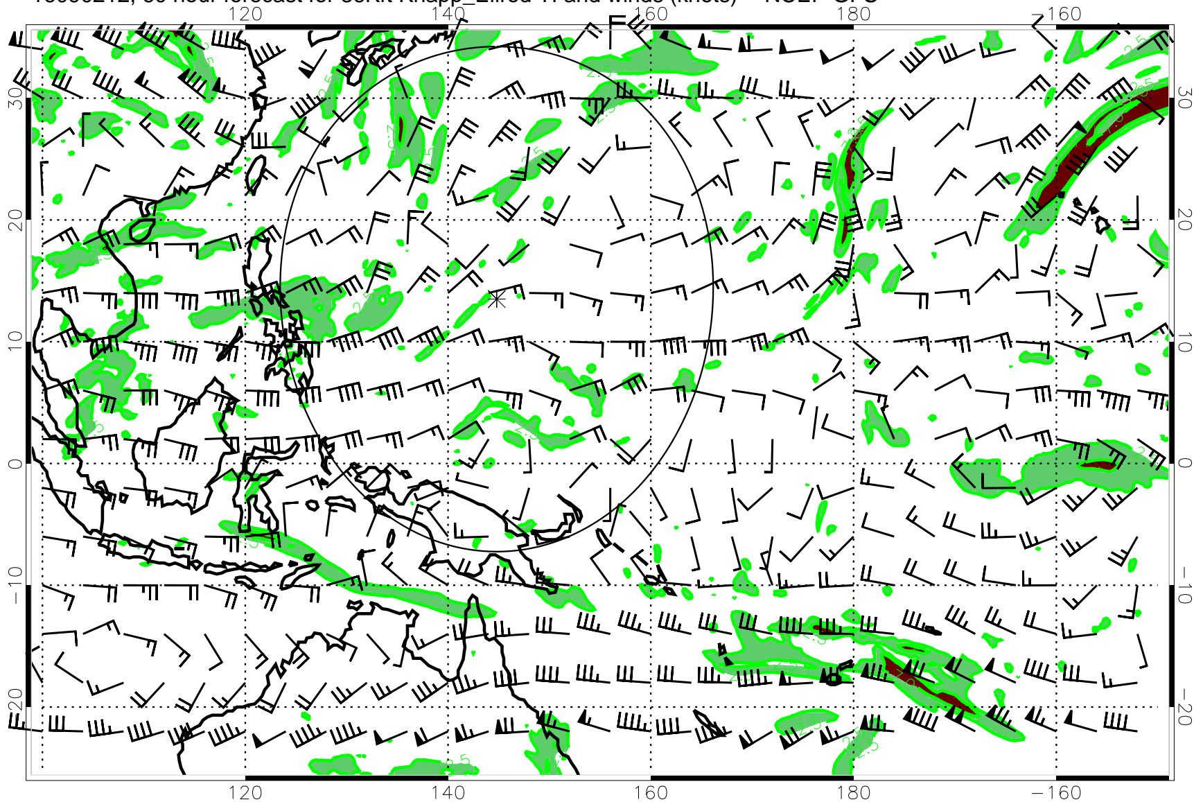
16090212, 60 hour forecast for 36Kft Knapp_Ellrod TI and winds (knots) -- NCEP GFS
