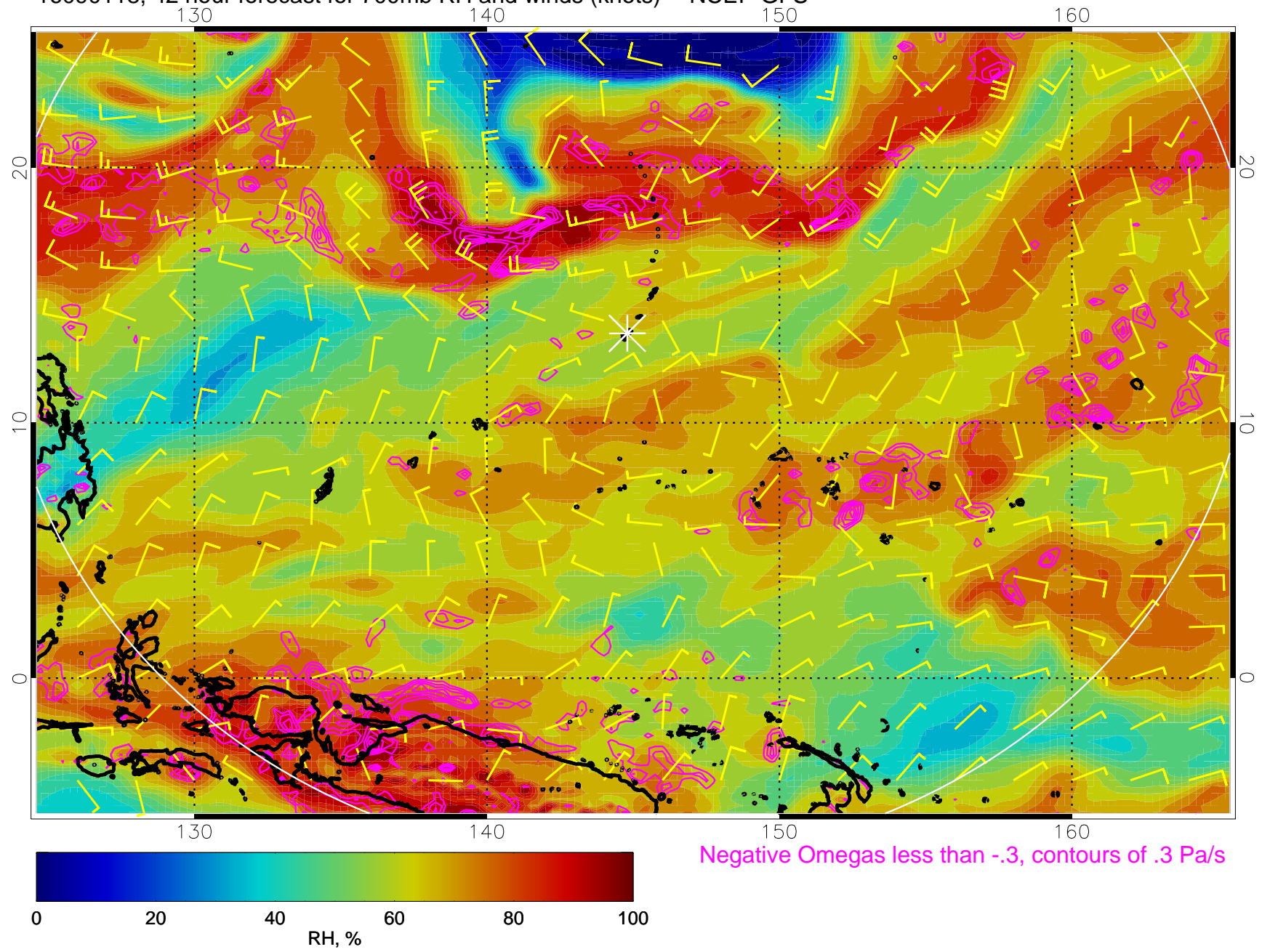
16090118, 42 hour forecast for 700mb RH and winds (knots) -- NCEP GFS
