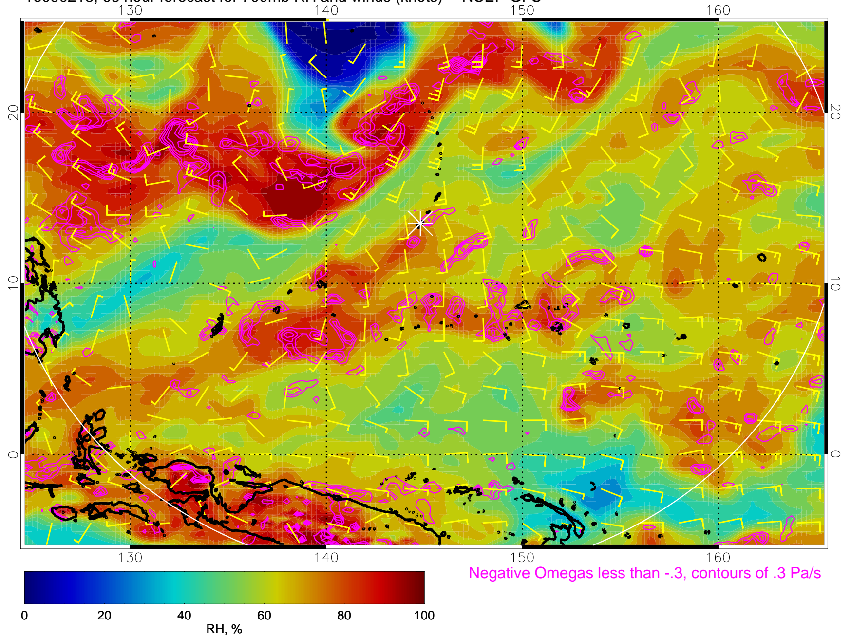
16090218, 66 hour forecast for 700mb RH and winds (knots) -- NCEP GFS
