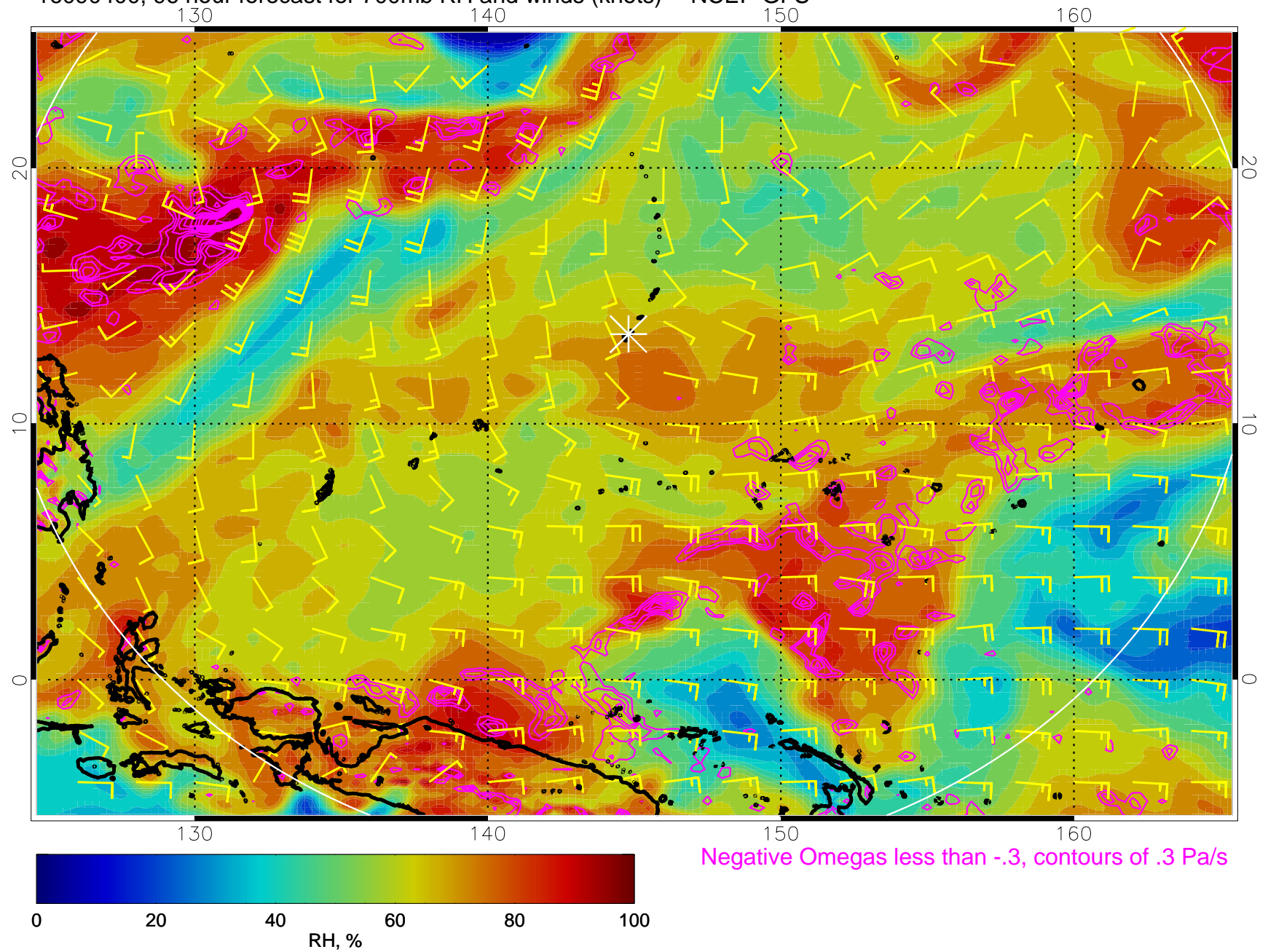
16090400, 96 hour forecast for 700mb RH and winds (knots) -- NCEP GFS
