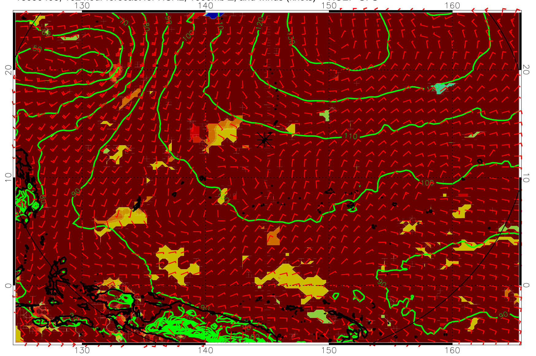
16090406, 102 hour forecast for HCAL, 1000mb Z, and winds (knots) -- NCEP GFS
