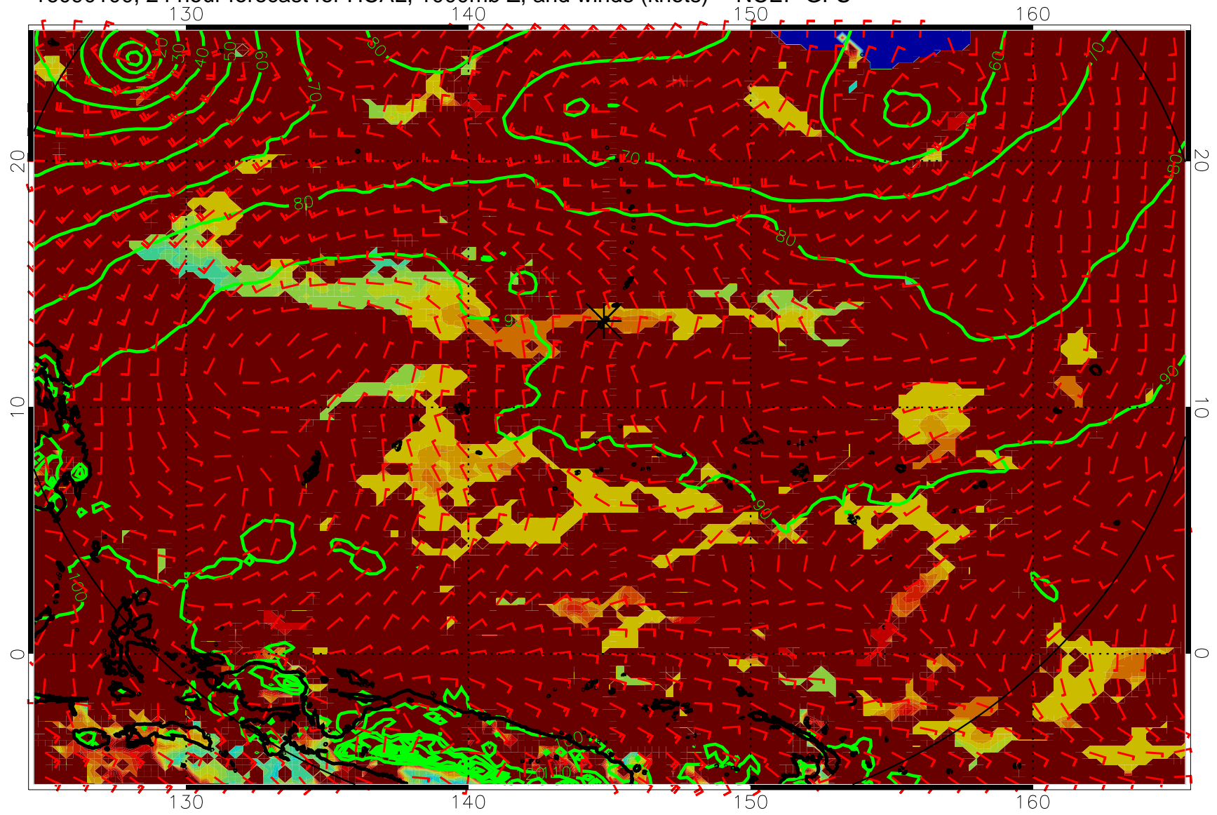
16090100, 24 hour forecast for HCAL, 1000mb Z, and winds (knots) -- NCEP GFS
