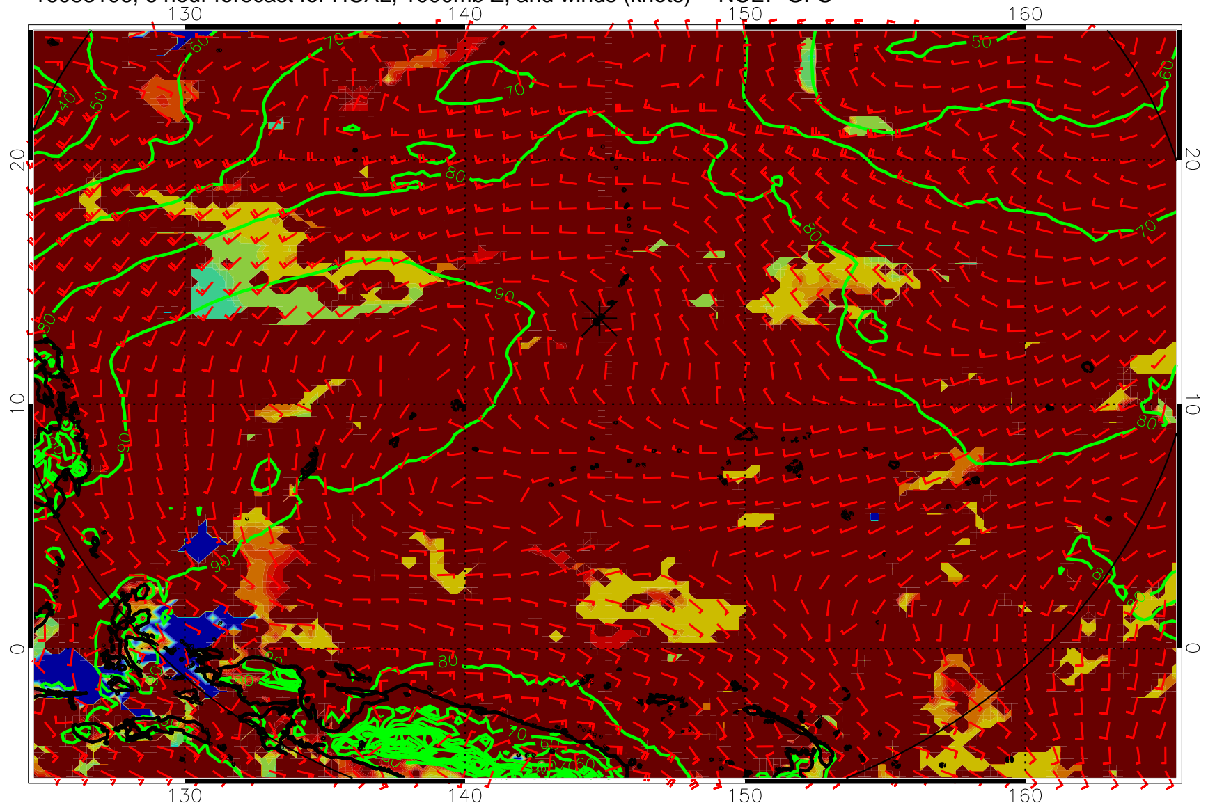
16083106, 6 hour forecast for HCAL, 1000mb Z, and winds (knots) -- NCEP GFS
