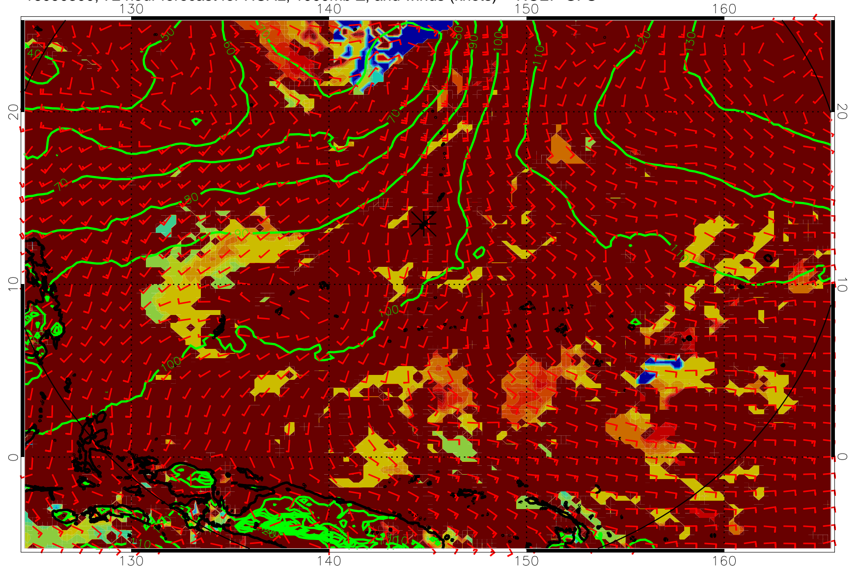
16090300, 72 hour forecast for HCAL, 1000mb Z, and winds (knots) -- NCEP GFS
