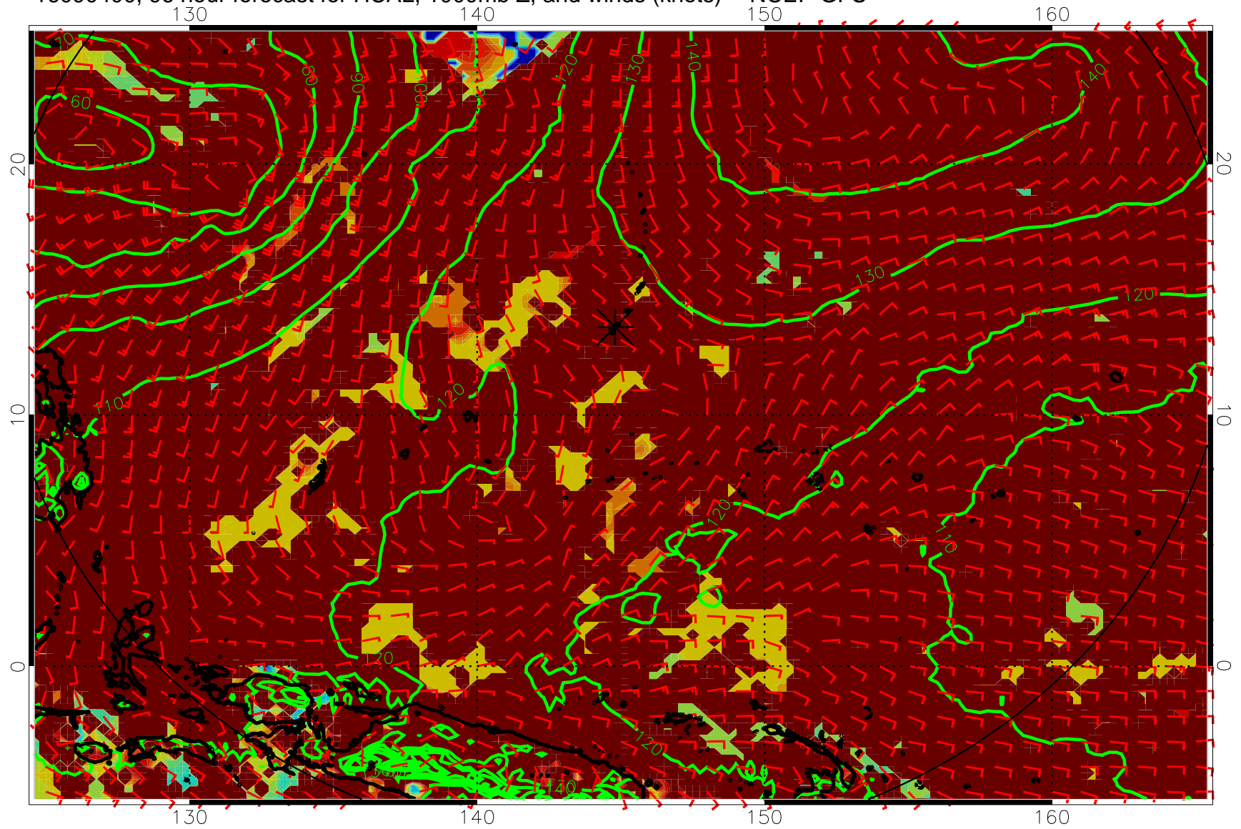
16090400, 96 hour forecast for HCAL, 1000mb Z, and winds (knots) -- NCEP GFS
