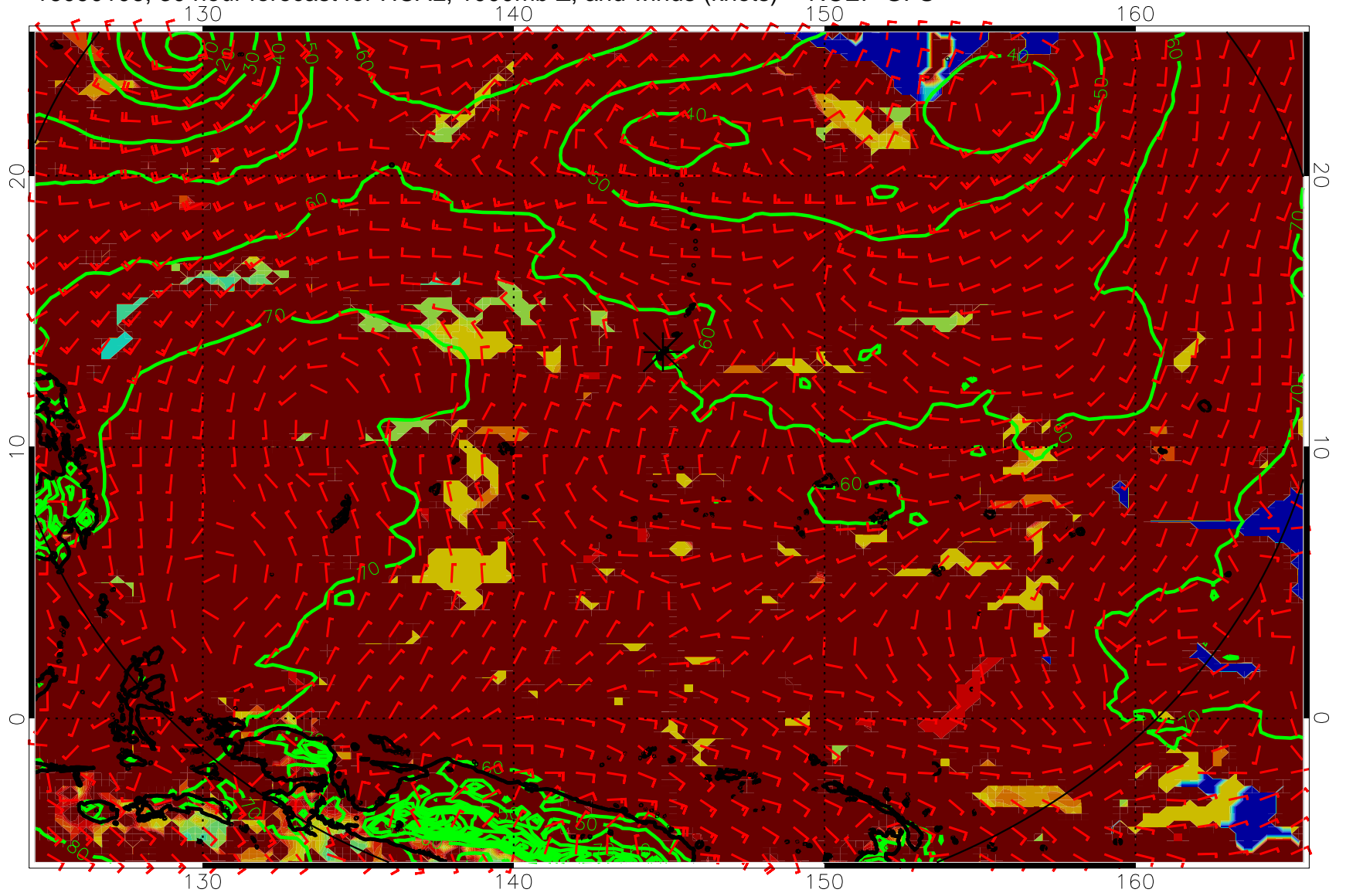
16090106, 30 hour forecast for HCAL, 1000mb Z, and winds (knots) -- NCEP GFS
