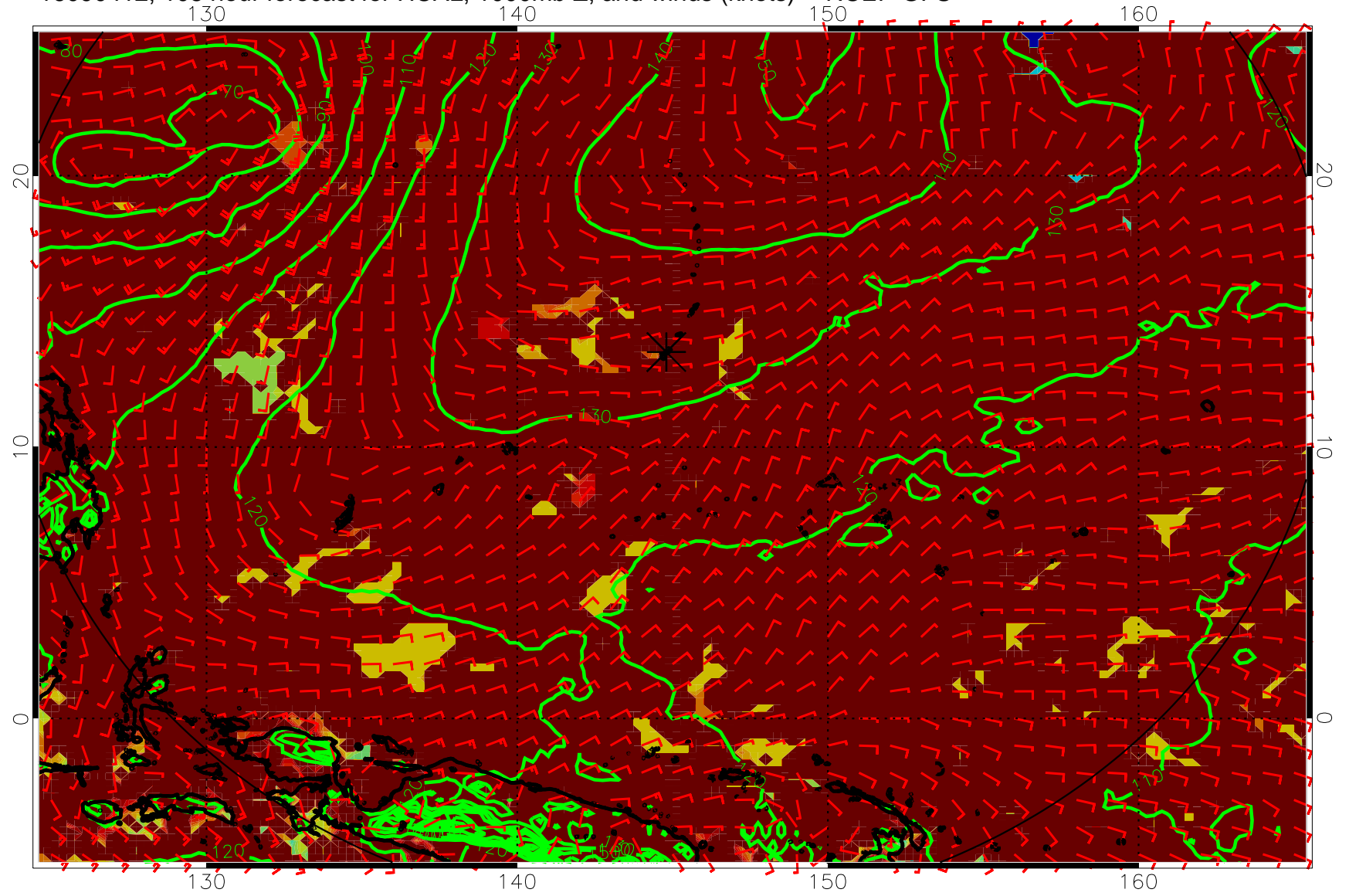
16090412, 108 hour forecast for HCAL, 1000mb Z, and winds (knots) -- NCEP GFS
