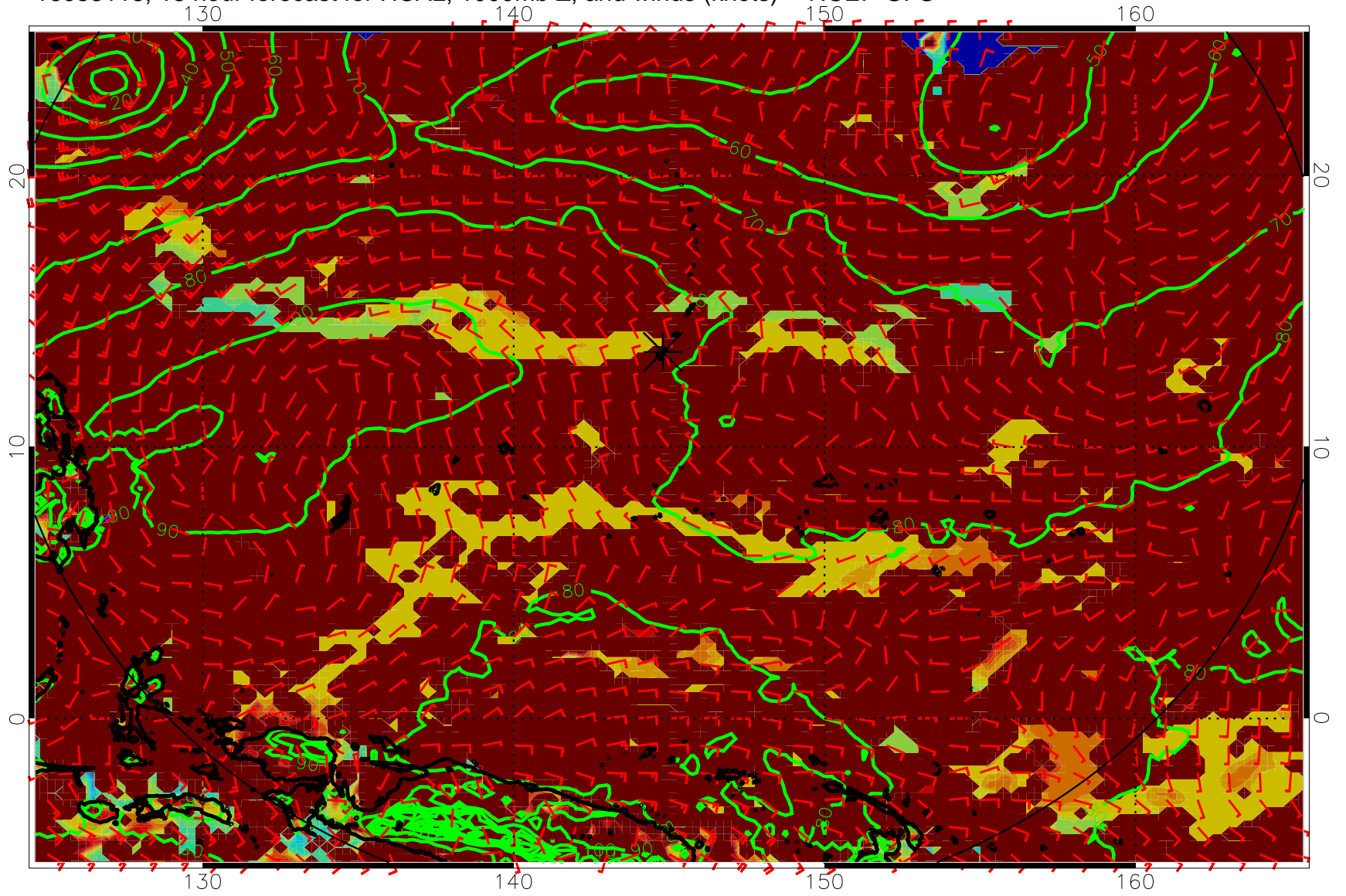
16083118, 18 hour forecast for HCAL, 1000mb Z, and winds (knots) -- NCEP GFS
