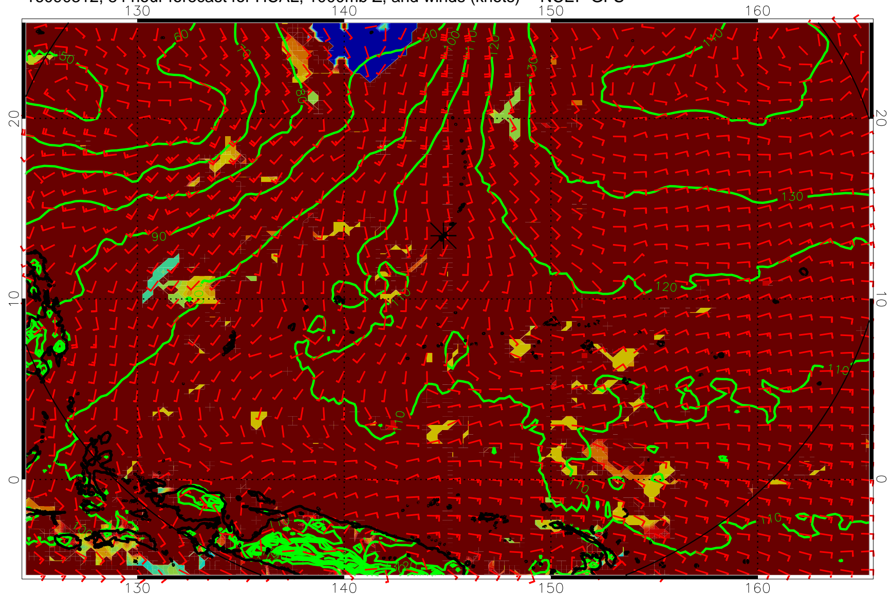
16090312, 84 hour forecast for HCAL, 1000mb Z, and winds (knots) -- NCEP GFS
