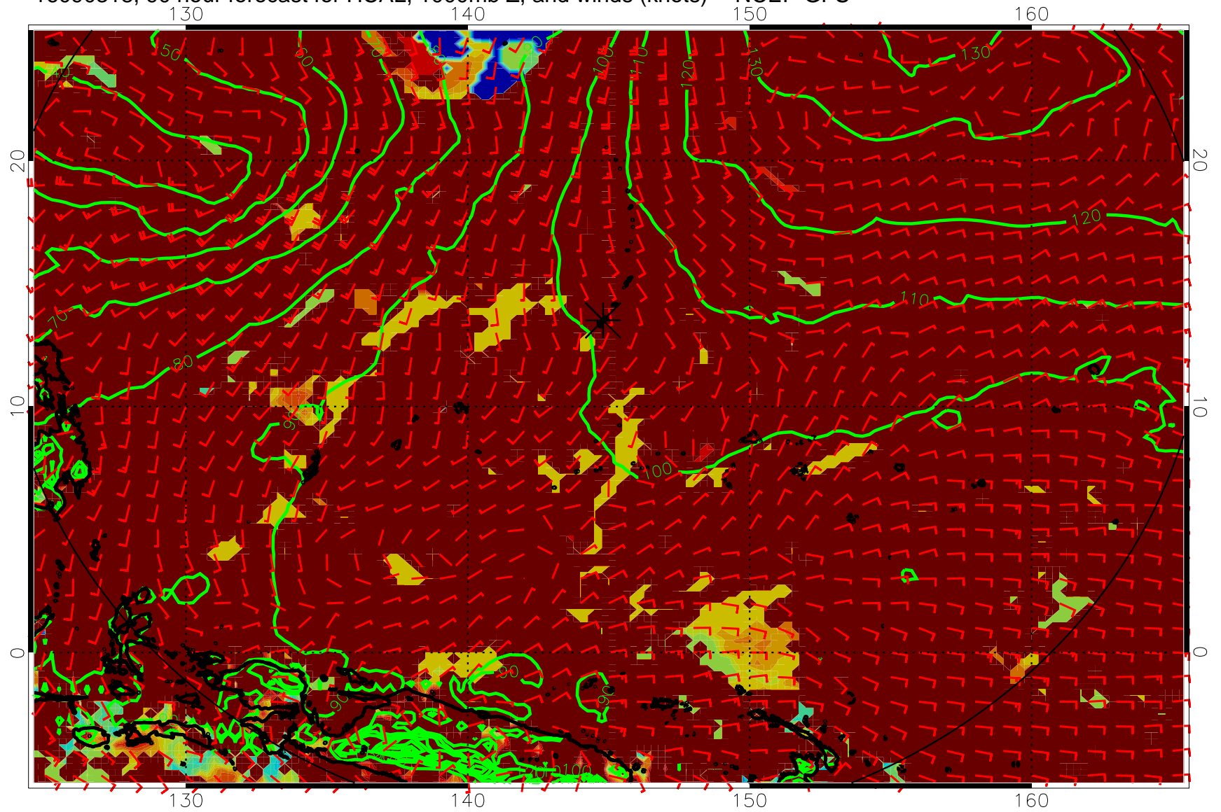
16090318, 90 hour forecast for HCAL, 1000mb Z, and winds (knots) -- NCEP GFS
