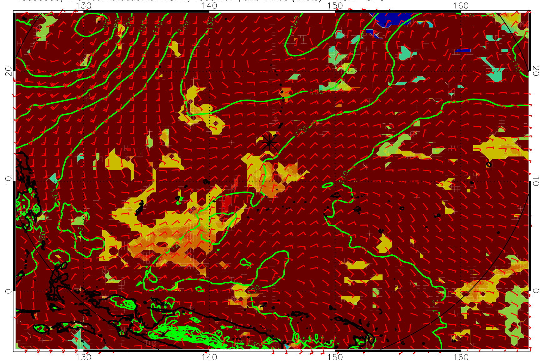
16090500, 120 hour forecast for HCAL, 1000mb Z, and winds (knots) -- NCEP GFS
