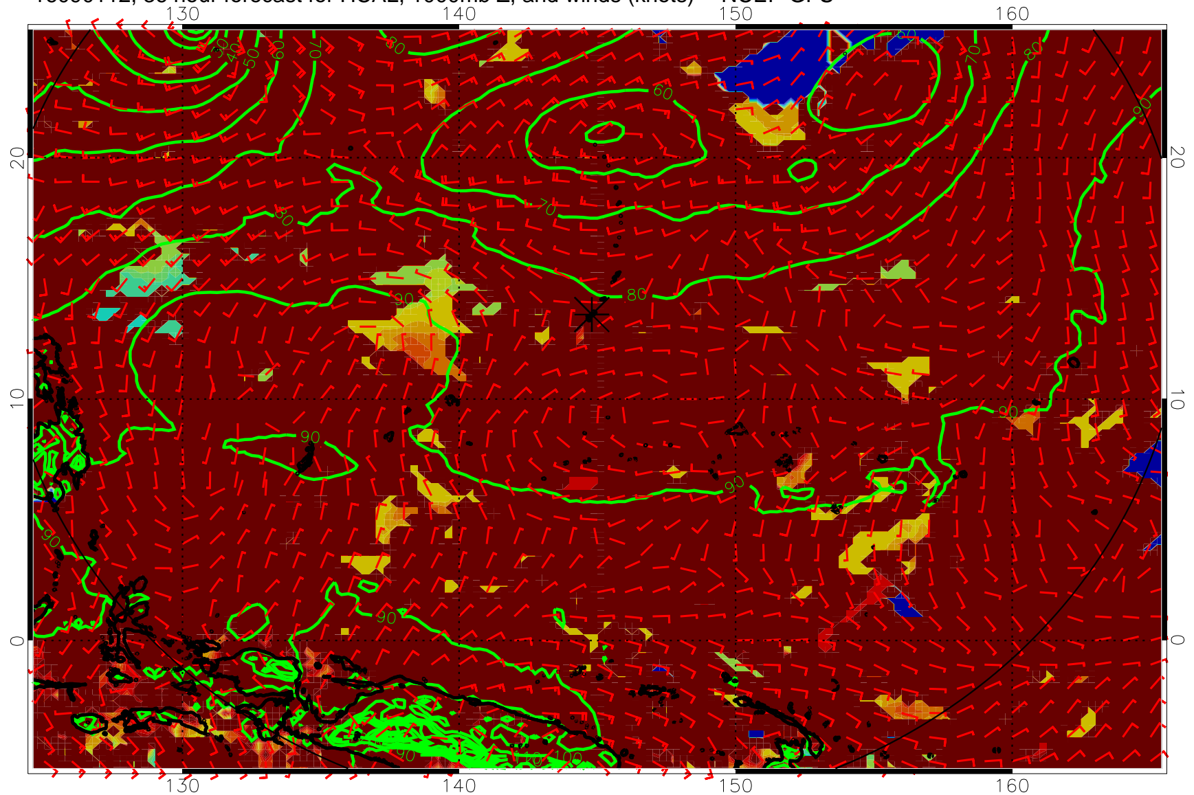
16090112, 36 hour forecast for HCAL, 1000mb Z, and winds (knots) -- NCEP GFS
