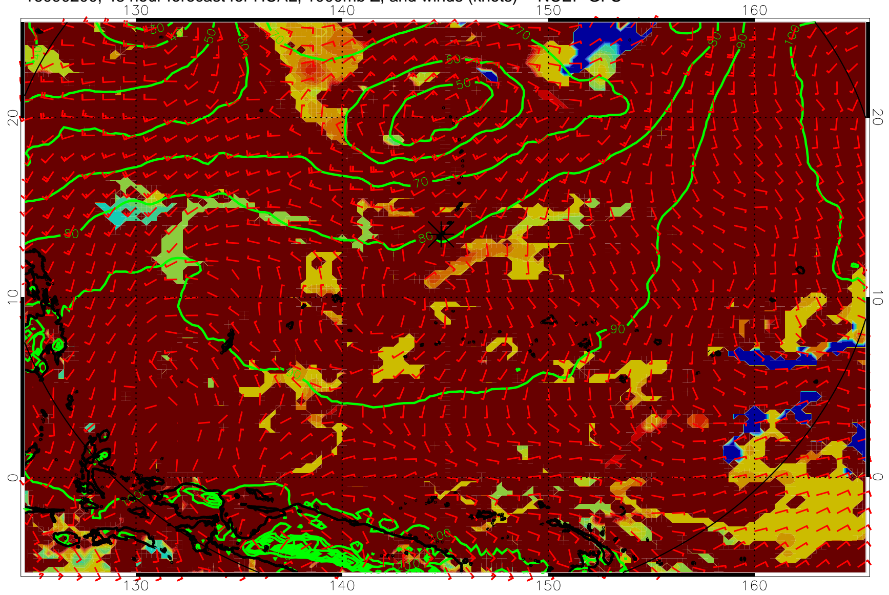
16090200, 48 hour forecast for HCAL, 1000mb Z, and winds (knots) -- NCEP GFS
