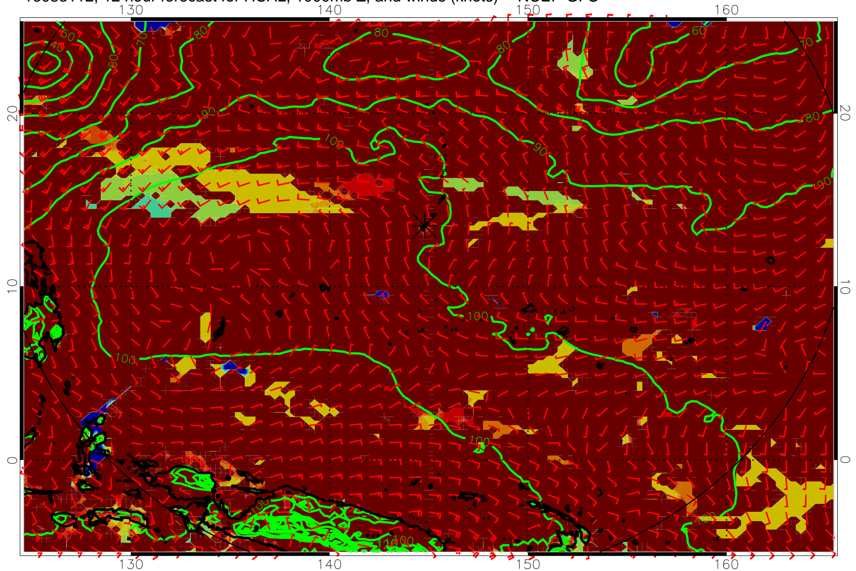
16083112, 12 hour forecast for HCAL, 1000mb Z, and winds (knots) -- NCEP GFS
