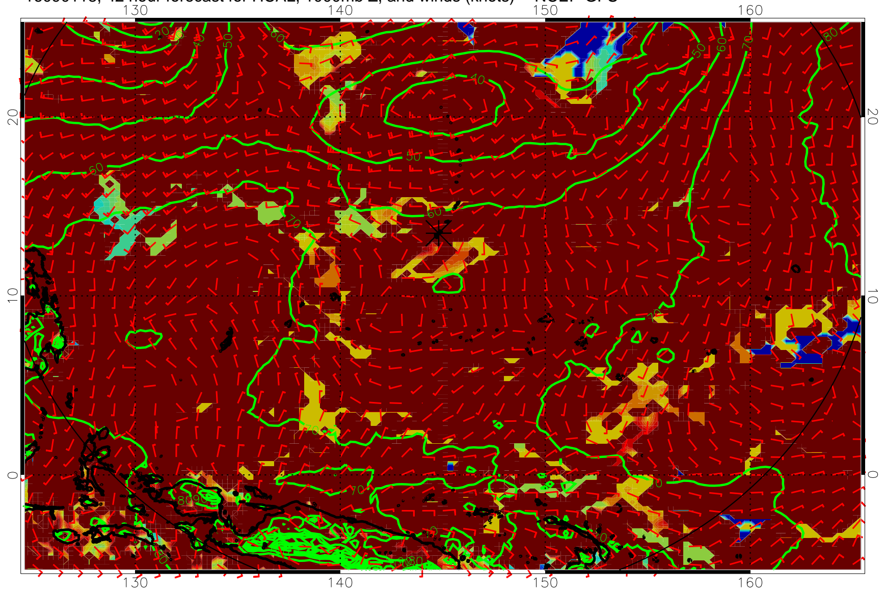
16090118, 42 hour forecast for HCAL, 1000mb Z, and winds (knots) -- NCEP GFS
