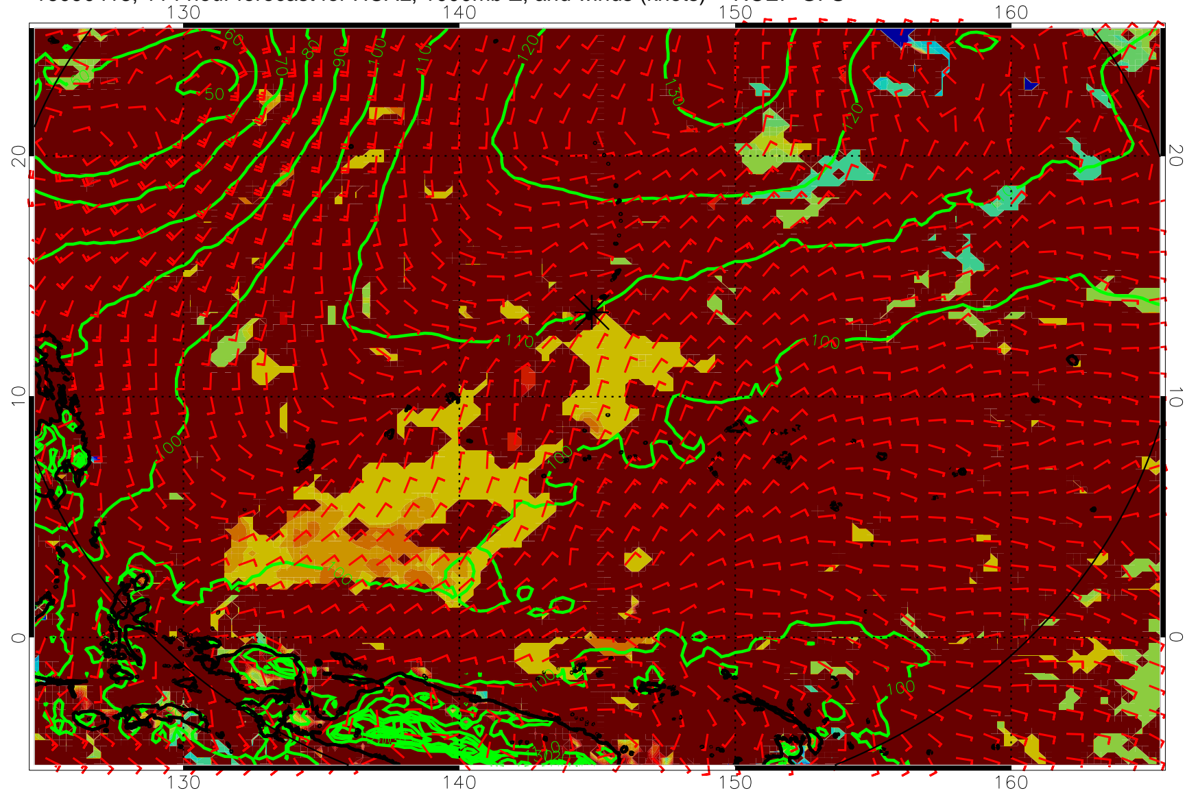
16090418, 114 hour forecast for HCAL, 1000mb Z, and winds (knots) -- NCEP GFS
