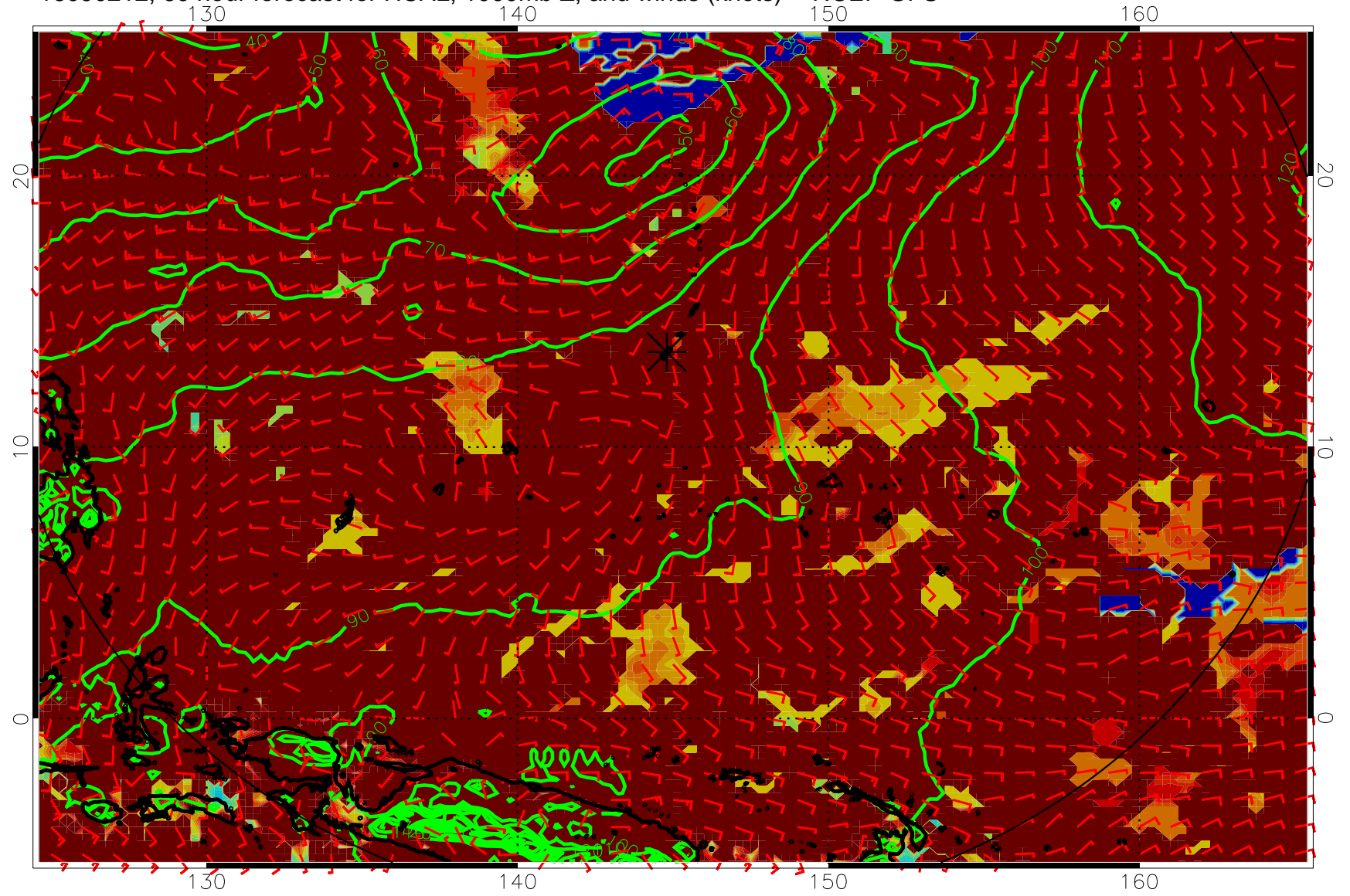
16090212, 60 hour forecast for HCAL, 1000mb Z, and winds (knots) -- NCEP GFS
