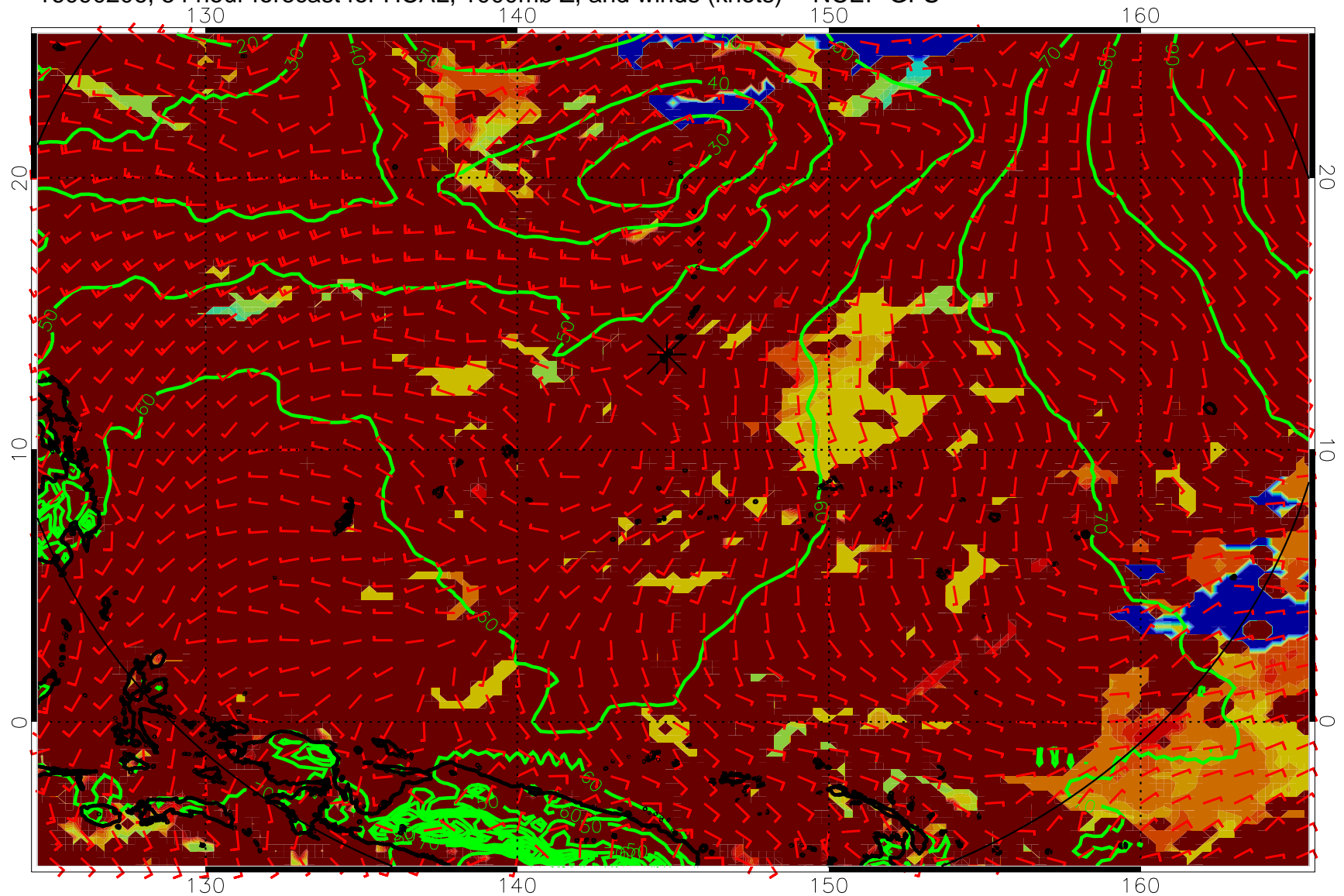
16090206, 54 hour forecast for HCAL, 1000mb Z, and winds (knots) -- NCEP GFS
