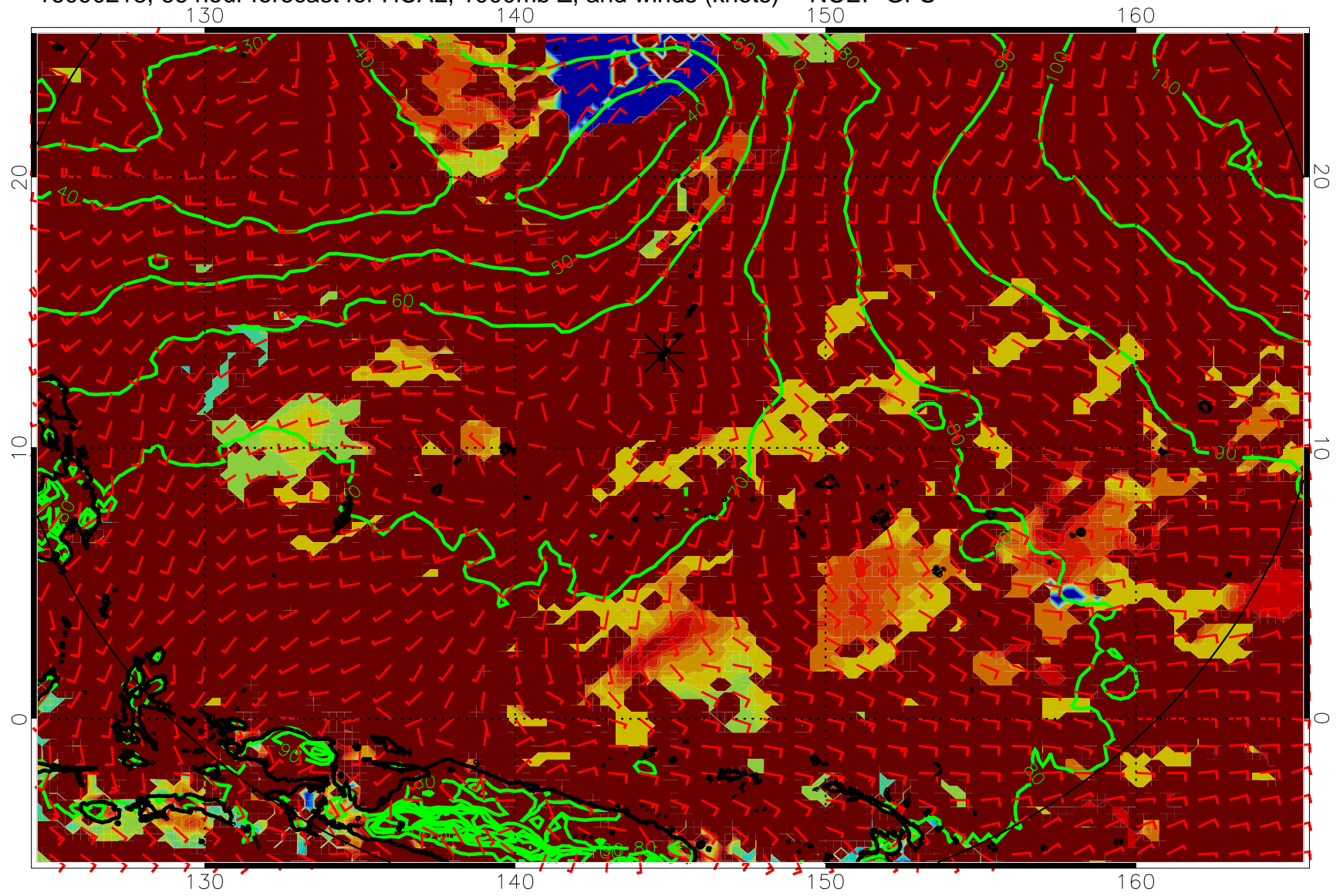
16090218, 66 hour forecast for HCAL, 1000mb Z, and winds (knots) -- NCEP GFS
