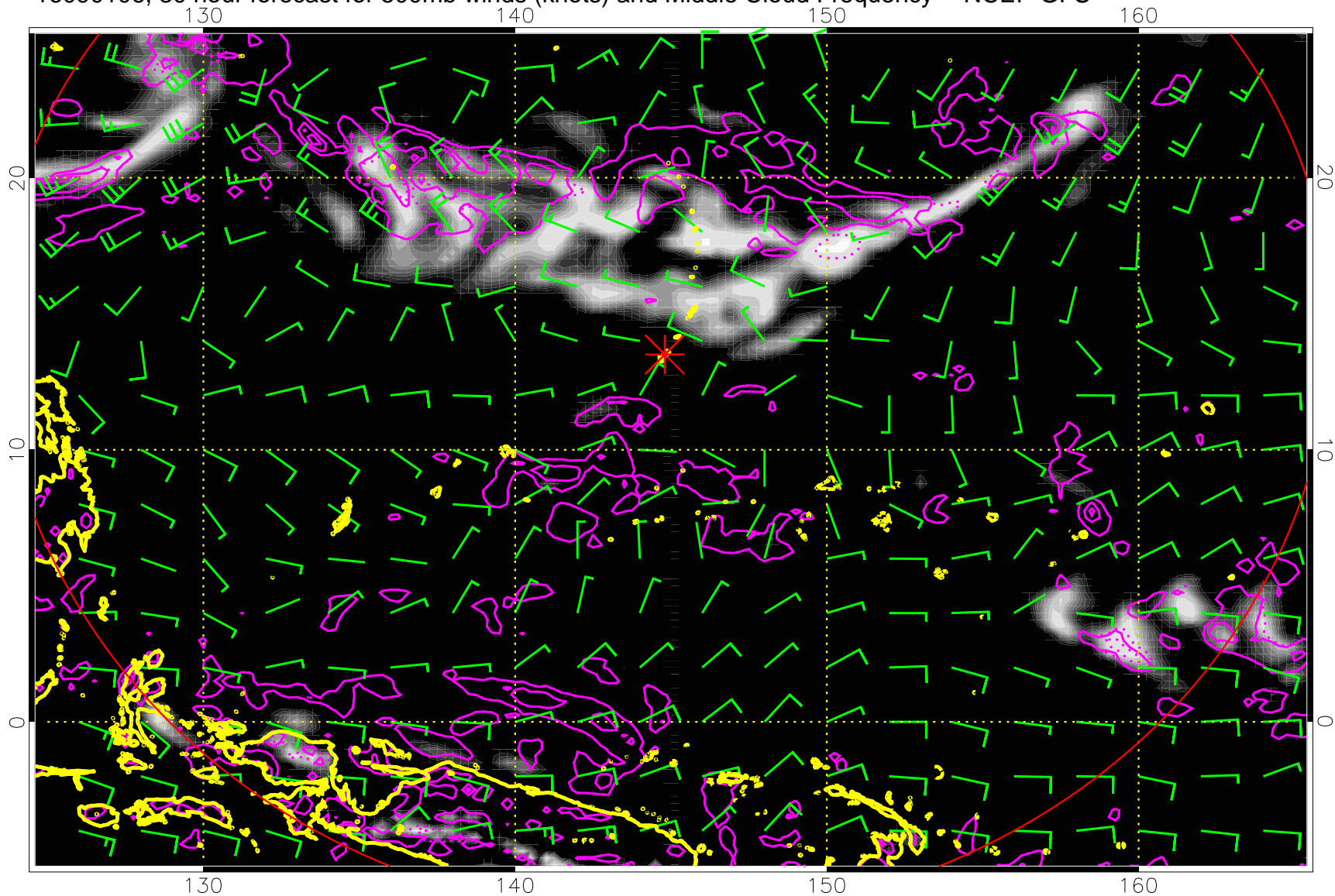
16090106, 30 hour forecast for 500mb winds (knots) and Middle Cloud Frequency -- NCEP GFS
