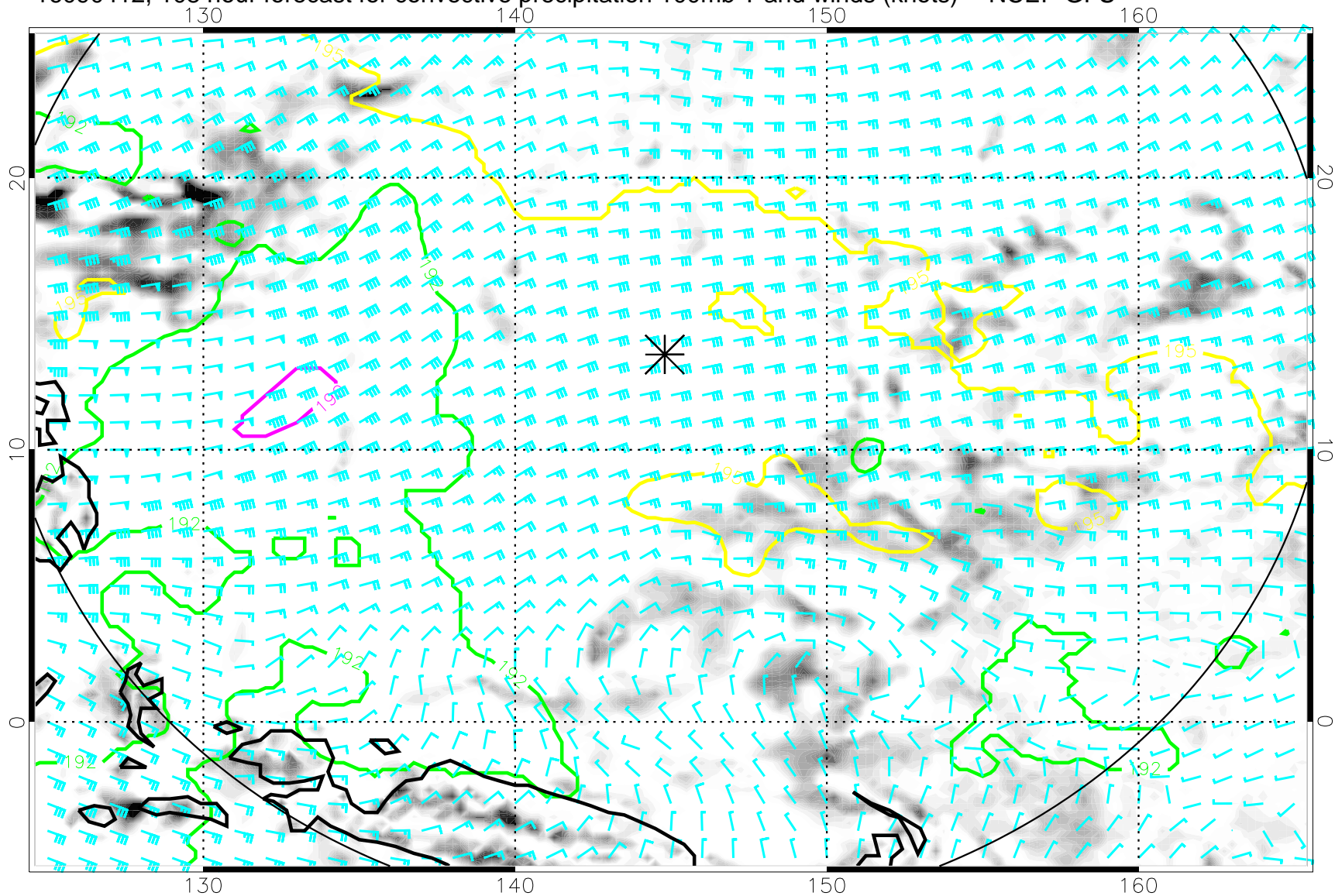
16090412, 108 hour forecast for convective precipitation 100mb T and winds (knots) -- NCEP GFS
