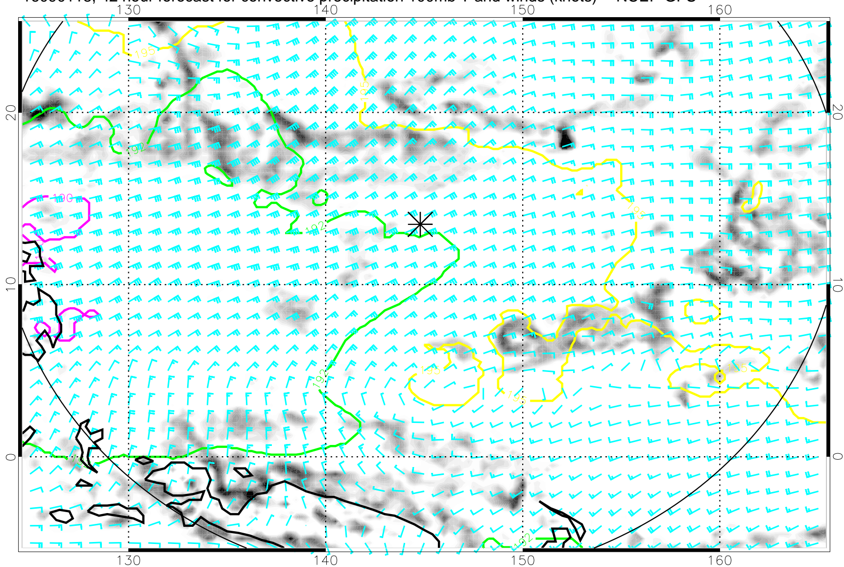
16090118, 42 hour forecast for convective precipitation 100mb T and winds (knots) -- NCEP GFS
