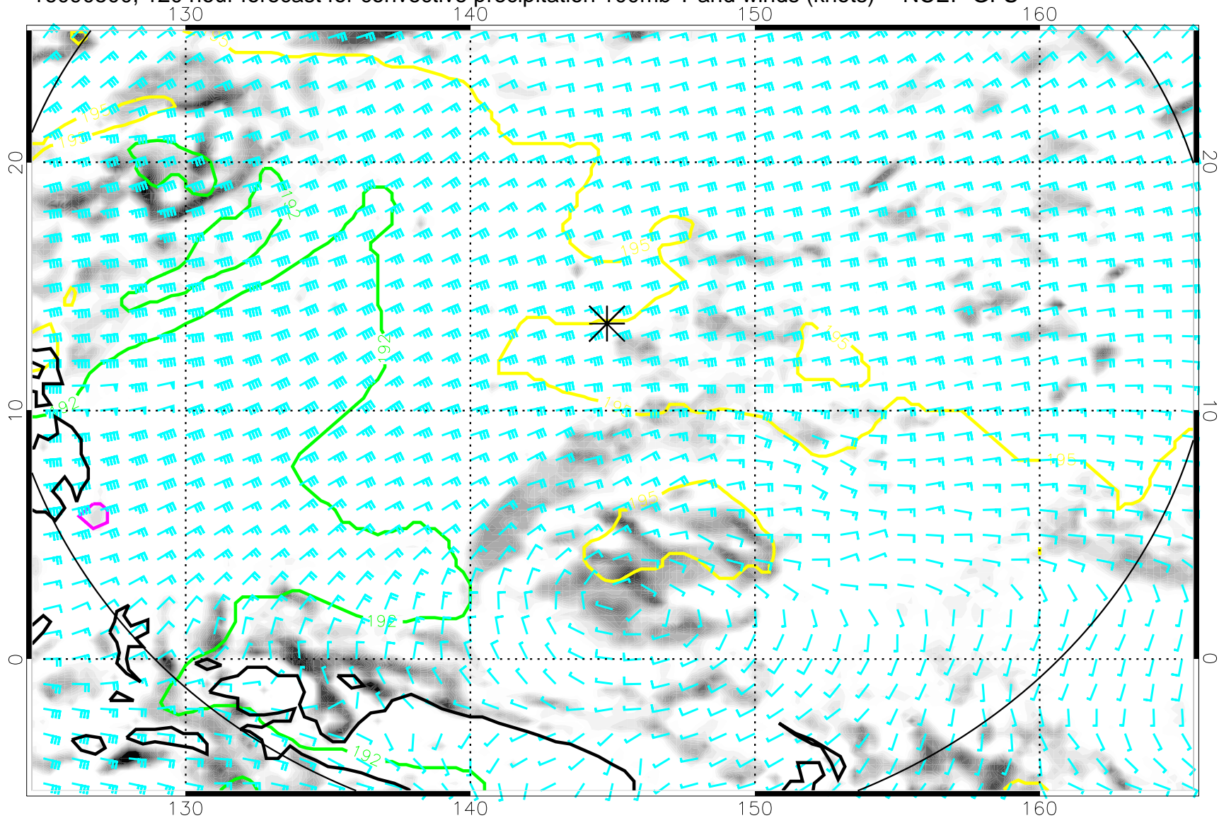
16090500, 120 hour forecast for convective precipitation 100mb T and winds (knots) -- NCEP GFS
