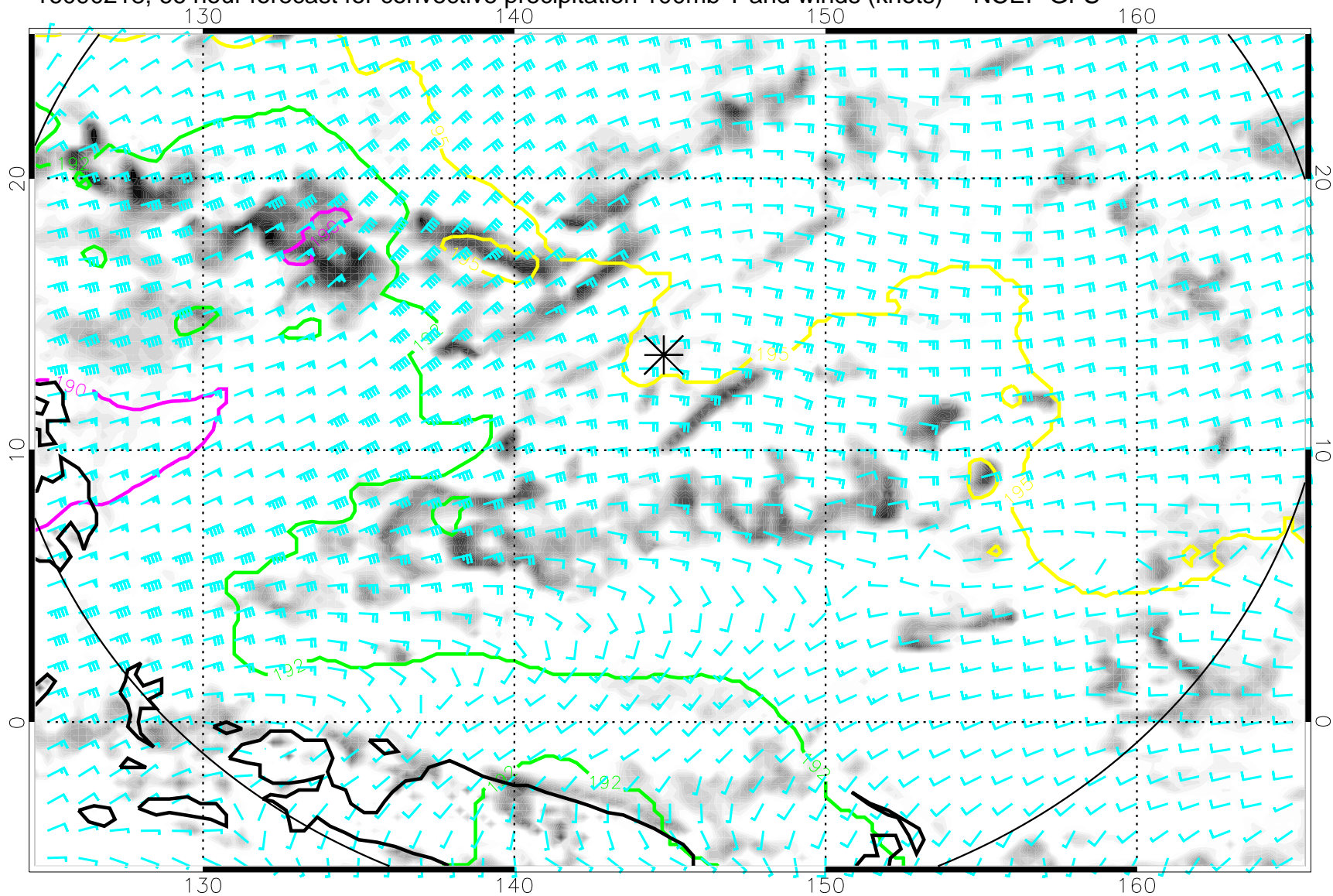
16090218, 66 hour forecast for convective precipitation 100mb T and winds (knots) -- NCEP GFS
