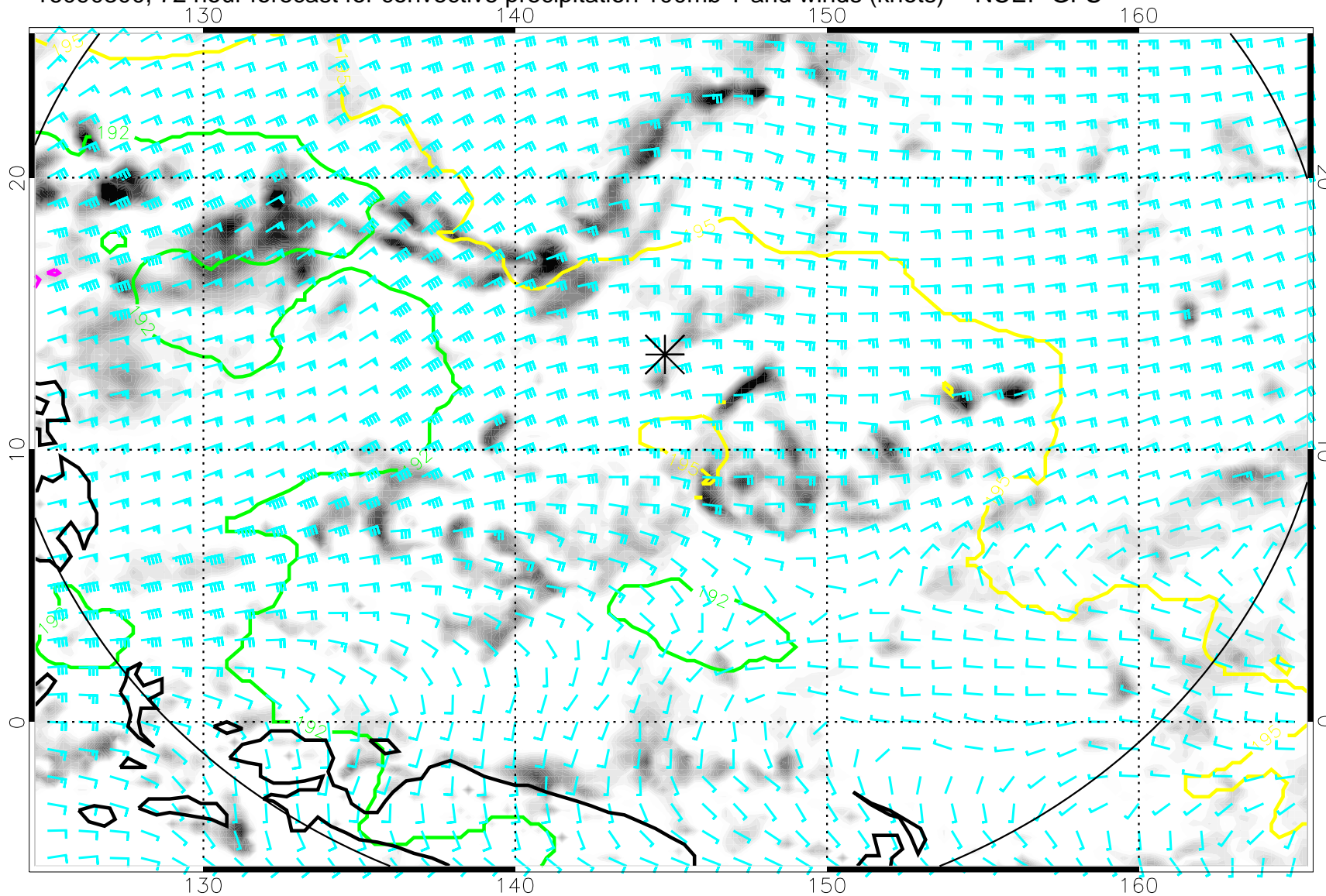
16090300, 72 hour forecast for convective precipitation 100mb T and winds (knots) -- NCEP GFS
