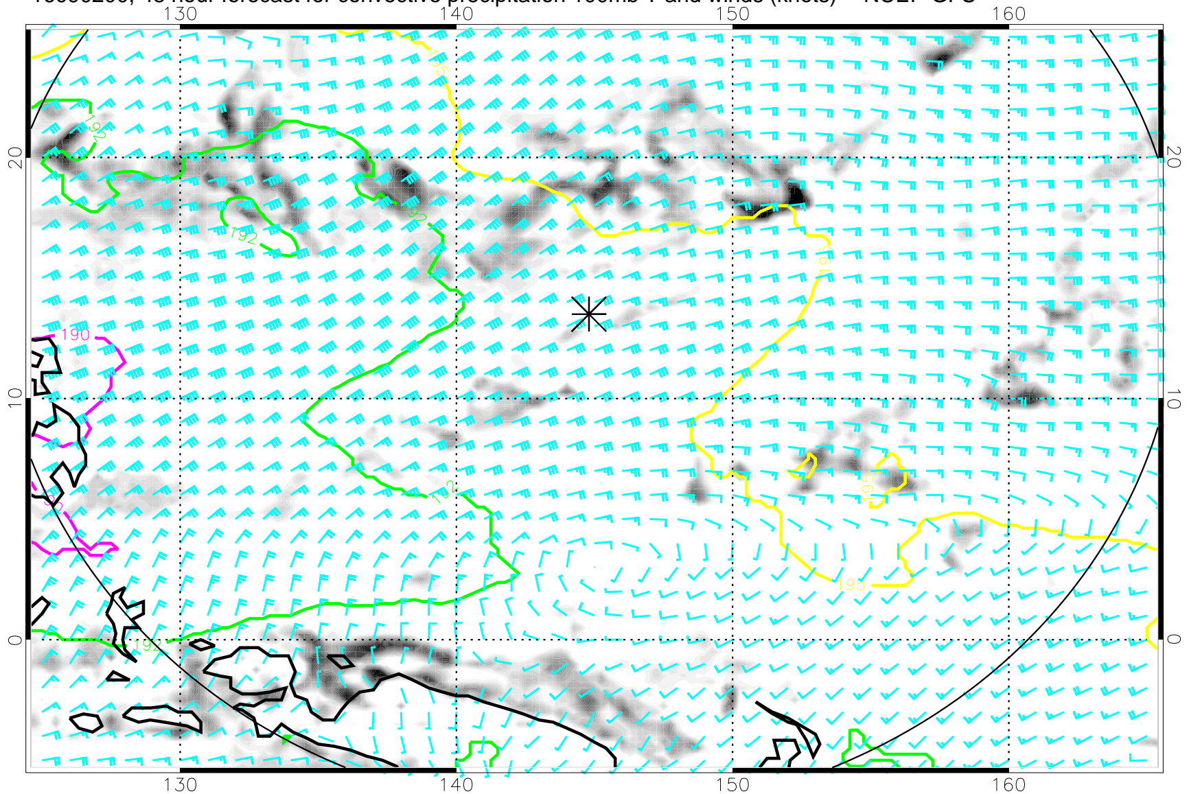
16090200, 48 hour forecast for convective precipitation 100mb T and winds (knots) -- NCEP GFS
