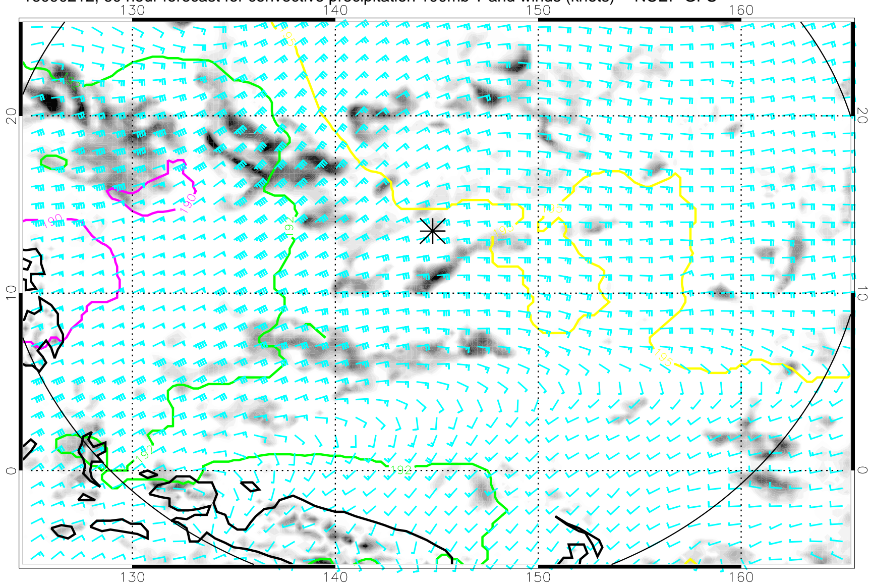
16090212, 60 hour forecast for convective precipitation 100mb T and winds (knots) -- NCEP GFS
