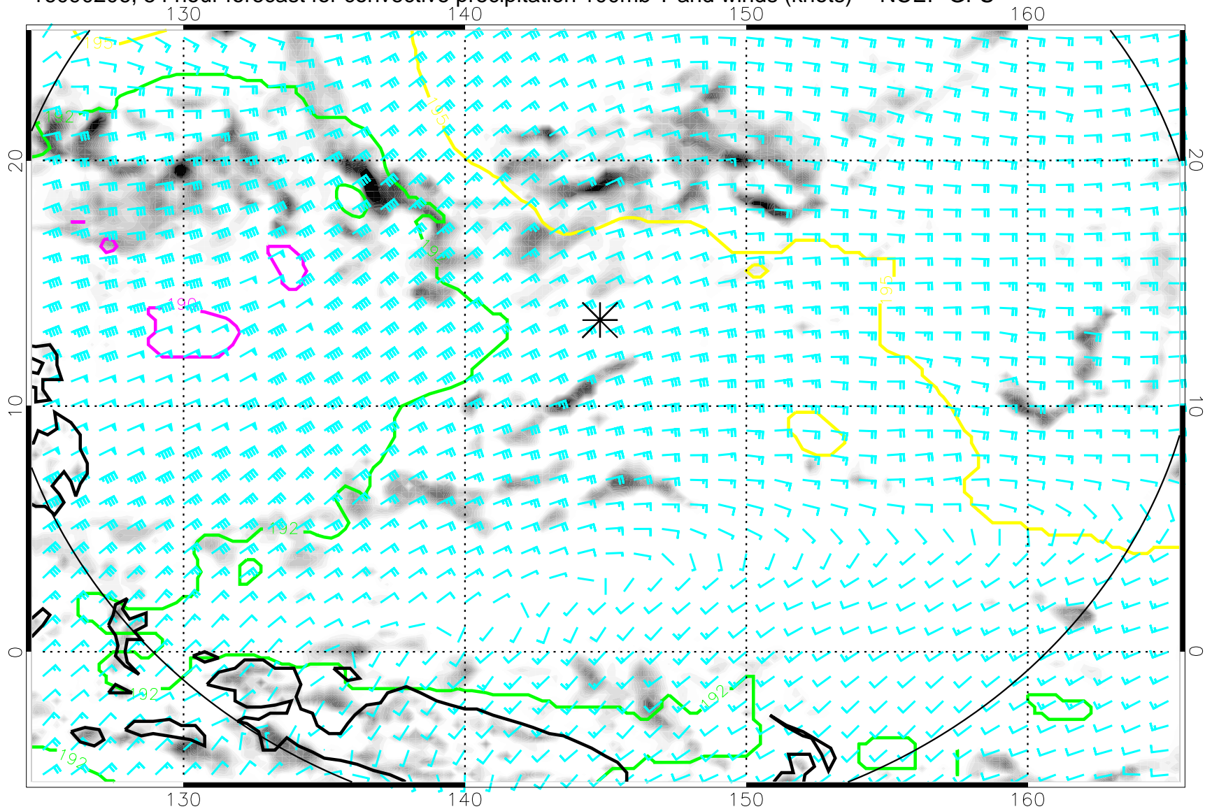
16090206, 54 hour forecast for convective precipitation 100mb T and winds (knots) -- NCEP GFS
