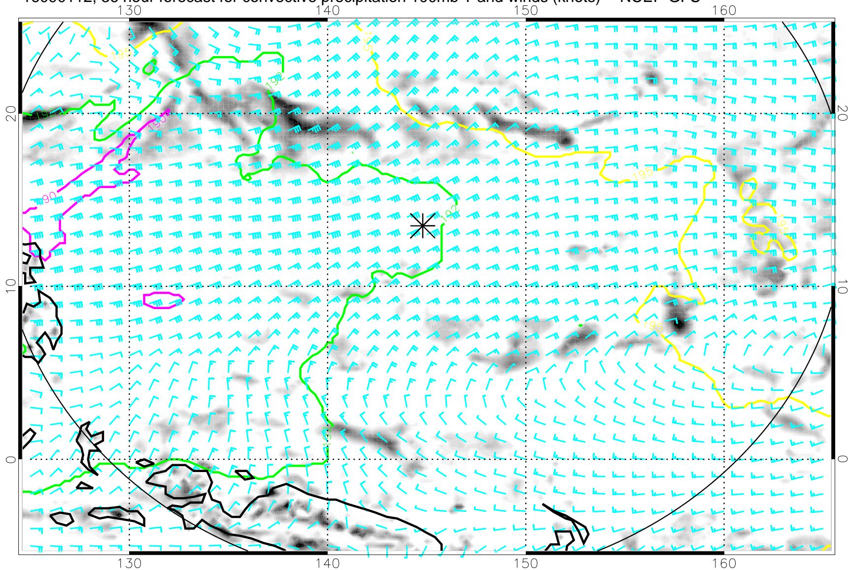
16090112, 36 hour forecast for convective precipitation 100mb T and winds (knots) -- NCEP GFS
