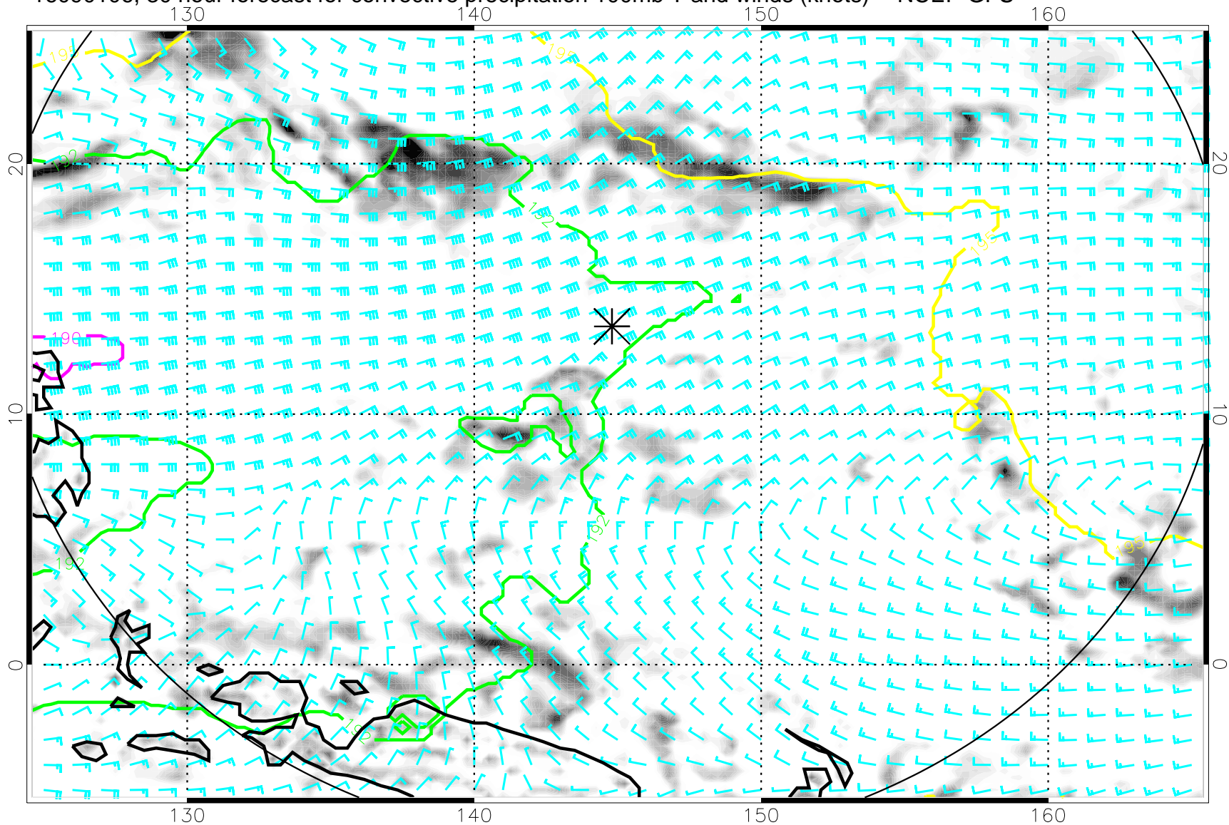
16090106, 30 hour forecast for convective precipitation 100mb T and winds (knots) -- NCEP GFS
