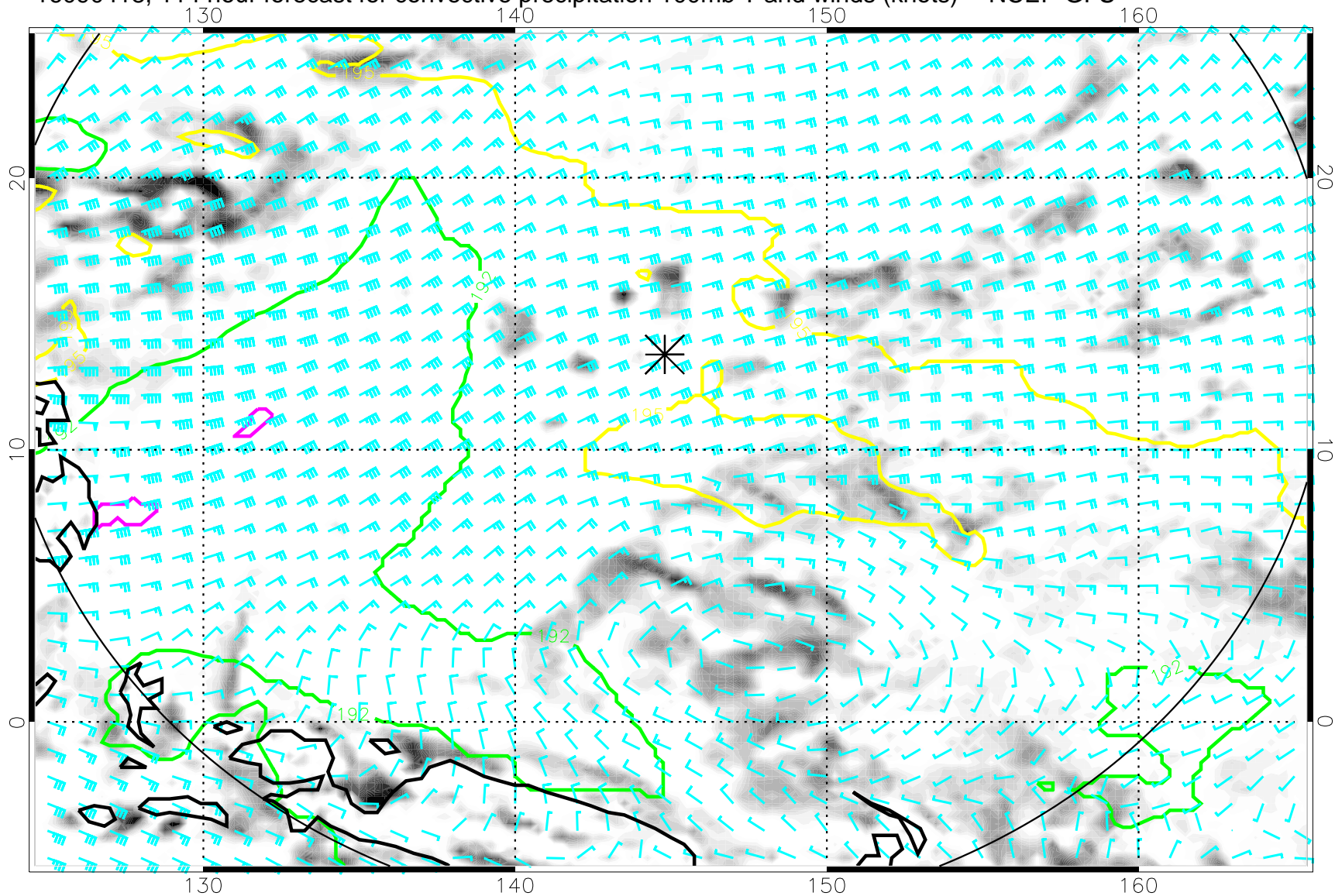
16090418, 114 hour forecast for convective precipitation 100mb T and winds (knots) -- NCEP GFS
