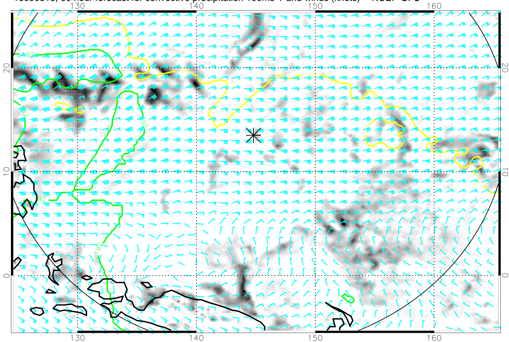
16090318, 90 hour forecast for convective precipitation 100mb T and winds (knots) -- NCEP GFS
