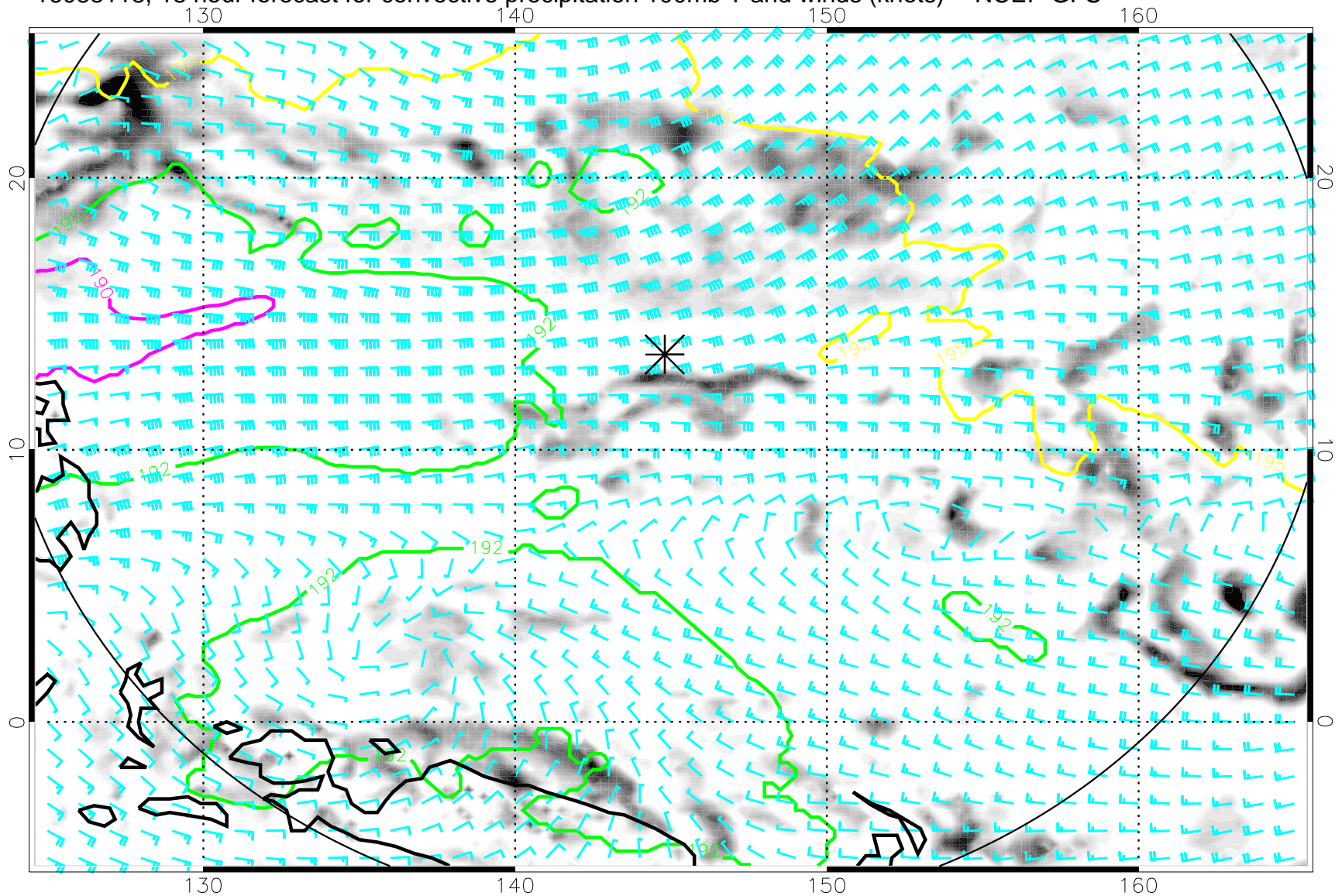
16083118, 18 hour forecast for convective precipitation 100mb T and winds (knots) -- NCEP GFS
