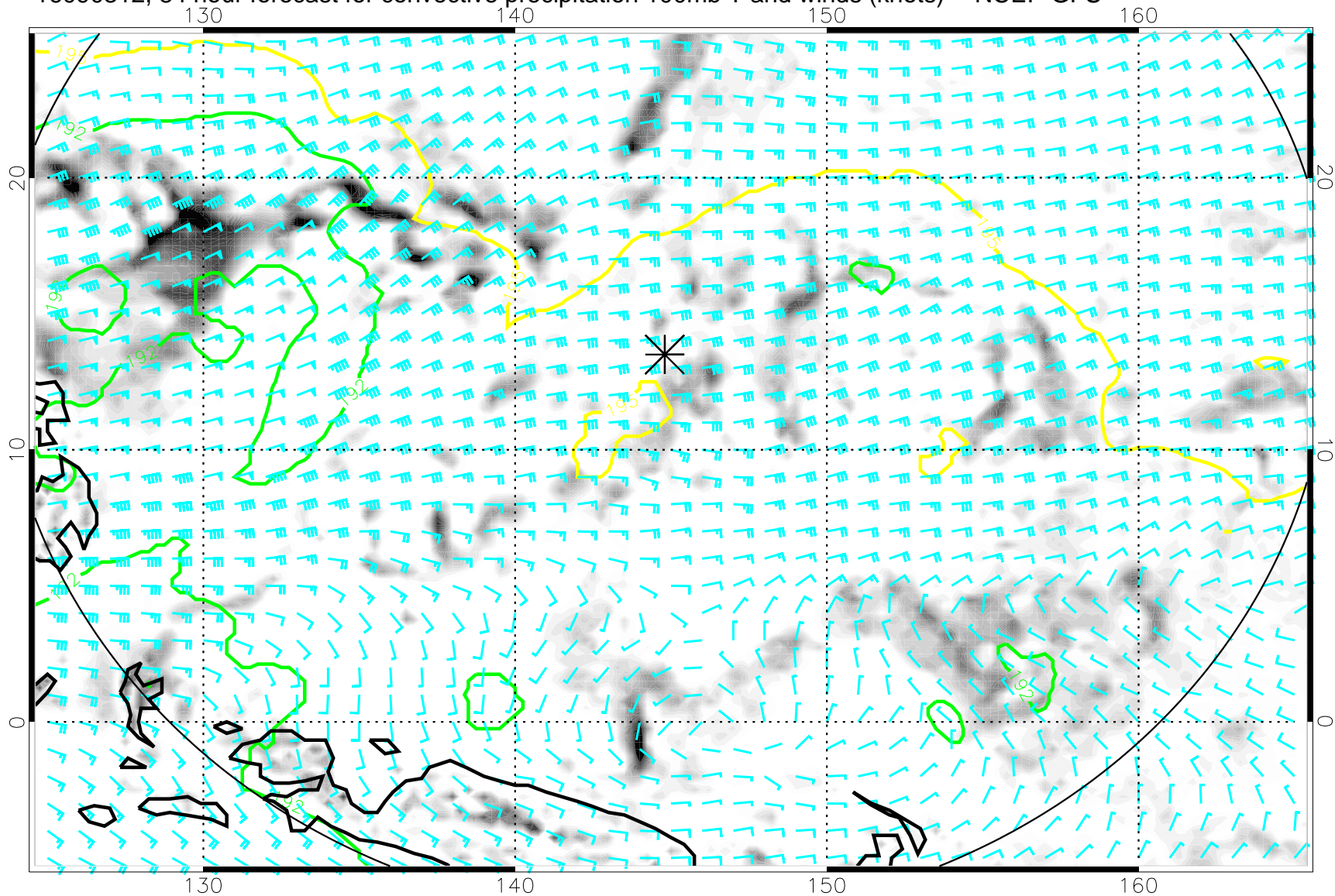
16090312, 84 hour forecast for convective precipitation 100mb T and winds (knots) -- NCEP GFS
