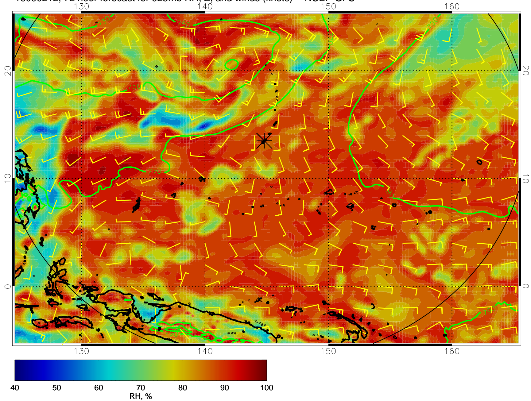
16090212, 72 hour forecast for 925mb RH, Z, and winds (knots) -- NCEP GFS
