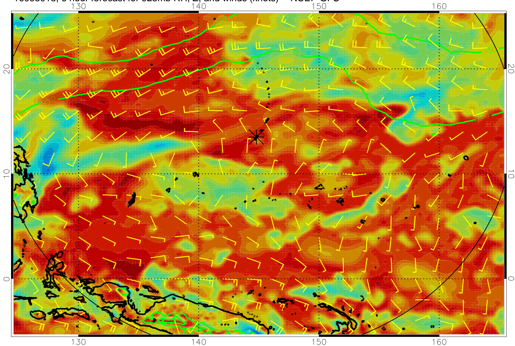
16083018, 6 hour forecast for 925mb RH, Z, and winds (knots) -- NCEP GFS
