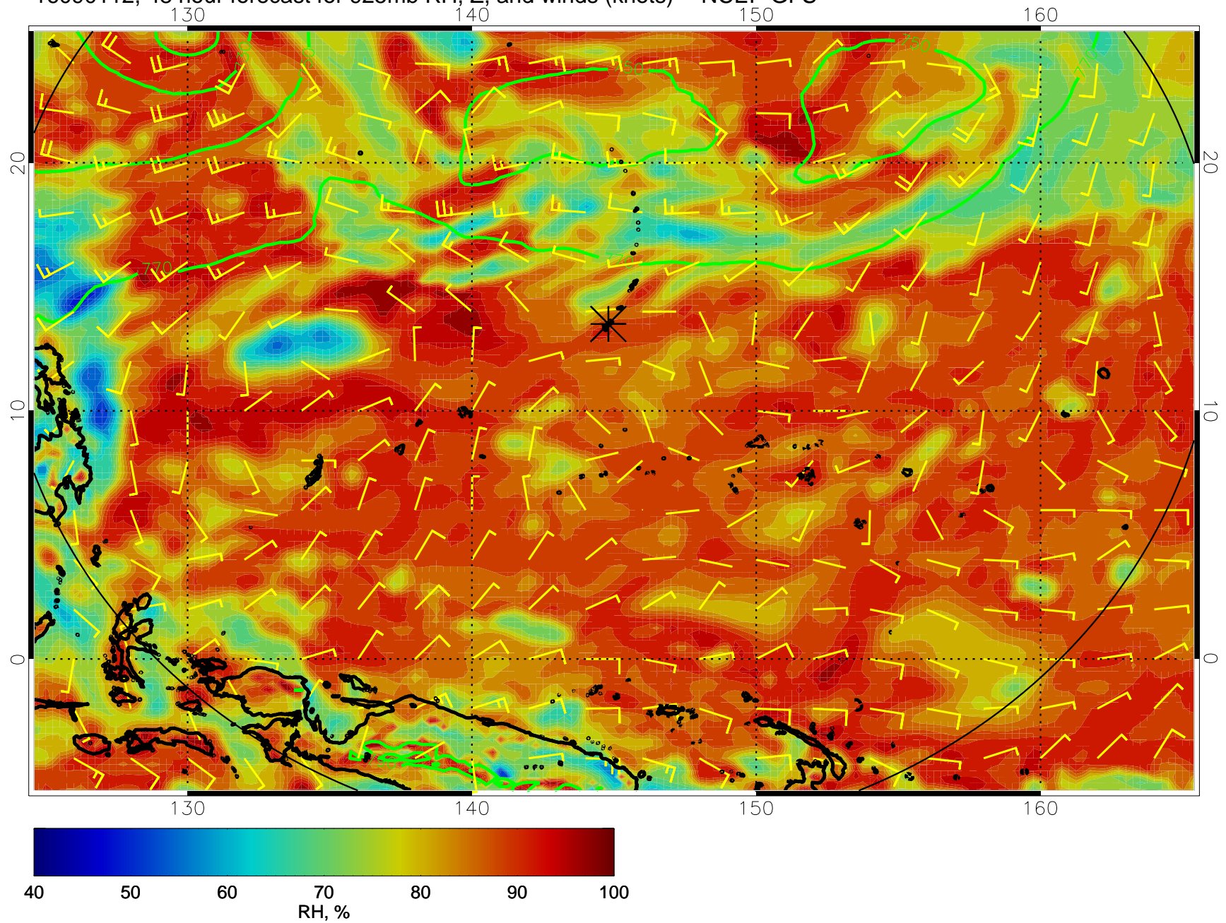
16090112, 48 hour forecast for 925mb RH, Z, and winds (knots) -- NCEP GFS
