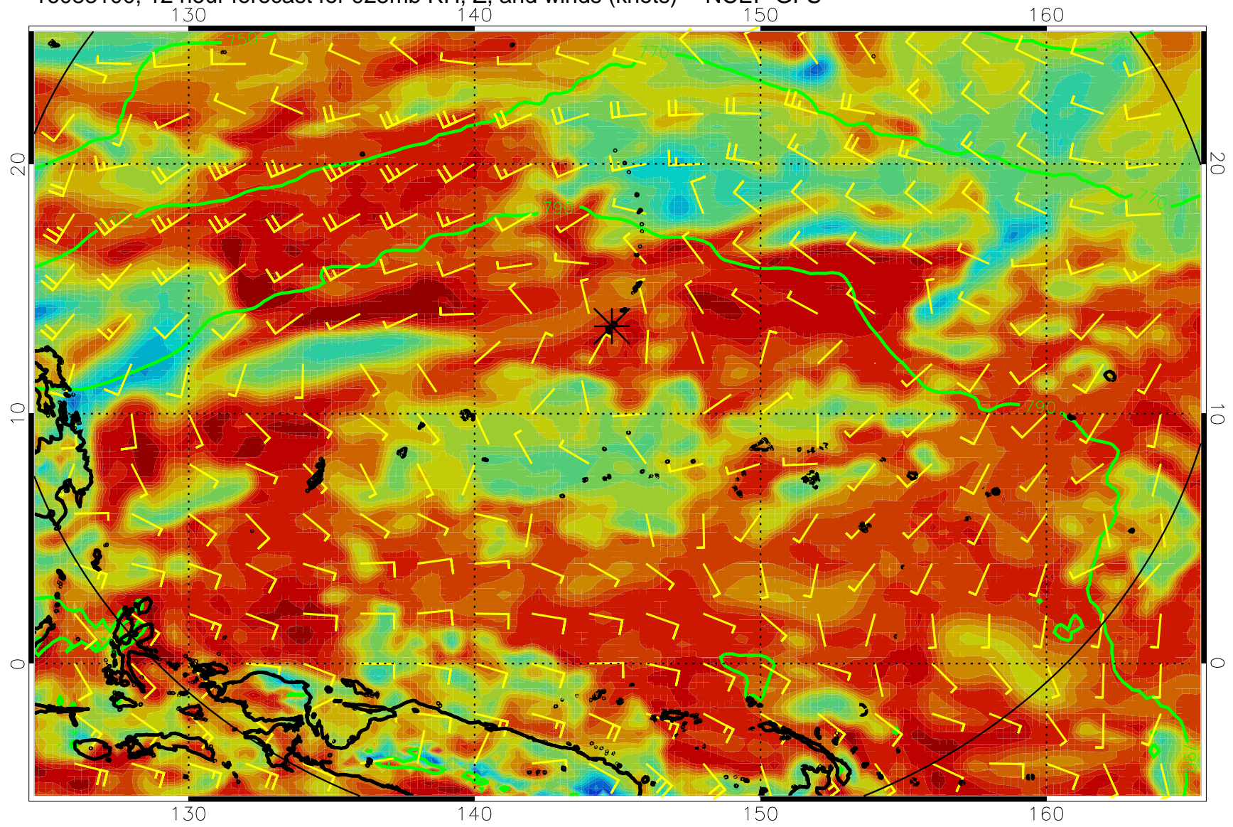
16083100, 12 hour forecast for 925mb RH, Z, and winds (knots) -- NCEP GFS
