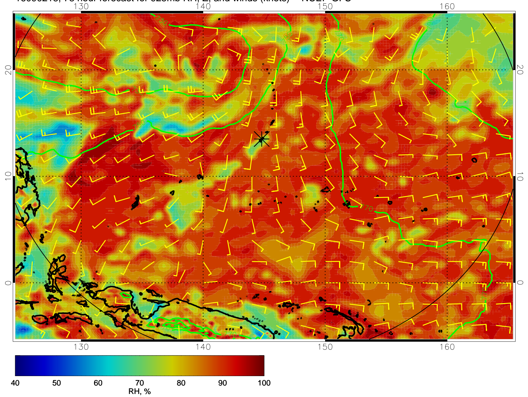
16090218, 78 hour forecast for 925mb RH, Z, and winds (knots) -- NCEP GFS
