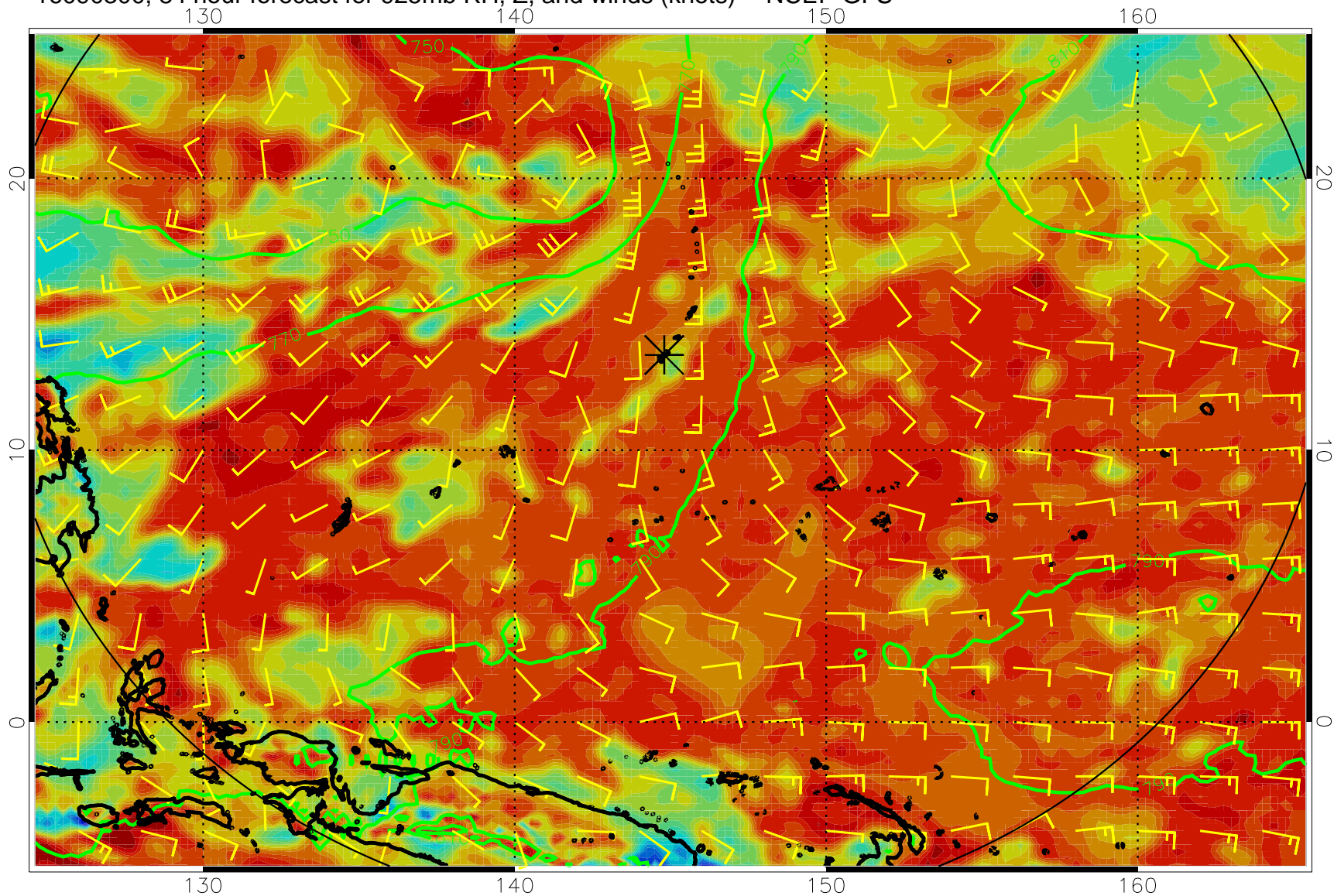
16090300, 84 hour forecast for 925mb RH, Z, and winds (knots) -- NCEP GFS
