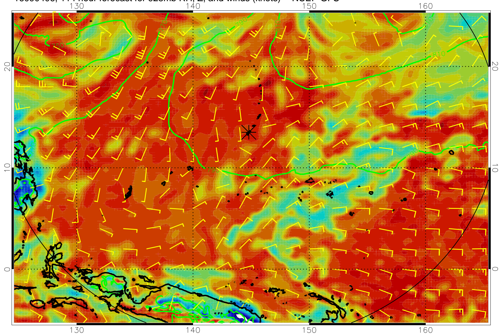
16090406, 114 hour forecast for 925mb RH, Z, and winds (knots) -- NCEP GFS
