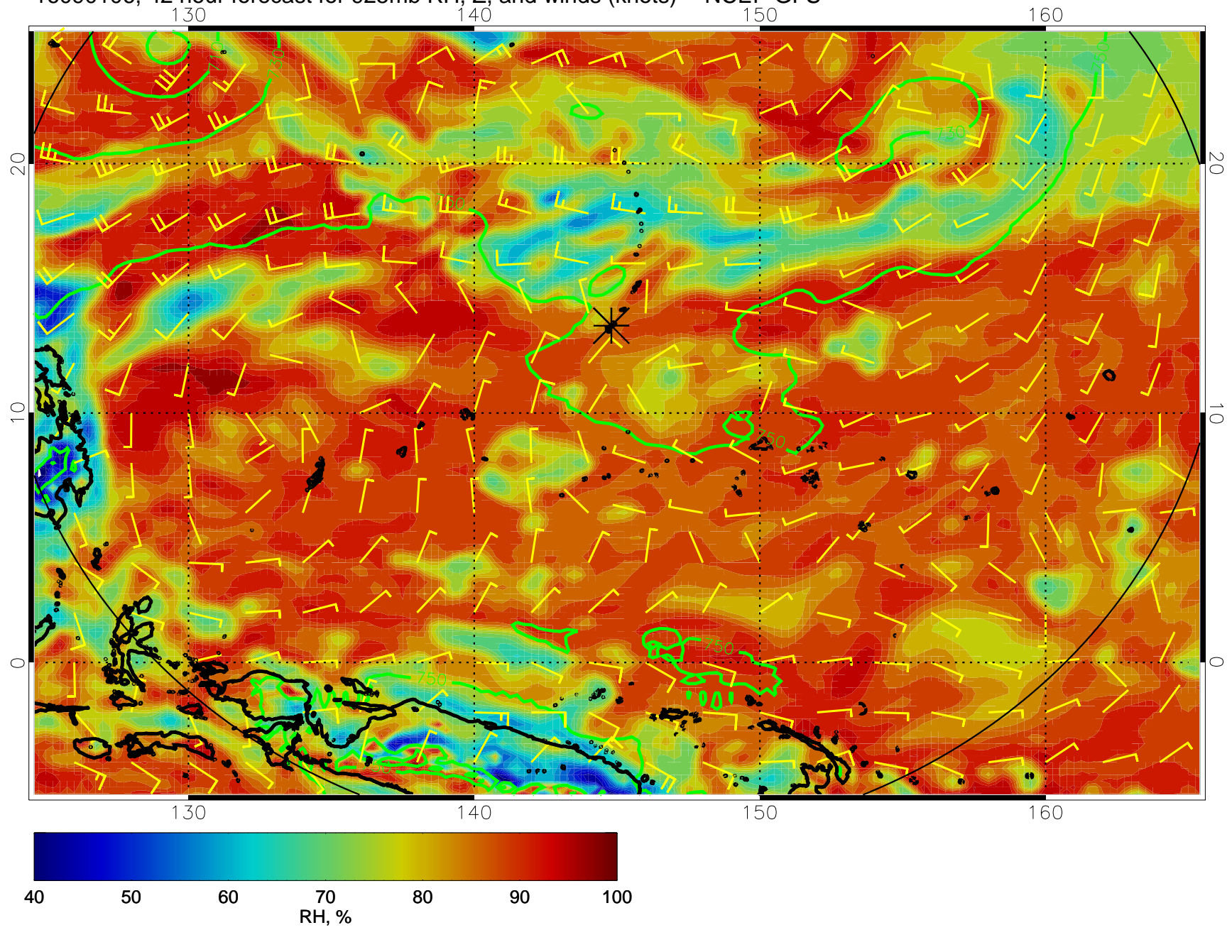
16090106, 42 hour forecast for 925mb RH, Z, and winds (knots) -- NCEP GFS
