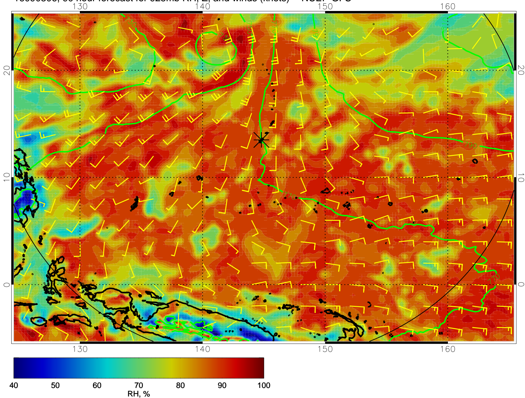
16090306, 90 hour forecast for 925mb RH, Z, and winds (knots) -- NCEP GFS
