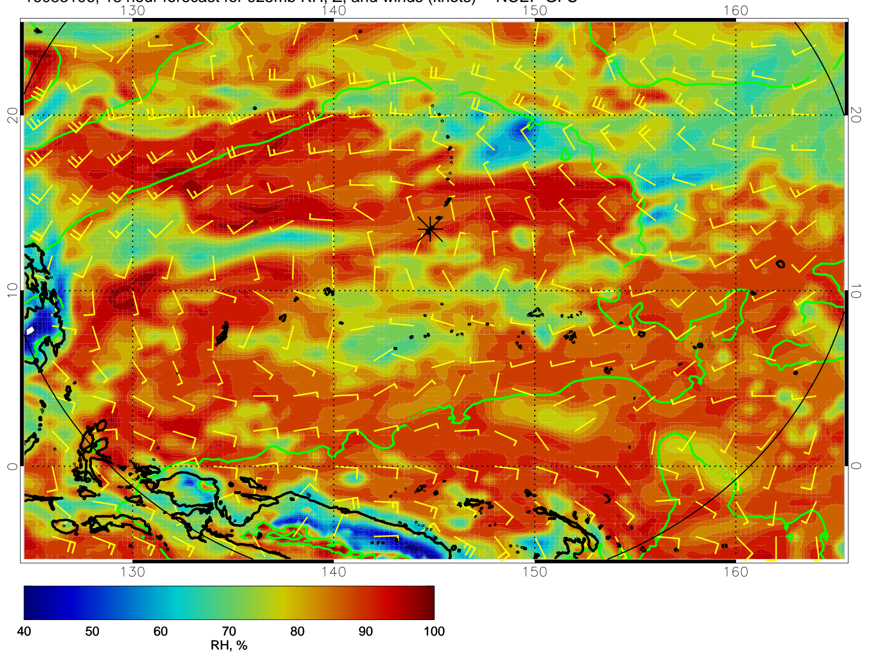
16083106, 18 hour forecast for 925mb RH, Z, and winds (knots) -- NCEP GFS
