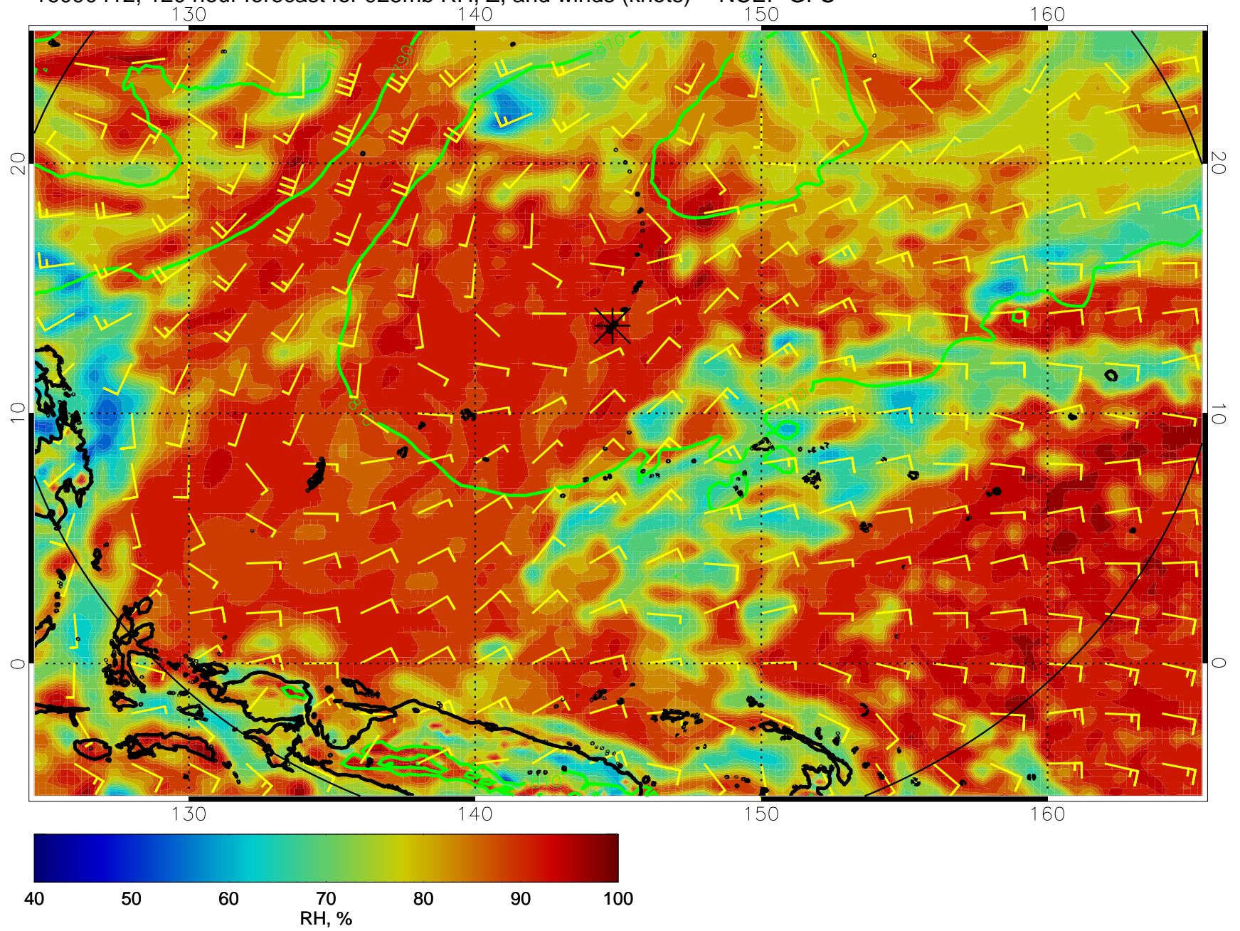
16090412, 120 hour forecast for 925mb RH, Z, and winds (knots) -- NCEP GFS
