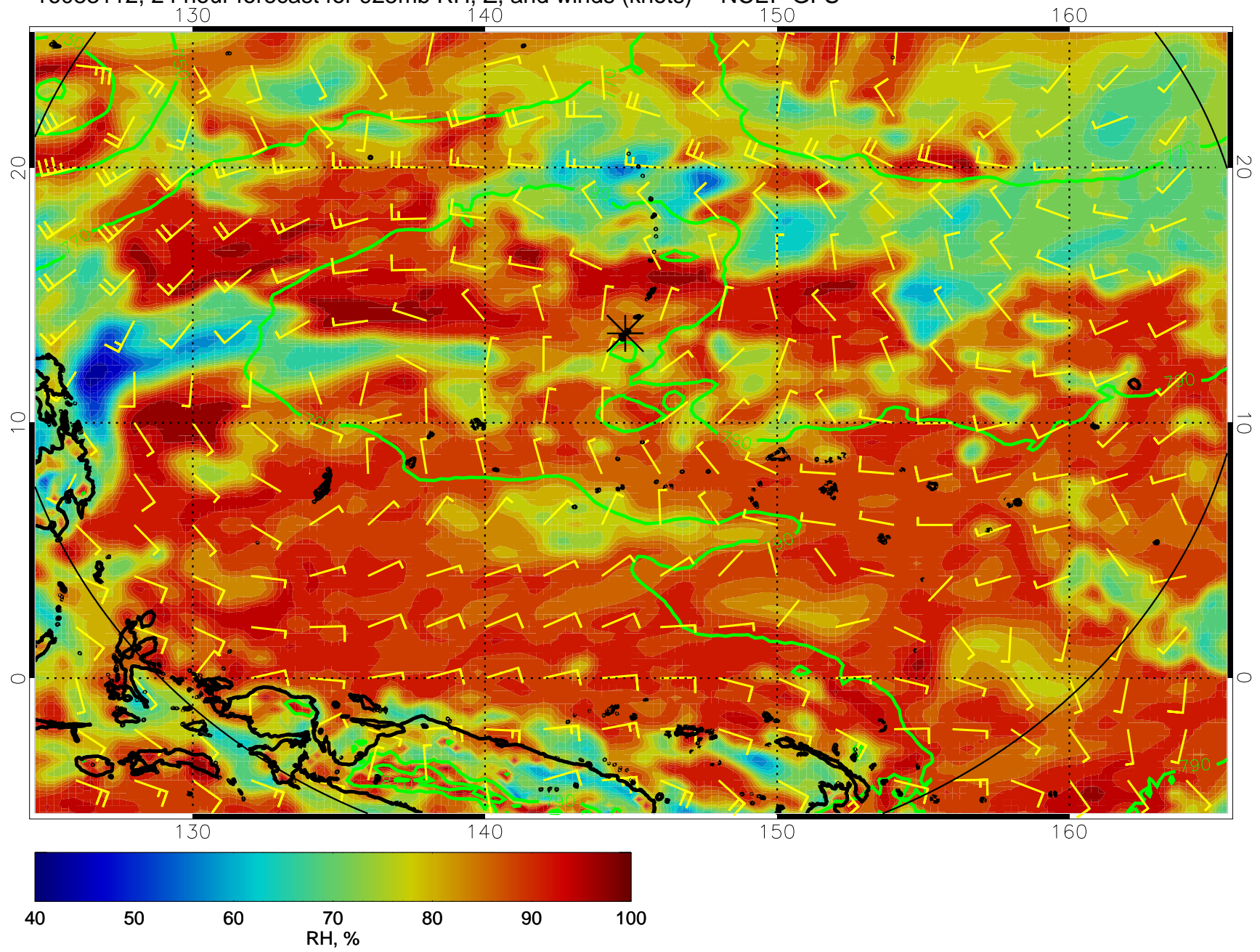
16083112, 24 hour forecast for 925mb RH, Z, and winds (knots) -- NCEP GFS
