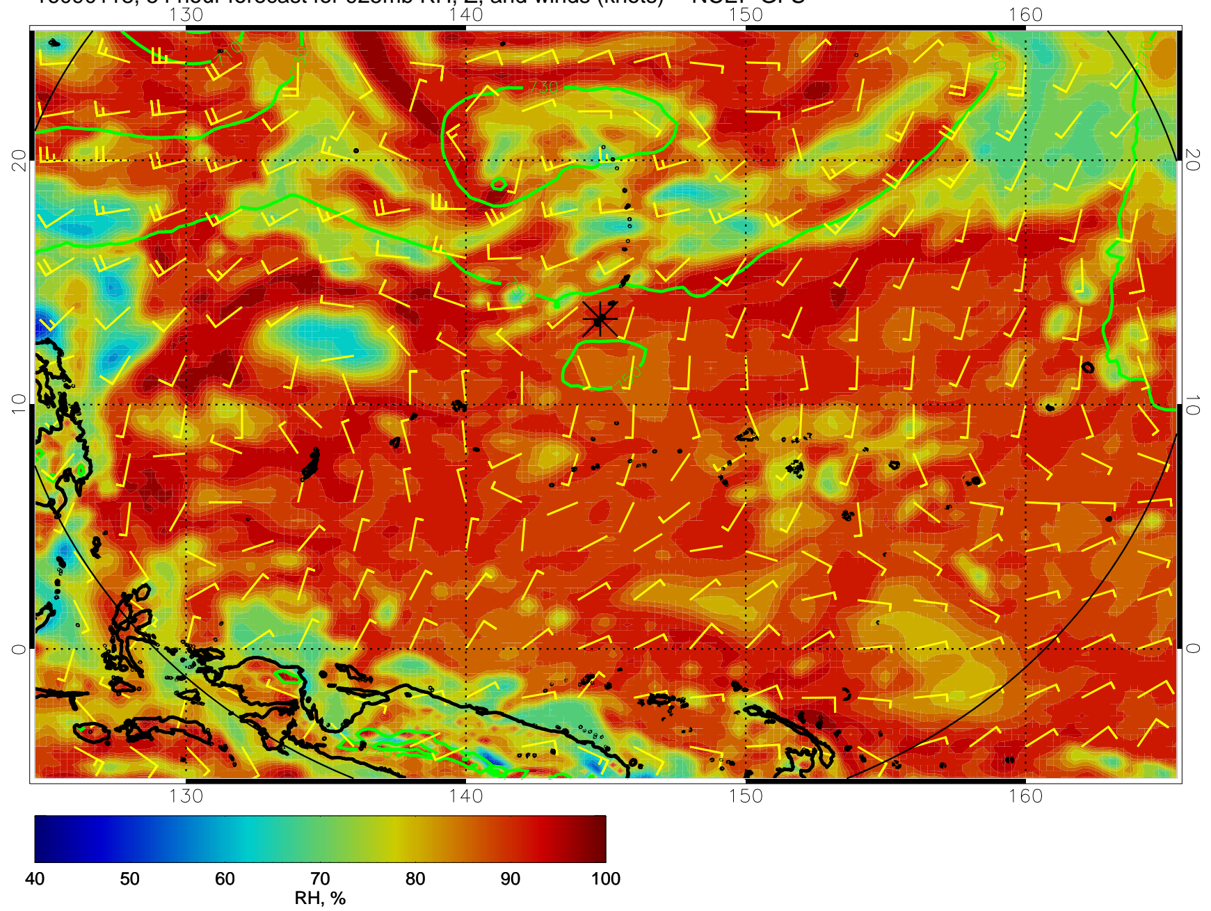
16090118, 54 hour forecast for 925mb RH, Z, and winds (knots) -- NCEP GFS
