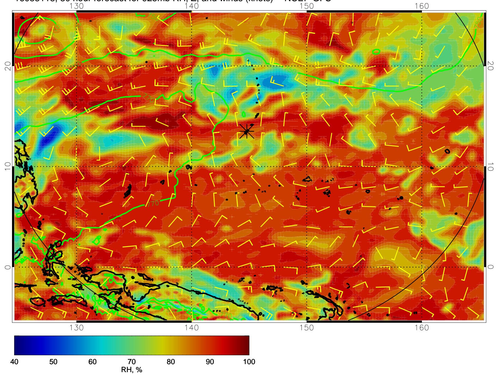
16083118, 30 hour forecast for 925mb RH, Z, and winds (knots) -- NCEP GFS
