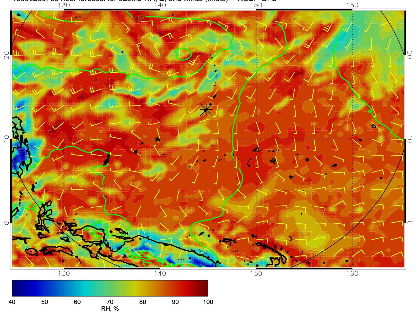
16090206, 66 hour forecast for 925mb RH, Z, and winds (knots) -- NCEP GFS
