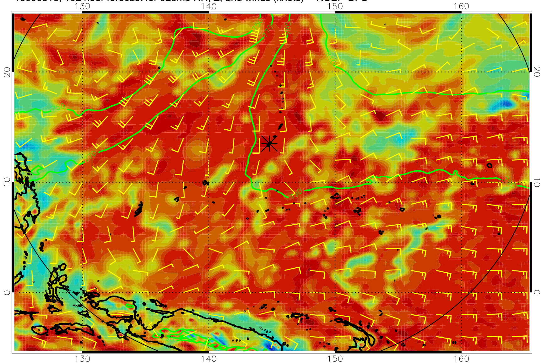
16090318, 102 hour forecast for 925mb RH, Z, and winds (knots) -- NCEP GFS
