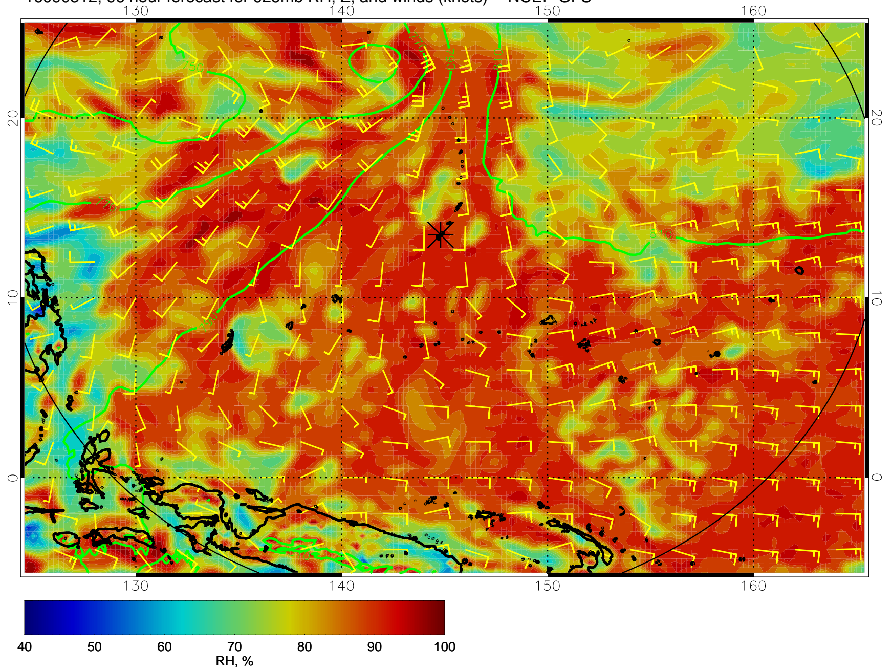
16090312, 96 hour forecast for 925mb RH, Z, and winds (knots) -- NCEP GFS
