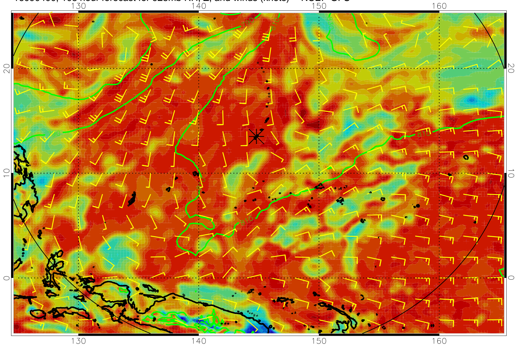
16090400, 108 hour forecast for 925mb RH, Z, and winds (knots) -- NCEP GFS
