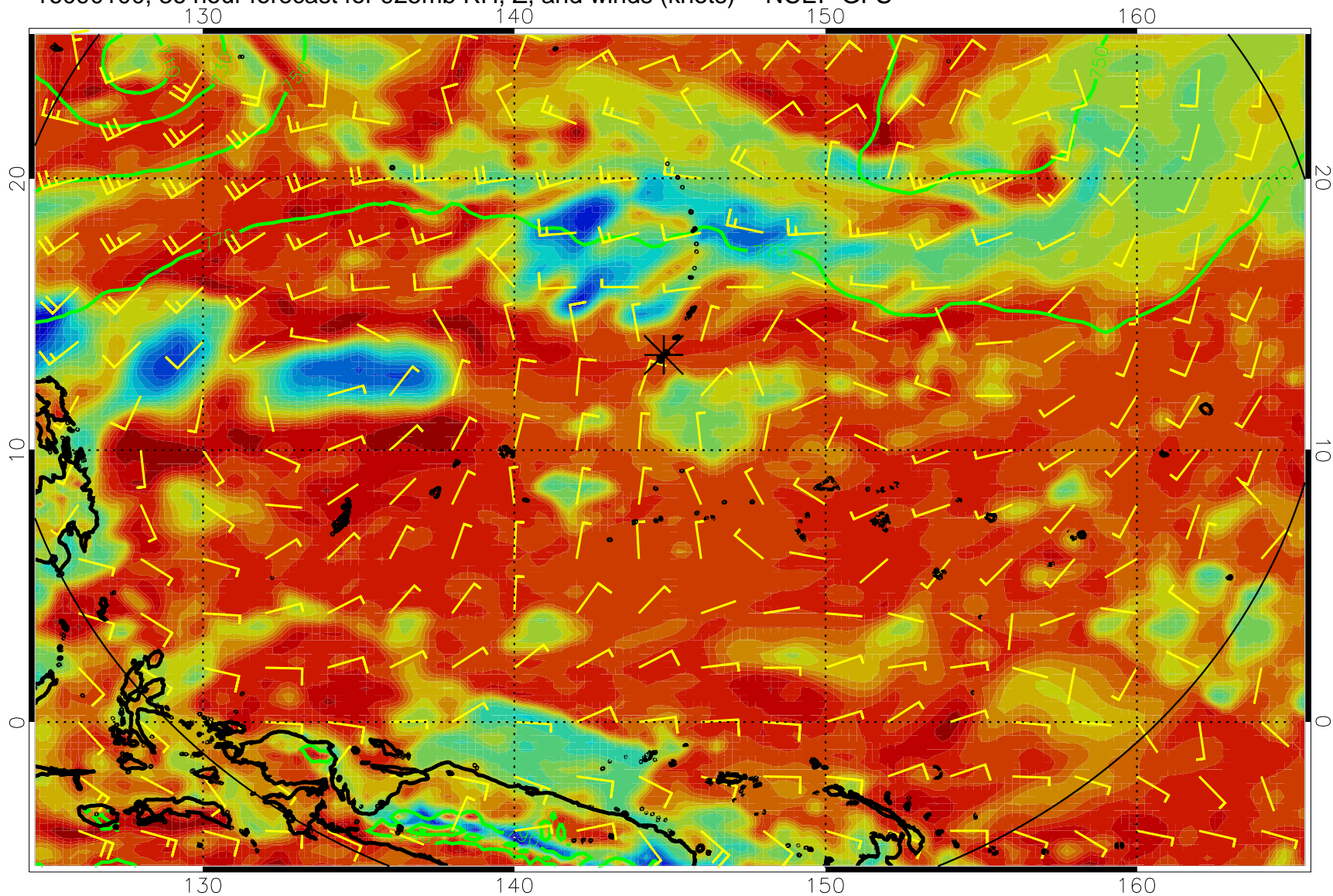
16090100, 36 hour forecast for 925mb RH, Z, and winds (knots) -- NCEP GFS
