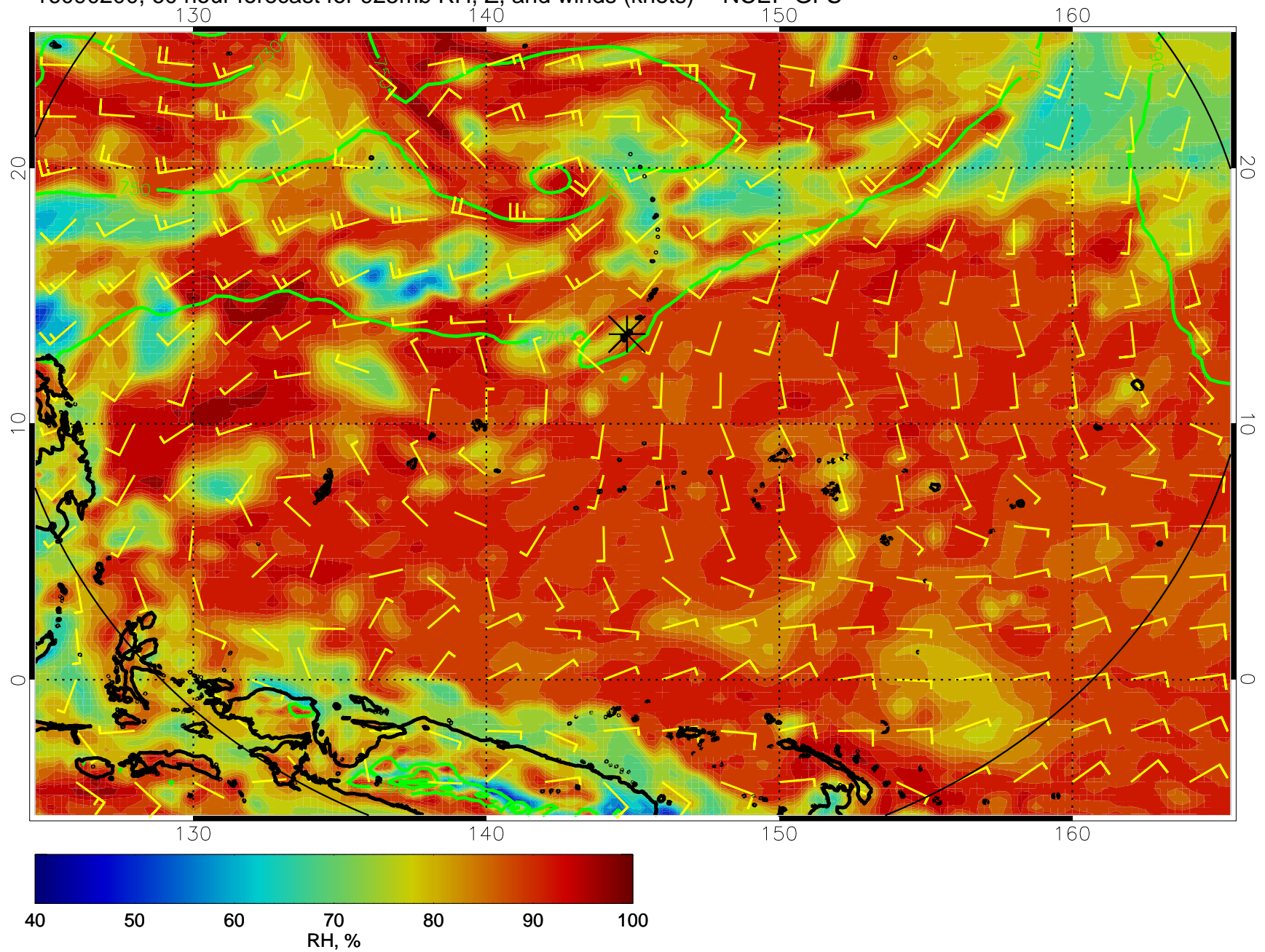
16090200, 60 hour forecast for 925mb RH, Z, and winds (knots) -- NCEP GFS
