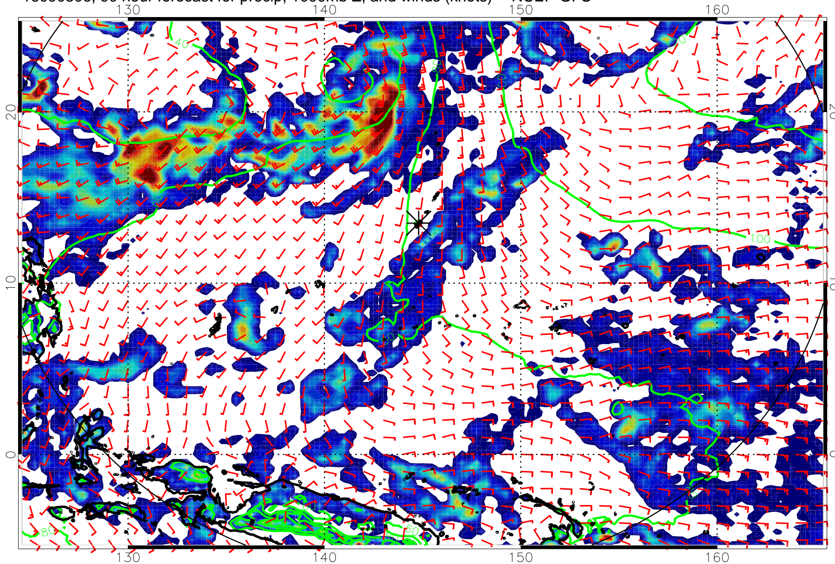
16090306, 90 hour forecast for precip, 1000mb Z, and winds (knots) -- NCEP GFS
