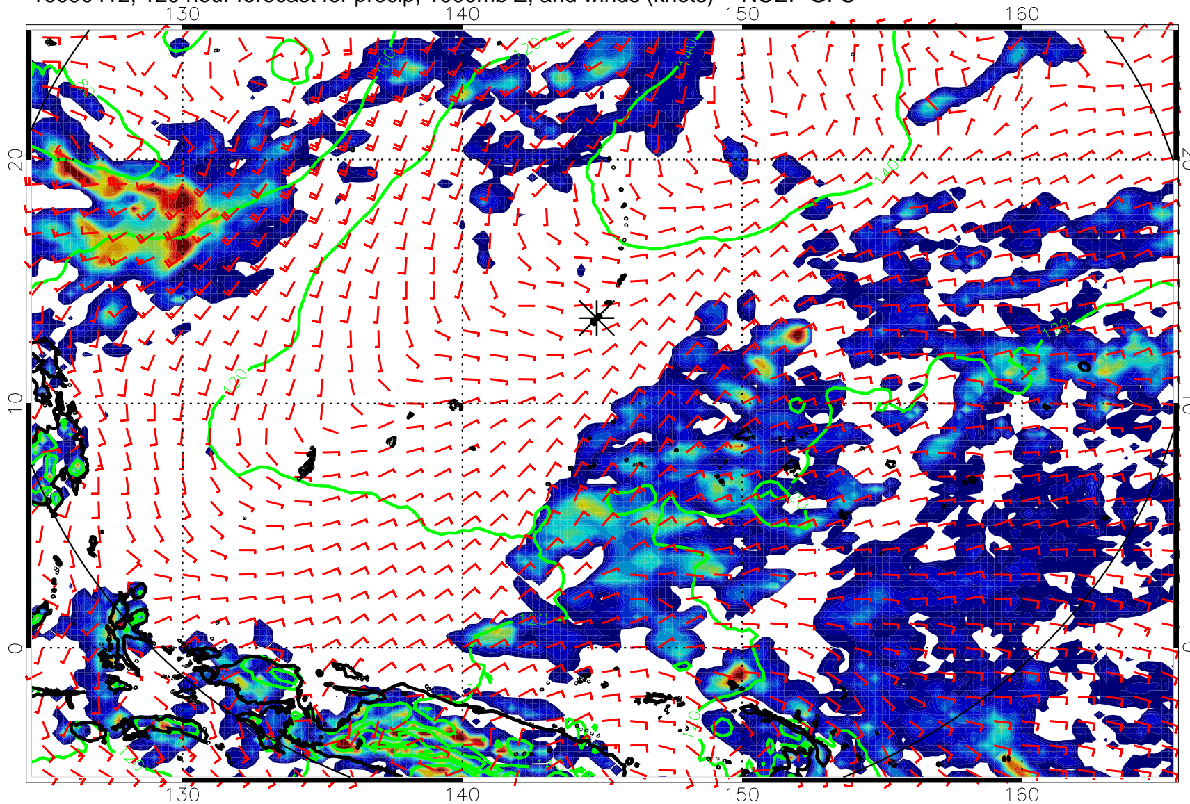
16090412, 120 hour forecast for precip, 1000mb Z, and winds (knots) -- NCEP GFS
