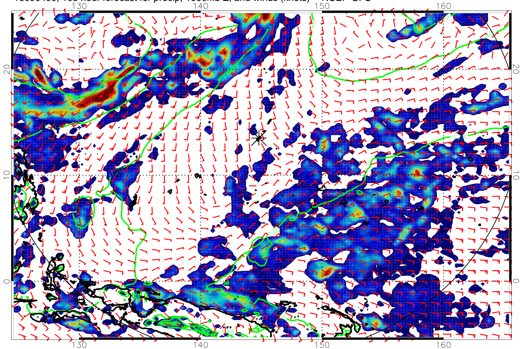
16090400, 108 hour forecast for precip, 1000mb Z, and winds (knots) -- NCEP GFS
