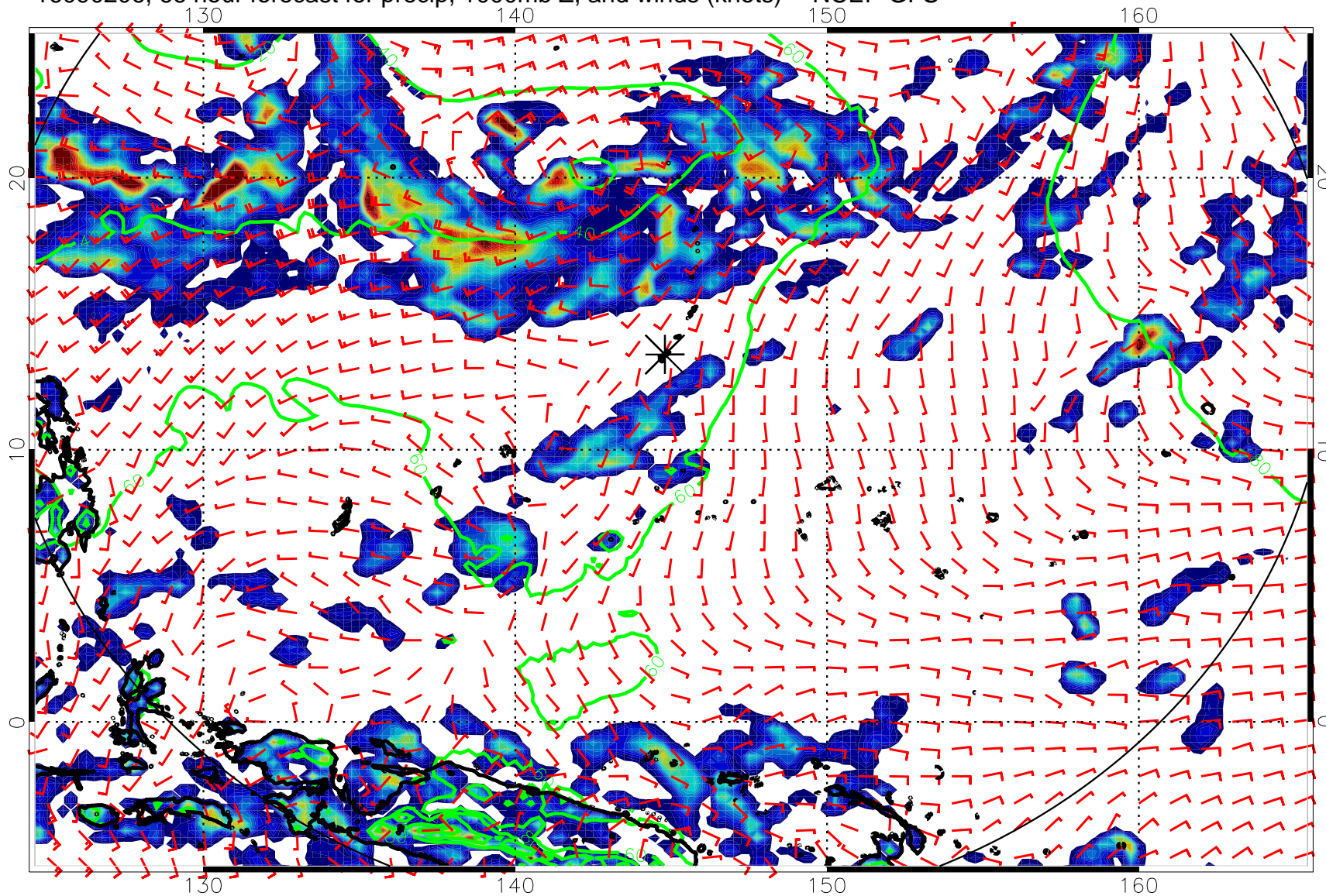
16090206, 66 hour forecast for precip, 1000mb Z, and winds (knots) -- NCEP GFS
