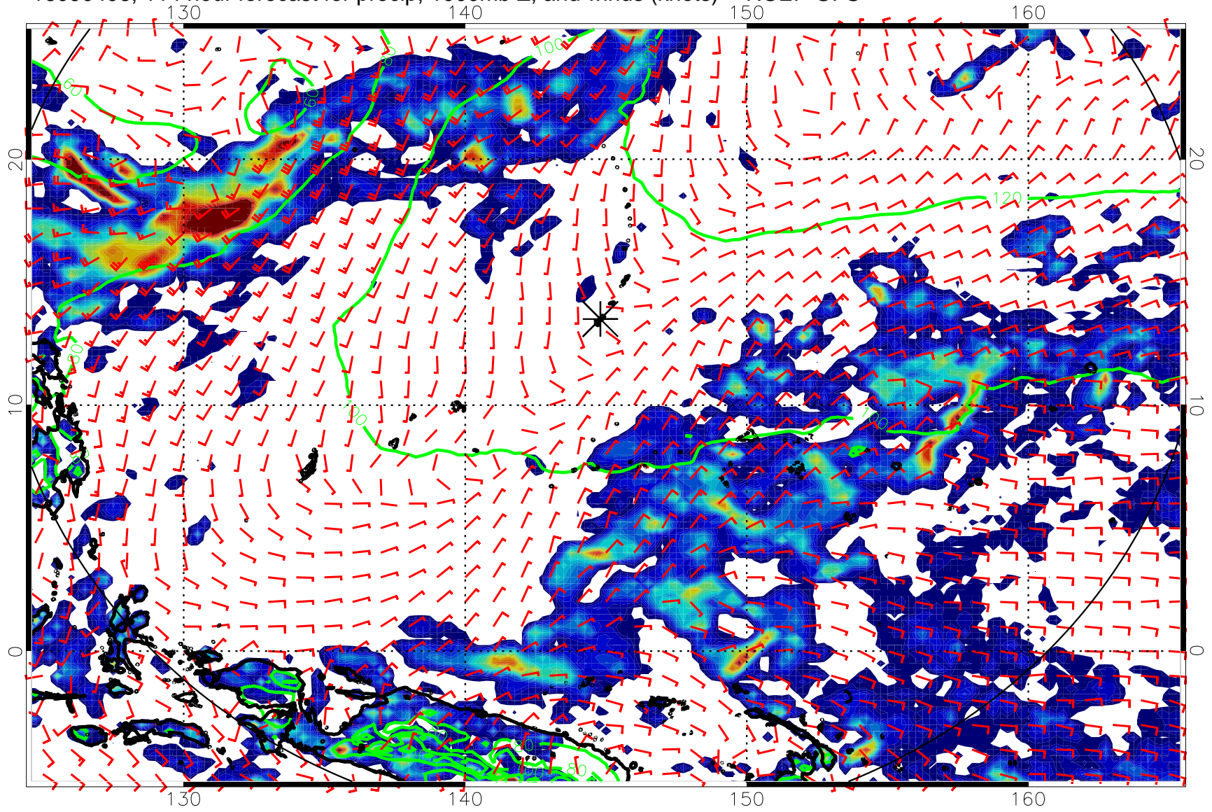
16090406, 114 hour forecast for precip, 1000mb Z, and winds (knots) -- NCEP GFS
