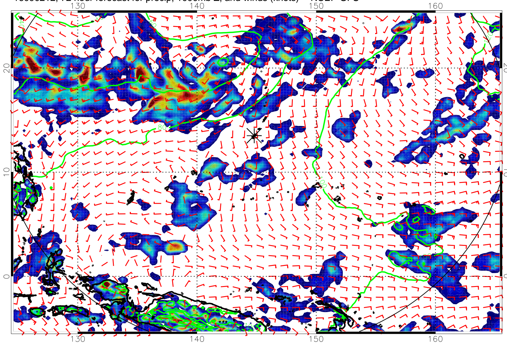
16090212, 72 hour forecast for precip, 1000mb Z, and winds (knots) -- NCEP GFS
