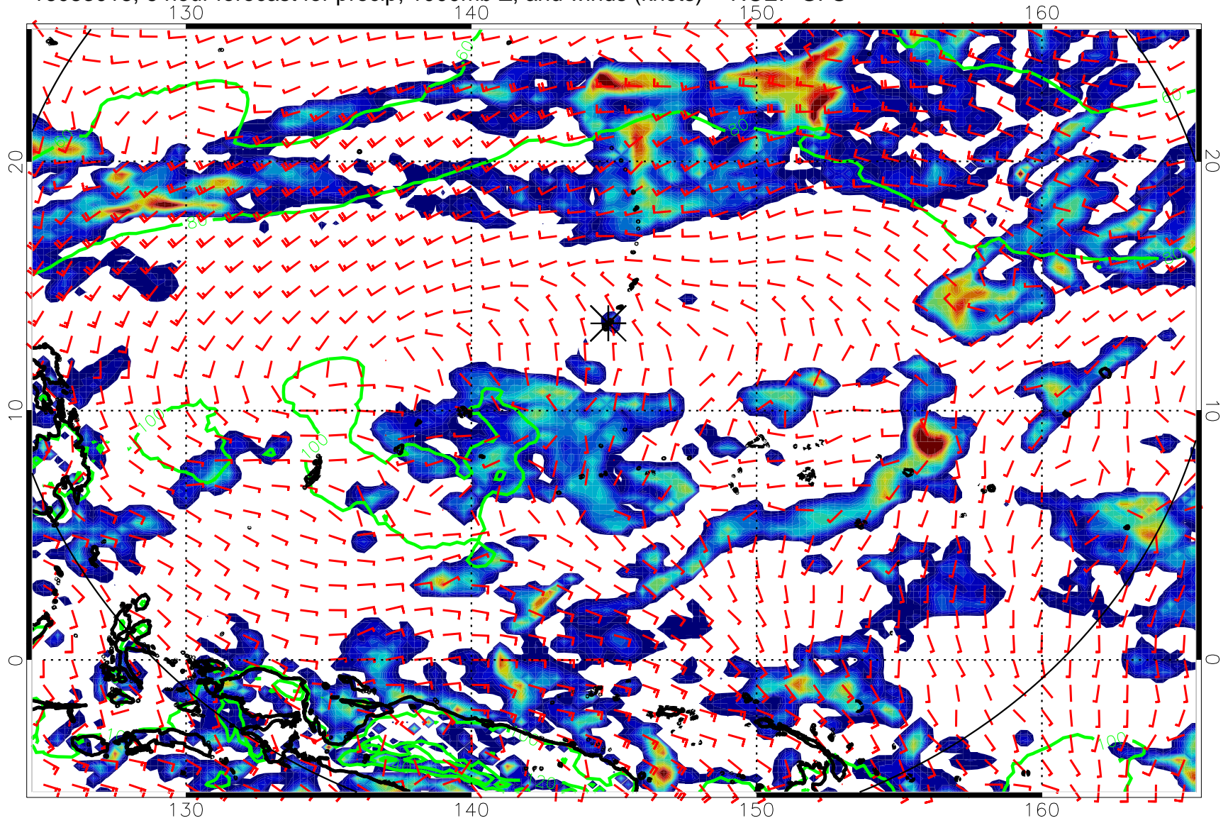
16083018, 6 hour forecast for precip, 1000mb Z, and winds (knots) -- NCEP GFS
