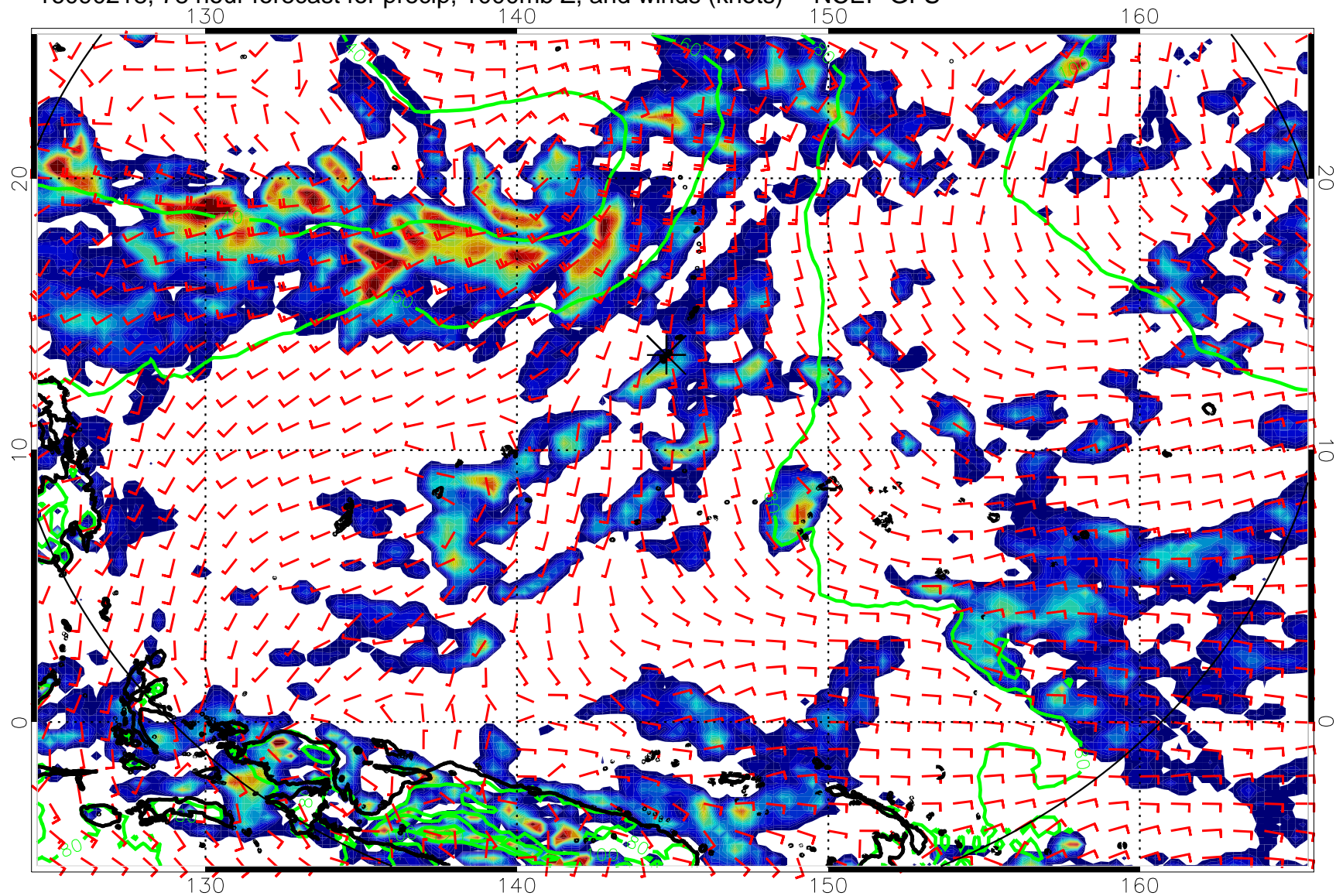
16090218, 78 hour forecast for precip, 1000mb Z, and winds (knots) -- NCEP GFS
