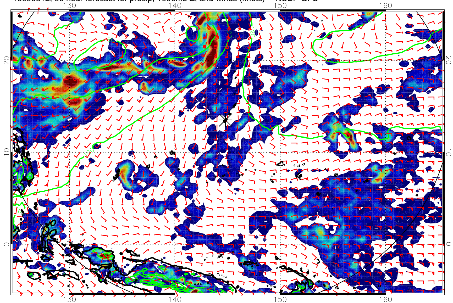
16090312, 96 hour forecast for precip, 1000mb Z, and winds (knots) -- NCEP GFS
