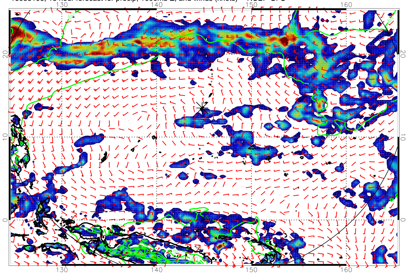
16083106, 18 hour forecast for precip, 1000mb Z, and winds (knots) -- NCEP GFS
