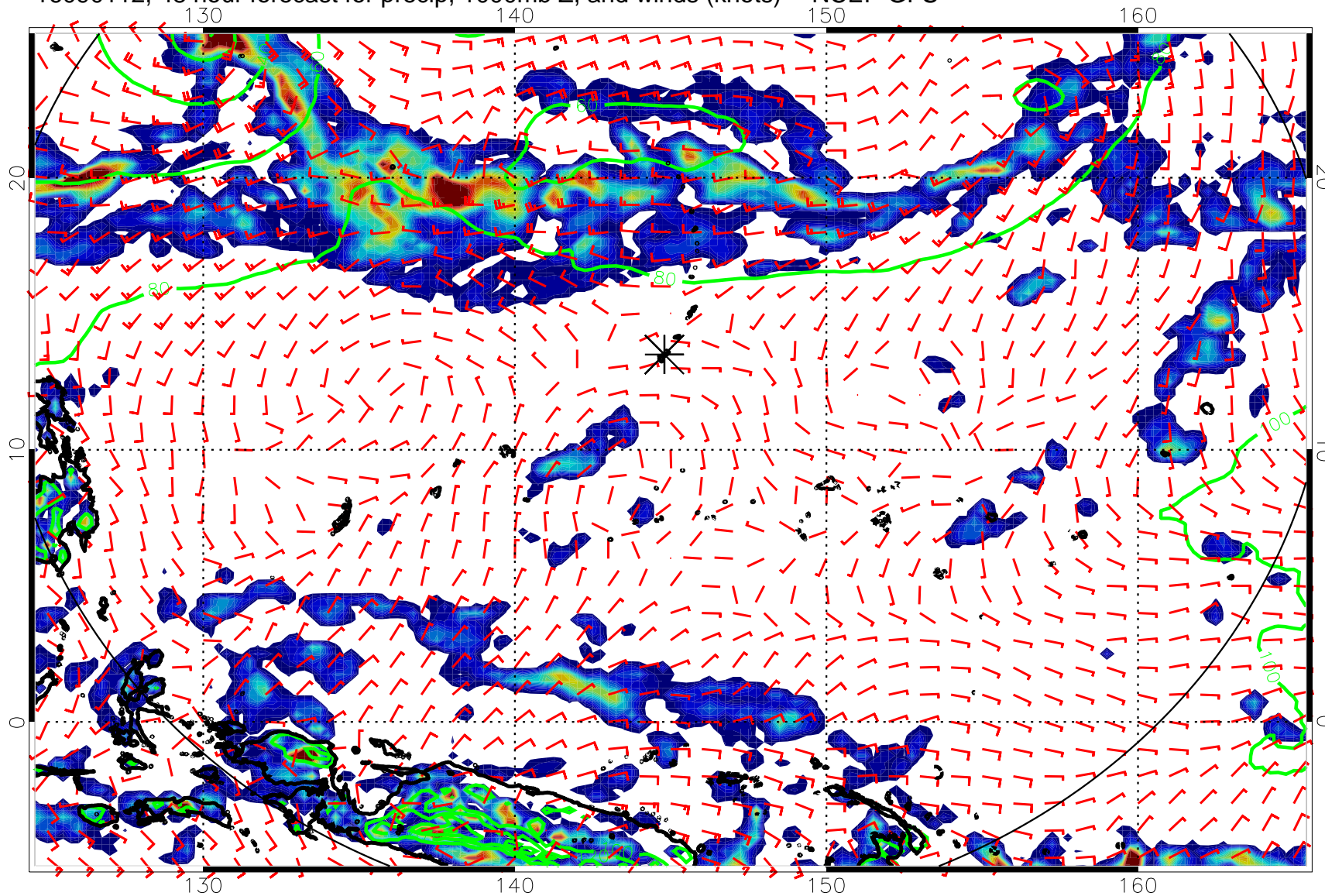
16090112, 48 hour forecast for precip, 1000mb Z, and winds (knots) -- NCEP GFS
