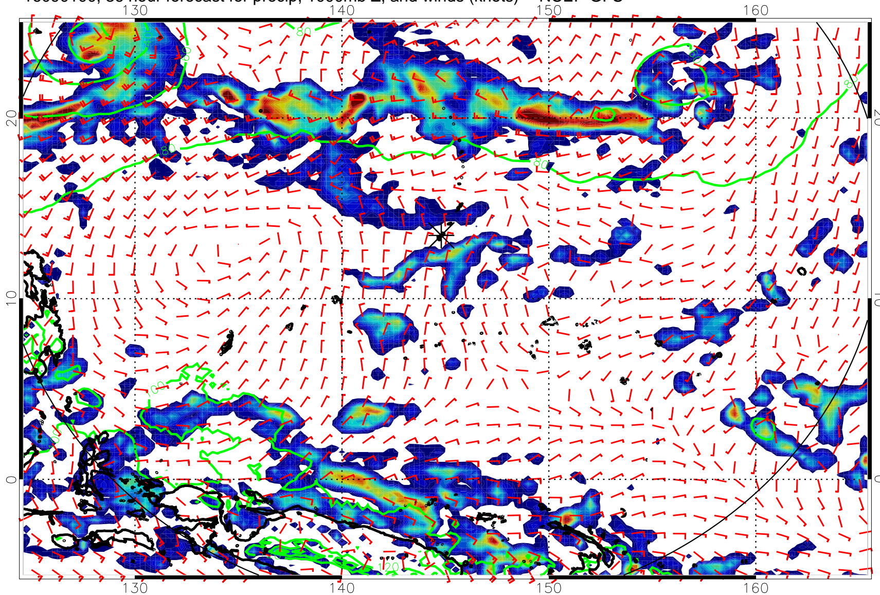
16090100, 36 hour forecast for precip, 1000mb Z, and winds (knots) -- NCEP GFS
