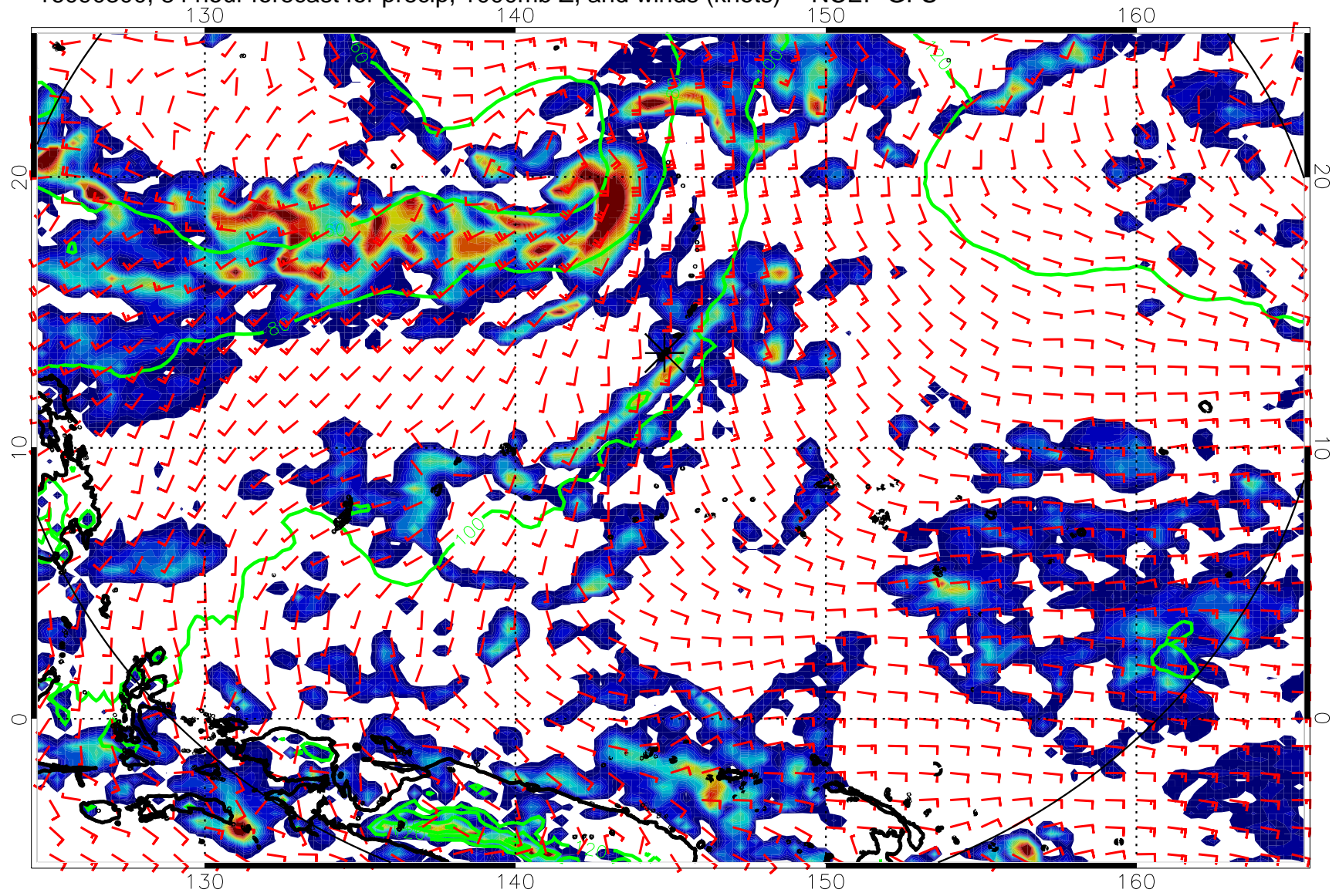
16090300, 84 hour forecast for precip, 1000mb Z, and winds (knots) -- NCEP GFS
