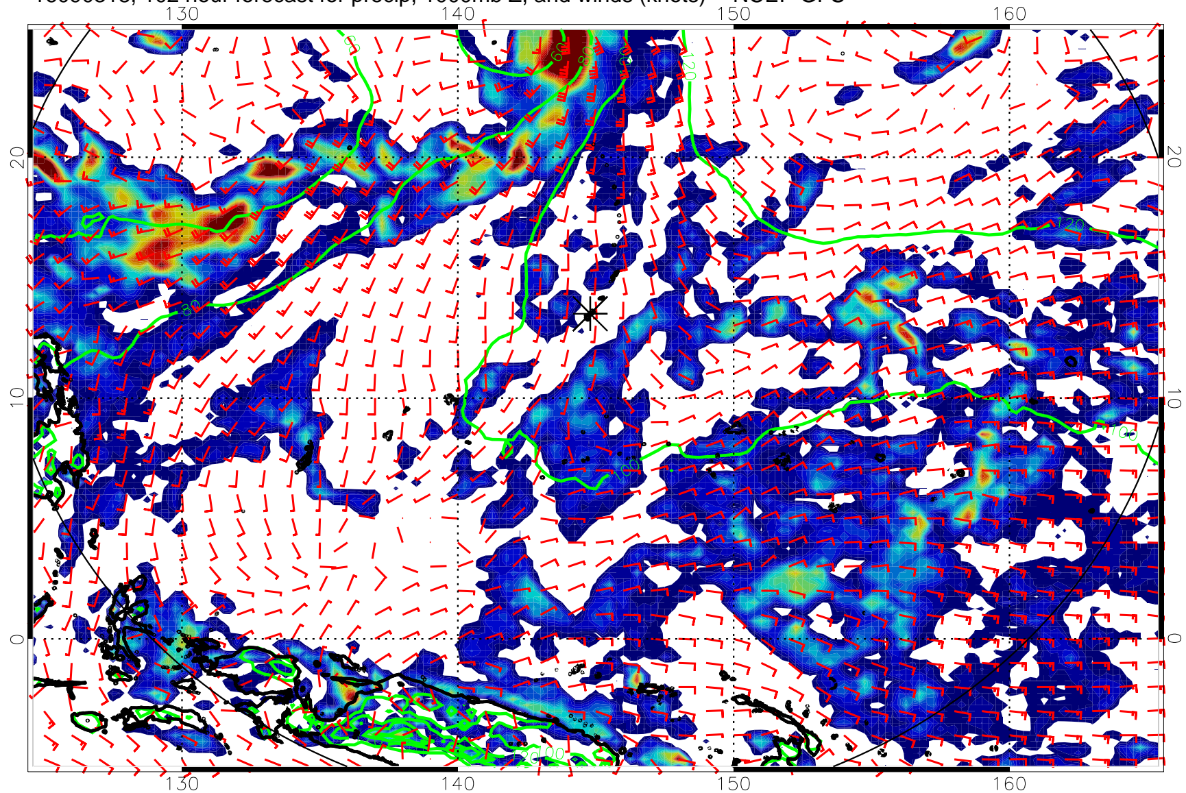
16090318, 102 hour forecast for precip, 1000mb Z, and winds (knots) -- NCEP GFS
