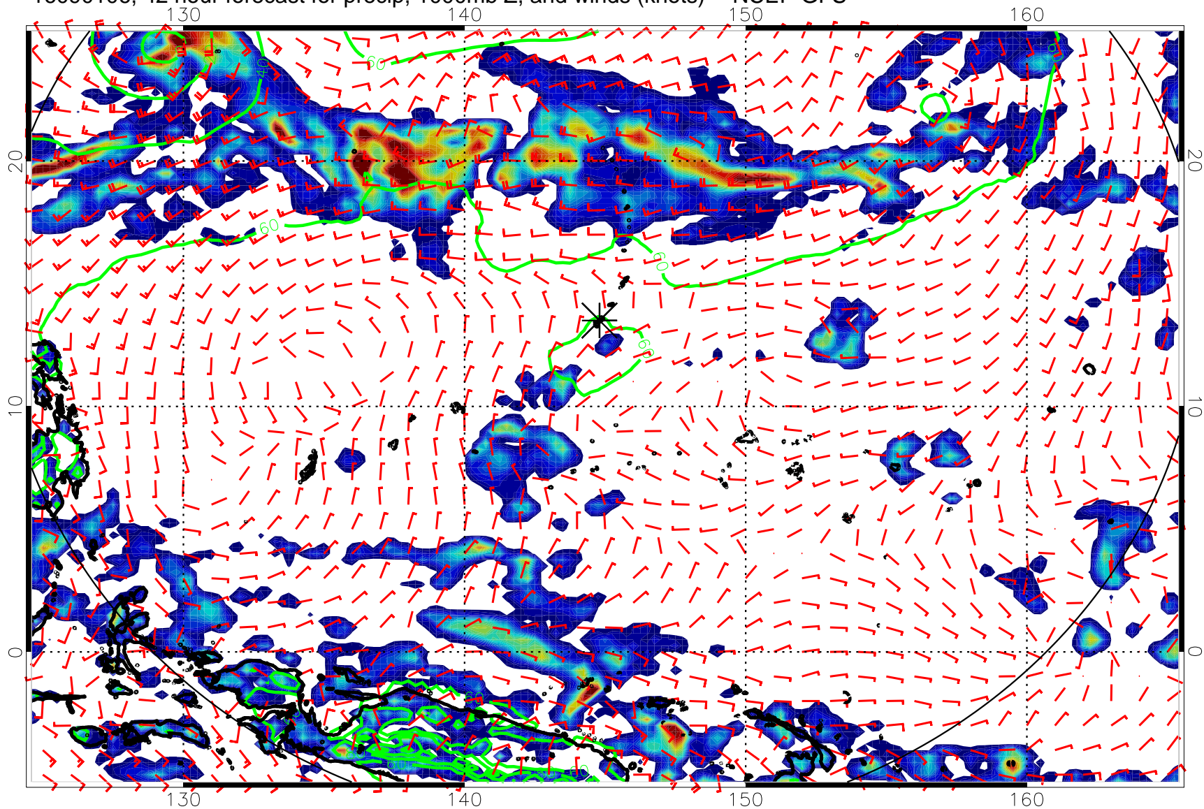
16090106, 42 hour forecast for precip, 1000mb Z, and winds (knots) -- NCEP GFS
