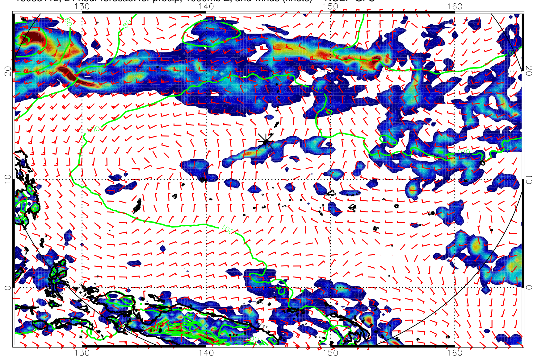
16083112, 24 hour forecast for precip, 1000mb Z, and winds (knots) -- NCEP GFS
