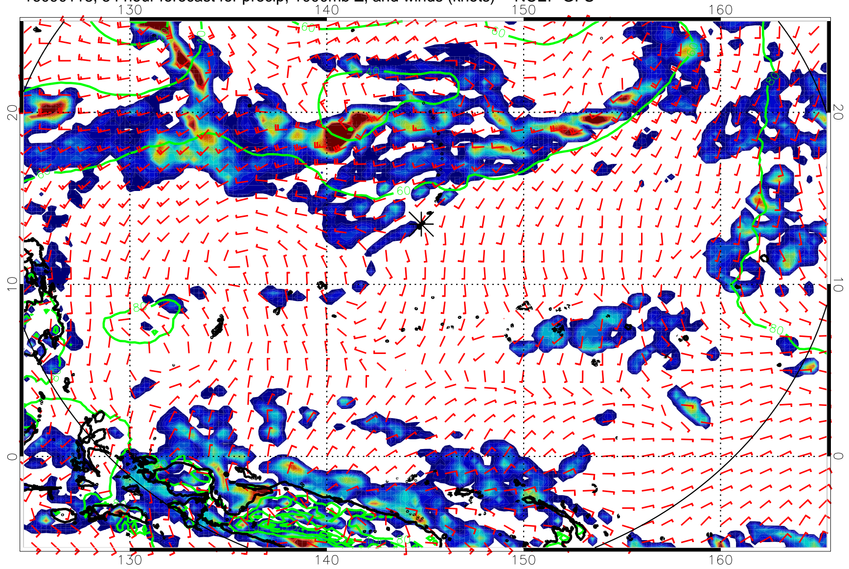
16090118, 54 hour forecast for precip, 1000mb Z, and winds (knots) -- NCEP GFS
