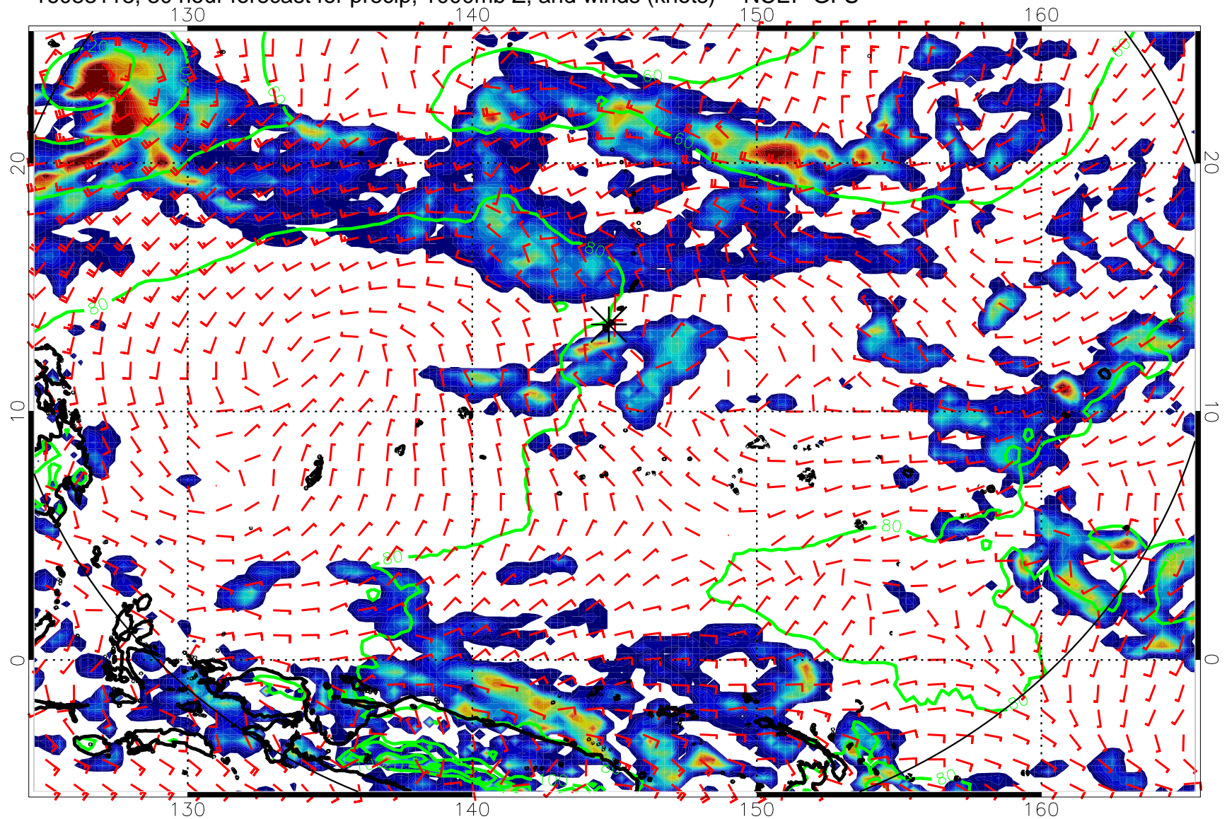
16083118, 30 hour forecast for precip, 1000mb Z, and winds (knots) -- NCEP GFS
