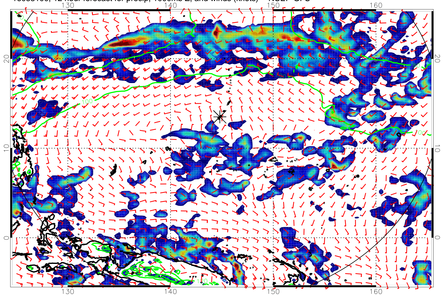
16083100, 12 hour forecast for precip, 1000mb Z, and winds (knots) -- NCEP GFS
