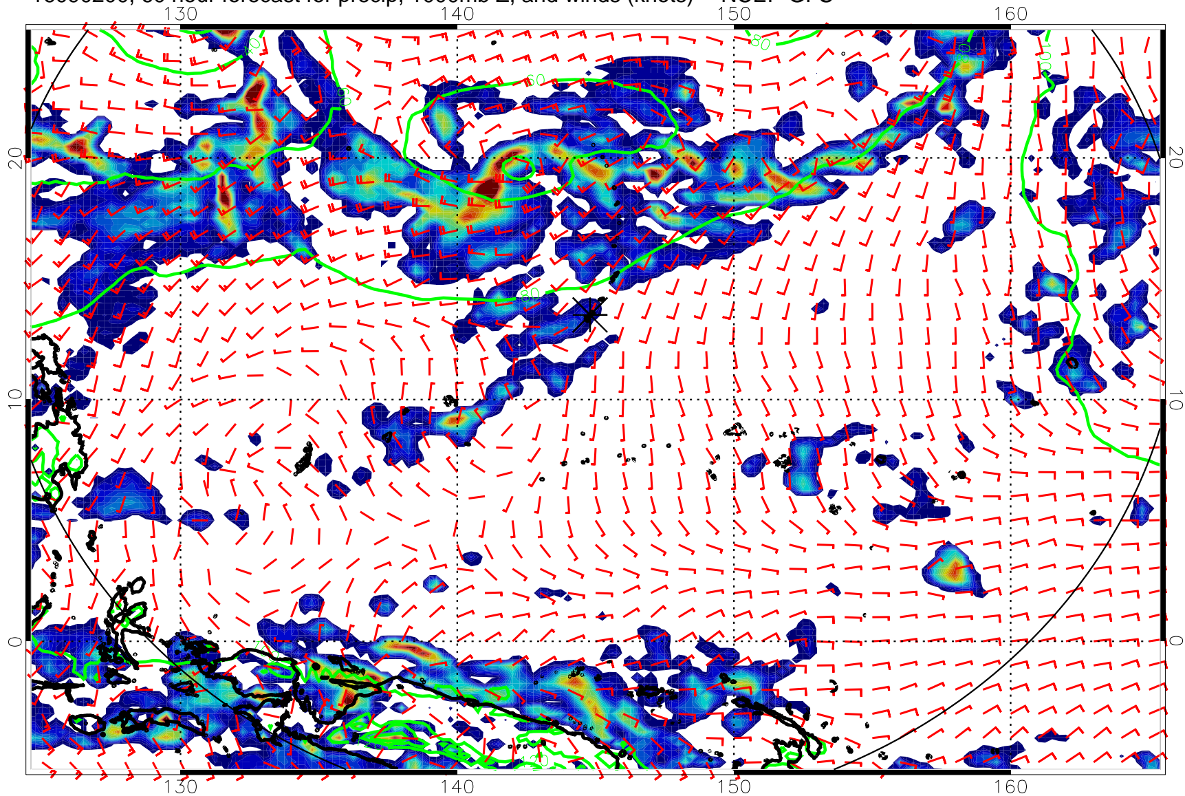
16090200, 60 hour forecast for precip, 1000mb Z, and winds (knots) -- NCEP GFS
