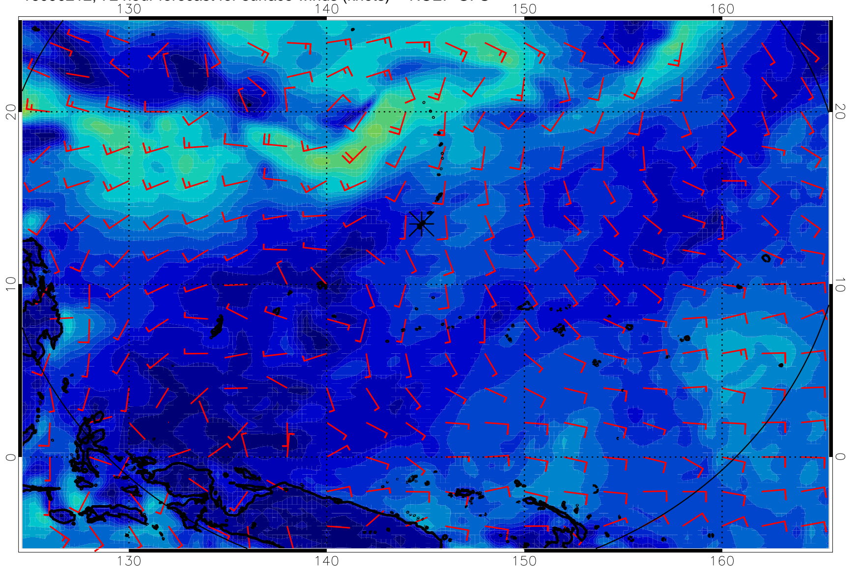
16090212, 72 hour forecast for surface winds (knots) -- NCEP GFS
