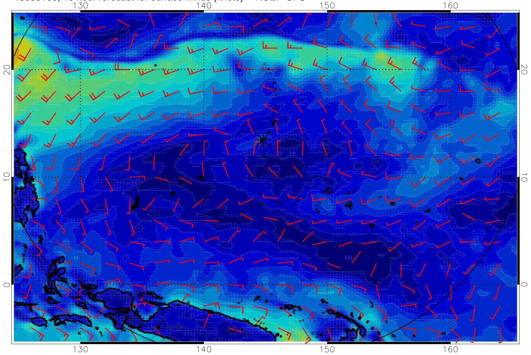
16083106, 18 hour forecast for surface winds (knots) -- NCEP GFS
