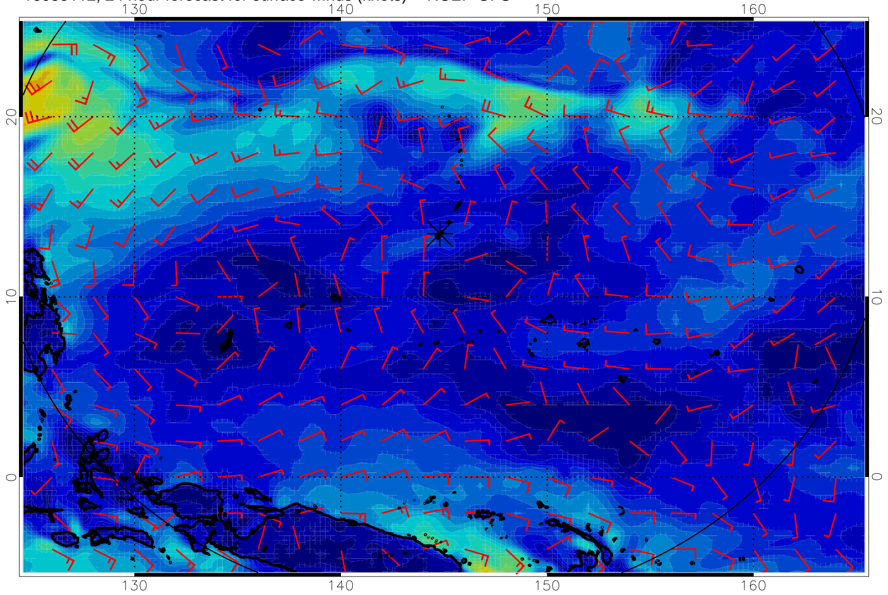
16083112, 24 hour forecast for surface winds (knots) -- NCEP GFS
