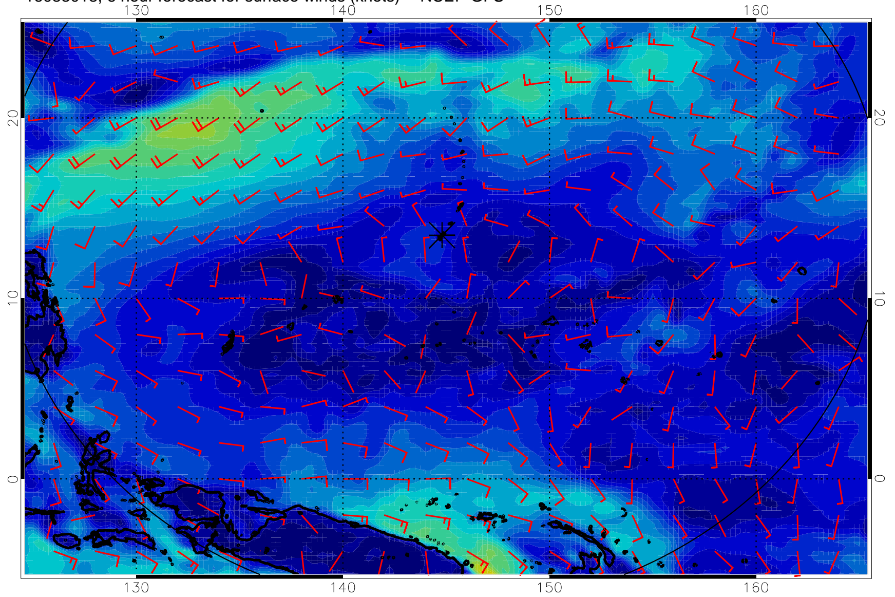
16083018, 6 hour forecast for surface winds (knots) -- NCEP GFS
