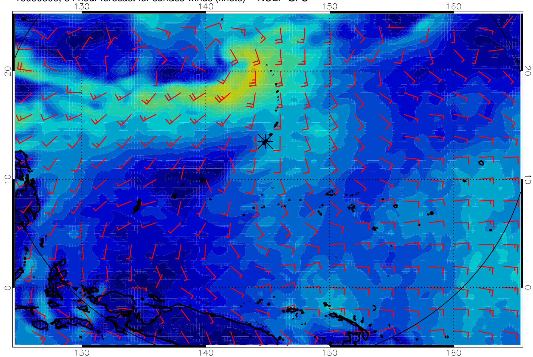
16090300, 84 hour forecast for surface winds (knots) -- NCEP GFS
