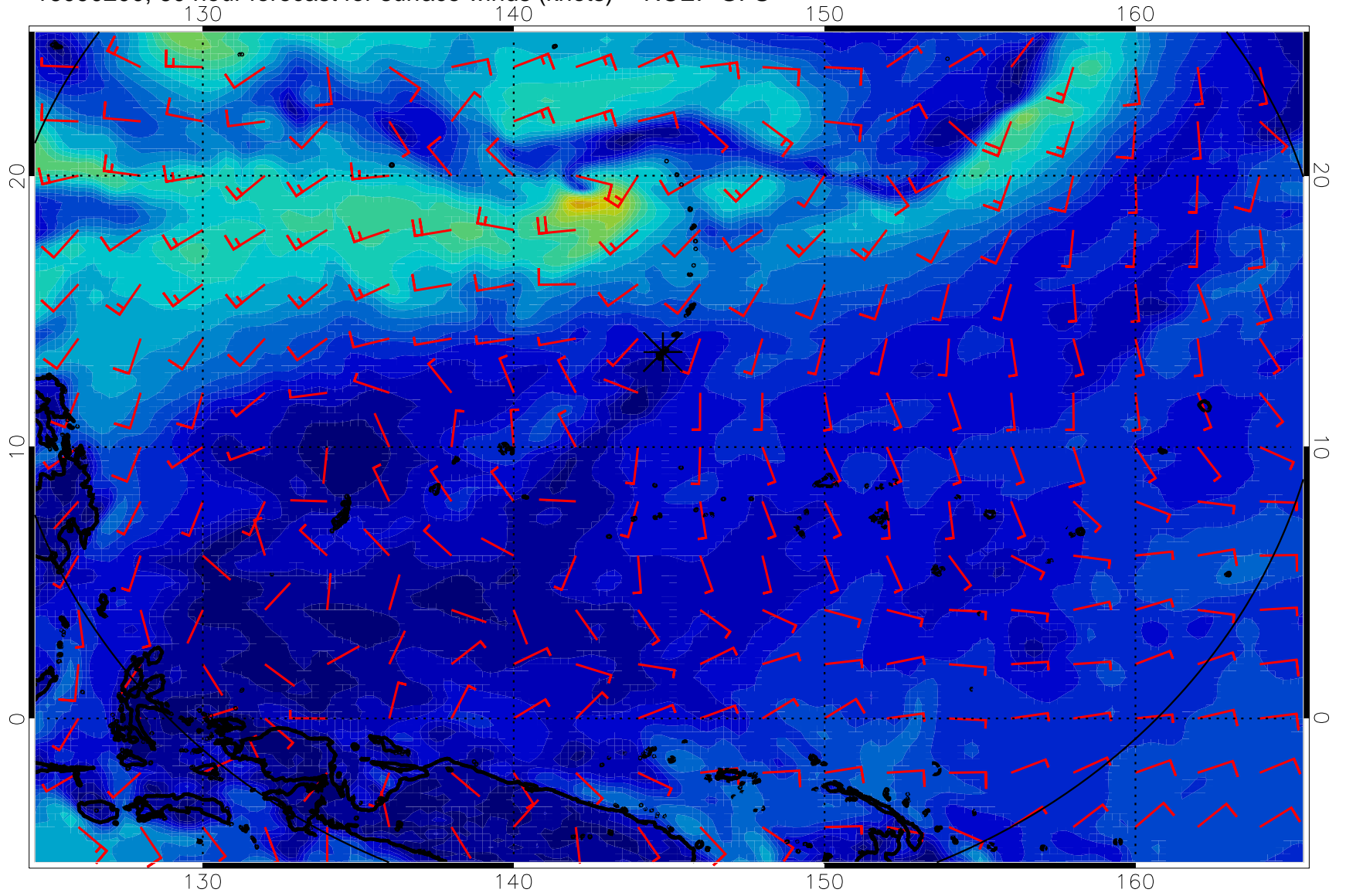
16090200, 60 hour forecast for surface winds (knots) -- NCEP GFS
