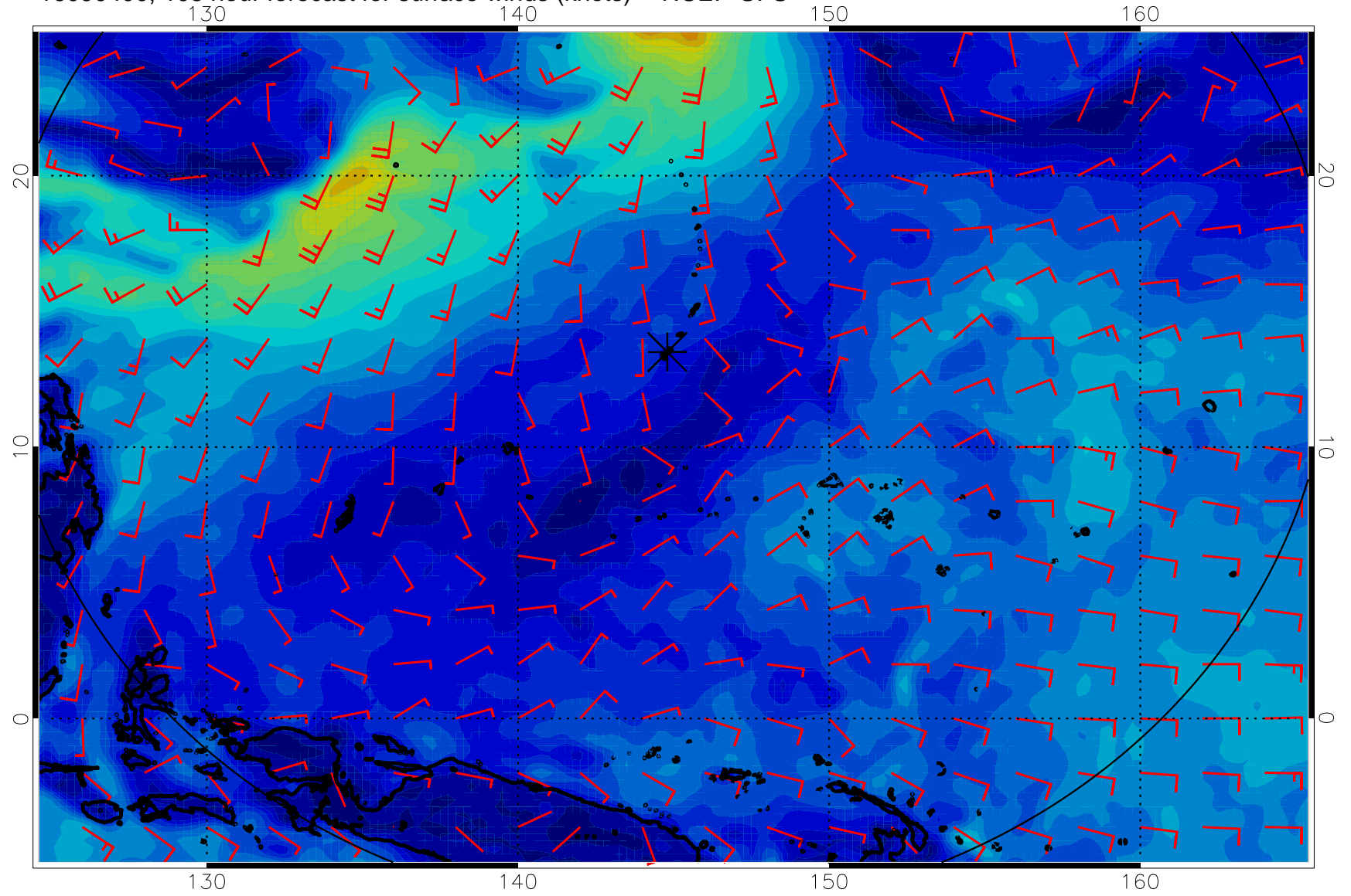
16090400, 108 hour forecast for surface winds (knots) -- NCEP GFS
