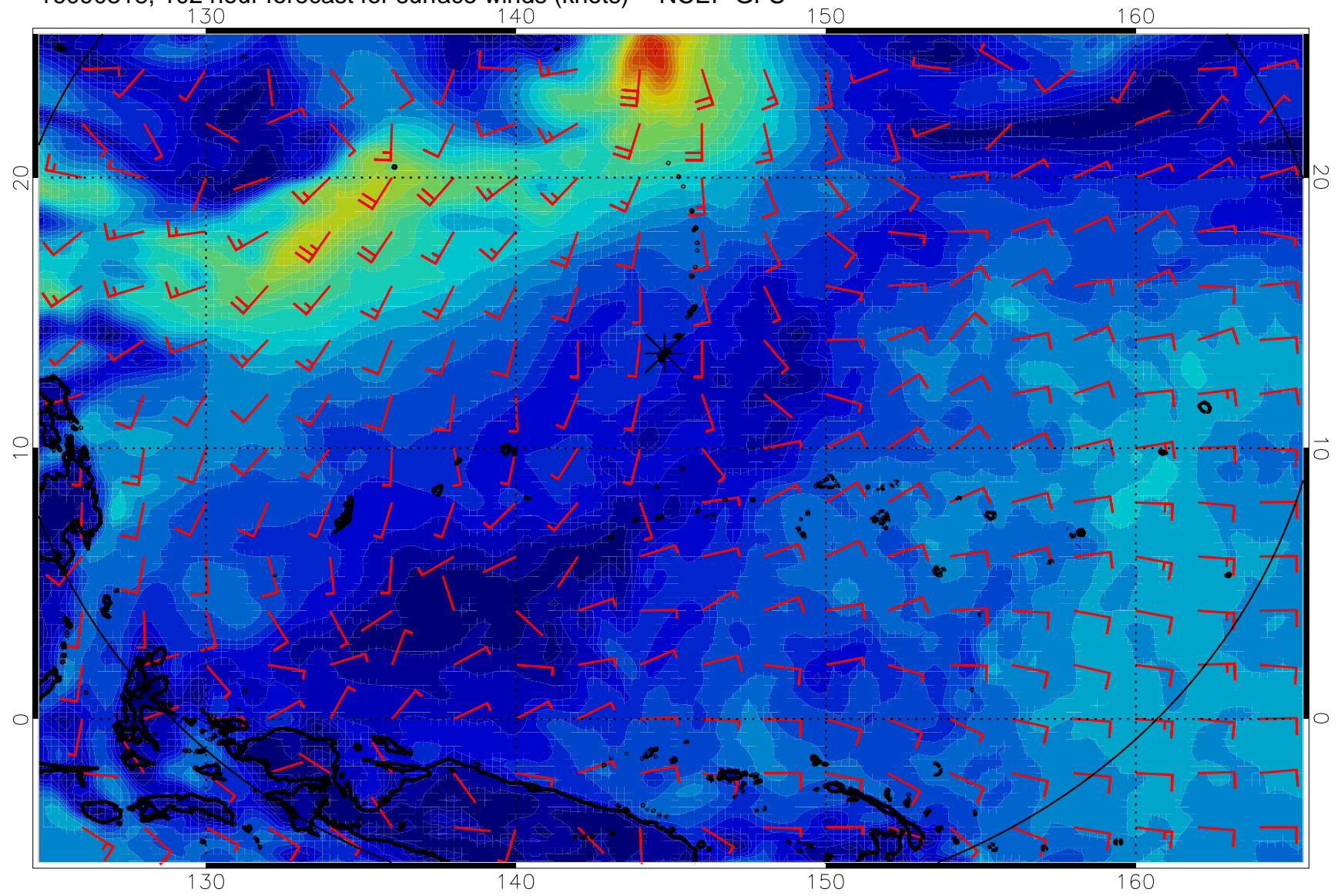
16090318, 102 hour forecast for surface winds (knots) -- NCEP GFS
