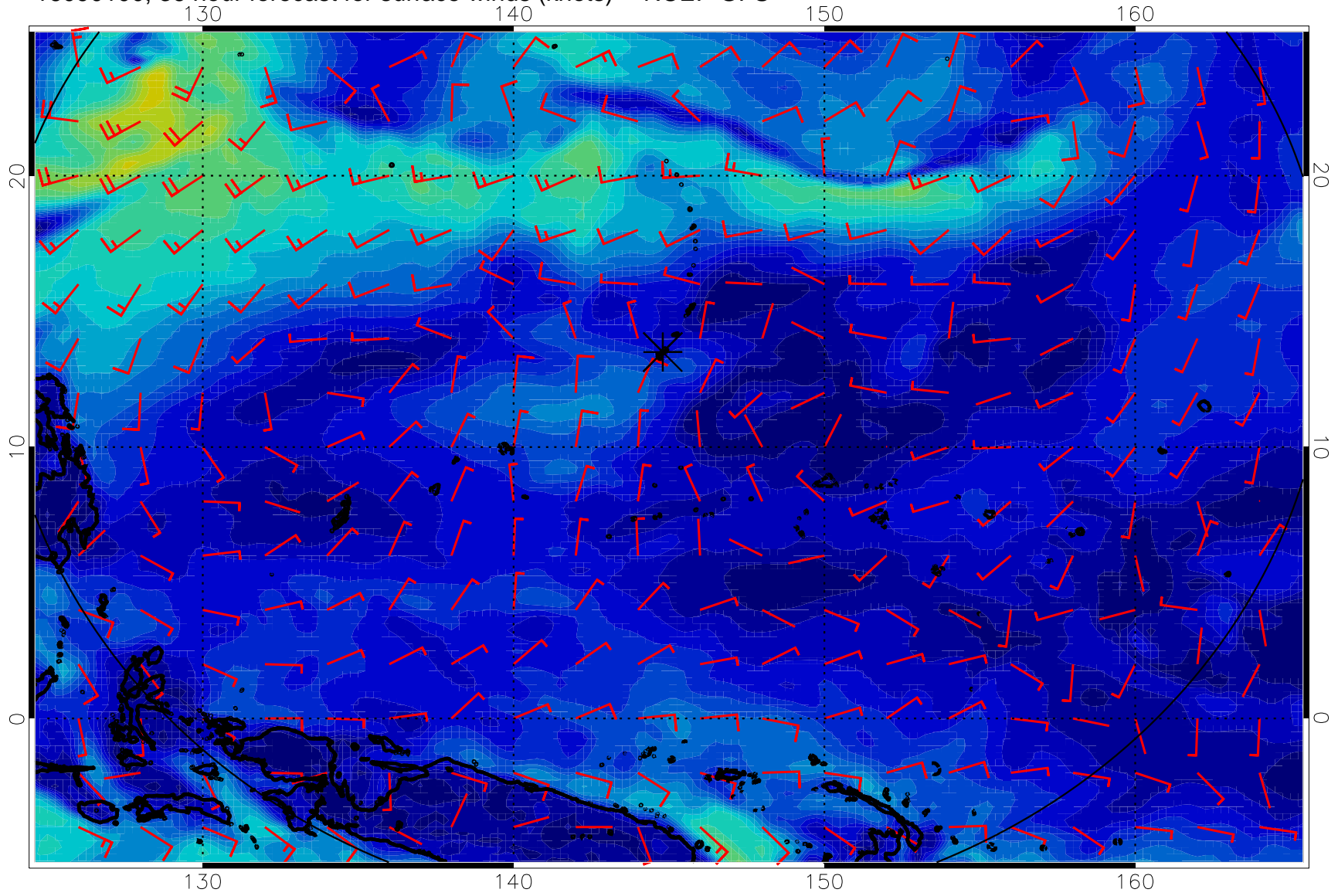
16090100, 36 hour forecast for surface winds (knots) -- NCEP GFS
