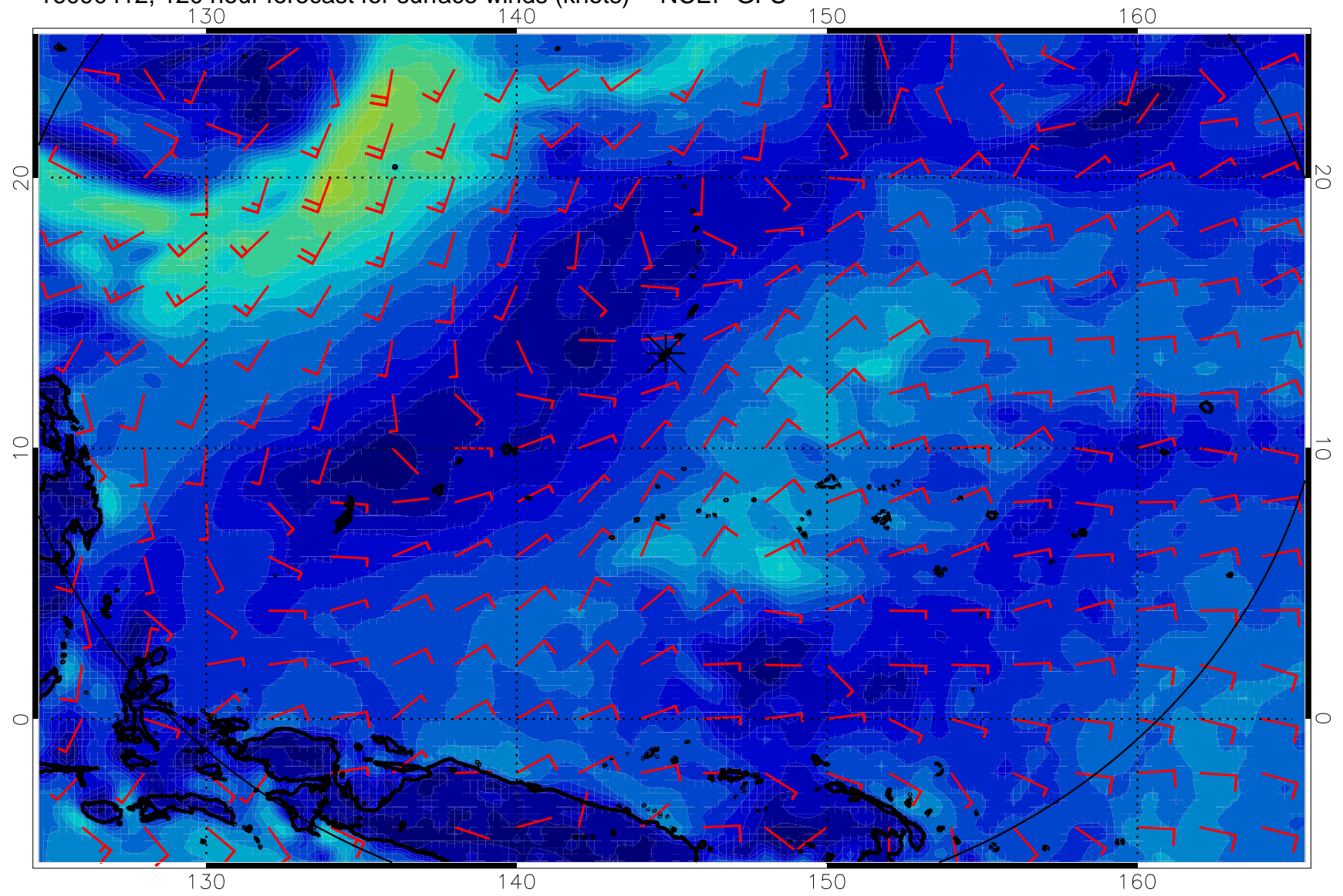
16090412, 120 hour forecast for surface winds (knots) -- NCEP GFS
