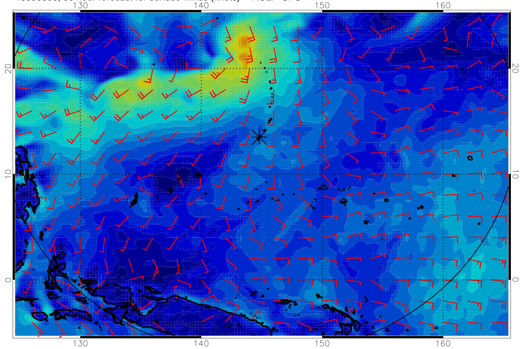
16090306, 90 hour forecast for surface winds (knots) -- NCEP GFS
