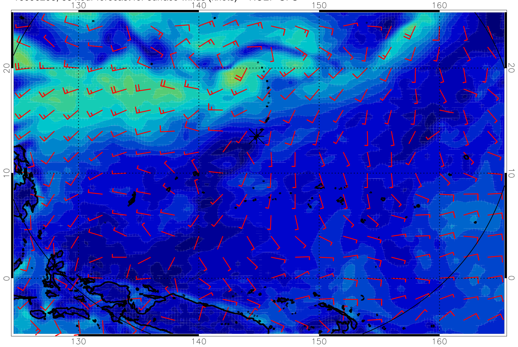
16090206, 66 hour forecast for surface winds (knots) -- NCEP GFS
