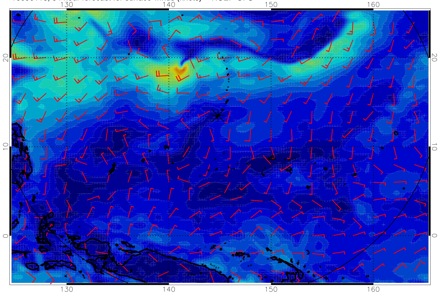
16090118, 54 hour forecast for surface winds (knots) -- NCEP GFS
