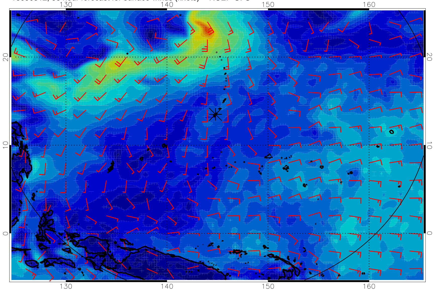
16090312, 96 hour forecast for surface winds (knots) -- NCEP GFS
