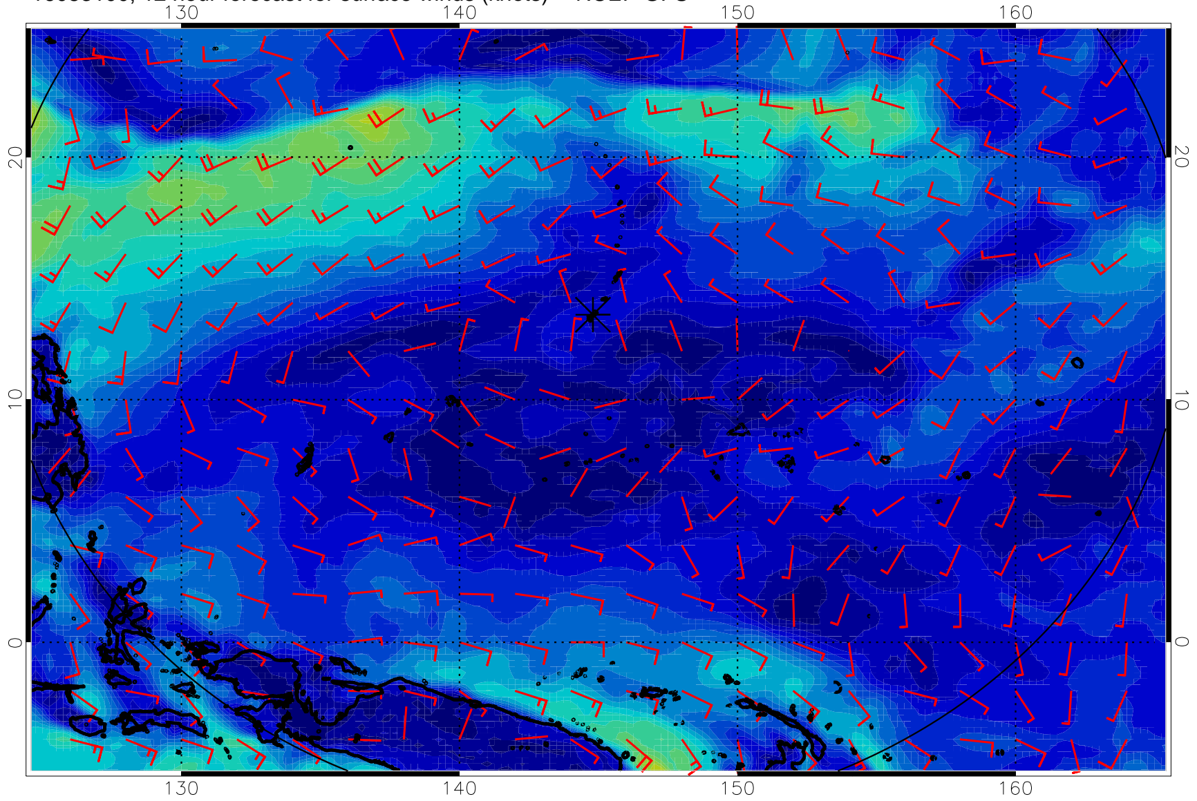
16083100, 12 hour forecast for surface winds (knots) -- NCEP GFS
