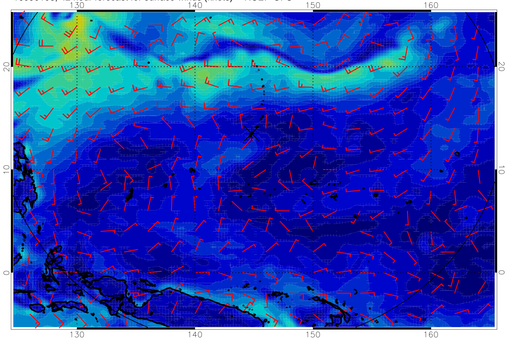
16090106, 42 hour forecast for surface winds (knots) -- NCEP GFS
