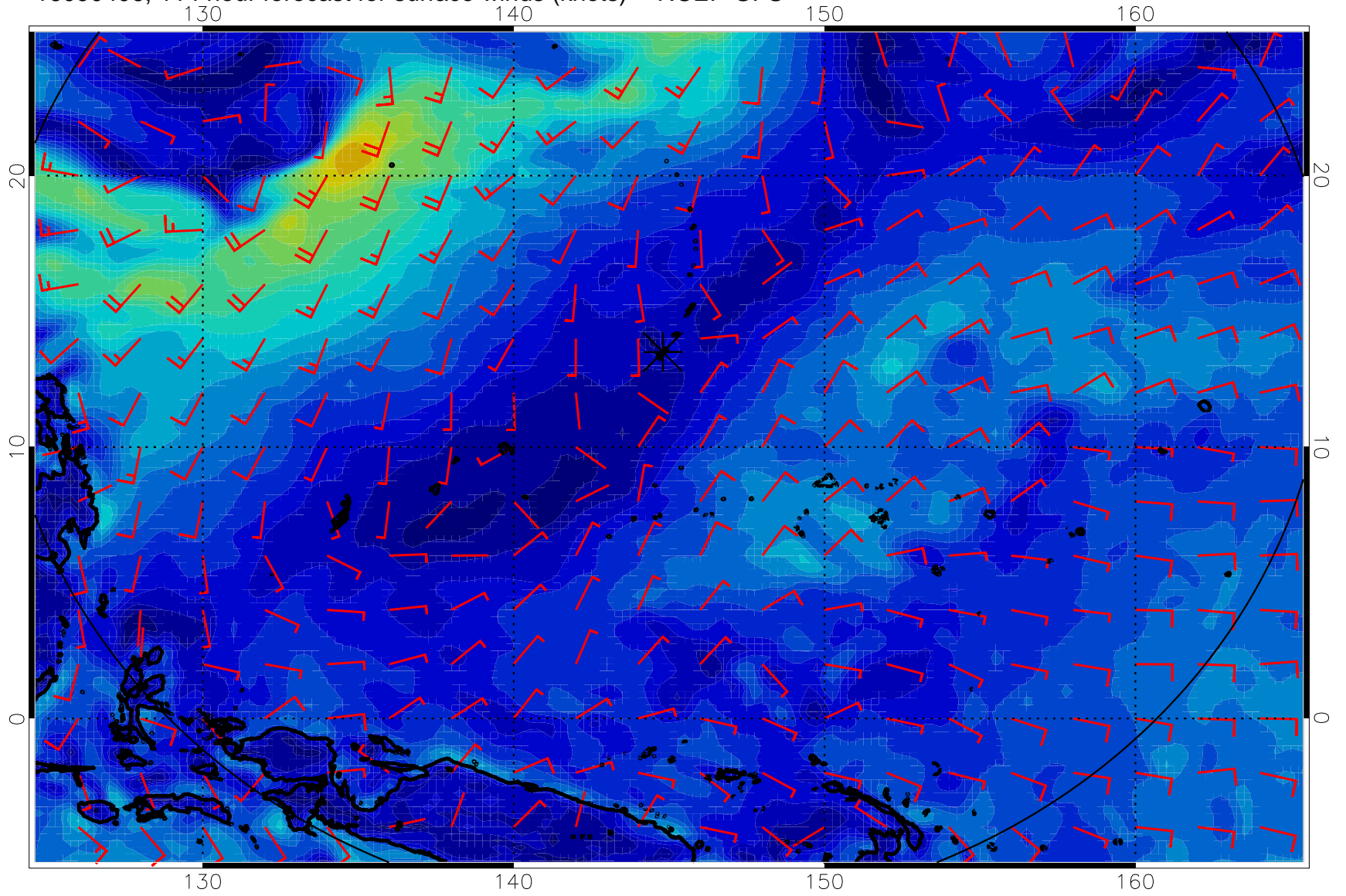
16090406, 114 hour forecast for surface winds (knots) -- NCEP GFS
