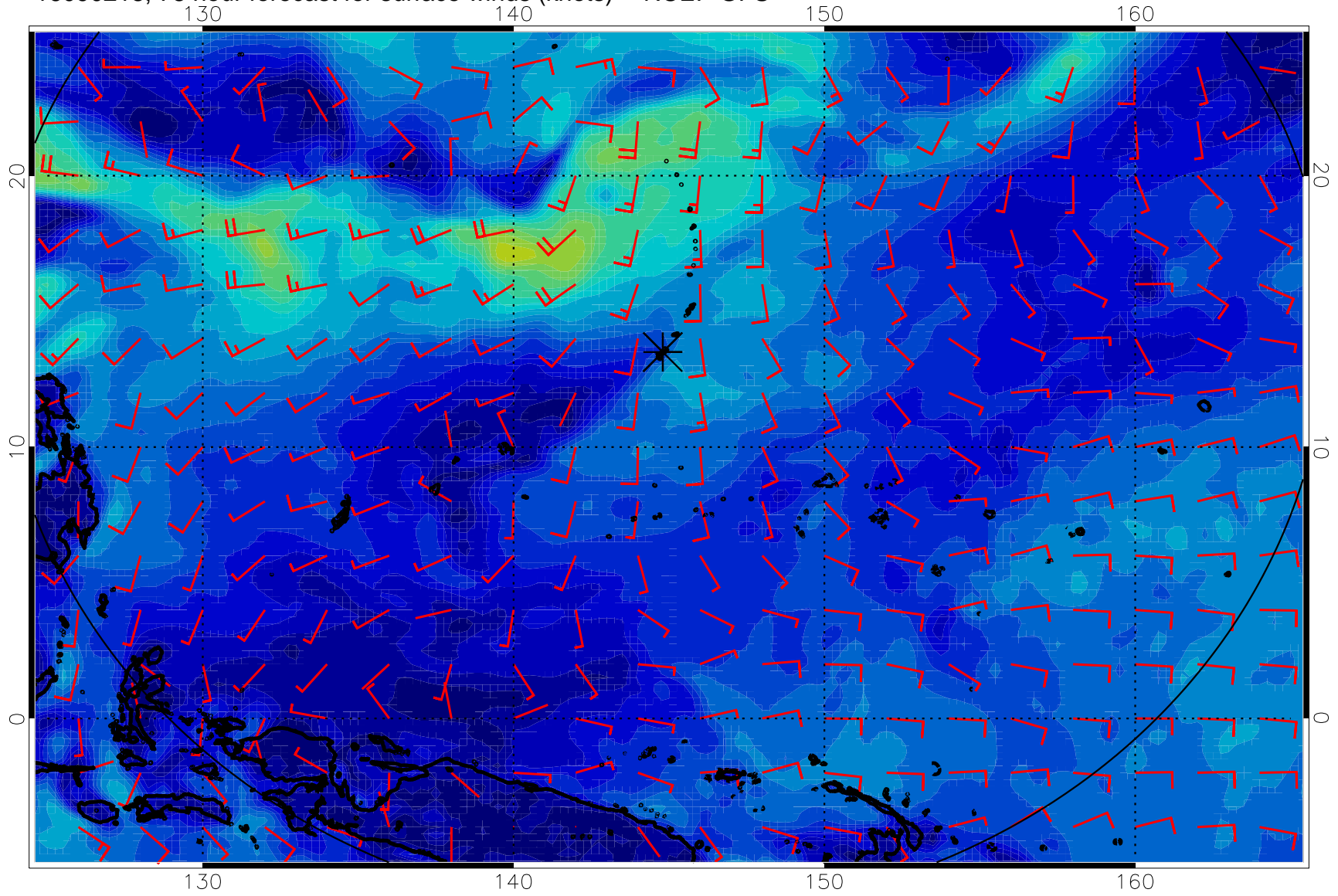
16090218, 78 hour forecast for surface winds (knots) -- NCEP GFS
