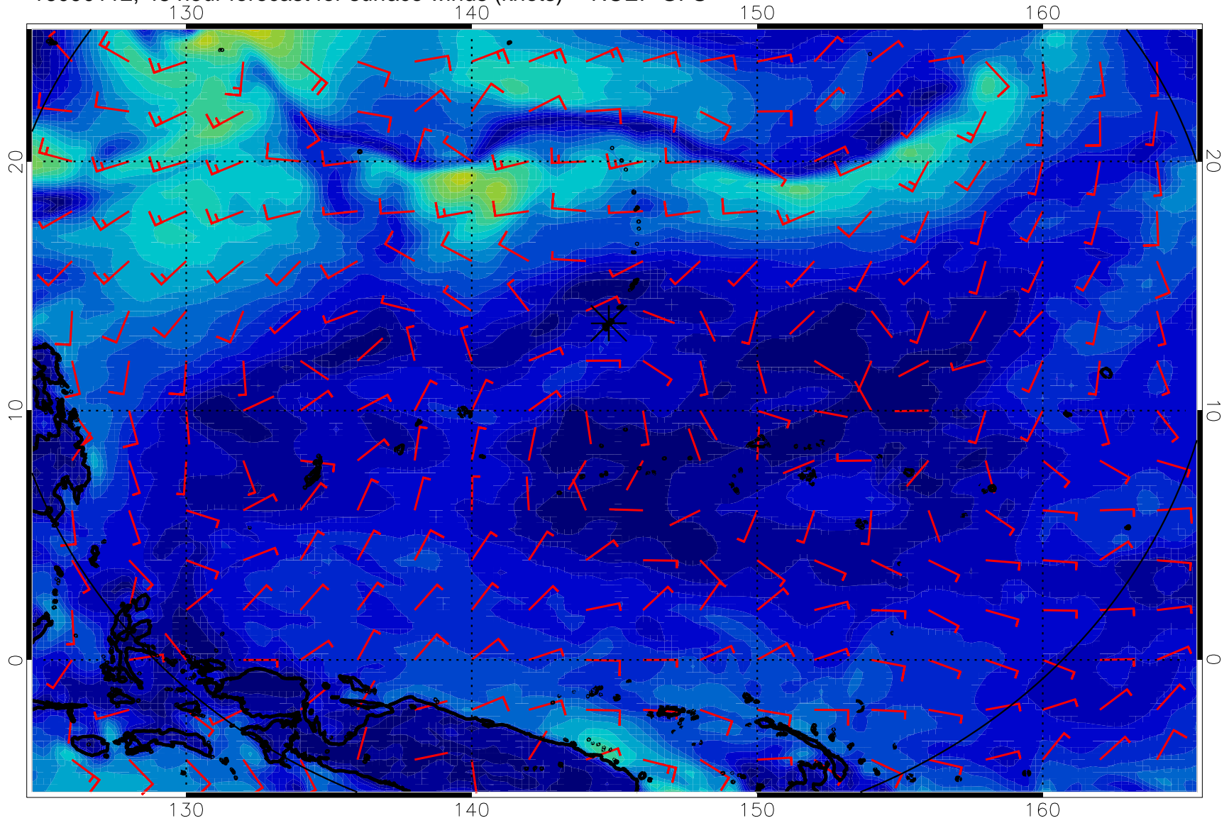
16090112, 48 hour forecast for surface winds (knots) -- NCEP GFS
