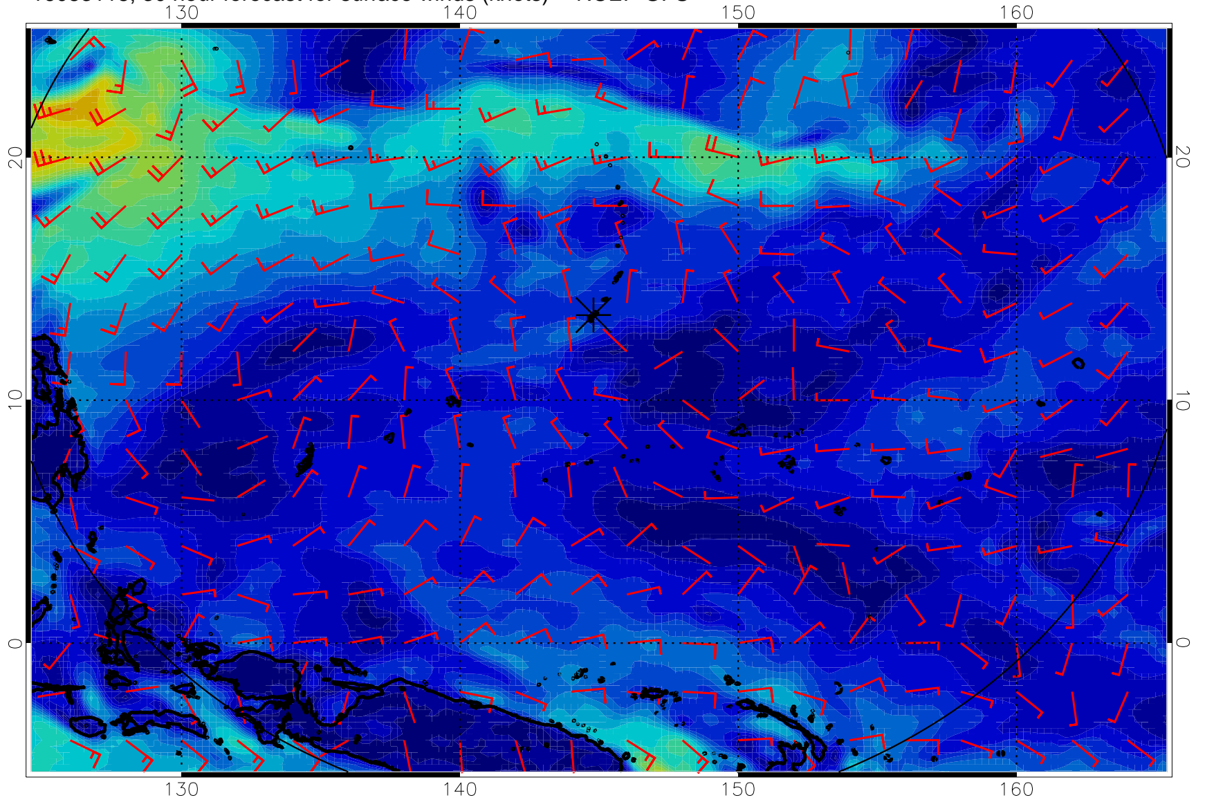
16083118, 30 hour forecast for surface winds (knots) -- NCEP GFS
