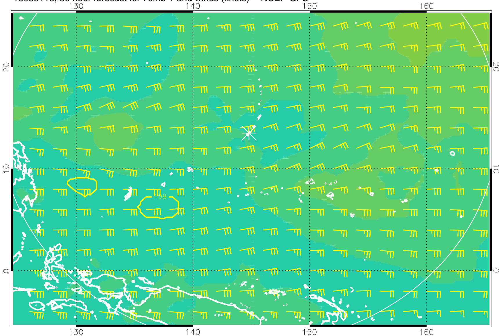
16083118, 30 hour forecast for 70mb T and winds (knots) -- NCEP GFS
