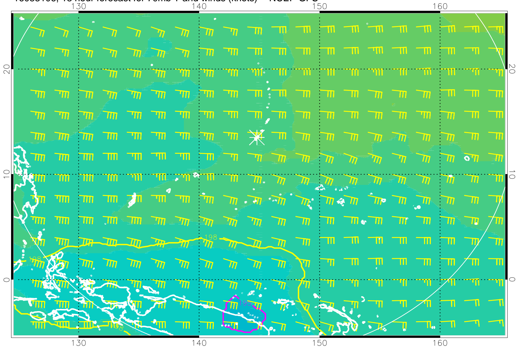
16083106, 18 hour forecast for 70mb T and winds (knots) -- NCEP GFS
