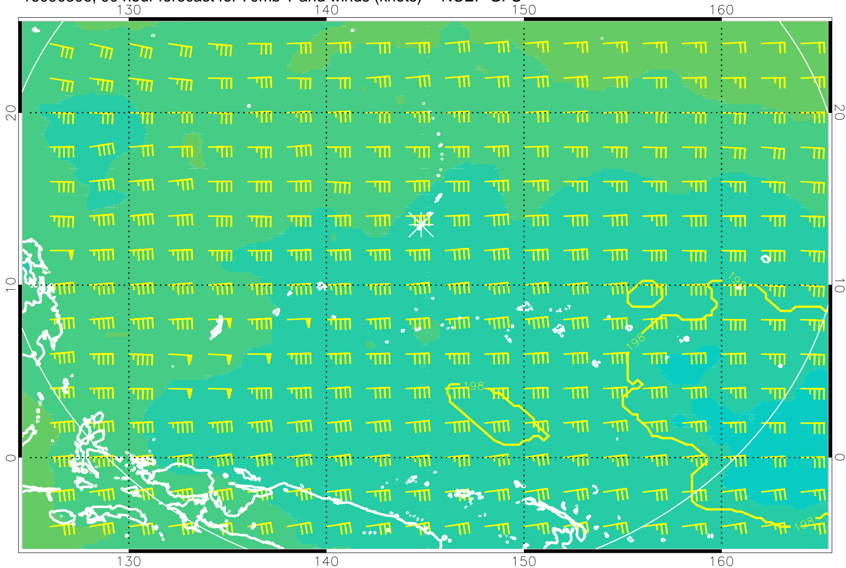
16090306, 90 hour forecast for 70mb T and winds (knots) -- NCEP GFS
