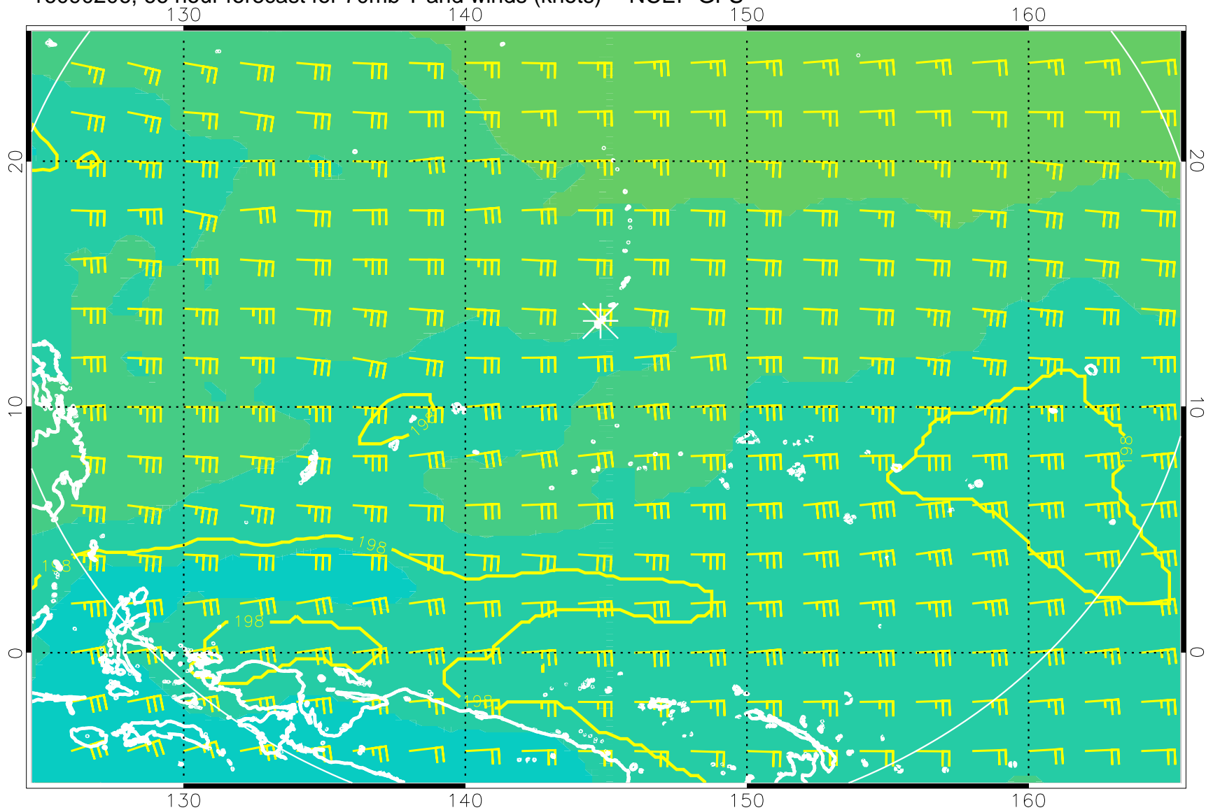
16090206, 66 hour forecast for 70mb T and winds (knots) -- NCEP GFS
