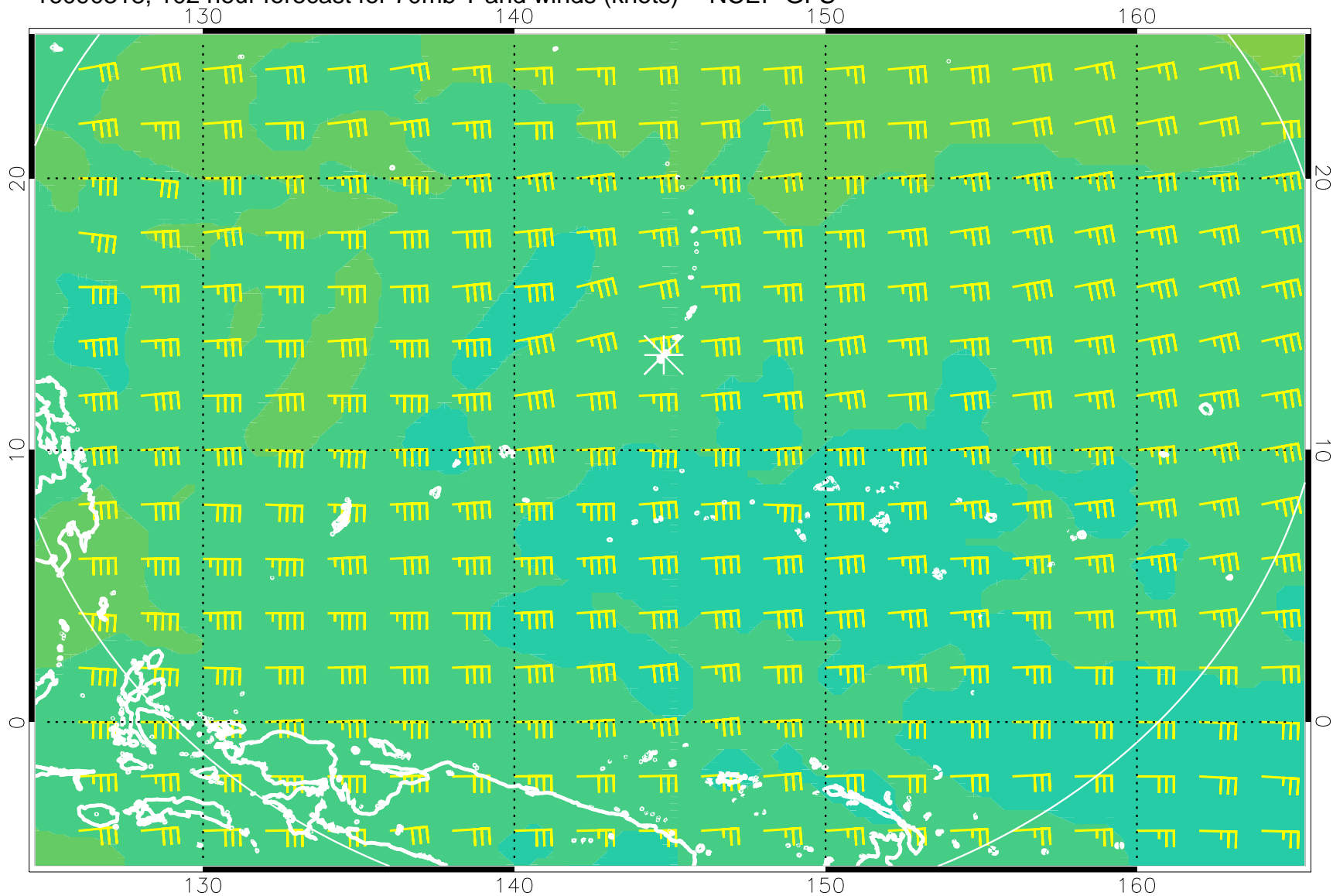
16090318, 102 hour forecast for 70mb T and winds (knots) -- NCEP GFS
