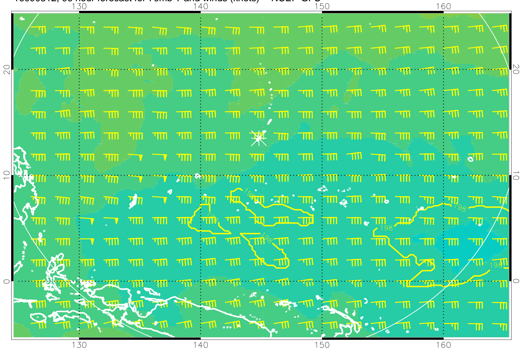
16090312, 96 hour forecast for 70mb T and winds (knots) -- NCEP GFS
