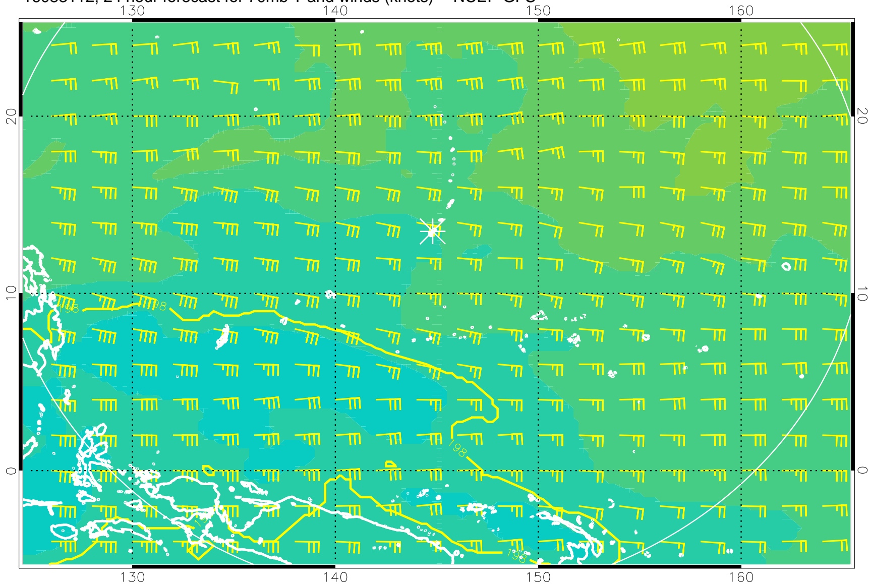
16083112, 24 hour forecast for 70mb T and winds (knots) -- NCEP GFS
