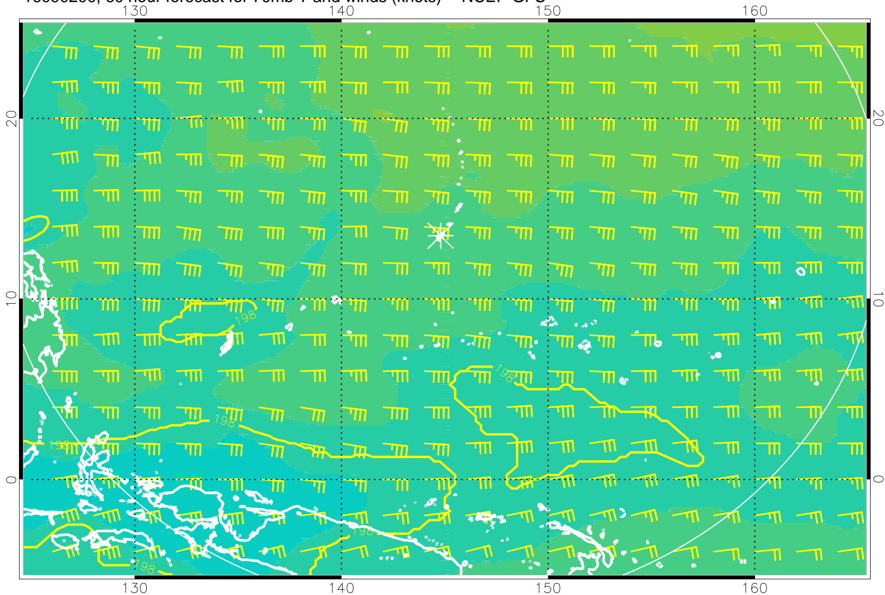
16090200, 60 hour forecast for 70mb T and winds (knots) -- NCEP GFS
