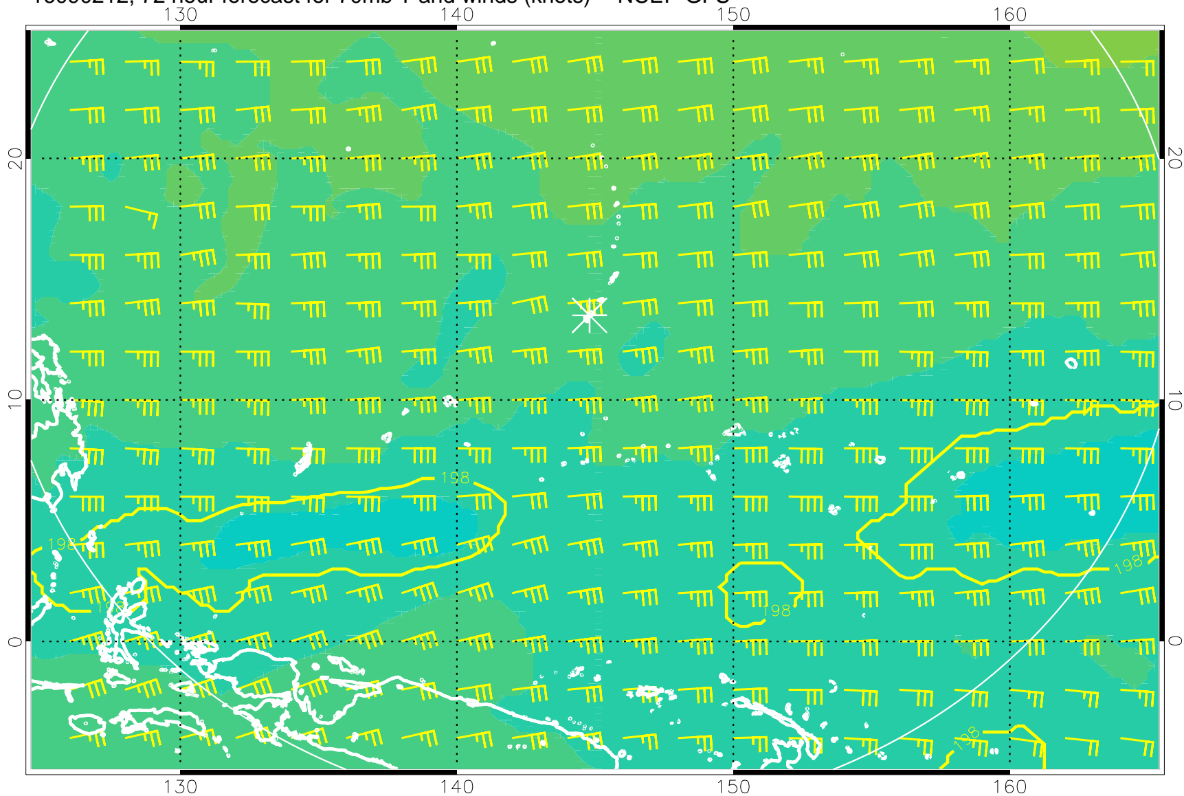
16090212, 72 hour forecast for 70mb T and winds (knots) -- NCEP GFS
