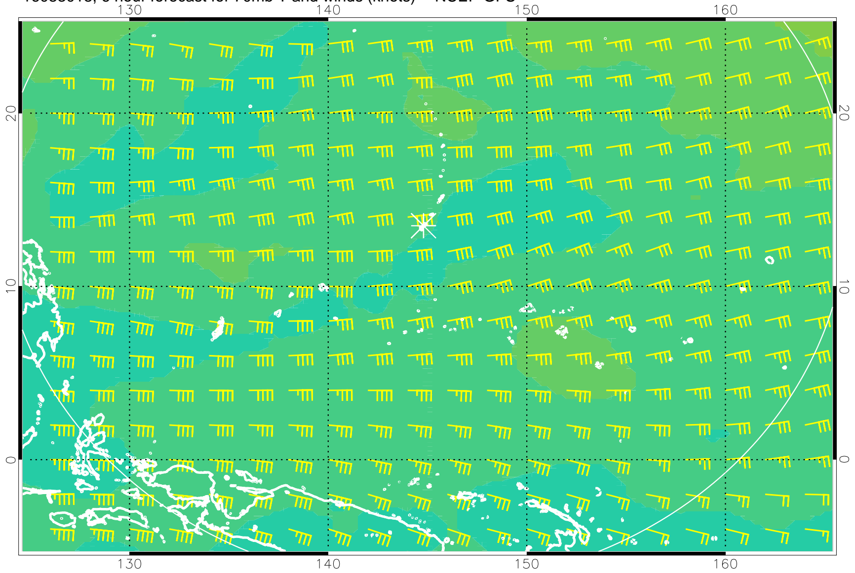
16083018, 6 hour forecast for 70mb T and winds (knots) -- NCEP GFS
