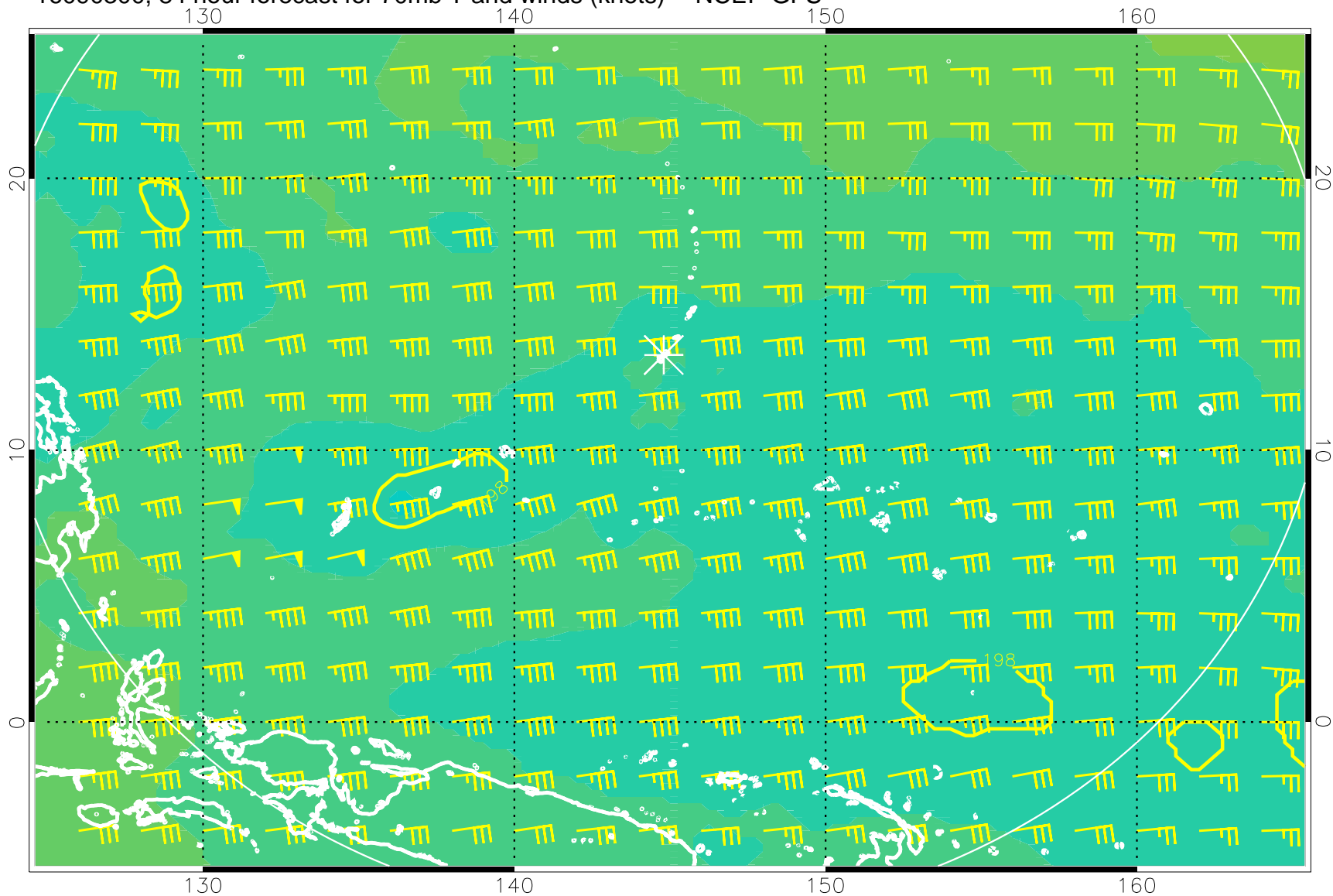
16090300, 84 hour forecast for 70mb T and winds (knots) -- NCEP GFS
