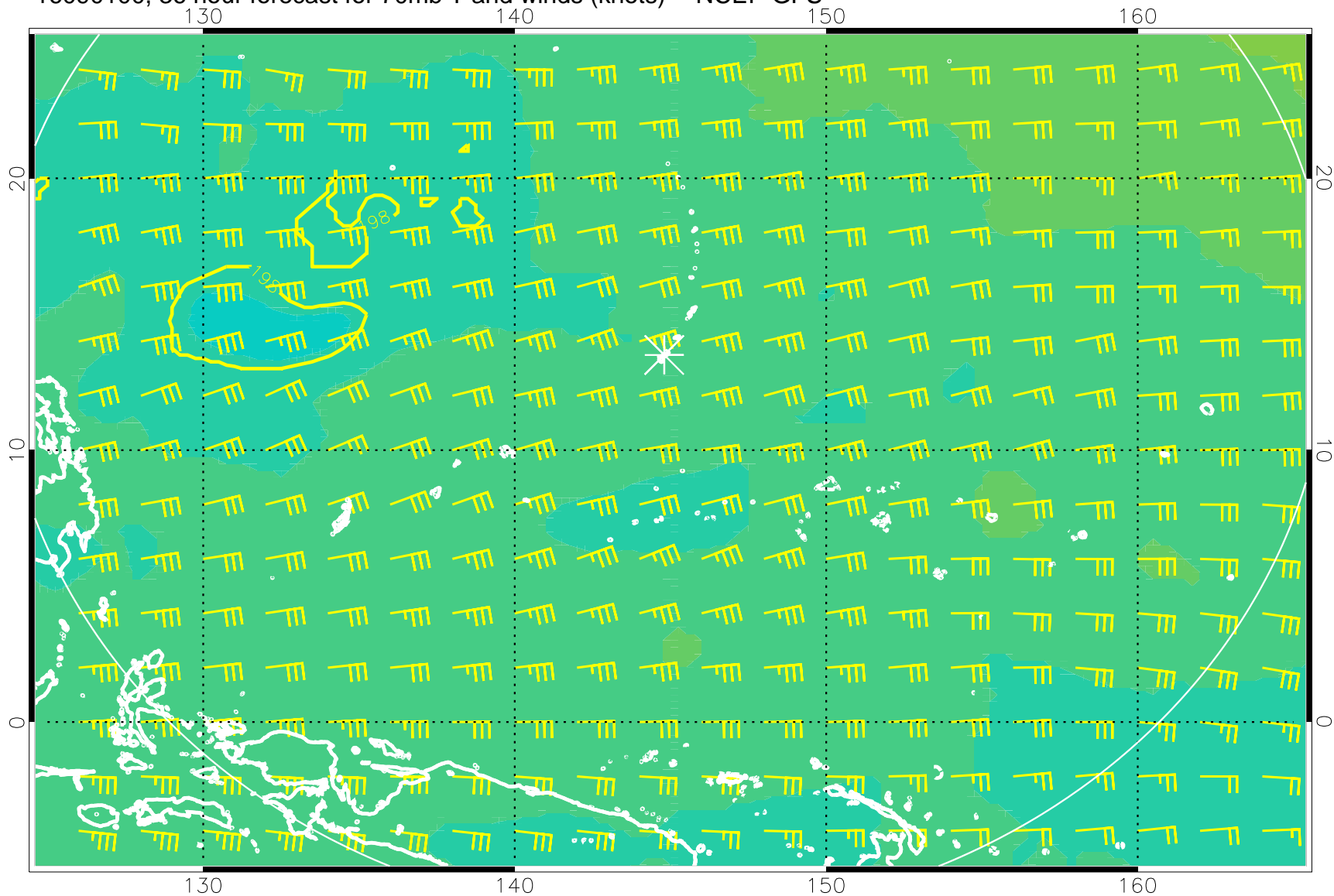
16090100, 36 hour forecast for 70mb T and winds (knots) -- NCEP GFS
