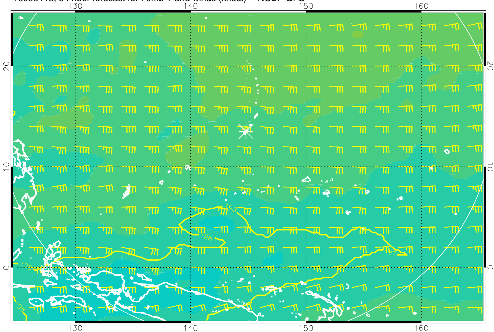
16090118, 54 hour forecast for 70mb T and winds (knots) -- NCEP GFS
