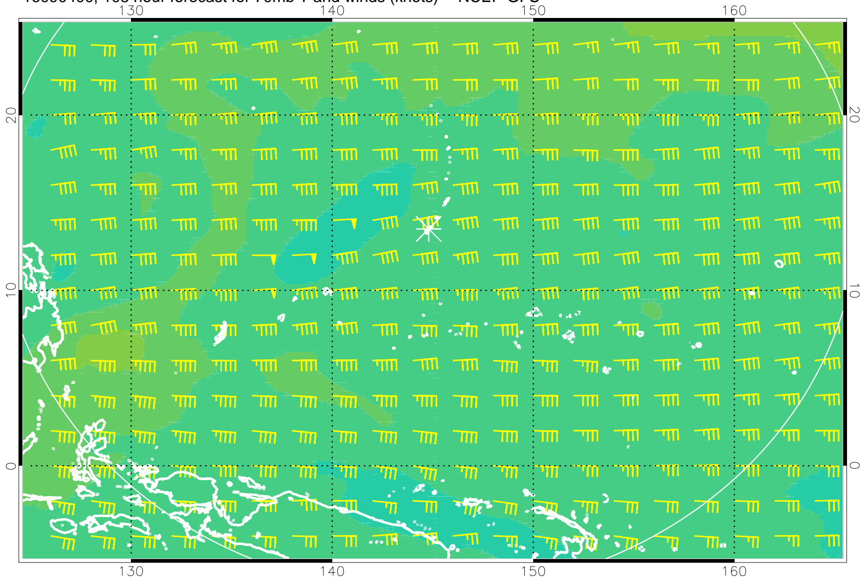
16090400, 108 hour forecast for 70mb T and winds (knots) -- NCEP GFS
