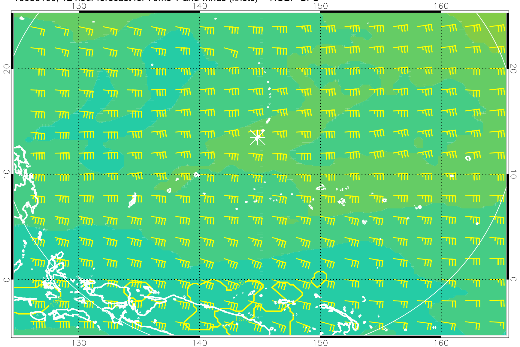
16083100, 12 hour forecast for 70mb T and winds (knots) -- NCEP GFS
