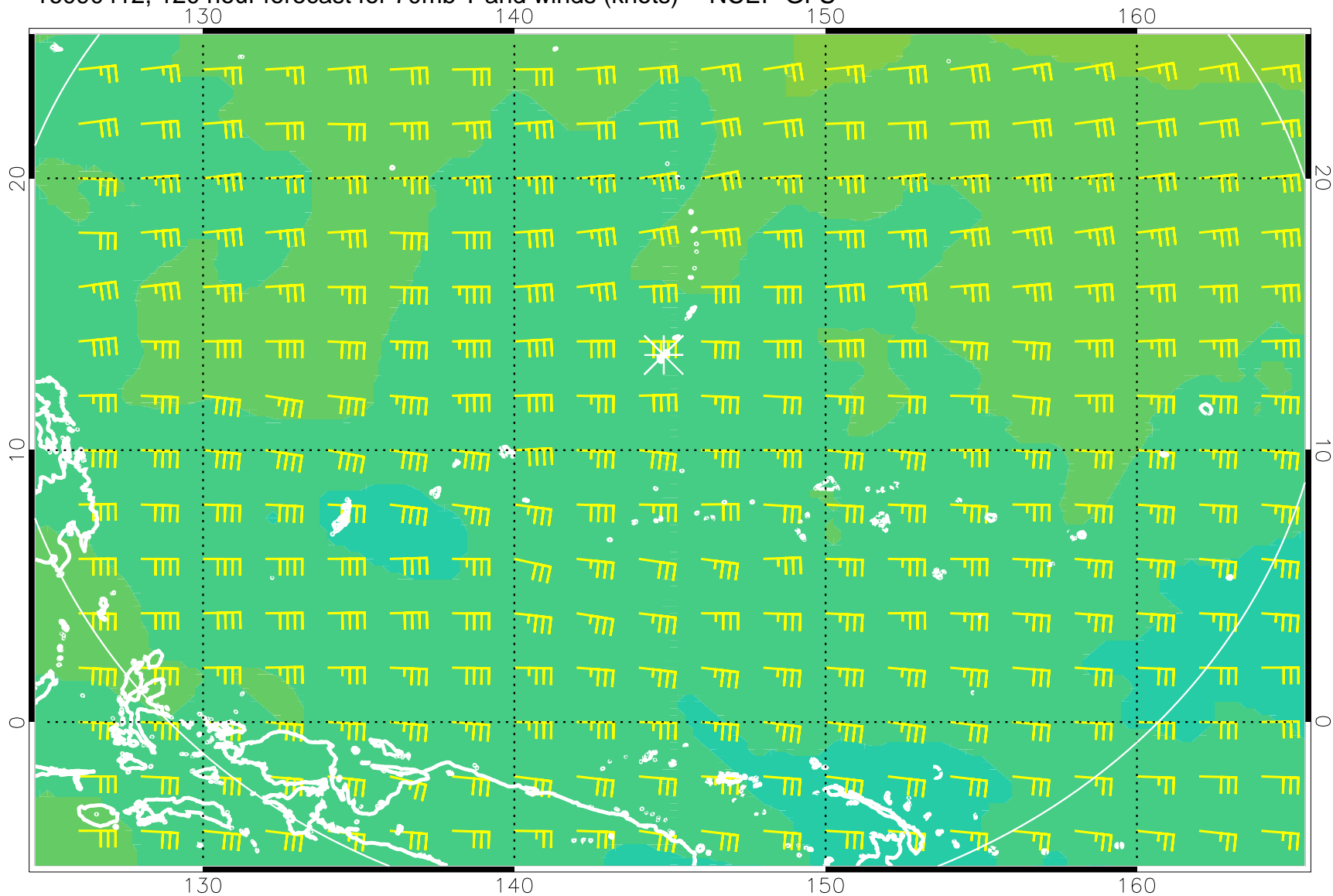
16090412, 120 hour forecast for 70mb T and winds (knots) -- NCEP GFS
