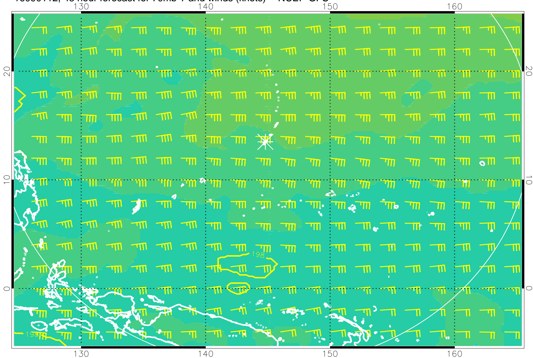
16090112, 48 hour forecast for 70mb T and winds (knots) -- NCEP GFS
