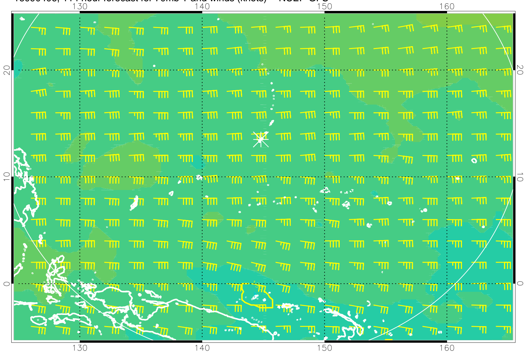
16090406, 114 hour forecast for 70mb T and winds (knots) -- NCEP GFS
