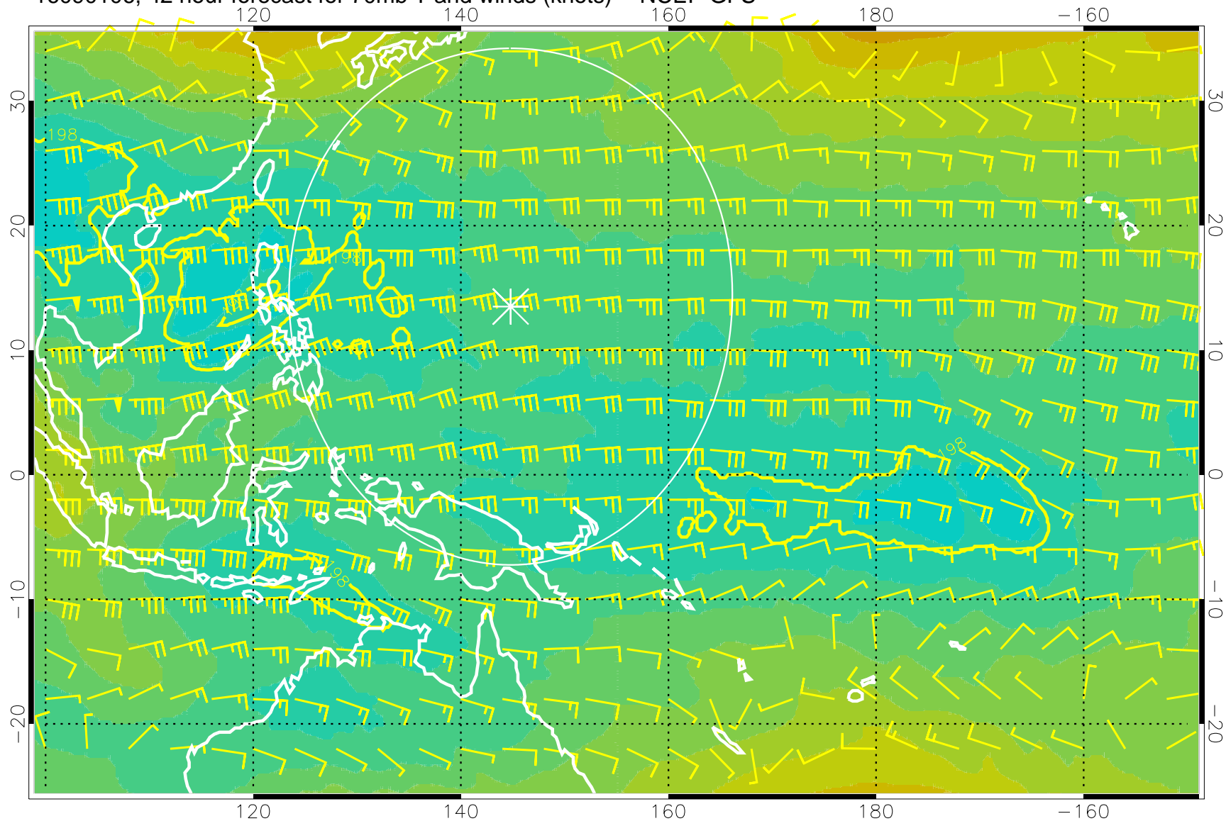
16090106, 42 hour forecast for 70mb T and winds (knots) -- NCEP GFS
