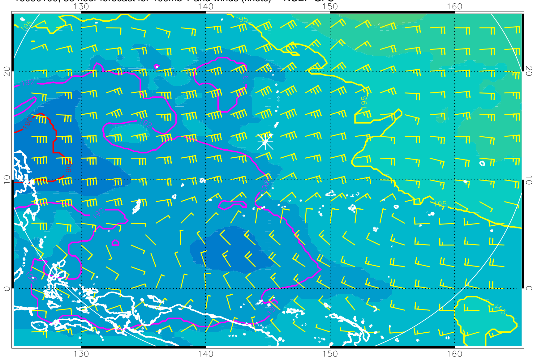
16090100, 36 hour forecast for 100mb T and winds (knots) -- NCEP GFS
