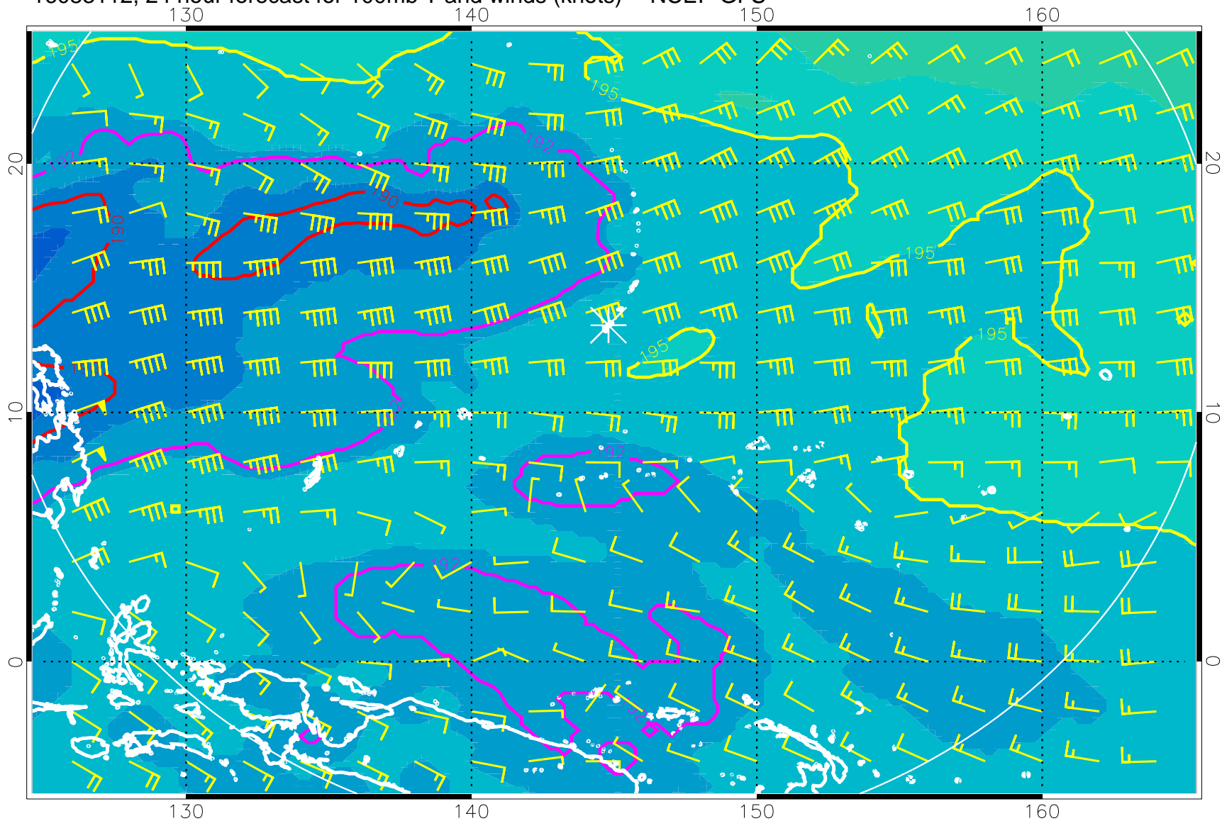
16083112, 24 hour forecast for 100mb T and winds (knots) -- NCEP GFS
