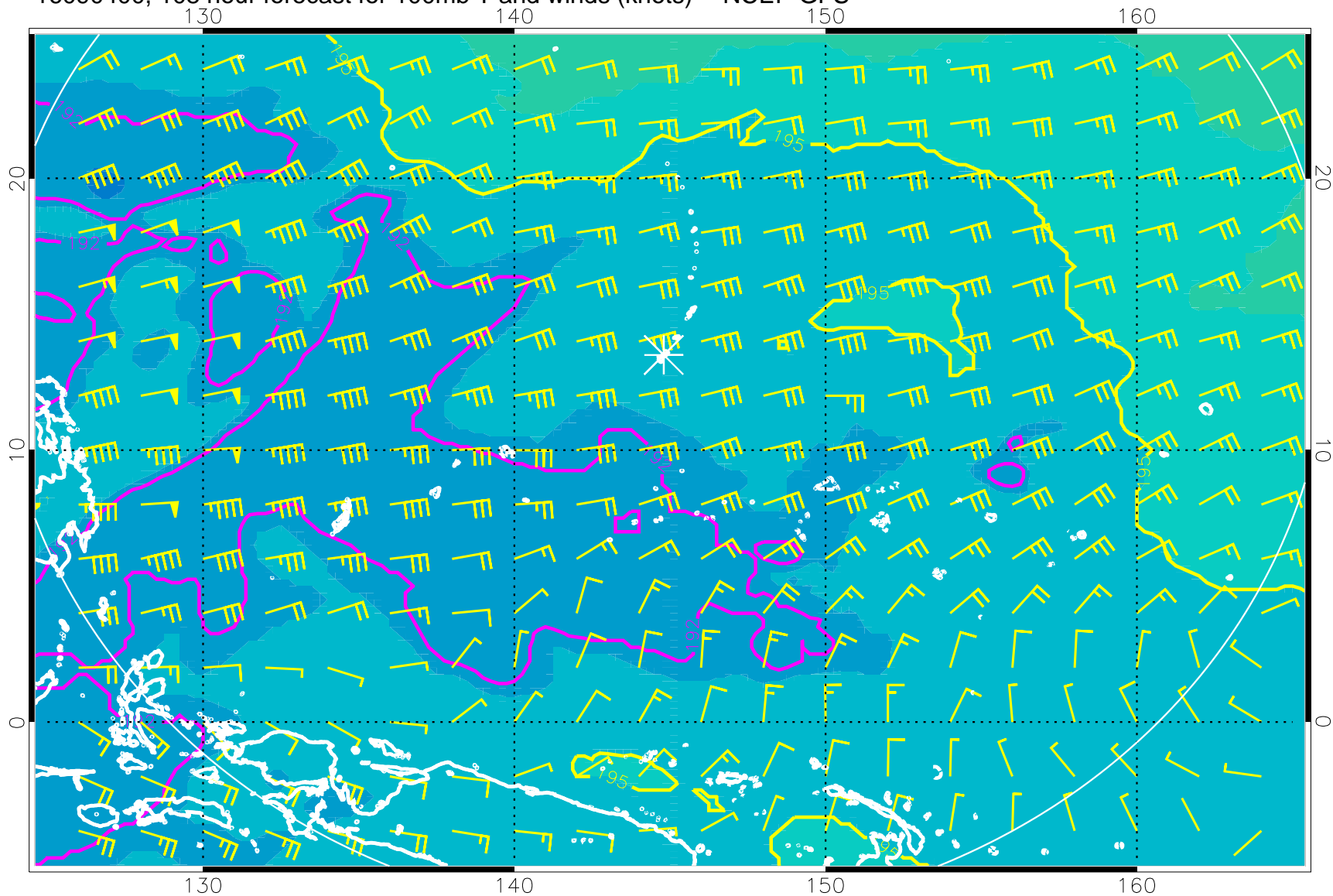
16090400, 108 hour forecast for 100mb T and winds (knots) -- NCEP GFS
