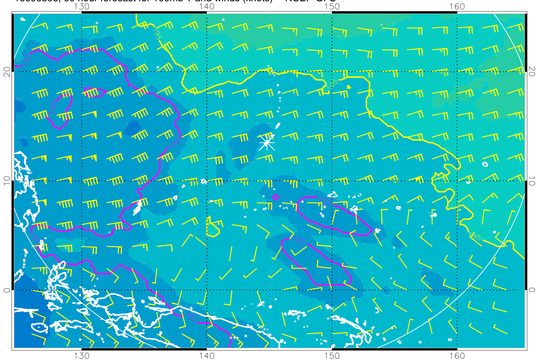
16090306, 90 hour forecast for 100mb T and winds (knots) -- NCEP GFS
