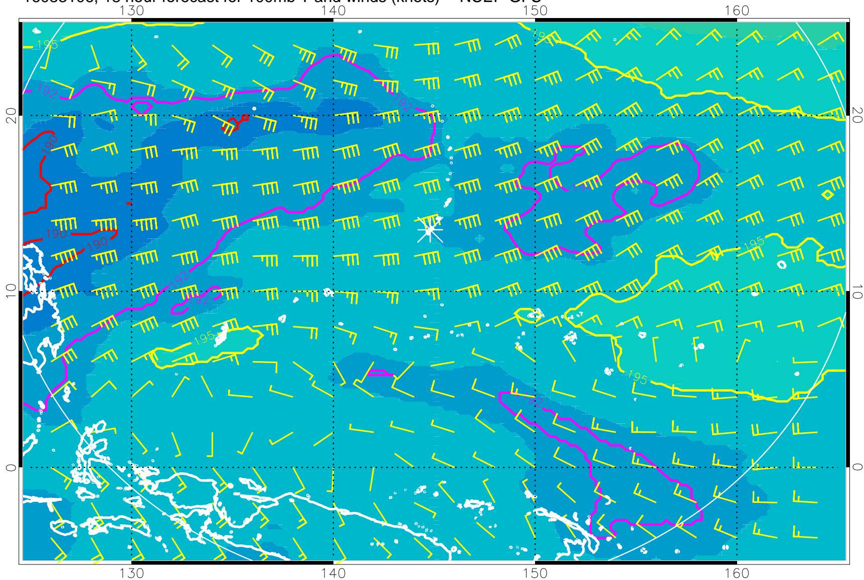
16083106, 18 hour forecast for 100mb T and winds (knots) -- NCEP GFS
