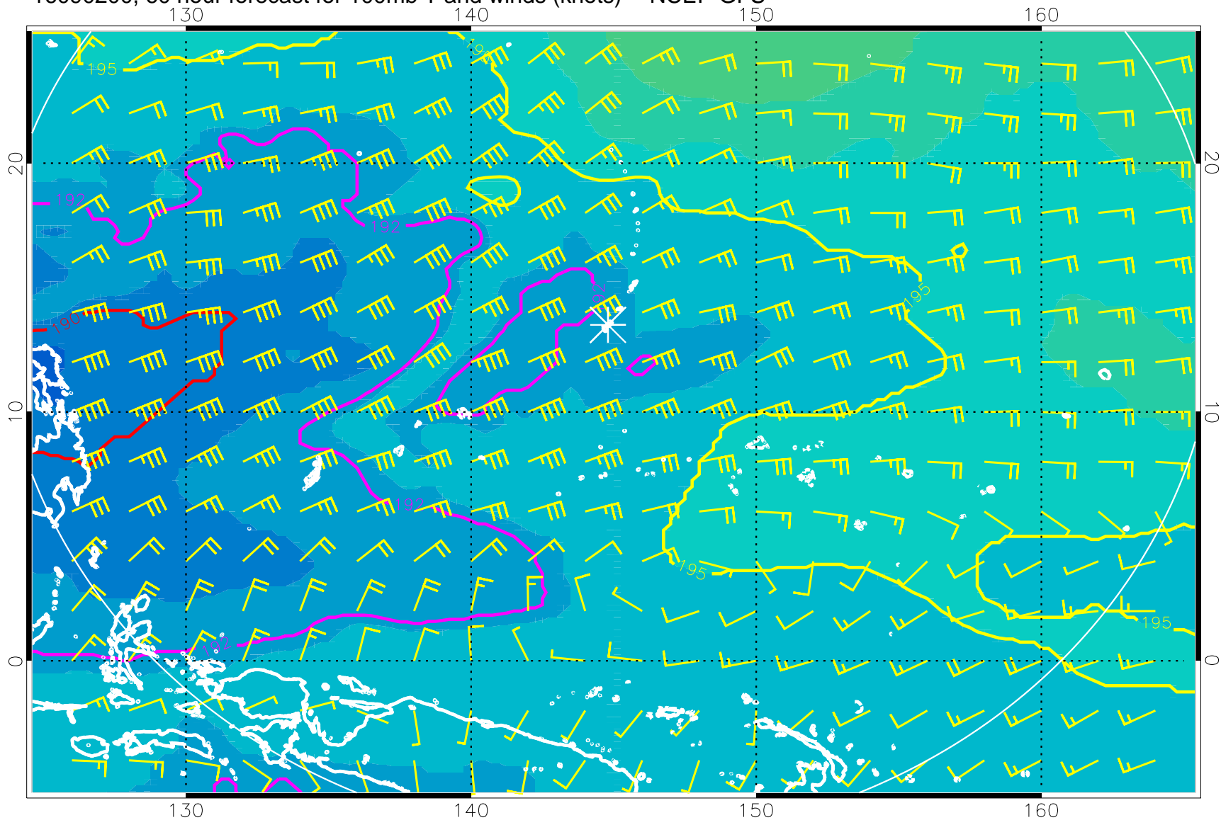
16090200, 60 hour forecast for 100mb T and winds (knots) -- NCEP GFS
