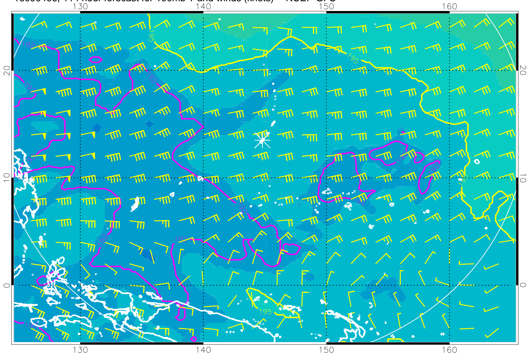
16090406, 114 hour forecast for 100mb T and winds (knots) -- NCEP GFS
