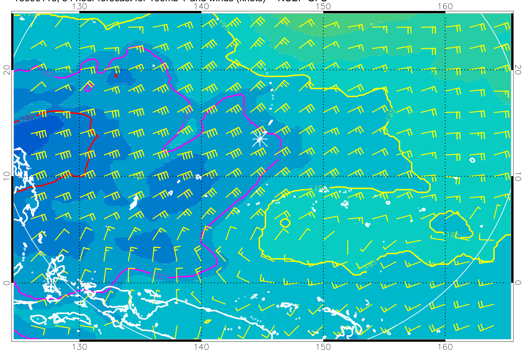
16090118, 54 hour forecast for 100mb T and winds (knots) -- NCEP GFS
