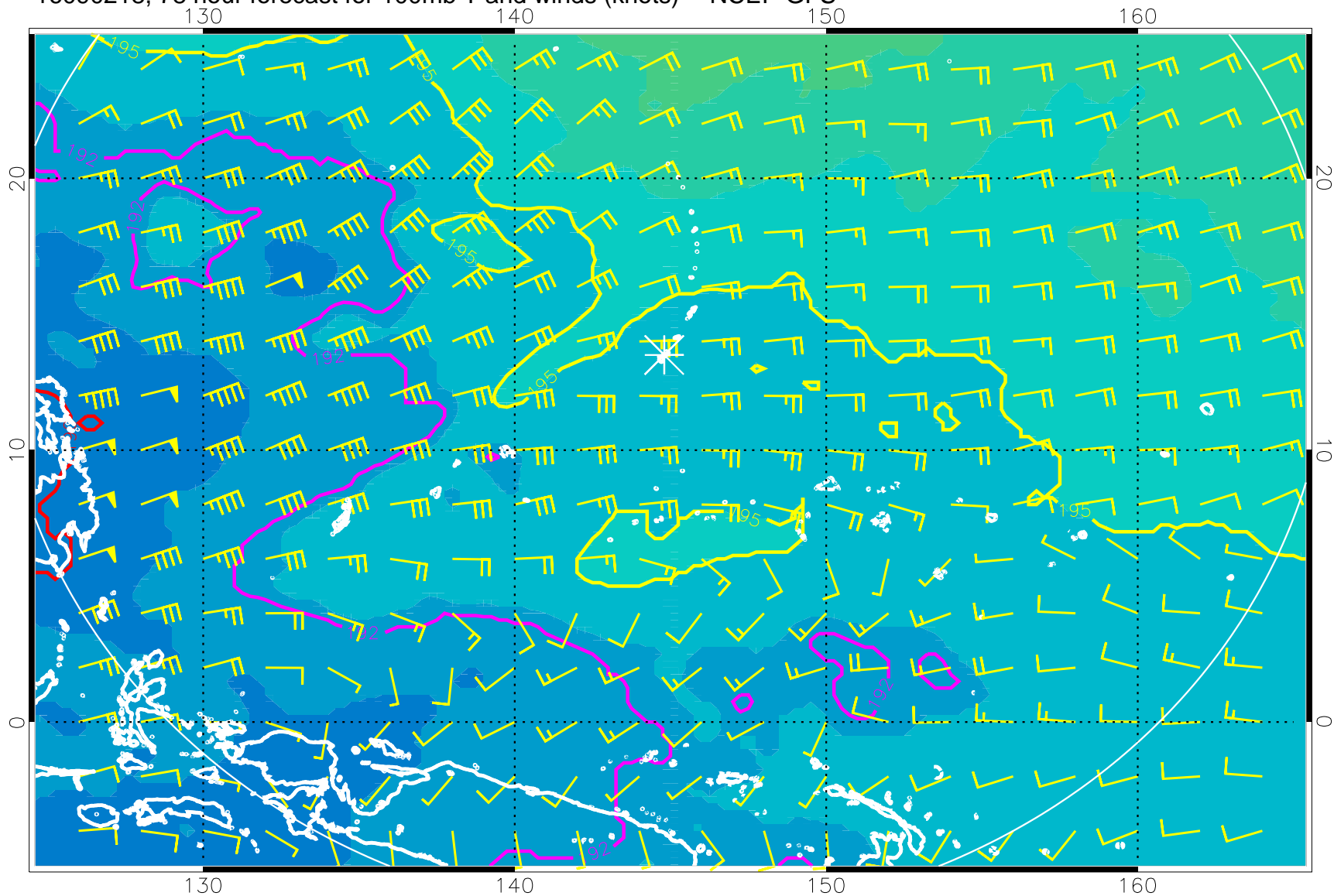
16090218, 78 hour forecast for 100mb T and winds (knots) -- NCEP GFS
