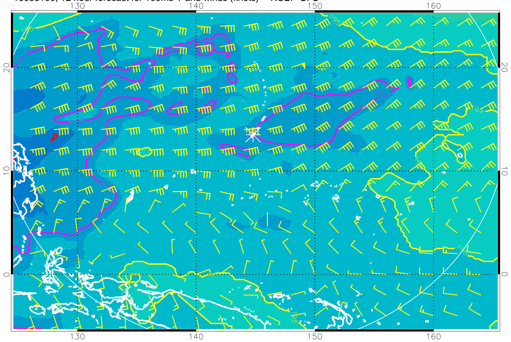
16083100, 12 hour forecast for 100mb T and winds (knots) -- NCEP GFS
