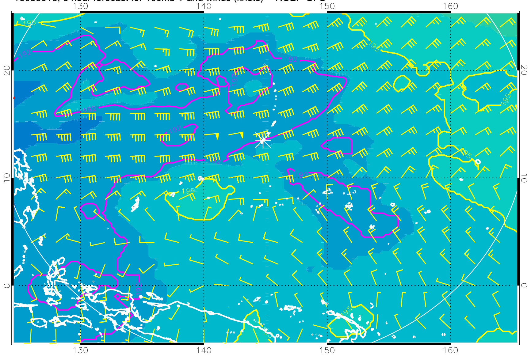
16083018, 6 hour forecast for 100mb T and winds (knots) -- NCEP GFS
