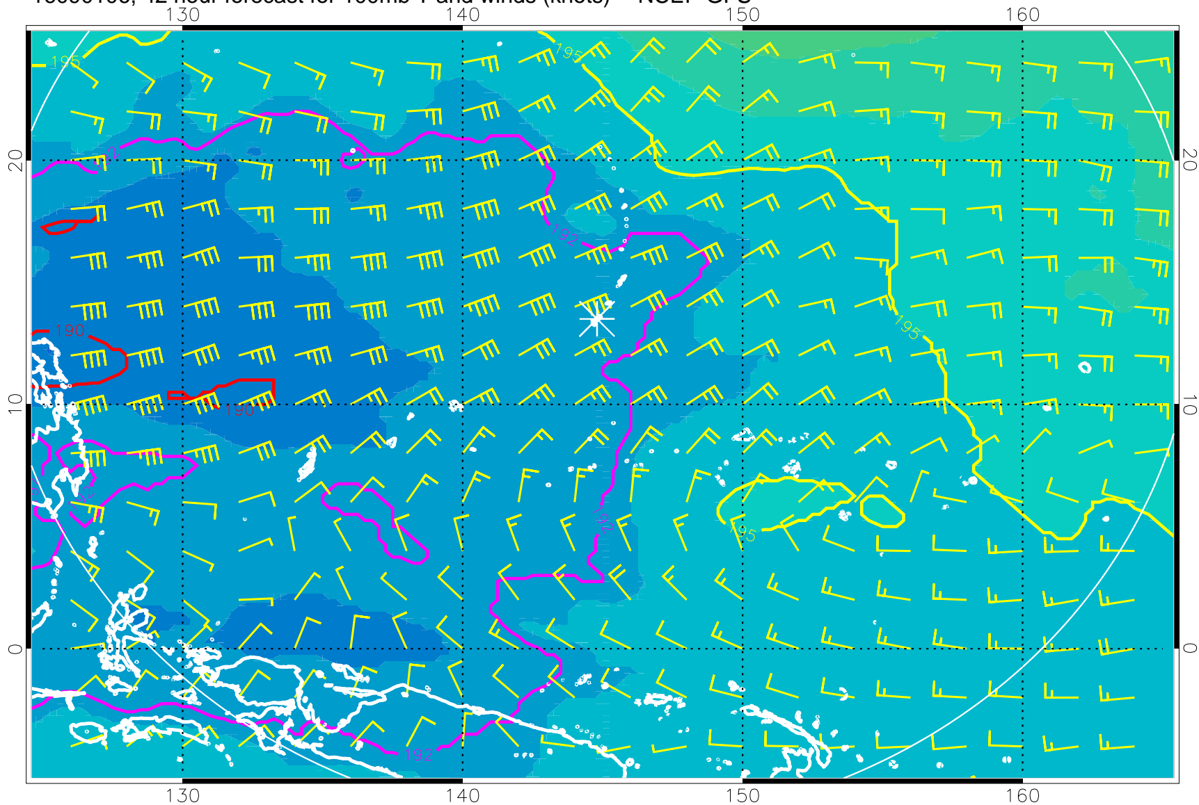
16090106, 42 hour forecast for 100mb T and winds (knots) -- NCEP GFS
