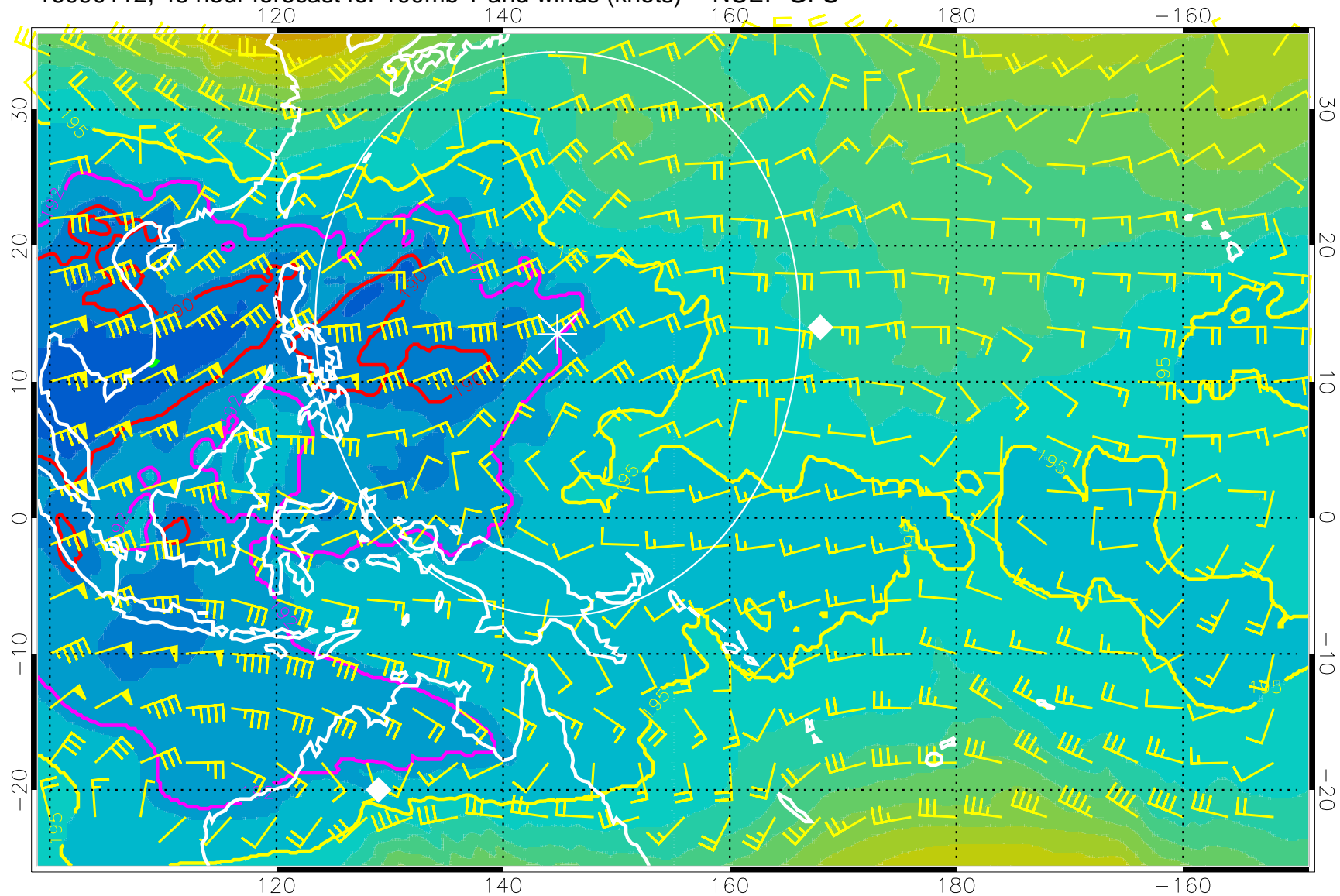
16090112, 48 hour forecast for 100mb T and winds (knots) -- NCEP GFS
