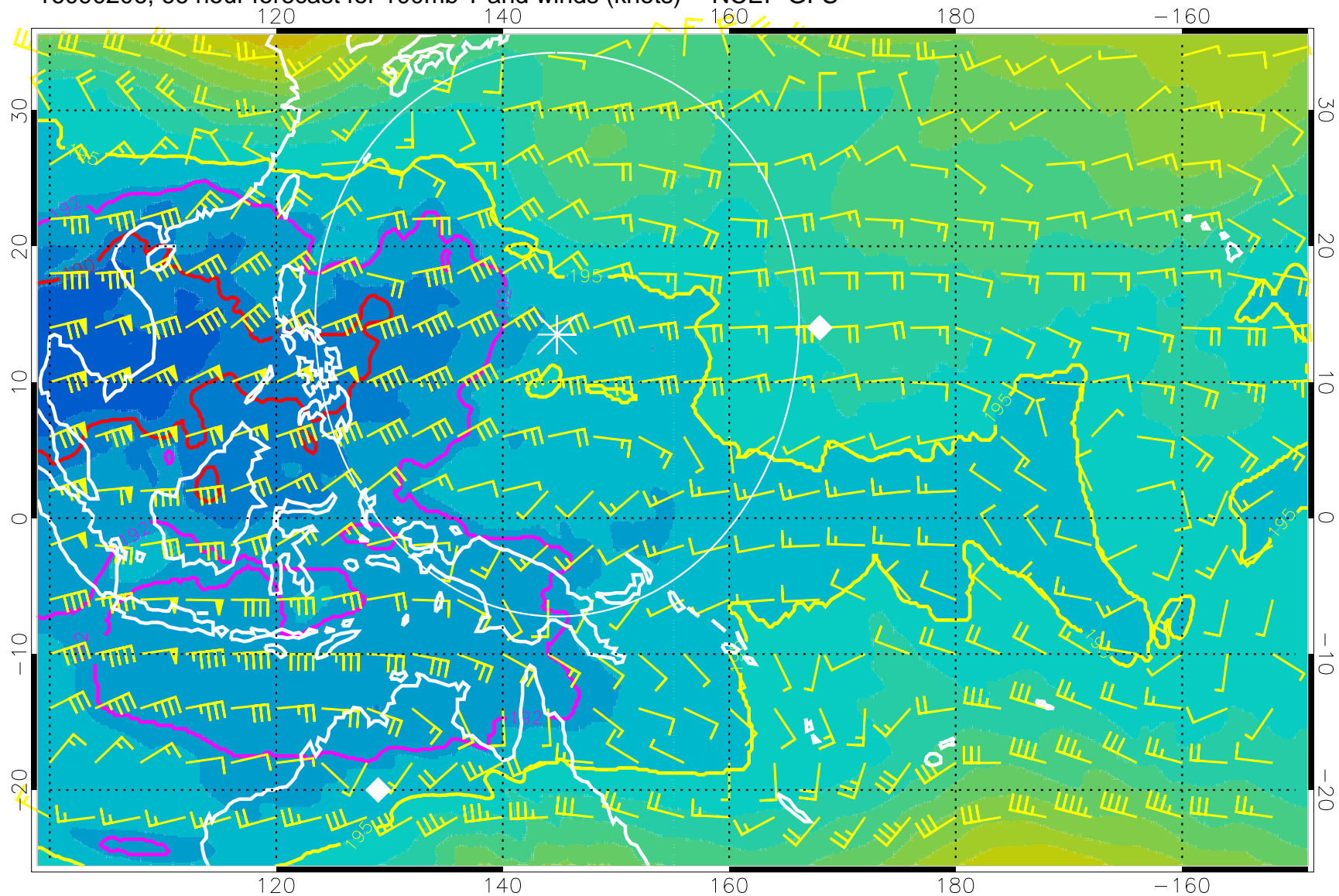
16090206, 66 hour forecast for 100mb T and winds (knots) -- NCEP GFS
