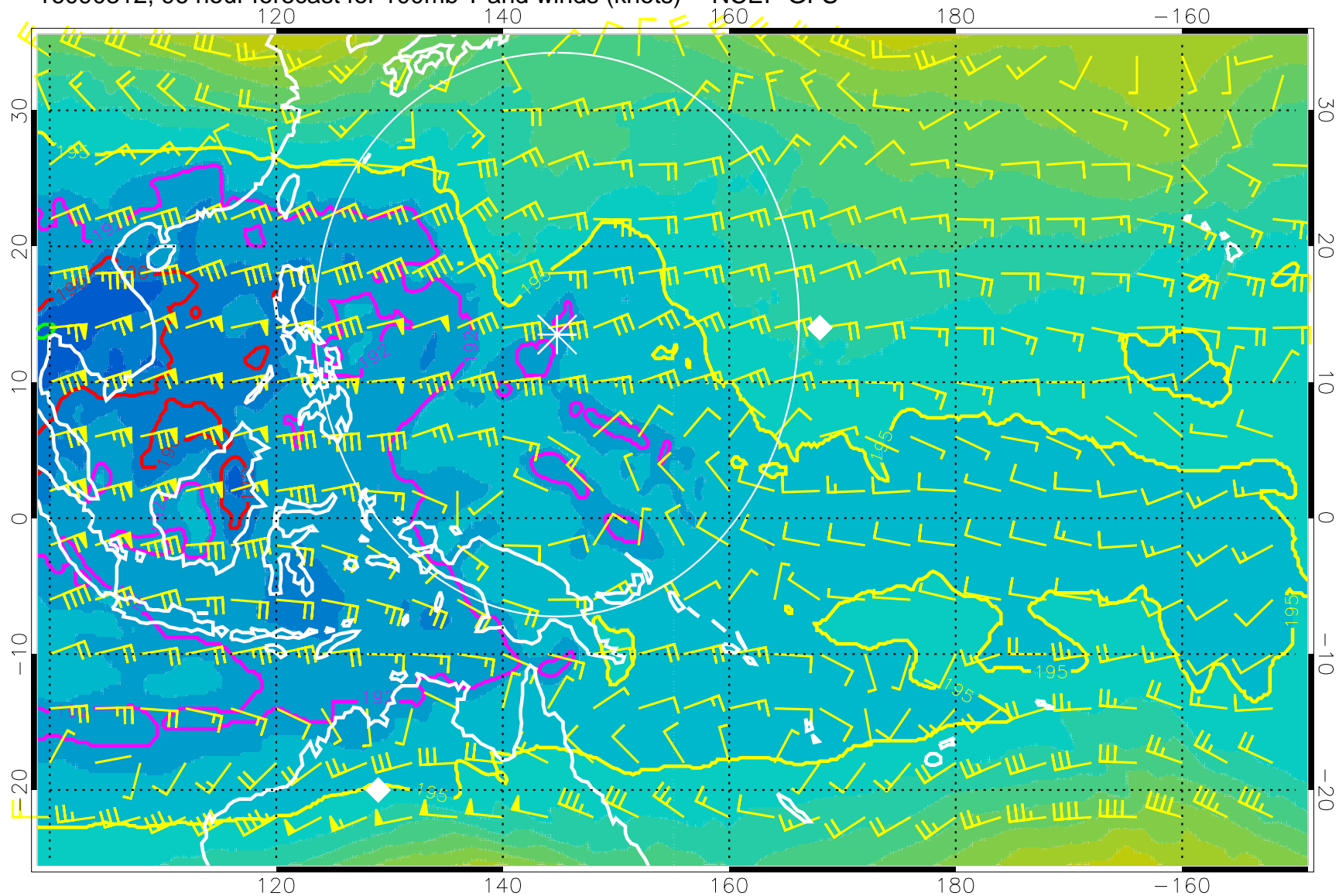
16090312, 96 hour forecast for 100mb T and winds (knots) -- NCEP GFS
