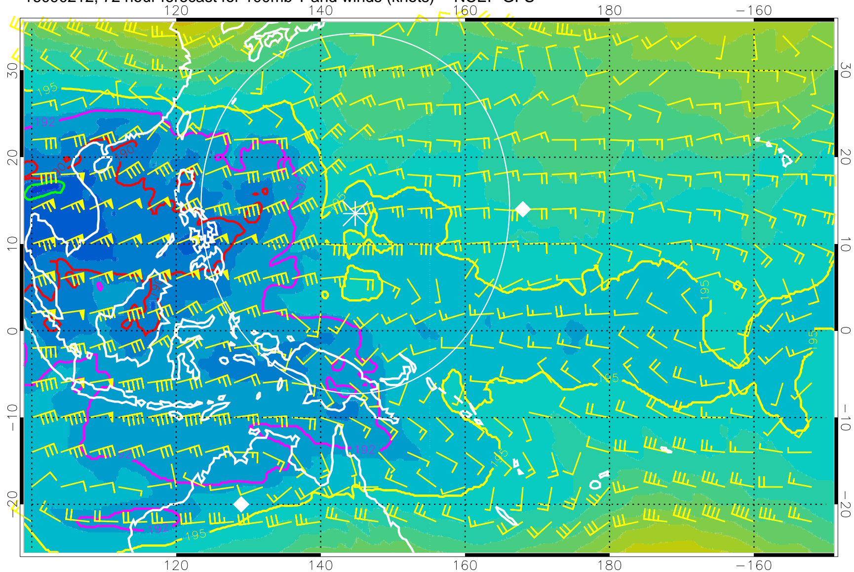
16090212, 72 hour forecast for 100mb T and winds (knots) -- NCEP GFS
