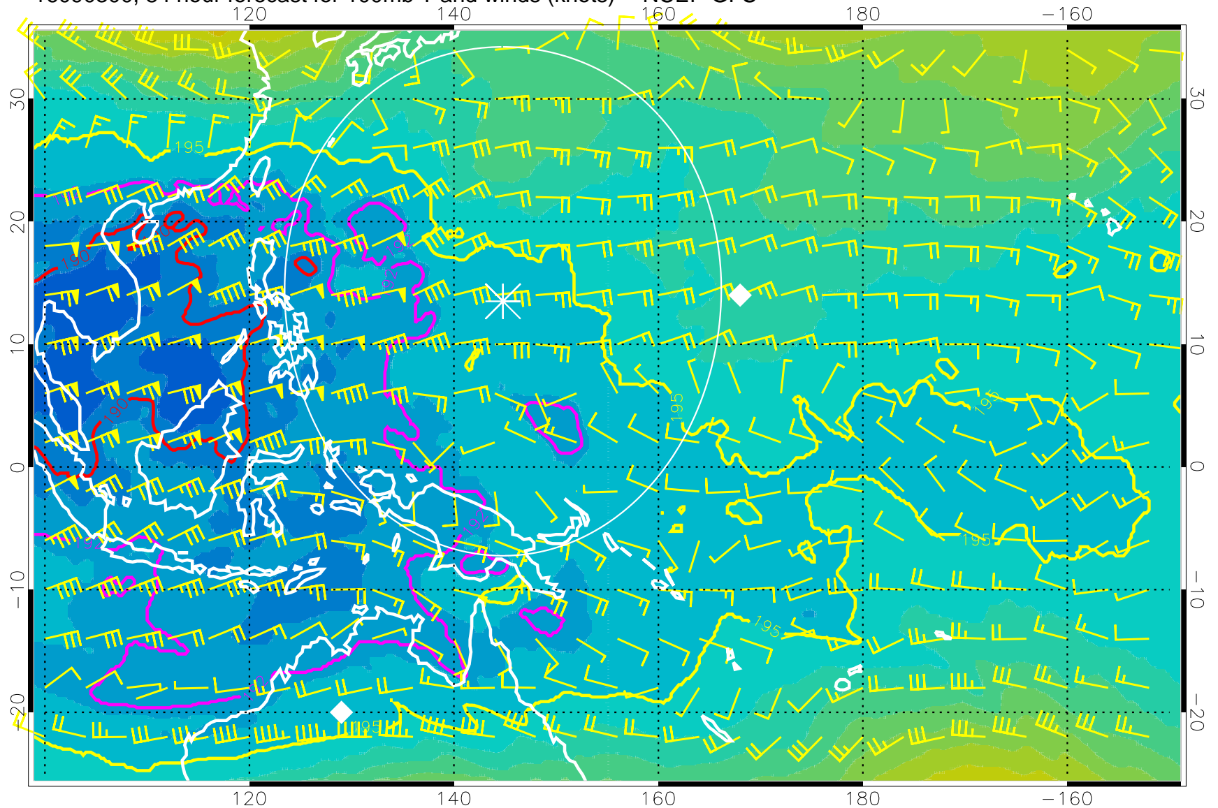
16090300, 84 hour forecast for 100mb T and winds (knots) -- NCEP GFS
