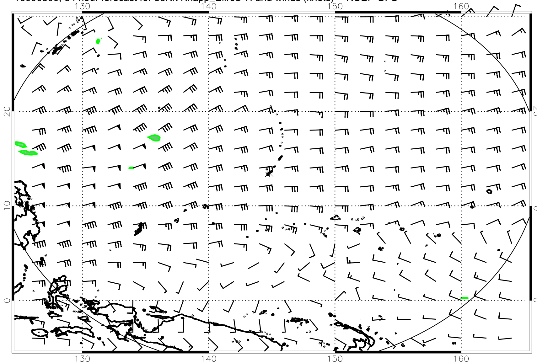
16090300, 84 hour forecast for 53Kft Knapp_Ellrod TI and winds (knots) -- NCEP GFS
