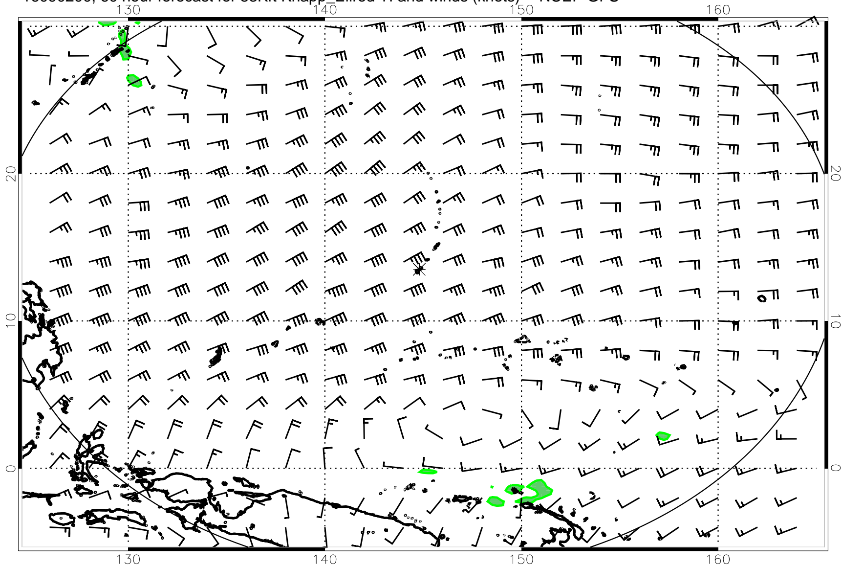
16090200, 60 hour forecast for 53Kft Knapp_Ellrod TI and winds (knots) -- NCEP GFS
