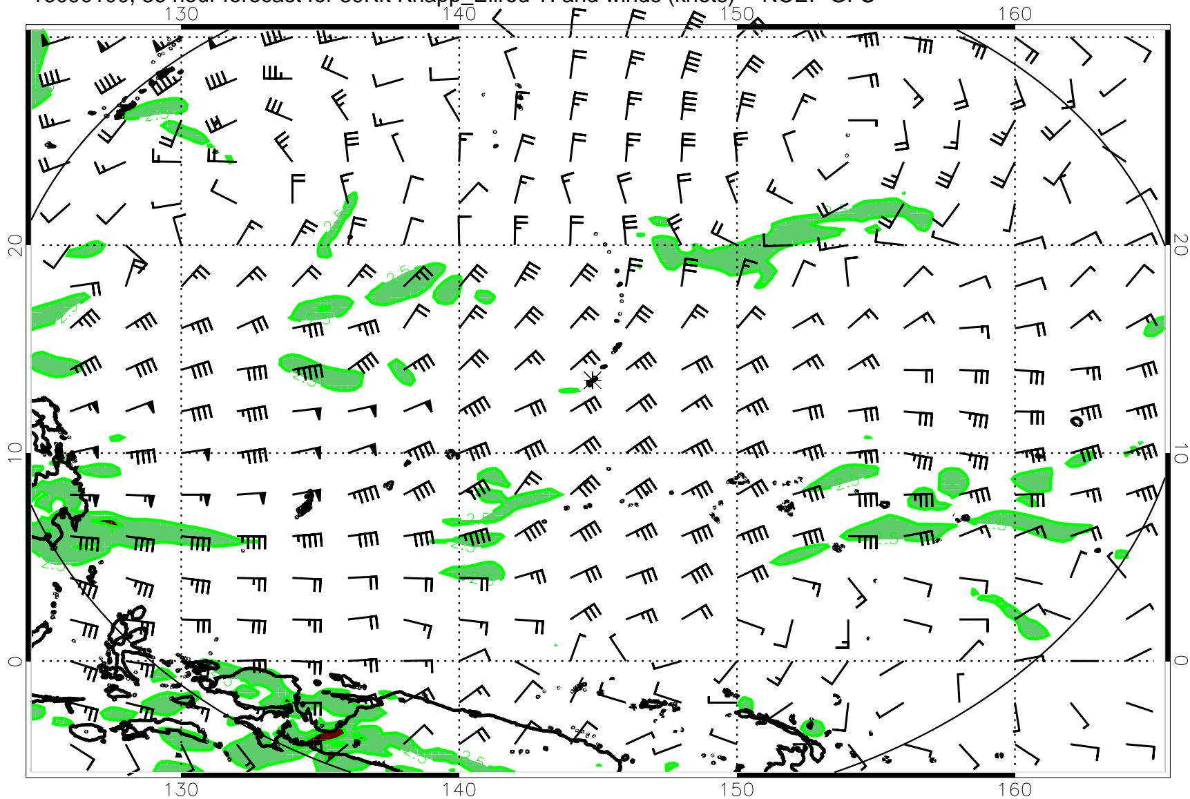
16090100, 36 hour forecast for 39Kft Knapp_Ellrod TI and winds (knots) -- NCEP GFS
