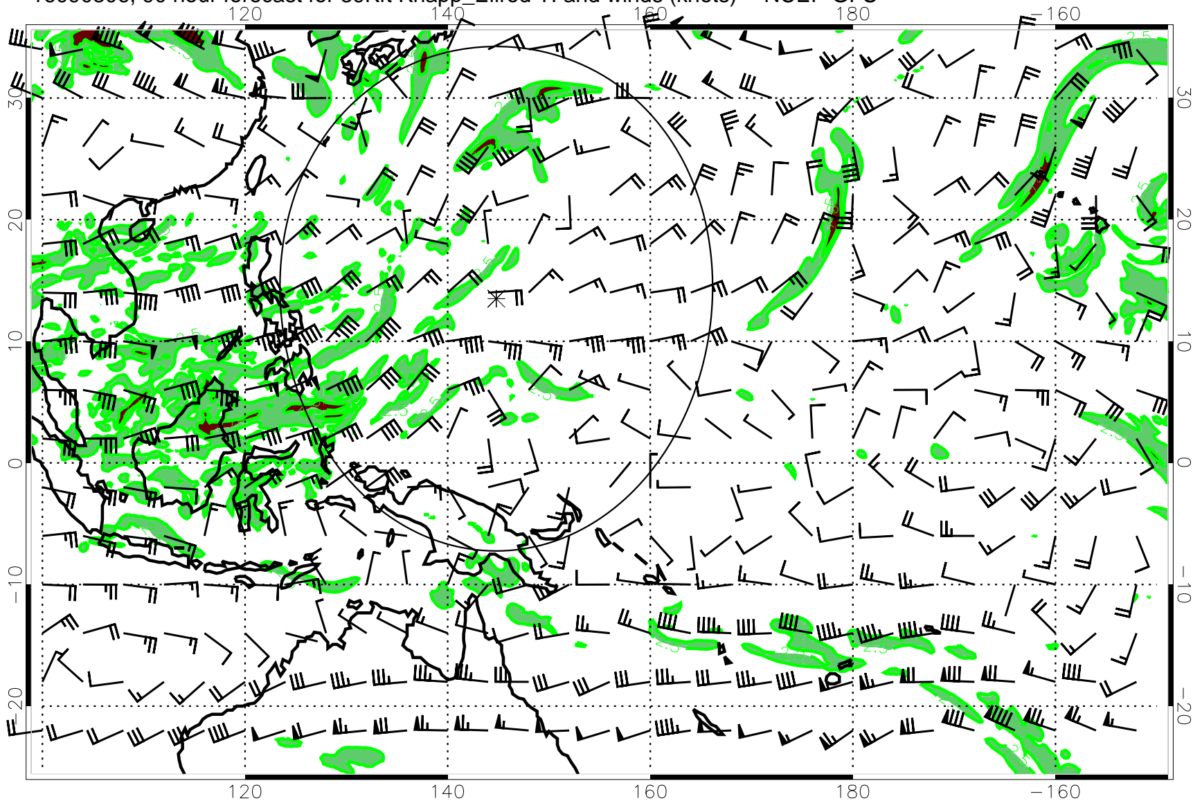
16090306, 90 hour forecast for 39Kft Knapp_Ellrod TI and winds (knots) -- NCEP GFS
