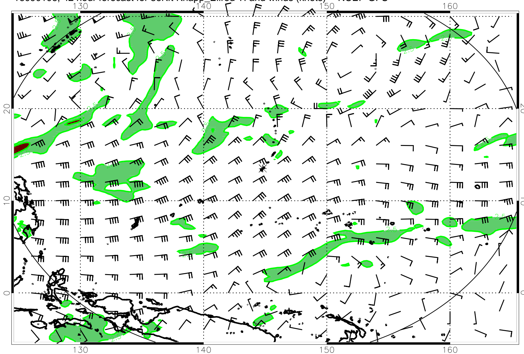
16090106, 42 hour forecast for 36Kft Knapp_Ellrod TI and winds (knots) -- NCEP GFS
