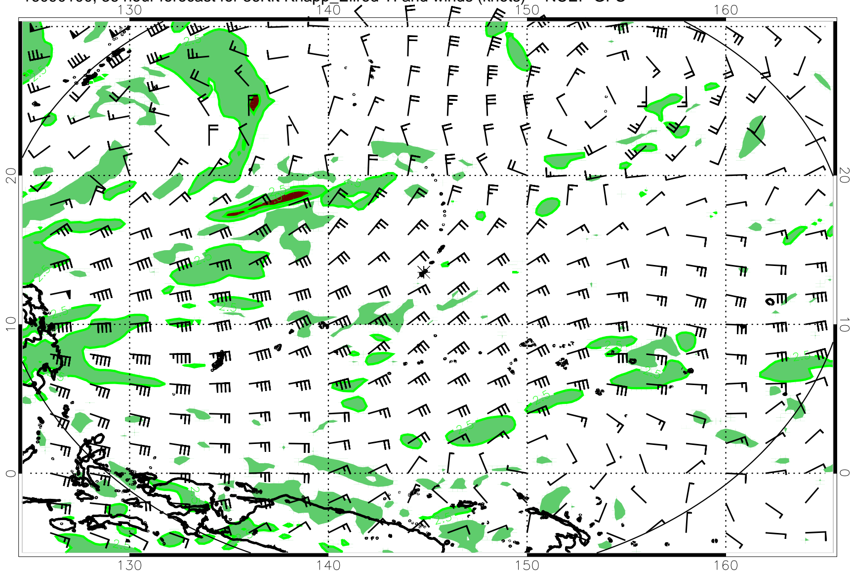
16090100, 36 hour forecast for 36Kft Knapp_Ellrod TI and winds (knots) -- NCEP GFS
