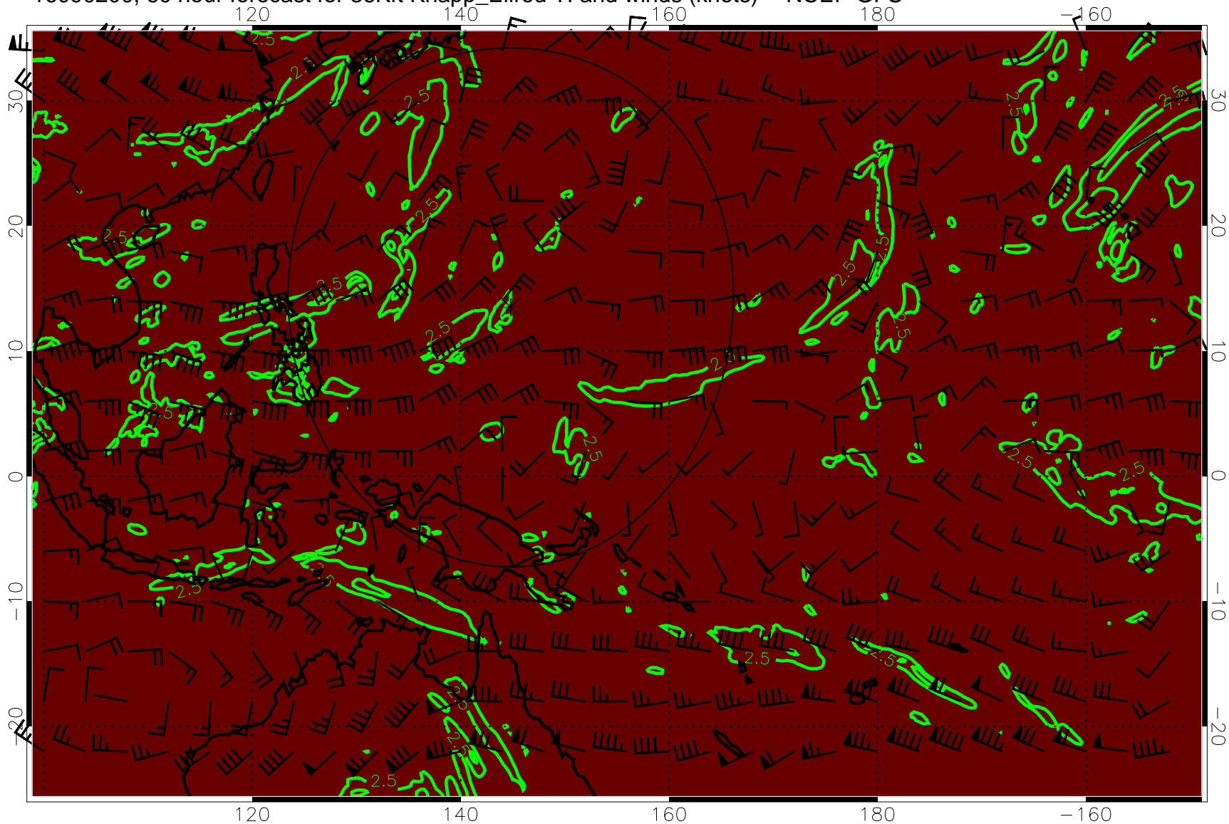
16090200, 60 hour forecast for 36Kft Knapp_Ellrod TI and winds (knots) -- NCEP GFS
