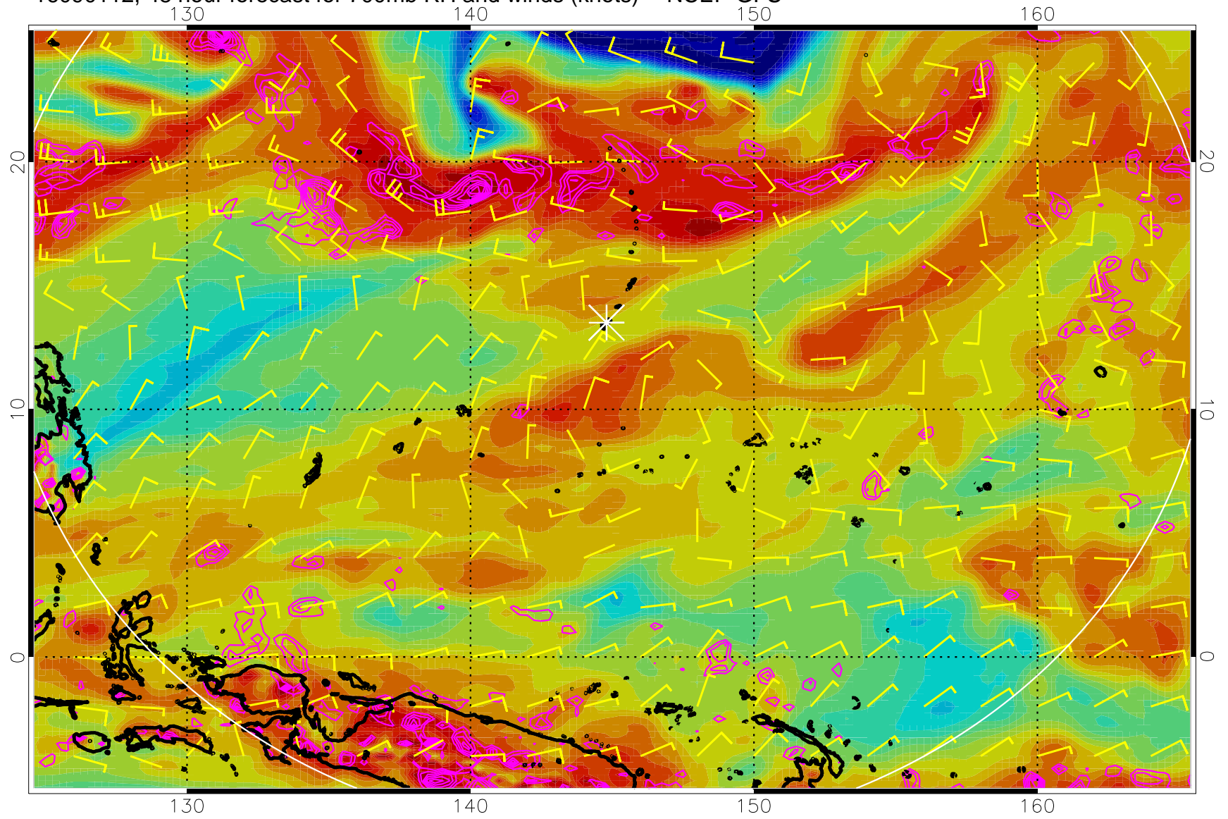
16090112, 48 hour forecast for 700mb RH and winds (knots) -- NCEP GFS
