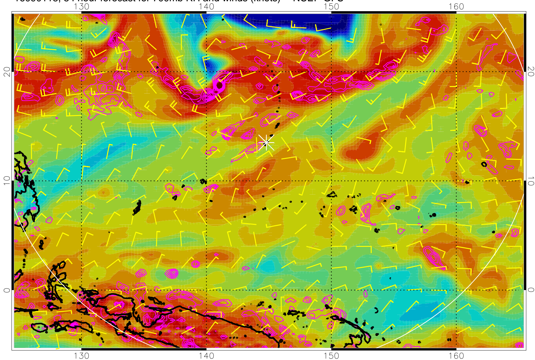
16090118, 54 hour forecast for 700mb RH and winds (knots) -- NCEP GFS
