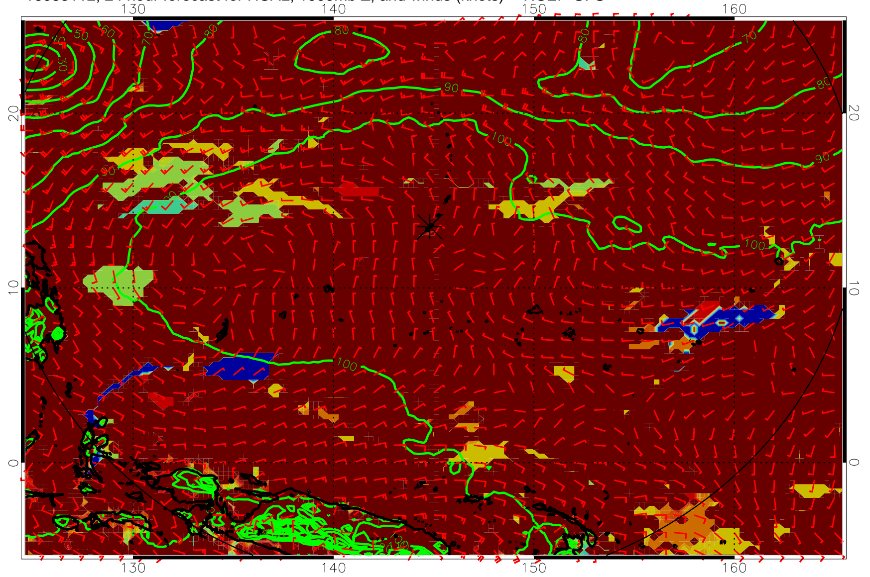
16083112, 24 hour forecast for HCAL, 1000mb Z, and winds (knots) -- NCEP GFS
