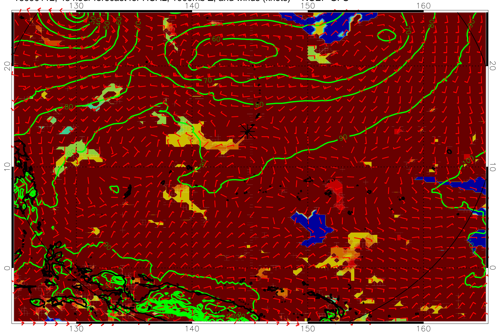
16090112, 48 hour forecast for HCAL, 1000mb Z, and winds (knots) -- NCEP GFS
