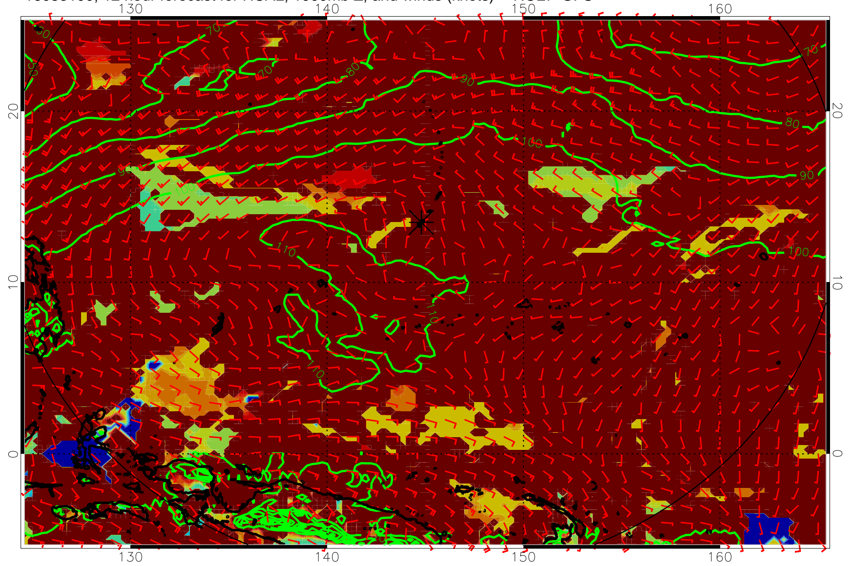
16083100, 12 hour forecast for HCAL, 1000mb Z, and winds (knots) -- NCEP GFS
