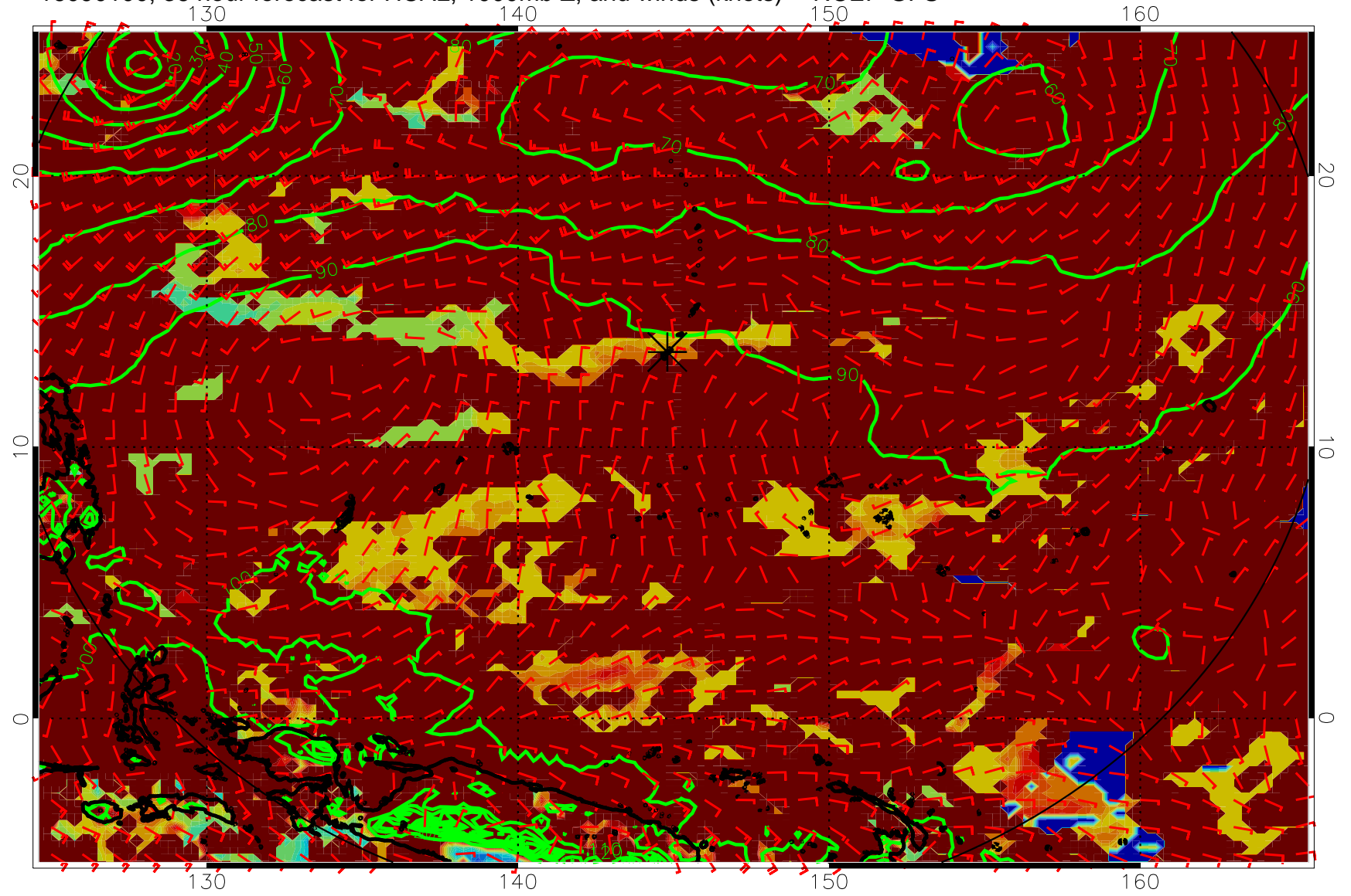
16090100, 36 hour forecast for HCAL, 1000mb Z, and winds (knots) -- NCEP GFS
