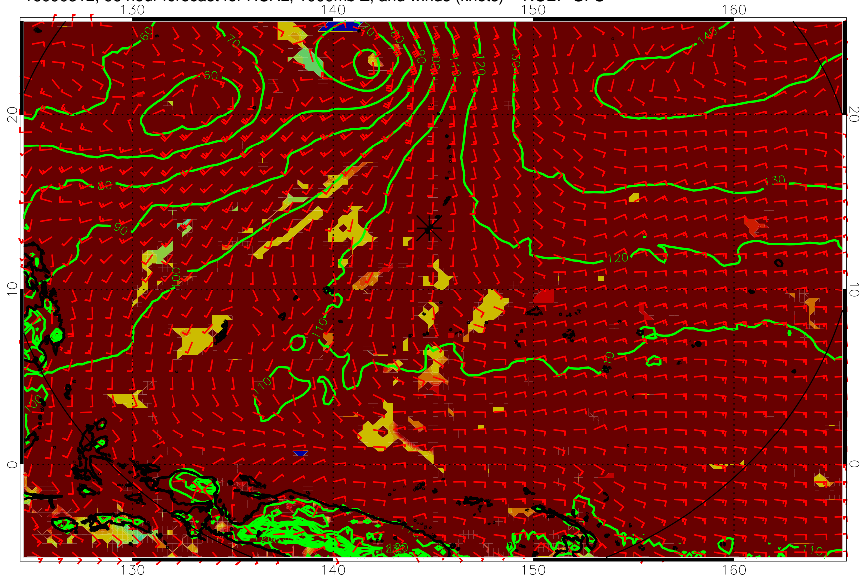
16090312, 96 hour forecast for HCAL, 1000mb Z, and winds (knots) -- NCEP GFS
