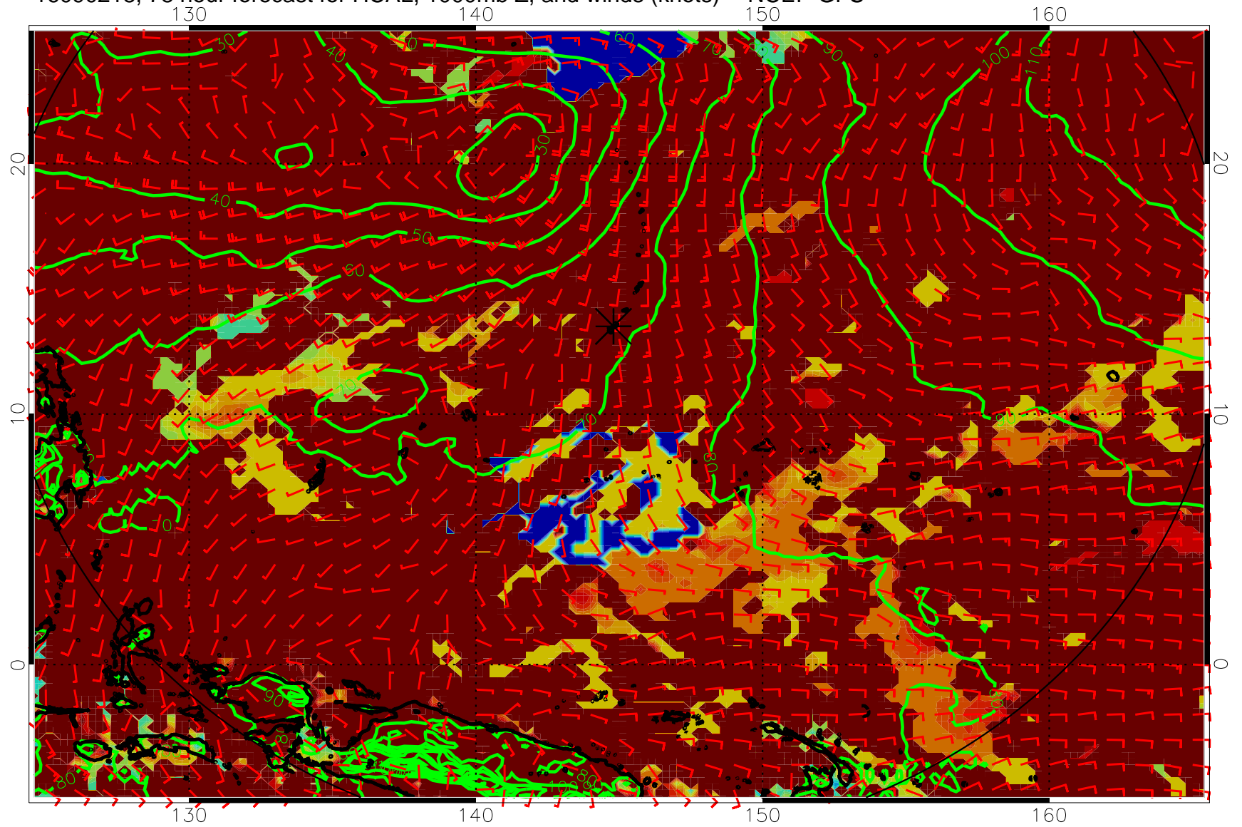
16090218, 78 hour forecast for HCAL, 1000mb Z, and winds (knots) -- NCEP GFS
