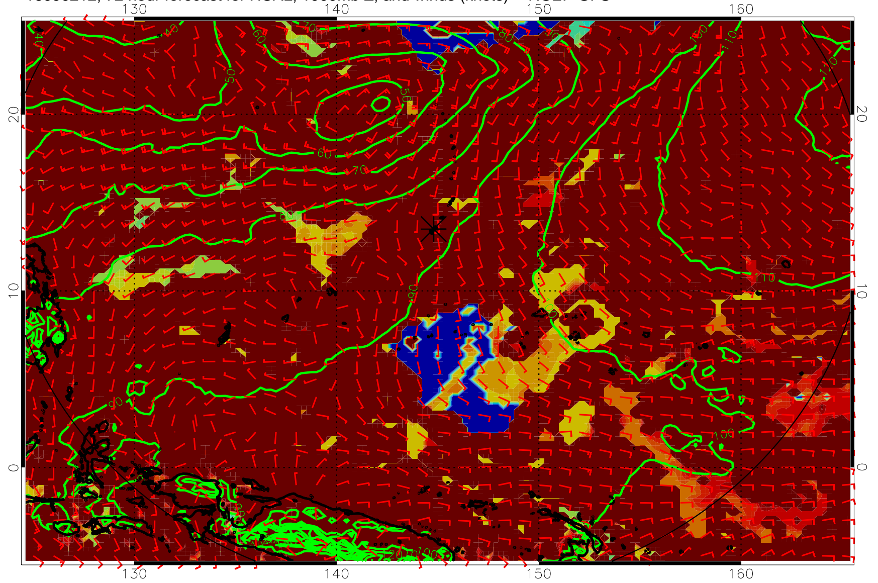
16090212, 72 hour forecast for HCAL, 1000mb Z, and winds (knots) -- NCEP GFS
