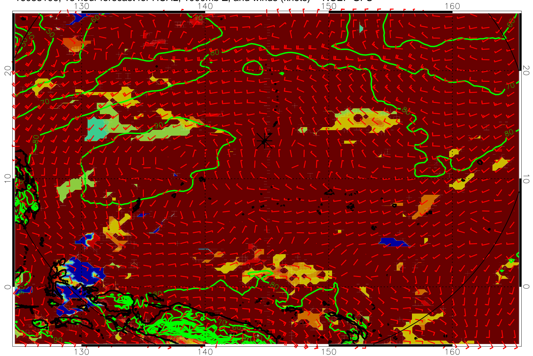
16083106, 18 hour forecast for HCAL, 1000mb Z, and winds (knots) -- NCEP GFS
