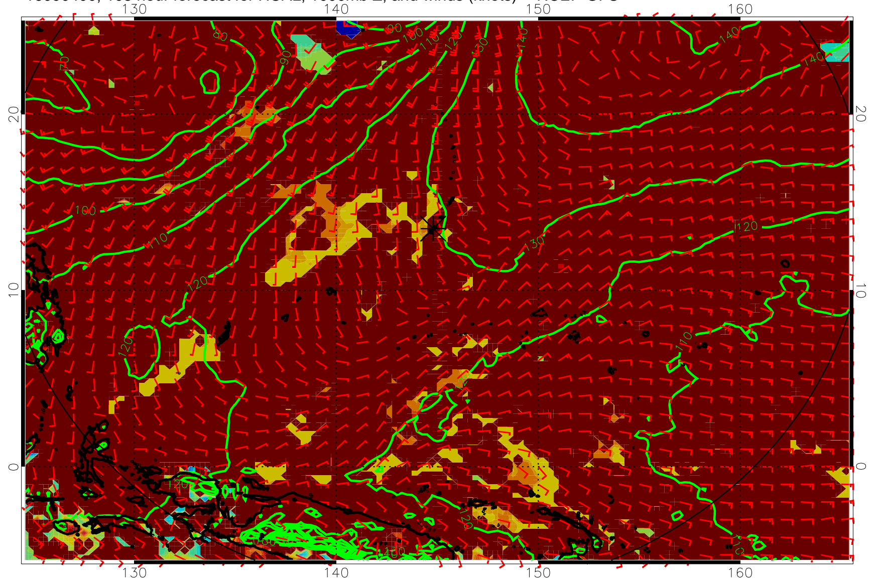
16090400, 108 hour forecast for HCAL, 1000mb Z, and winds (knots) -- NCEP GFS
