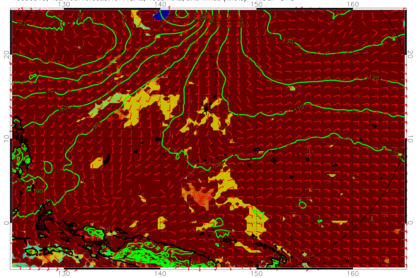
16090318, 102 hour forecast for HCAL, 1000mb Z, and winds (knots) -- NCEP GFS
