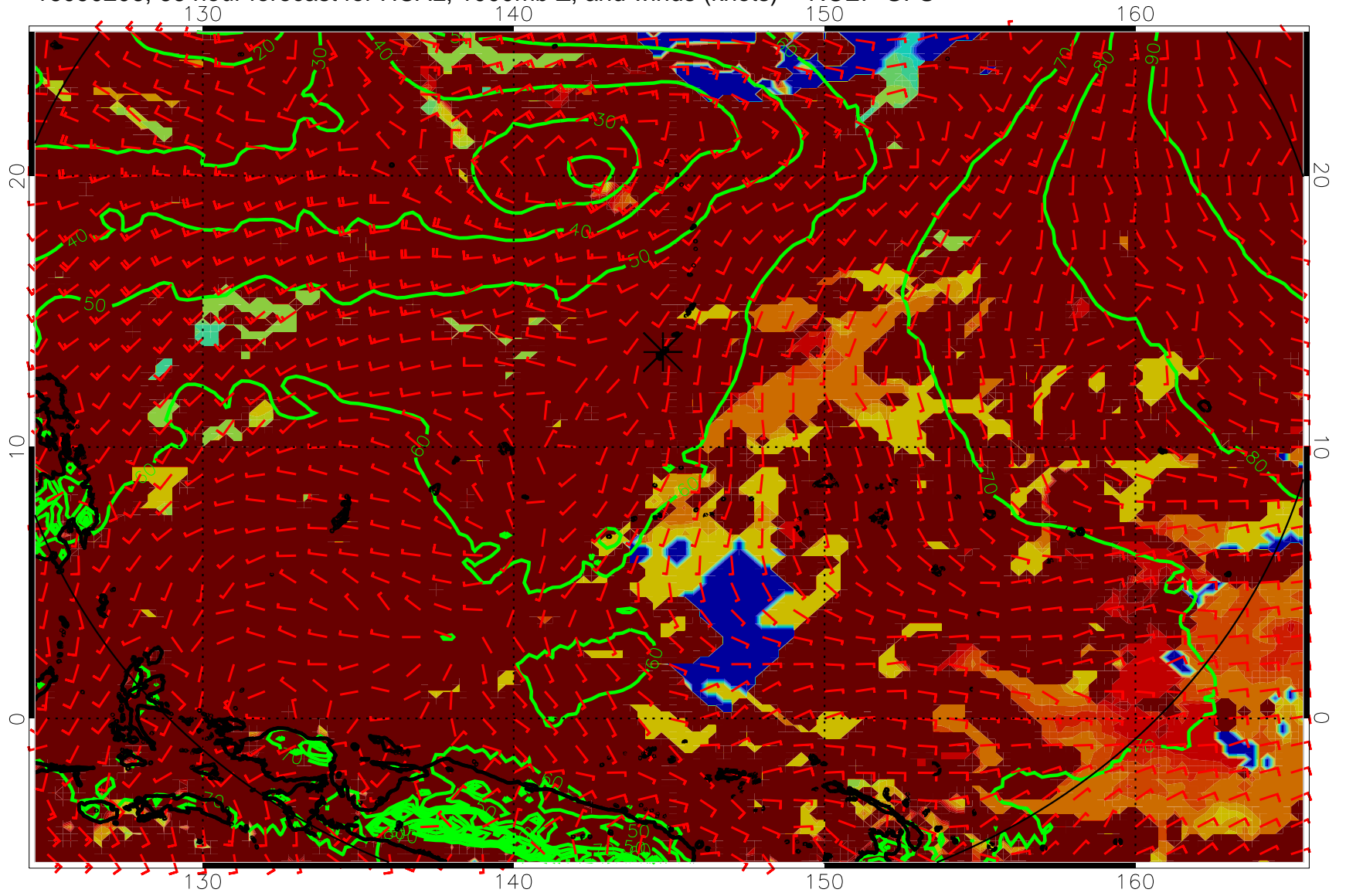
16090206, 66 hour forecast for HCAL, 1000mb Z, and winds (knots) -- NCEP GFS
