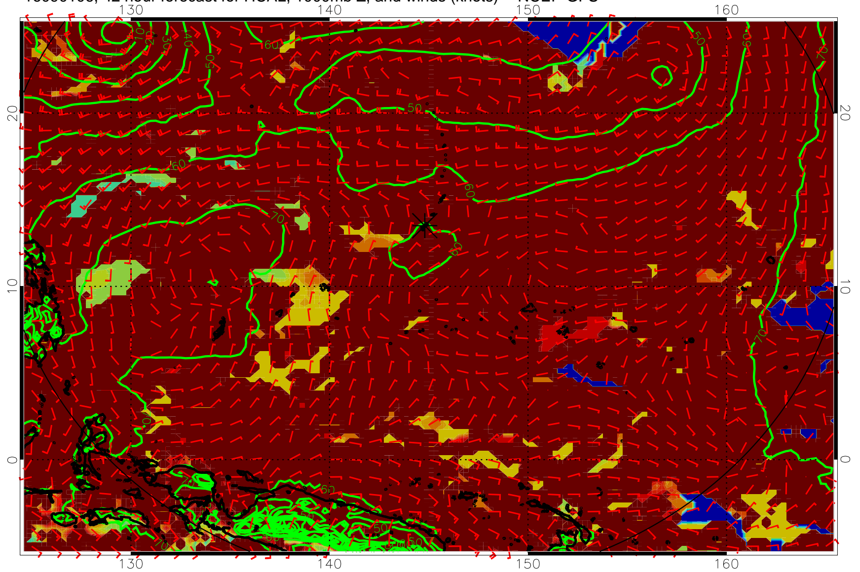
16090106, 42 hour forecast for HCAL, 1000mb Z, and winds (knots) -- NCEP GFS
