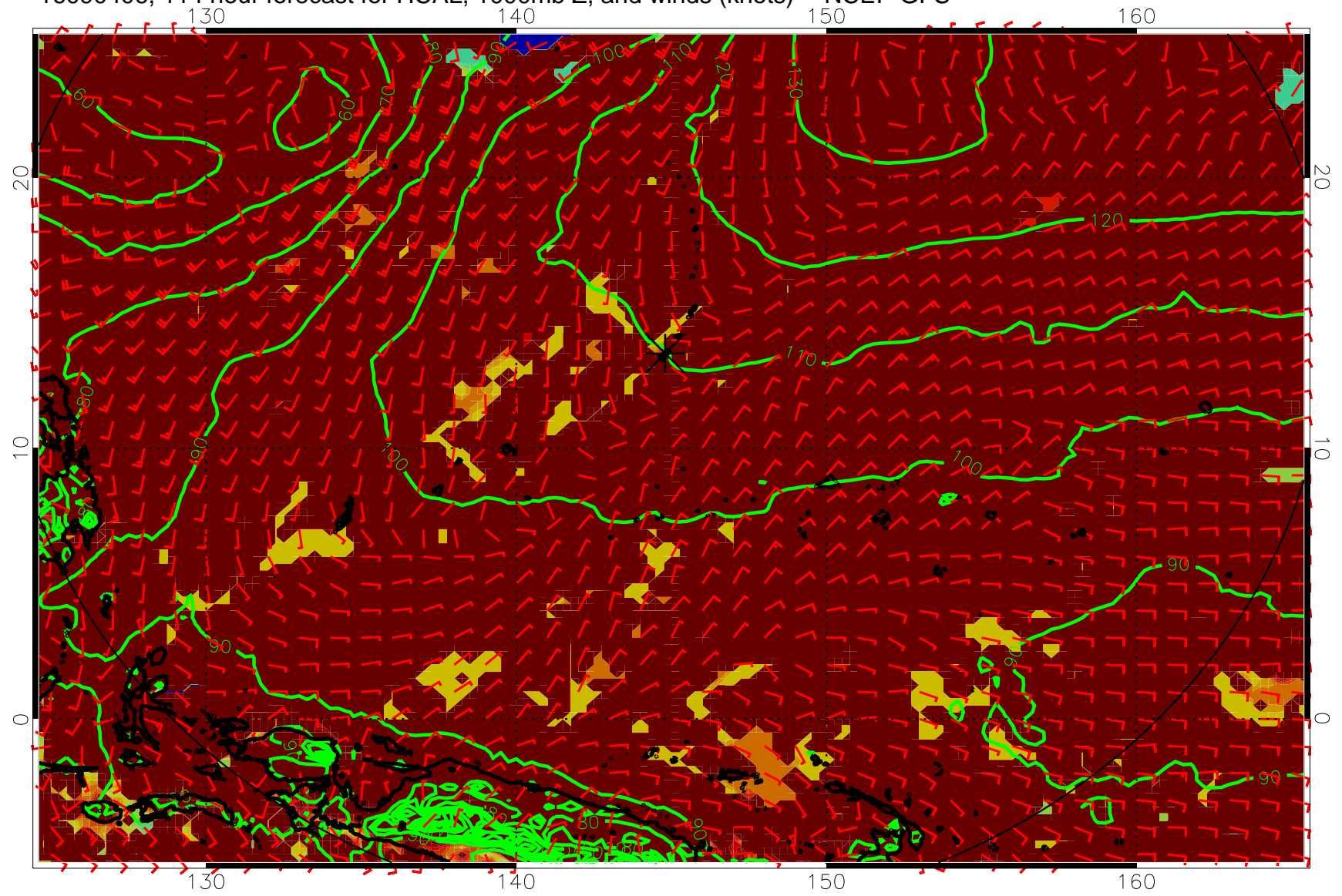
16090406, 114 hour forecast for HCAL, 1000mb Z, and winds (knots) -- NCEP GFS
