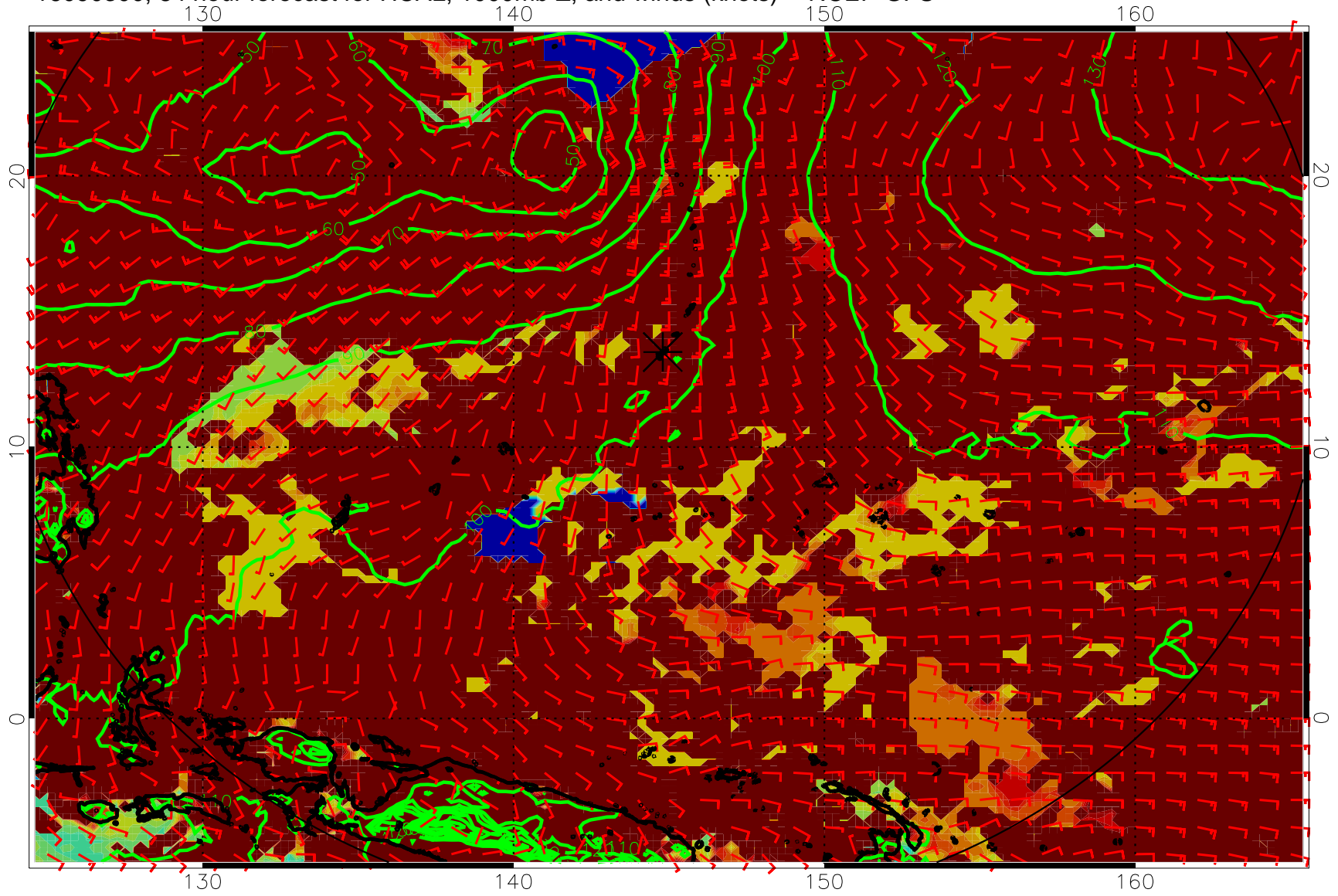
16090300, 84 hour forecast for HCAL, 1000mb Z, and winds (knots) -- NCEP GFS
