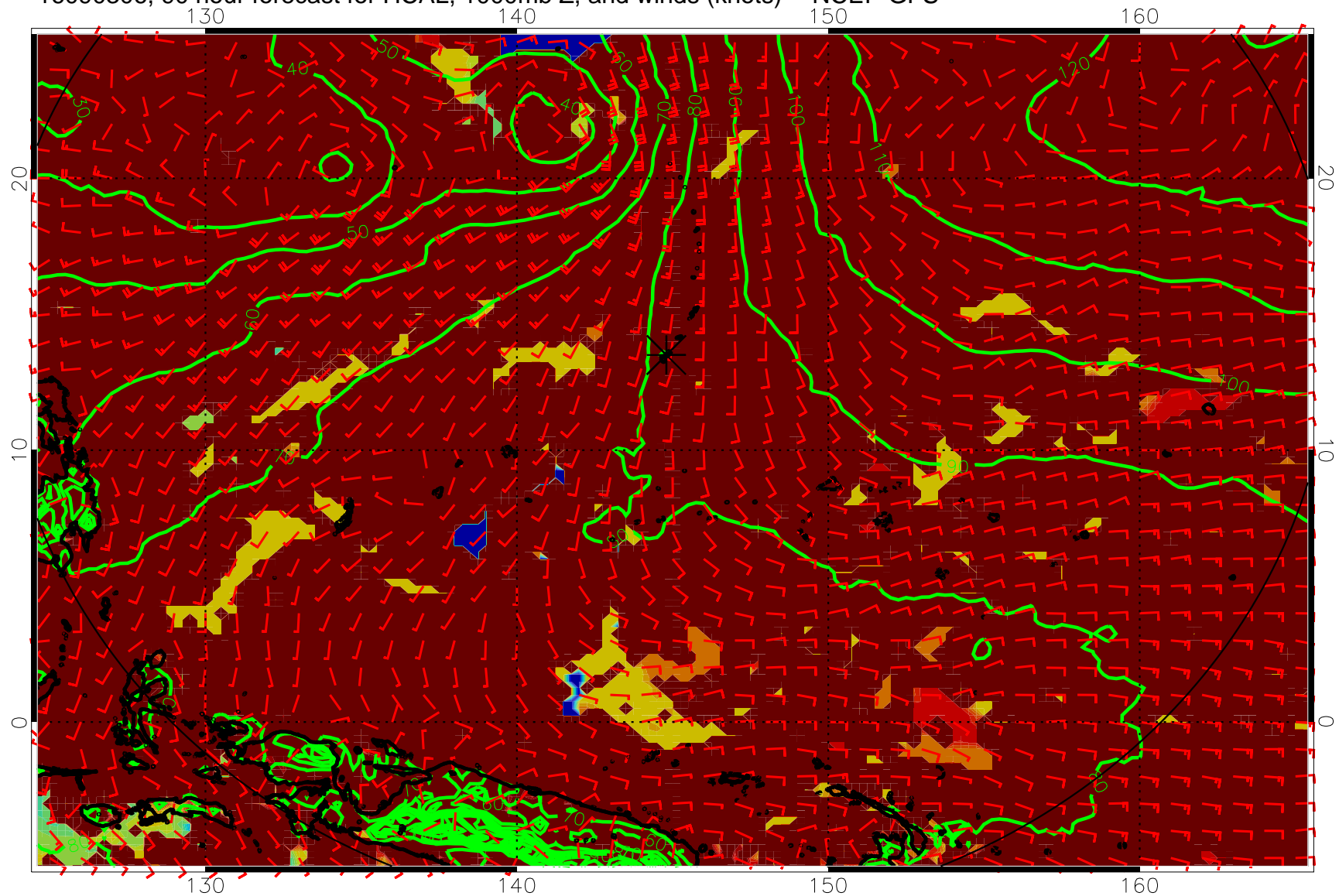
16090306, 90 hour forecast for HCAL, 1000mb Z, and winds (knots) -- NCEP GFS
