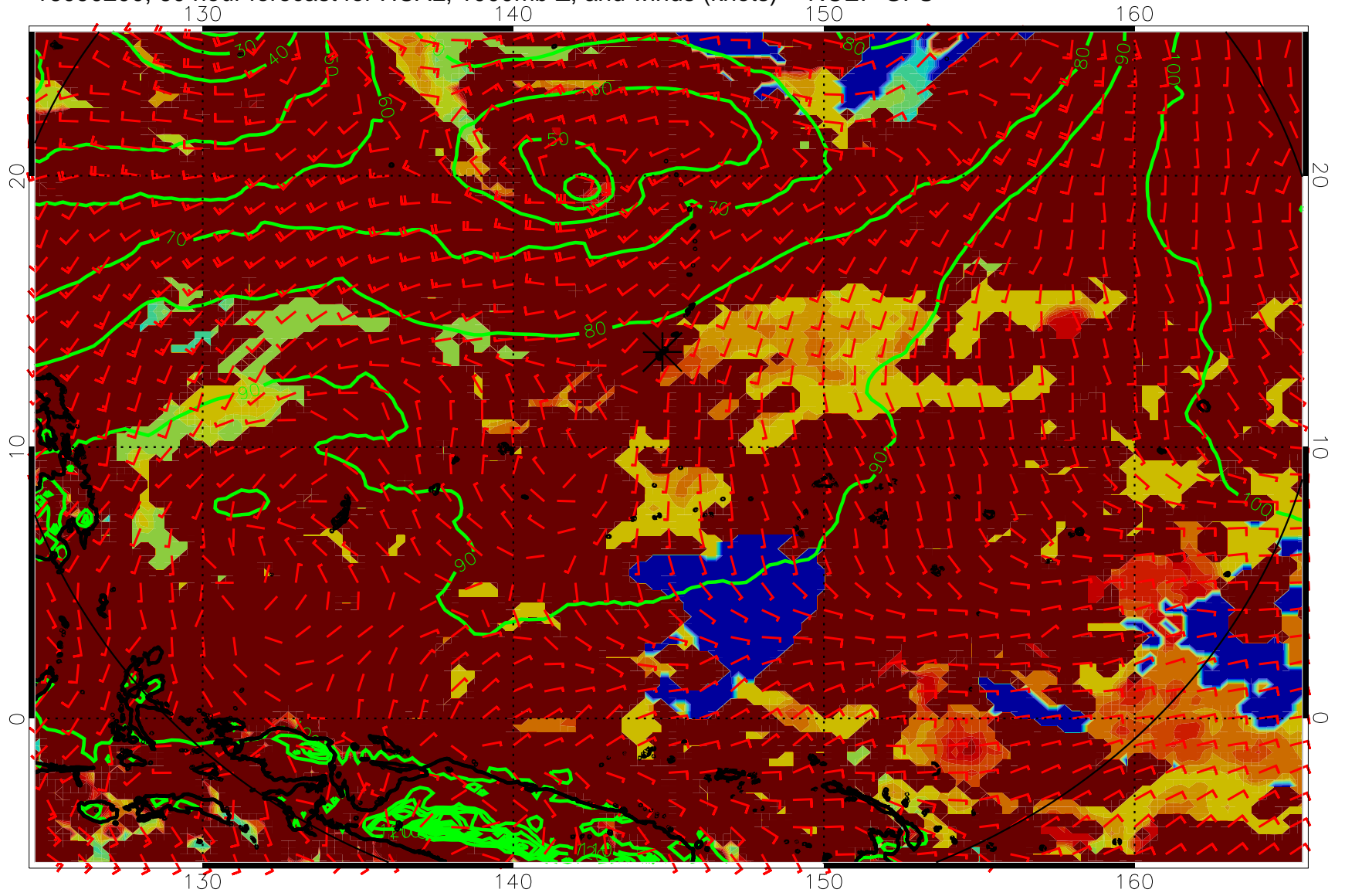
16090200, 60 hour forecast for HCAL, 1000mb Z, and winds (knots) -- NCEP GFS
