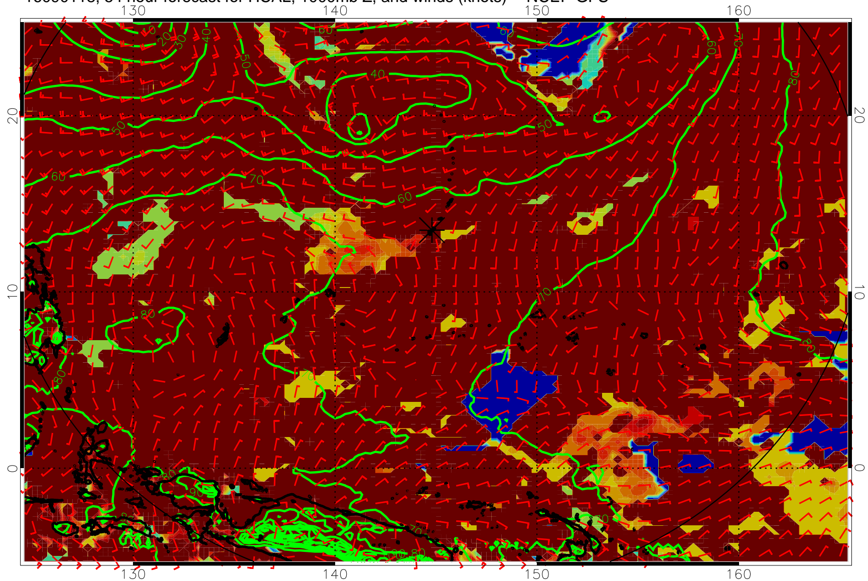
16090118, 54 hour forecast for HCAL, 1000mb Z, and winds (knots) -- NCEP GFS
