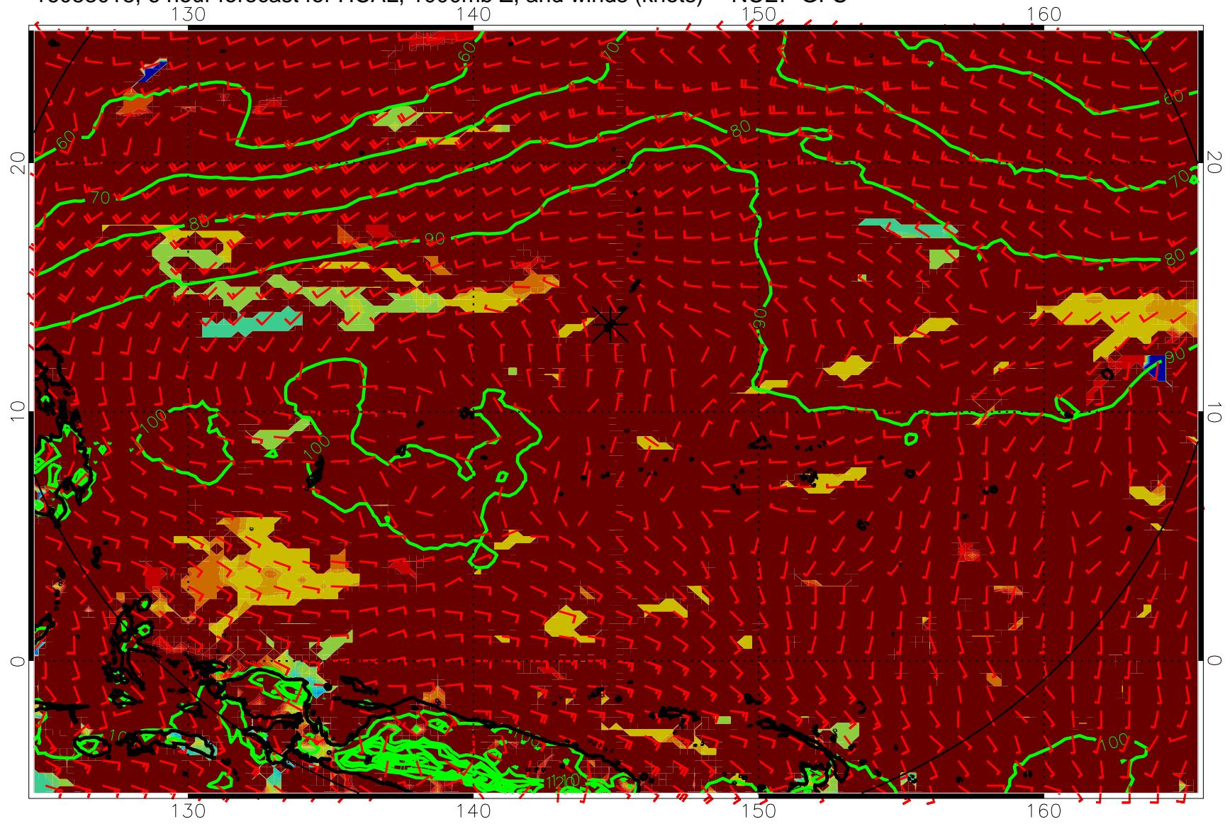
16083018, 6 hour forecast for HCAL, 1000mb Z, and winds (knots) -- NCEP GFS
