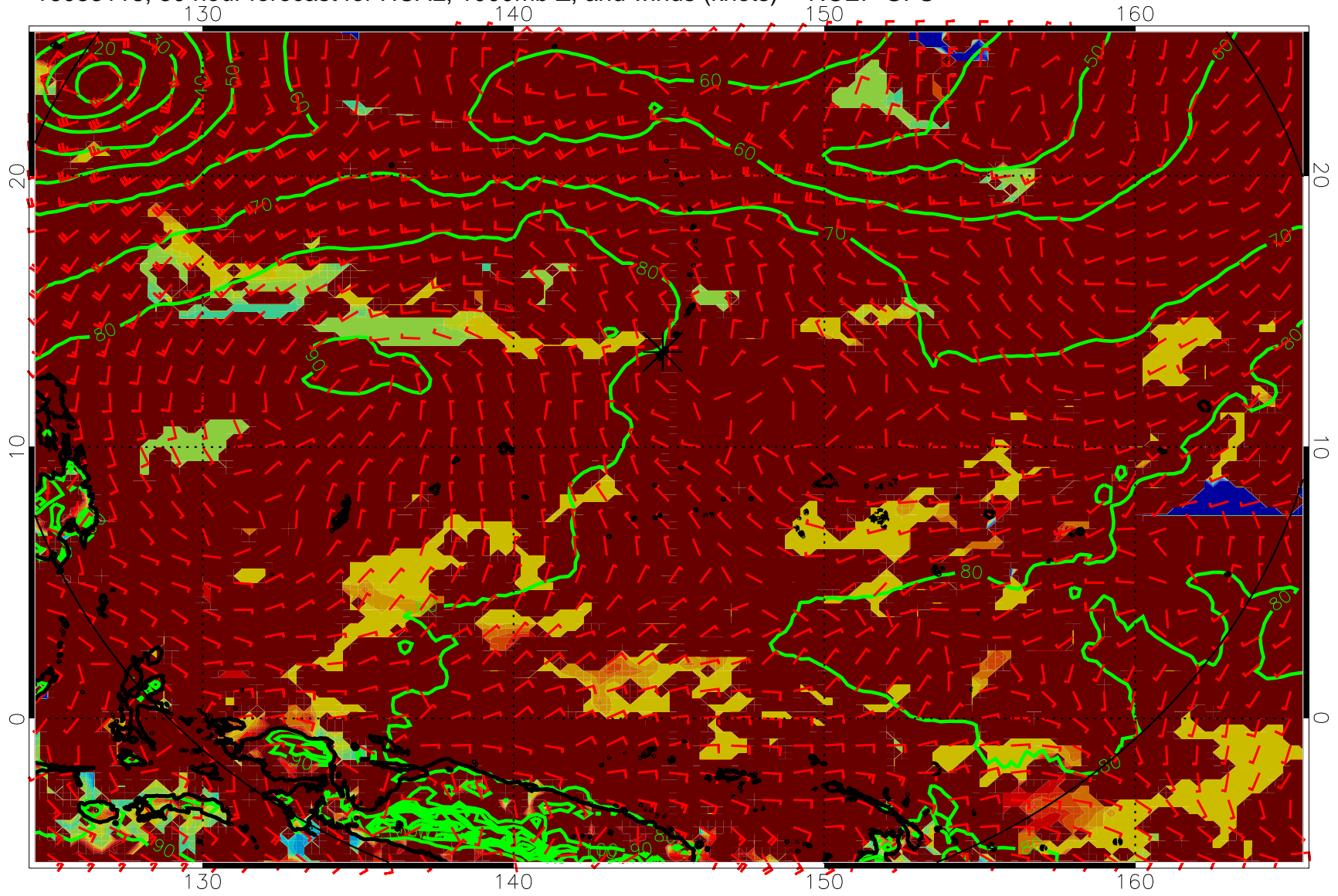
16083118, 30 hour forecast for HCAL, 1000mb Z, and winds (knots) -- NCEP GFS
