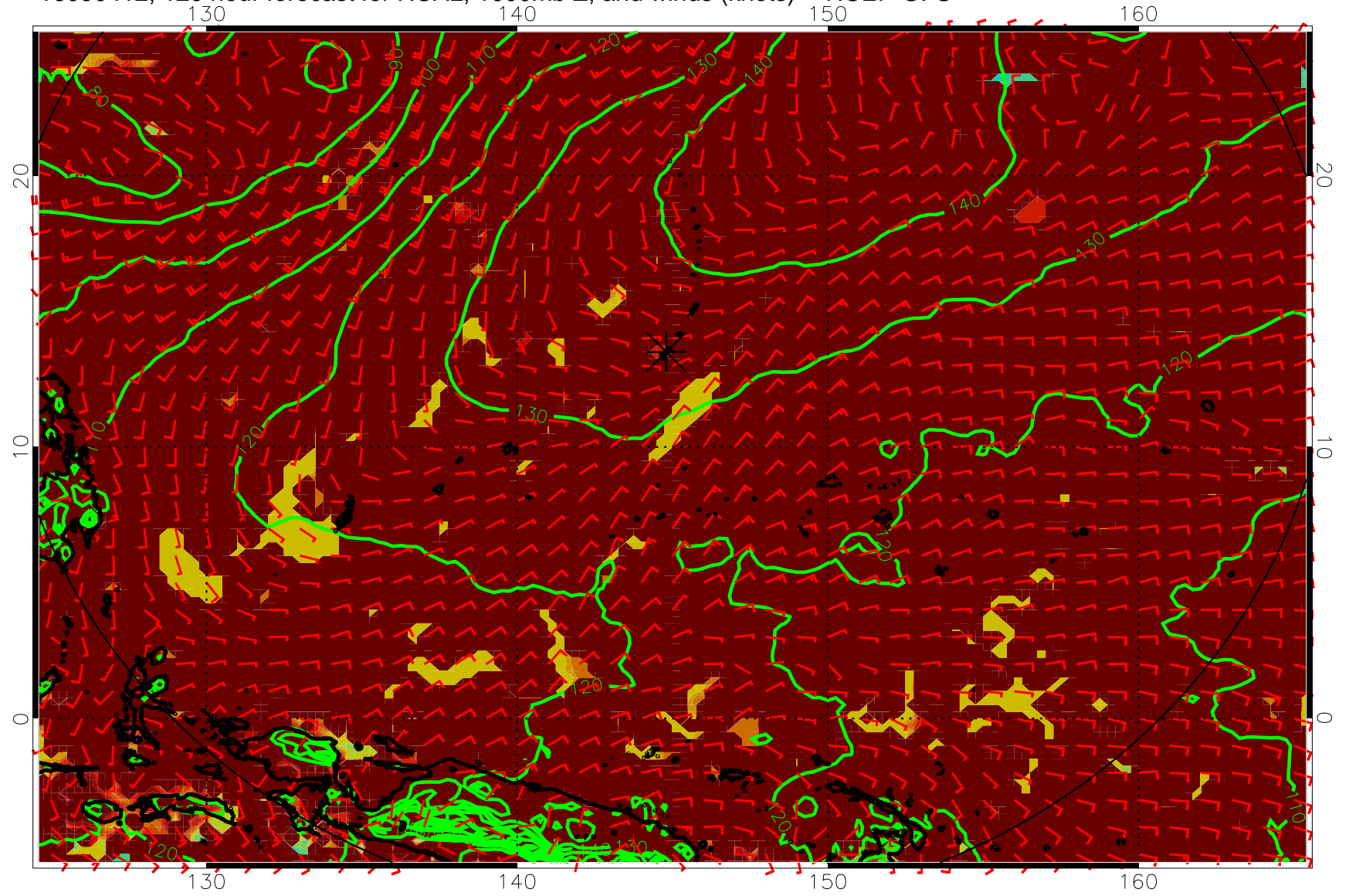
16090412, 120 hour forecast for HCAL, 1000mb Z, and winds (knots) -- NCEP GFS
