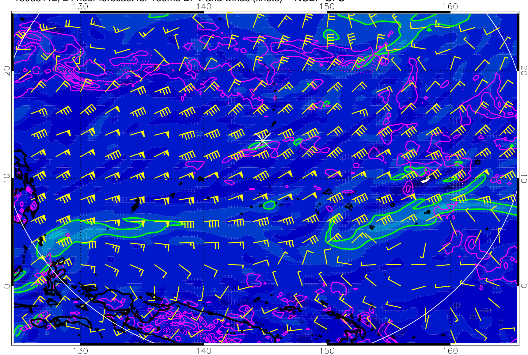
16083112, 24 hour forecast for 150mb EPV and winds (knots) -- NCEP GFS
