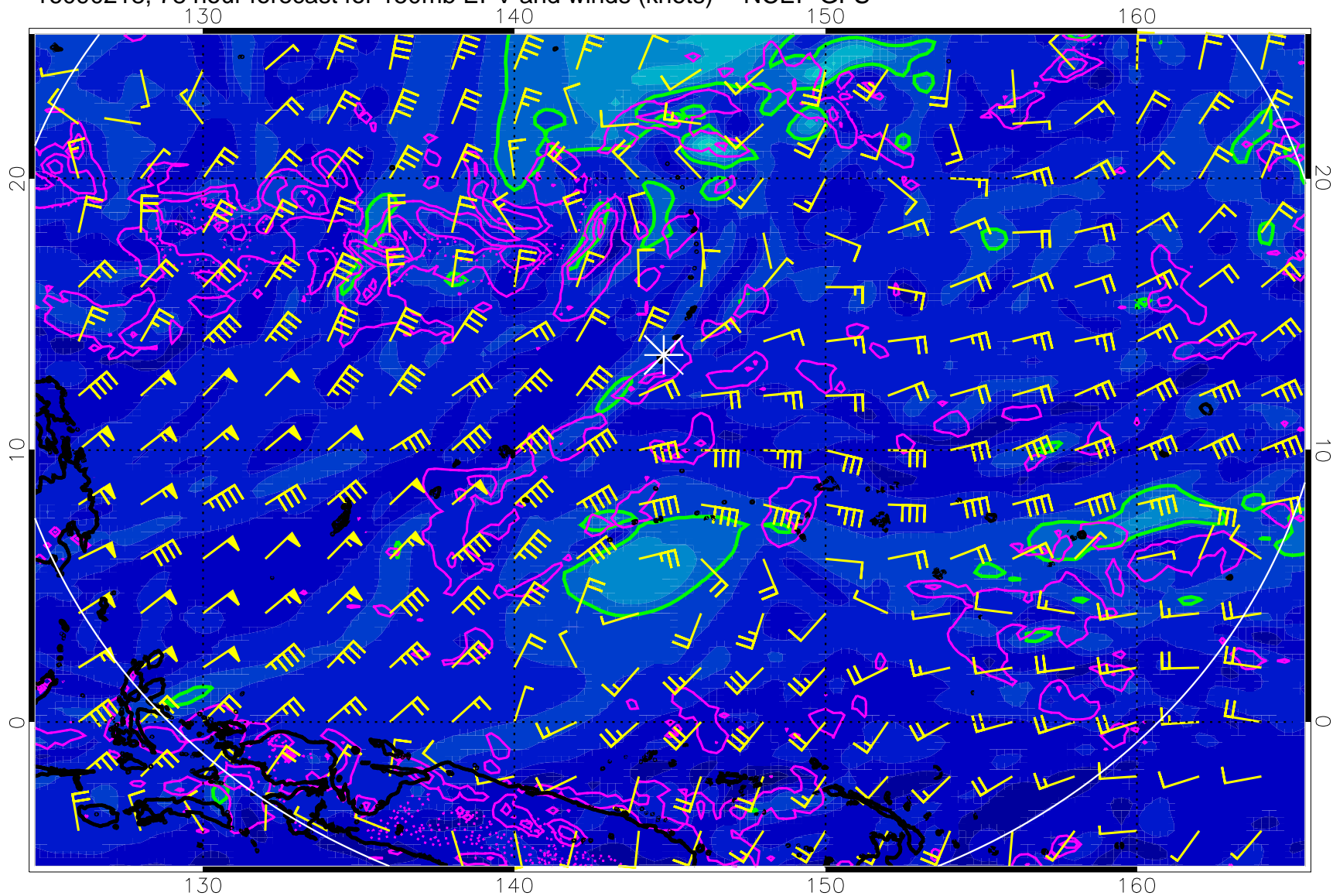
16090218, 78 hour forecast for 150mb EPV and winds (knots) -- NCEP GFS
