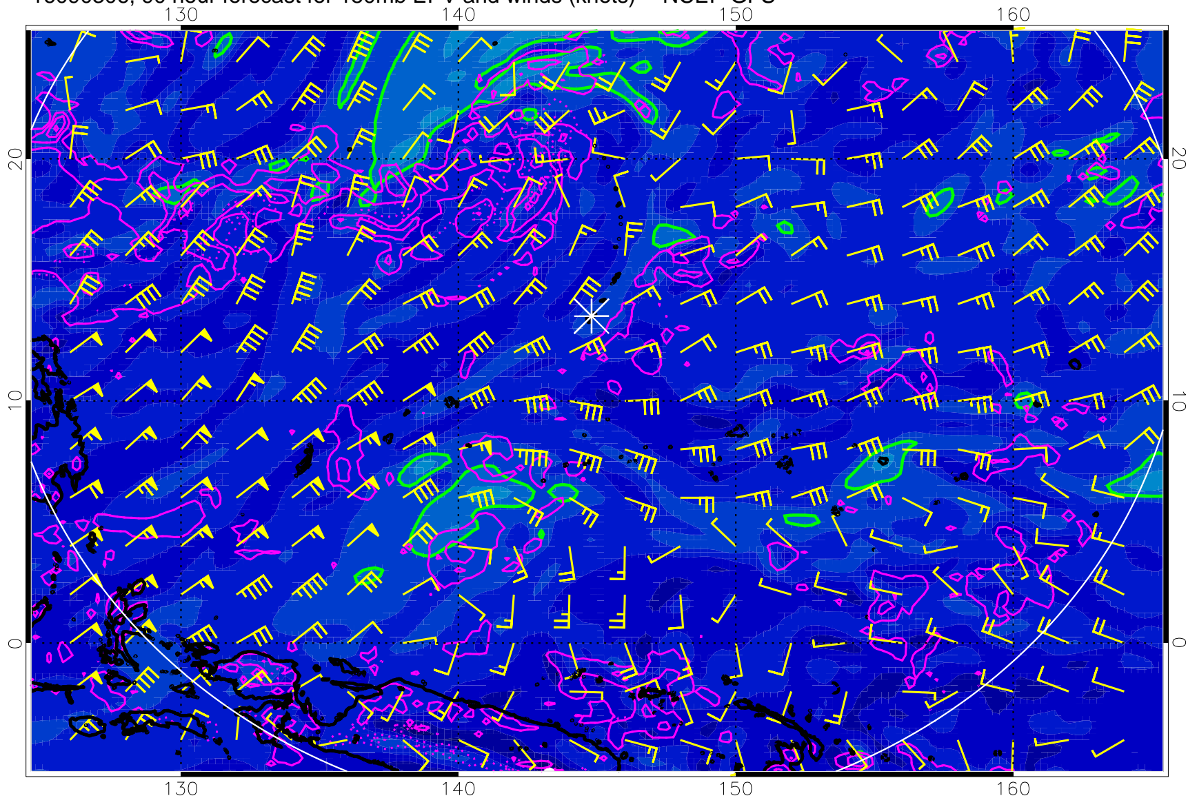
16090306, 90 hour forecast for 150mb EPV and winds (knots) -- NCEP GFS
