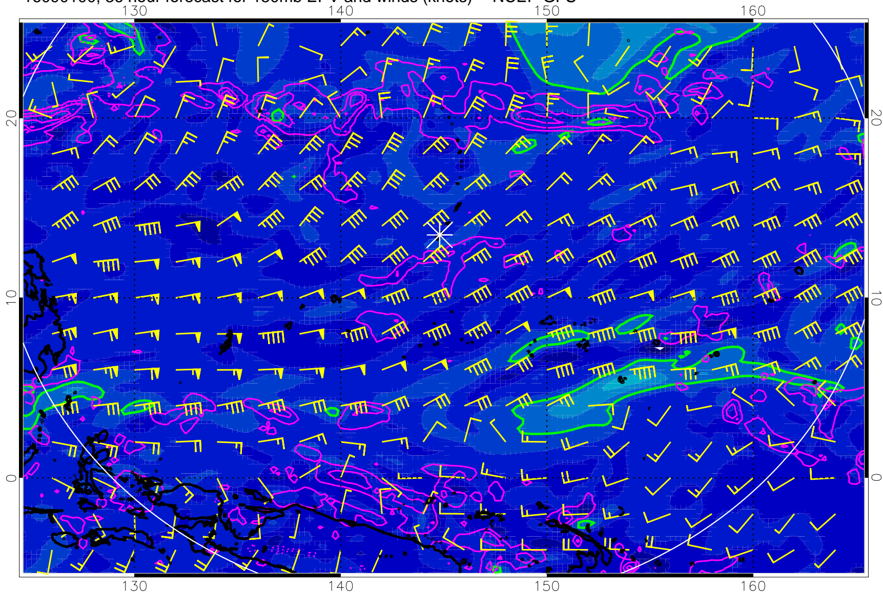
16090100, 36 hour forecast for 150mb EPV and winds (knots) -- NCEP GFS
