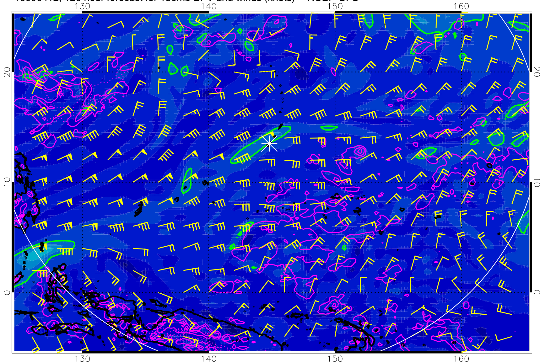
16090412, 120 hour forecast for 150mb EPV and winds (knots) -- NCEP GFS
