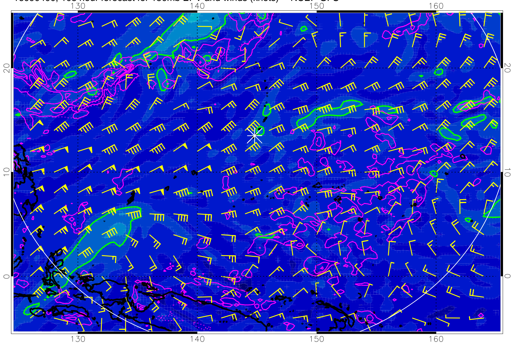
16090400, 108 hour forecast for 150mb EPV and winds (knots) -- NCEP GFS
