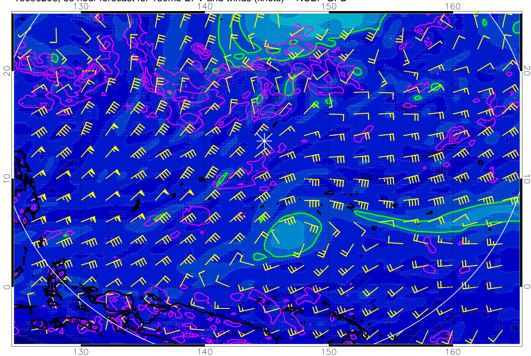
16090206, 66 hour forecast for 150mb EPV and winds (knots) -- NCEP GFS
