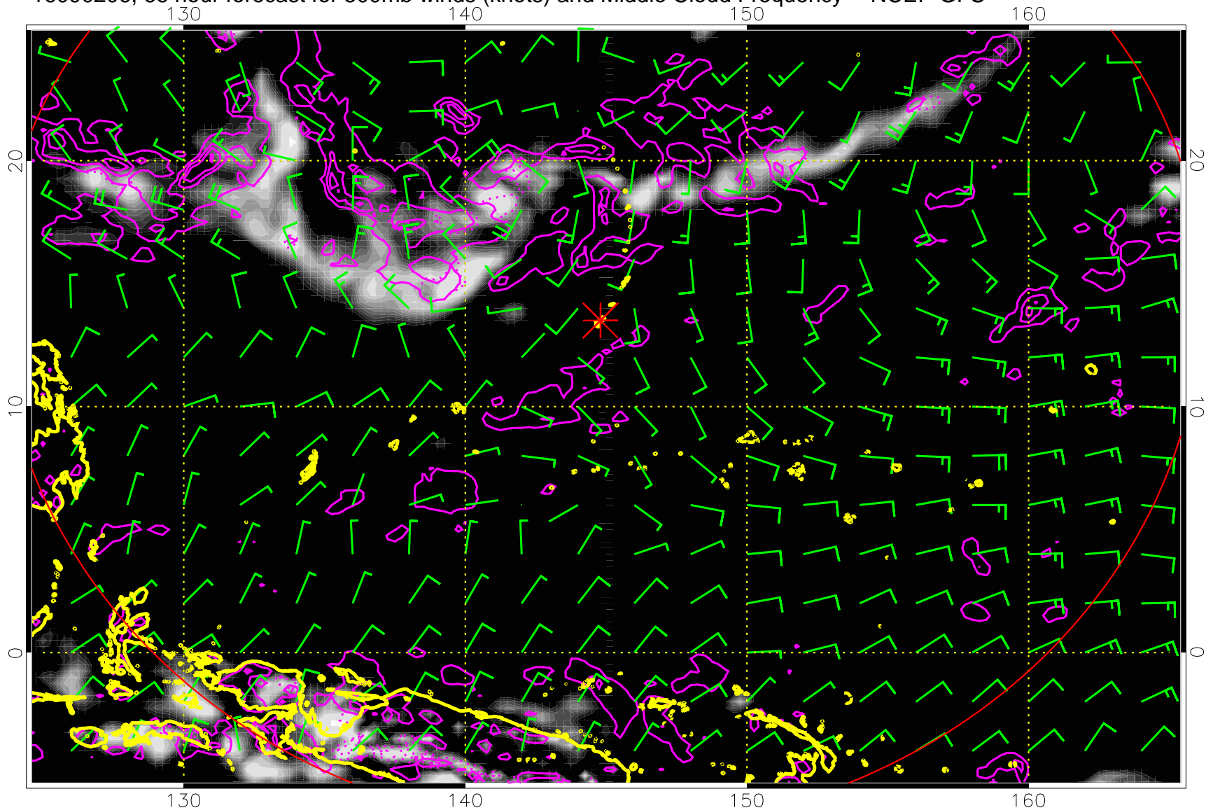
16090206, 66 hour forecast for 500mb winds (knots) and Middle Cloud Frequency -- NCEP GFS
