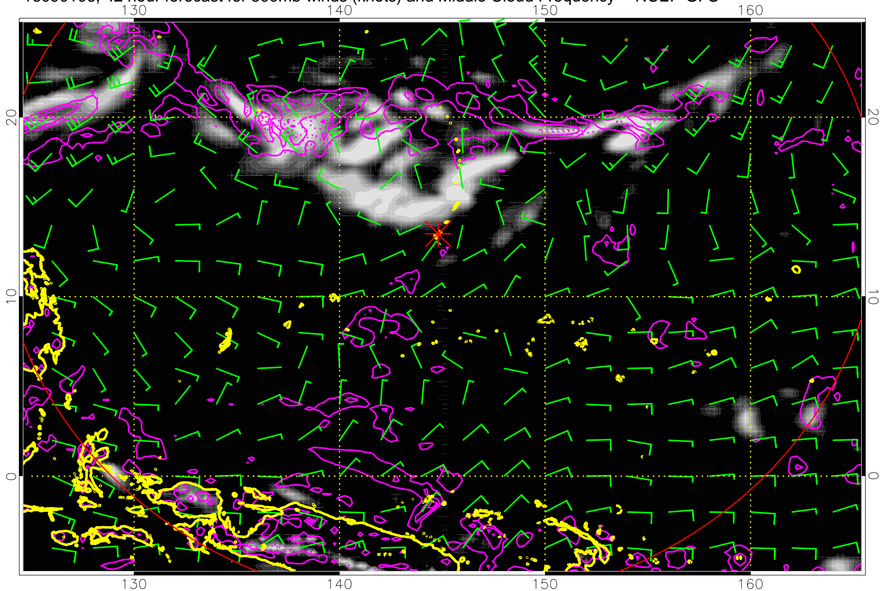
16090106, 42 hour forecast for 500mb winds (knots) and Middle Cloud Frequency -- NCEP GFS
