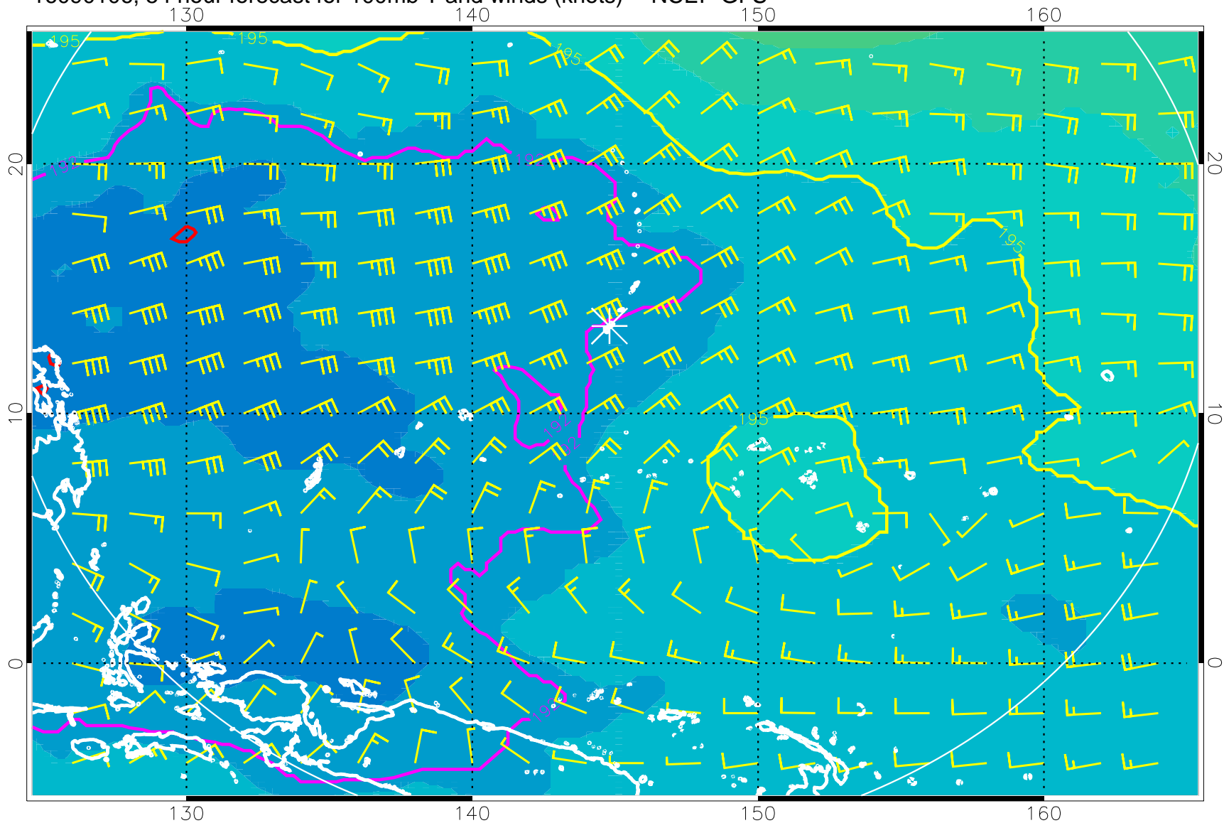
16090106, 54 hour forecast for 100mb T and winds (knots) -- NCEP GFS
