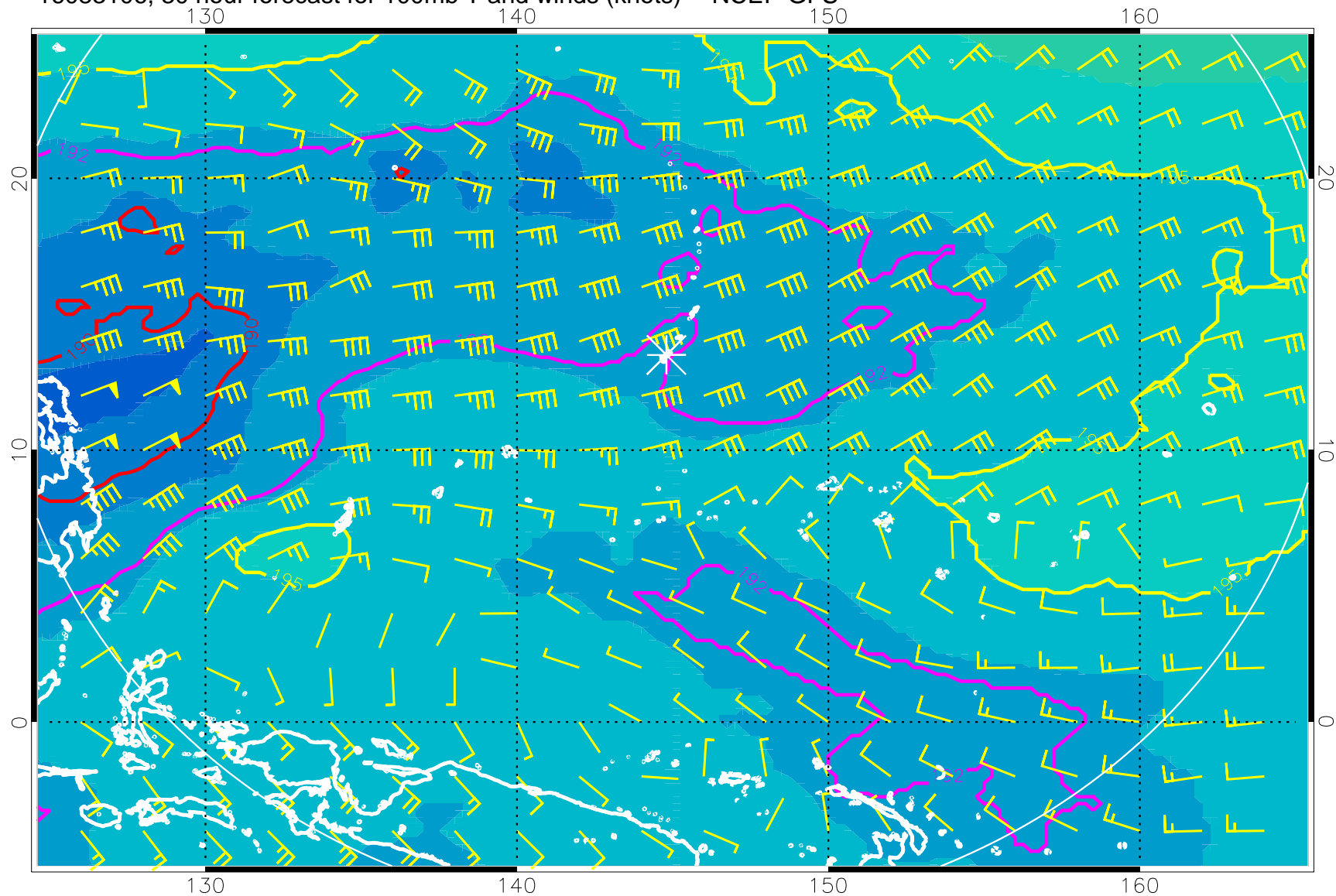
16083106, 30 hour forecast for 100mb T and winds (knots) -- NCEP GFS
