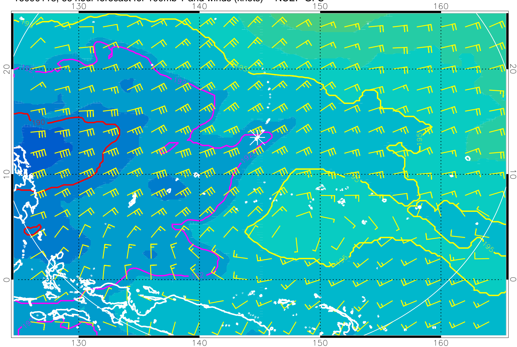
16090118, 66 hour forecast for 100mb T and winds (knots) -- NCEP GFS
