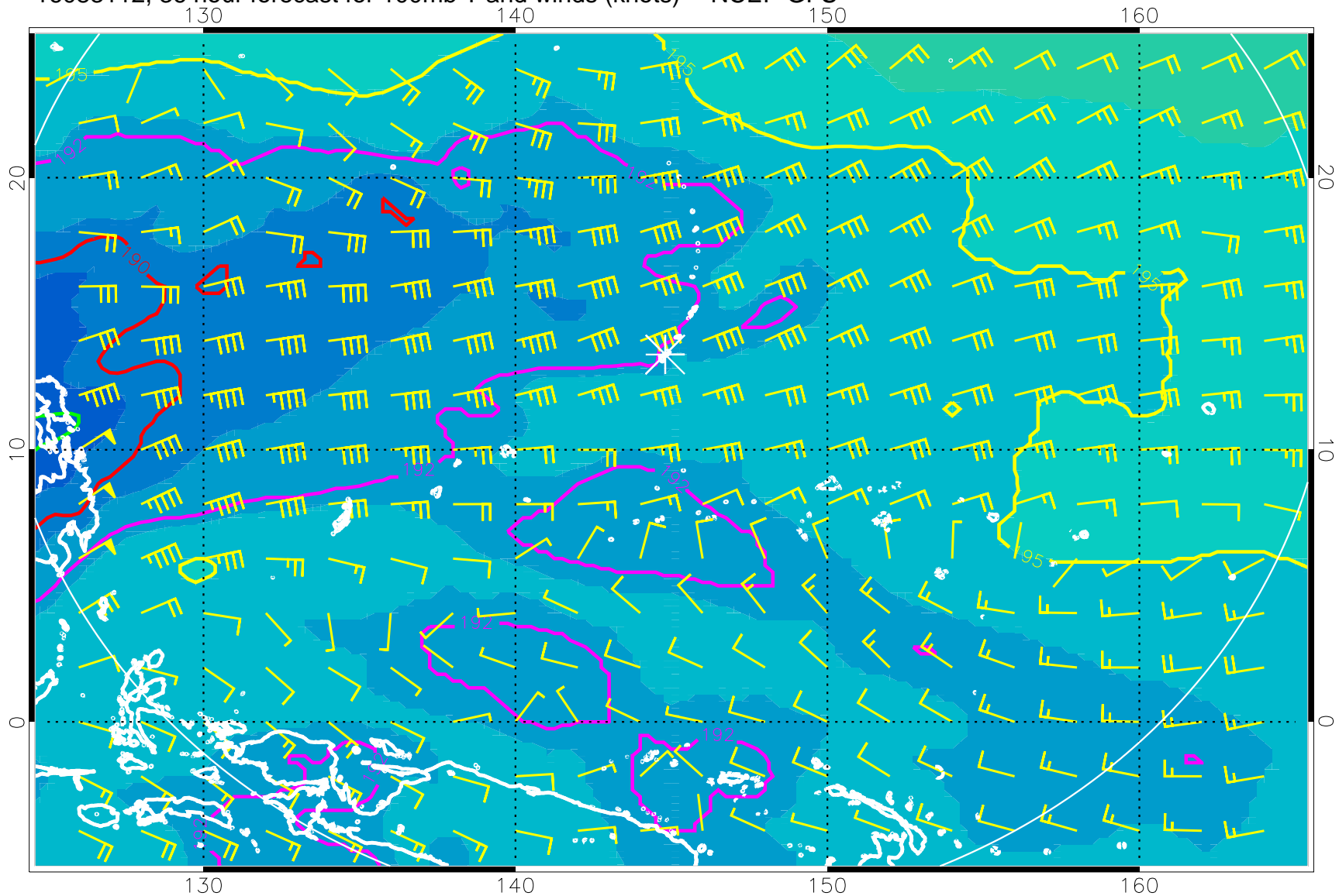
16083112, 36 hour forecast for 100mb T and winds (knots) -- NCEP GFS
