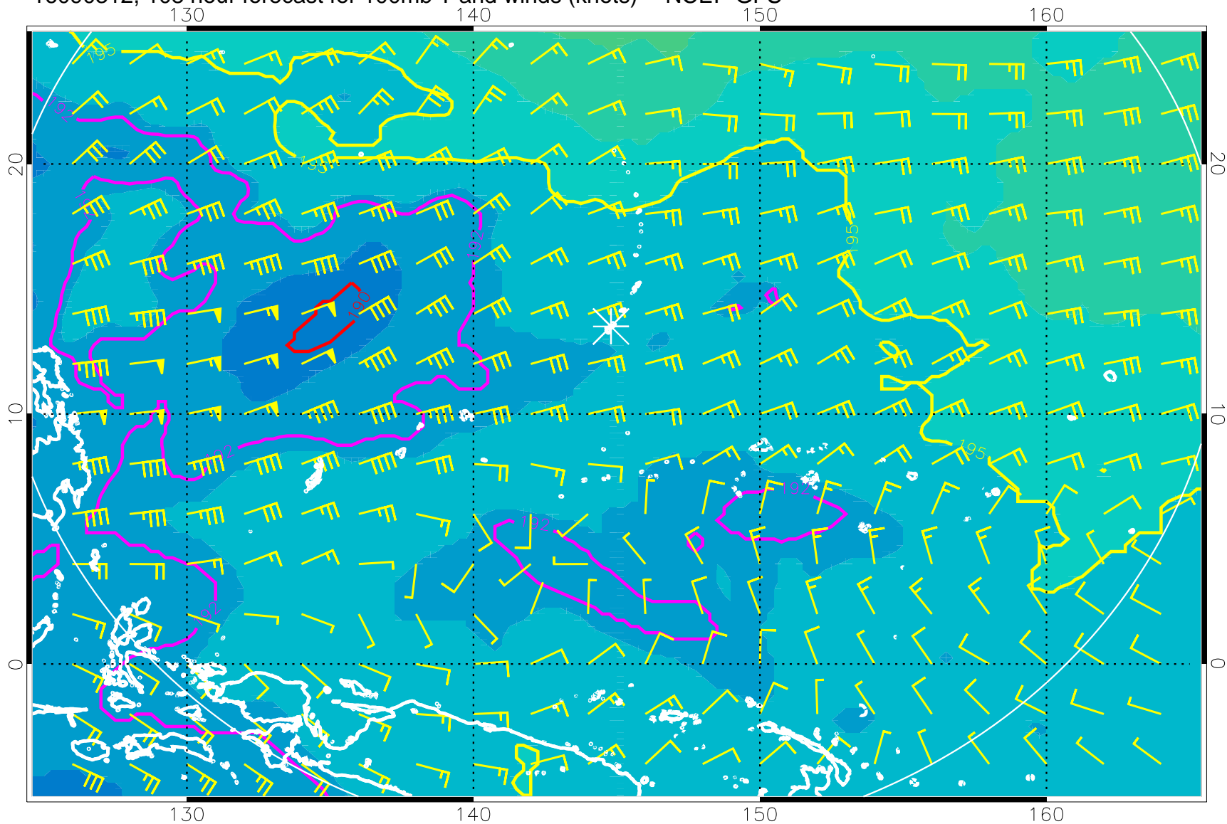
16090312, 108 hour forecast for 100mb T and winds (knots) -- NCEP GFS
