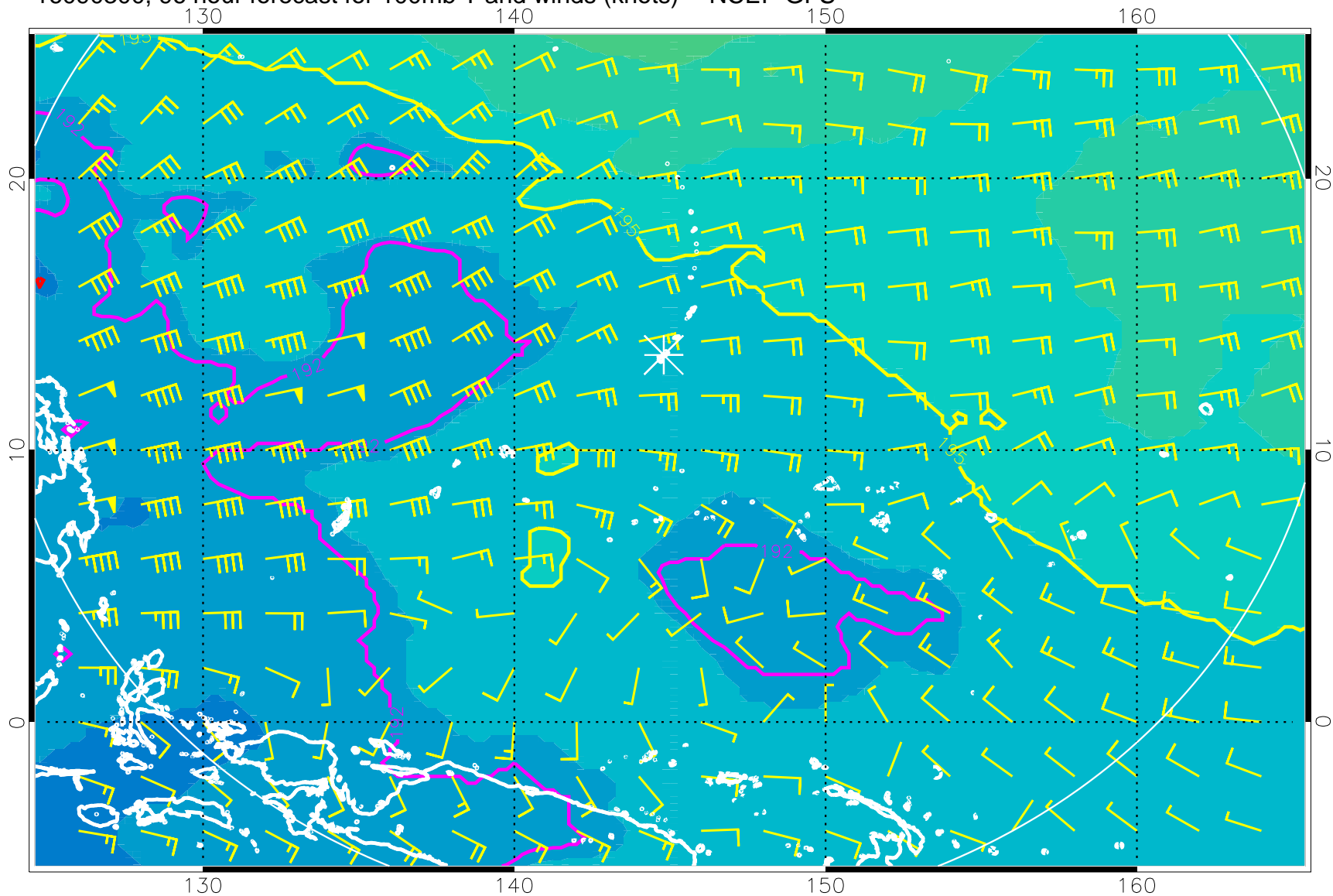
16090300, 96 hour forecast for 100mb T and winds (knots) -- NCEP GFS
