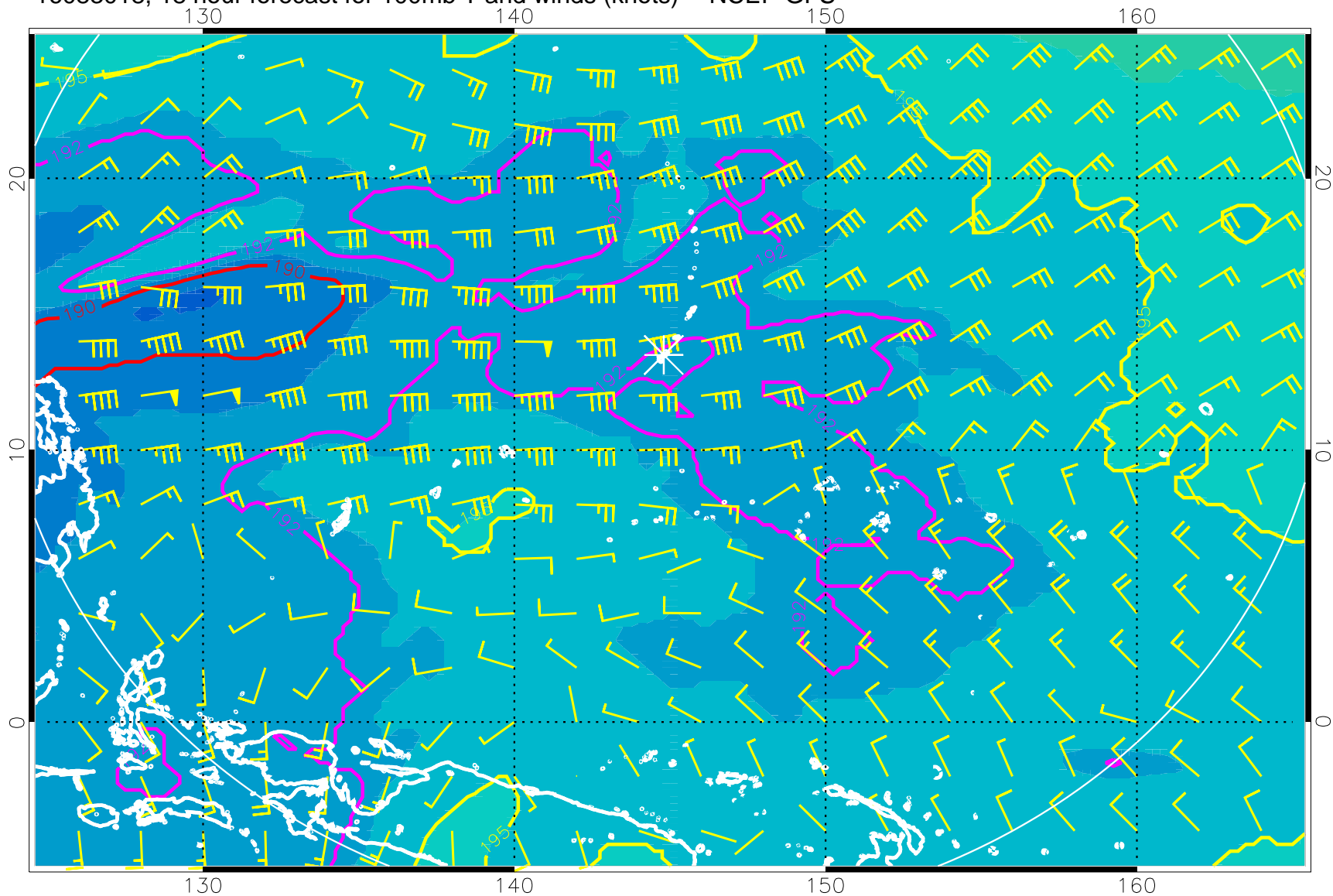
16083018, 18 hour forecast for 100mb T and winds (knots) -- NCEP GFS
