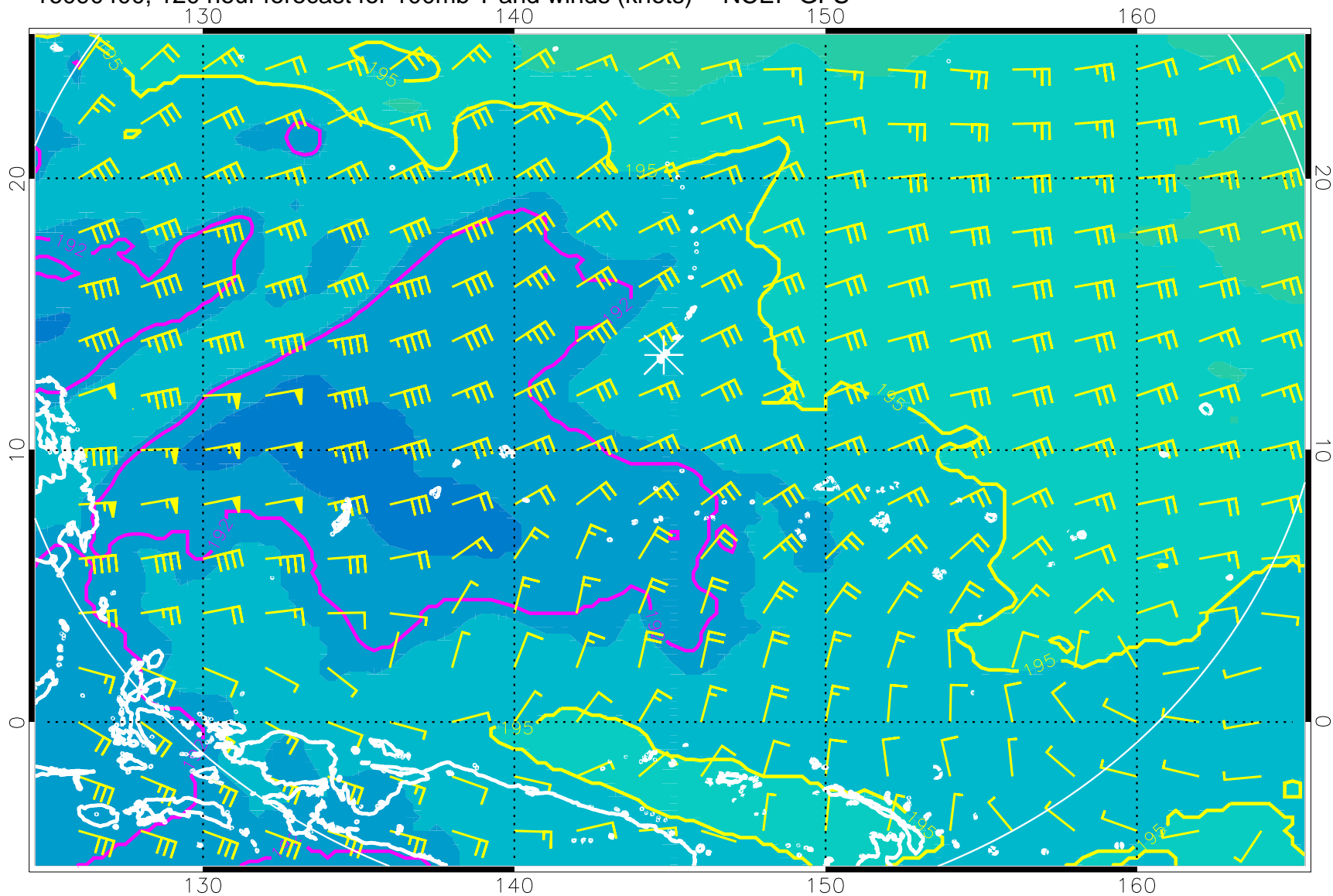
16090400, 120 hour forecast for 100mb T and winds (knots) -- NCEP GFS
