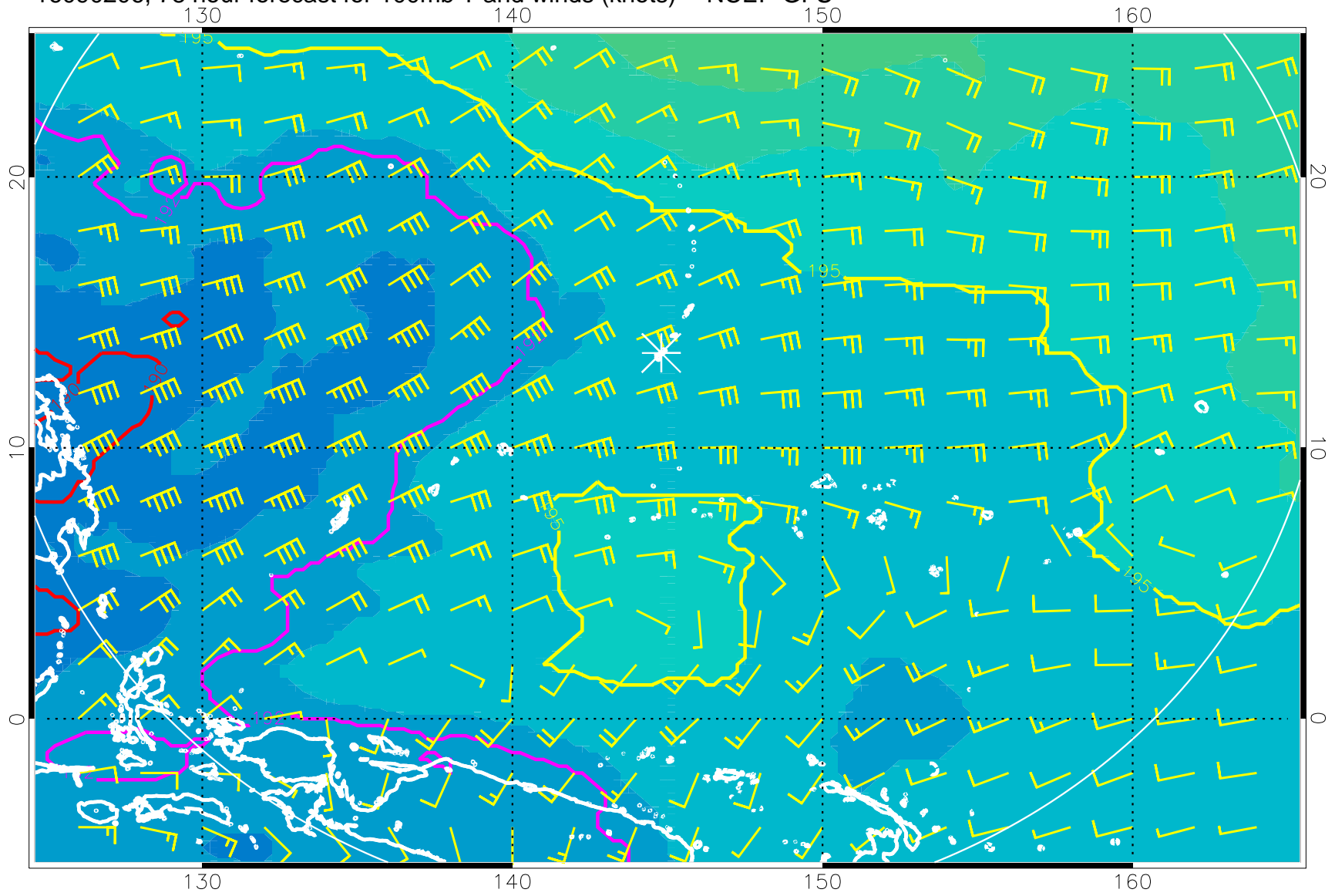
16090206, 78 hour forecast for 100mb T and winds (knots) -- NCEP GFS
