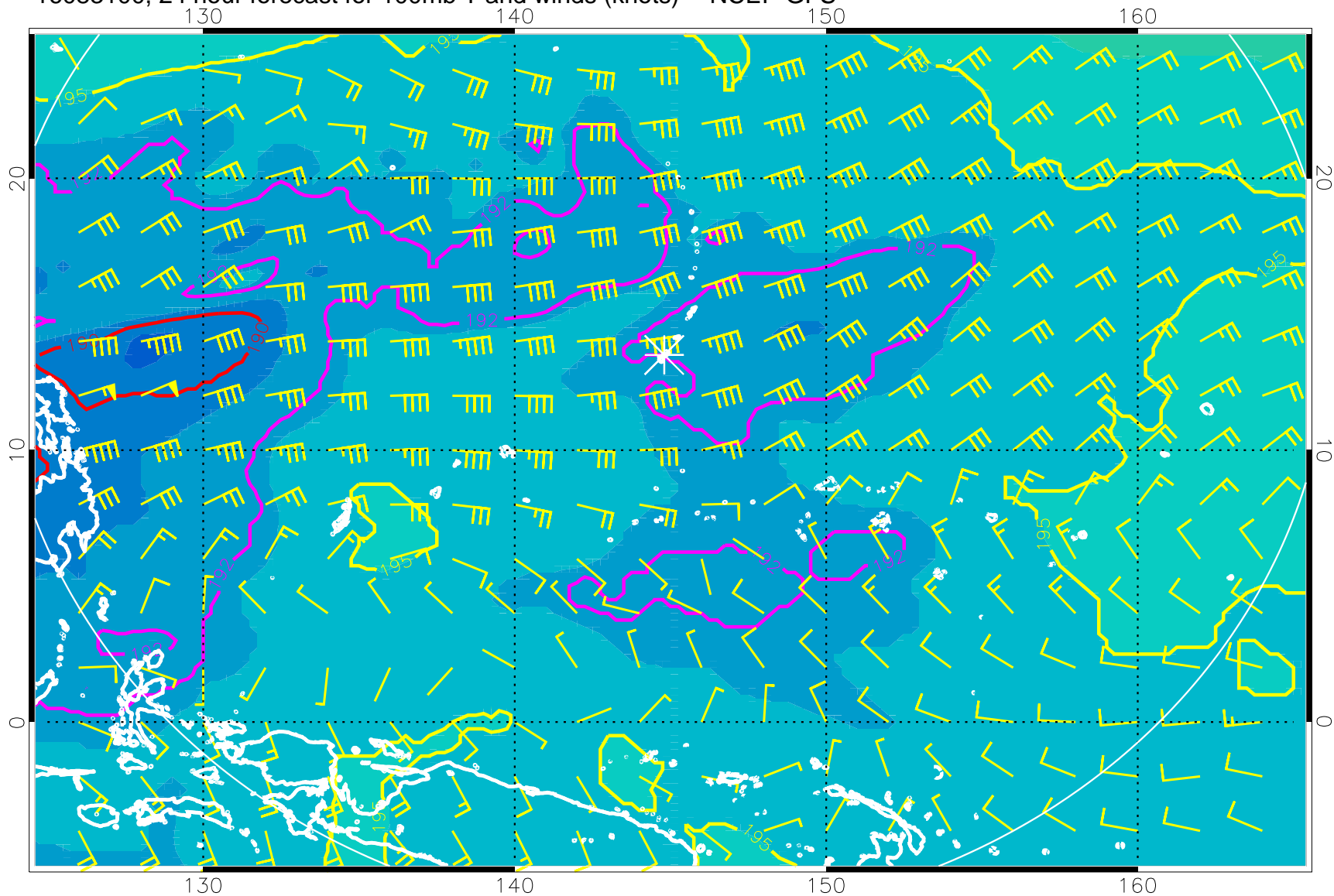
16083100, 24 hour forecast for 100mb T and winds (knots) -- NCEP GFS
