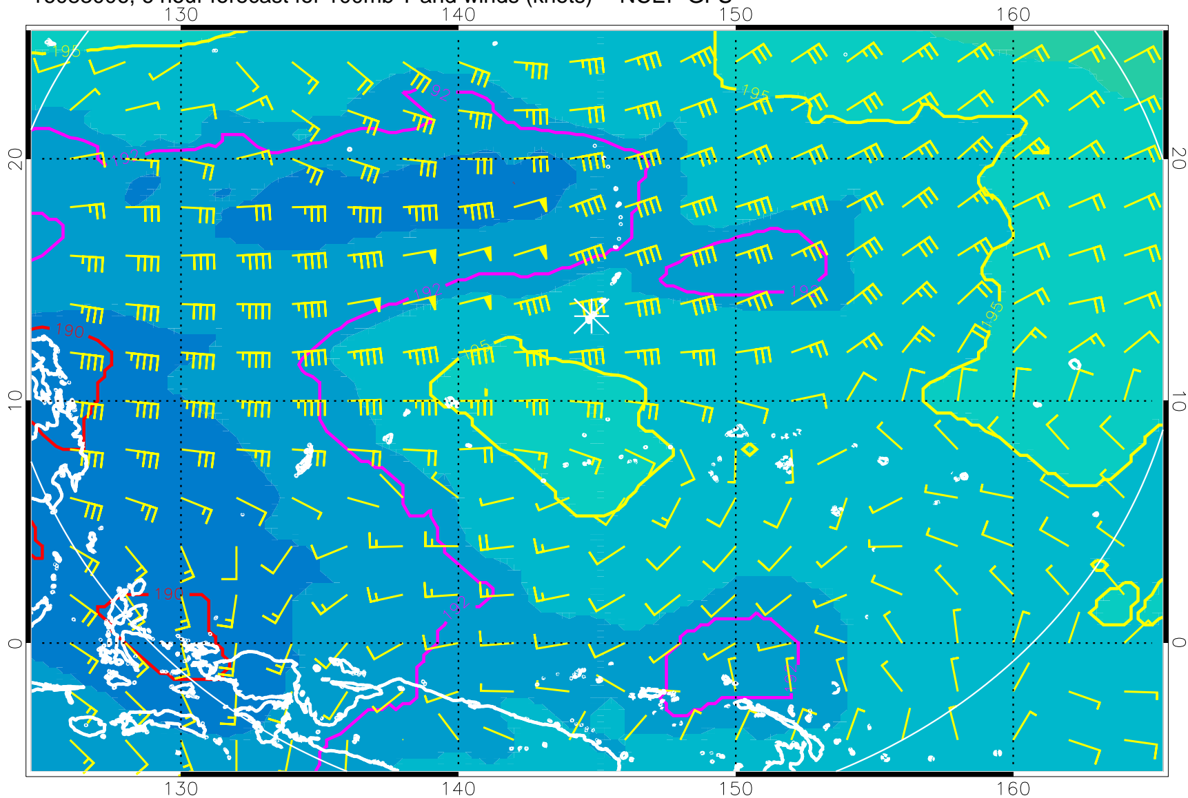
16083006, 6 hour forecast for 100mb T and winds (knots) -- NCEP GFS
