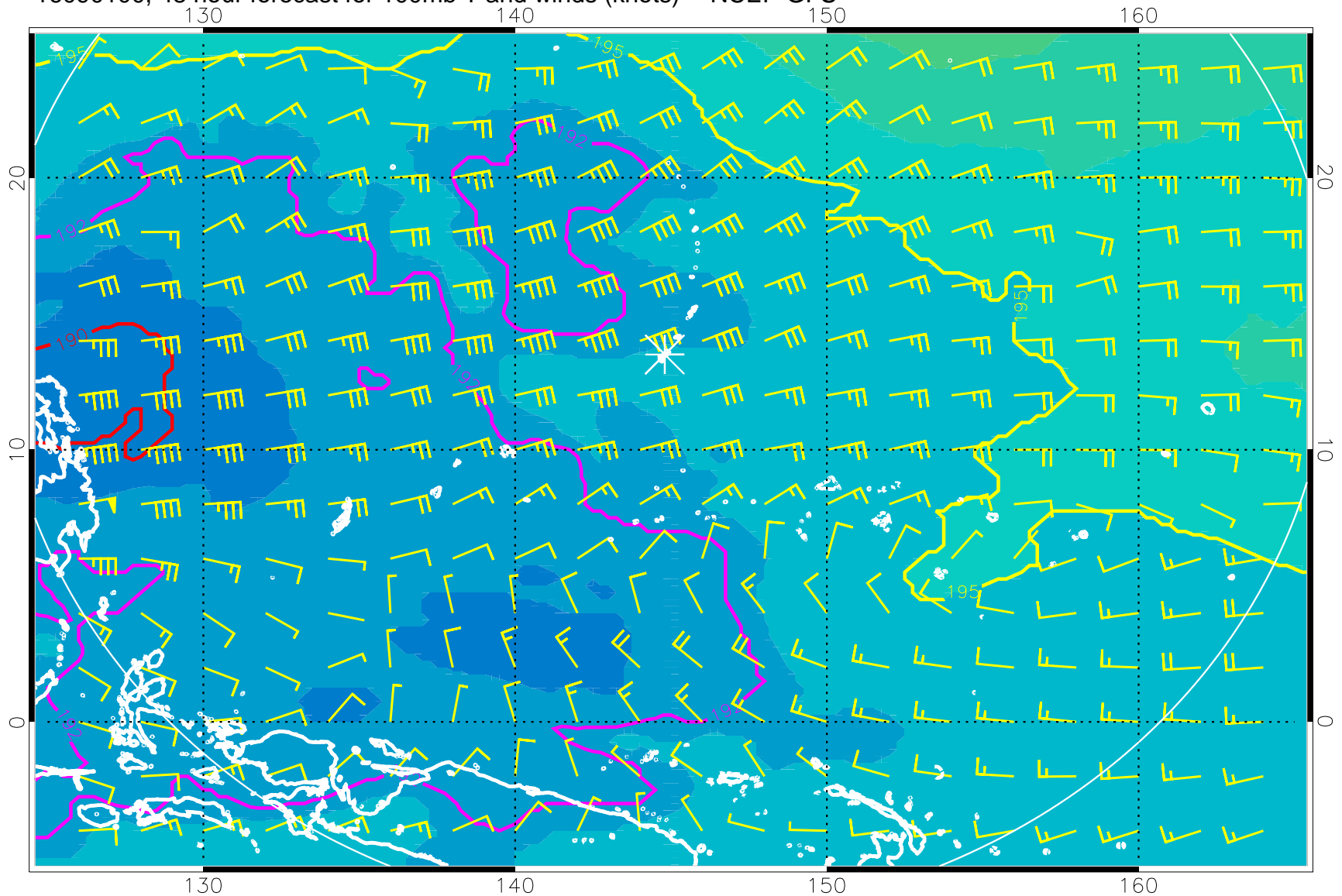
16090100, 48 hour forecast for 100mb T and winds (knots) -- NCEP GFS
