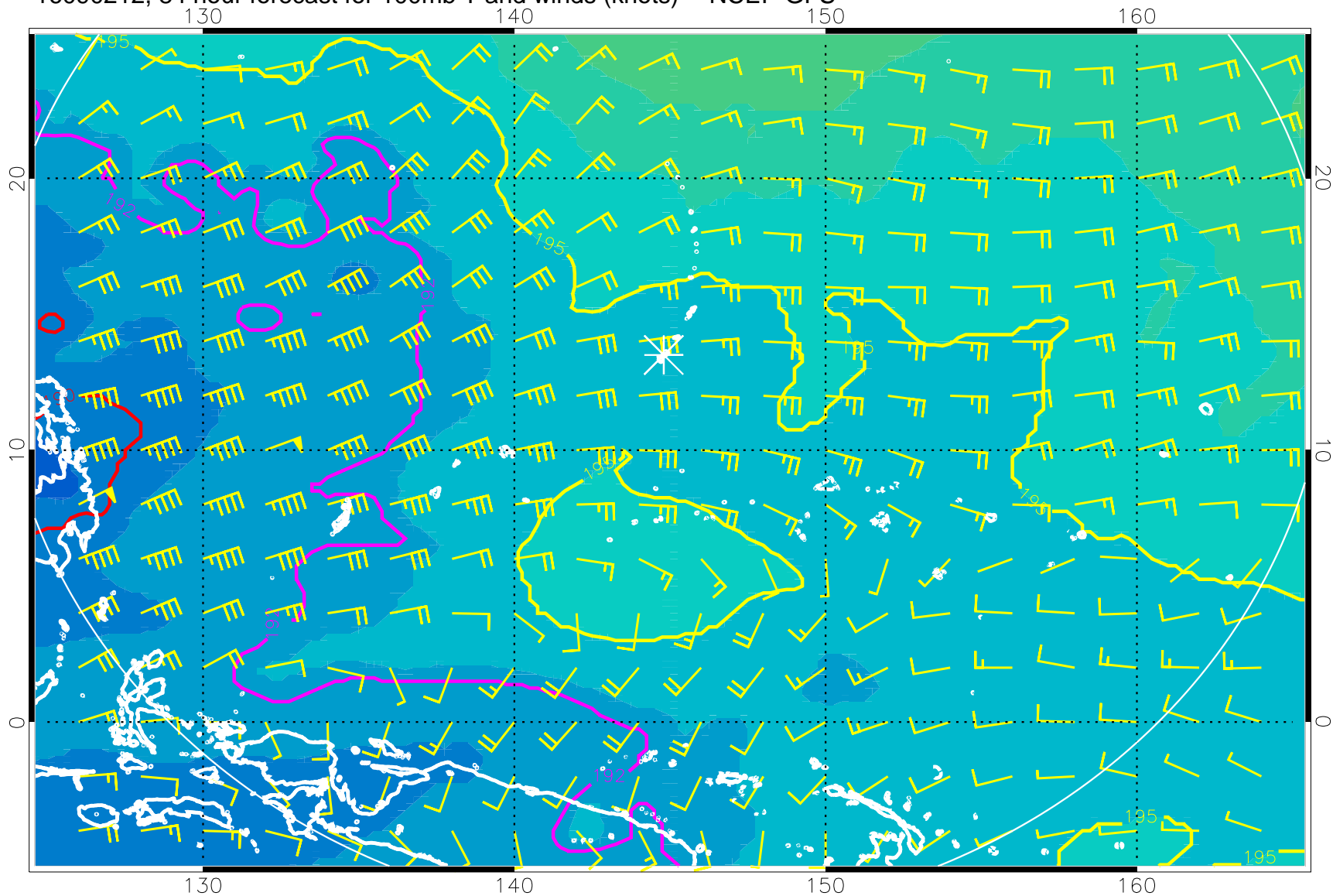
16090212, 84 hour forecast for 100mb T and winds (knots) -- NCEP GFS
