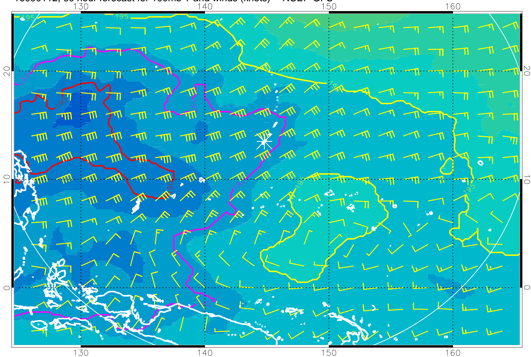
16090112, 60 hour forecast for 100mb T and winds (knots) -- NCEP GFS
