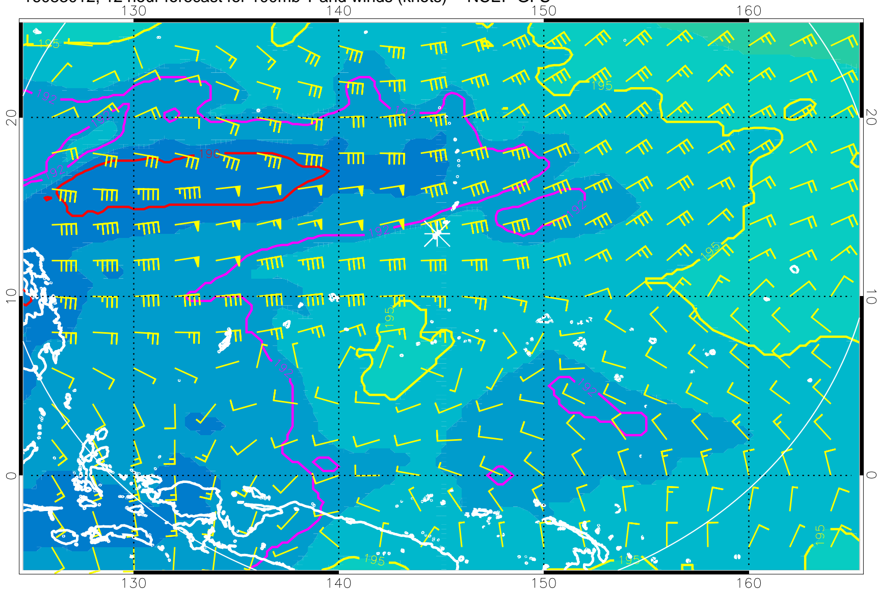
16083012, 12 hour forecast for 100mb T and winds (knots) -- NCEP GFS
