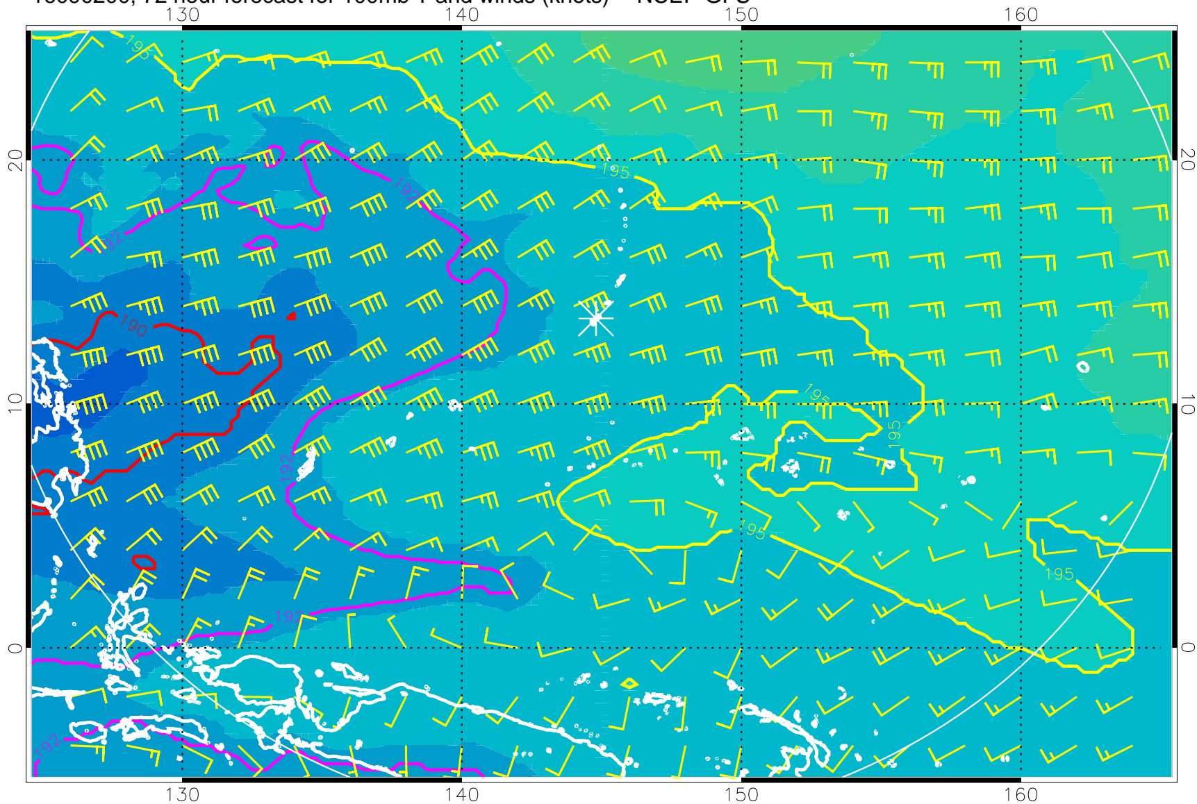
16090200, 72 hour forecast for 100mb T and winds (knots) -- NCEP GFS
