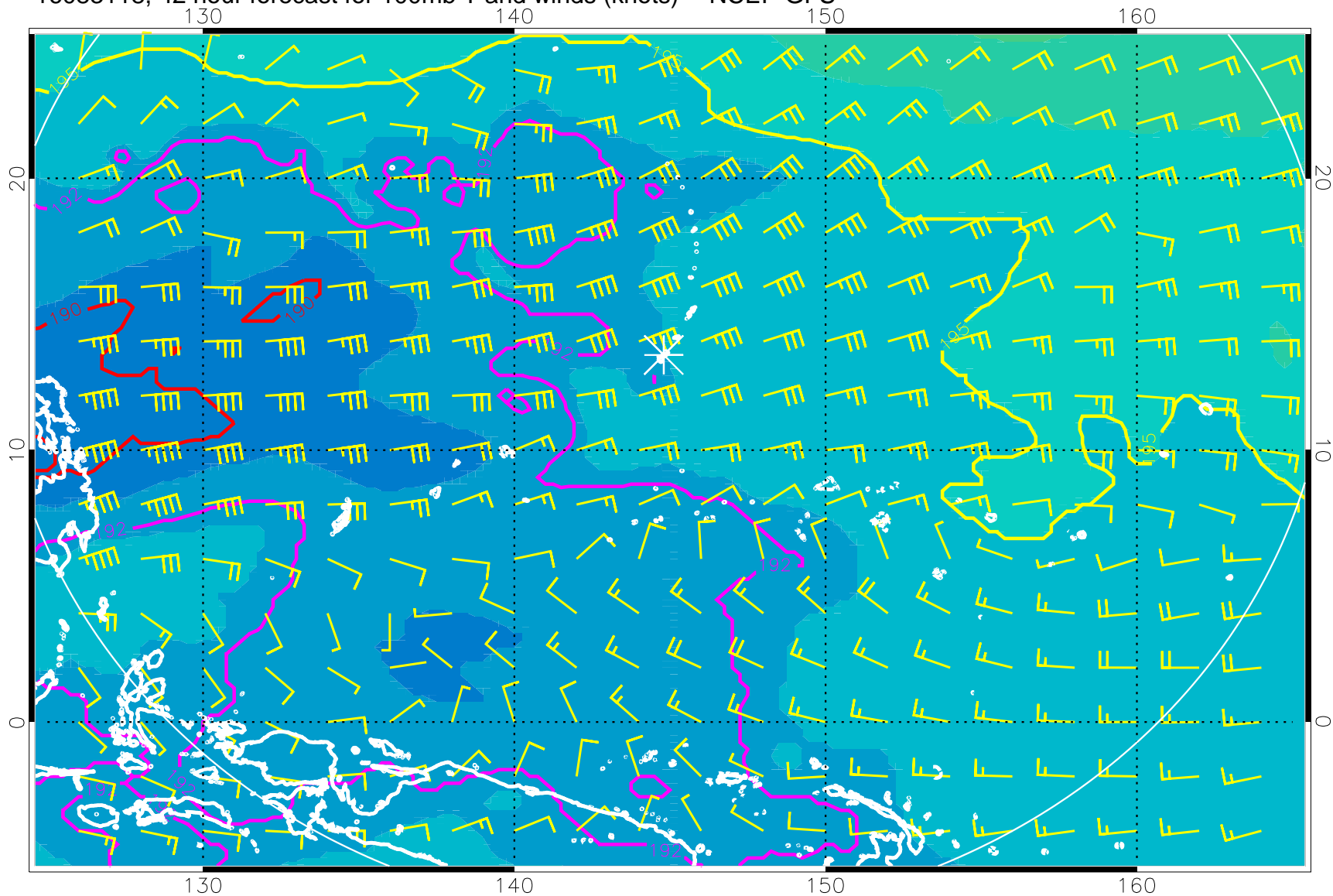
16083118, 42 hour forecast for 100mb T and winds (knots) -- NCEP GFS
