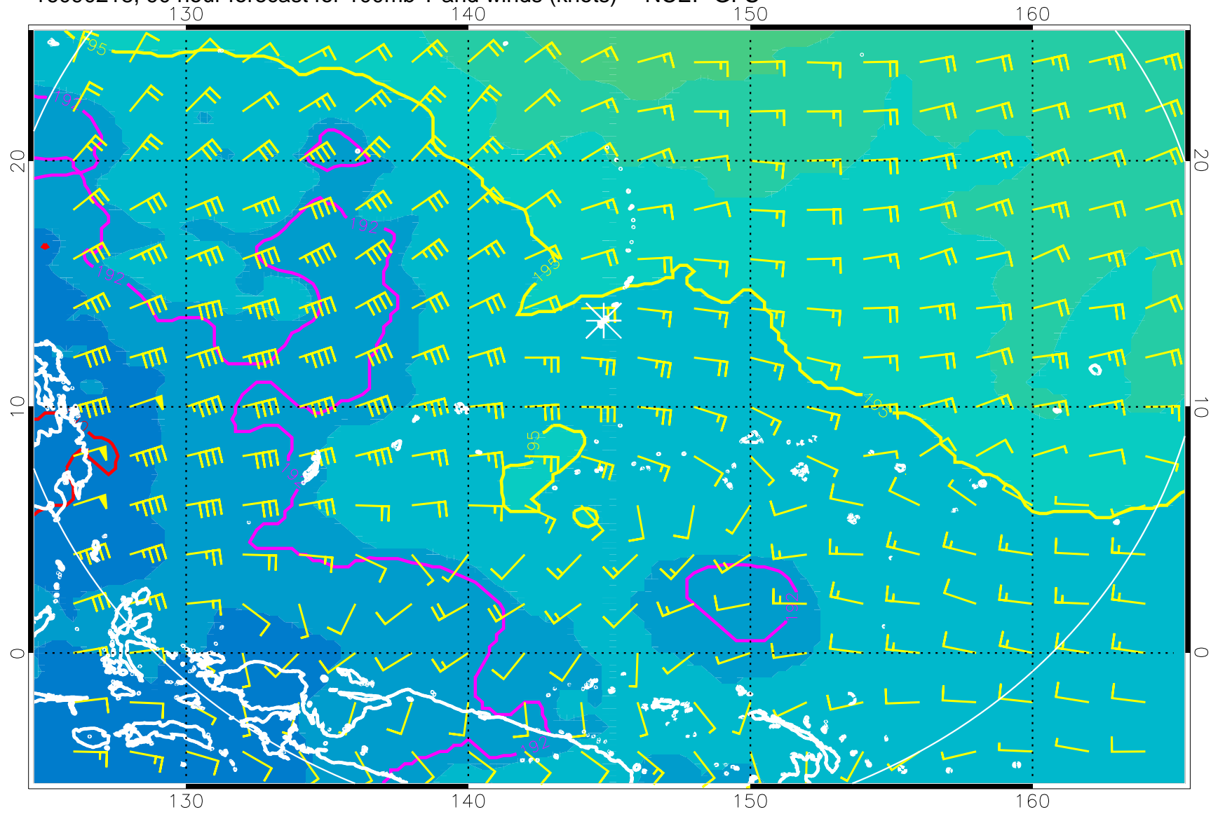
16090218, 90 hour forecast for 100mb T and winds (knots) -- NCEP GFS
