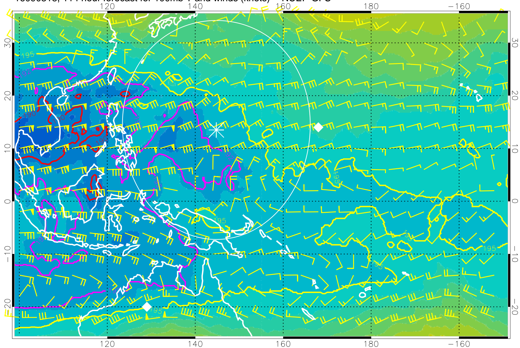
16090318, 114 hour forecast for 100mb T and winds (knots) -- NCEP GFS
